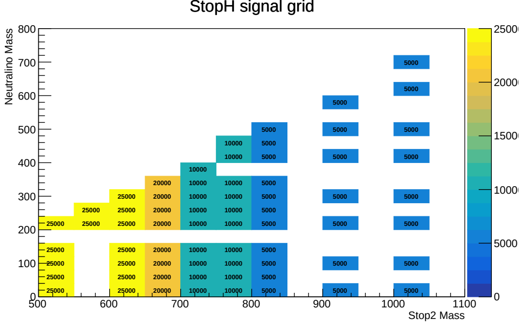
Figure 4.7: Number of events generated for each simplified signal model in the \tilde{t}_2 - \tilde{\chi}_1^0 mass plane with a 100% BR of \tilde{t}_2 \rightarrow \tilde{t}_1 + h considered for the optimisation and interpretation of the analysis.
