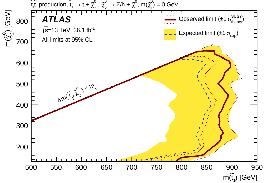
Figure 7.2: Exclusion limits at 95% CL from the analysis of 36.1 fb -1 of 13 TeV pp collision data on the masses of the \tilde{t}_1 and \tilde{\chi}_2^0 .
