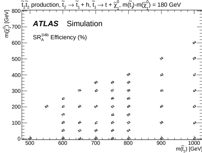
Figure A.1: Selection efficiency, defined as the ratio between the reconstructed events by the ATLAS detector and the total expected events by MonteCarlo simulations in events of the \tilde{t}_2 - \tilde{\chi}_1^0 mass models passing SR_A^{1\ell 4b} selections.
