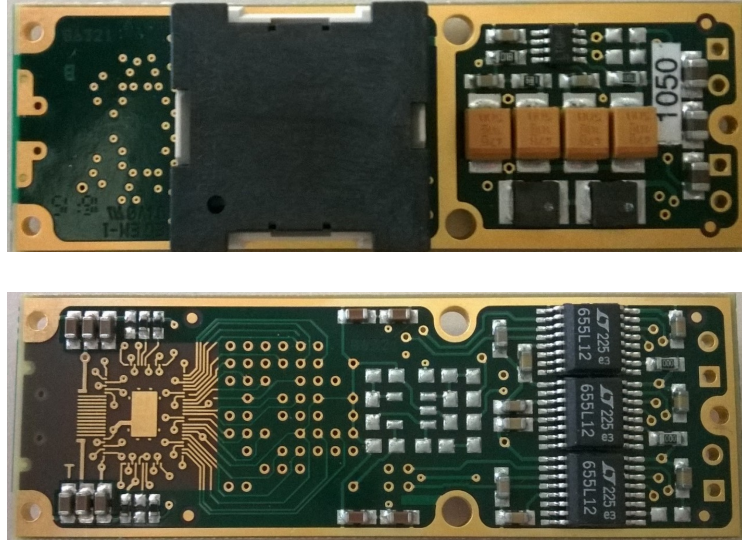
Figure 2.17: Front (top) and back (bottom) of the PCB which is base for the IBLBOC RX-plugin. The 10×10 SNAP12 connector is covered by a black cap. The gold-plated area on the left-bottom will host the DRX-12 II ASIC.
