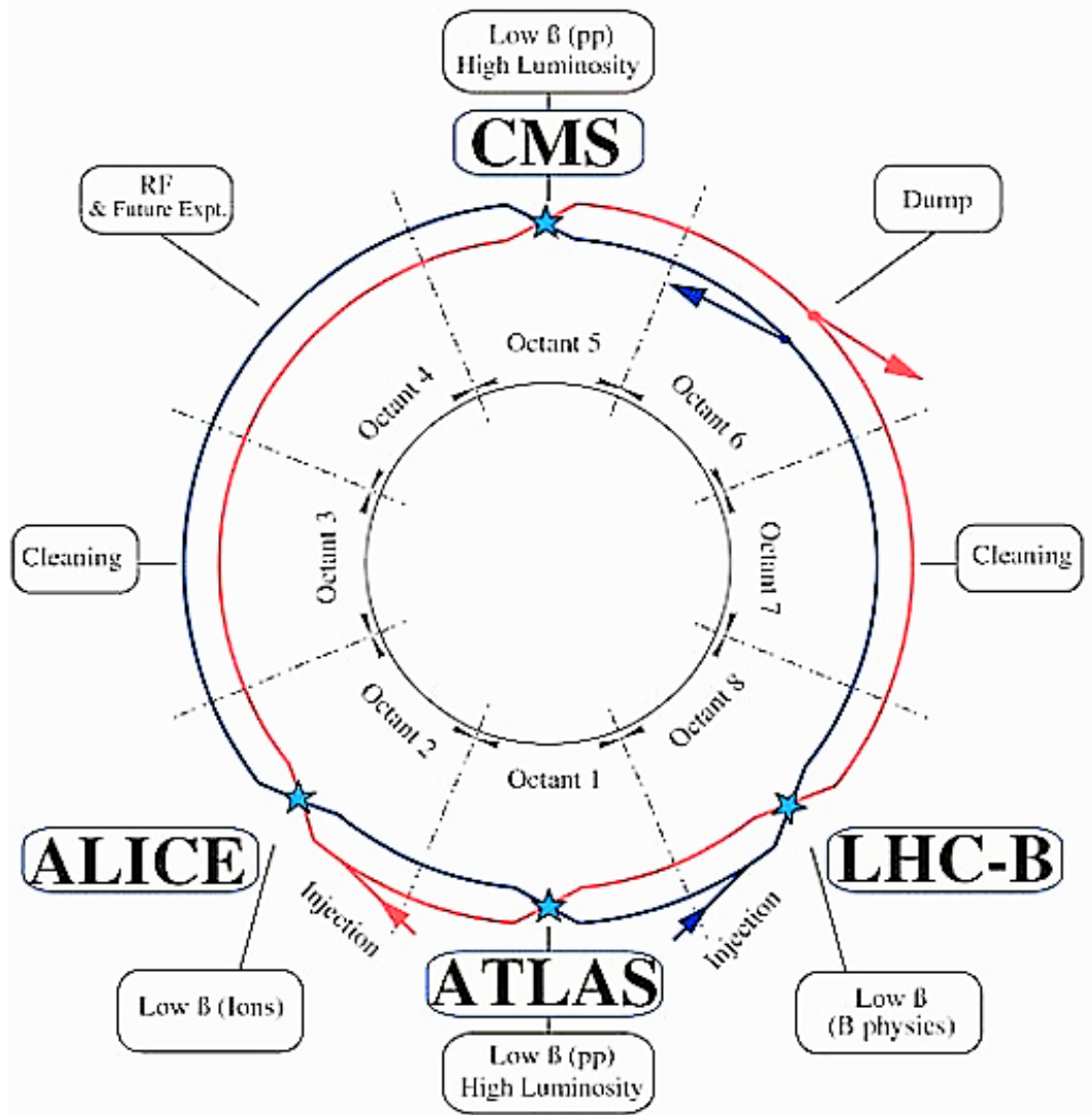
Figure 1.3: Layout of the LHC, focusing on the position of the four main experiments with respect to the interaction points. Radio-frequency cavities and utility insertions are present in octants not covered by experimental setups.
