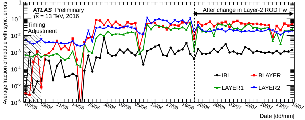
Figure 2.23: The average fraction of pixel and IBL modules with synchronization errors per event in 2016 runs. Each point shows the average fraction in a given run. The synchronization error signals a discrepancy between the level-1 trigger or bunch crossing identifiers recorded in the front-end chips and those stored in the central acquisition system. Different readout windows were used for Pixel and IBL in the first 5 runs due to timing adjustments. Runs until the middle of May were characterized by a low number of interactions per bunch crossing ( < 25 ) and colliding bunches ( < 1200 ). The effect of the subsequent increase in the number of interactions per bunch crossing and colliding bunches in the machine (up to approximately 32 and 2100 respectively) is visible until the end of June, when a change in the Layer-2 off-detector firmware (ROD Fw) was adopted, leading to a factor 10 decrease in the synchronization error rate. Data used in this plot have been collected by a mixture of triggers used in the monitoring stream.
