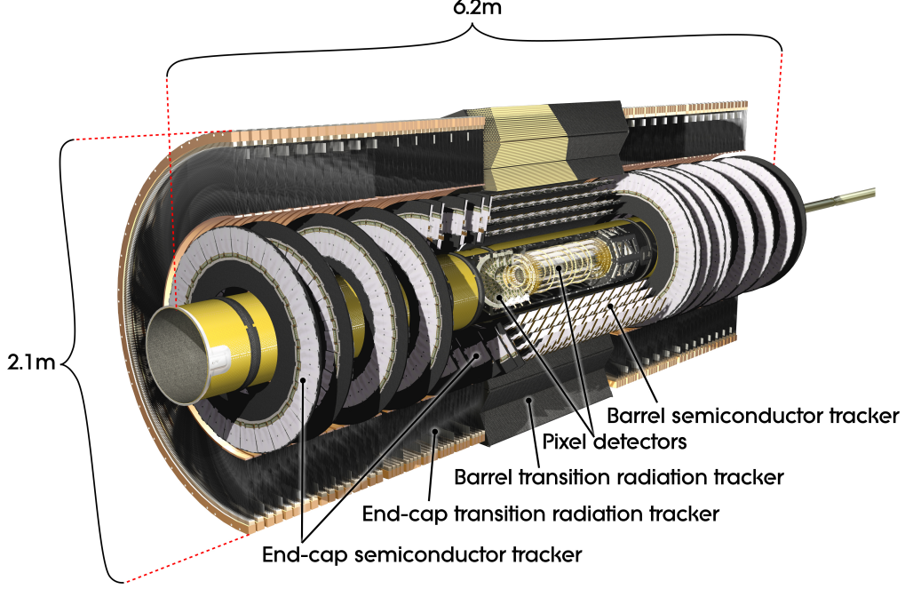
Figure 1.8: The Inner Detector of the ATLAS experiment, composed by the Pixel Detector Layers (IBL, B-Layer, Layer-1, Layer-2) and the Trackers (Semi Conductor Tracker, Transition Radiation Tracker).
