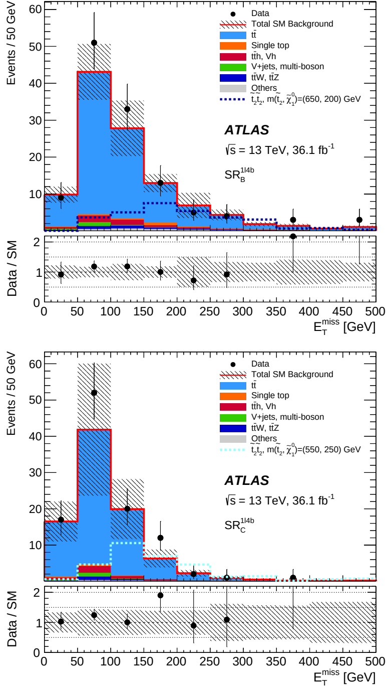
Figure 6.2: Distribution of E_T^{\text{miss}} for events passing all the signal candidate selection requirements, except that on E_T^{\text{miss}} , for the signal regions SR_B (top) and SR_C (bottom) after the background fit described in Sec. 5.4. The contribution from all SM backgrounds are shown; the bands represent the total uncertainty. The expected distributions for signal models with (m_{\tilde{t}_2}, m_{\tilde{\chi}_1^0}) = (650, 200) \text{ GeV} and (m_{\tilde{t}_2}, m_{\tilde{\chi}_1^0}) = (550, 250) \text{ GeV} are also shown as dashed lines. The last bin in each figure contains the overflow. The lower panels show the ratio of the observed data to the total SM background prediction, with the bands representing the total uncertainty in the background prediction.
