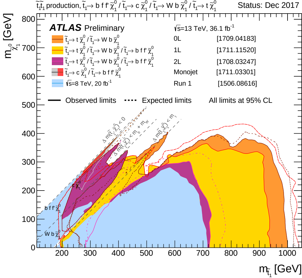
Figure 7.3: Summary of the dedicated ATLAS searches for top squark (stop) pair production based on 3.2 to 36 \text{fb}^{-1} of pp collision data taken at \sqrt{s} = 13 TeV. Exclusion limits at 95% CL are shown in the \tilde{t}_1 - \tilde{\chi}_1^0 mass plane. The dashed and solid lines show the expected and observed limits, respectively, including all uncertainties except the theoretical signal cross section uncertainty (PDF and scale). Four decay modes are considered separately with 100% BR: \tilde{t}_1 \rightarrow t + \tilde{\chi}_1^0 , \tilde{t}_1 \rightarrow W + b + \tilde{\chi}_1^0 (3-body decay allowed for m_{\tilde{t}_1} < m_t + m_{\tilde{\chi}_1^0} ), \tilde{t}_1 \rightarrow c + \tilde{\chi}_1^0 and \tilde{t}_1 \rightarrow f + f' + \tilde{\chi}_1^0 (4-body decay), with the latter two decay modes are superimposed.
