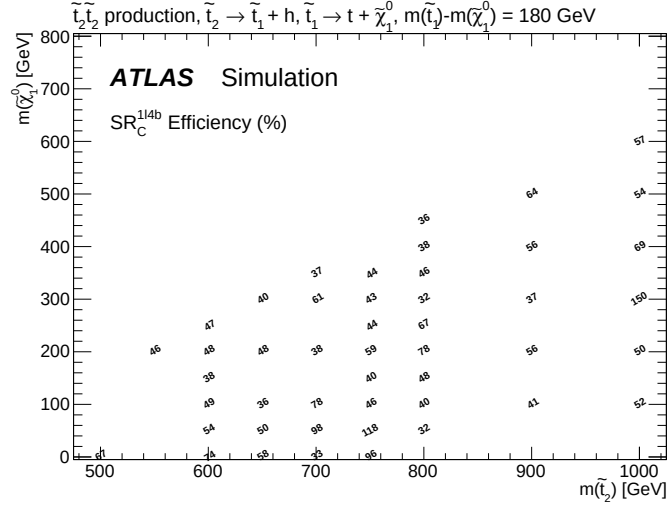
Figure A.3: Selection efficiency, defined as the ratio between the reconstructed events by the ATLAS detector and the total expected events by MonteCarlo simulations in events of the \tilde{t}_2 - \tilde{\chi}_1^0 mass models passing SR_C^{1\ell 4b} selections.
