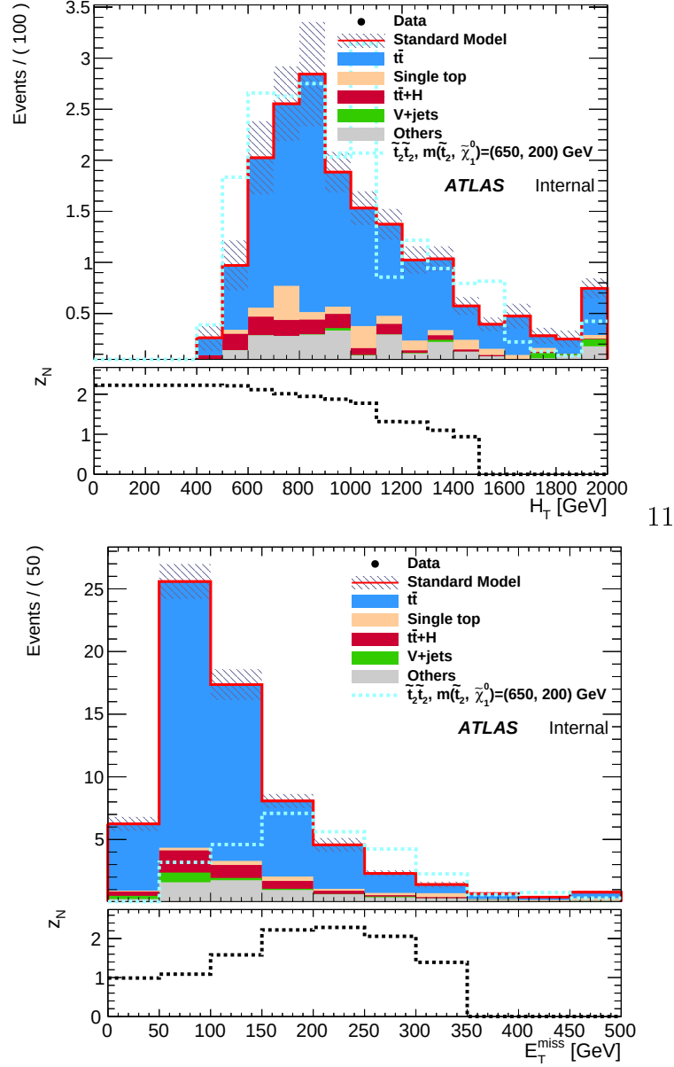
Figure 5.7: Distribution of the scalar sum of jet momenta H_T (top) and E_T^{miss} (bottom) for events lying in SR_C^{1\ell 4b} . The contribution from all SM backgrounds are shown; the bands represent the total uncertainty. The expected distributions for the signal model with (m_{\tilde{t}_2}, m_{\tilde{\chi}_1^0}) = (650, 200) GeV is also shown as a dashed line. The last bin in each figure contains the overflow. The lower panels show the significance of the signal model to the total SM background prediction.
