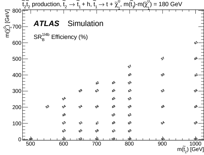
Figure A.2: Selection efficiency, defined as the ratio between the reconstructed events by the ATLAS detector and the total expected events by MonteCarlo simulations in events of the \tilde{t}_2 - \tilde{\chi}_1^0 mass models passing SR_B^{1\ell 4b} selections.
