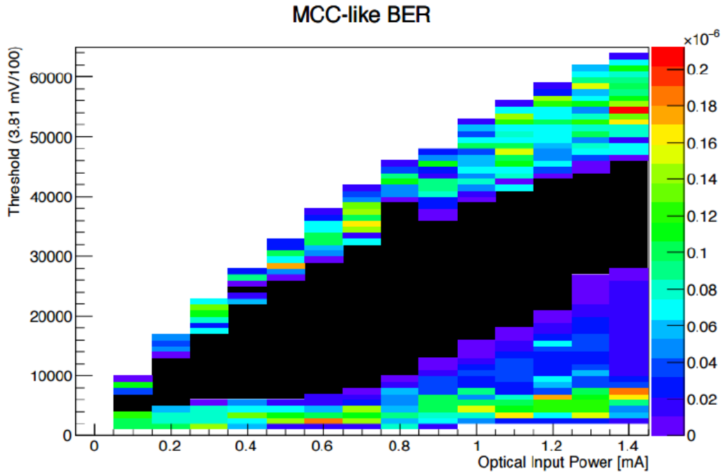
Figure 2.21: Typical test result of an RX-plugin Bit Error Rate Test. Different colors indicates different fractions of bit-error rate in the readback data. At least a subset of the V_{thres} - I_{input} region is expected to be stable and not show any transmission error after 10^{12} bit transmissions, here shown in black. The white region is out of specifications for this transmission and has not been tested.
