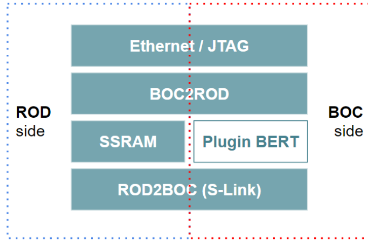
Figure 2.11: Block diagram of the testing procedures operated at CERN on the IBL data taking boards for the Layer-2 upgrade in 2015. The tests have been executed serially starting from the topmost, except for the SSRAM test and the Plugin BERT, which have been executed in parallel on the IBLROD and IBLBOC, respectively.
