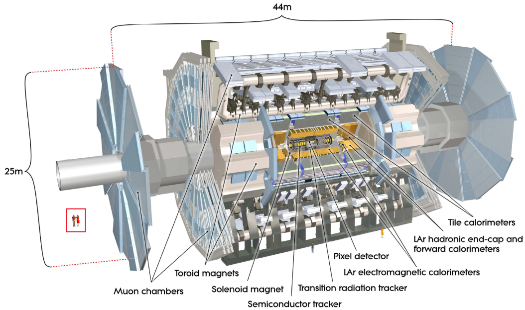
Figure 1.6: View of the ATLAS detector. The system is built with cylindrical symmetry with the beam pipe as the axis. From the innermost (closer to the beam pipe) to the outermost, all the subdetectors of ATLAS are shown. It is possible to compare the size of the ATLAS experiment with the humans in the red box.
