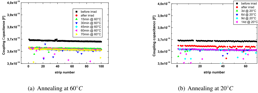
Figure 6.49: Annealing of coupling capacitances after proton irradiation: Since no changes in time are observed, the changes in the coupling capacitance values are coming from the fluence changing the properties of the dielectric layers. The middle values on the right hand side are caused by bad electrical contact and dust on the tip of the needle used for the measurement [Fur05].
