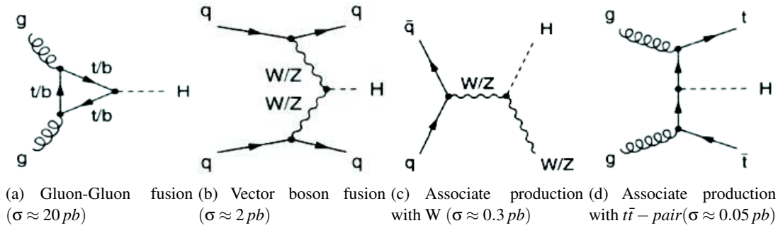
Figure 1.2: Higgs production at LHC: The most likely channels for the Higgs productions in the standard model are the gluon-gluon fusions in 1.2(a). The vector boson fusion and the associated production mechanisms have much lower cross sections. The cross sections are estimated for an expected Higgs mass of 120 \text{ GeV} and a top mass of 175 \text{ GeV} .
