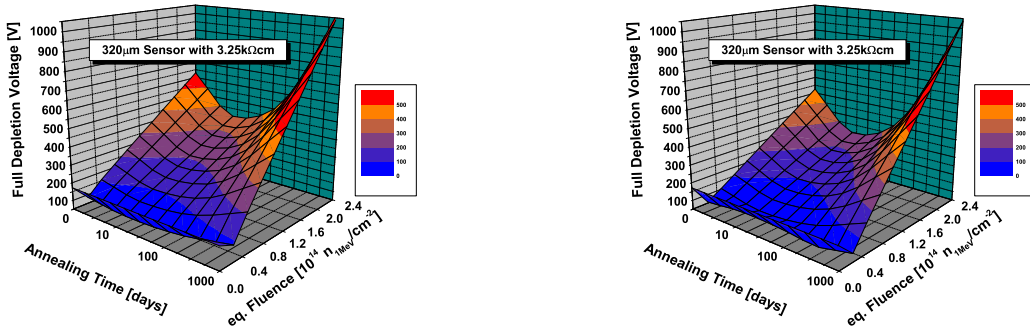
(a) Full depletion voltage of IB1 sensors with literature values [Mol99]
