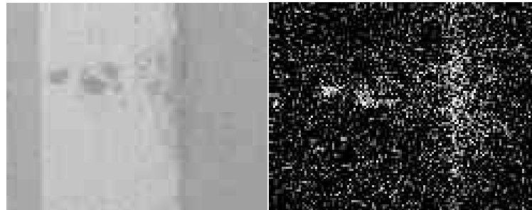
Figure 5.26: Potassium distribution on guard ring of STM sensor: The plot on the right hand side shows the potassium distribution within the guard ring region on the plot on the left hand side. The potassium is not only found at the edge regions of the aluminium structures but also in the middle without connection to the edge regions.
