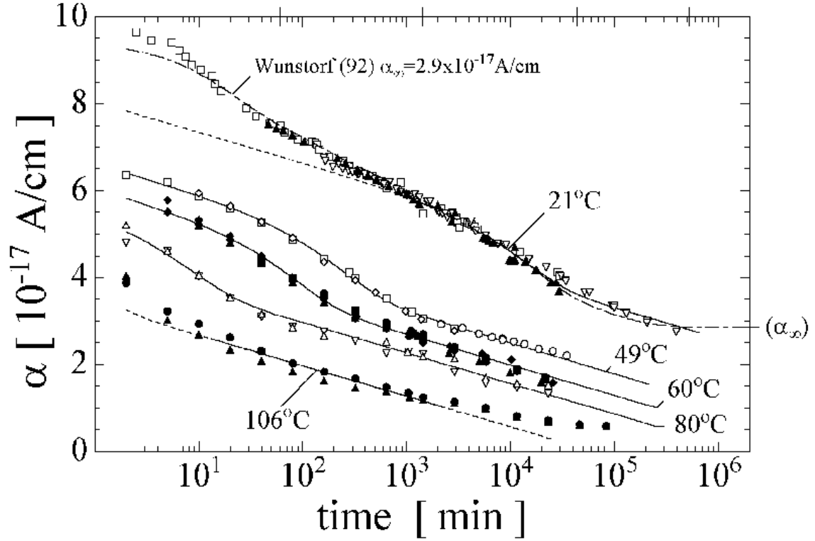
Figure 3.5: Current annealing of irradiated silicon: The current related damage rate anneals with time. The saturation value \alpha_{\infty} = 2.9 \cdot 10^{-17} \text{ A/cm} is reached for 21^{\circ}\text{C} after orders of 10^5 \text{ min} . For higher temperatures \alpha can reach even lower values [Mol99].
