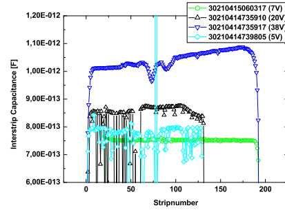
(b) Interstrip capacitances after proton irradiation with inner barrel fluence and standard annealing of 80min and 60°C
