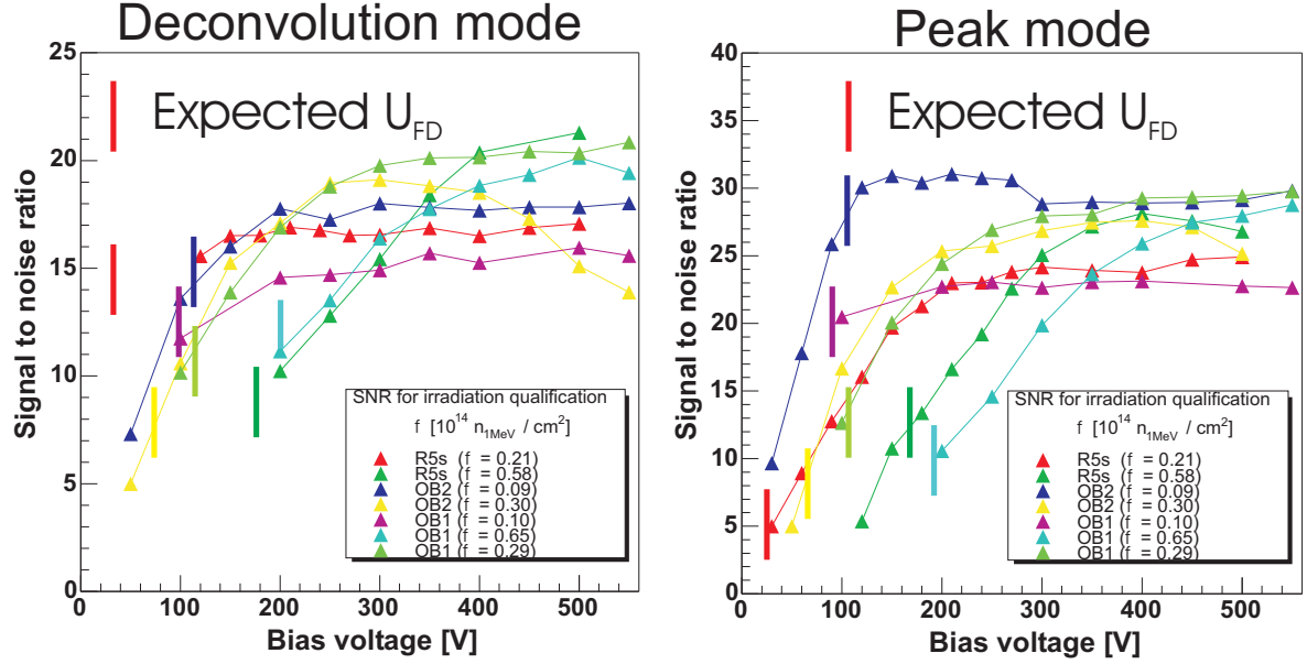
Figure 6.60: Signal to noise ratio of CMS detector modules with final STM pre-series sensors after proton irradiation: The signal to noise ratios are above ten for all detector modules in deconvolution mode (left hand side) and peak mode (right hand side) but not all of them are irradiated with the full expected design fluence. For some sensors a higher overdepletion than 50% is necessary to reach the saturation of maximum SNR.
