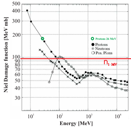
Figure 6.1: NIEL damage functions for positive pions, protons, and neutrons: The damage functions are decreasing with increasing energy. The damage function of neutrons with an energy of 1\text{ MeV} and a damage function value of 95\text{ MeVmb} is used as reference for scaling of particle fluences. Damage function ratios of other particles and energies to the reference value is called "hardness factor" (see Equation 3.4). For protons with an energy of 26\text{ MeV} used in the Kompakt-Zyklotron in Karlsruhe the hardness factor is 1.85. The averaged hardness factor of the neutron spectrum used for the spectrum of neutrons in Louvain-la-Neuve is 1.95.
