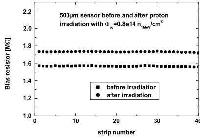
(a) The bias resistors have an average increase of 0.15 M\Omega for fluences of 0.8 \cdot 10^{14} n_{1MeV}/cm^2 and after standard annealing procedure [Fur03].
