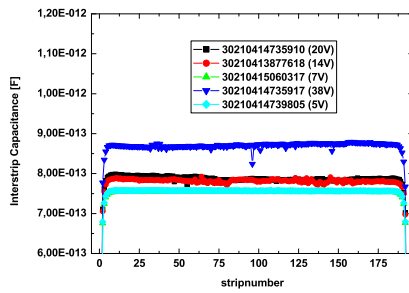
(a) Interstrip capacitances before irradiation
