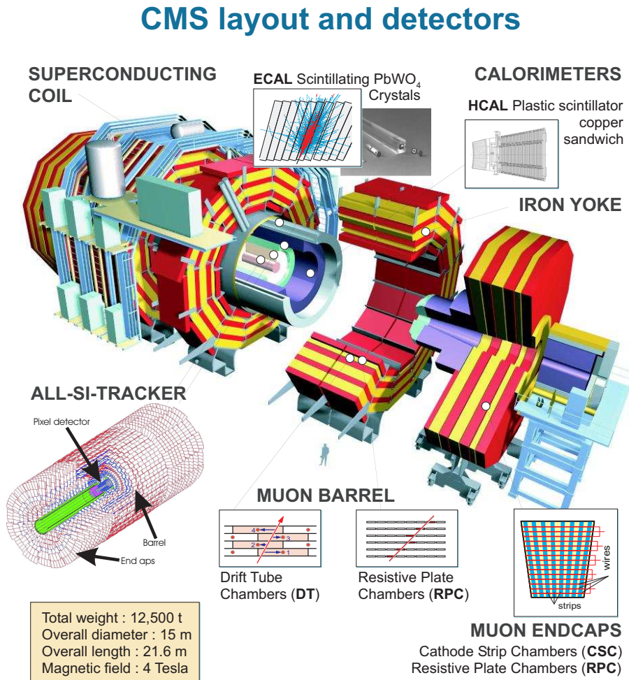
Figure 1.6: The CMS detector: The CMS detector consists of a silicon tracker, a electromagnetic, a hadronic calorimeter, and muon barrels inserted in the iron yoke of the magnet. All subdetectors are subdivided in barrels and endcaps.
