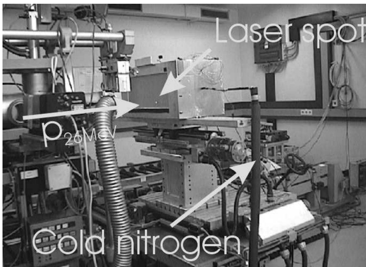
Figure 6.2: The Kompakt-Zyklotron in Karlsruhe: At the Kompakt Zyklotron at the Forschungszentrum in Karlsruhe protons with an energy of 18 MeV up to 40 MeV are available for irradiation. The box supporting the structures to be irradiated can move in two directions. During irradiation, scans in front of the proton beam are performed. With a proton current of 2\mu\text{A} only 15 min are necessary to irradiate an area of 100\text{cm}^2 to a fluence of 1 \cdot 10^{14} n_{1\text{MeV}}/\text{cm}^2 . The box is flooded with cold nitrogen gas to keep the temperature during and after irradiation as cold as necessary to avoid local overheating or annealing effects. A red laser is used for aligning the scan areas.
