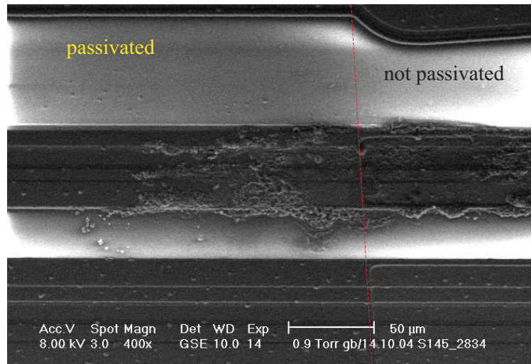
Figure 5.27: Picture of partially passivated bias ring on STM sensor: The picture shows a top view of a bias ring which is passivated on the left hand side and where the passivation layer is removed on the right hand side. The chemical reaction underneath the passivation layer is not connected with the chemical reaction in the non passivated area.
