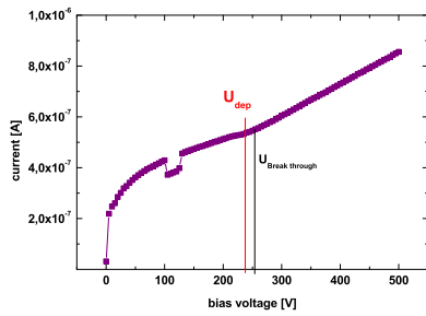
(a) Total leakage current before irradiation
