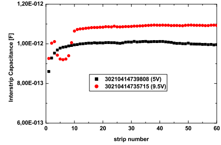
(b) Interstrip capacitances after second proton irradiation (18 years service life at LHC)
