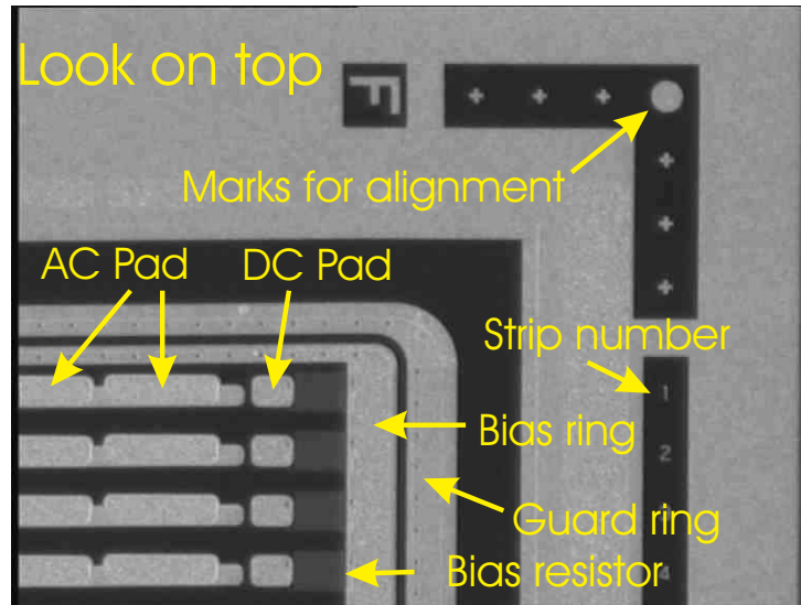
Figure 4.1: Principle design of a CMS sensor: The CMS sensors are single-sided sensors with p^+ strip implants on n -bulk, with poly crystalline bias resistors and AC coupling [Kra04][Har02]. The bias ring and the guard ring enclose the strip implants. Since the bias ring is connected to low potential the guard ring is floating. Both define the active volume of the sensor and they are responsible for the adjusting of the field configuration to the edges. The backside of the wafer has a heavily doped n^+ layer between the bulk and the aluminium layer which avoids a Shottky contact. The outer n^+ ring encloses the guard ring and avoids the flow of edge currents into the active inner area of the sensors. The ends of the aluminium strips are wider than the strip and are called AC pads. The p^+ implants are connected with aluminium vias to the bias resistors connecting the bias ring. The upper enlarged part of the vias which is used for contact is called DC pad. The metal strips have a 4\mu\text{m} larger width than the p^+ implants. This metal overhang shifts the breakthrough mechanism to high voltages (far beyond full depletion voltage) of the p - n junctions by moving the points of highest electric field density into the isolating layer.
