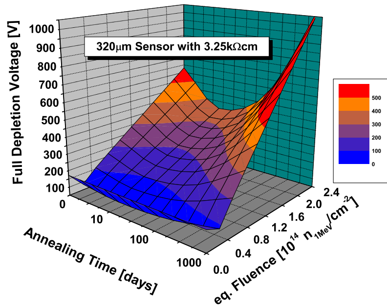
Figure 3.8: Full depletion voltage versus fluence and annealing time: The full depletion voltage of n -doped silicon first decreases with fluence and increases after type inversion. After type inversion the full depletion voltage decreases with annealing time (beneficial annealing) and increases afterwards (long-term reverse annealing).
