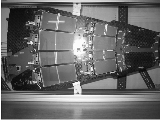
(a) Picture of a CMS endcap petal
