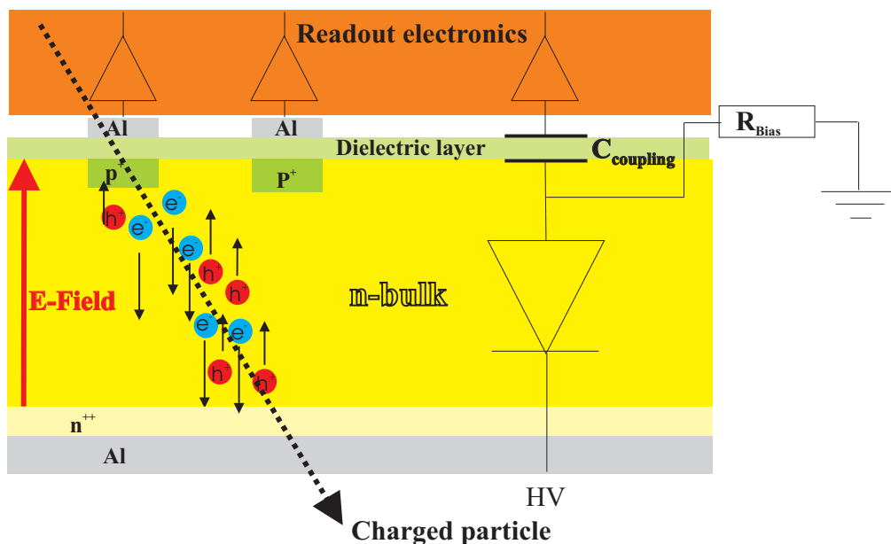
Figure 2.12: Schematics of a semiconductor sensor: The sensor is built of p - n -junctions which are fully depleted by an applied reverse bias voltage. Since charged particles traversing semiconductors produce electron-hole pairs, the applied electric field separates electrons and holes from each other and collects them at the electrodes. In single sided strip or pixel sensors one charge carrier type is collected while the other charge carrier type is drifting to the unstructured contact and gets lost. The dark current of the fully depleted p - n -junction is separated from the readout electronics by capacitances. These are realized by a small non conductive dielectric layer between the implants and the metal segmentations above. Bias resistors are necessary to apply a potential to the implants and to form a certain RC value with the coupling capacitance.
