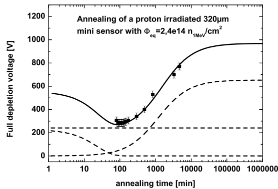
Figure 6.12: Beneficial and reverse annealing of full depletion voltage on HPK sensor: This plot shows the annealing at 60°C including reverse annealing. For annealing steps above 70min at each annealing step the sensor has been annealed at room temperature for 24h. This causes a drop of the full depletion voltage of 40V and the sensors full depletion voltage follows the valid parametrization of the Hamburg model. With this procedure the mystery of the 40V difference in figures 6.11(a) and 6.11(b) can be explained with either excited states of radiation damage or with appearance of further damage which decays at room temperature. This fact cannot be observed for the total capacitance.
