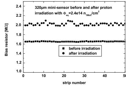
(b) The bias resistors have an average increase of 0.35 M\Omega for fluences up to 2.4 \cdot 10^{14} n_{1MeV}/cm^2 and after standard annealing procedure [Fur03].
