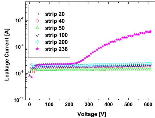
Figure 5.31: Single strip leakage current of a STM sensor under mechanical stress: The high total leakage current under mechanical stress is driven by high single strip leakage currents. The full depletion voltage of this sensor is around 200V and the kink of the current is observed 20 – 30V above full depletion voltage.
