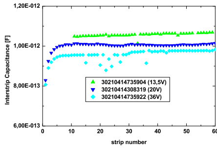
(c) Interstrip capacitances after second proton irradiation (10 years service life at LHC)
