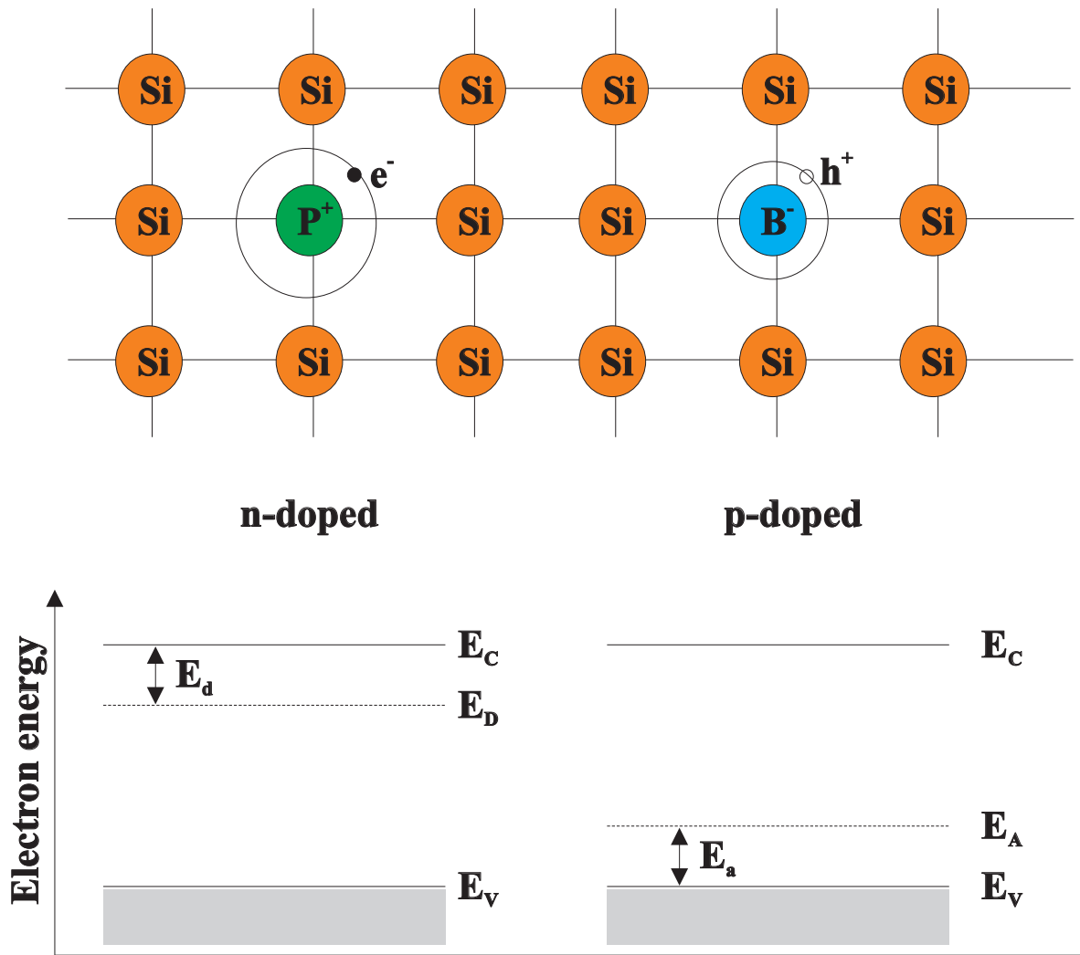
Figure 2.4: Energy levels of p- and n-doped silicon: For n-doping of silicon in most cases phosphorous is used and for p-doping boron, respectively. The fifth covalent electron of the phosphorous atom is an additional negative free charge. Boron has instead only three covalent electrons. The missing covalent electron to the corresponding silicon neighbor is a trap for a negative charge. The missing negative charge acts as a free positive charge in the silicon lattice. The concentrations of the doping atoms is in the order of impurities in the silicon crystal.
