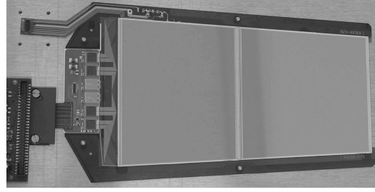
(b) Picture of a CMS petal detector module
