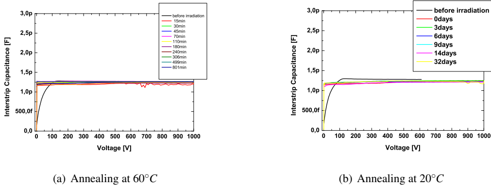
Figure 6.54: Annealing of interstrip capacitance of HPK sensors measured between DC pads: The interstrip capacitance does neither change with fluence (here proton irradiated to 2.4 \cdot 10^{14} \text{ n}_{1\text{MeV}}/\text{cm}^2 ) nor with annealing. The annealing of the capacitance of the strips to the backside contact (see Figure 6.10 on Page 96) does hardly influence the interstrip capacitance values.
