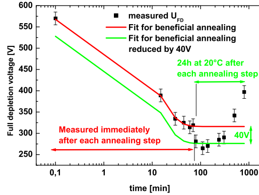
Figure 6.12: Beneficial and reverse annealing of full depletion voltage on HPK sensor: This plot shows the annealing at 60°C including reverse annealing. For annealing steps above 70min at each annealing step the sensor has been annealed at room temperature for 24h. This causes a drop of the full depletion voltage of 40V and the sensors full depletion voltage follows the valid parametrization of the Hamburg model. With this procedure the mystery of the 40V difference in figures 6.11(a) and 6.11(b) can be explained with either excited states of radiation damage or with appearance of further damage which decays at room temperature. This fact cannot be observed for the total capacitance.
