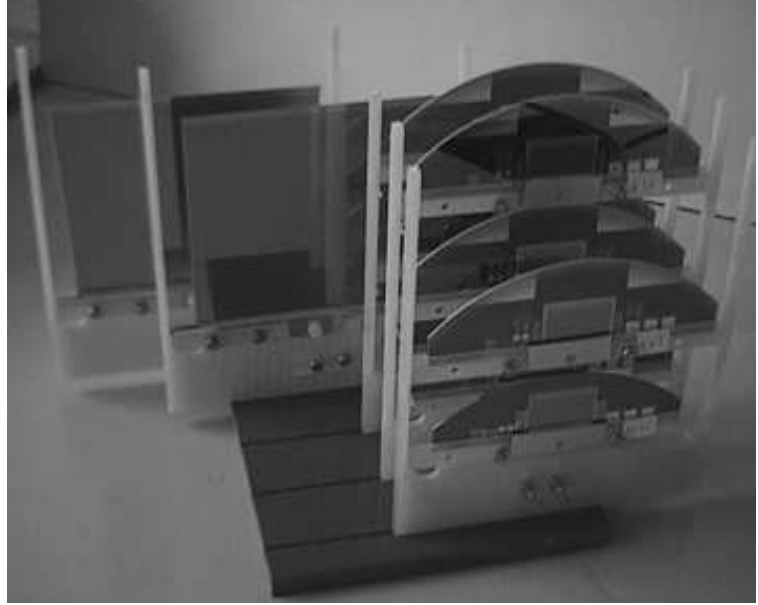
Figure 6.3: Picture of CMS sensors in stacks ready for irradiation: The sensors and test structures to be irradiated are stacked in frames of glass fiber or teflon. The clamps fixing the structures contain electrical contacts, which allow to apply a certain voltage to the structures.
