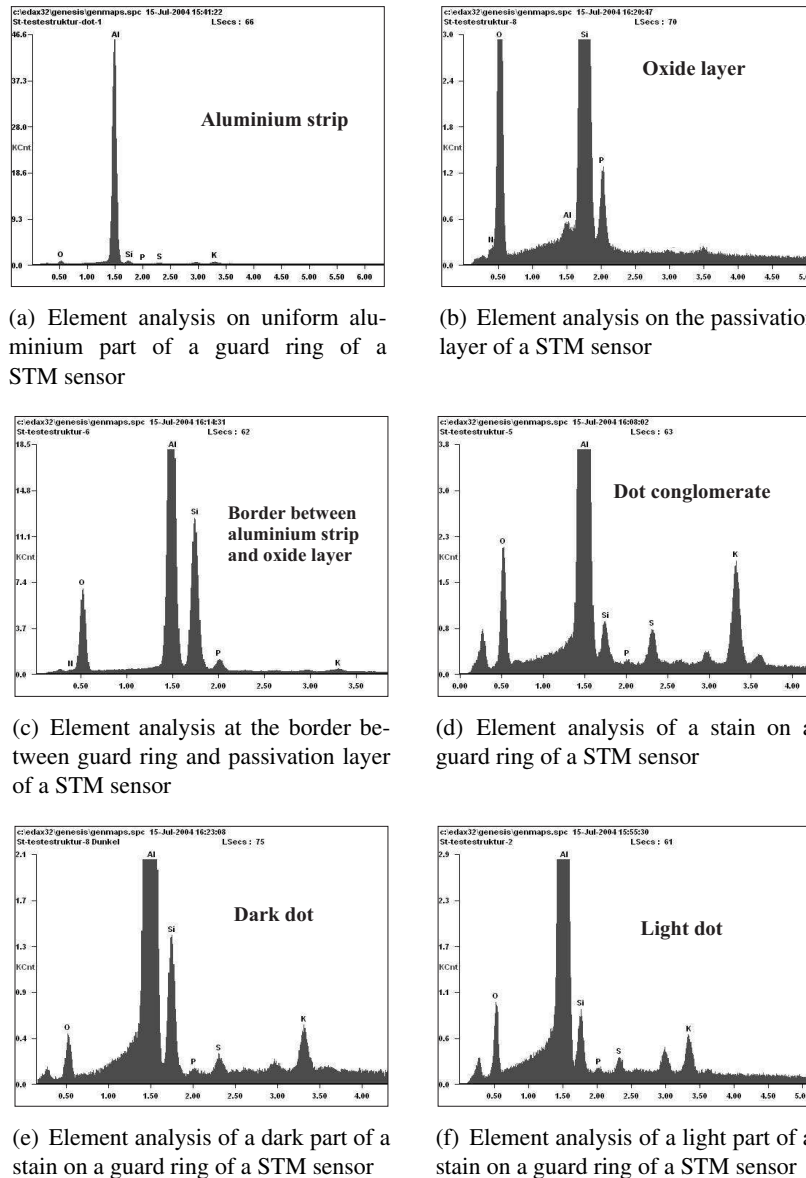
Figure 5.23: Element analysis on STM sensor with electron microscope: The graphs show electron counts versus photon energies for different STM sensor regions. The aluminium, the passivation layer far away from the stain, and the border between aluminium and passivation layer (5.23(a) - 5.23(c)) show the expected distribution of Al, Si, and O. P is found everywhere on the sensor with higher concentrations in the passivation layer. The entire dot conglomerate (5.23(d)) of Figure 5.22, the dark (5.23(e)) and the light parts (5.23(f)) of this stain, contain high additional concentrations of potassium and sulphur.
