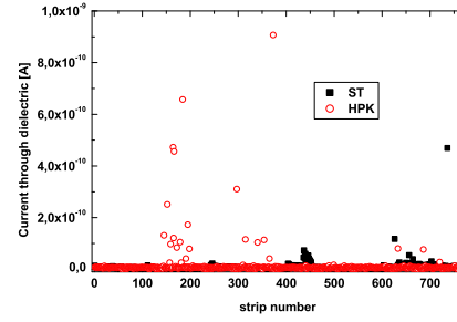
(b) The current through the dielectric layer of the coupling capacitances is below the limit of 1\text{ nA} .
