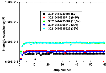
(a) Interstrip capacitances before second irradiation
