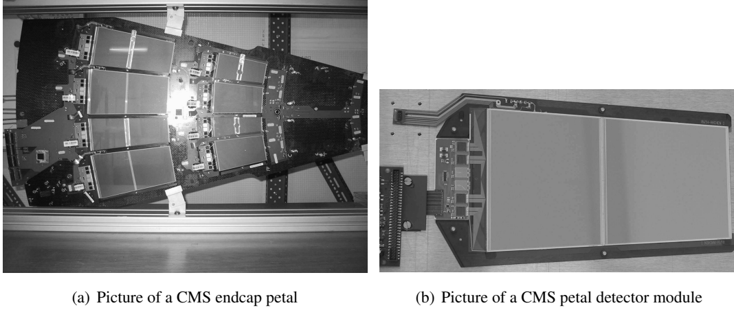
Figure 1.8: Pictures of a CMS petal and a CMS wedge shaped detector module
