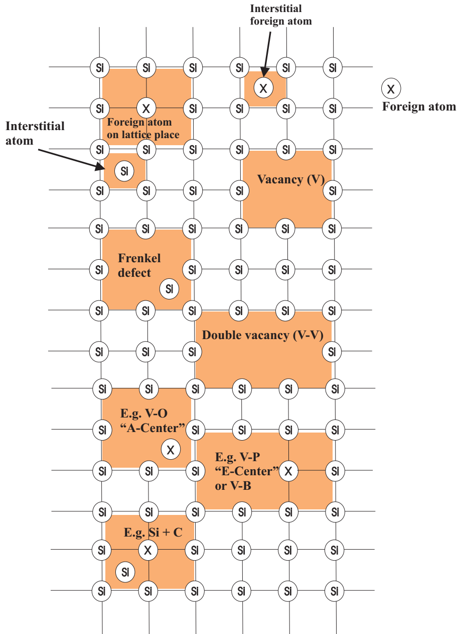
Figure 3.1: Examples of different lattice damage in silicon: The variety of damage in the silicon lattice is large and therefore only a few examples are represented. Important damage caused by radiation are vacancies "V" and oxygen containing damage structures like the "A-Center". All of this damage can also be clustered in large defect centers.
