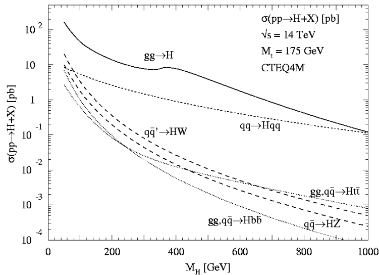
Figure 1.3: Production cross sections of the Higgs boson in the standard model: The most likely channels for the Higgs production are gluon-gluon fusions. All cross sections decrease with increasing mass of the Higgs boson [SSZ00].
