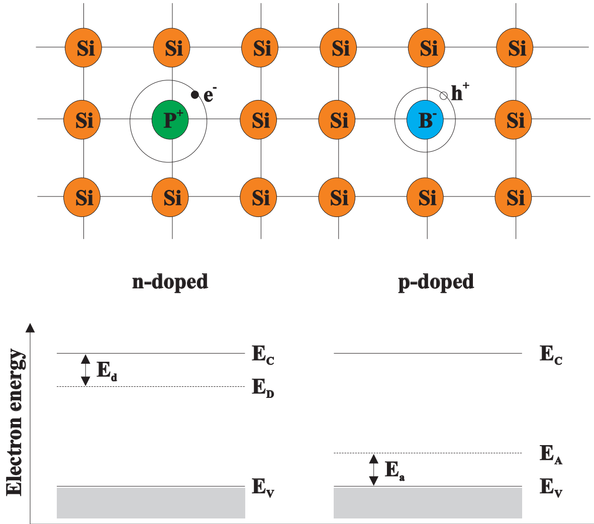
Figure 2.4: Energy levels of p- and n-doped silicon: For n -doping of silicon in most cases phosphorous is used and for p -doping boron, respectively. The fifth covalent electron of the phosphorous atom is an additional negative free charge. Boron has instead only three covalent electrons. The missing covalent electron to the corresponding silicon neighbor is a trap for a negative charge. The missing negative charge acts as a free positive charge in the silicon lattice. The concentrations of the doping atoms is in the order of impurities in the silicon crystal.
