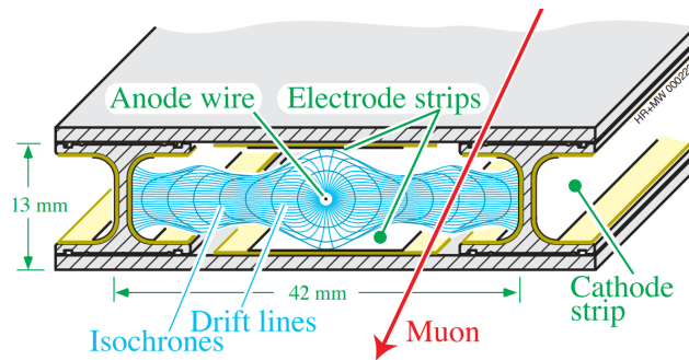
Figure 3.9 – Sketch of the drift cells highlighting the electric field lines converging towards the anode wire [11].
