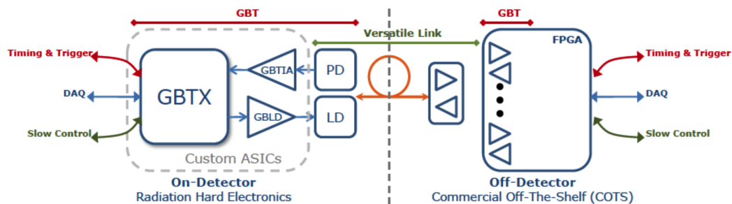
Figure 5.4 – Architecture of the radiation hard optical link setup integrating the GBT and Versatile Link projects [30].
