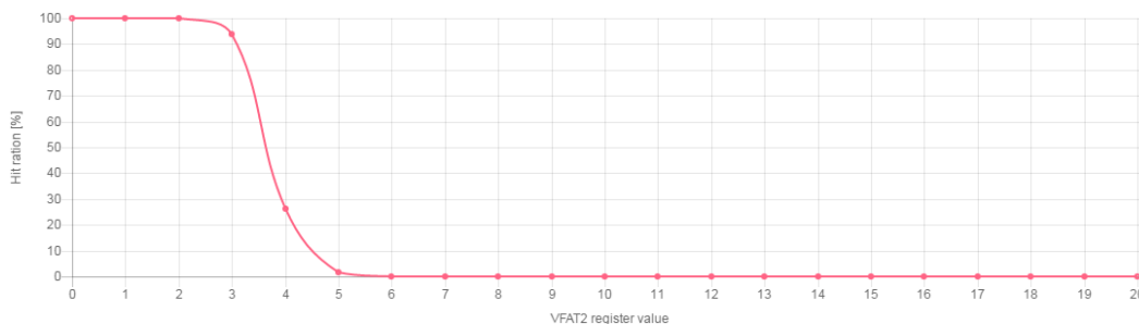
Figure 6.11 – Illustration of a threshold scan representing the hit percentage as a function of the threshold of the VFAT2.
