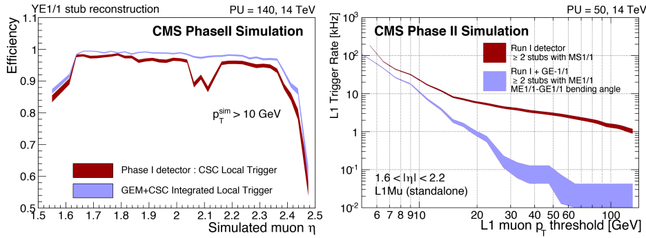
Figure 4.3 – Left: reconstruction efficiency of the integrated GEM-CSC trigger as a function of the simulated muon |\eta| , compared to the same for the Phase-I CSC-only algorithm. Right: level 1 muon trigger rates before and after the GE1/1 upgrade at a luminosity of 2 \times 10^{34} \text{ cm}^{-2} \text{ s}^{-1} . MS1/1 denotes the first endcap muon station level 1 trigger in both cases, i.e. with CSC-only or with the combination CSC and GEM trigger information [24].
