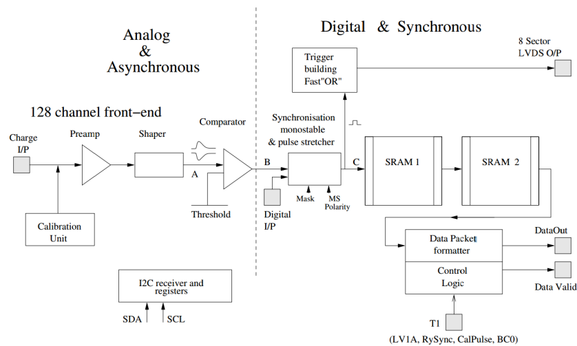
Figure 5.13 – Schematic diagram of the VFAT2 showing the analog front-end on the left and the digital control and readout system on the right [35].
