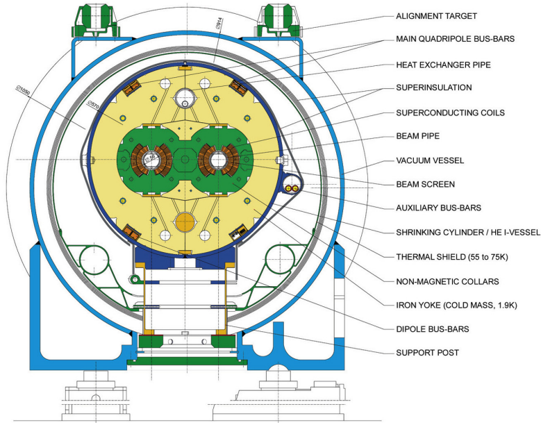
Figure 2.3 – Cross-section of a cryodipole of the LHC representing the two beam pipes equipped with superconducting NbTi coils surrounded by iron cold mass at 1.9 K [8].
