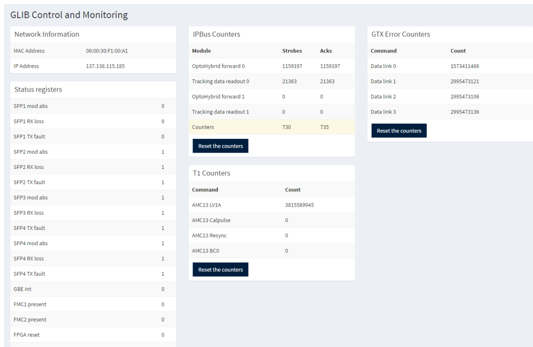
Figure 6.16 – Screenshots of the page used to control and monitor the GLIB.
