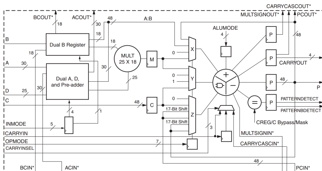
Figure 8.2 – Diagram of the DSP48E1 slices present in the Xilinx Virtex-6 family [55].
