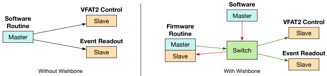
Figure 6.2 – Schematic illustration of the architecture of the system without Wishbone on the left and with Wishbone on the right.
