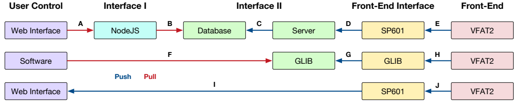
Figure 11.9 – Nodes of the DAQ systems and the interactions they have in order to transmit the data from the front-end electronics to the user control. Blue arrows indicate that data is pushed to the next node, and red arrows that the data is pulled from the node.
