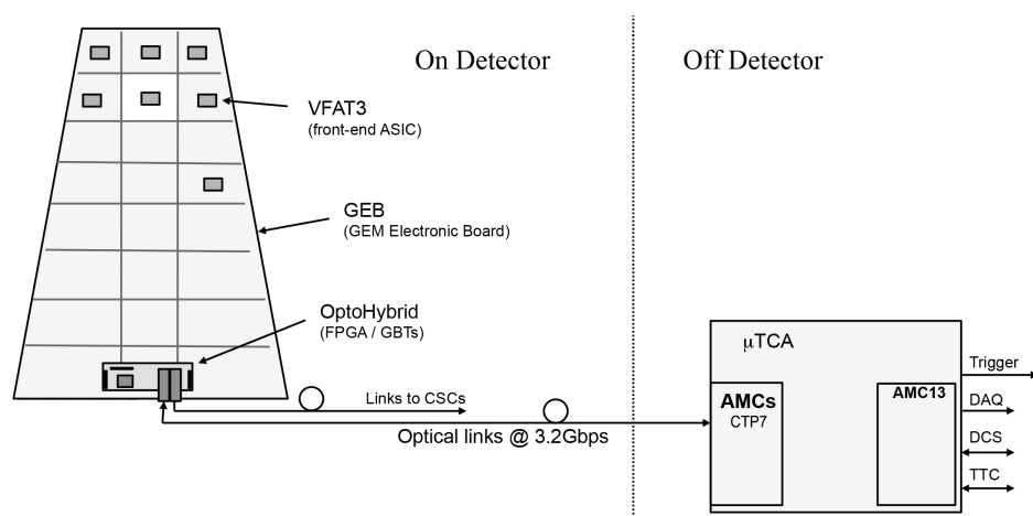
Figure 5.1 – Architecture of the GE1/1 DAQ system divided into two sectors: the on-detector electronics composed of the VFAT3 ASICs, GEB, and OptoHybrid, and the off-detector electronics with CTP7 and AMC13 mezzanines located in a microTCA crate [24].
