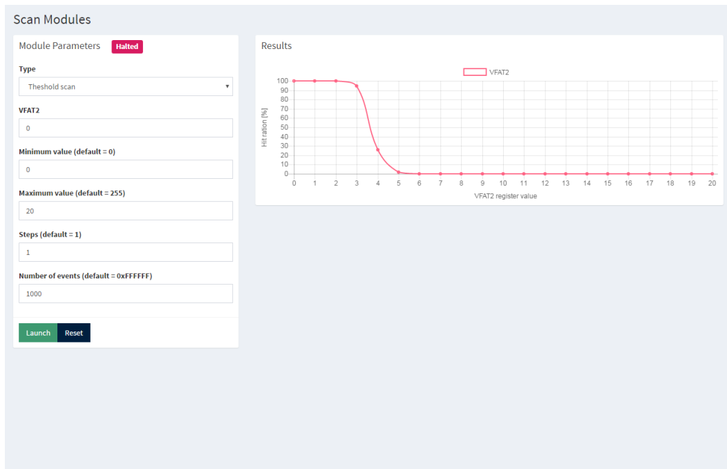
Figure 6.20 – Screenshot of the page of the web application used to perform calibration scans of the VFAT2s.
