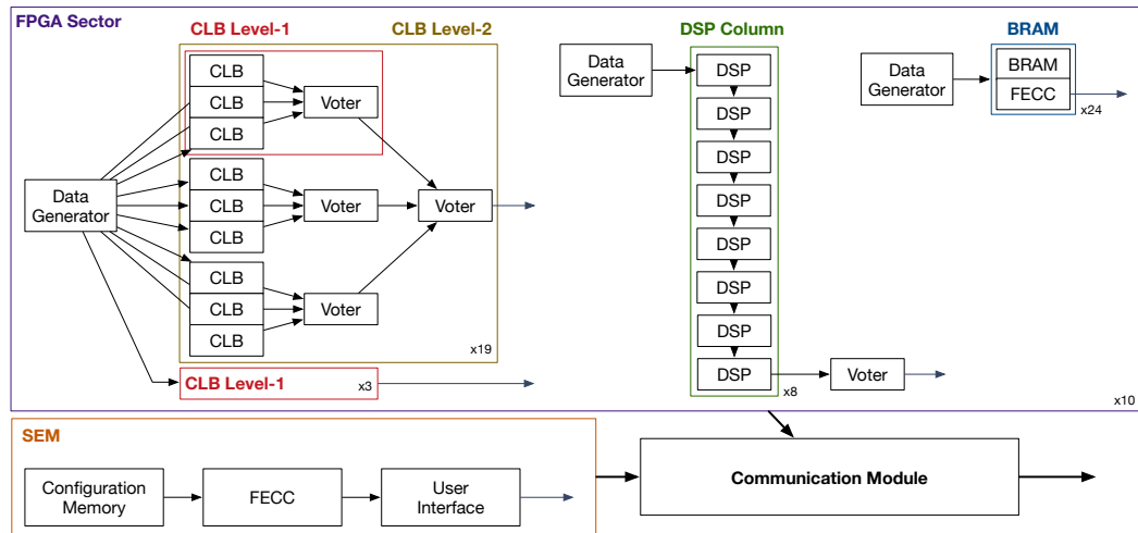
Figure 8.7 – Logic diagram of the firmware designed to detect errors in the irradiated FPGA.
