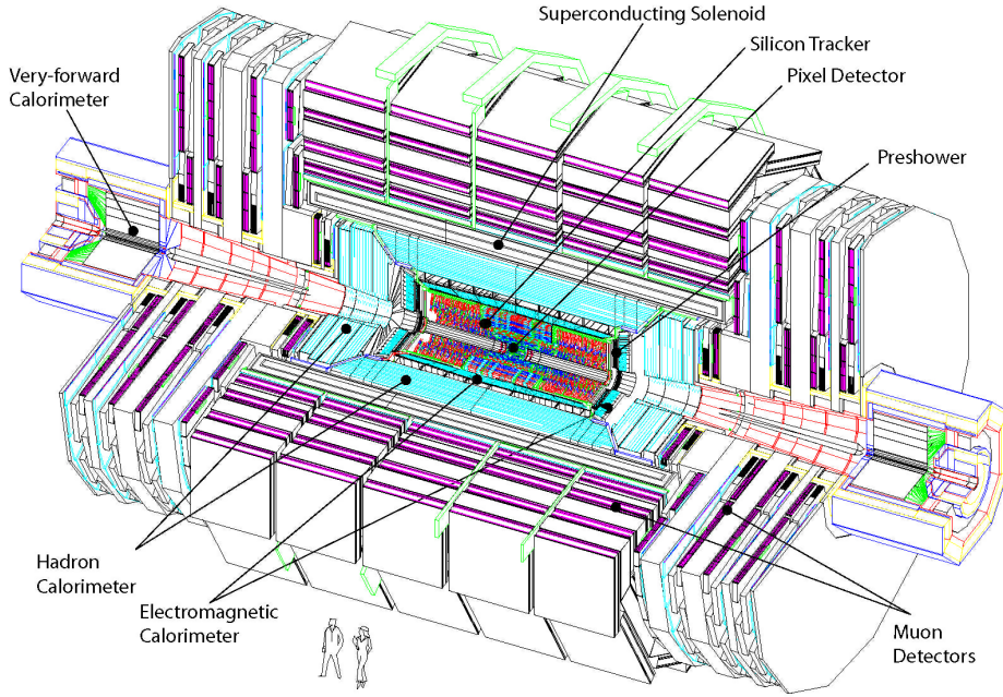
Figure 3.1 – The Compact Muon Solenoid detector and its subsystems installed at LHC [11].
