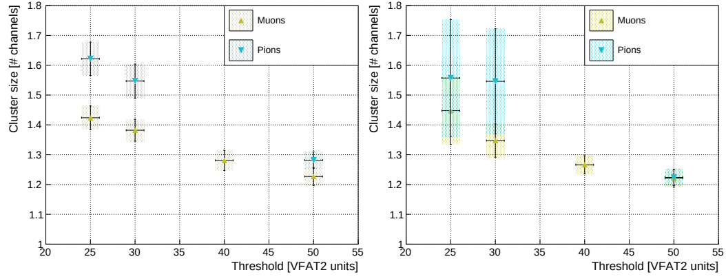
Figure 6.36 – Plots of the cluster size for muons (green) and pions (blue) as a function of the VFAT2 threshold in terms of VFAT2 units for GEM0 on the left and GEM1 on the right.
