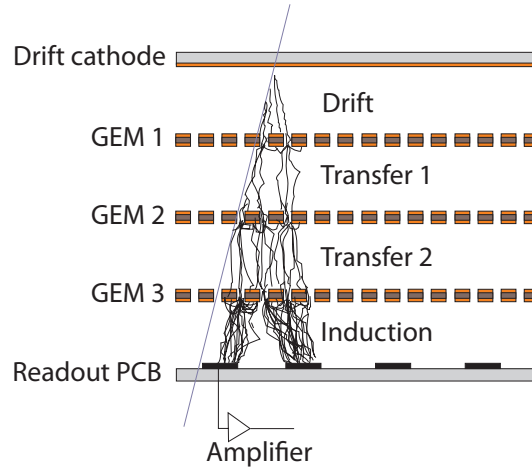
Figure 4.6 – Principle of operation of a generic triple-GEM chamber and definition of drift, transfer, and signal induction gap regions within the detector [24].
