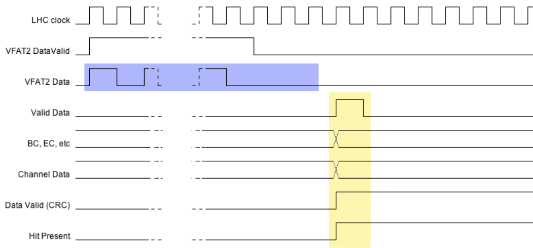
Figure 6.7 – Chronograph of the serial decoding of an incoming data packet (blue) which is analyzed and placed in parallel busses (yellow) with the CRC check bit and the hit present bit.
