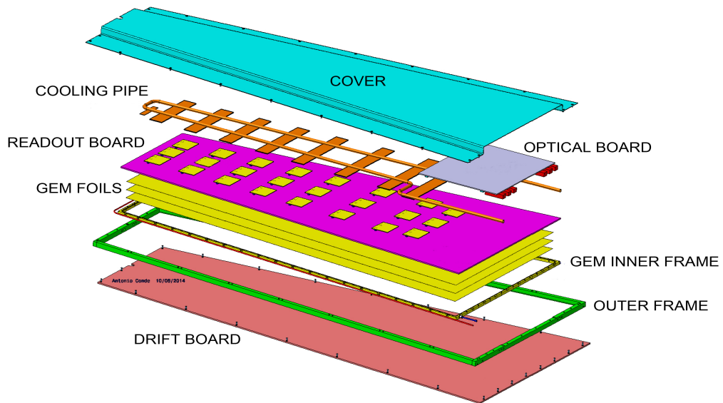
Figure 4.8 – Exploded view of the mechanical design of a Triple-GEM chamber [24].
