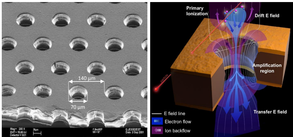
Figure 4.5 – Left: scanning electron microscope picture of a GEM foil. Right: schematic view of the electric field lines (white), electron flow (blue), and ion flow (purple) through a bi-conical GEM hole [24].
