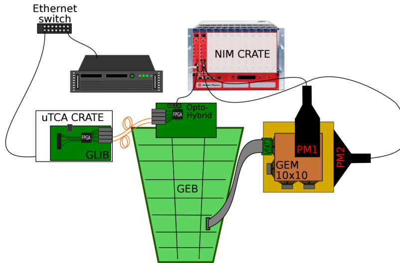
Figure 10.12 – Schematic view of the third prototype of the DAQ system of the 10 cm \times 10 cm Triple-GEM prototype. The VFAT2 Hybrid is connected through the GEB to the OptoHybrid, in turn connected to the GLIB through optical fibers. A NIM crate is used to perform the coincidence between the photomultipliers and send a trigger to the VFAT2 Hybrid through the OptoHybrid [67].
