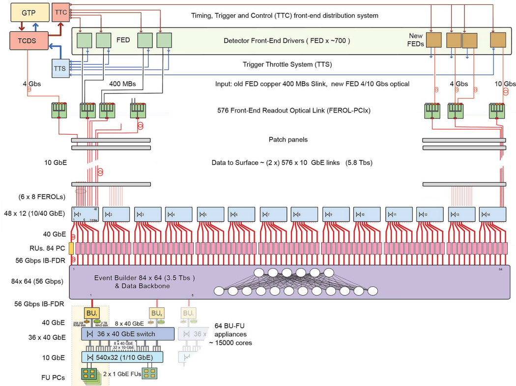
Figure 3.13 – Architecture of the DAQ system of CMS [23].
