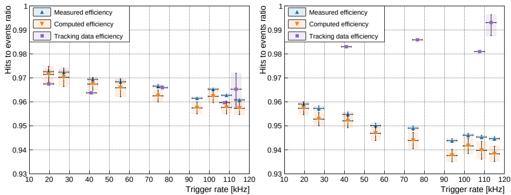
Figure 6.33 – Plots of the measured efficiency (blue), computed efficiency (orange), and tracking data based efficiency (purple) as a function of the trigger rates for GEM0 on the left and GEM1 on the right with pions.
