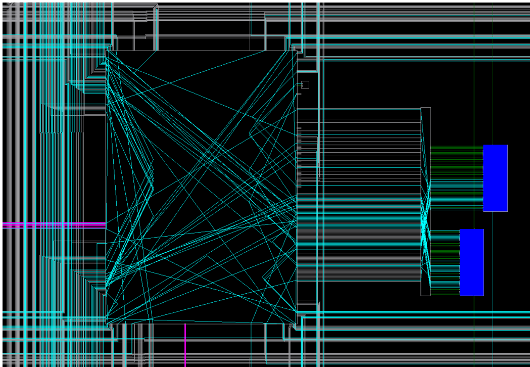
Figure 8.3 – Schematic of two slices (blue) connected to an element of the switching matrix which routes the signals (cyan) between components over the multitude of existing paths (gray).
