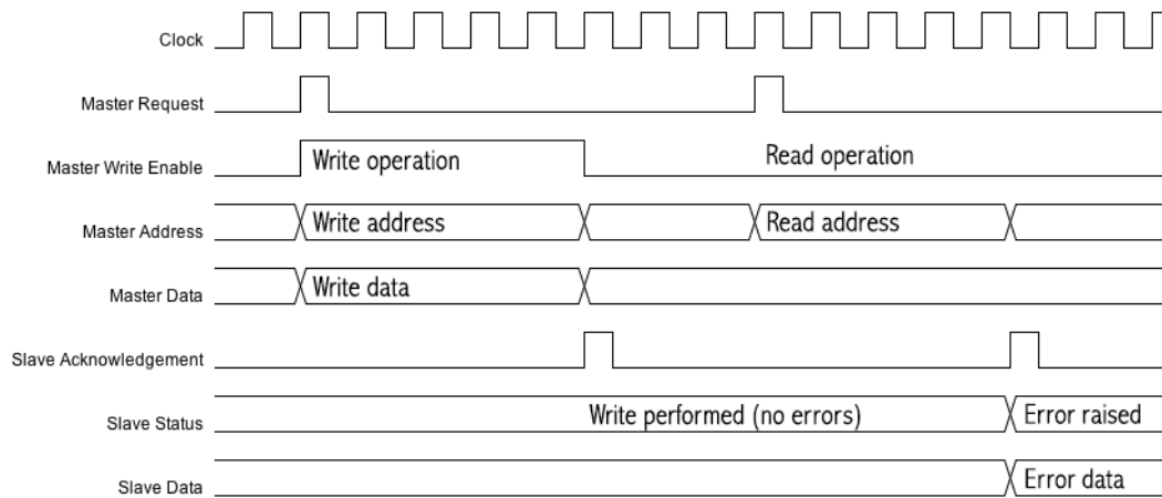
Figure 6.4 – Chronograph of two wishbone communications between a master and a slave for a successful write operation and a read operation resulting in an error.
