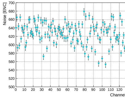
Figure 7.8 – Plot of the Equivalent Noise Charge (ENC) for each channel.
