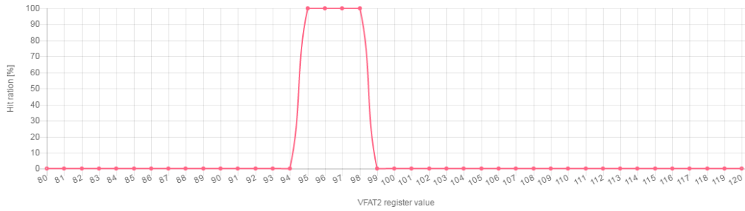
Figure 6.12 – Illustration of an ideal latency scan representing the hit percentage as a function of the latency of the VFAT2.
