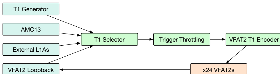
Figure 6.6 – Diagram of the switching and throttling process for T1 commands highlighting the various sources of T1 commands (blue) and the involved modules (green) before the signal is sent to the VFAT2 chips (orange).
