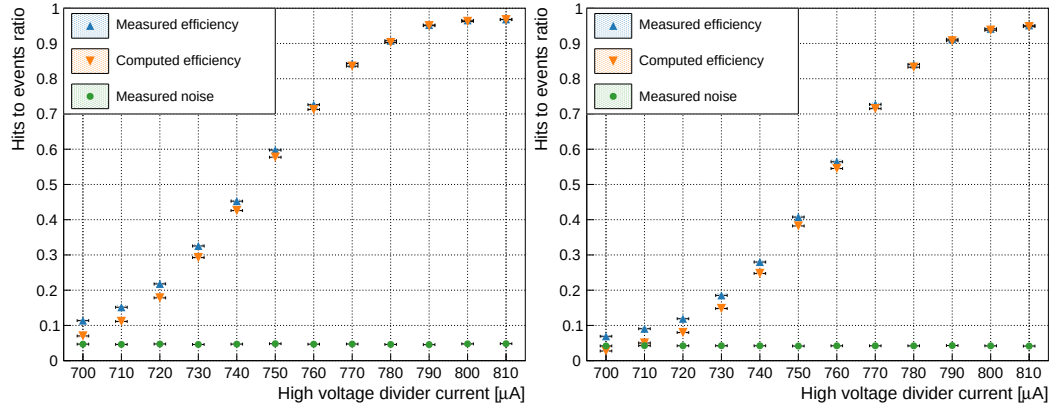
Figure 6.31 – Plots of the measured noise (green), measured efficiency (blue), and computed efficiency (orange) as a function of the high-voltage expressed in \mu\text{A} for GEM0 on the left and GEM1 on the right with muons.
