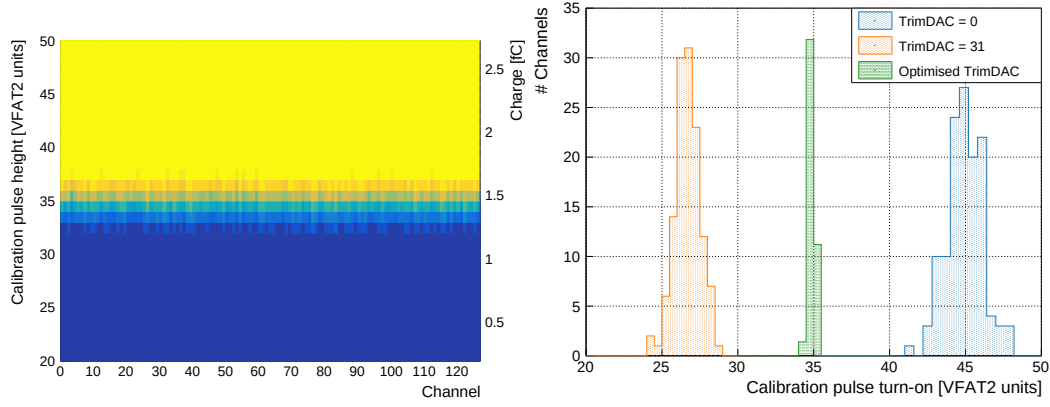
Figure 7.7 – Left: plot of the s-curve scan for each channel with the aligned values for the channel register. Right: dispersion of the turn-on value for the non-aligned (orange and blue) and aligned configurations (green, scaled by a factor of 0.35).
