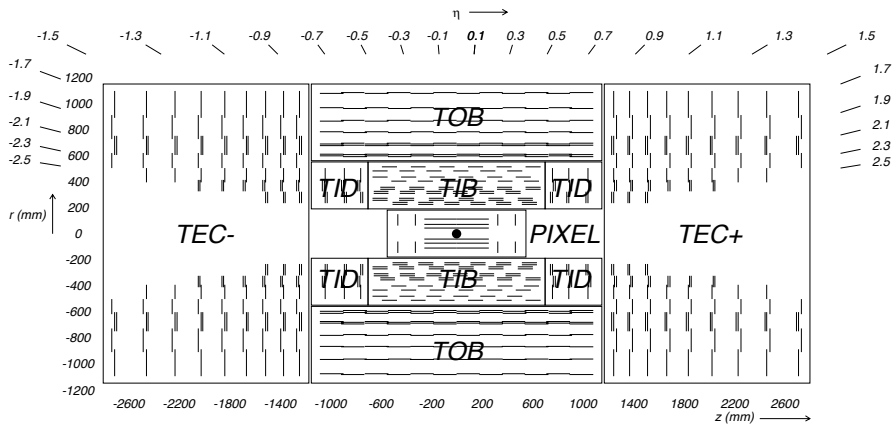
Figure 3.2 – Disposition of the silicon pixels (PIXEL) and strips (TIB, TID, TOB, and TEC) modules inside the tracker of CMS [11].
