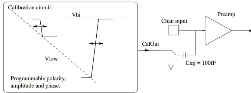
Figure 7.3 – Diagram of the injection and calibration circuit of the VFAT2 highlighting the path of the calibration pulse towards a given channel [53].
