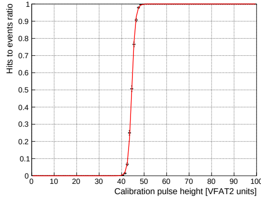
Figure 7.4 – Plot of the hit-to-event ratio as a function of the calibration pulse height in VFAT2 units for a threshold of 25.
