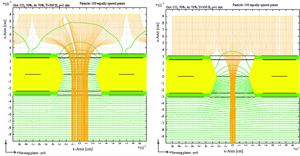
Figure 6.34 – Drift path (without diffusion) of electrons (orange) starting 90\ \mu\text{m} above the GEM, in an electrostatic configuration (green) without charges on the Kapton surface on the left and with charges on the Kapton surface on the right [50].
