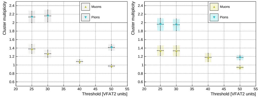
Figure 6.35 – Plots of the cluster multiplicity for muons (green) and pions (blue) as a function of the VFAT2 threshold in terms of VFAT2 units for GEM0 on the left and GEM1 on the right.
