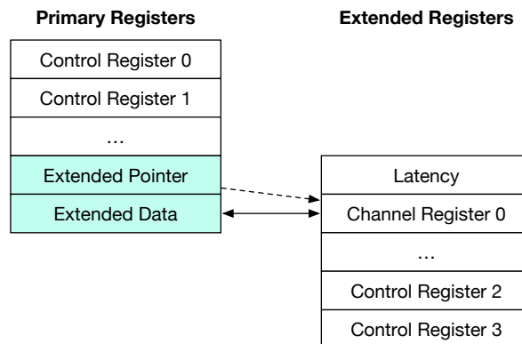
Figure 6.10 – Addressing of the extended registers through two primary registers.
