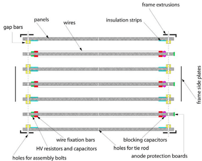
Figure 3.10 – Schematic view of a CSC detailing the different layers that compose it [11].
