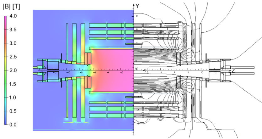
Figure 3.7 – Representation of the amplitude of the magnetic field and the field lines predicted on a longitudinal section of the CMS detector using simulations [21].
