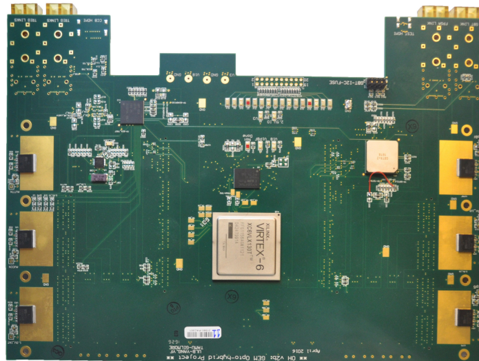
Figure 5.20 – Photograph of the OptoHybrid V2b that provides a testing platform for the GBT chipset.
