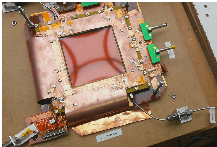
Figure 10.1 – Photograph of the 10 cm \times 10 cm Triple-GEM prototype along with the high voltage resistive divider in the bottom-left corner, the gas supply in the bottom-right corner, and the four readout sectors on the right and top of the image.
