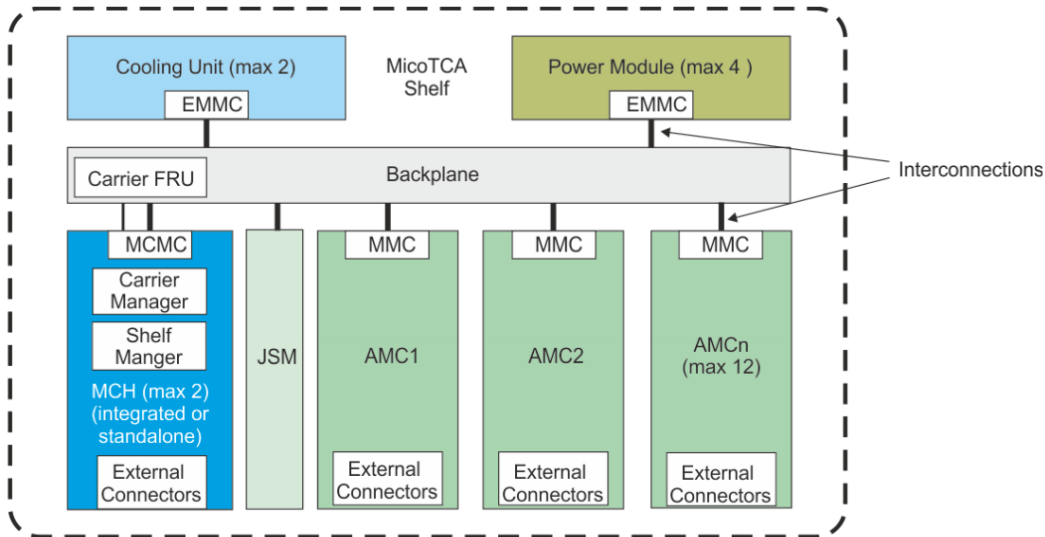
Figure 5.8 – Schematic representation of the architecture of a microTCA crate [32].
