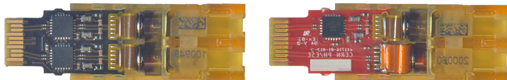
Figure 5.7 – Picture of the VTTx (left) and VTRx (right) optical transceivers of the Versatile Link project.
