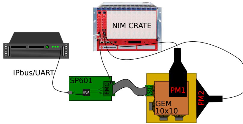
Figure 10.6 – Schematic view of the first prototype of the DAQ system of the 10 cm \times 10 cm Triple-GEM prototype. The VFAT2 Hybrid is connected through an FMC module to the SP601 development board, in turn connected to a server through IPbus over UART. A NIM crate is used to perform the coincidence between the photomultipliers and send a trigger to the VFAT2 Hybrid through the FMC [67].
