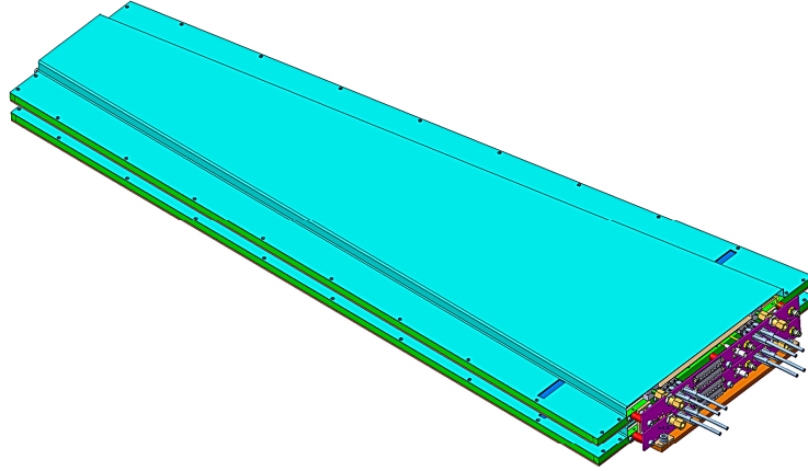
Figure 4.7 – A pair of GEM chambers form a superchamber [24].
