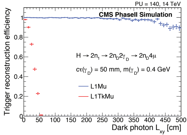
Figure 4.4 – The probability of reconstructing at least one muon candidate produced in the decay of a light long-lived particle decaying to a pair of muons \gamma_d \rightarrow \mu\mu as a function of L_{xy} , the distance between the \gamma_d decay vertex to the beamline in the transverse plane. Standalone muon trigger L1Mu performance is compared to that of L1TrkMu, a trigger based on matching muon and track trigger candidates with the CMS Phase-II detector simulation [24].
