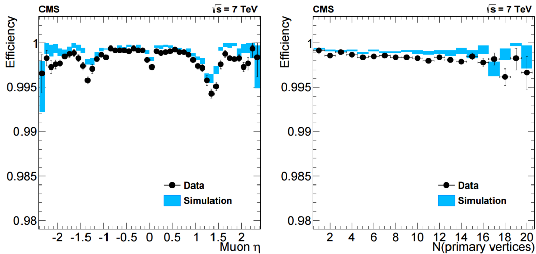
Figure 3.3 – Tracking efficiency measured with a tag-and-probe technique, for muons from Z decays, as a function of the muon \eta (left) and the number of reconstructed primary vertices in the event (right) for data (black dots) and simulation (blue bands) [19].
