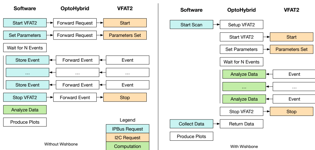
Figure 6.3 – Flow of operations for a custom calibration routine performed on the system without Wishbone on the left and with Wishbone on the right.
