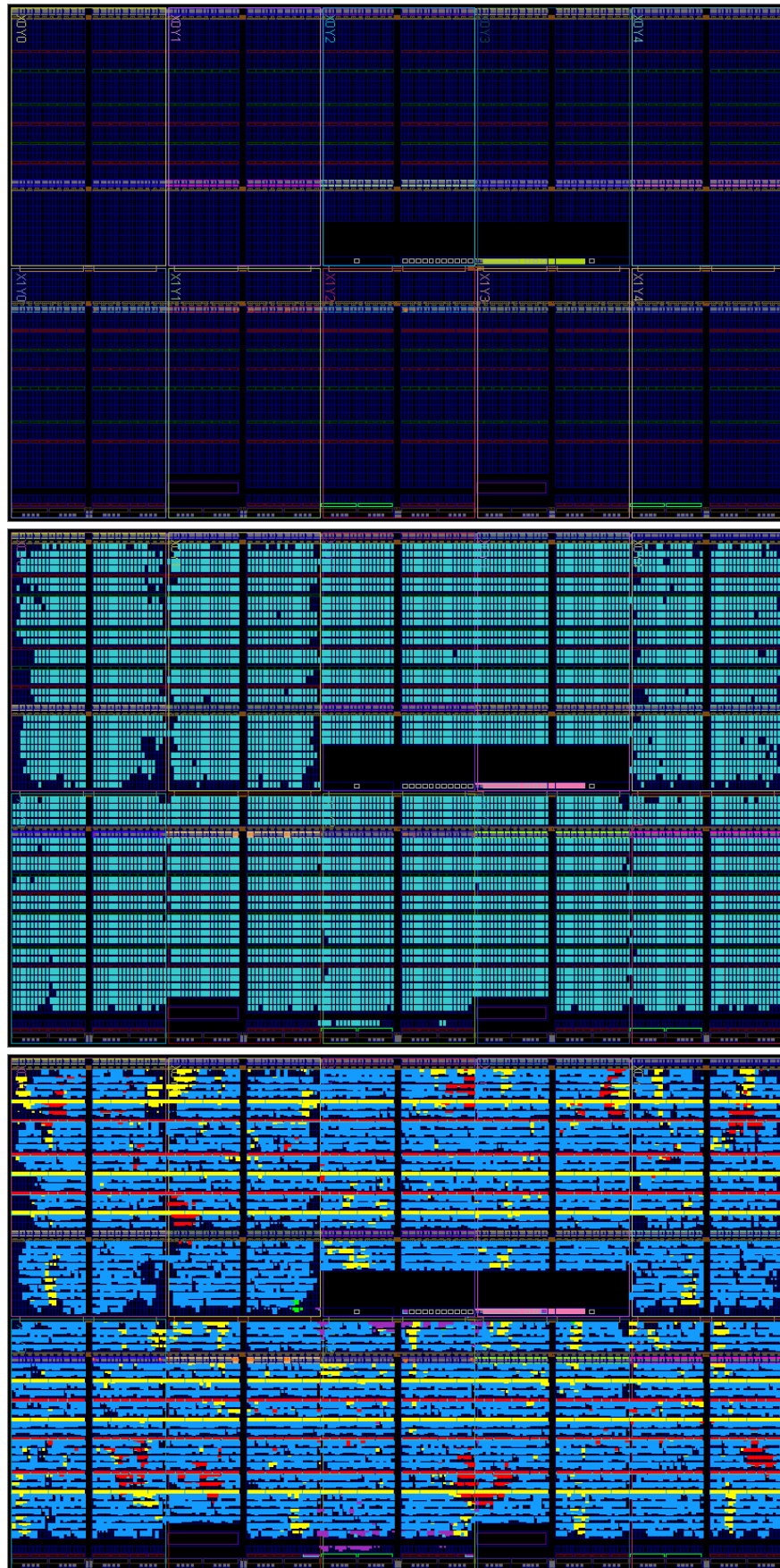
Figure 8.6 – Schematic view of the occupancy of the FPGA. Left: sectors of the FPGA labeled XaYb composed of CLBs in dark blue, BRAMs in red, and DSPs in green. Middle: highlight of the resources used by the design. Right: occupancy of the code developed to test the CLBs in blue, BRAMs in yellow, DSPs in red, SEM in purple, and the communication protocol in green.
