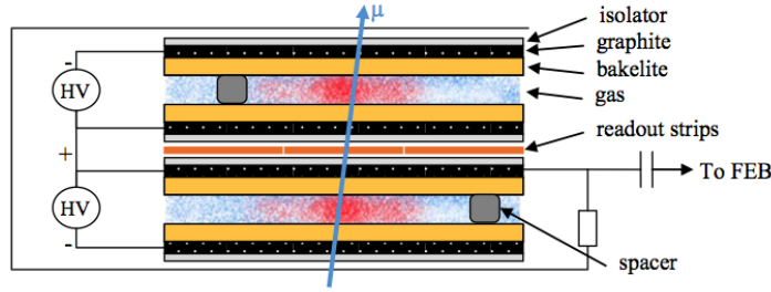
Figure 3.11 – Diagram of the RPCs double gap layout [11].
