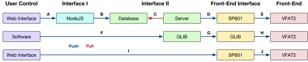
Figure 11.8 – Nodes of the DAQ systems and the interactions they have in order to transmit the request from the user control to the front-end electronics. Blue arrows indicate that data is pushed to the next node, and red arrows that the data is pulled from the node.
