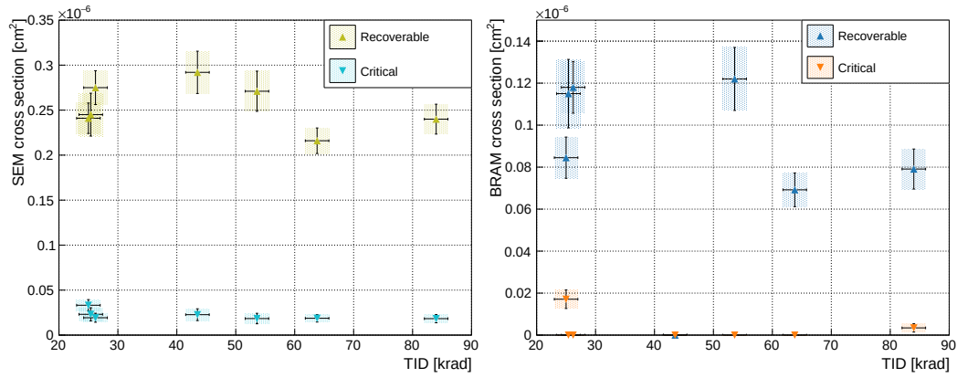
Figure 8.11 – Interaction cross section of particles as a function of the TID at an energy of 49.7 MeV for the configuration memory resulting in recoverable (green) and critical (blue) errors on the left, and with the BRAMs resulting in recoverable (blue) and critical (orange) errors on the right.
