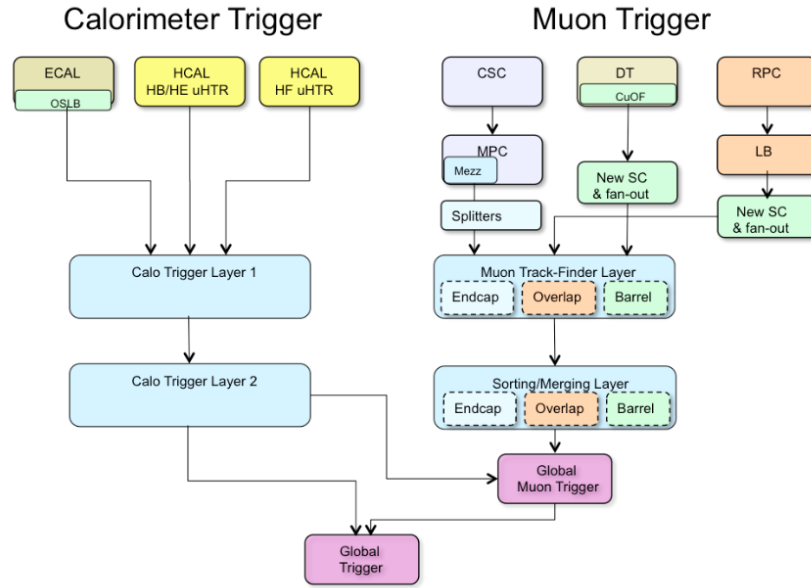
Figure 3.12 – Architecture of the CMS trigger system for both the calorimeter trigger and the muon trigger [22].
