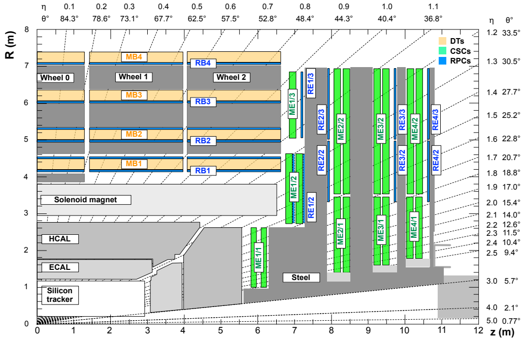
Figure 3.8 – Layout of the muon spectrometer of CMS depicting the three gaseous detectors in use: Drift Tubes (DTs) in orange labeled MBx, Cathode Strip Chambers (CSCs) in green labeled MEx/y, and Resistive Plate Chambers (RPCs) in blue labeled RBx and REx/y [11].
