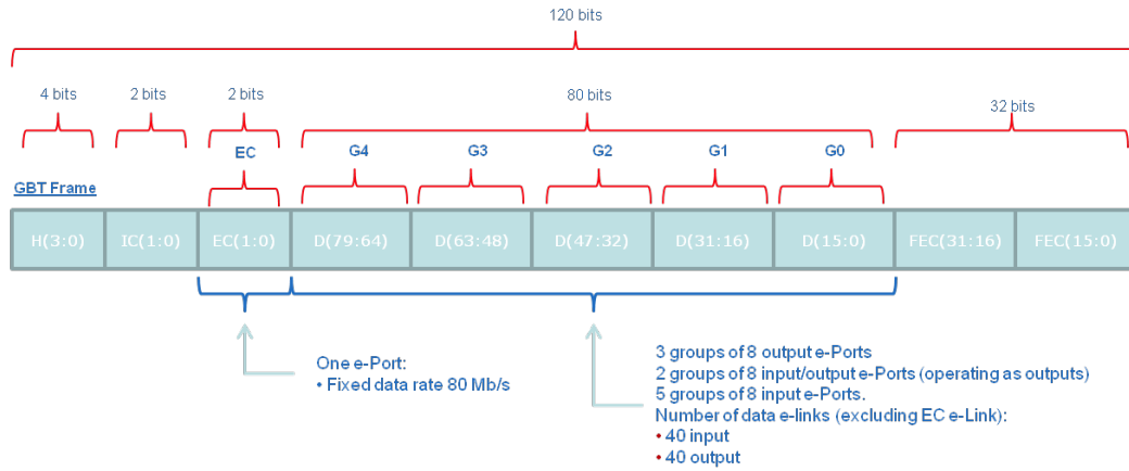
Figure 5.5 – Data format of a GBT frame [30].
