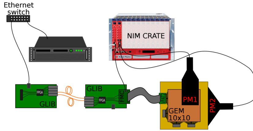
Figure 10.11 – Schematic view of the second prototype of the DAQ system of the 10 cm \times 10 cm Triple-GEM prototype. The VFAT2 Hybrid is connected through an FMC module to a first GLIB, in turn connected to a second GLIB through optical fibers. A NIM crate is used to perform the coincidence between the photomultipliers and send a trigger to the VFAT2 Hybrid through the FMC [67].
