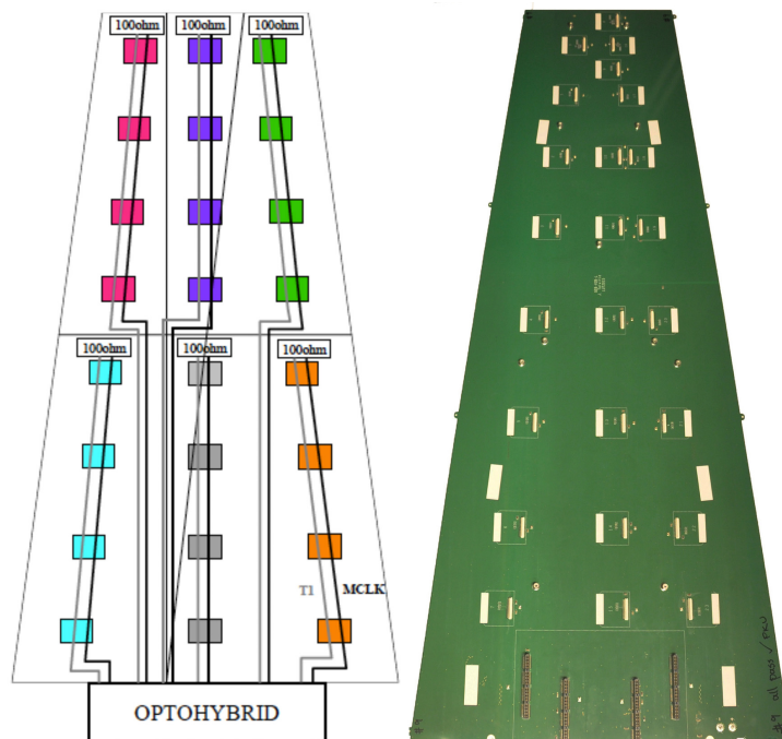
Figure 5.3 – Pictures of a prototype of the GEB, a PCB of the same dimension as the GEM detector designed to route the signals of the front-end chips to the OptoHybrid [24].
