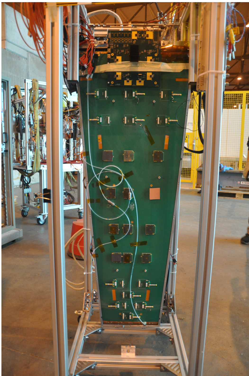
Figure 6.25 – Photograph of the GEM detectors used during the test beam and equipped with the full electronics system.
