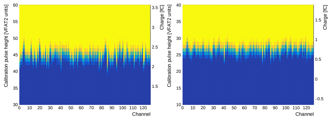
Figure 7.6 – Plots of the s-curve scans for each channel with the minimum value of the channel registers on the left and the maximum value on the right.
