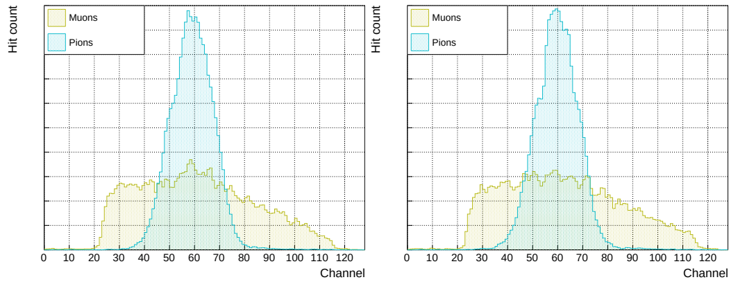
Figure 6.37 – Plots of the beam profile for muons (green) and pions (blue) for GEM0 on the left and GEM1 on the right.
