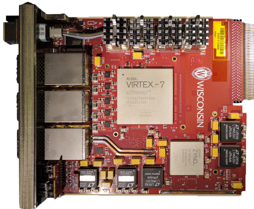
Figure 5.9 – Photograph of the CTP7 AMC developed by the University of Wisconsin used as back-end electronics [33].
