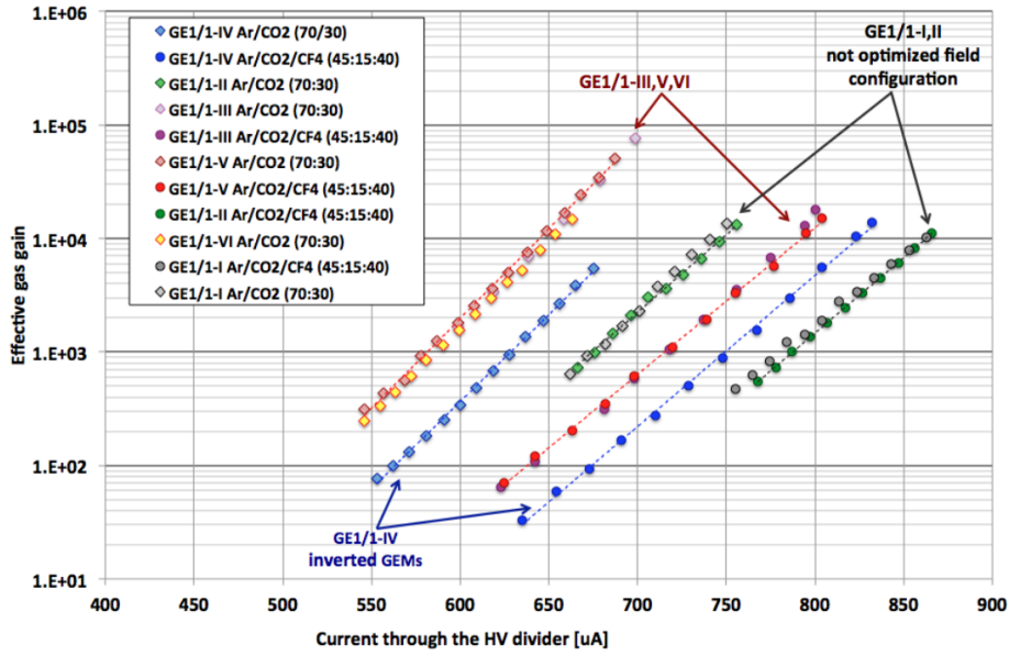
Figure 6.26 – Measured gas gains as a function of the current through the high voltage divider for the different generations of GEM detectors and for Ar/CO 2 70:30 and Ar/CO 2 /CF 4 45:15:40 [46].
