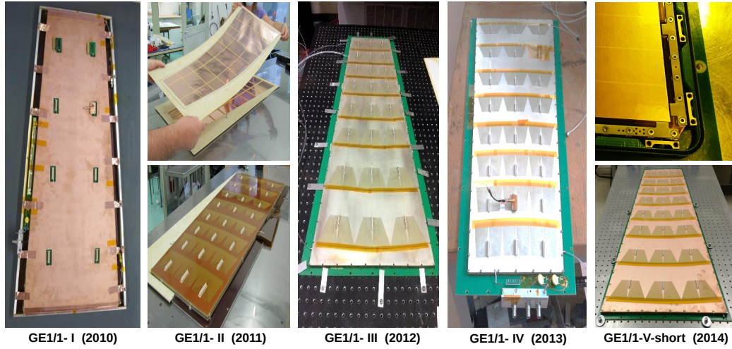
Figure 4.10 – Five generations of GE1/1 prototype chambers constructed and tested by the GEM collaboration in 2010-2014. The split figures for GE1/1-II and GE1/1-V demonstrate the evolution from construction using spacer frames to purely mechanical stretching of GEM foils without any spacers [24].
