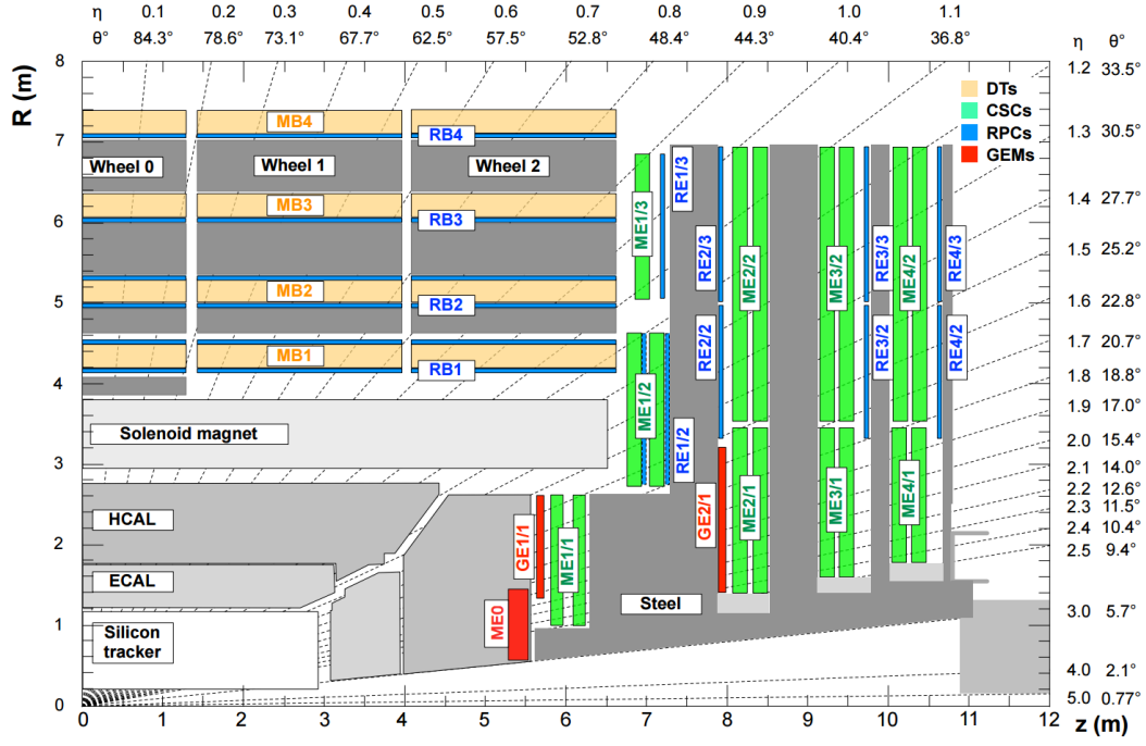
Figure 4.14 – Longitudinal view of a quadrant of CMS highlighting the location of the GE1/1, GE2/1, and ME0 detectors colored in red within the muon spectrometer. DTs are represented in yellow, CSCs in green, and RPCs in blue [28].
