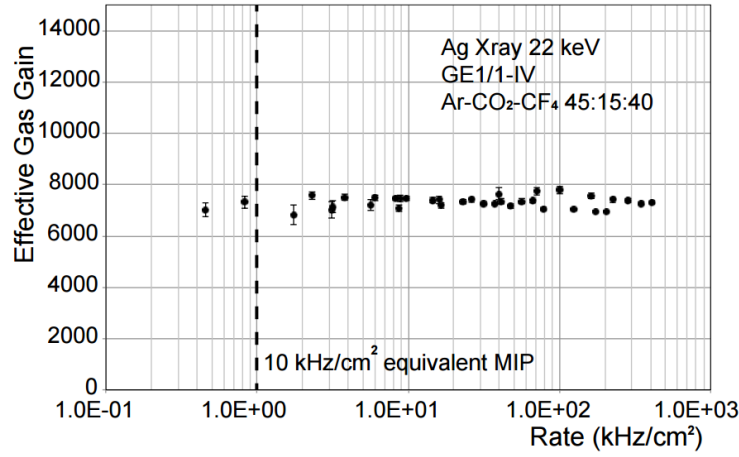
Figure 4.11 – Effective gas gain as a function of the rate of incident particles in a GE1/1-IV detector irradiated with a 22 keV X-ray source [24].
