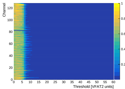
Figure 7.1 – Two-dimensional graph plotting the evolution of the noise level for each channel as a function of the VFAT2 threshold in VFAT2 units.
