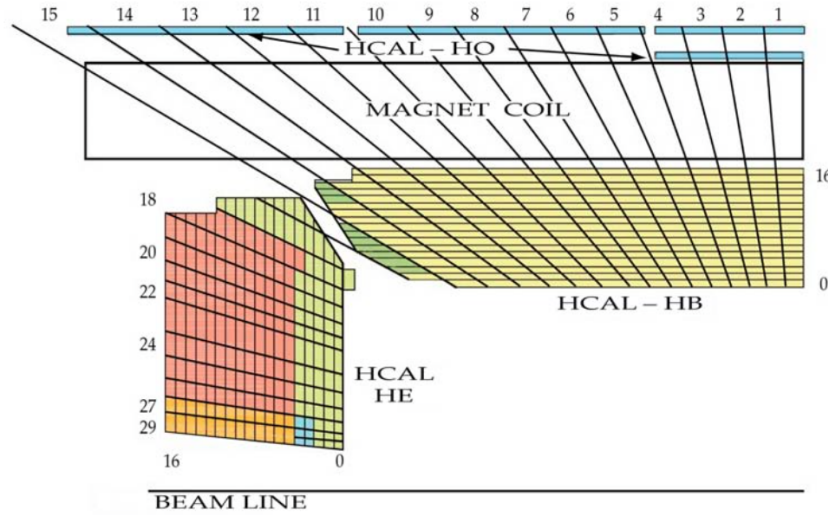
Figure 3.6 – Longitudinal view of the HCAL showing the disposition of the barrel, endcaps, and outer calorimeters [11].
