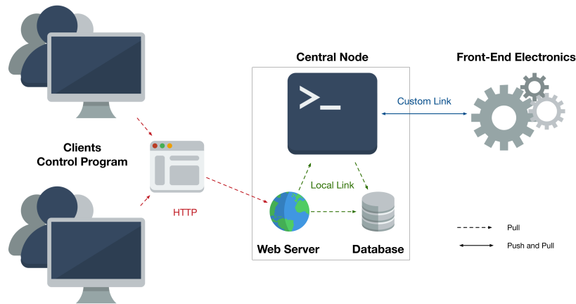
Figure 11.6 – Diagram of the architecture used in most DAQ systems in which the whole system relies on the presence of the server which acts as the central node.
