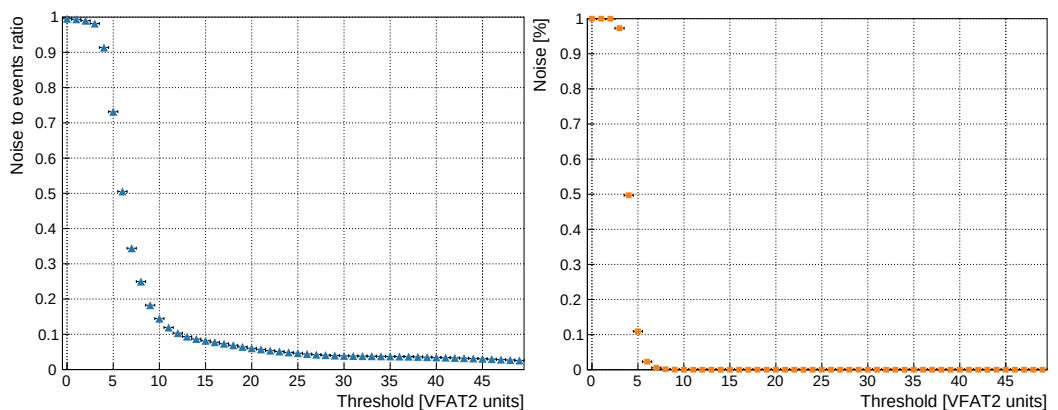
Figure 6.29 – Plots of the noise level as a function of the VFAT2 threshold in terms of VFAT2 units with results obtained during the test beam on the left and with the improved noise cancellation on the right.
