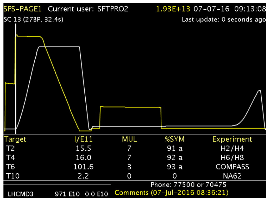
Figure 6.24 – Monitoring page of the SPS indicating the presence of spills of particles (yellow).
