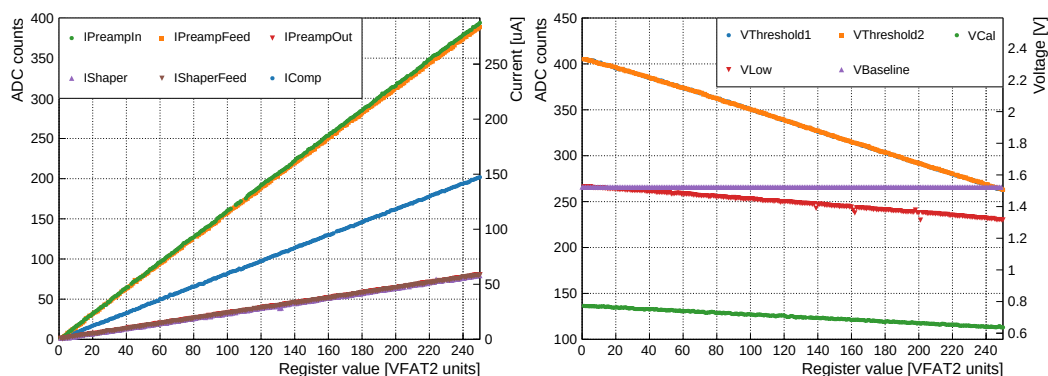
Figure 7.2 – Plots of the ADC counts, current values on the left, and voltage values on the right of each settable register of the VFAT2 as a function of the 8-bit value written in the register.
