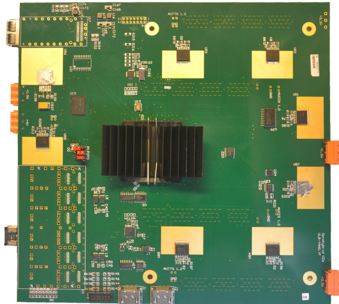
Figure 5.18 – Photograph of the OptoHybrid V2a equipped with a Xilinx Virtex-6 FPGA that concentrates the data from the 24 VFAT2 Hybrids and transmits it to the off-detector electronics.
