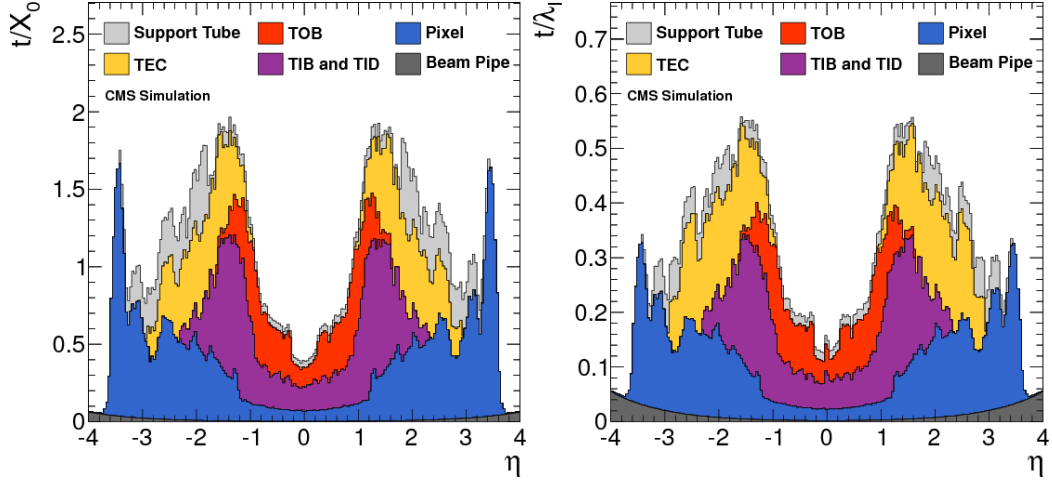
Figure 3.4 – Material budget of the tracker expressed in terms of radiation length X_0 on the left and hadronic interaction length \lambda_I on the right [19].
