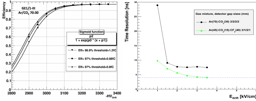
Figure 4.12 – Left: evolution of the efficiency as a function of the high voltage applied to the drift electrode for a GE1/1-III chamber operated with Ar/CO 2 at 70% and 30% respectively and for different offline cuts on the collected charge [24]. Right: time resolution of a small Triple-GEM detector as a function of the electric field in the drift gap [28].
