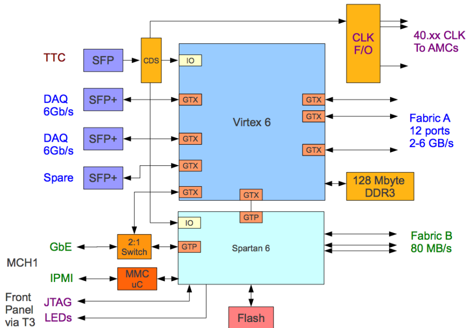
Figure 5.10 – Functional diagram of the AMC13 highlighting the external connections to the TTC system, backplane, and MCH of the microTCA crate [34].
