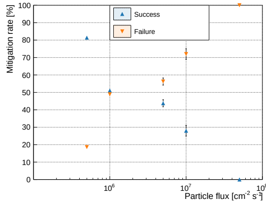
Figure 8.13 – Success (blue) and failure (orange) percentage of the triplication method according to the flux of particles when an SEU appears.
