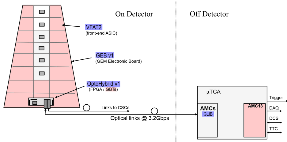
Figure 5.12 – Architecture of the first prototype of the GE1/1 DAQ system with the VFAT2 ASIC, first version of the GEB, first version of the OptoHybrid, and GLIB AMC.
