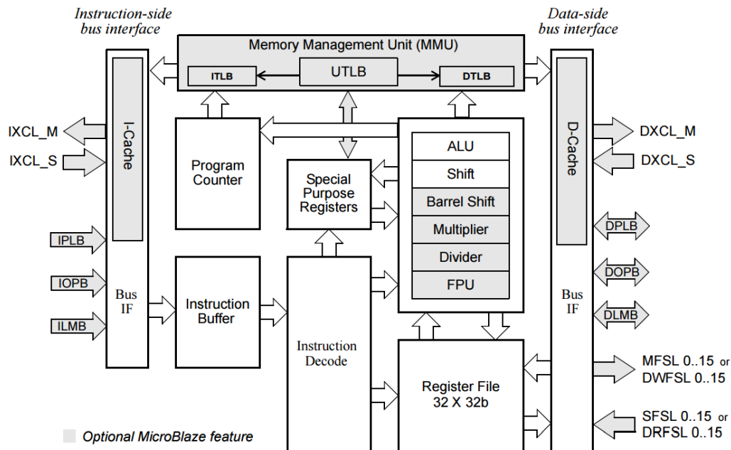
Figure 10.8 – Functional diagram of the architecture of the Microblaze soft core processor developed by Xilinx [68].
