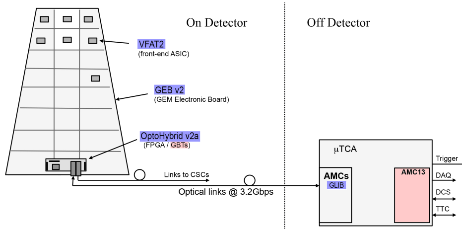
Figure 5.17 – Architecture of the GE1/1 DAQ system used during the test beam with the VFAT2 ASIC, second version of the GEB, second version of the OptoHybrid, and GLIB AMC.
