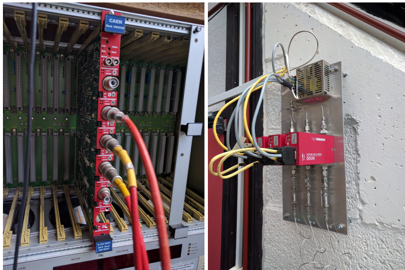
Figure 10.2 – Photographs of the CAEN V6533N VME high voltage module inserted in a VME crate on the left, and of the three mass flow meters connected to the gas bottles on the right.
