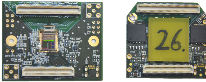
Figure 5.14 – Photograph of the VFAT2 Hybrids on which the VFAT2 ASICs are mounted to be interfaced with the GEB.
