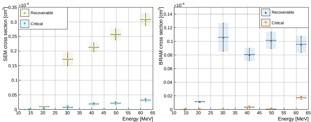
Figure 8.10 – Interaction cross section of particles as a function of the energy of the beam for the configuration memory resulting in recoverable (green) and critical (blue) errors on the left, and with the BRAMs resulting in recoverable (blue) and critical (orange) errors on the right.
