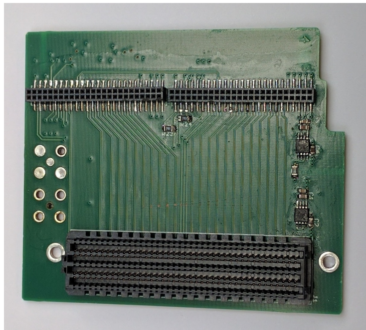
Figure 10.7 – Photograph of the VFAT2 FMC module which connects the SP601 development board to two VFAT2 Hybrids, provides power to the latter, and is able to receive or send trigger through two LEMO connectors.
