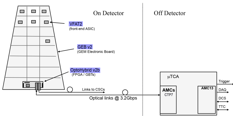
Figure 5.19 – Architecture of the GE1/1 DAQ system foreseen for the slice test with the VFAT2 ASIC, second version of the GEB, second version of the OptoHybrid, CTP7 AMC, and AMC13.
