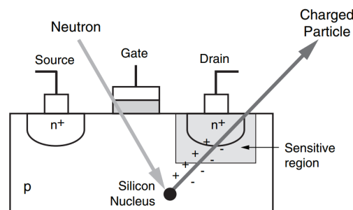
Figure 8.4 – Charge deposition by a charged particle inside a transistor affecting the state of the circuit [57].
