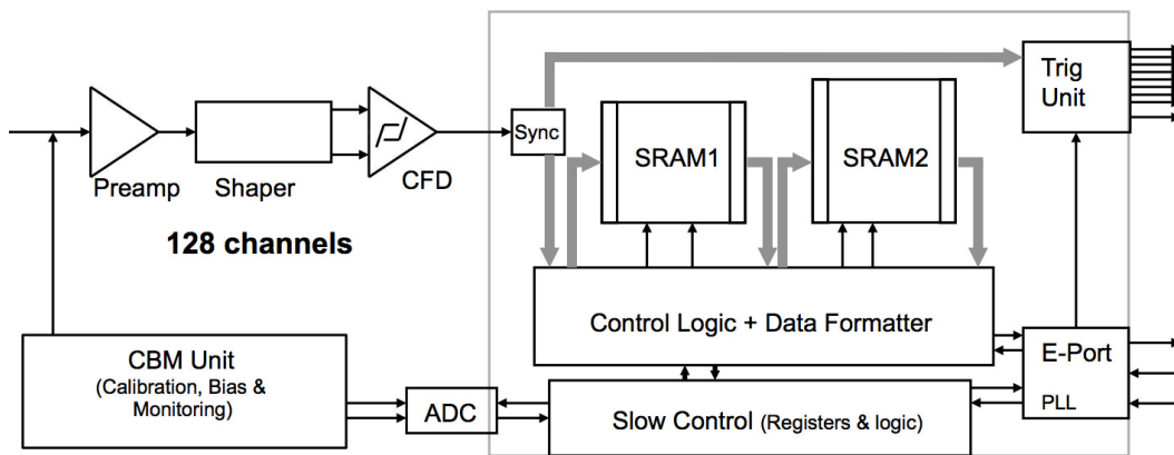
Figure 5.2 – Schematic diagram of the VFAT3 showing the analog front-end on the left and the digital control and readout system on the right [24].
