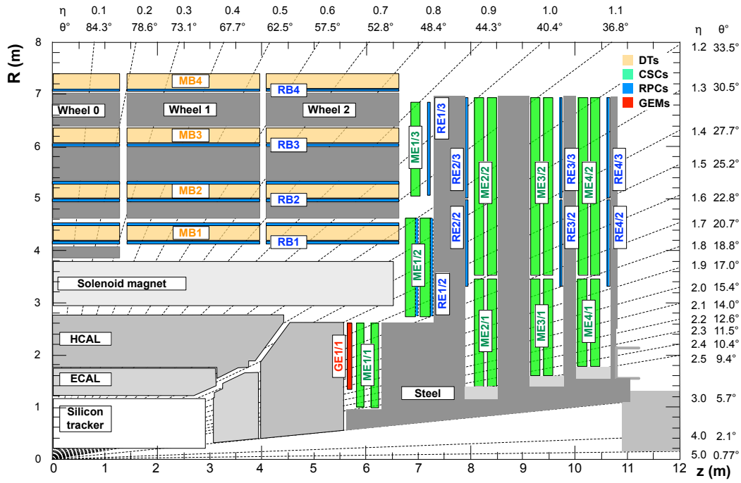
Figure 4.1 – Longitudinal view of a quadrant of CMS highlighting the location of the GE1/1 detectors colored in red within the muon spectrometer. DTs are represented in yellow, CSCs in green, and RPCs in blue [24].
