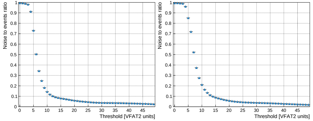
Figure 6.28 – Plots of the noise level as a function of the VFAT2 threshold in terms of VFAT2 units, the decimal value written in the 8 bit register afterwards converted to a voltage level, for GEM0 on the left and GEM1 on the right.
