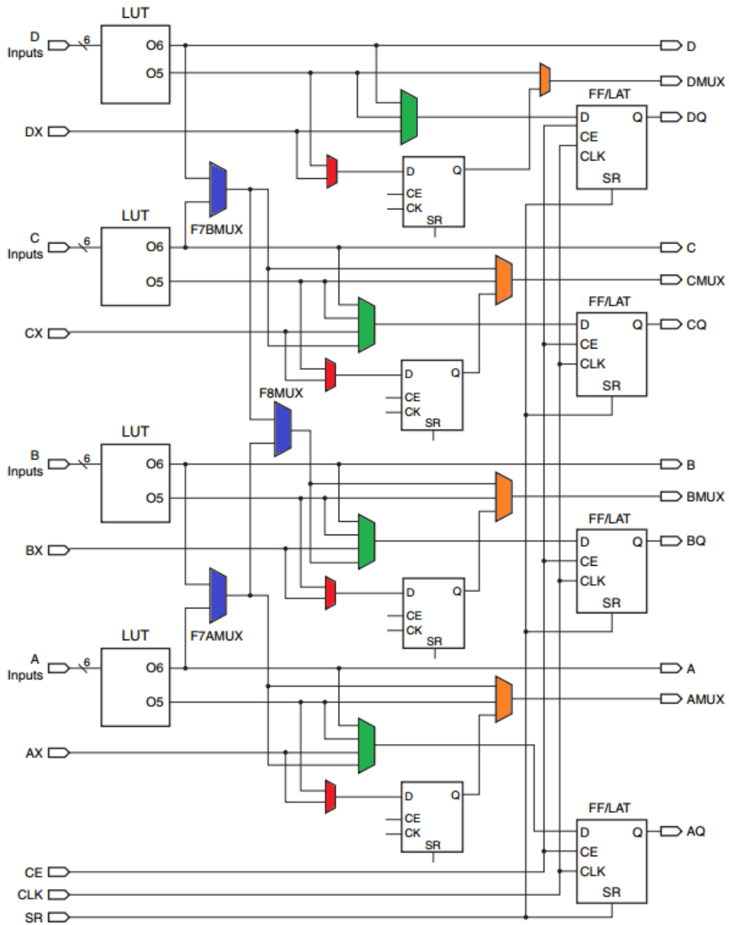
Figure 8.1 – Simplified view of a slice composed of four LUTs on the left and eight registers on the right [54].
