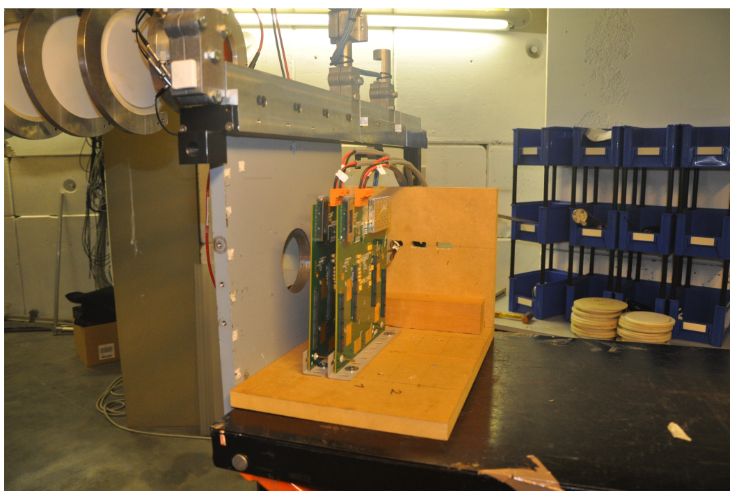
Figure 8.9 – Top: photograph of the beam line delivering the protons in the irradiation area in front of which degraders can be placed in order to change the energy of the particles. Bottom: photograph of the two OptoHybrids being aligned in front of the beam using lasers.
