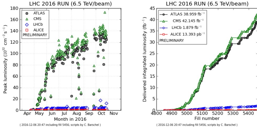
Figure 2.4 – Monthly evolution of the peak delivered luminosity (left) for the four main experiments of the LHC and the corresponding integrated luminosity (right) [17].
