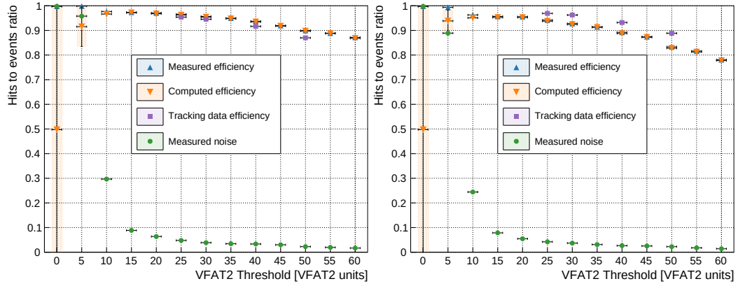
Figure 6.32 – Plots of the measured noise (green), measured efficiency (blue), computed efficiency (orange), and tracking data based efficiency (purple) as a function of the VFAT2 threshold in terms of VFAT2 units for GEM0 on the left and GEM1 on the right with muons.
