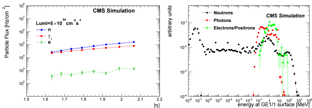
Figure 8.14 – Left: particle fluxes for the GE1/1 station as a function of the pseudorapidity for the LHC Phase II [63]. Right: energy spectrum of the background particles in GE1/1 [63].
