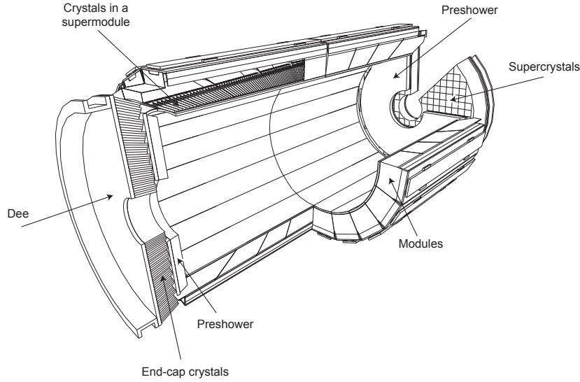
Figure 3.5 – Layout of the ECAL showing the disposition of the crystals, modules, supermodules, and preshower [11].
