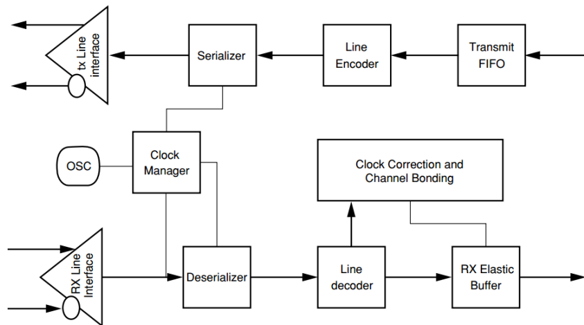
Figure 6.13 – Fonctionnal diagram of the Gigabit Transceiver X module used inside the Xilinx Virtex-6 FPGAs for high-speed serial communication [41].
