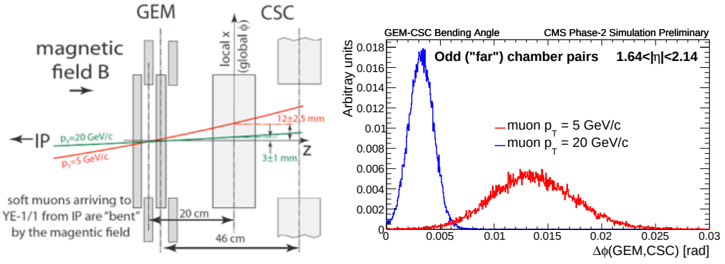
Figure 4.2 – Left: sketch of the measurement of the bending angle with a pair of CSC and GEM chambers, illustrating the difference between lower and higher momentum muons. Right: \Delta\phi = \phi_{GE1/1} - \phi_{ME1/1} distribution for 5 GeV/c and 20 GeV/c p_T muons demonstrating the discrimination power of the combined GEM-CSC system [24].
