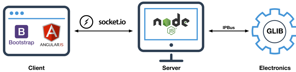
Figure 6.14 – Functional diagram of the architecture of the application used to control and monitor the GEM detectors.
