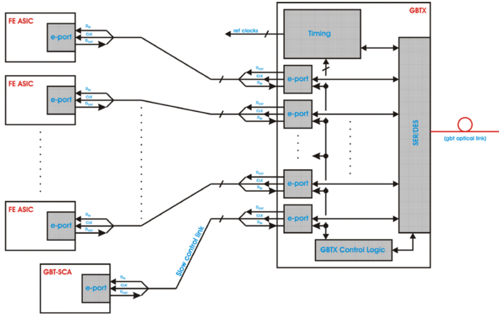
Figure 5.6 – Interaction between the GBTX ASIC and external front-end drivers through E-links [30].
