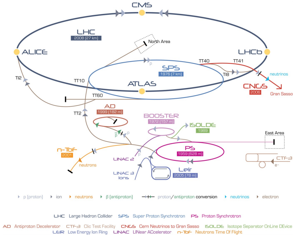
Figure 2.2 – Schematic diagram of the injection chain of the LHC composed of multiple smaller accelerators [16].
