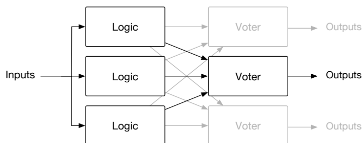
Figure 8.5 – Logic diagram of a triplicated module coupled to a single voter (black) or to three distinct voters (gray).
