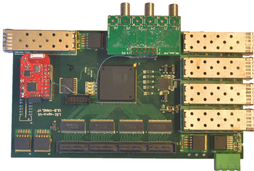
Figure 5.15 – Photograph of the OptoHybrid V1 equipped with a Xilinx Spartan-6 FPGA that concentrates the data from the six VFAT2 Hybrids and transmits it over four optical links to the off-detector electronics.
