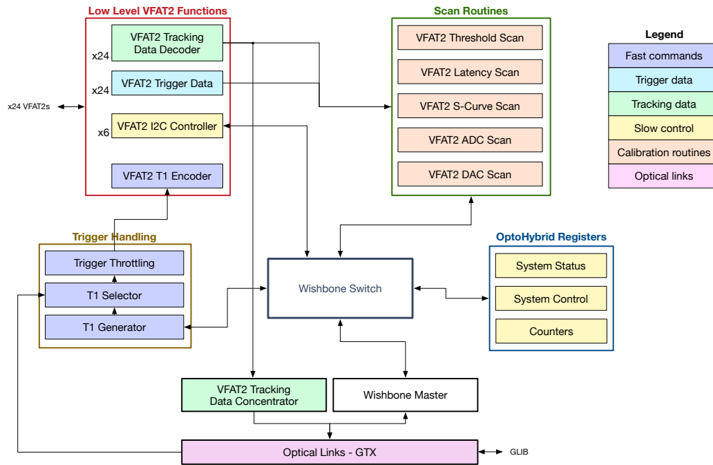
Figure 6.1 – Schematic diagram of the modules implemented in the firmware of the OptoHybrid regrouped by functionality.
