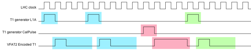
Figure 6.5 – Chronograph of two events generated by the T1 generator and encoded on the T1 lines for the VFAT2s: first two L1As (blue) are sent with a fixed interval, then a CalPulse (red) is generated followed by a L1A (green) after a defined delay. The T1 commands are encoded on three bits for the VFAT2s ("100" for L1As and "111" for CalPulses).
