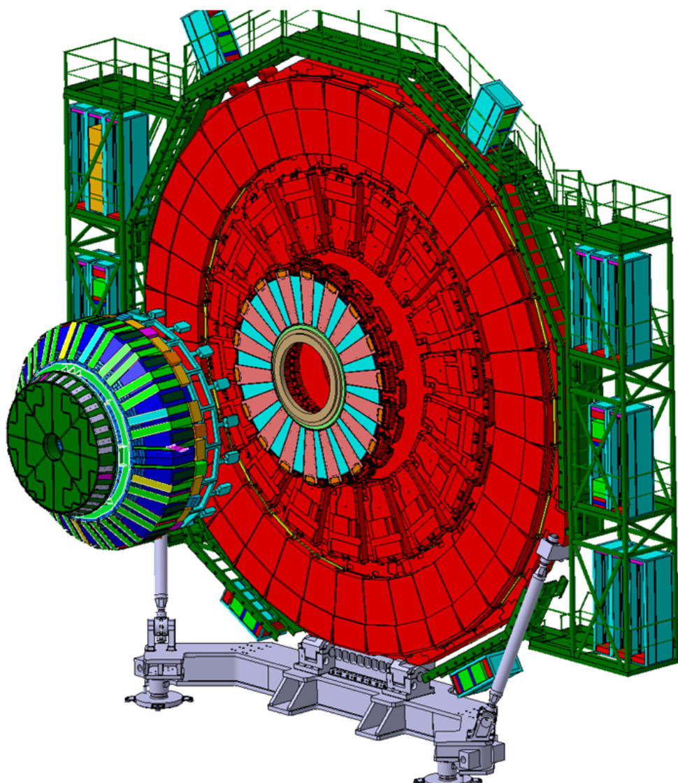
Figure 4.9 – First CMS muon endcap station where the inner ring is equipped with 18 long (red) and 18 short (blue) triple GEM superchambers [24].
