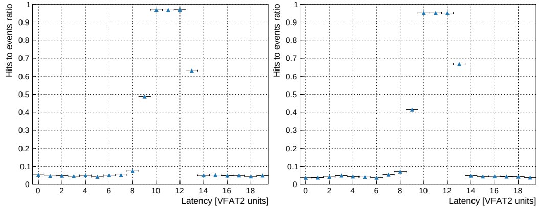
Figure 6.30 – Plots of the ratio of hit events as a function of the VFAT2 latency in terms of BXs for a monostable pulse length of four clock cycles for GEM0 on the left and GEM1 on the right with muons.
