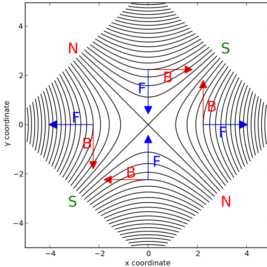
Figure 2-3. Magnetic field of an ideal quadrupole. Plot taken from Ref. [5].
