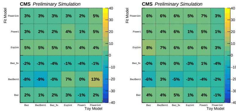
Figure 6-17. Bias in different BDT-based ZH subcategories. The subcategories are: Cat1 BDT [-1.0, -0.1] (left), Cat2 BDT [-0.1, 1.0] (right). In the tables, the "Power" stands for a single power function and the "PowerInt" stands for a single power function plus a constant.
