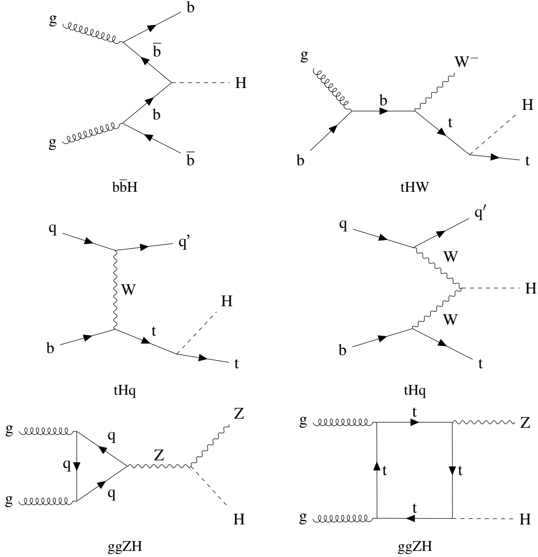
Figure 3-3. Examples of minor Higgs boson production modes.
