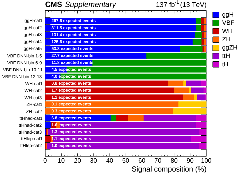
Figure 7-1. Expected fraction of signal events per production mode in the different subcategories for m_H = 125.38 GeV. The tH contribution is defined as the sum of tHq and tHW processes.
