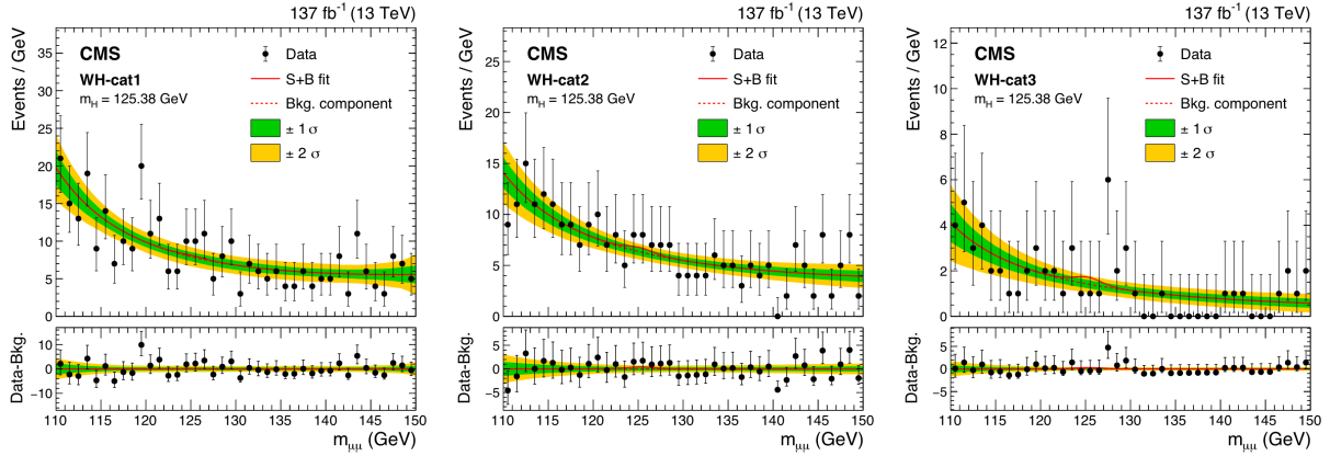
Figure 6-18. Post-fit m_{\mu\mu} distribution of the WH subcategories. The subcategories are: Cat1 BDT [-1.0, -0.1] (left), Cat2 BDT [-0.1, 0.3] (middle), Cat3 BDT [0.3, 1.0] (right). The upper panel in the plots shows the distribution of observed data and the shape of the signal-plus-background fit. The lower panel in the plots shows the residual distribution after subtracting the background component in the fits. The green and yellow bands show the one and two standard deviation of the background component uncertainty.
