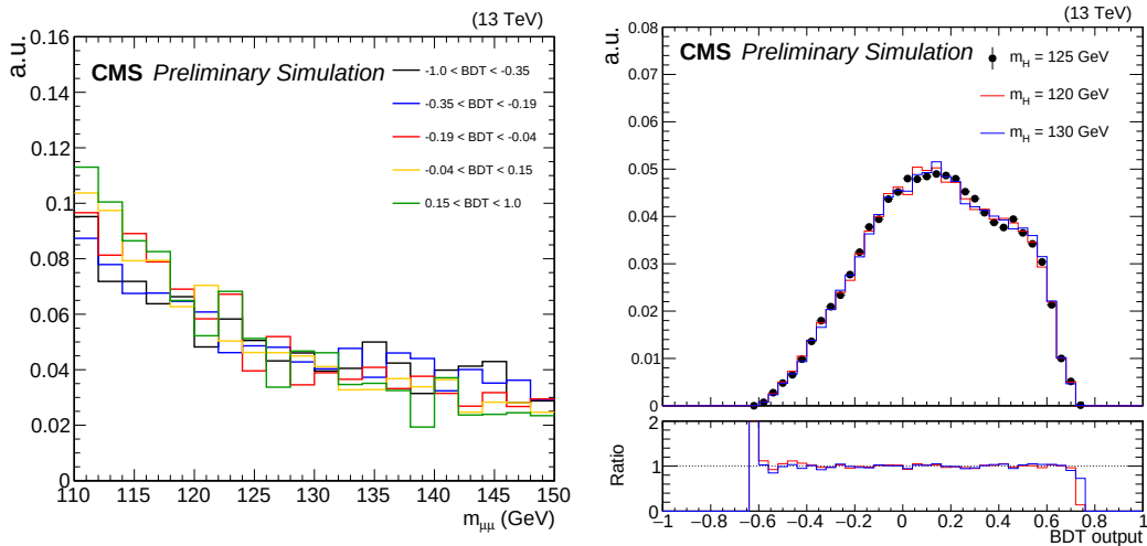
Figure 6-5. For the WH BDT, the distribution of the dimuon mass shape in the background for five different BDT quantile (left), and the distribution of the BDT output for three different signal mass assumptions (right).
