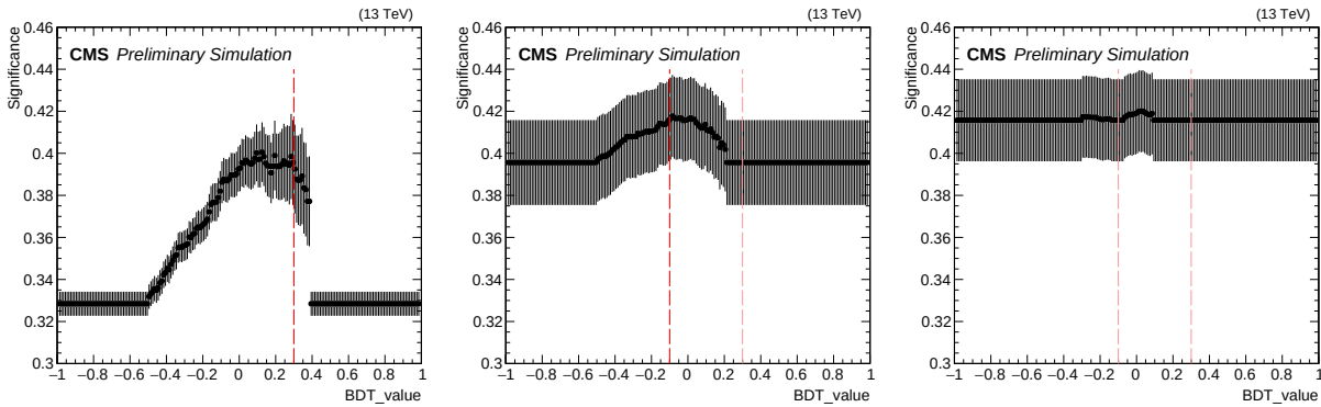
Figure 6-11. Scans for the first (left), second (middle) and a potential third (right) BDT cut in the WH channel. The first BDT cut is chosen at 0.3. The second BDT cut is chosen at -0.1. A third BDT cut is not necessary.
