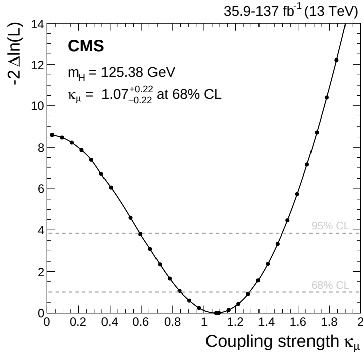
Figure 7-6. The observed profile likelihood ratio as a function of \kappa_\mu for m_H = 125.38 GeV.
