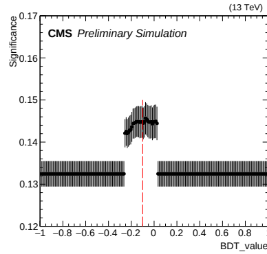
Figure 6-12. Scans for the BDT cut in the ZH channel. The BDT cut is chosen at -0.1.
