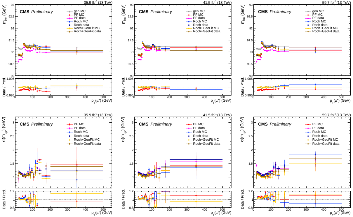
Figure 5-16. Muon calibration plots vs p_T(\mu^+) , for 2016 (left column), 2017 (middle column) and 2018 (right column). The top row shows the mean value of the Voigtian fit to the m_{\mu\mu} distribution, while the bottom row shows its experimental resolution. The p_T binning sculpts the shape of the m_{\mu\mu} peak, which leads to a jump at the p_T = 45 GeV in the plots.
