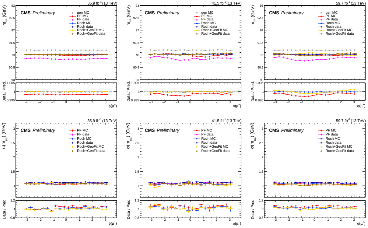
Figure 5-14. Muon calibration plots vs \phi(\mu^+) , for 2016 (left column), 2017 (middle column) and 2018 (right column). The top row shows the mean value of the Voigtian fit to the m_{\mu\mu} distribution, while the bottom row shows its experimental resolution.
