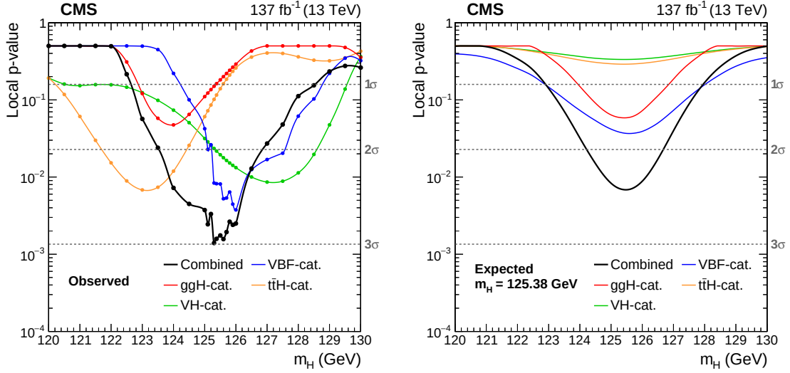
Figure 7-5. The local p -values as a function of different m_H hypotheses, for each individual categories as well as the overall combination. The left plot shows the observed p -values, each solid marker indicating a mass point, for which the observed p -values are computed. The right plot shows the expected p -values calculated using the background estimate from the S+B fit and injecting a signal with m_H = 125.38 GeV and \mu = 1 .
