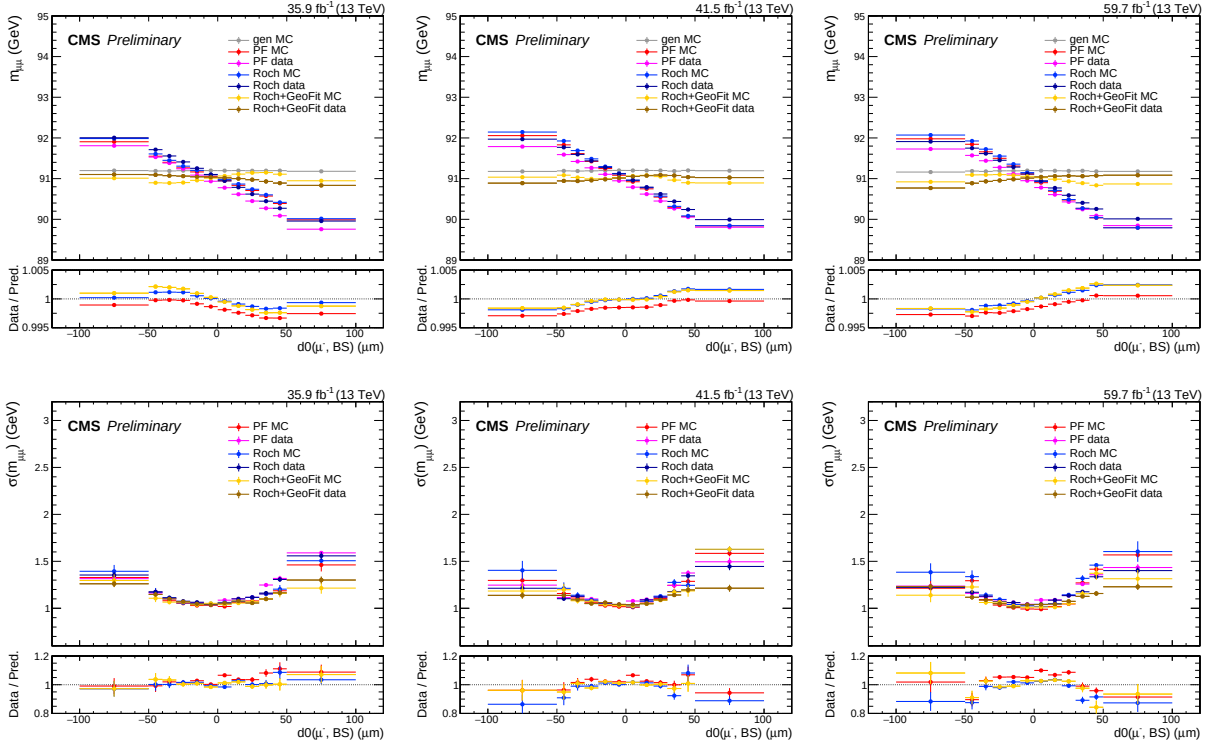
Figure 5-20. Muon calibration plots vs d_0(\mu^-) , for 2016 (left column), 2017 (middle column) and 2018 (right column). The top row shows the mean value of the Voigtian fit to the m_{\mu\mu} distribution, while the bottom row shows its experimental resolution.
