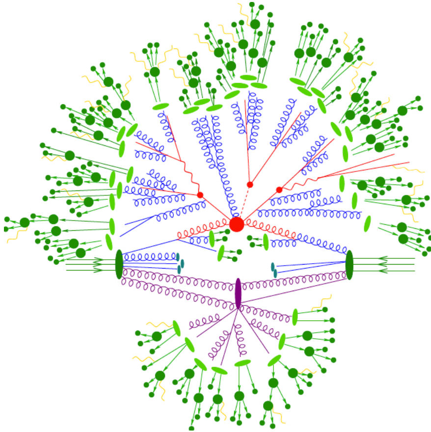
Figure 2-5. An illustration of the interactions in a pp collision. The primary interaction in this example is the Higgs boson production in association with a top quark pair, whose Feynman diagram is shown in 3-2. Plot taken from Ref. [7].
