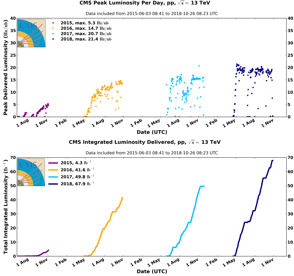
Figure 2-4. The evolutions of the peak instantaneous luminosity (upper plot) and the cumulative integrated luminosity (lower plot) of the LHC Run 2 (2015-2018) pp collisions. Plot taken from Ref. [6].
