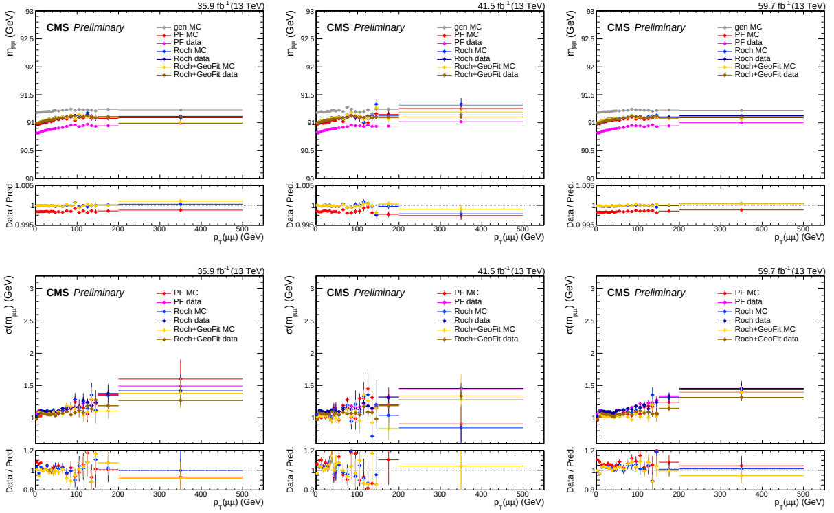
Figure 5-17. Muon calibration plots vs p_T(\mu\mu) , for 2016 (left column), 2017 (middle column) and 2018 (right column). The top row shows the mean value of the Voigtian fit to the m_{\mu\mu} distribution, while the bottom row shows its experimental resolution.
