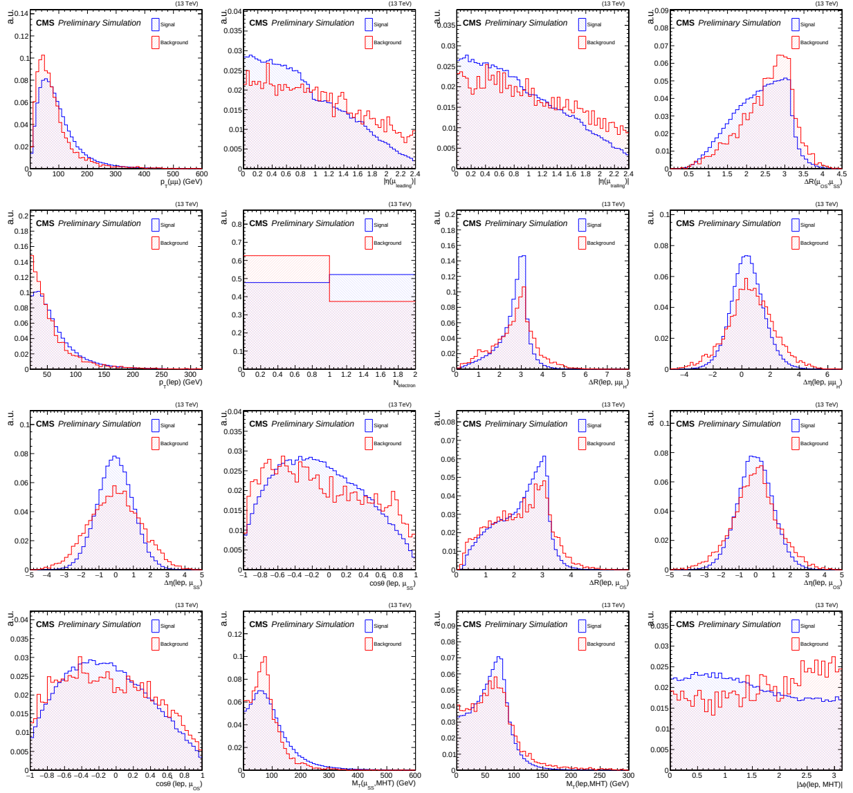
Figure 6-2. Input variables to the WH \rightarrow 3\ell BDT, with signal in blue and background in red.
