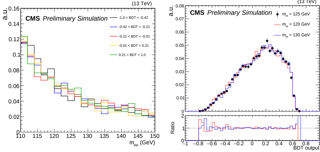
Figure 6-6. For the ZH BDT, the distribution of the dimuon mass shape in the background for five different BDT quantile (left), and the distribution of the BDT output for three different signal mass assumptions (right).
