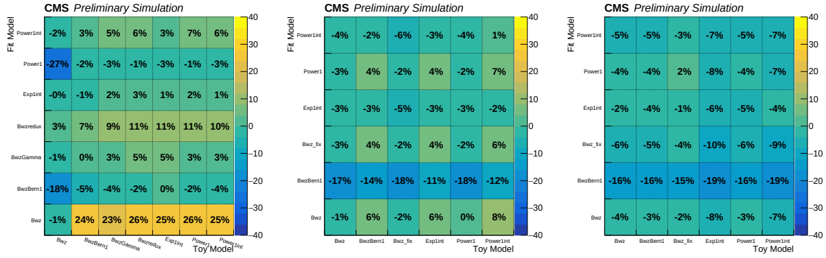
Figure 6-16. Bias in different BDT-based WH subcategories. The subcategories are: Cat1 BDT [-1.0, -0.1] (left), Cat2 BDT [-0.1, 0.3] (middle), Cat3 BDT [0.3, 1.0] (right). In the tables, the Power stands for a single "Power" function and the "PowerInt" stands for a single power function plus a constant.
