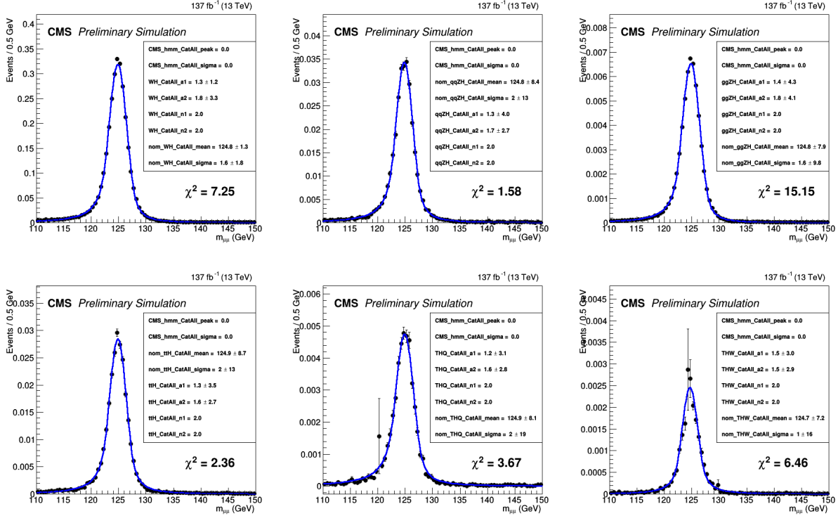
Figure 6-13. The signal modeling in the WH \rightarrow \ell + \mu\mu inclusive category. Considered signal modes are WH (top left), qqZH (top middle), ggZH (top right), ttH (bottom left), THQ (bottom middle), and THW (bottom right).
