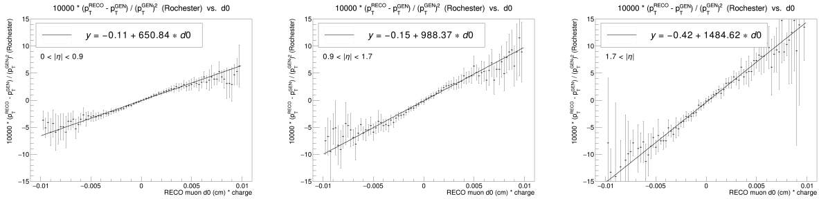
Figure 5-8. Plots for the (p_T^{reco} - p_T^{gen}) / (p_T^{gen})^2 vs d_0 correlation in the 2018 DY simulation, and the linear fits to them. Muon tracks are divided into three different |\eta| regions: |\eta| < 0.9 (left), 0.9 < |\eta| < 1.7 (middle), and 1.7 < |\eta| (right). Plots credit to Efe Yigitbasi.
