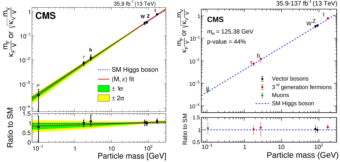
Figure 7-7. Left: A duplicate of Figure 1-3, taken from Ref. [2]. Summary of the CMS measurements on the Higgs coupling to fermions and bosons based on data recorded in 2016. Right: The coupling strength measurements updated with this H \rightarrow \mu\mu result.
