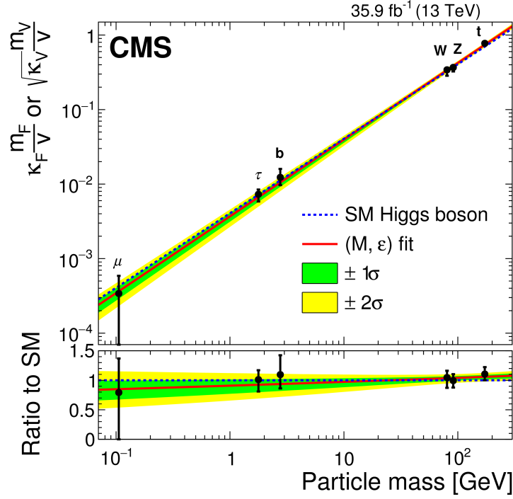
Figure 1-3. Summary of the CMS measurements on the Higgs coupling to fermions and bosons. Plot taken from [2].
