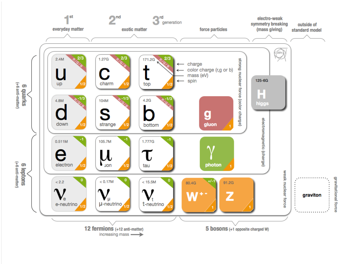
Figure 1-1. The Standard Model of particles physics: 12 elementary fermions and 5 elementary bosons. Plot taken from [1].
