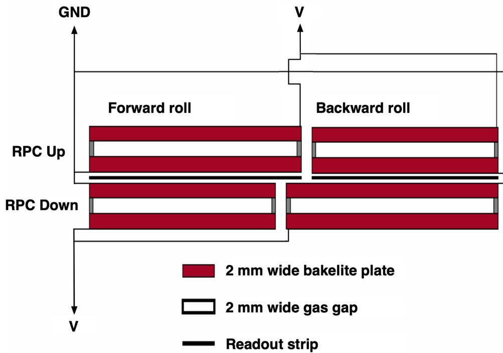
Figure 2-15. Schematic view of a double gap RPC. Plot taken from Ref. [17].
