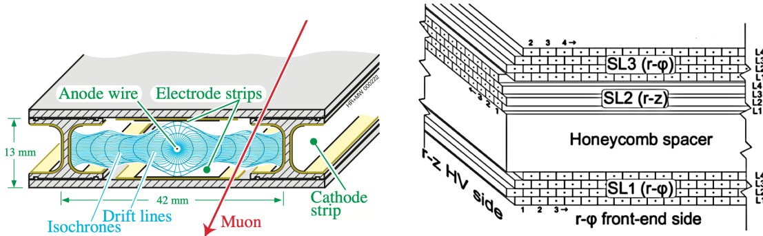
Figure 2-13. Left: sketch of a cell of the drift tube detector showing drift lines and isochrones. Right: schematic view of DT superlayers. Plot taken from Ref. [17].
