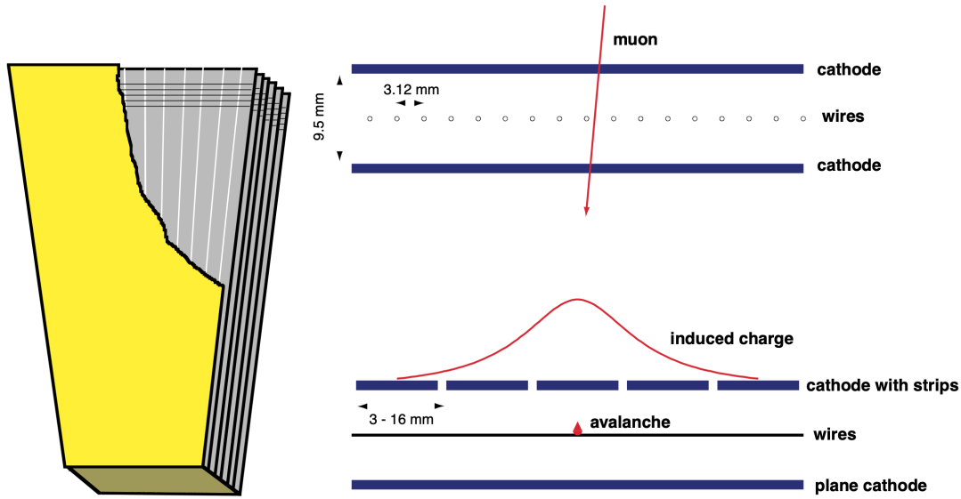
Figure 2-14. Left: layout of a CSC chamber showing arrangement of anode wires and cathode strips. Right: an illustration of the principle of CSC operation. Plots taken from Ref. [17].
