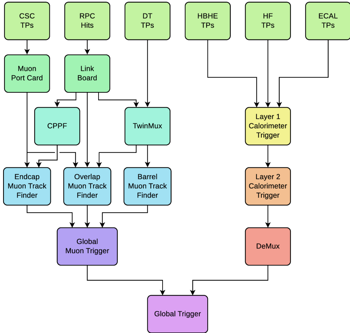
Figure 2-17. Diagram of the CMS Level-1 trigger structure during Run 2. Plot taken from Ref. [18].
