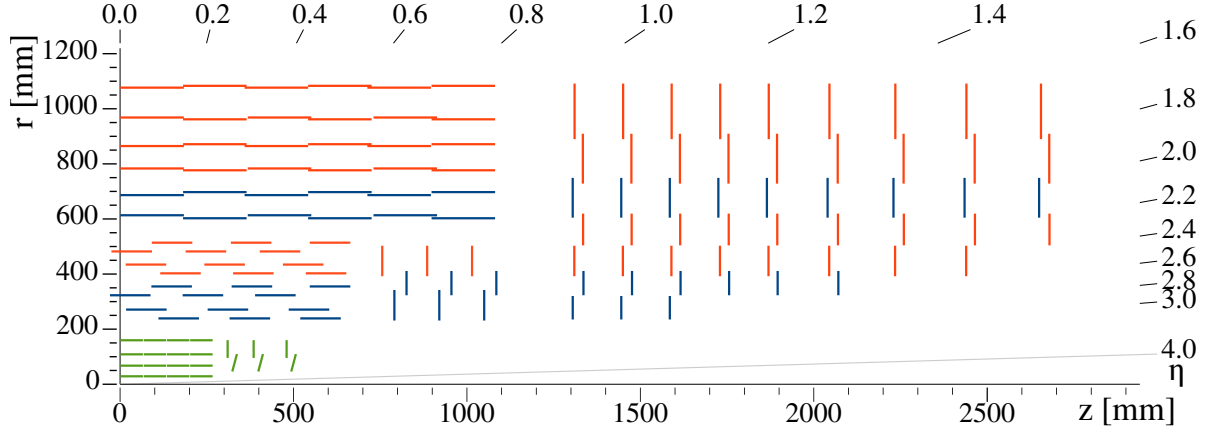
Figure 2-9. Sketch of one quarter of the Phase-1 CMS tracking system in r - z view. The pixel detectors are shown in green, while single-sided and double-sided strip modules are depicted as red and blue segments, respectively. Plot taken from Ref. [14].
