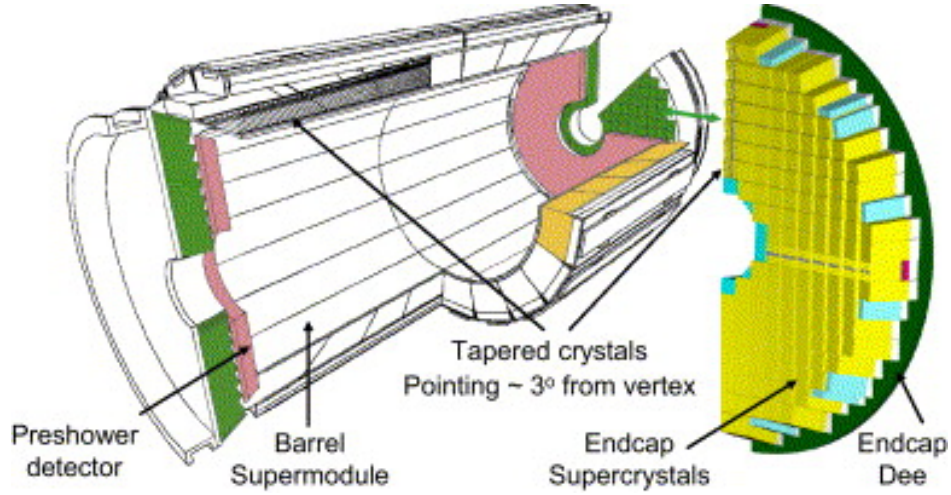
Figure 2-10. Schematic view of the CMS ECAL. Plot taken from Ref. [15].
