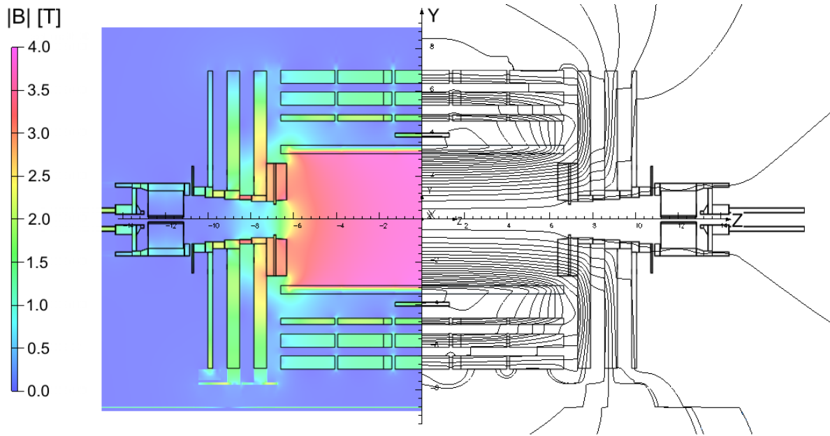
Figure 2-8. The magnetic field in CMS displayed in a longitudinal section, operating with a central field strength of 3.8 T. The field value |B| is shown on the left and the field lines are shown on the right. Plot taken from Ref. [13].
