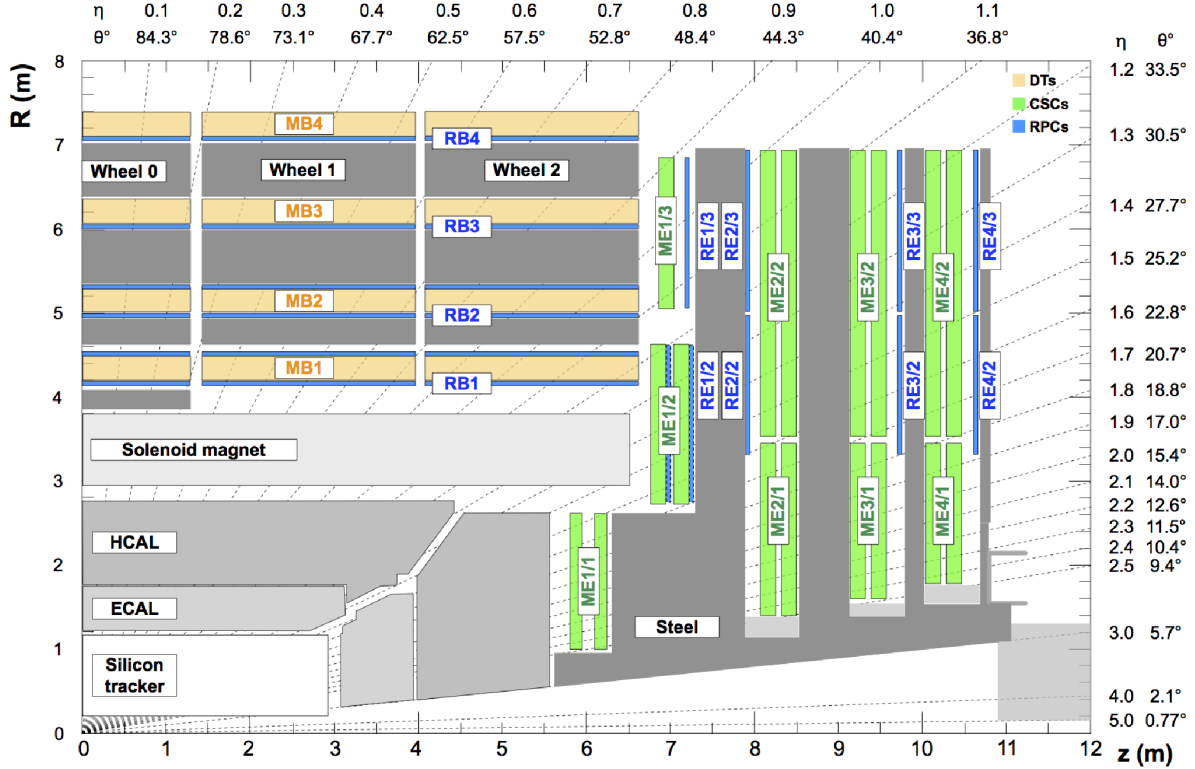
Figure 2-7. A longitudinal section view of the CMS detector, gridded with the CMS coordinates. Plot taken from Ref. [12].
