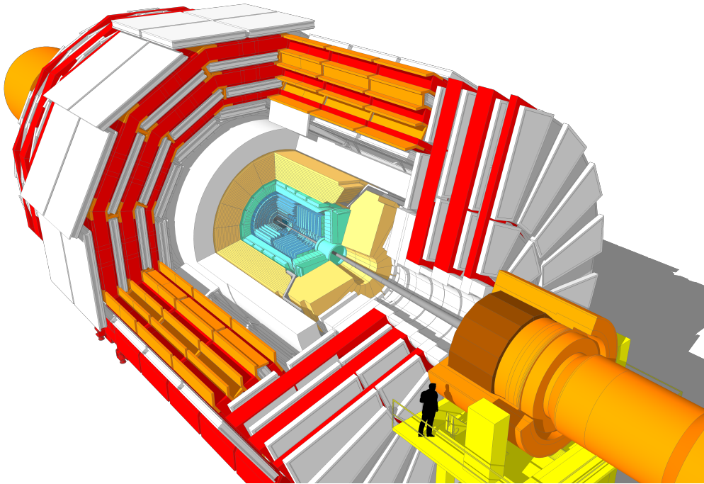
Figure 2-6. A cutaway diagram of the CMS detector. The design is specified to a design stage called the Phase-1 detector upgrade [8, 9, 10]. Plot taken from Ref. [11].
