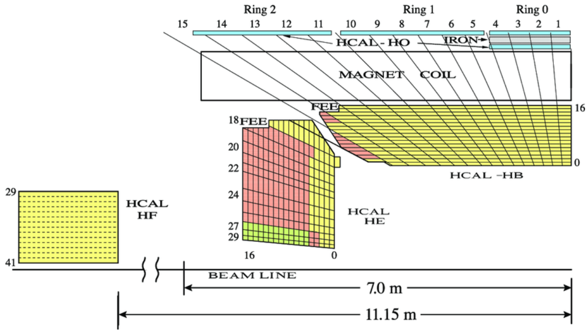
Figure 2-11. Schematic view of one quarter of the Phase-1 CMS HCAL in r - z view, showing the locations of the HB, HE, HO, and HF calorimeters. Plot taken from Ref. [9].
