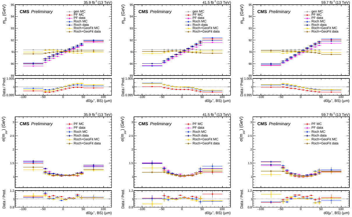
Figure 5-19. Muon calibration plots vs d_0(\mu^+) , for 2016 (left column), 2017 (middle column) and 2018 (right column). The top row shows the mean value of the Voigtian fit to the m_{\mu\mu} distribution, while the bottom row shows its experimental resolution.
