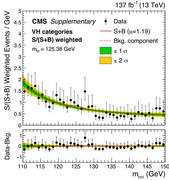
Figure 6-20. Post-fit m_{\mu\mu} distribution of the weighted combination of all WH and ZH subcategories. Subcategories are weighted proportionally to S/(S+B) ratio. The upper panel in the plots shows the distribution of observed data and the shape of the signal-plus-background fit. The lower panel in the plots shows the residual distribution after subtracting the background component in the fits. The green and yellow bands show the one and two standard deviation of the background component uncertainty.
