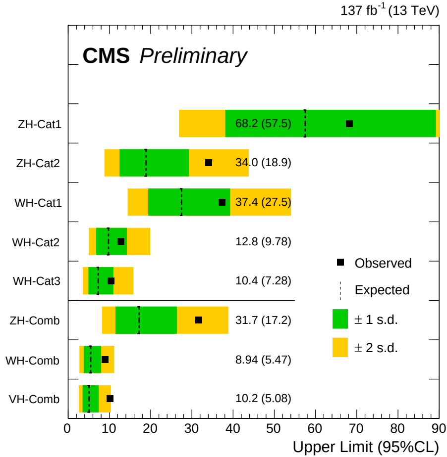
Figure 6-22. The 95% CL upper limits on the signal strength in subcategories and combinations. Observed (expected) values are marked in the plot.
