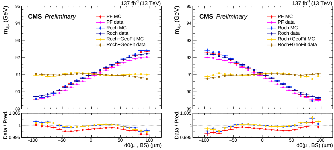
Figure 5-9. Plots showing the p_T dependence on the d_0 value with different stages of muon correction. The plots compare the Z \rightarrow \mu\mu peak in data and simulation for three years (2016-2018) combined. All positively charged muons are put in the left plot and all negatively charged ones are put in the right plot. The p_T - d_0 dependence is reversed for positive and negative muons.
