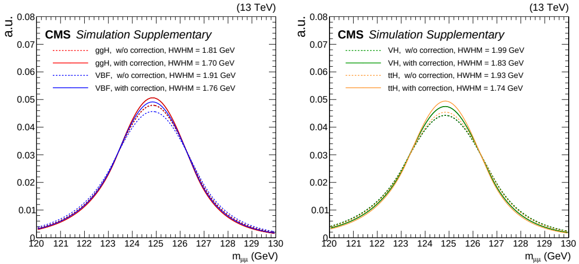
Figure 5-10. Plots showing the GeoFit correction improvement on the four main H \rightarrow \mu\mu signal modes, ggH and VBF plotted on the left, and VH and t\bar{t}H plotted on the right. The plots are made combining the expected signal in all three years of data-taking (2016-2018). The relative improvements on m_{\mu\mu} resolution for ggH, VBF, VH, and t\bar{t}H modes are, respectively, 6.1%, 7.8%, 8.0%, and 9.8%.
