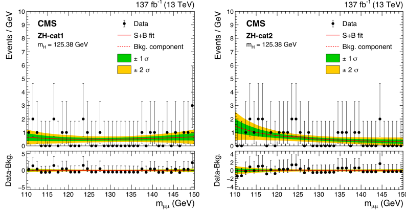
Figure 6-19. Post-fit m_{\mu\mu} distribution of the ZH subcategories. The subcategories are: Cat1 BDT [-1.0, -0.1] (left), Cat2 BDT [-0.1, 1.0] (right). The upper panel in the plots shows the distribution of observed data and the shape of the signal-plus-background fit. The lower panel in the plots shows the residual distribution after subtracting the background component in the fits. The green and yellow bands show the one and two standard deviation of the background component uncertainty.
