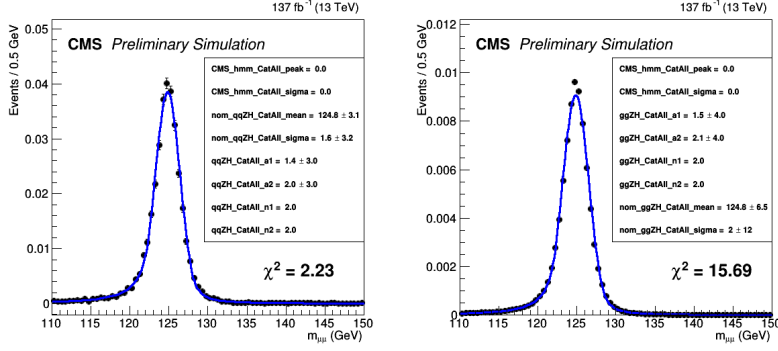
Figure 6-14. The signal modeling in the ZH \rightarrow \ell\ell + \mu\mu inclusive category. Considered signals modes are qqZH (left) and ggZH (right).
