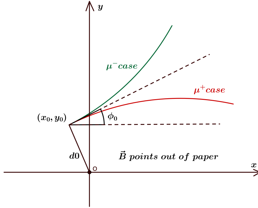
Figure 5-3. Scheme of the d_0 definition in CMS. The (x_0, y_0) is the coordinate of a point near the vertex in the frame where the vertex is at (0, 0) , and the \phi_0 is the azimuthal angle of the track at (x_0, y_0) .
