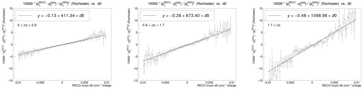
Figure 5-6. Plots for the (p_T^{reco} - p_T^{gen})/(p_T^{gen})^2 vs d_0 correlation in the 2016 DY simulation, and the linear fits to them. Muon tracks are divided into three different |\eta| regions: |\eta| < 0.9 (left), 0.9 < |\eta| < 1.7 (middle), and 1.7 < |\eta| (right). Plots credit to Efe Yigitbasi.
