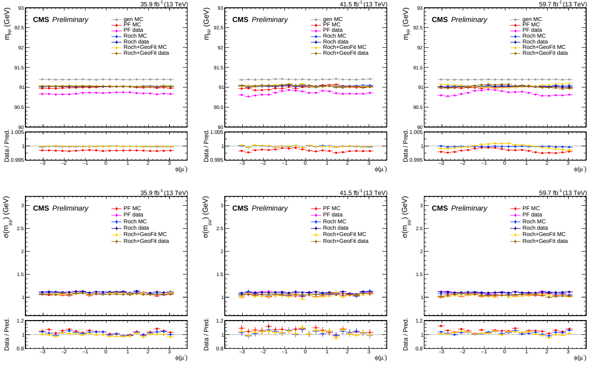
Figure 5-15. Muon calibration plots vs \phi(\mu^-) , for 2016 (left column), 2017 (middle column) and 2018 (right column). The top row shows the mean value of the Voigtian fit to the m_{\mu\mu} distribution, while the bottom row shows its experimental resolution.
