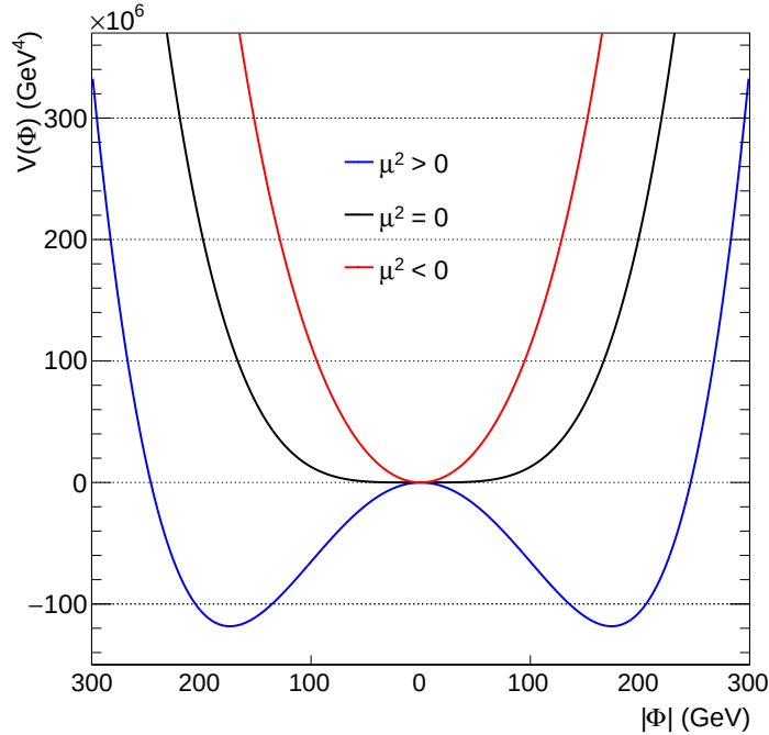
Figure 1-2. The shape of the Higgs potential with different \mu^2 parameter configurations.
