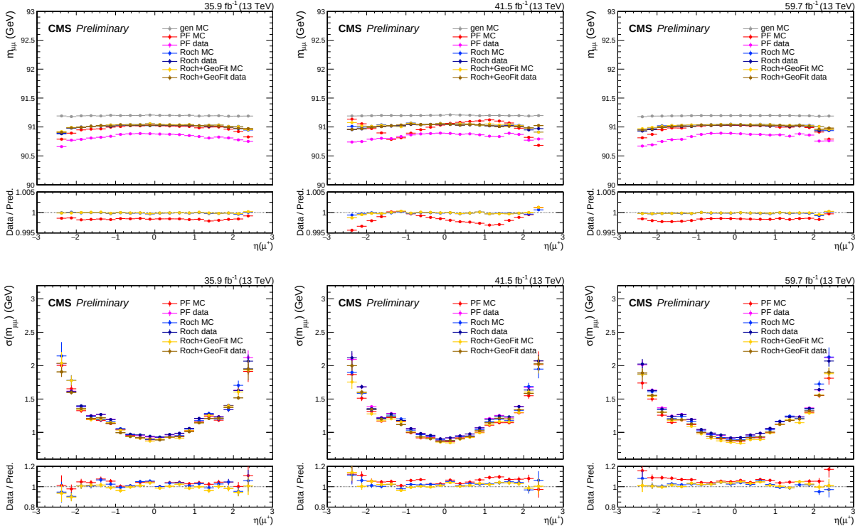
Figure 5-13. Muon calibration plots vs \eta(\mu^+) , for 2016 (left column), 2017 (middle column) and 2018 (right column). The top row shows the mean value of the Voigtian fit to the m_{\mu\mu} distribution, while the bottom row shows its experimental resolution.
