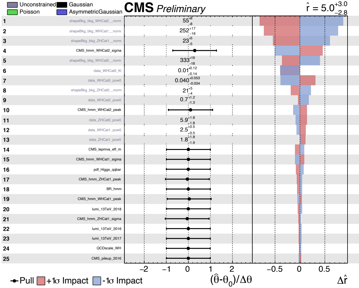
Figure 6-21. Impacts of the nuisance parameters \theta on the signal strength \hat{r} . Parameter names in black are systematic uncertainties, which are Gaussian-constrained to their pre-fit uncertainties. Parameter names in gray are shape and normalization parameters, which do not have pre-fit constraints. (\hat{\theta} - \theta_0)/\Delta\theta shows the pull of each nuisance parameter, while \Delta\hat{r} is its impact on signal strength. Unconstrained parameters do not have pre-fit assumptions and therefore no pulls. The best-fit values of them are shown in the place of pulls.
