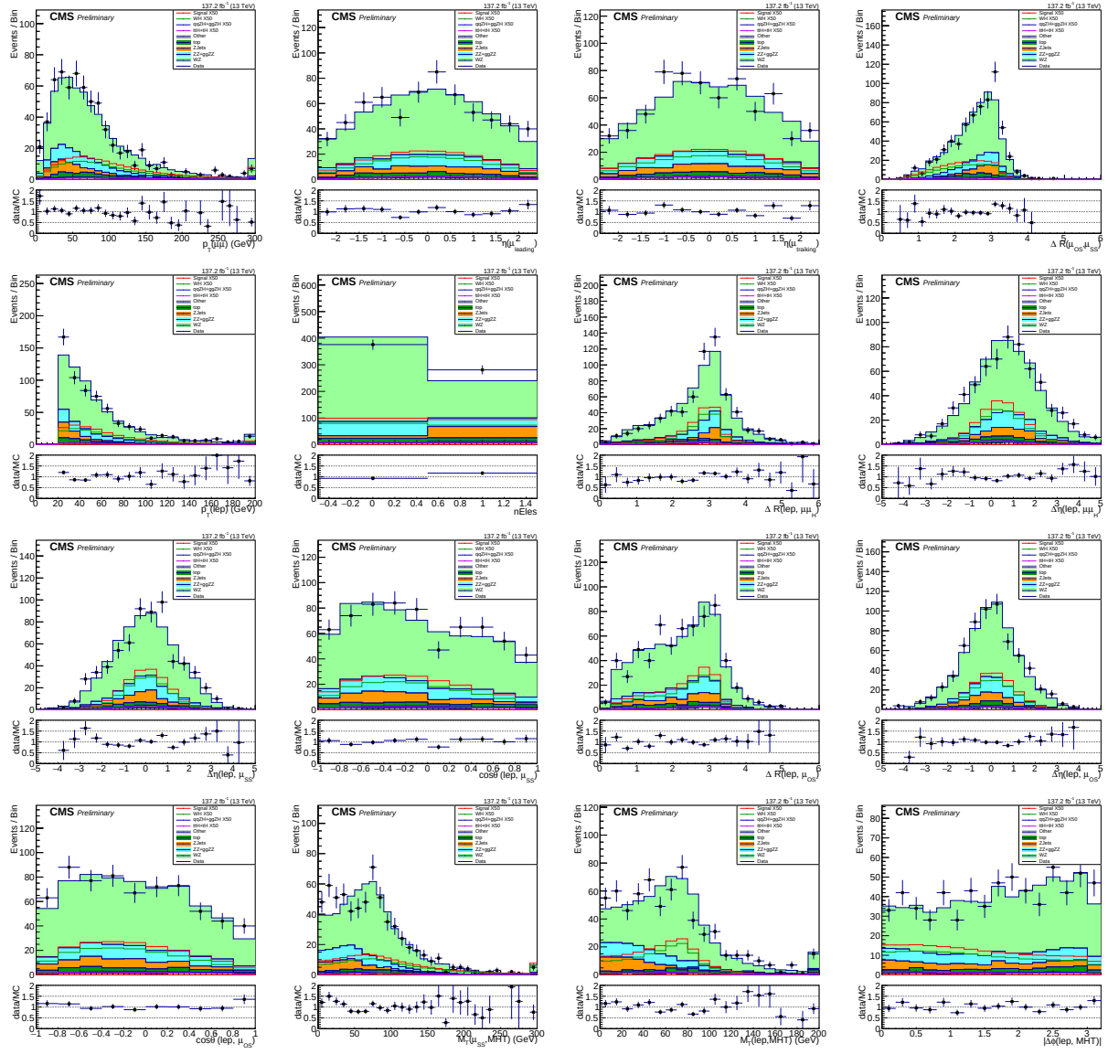
Figure 6-8. Input variables to the WH BDT in full Run 2 in the signal region 110 \text{ GeV} < m_{\mu\mu} < 150 \text{ GeV} .
