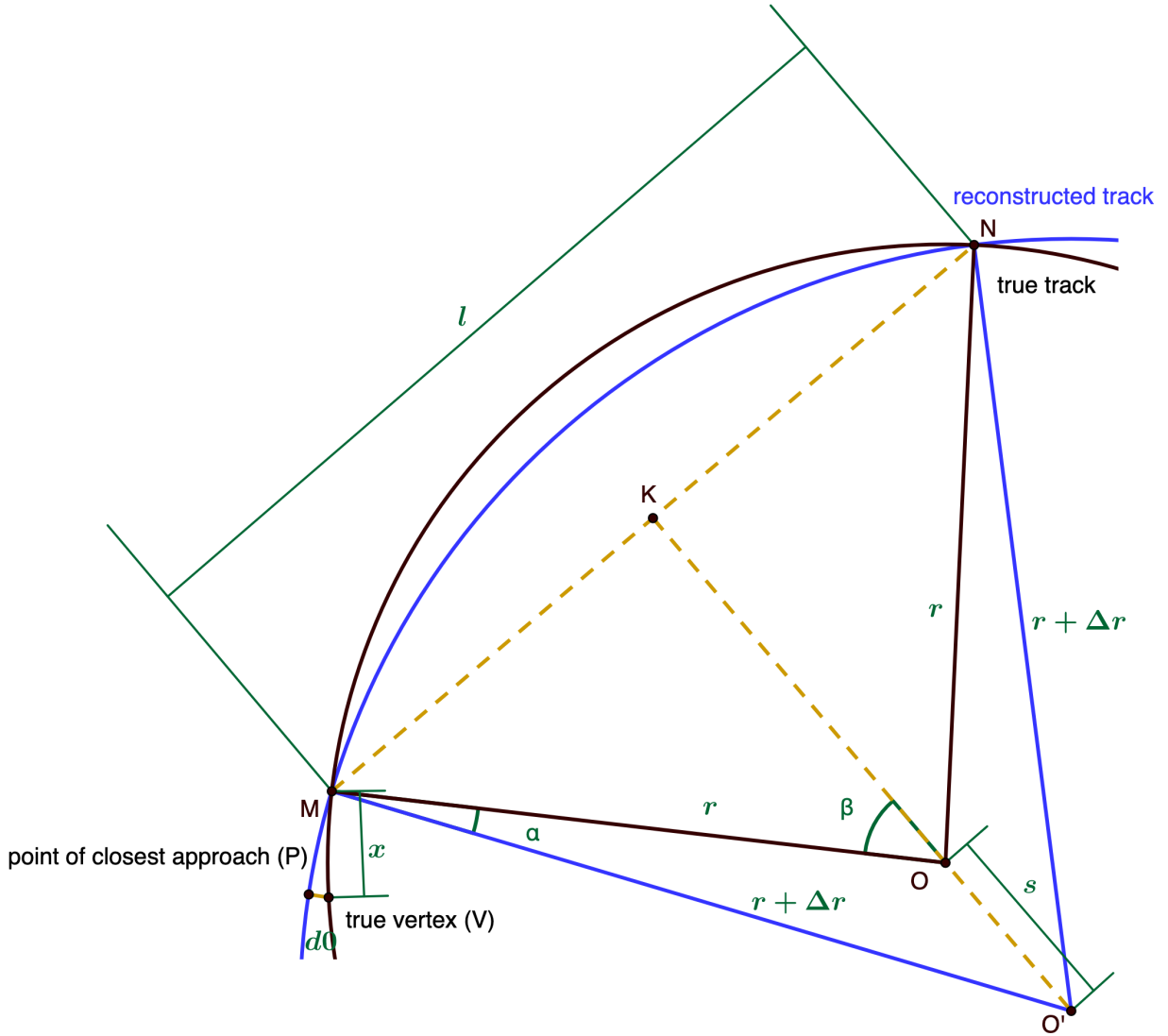
Figure 5-4. Scheme of the track geometry in the transverse plane. The blue lines show the geometry of the reconstructed track, compared to the black lines, which are the geometry of the true track. The difference between the blue track and black track is exaggerated in this scheme. The blue track and the black track must intersect at two points. l is the distance between the two intersections, and x is the distance between the true vertex and the first intersection. s is the distance between the circular centers of the two tracks.
