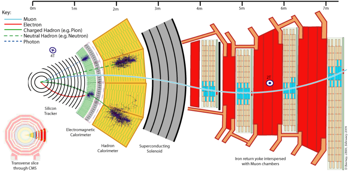
Figure 4-1. A transverse view of the CMS detector layout in the barrel region, with illustrations of the interactions between different particles and different detector components. Plot taken from Ref. [19].
