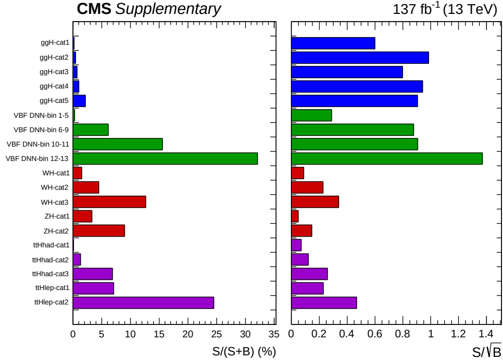
Figure 7-2. Expected S/(S+B) and S/\sqrt{B} in different subcategories, where S and B indicate the number of expected signal and background events, respectively.
