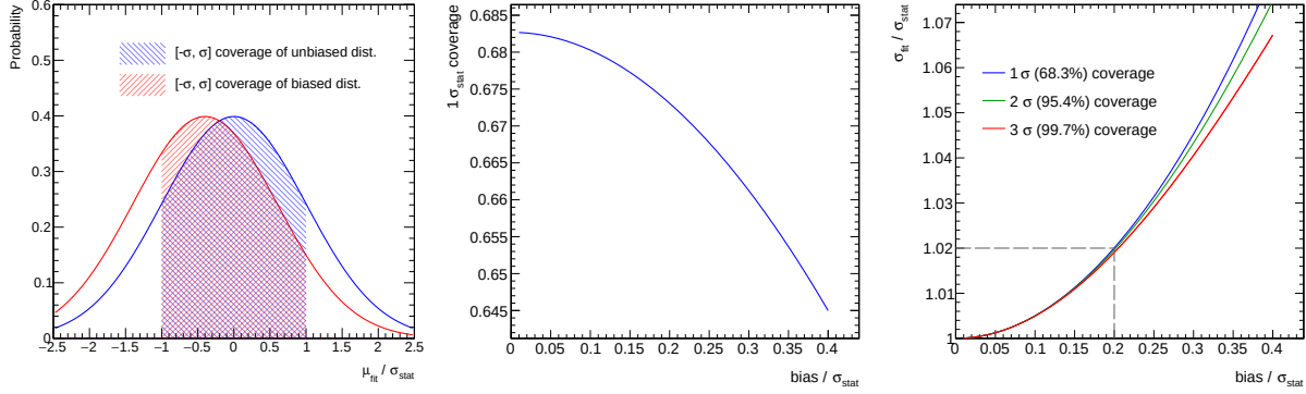
Figure 6-15. Schemes on how the bias affects the uncertainty on the signal strength measurement. The left plot is an illustration of the [-\sigma, \sigma] coverage of the biased signal strength measurement. The middle plot shows this coverage becomes less as the bias gets larger. The right plot shows how the bias impacts the best fit signal strength uncertainty \sigma_{fit} . The gray dash lines in the right plot indicates the conventional acceptable range of the bias in this analysis.
