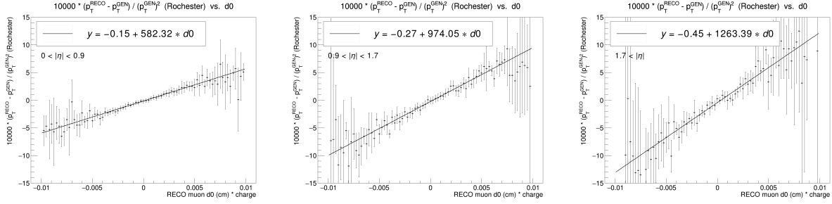
Figure 5-7. Plots for the (p_T^{reco} - p_T^{gen}) / (p_T^{gen})^2 vs d_0 correlation in the 2017 DY simulation, and the linear fits to them. Muon tracks are divided into three different |\eta| regions: |\eta| < 0.9 (left), 0.9 < |\eta| < 1.7 (middle), and 1.7 < |\eta| (right). Plots credit to Efe Yigitbasi.
