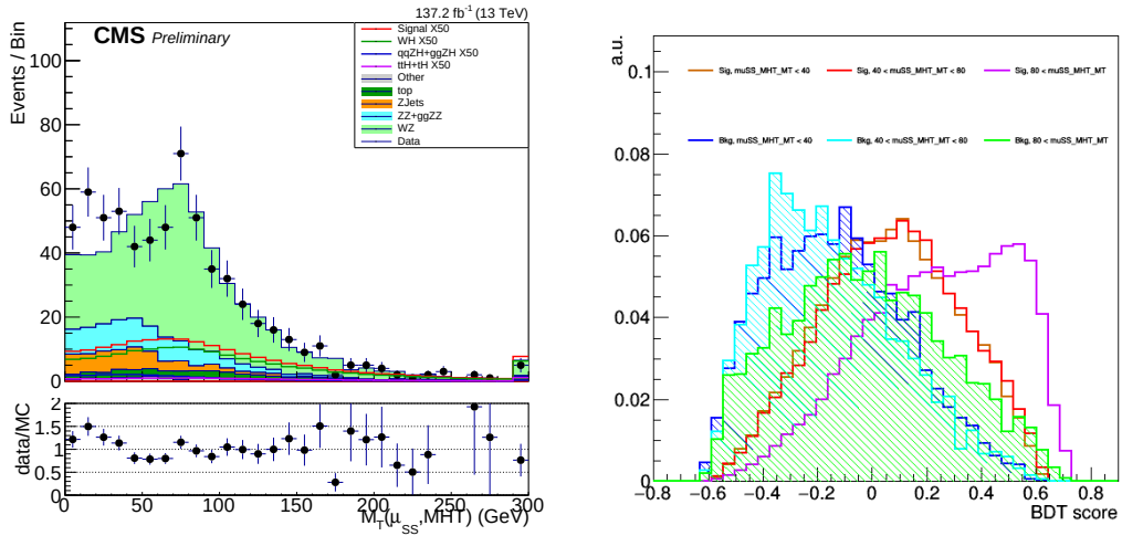
Figure 6-10. The input variable M_T(\mu_{SS}, MHT) to the WH BDT (left), and the BDT output for signal and background in different M_T(\mu_{SS}, MHT) bins (right). A mild disagreement is seen between the simulation and data in the low bins of M_T(\mu_{SS}, MHT) , while the BDT is not sensitive to the M_T(\mu_{SS}, MHT) values in that region.
