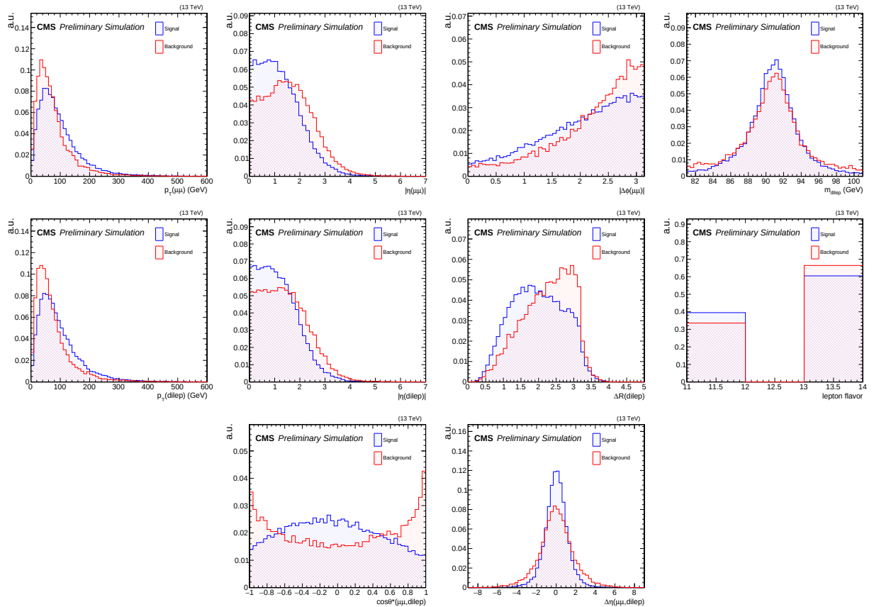
Figure 6-4. Input variables to the ZH \rightarrow 4\ell BDT, with signal in blue and background in red.
