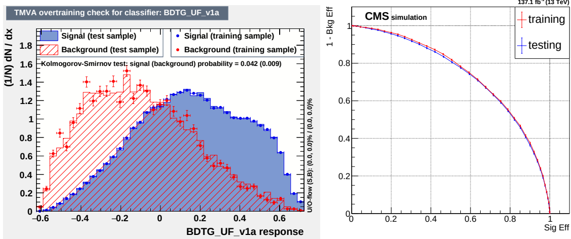
Figure 6-1. Plots of the performance of the WH \rightarrow 3\ell . On the left, the BDT output score, with signal in blue and background in red. On the right, the receiver operating characteristic (ROC) curve, with training sample in red and testing sample in blue. A slight over-training is observed in the region of low signal efficiency, because of the fluctuation in background. As will be shown in Fig. 6-5, the BDT does not sculpt the shape of m_{\mu\mu} .
