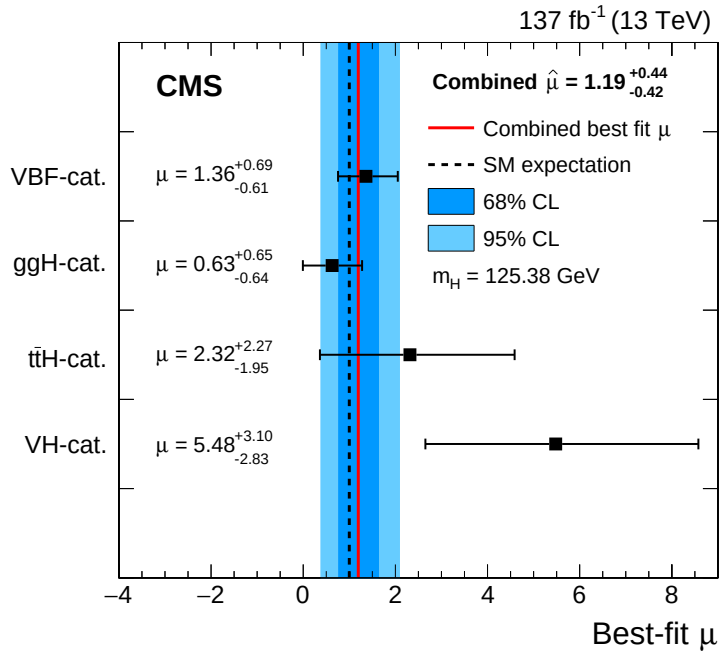
Figure 7-3. Signal strength modifiers measured for m_H = 125.38 GeV in each production category (black points) are compared to the result of the combined fit (solid red line) and the SM expectation (dashed gray line).
