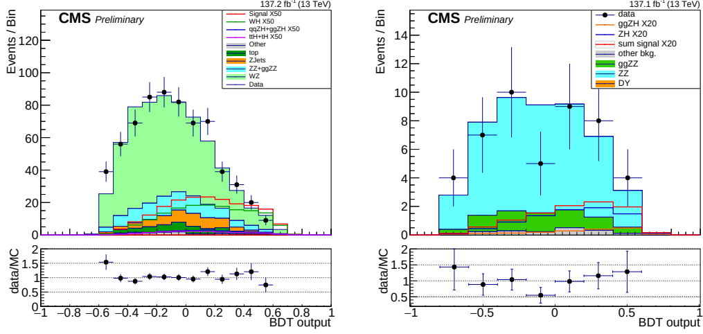
Figure 6-7. The WH BDT output (left) and the ZH BDT output (right) in full Run 2 in the signal region 110 \text{ GeV} < m_{\mu\mu} < 150 \text{ GeV} .
