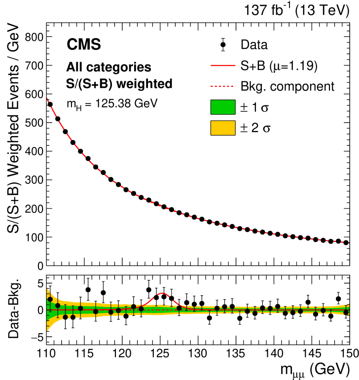
Figure 7-4. Post-fit m_{\mu\mu} distribution of the weighted combination of all categories. Subcategories are weighted proportionally to S/(S+B) ratio. The lower panel in the plots shows the residual distribution after background subtraction. The green and yellow bands show the one and two standard deviation of the background component uncertainty.
