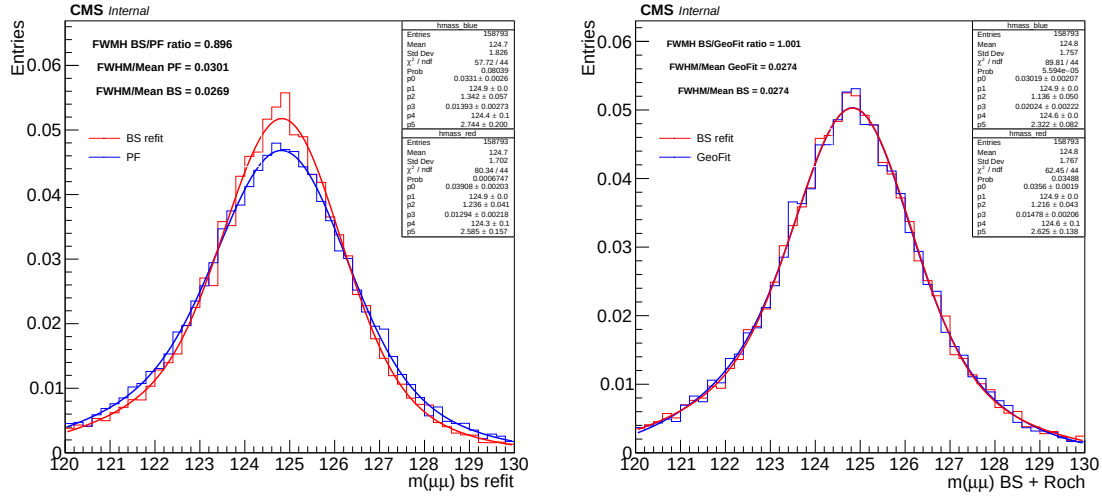
Figure 5-12. Plots of the m_{\mu\mu} shape of the 2018 ggH simulation sample, comparing different muon correction methods. The left plot shows the m_{\mu\mu} distribution calculated with muon tracks refitted with the additional BS constraint, compared with the particle flow shape (left plot). The Rochester correction is not applied in the left plot for both the red and the blue lines. The right plot shows the m_{\mu\mu} distribution from the refit method, with the Rochester correction applied, compared with the shape from GeoFit correction + Rochester correction (right plot). Plots credit to Pierluigi Bortignon.
