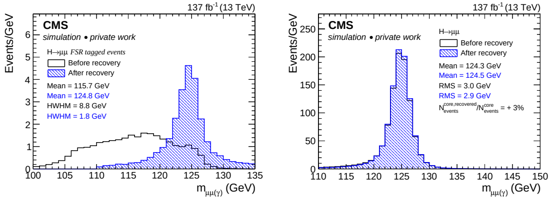
Figure 5-1. Performance of the FSR recovery in the simulated H \rightarrow \mu\mu events. The m_{\mu\mu} before and after the FSR recovery are shown for the events that contain at least one FSR photon (left), and for the inclusive signal events (right). Plot taken from Ref. [20].
