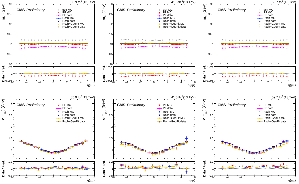
Figure 5-18. Muon calibration plots vs \eta(\mu\mu) , for 2016 (left column), 2017 (middle column) and 2018 (right column). The top row shows the mean value of the Voigtian fit to the m_{\mu\mu} distribution, while the bottom row shows its experimental resolution.
