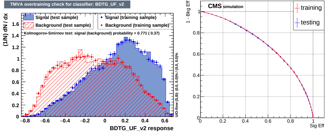
Figure 6-3. Plots of the performance of the ZH \rightarrow 4\ell BDT. On the left, the BDT output score, with signal in blue and background in red. On the right, the receiver operating characteristic (ROC) curve, with training in red and testing in blue.
