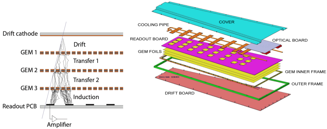
Figure 2-16. Left: schematic view showing the GEM structure and its working principle. Right: exploded view of the mechanical design of GEM. Plot taken from Ref. [16].
