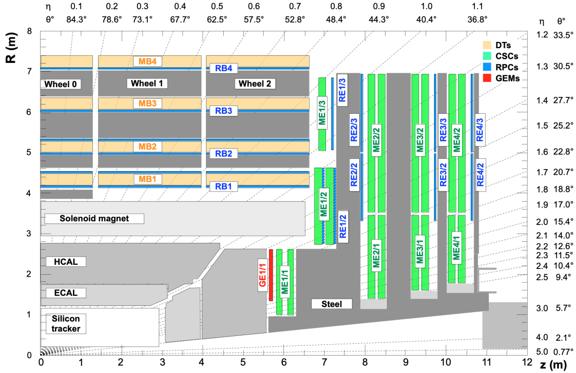
Figure 2-12. A longitudinal section view of the current CMS detector specifying the locations of muon chambers. This plot is different from Figure 2-7 only by the GEM detector installed in 2019/2020. Plot taken from Ref. [16].
