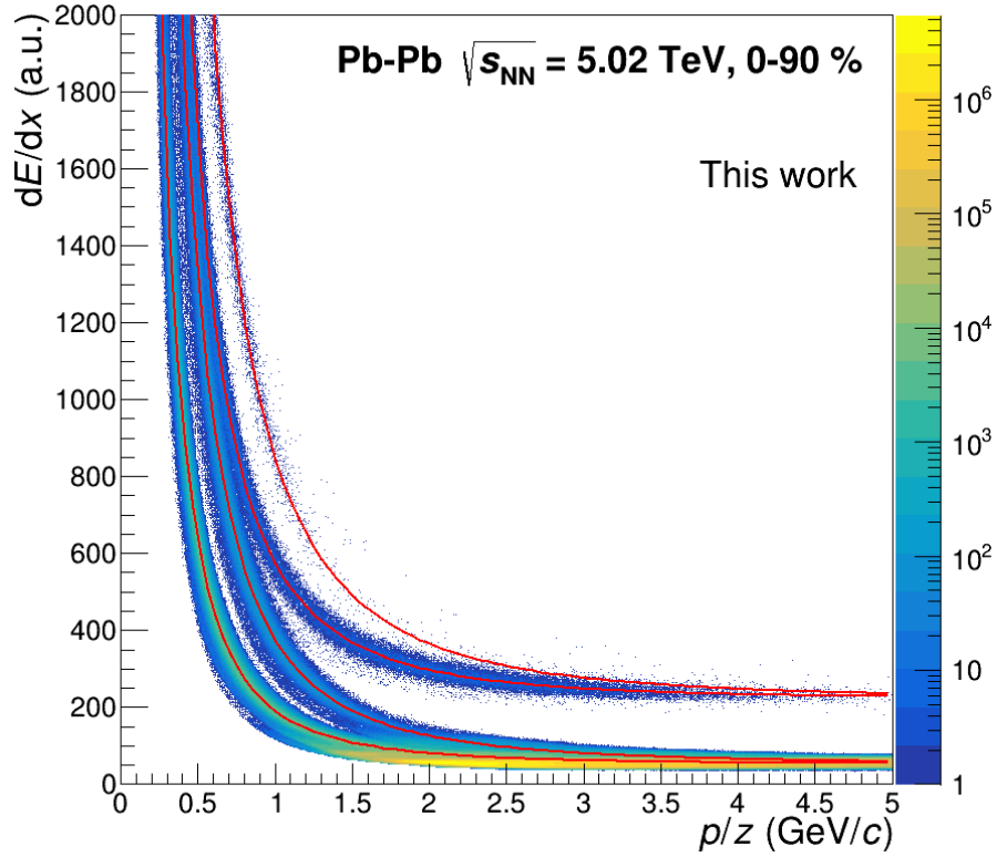
Figure 4.3: Specific energy loss in the TPC versus rigidity (from left to right) for deuterons, tritons, ^3\text{He} and ^4\text{He} in Pb–Pb collisions at \sqrt{s_{NN}} = 5.02 \text{ TeV} for particles and antiparticles together (LHC18q+r, 0-90 %). The red lines represent the fitted Bethe-Bloch curves.
