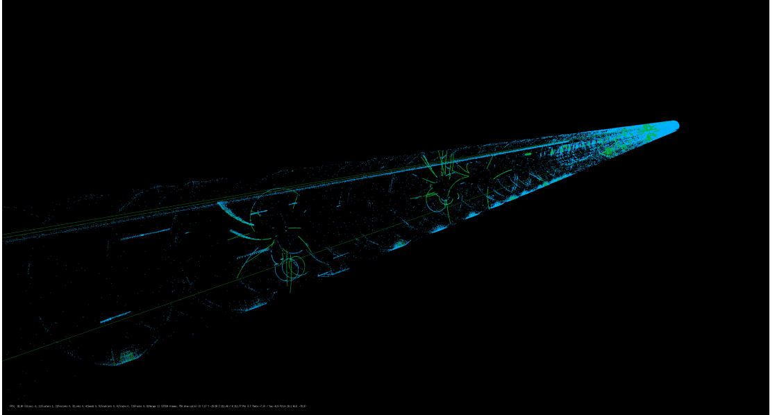
Figure 6.7: Event display of the GEM TPC with continuous readout.
