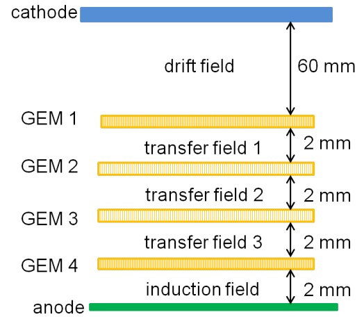
(b) Schematic diagram of a stack of four GEM foils.
