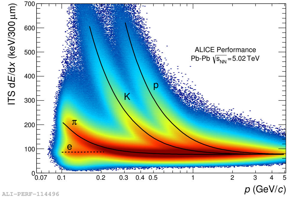
Figure 3.5: Specific energy loss ( dE/dx ) in the ITS versus momentum during the Pb–Pb data-taking period of 2015 [54].
