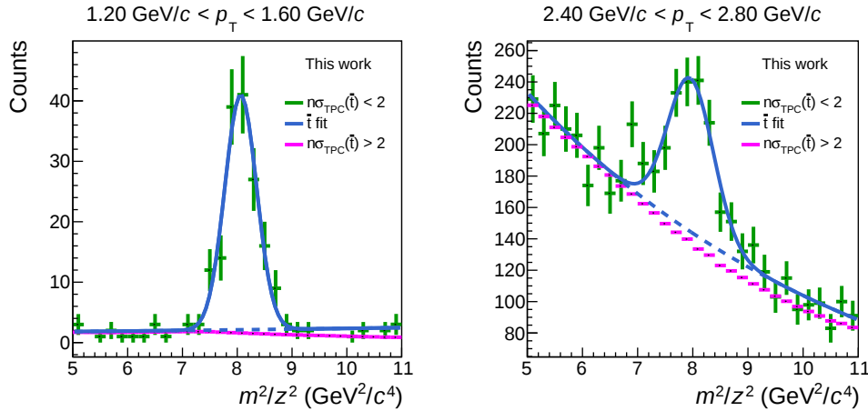
Figure 4.8: m^2/z^2 distribution of antitritons ( |n\sigma_{\text{TPC}}(\hat{t})| < 2 , green) with fit (exponential + gauss · exponential, blue) and scaled background ( |n\sigma_{\text{TPC}}(\hat{t})| > 2 , magenta) exemplary for two p_T bins of the 0-10 % centrality interval.
