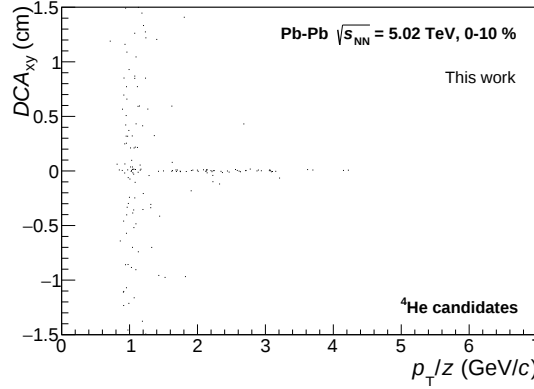
Figure 4.15: DCA_{xy} distribution versus p_T/z for ^4\text{He} in the 0-10 % centrality interval. The broad distribution at low p_T/z indicates the large contribution from material knock-out (spallation).
