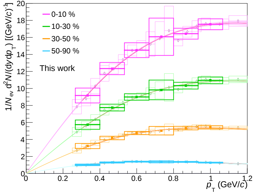
(a) Rebinned proton spectra to match the (anti)triton p_T bins. The first point of each averaged centrality interval was set to the fit value as the measurement only starts from 0.3 GeV/ c .
