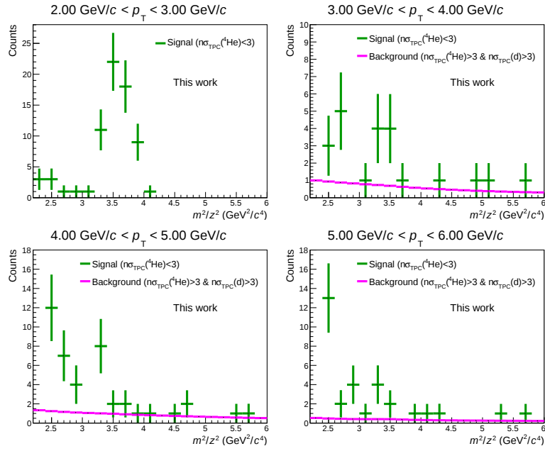
Figure 4.18: m^2/z^2 distribution of ^4\text{He} ( |n\sigma_{\text{TPC}}(^4\text{He})| < 3 , green) and scaled background ( |n\sigma_{\text{TPC}}(^4\text{He})| > 3 and |n\sigma_{\text{TPC}}(d)| > 3 , magenta) for the different p_T bins in the 0-10% centrality interval. In the first p_T bin the contribution from material knock-out is visible.
