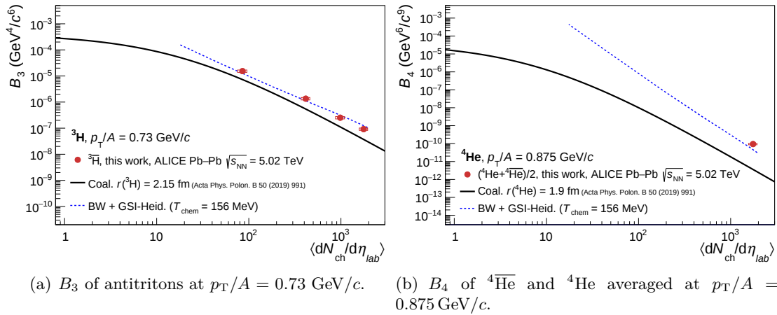
Figure 5.11: Measured coalescence parameters versus charged-particle multiplicity compared to coalescence and BW + GSI-Heidelberg models.
