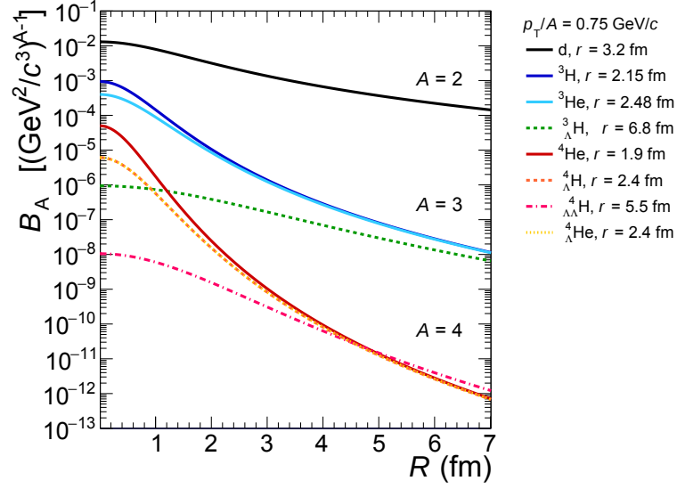
Figure 2.4: B_A calculation for A = 2, 3 and 4 for various (hyper)nuclei as a function of the source radius for p_T/A = 0.75 \text{ GeV}/c . The radius of the nucleus used for the calculation is indicated in the legend [26].
