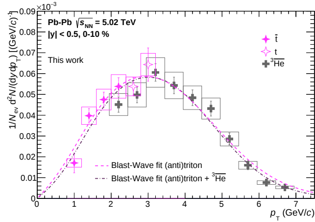
(c) Comparison of the (anti)triton BW fit to a BW fit of (anti)triton with ALICE preliminary {}^3\text{He} [70, 71] combined in the 0-10 % centrality interval.
