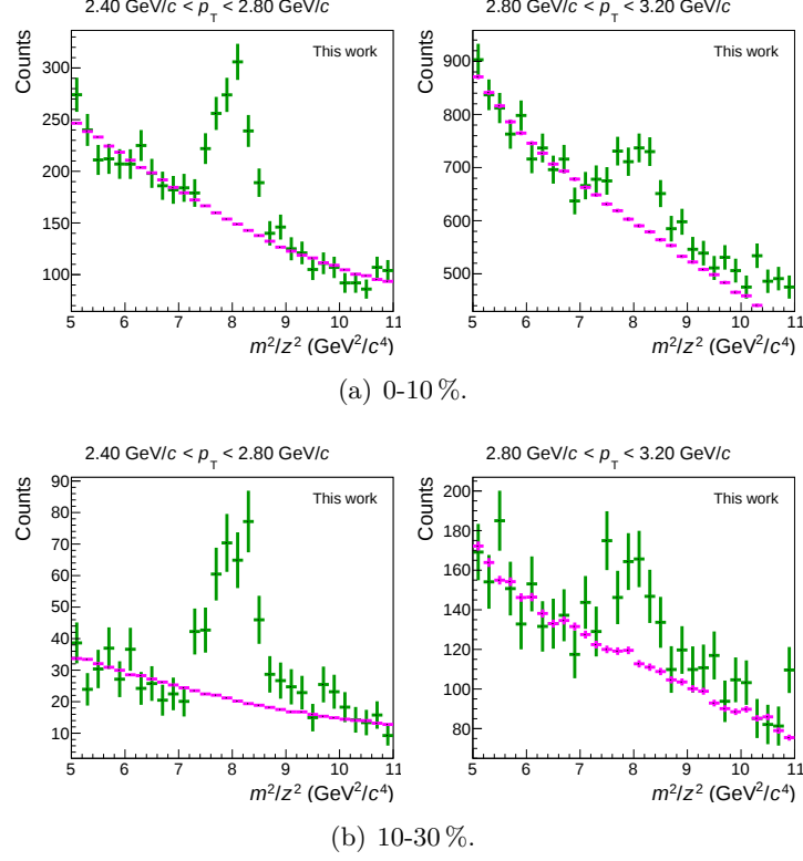
Figure 4.11: m^2 distribution of tritons ( |\sigma_{\text{TPC}}(t)| < 2 , green) and scaled background ( |\sigma_{\text{TPC}}(t)| > 2 , magenta) for the different p_T bins in the 0-10 % (top) and 10-30 % (bottom) centrality interval.
