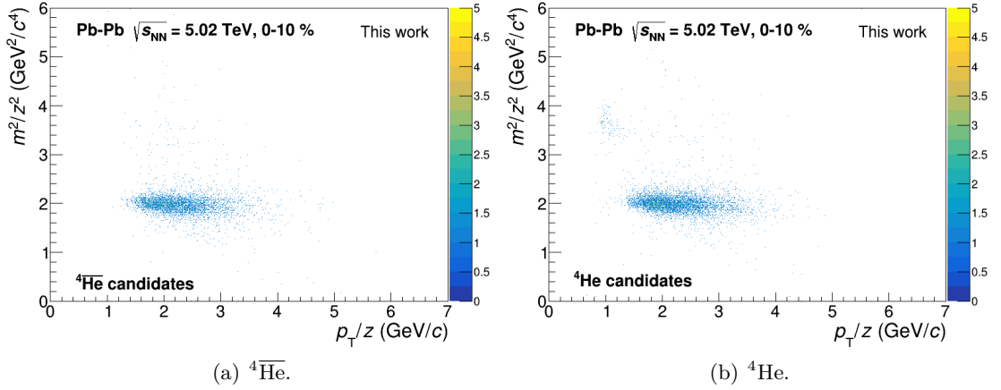
Figure 4.14: m^2/z^2 distribution of the TOF detector versus the transverse momentum in the 0-10 % centrality interval for ^4\overline{\text{He}} on the left and ^4\text{He} on the right ( m_{^4\text{He}}^2/z^2 = 3.475 \text{ GeV}^2/c^4 ). A |n\sigma_{\text{TPC}}(^4\text{He})| < 3 selection around the (anti) ^4\text{He} band in the TPC has been done before. Some background is visible over the m^2 range. In comparison to the ^4\overline{\text{He}} on the left side, on the right side there is a significant contribution visible at low p_T/z from knocked-out ^4\text{He} coming from the beam pipe or the detector material. However, the main contribution visible is the (anti) ^3\text{He} at 2 \text{ GeV}^2/c^4 , well separated from the (anti) ^4\text{He} in the TOF mass.
