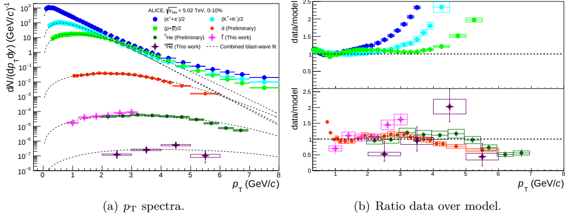
Figure 5.7: Combined Blast-Wave fit of several particle species, including \bar{t} and {}^4\bar{\text{He}} , in Pb–Pb collisions at \sqrt{s_{\text{NN}}} = 5.02 TeV in the 0–10% centrality interval.
