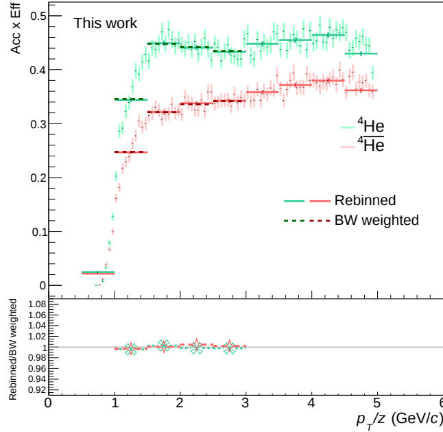
Figure 4.23: Acceptance x Efficiency versus p_T/z for ^4\text{He} (green markers) and \bar{^4\text{He}} (red markers) in the 0-10 % centrality interval. The Acc x Eff is rebinned in the bins of the analysis (solid lines) and weighted with a Blast-Wave shape (dashed lines). In the lower panel the ratio between the rebinned and the weighted Acc x Eff is shown.
