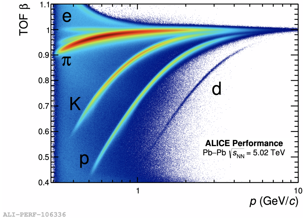
Figure 3.7: TOF \beta versus momentum measured during the Pb–Pb data-taking period of 2015 [55].
