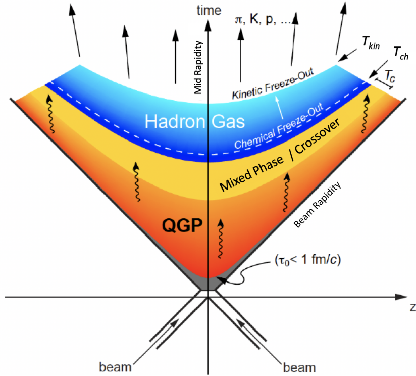
Figure 1.6: Space-time diagram of a heavy-ion collision in the center-of-mass system [10].
