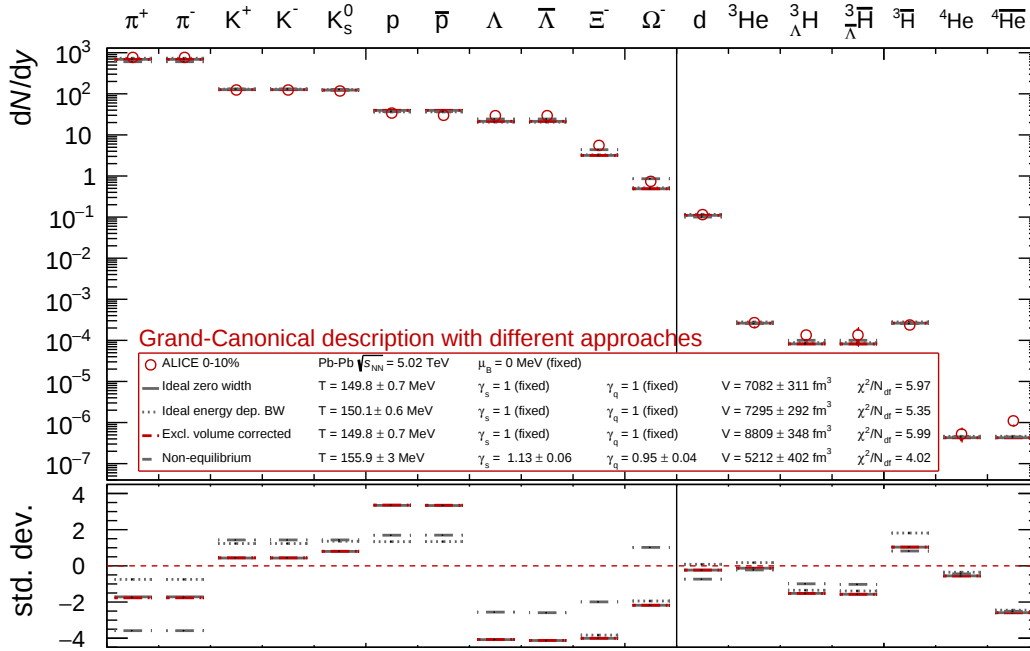
Figure 5.8: p_T -integrated production yields dN/dy of different particle species, including \bar{t} and ^4\overline{\text{He}} , in Pb-Pb collisions at \sqrt{s_{\text{NN}}} = 5.02 TeV in the 0-10 % centrality interval fitted with four implementations of the thermal model.
