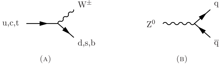
FIGURE 1.1: Weak interactions of quarks in the Standard Model. Left: A charged weak boson changes the flavor of an up-type quark to down-type within the same generation. Right: A neutral weak boson decays into a quark anti-quark pair. Time flows from left to right.
