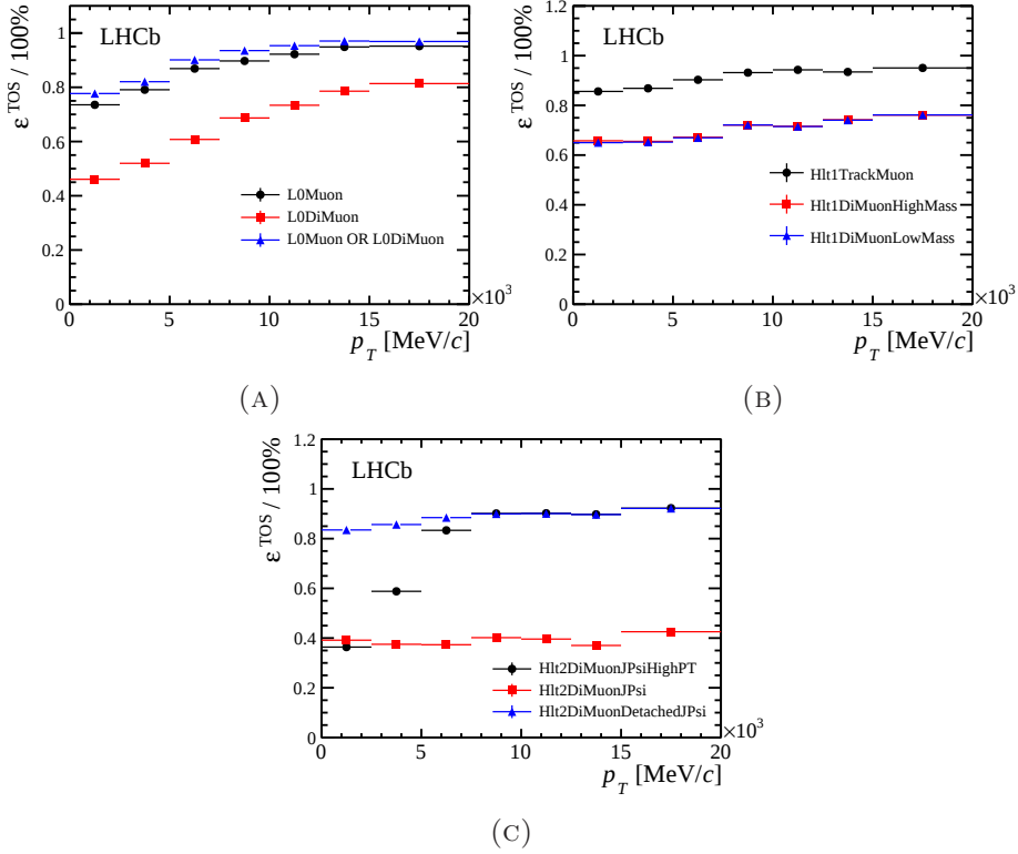
FIGURE 2.6: Muon trigger line tos efficiencies, see text, during Run 1 respectively for the L0 (A), HLT1 (B) and HLT2 (C) trigger stages.
