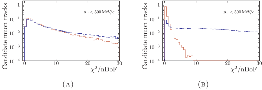
FIGURE 3.4: Distribution of the \chi^2 between the old (left) and new (right) matching algorithms. Only low momentum muon tracks are considered. Matched (not matched) muon tracks are shown with red (blue).
