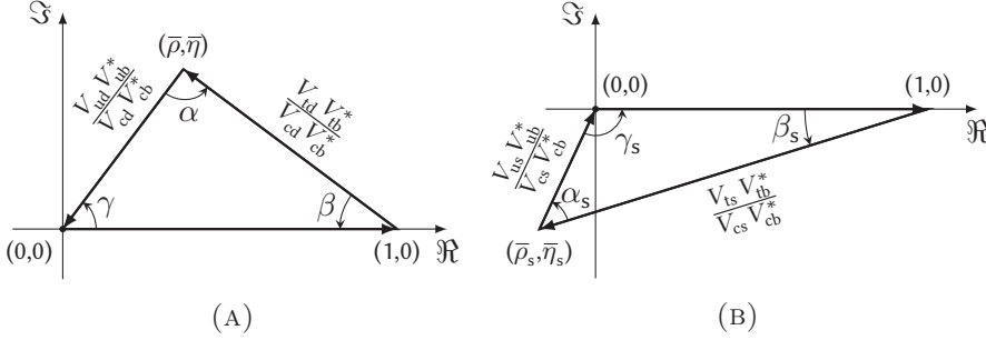
FIGURE 1.3: CKM-unity triangles. B^0 triangle (left), corresponding to Eq. 1.9a. B_s^0 triangle (right), corresponding to Eq. 1.9b. Triangle sides have been normalized, see text. This way one of the sides is real with unit length. Note that triangles are not drawn to scale. Figures from [31].
