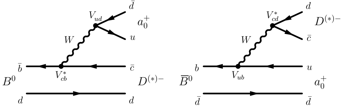
Figure 9.1: The CKM allowed B^0 decay (left) and the CKM suppressed \bar{B}^0 decay (right) to the final state D^{(*)-}a_0^+ .
