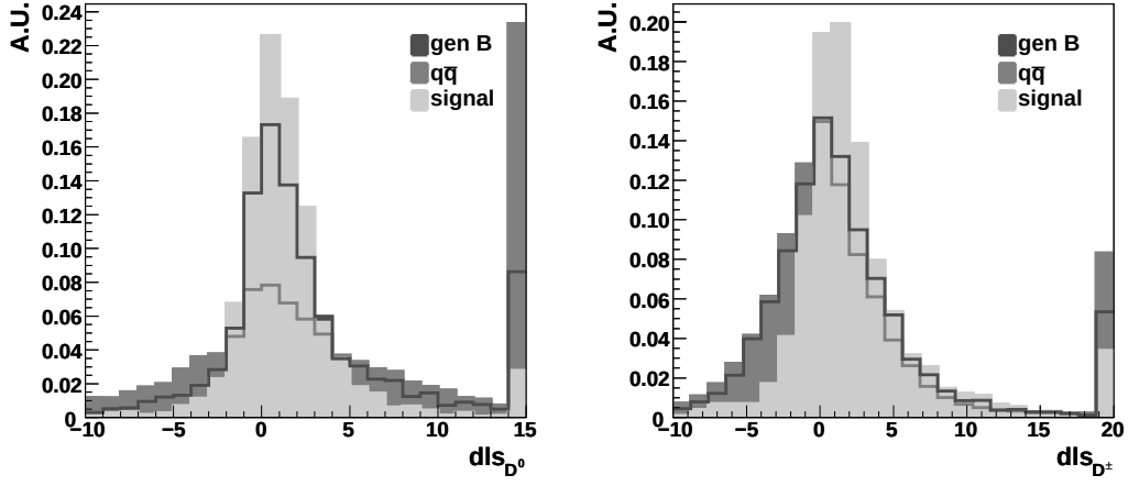
Figure 4.8: Normalized distribution for the decay length significance of the reconstructed D^0 ( left ) or D^\pm ( right ) meson for signal, generic B and q\bar{q} events reconstructed in the DstI ( left ) and DchII ( right ) decay mode. The last bin shows the overflow, or integral of the area on the right of the plotted region.
