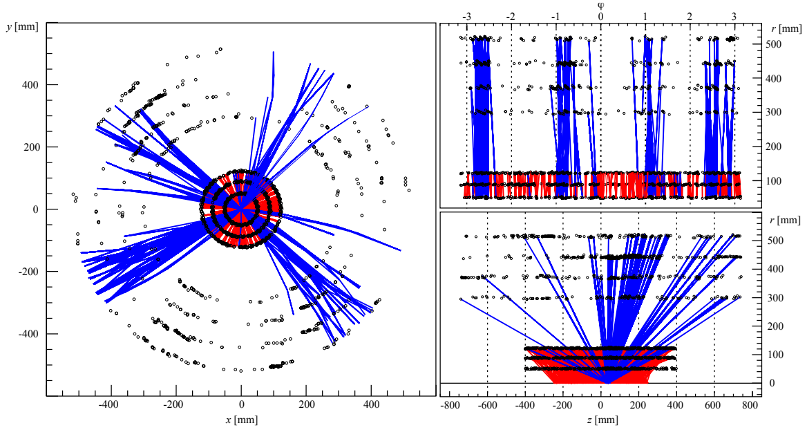
Figure 3: SpacePoint seeds consisting of two (short seeds) respectively three (long seeds) objects in the ATLAS Inner Detector barrel for a t\bar{t} event, found with the z -vertex constraint seed search: the seeds consisting of two SpacePoint objects are used to determine z -coordinates of the predicted vertex positions. Only vertices within a defined range around the interaction point are used to constrain further seeds with three or more SpacePoint objects. For convenience, only seeds that are entirely in the barrel region are drawn.
