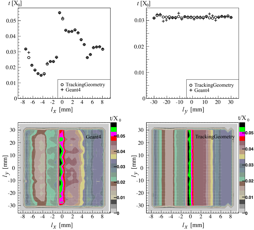
Figure 18: The material distribution in terms of radiation length thickness of a sample Pixel B layer module in the comparison between full simulation (Geant4) and reconstruction (TrackingGeometry). Refined structures can be in the TrackingGeometry separately described by the so-called ReferenceMaterial mechanism. The first plots shows the ReferenceMaterial description in a direct comparison of the material thickness in units of radiation length along the local x and local y coordinate of the surface, respectively. The latter two plots show two-dimensional scatter plots of the material distribution within the sensitive area.
