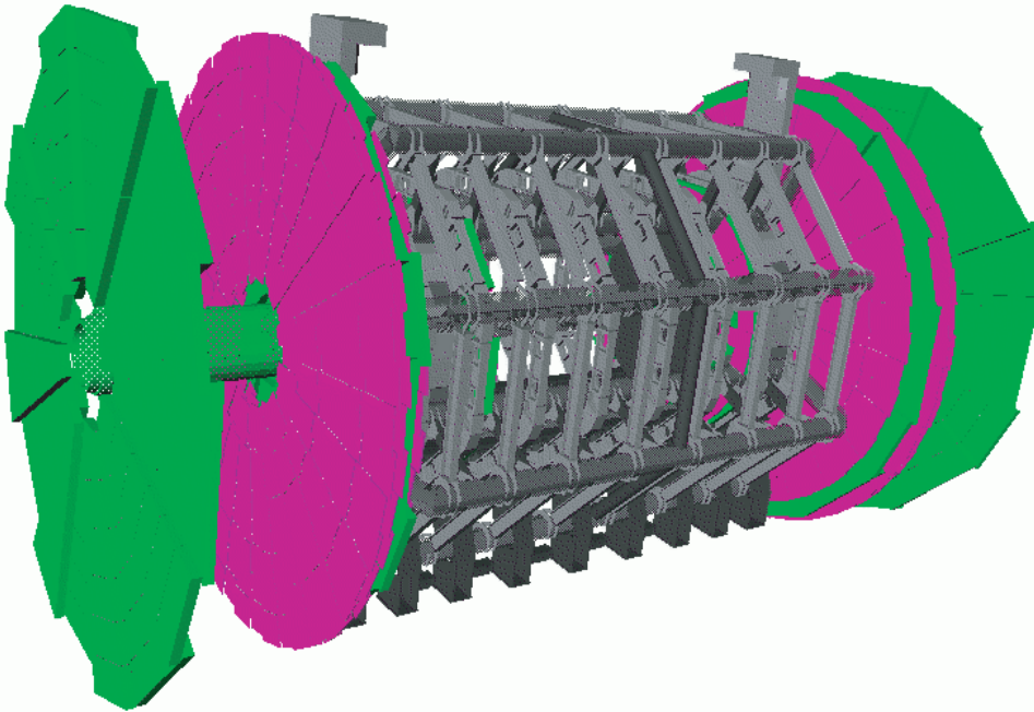
Figure 13: Parts of the Muon System TrackingGeometry visualised with the ATLAS HepVis event display, the Barrel stations are omitted in this illustration. The most complex version of the Muon System TrackingGeometry is generated by parsing and translating the GeoModel detector description.
