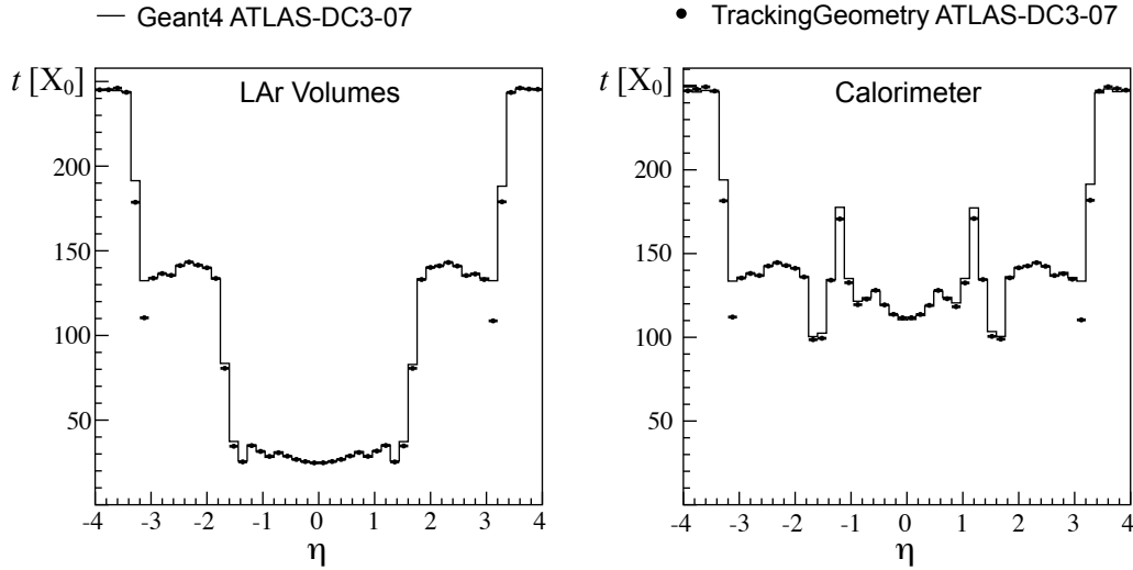
Figure 19: Comparison of the material budget in terms of radiation lengths for the Liquid Argon volumes (including forward calorimeter, FCAL, and the hadronic endcap calorimeters, HEC) and the entire Calorimeter between simulation (Geant4) and reconstruction (TrackingGeometry) geometry.
