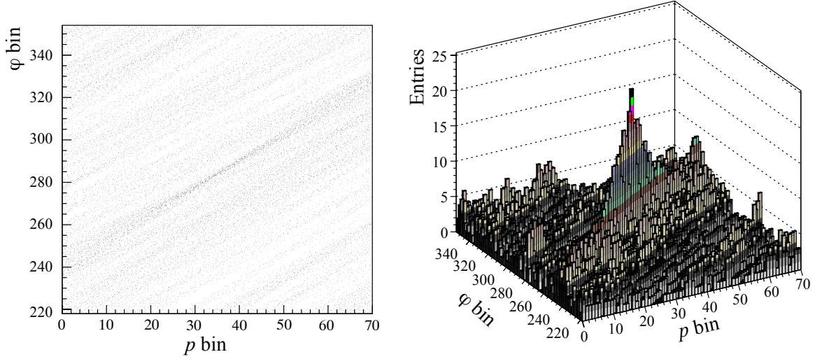
Figure 8: Straw representations in a part of the parameter space ( \phi bins and momentum bins) after applying the Hough transform. The illustration shows a subset of the full parameter space that is divided in the standard configuration into 500 bins in the azimuthal direction, while trying 70 momentum hypotheses. The left side shows the Hough space in a scatter plot, while the right histogram shows the same subset in a three-dimensional version, where the most probably (\phi_0, c_T) hypothesis can be clearly identified; the plot is restricted to a single \eta slice.
