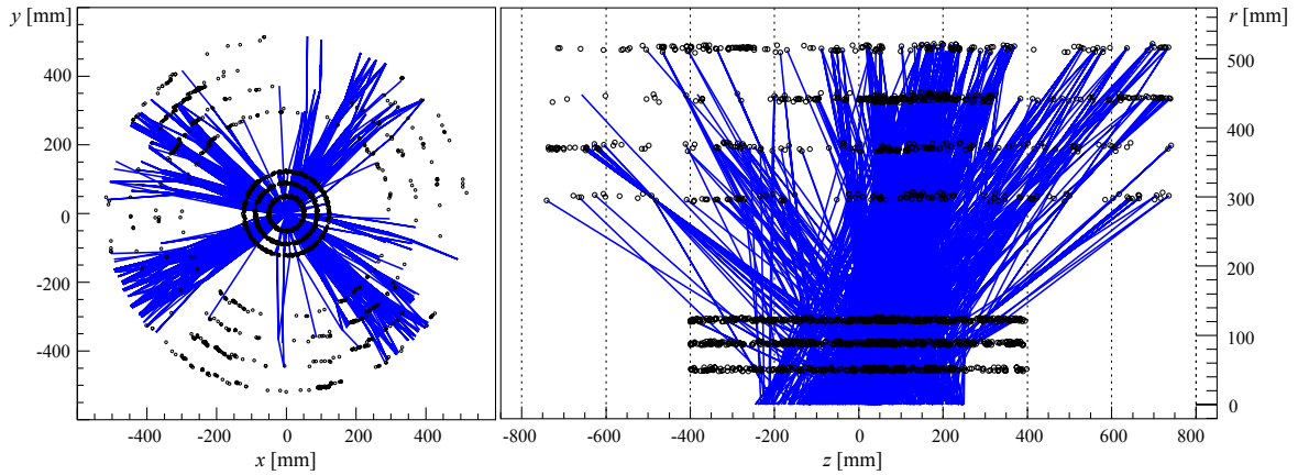
Figure 5: The same event as shown in Fig. 3 using the second silicon seed strategy without vertex constraint. The SpacePoint seed build of three objects are spread over a large z -range that leads to an increase of the track candidates for further processing.
