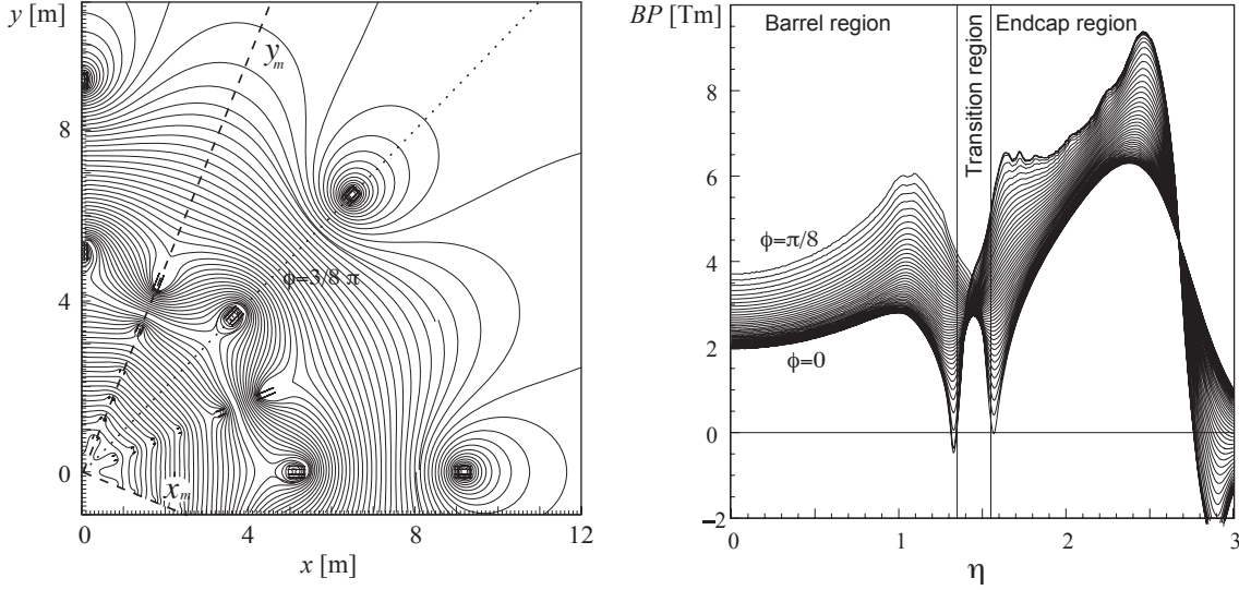
Figure 3.9: The magnetic field in the ATLAS Muon System: one quarter of the barrel magnetic field with its eight-fold symmetry is shown to the left. The right plot shows the dependency of the magnetic field along the beam direction, including the highly inhomogeneous transition region between the barrel and one endcap toroid.
