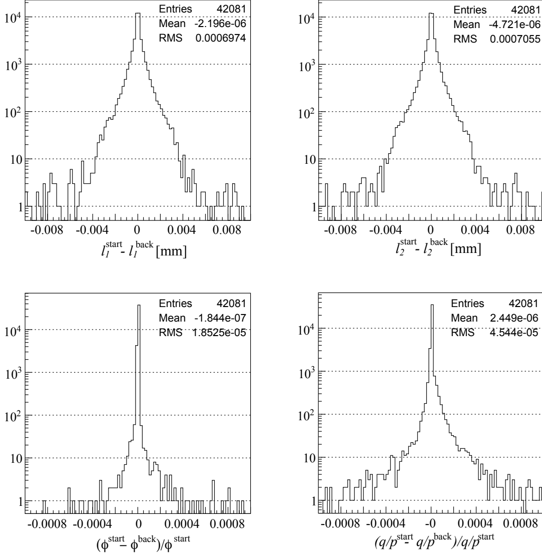
Figure 15: The absolute respectively relative error of about for sample extrapolations within the Inner Detector including full navigation and material effects integration. About 40000 extrapolations for the interaction region (smeared start parameters) to randomly distributed planar surfaces in the Inner Detector and back to the start surface are performed. The two upper plots show the absolute difference of the local coordinates of the start parameters with the back propagated ones. The latter plots show the relative error on the initial \phi respectively \frac{q}{p} values, the start parameters have been generated equally distributed over the entire azimuthal range and in the momentum interval between 500 MeV and 150 GeV.
