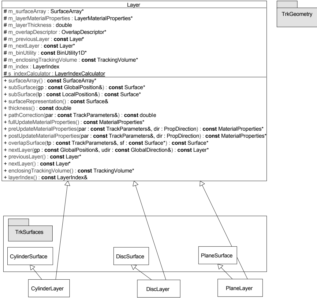
Figure 6: Simplified UML diagram for the layer class in the TrkGeometry package. The double inheritance of a layer from its dedicated surface representation and a common base class is shown. For convenience constructors and destructors are omitted in this diagram.
