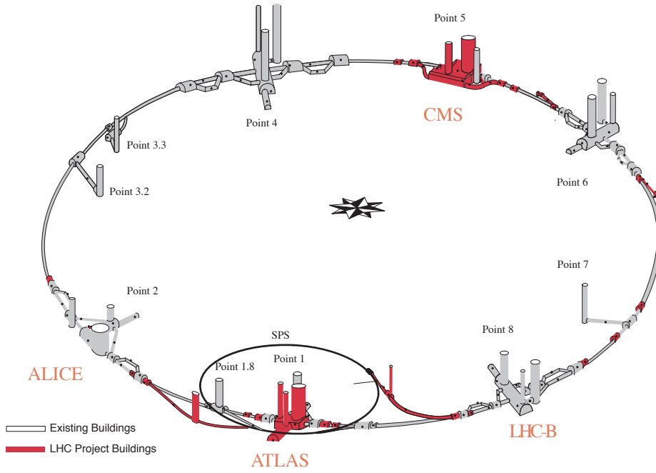
Figure 2.1: The experimental areas at the Large Hadron Collider that is located at CERN. The illustration shows the positioning of the four LHC experiments along the 27 kilometer long tunnel that has previously hosted the Large Electron Proton Collider (LEP). While for the two huge general purpose experiments, ATLAS and CMS, new caverns had to be constructed, ALICE and LHCb could use existing facilities of the prior LEP experiments. The picture includes also the Super Proton Synchrotron (SPS) with a circumference of about seven kilometers that is used as an injector to the LHC.
