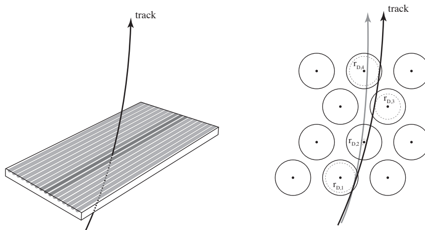
Figure 4.1: Schematic illustration of cluster and drift circle measurements. The left picture shows the principle of a cluster measurement through a segmented planar surface. The resolution that can be achieved is often higher than the segmentation of the measurement device since an interpolation of several neighboring cells can be done. The illustration to the right shows several drift circle measurements: the correct track candidate can hereby be only found through a collection of drift circle measurements or a well defined track seed. The illustration shows how a possible second track candidate that is still compatible with the drift circle measurements in tube 1 and 2 is ruled out by drift measurements in the layers 3 and 4.
