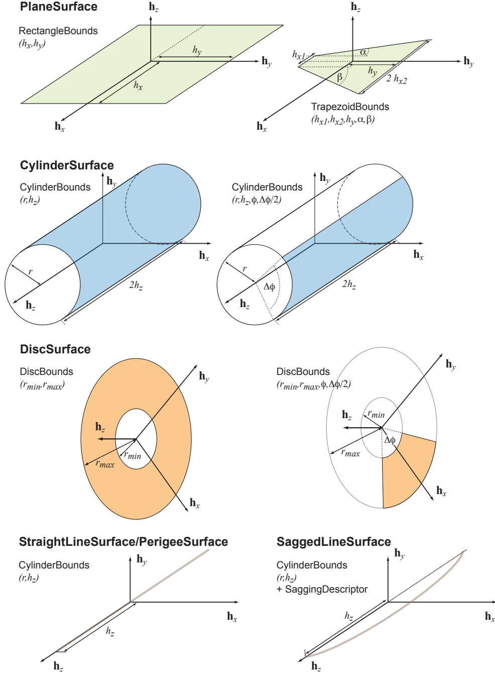
Figure 2: The different surface types and the main boundary shapes as used in the EDM and implemented in the TrkSurfaces package. In general, different surface types were chosen for different intrinsic coordinate systems. This concept is broken for performance reasons by the introduction of the PerigeeSurface type that is a specialisation of the StraightLineSurface type. The picture also includes the prototype of a SaggedLineSurface which has been designed to describe the sagging of wires due to gravitation, a more detailed description of this aspect can be found in Sec. 7.
