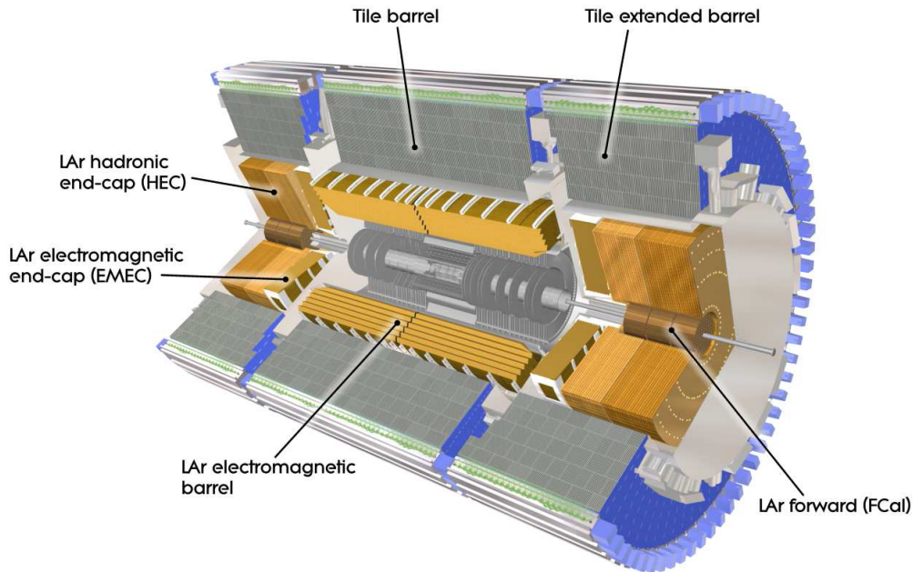
Figure 3.7: Cut-away view of the ATLAS calorimetry devices. The illustration contains the central Inner Detector, the LAr calorimeter, the Tile barrels and forward calorimeters.
