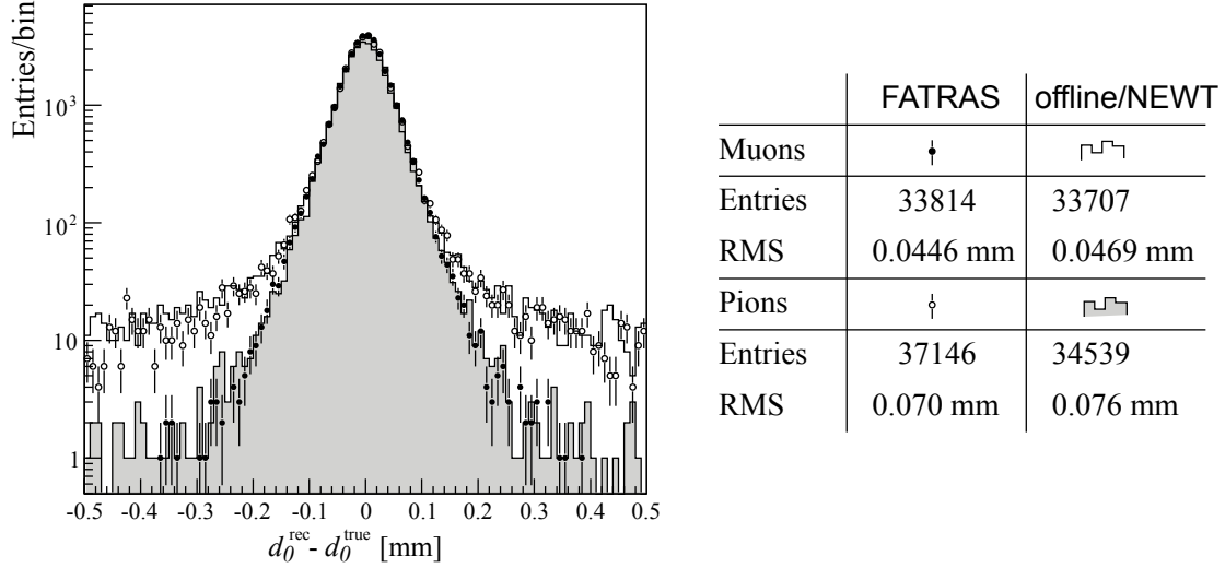
Figure 25: The transverse impact parameter resolution d_0 for single muon and pion tracks of transverse momentum 5 GeV. The results of FATRAS and the full offline chain are shown without applying any quality or matching cuts to include secondary tracks caused by hadronic shower interactions.
