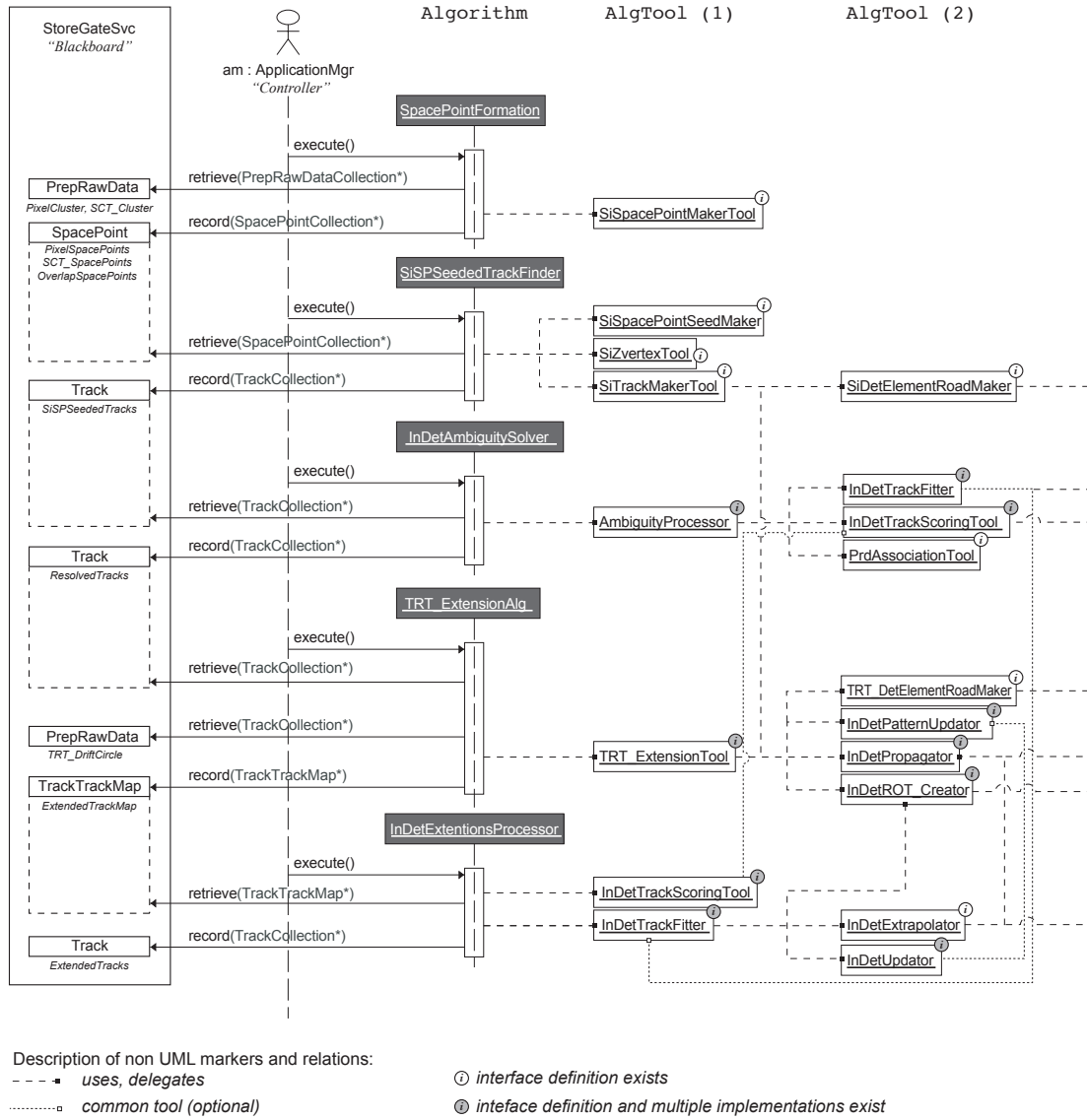
Figure 2: The main sequence of modules and some of the AlgTool classes used in the ATLAS New Tracking for the Inner Detector illustrated as an extended UML sequence diagram. Following a blackboard architecture structure, the transient event store (StoreGateSvc) acts as the blackboard for reading and writing of event data, the ApplicationMgr as the controller of the system. Only two levels of embedded AlgTool classes are shown, where dashed lines indicate a uses relationship, while the dotted line indicates possible sharing of AlgTool instances.
