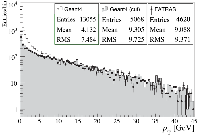
Figure 31: Photon momenta of radiated brem photons simulated with FATRAS and Geant4. The blank histogram shows the standard Geant4 setup, while the shaded area shows the Geant4 results when being restricted to one single photon/conversion iteration (i.e. the identical setup to FATRAS in this comparison).
