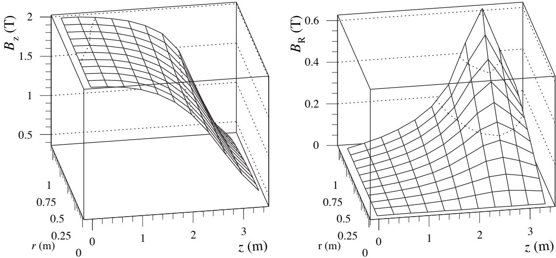
Figure 3.3: Inhomogeneity of the solenoidal magnetic field in the Inner Detector, showing the dependency of the transverse magnetic field B_r and the longitudinal magnetic field B_z as a function of z and the radius r .
