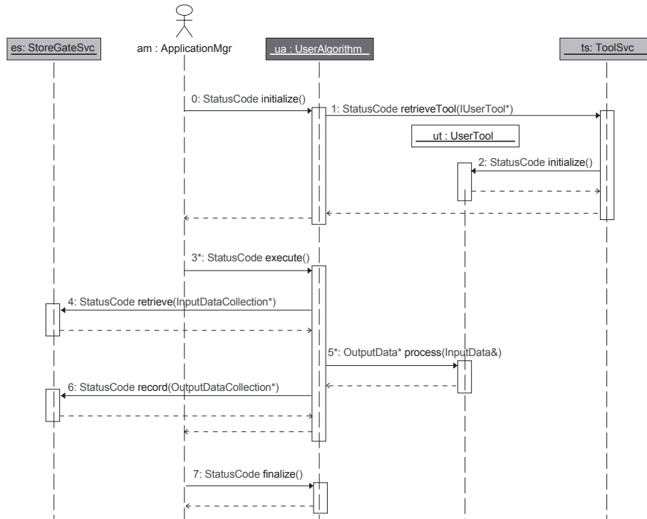
Figure 1: A simplified UML sequence diagram for the data flow and sequence steering in the ATHENA framework. Every Algorithm is registered to the ApplicationMgr that calls the initialize() interface method at job startup, the execute() for every event and the finalize() method in the job termination phase. The initialize() call to the Algorithm may trigger the retrieval of an AlgTool from the ToolSvc . The main framework methods are templated and return a StatusCode object that indicates the success state of the performed operation.
