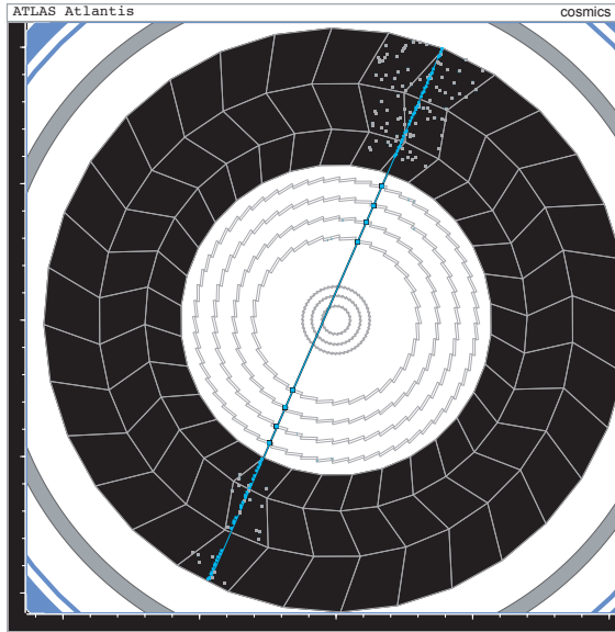
Figure 10: A real cosmic ray event found by the CTBTracking package and shown with the ATLAS event display ATLANTIS. The CTBTracking has been initially developed for the combined test beam run and was the first reconstruction sequence entirely build from New Tracking components using the common event data model. The CTBTracking has been also adopted to serve the needs for reconstructing cosmic ray tracks.
