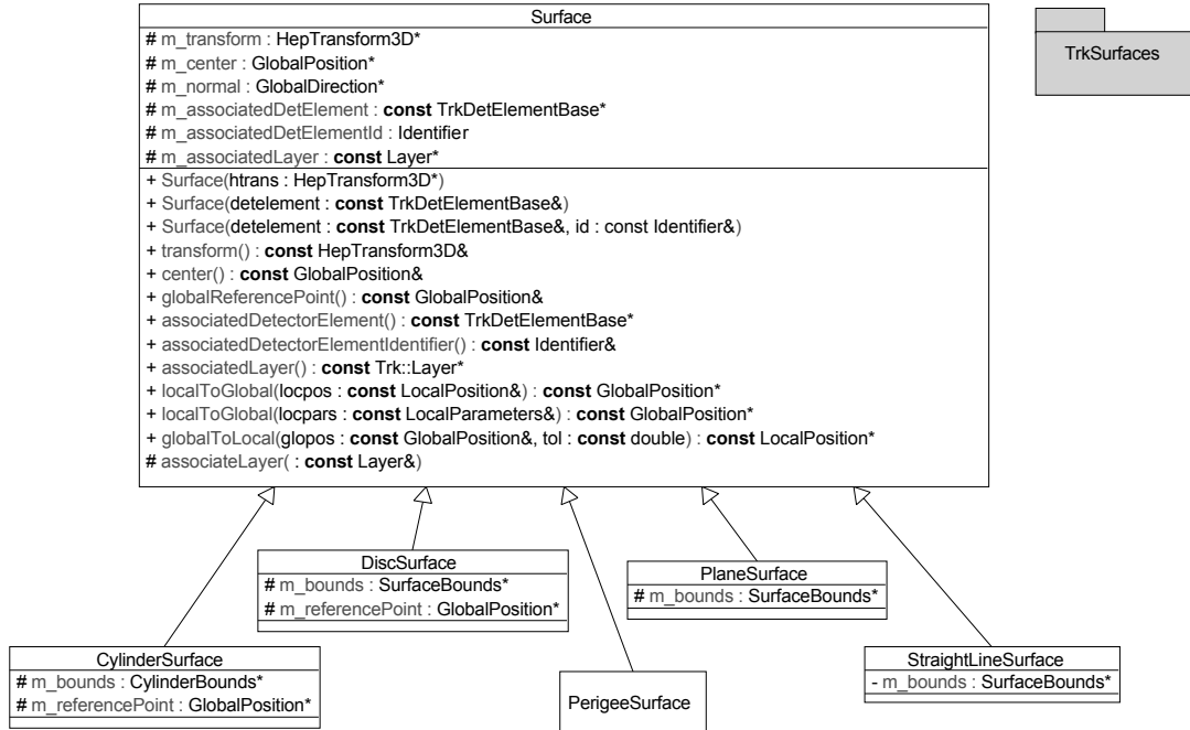
Figure 1: Simplified UML diagram for the surface classes of the ATLAS (tracking) detector description. The base class constructors indicate the two different surface types private and public : Surface instances associated to a TrkDetElementBase are public surfaces. They are owned and managed by the central ATLAS detector description GeoModel . Private surfaces can either be constituents of the TrackingVolume instances or reference surfaces for EDM objects that are not bound to sensitive detector elements. The diagram also shows the main local to global transformation methods provided by the surface interface. These transformations are overloaded by the extended child classes respecting the internal or natural surface coordinate system.
