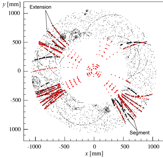
Figure 7: The same t\bar{t} event as shown in Fig. 3 for the two possible TRT hit associations (only the barrel measurements): the brighter colored hits show the extensions that originate from following the SpacePoint seeded tracks into the TRT, the silicon SpacePoint objects are also shown in the same color. The black circles mark hits that have been associated to TRT segments, which builds the start point of the back tracking application. The particular power of the back tracking approach is to find the additional track segments, that have not been found through the inside-out sequence, simply for the fact that no appropriate silicon seed did exist for the further extension process. This is mainly due to strong energy loss of the particle, or due to the fact that the track segments originate from photon conversions or other decay vertices inside the Inner Detector volume.
