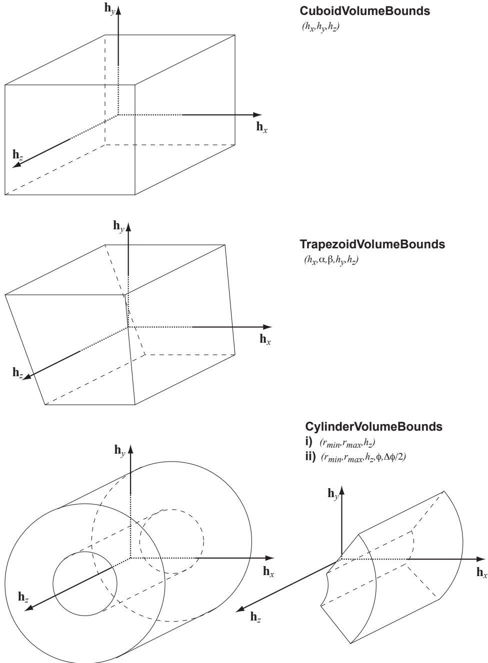
Figure 3: The three main volume types given by the different volume boundary classes. Volumes are mainly characterised by the set of confining boundary surfaces that are handled and owned by the VolumeBounds class. More complex volume shapes such as e.g. the bevelled cylinder shape can also be found in the TrkVolumes repository, they are mainly used for the construction of the complex TrackingGeometry of the Muon System.
