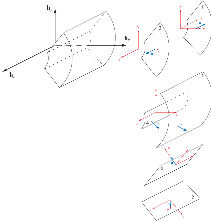
Figure 4: A (sectorial) cylindrical volume shape and its decomposition into boundary surfaces; the uniquely defined normal vectors of the boundary surfaces enhance the pointing to the inside respectively outside neighbor and serve as the key for the navigation between volumes.
