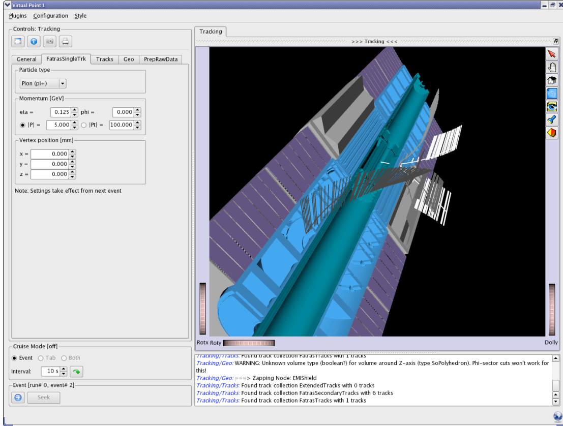
Figure 32: The VP1 FATRAS plugin for single particle event simulation. The current event shows a \pi^+ particle that causes a hadronic shower after interaction with the detector material.
