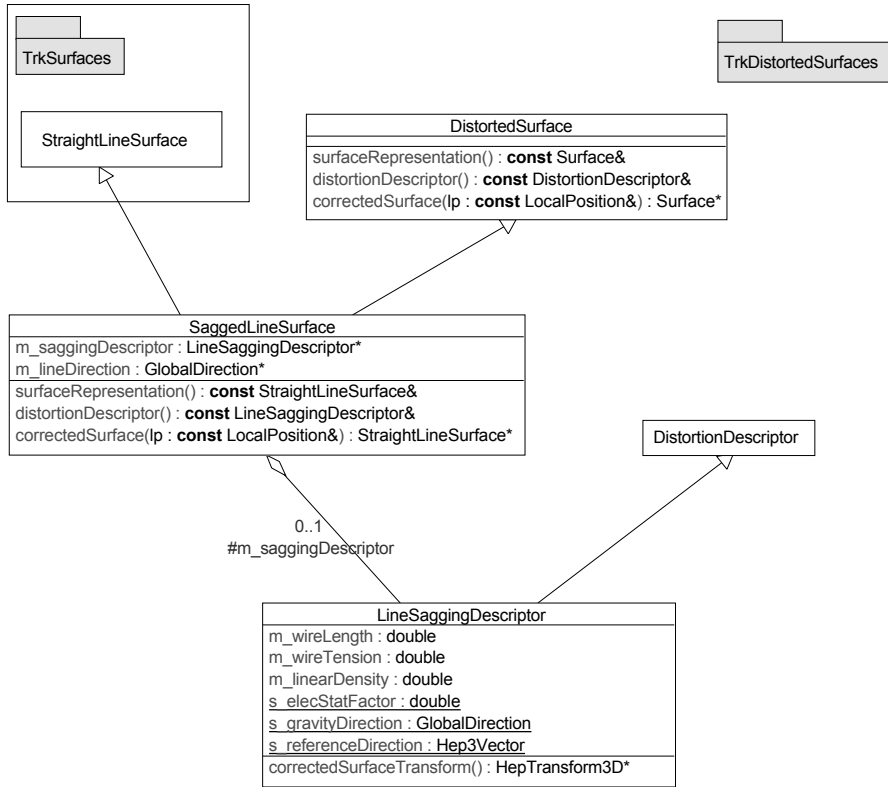
Figure 21: Simplified UML class diagram of a SaggedLineSurface . This class extends the StraightLineSurface and can therefore be naturally used within the extrapolation package. A concrete implementation of a LineSaggingDescriptor concentrates the mathematical description of a wire sag and provides a corrected rotation and position with respect to the local longitudinal direction on the line. Constructors and Destructors are omitted in this diagram.
