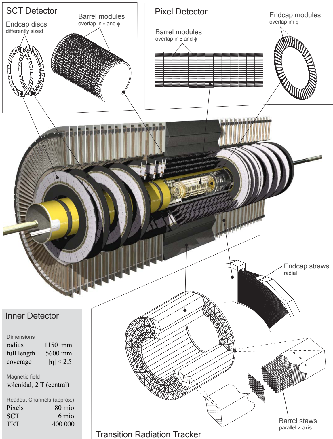
Figure 3.2: Overview of the Inner Detector and its components. Although the geometrical coverage of the ID expands to a pseudorapidity of about |\eta| < 2.7 , track reconstruction is limited to |\eta| < 2.5 , since a minimal required number of modules has to be intersected to allow the trajectory finding and constrain the track fit.
