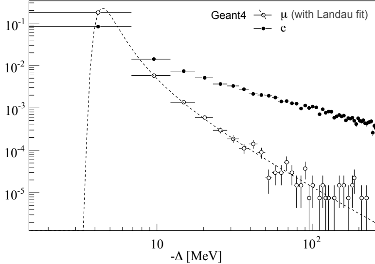
Figure 13: Comparison of muon energy loss to electron energy loss in a silicon layer of 10% X_0 thickness. The particles have been generated using Geant4 and where propagated with a initial momentum of 2 GeV. The muon energy loss distribution follows hereby the Landau distribution, while the electron energy loss distribution is disturbed by the long tail due to radiation loss. This results in a theoretical mean value up to 10 times bigger than for pure ionisation loss.
