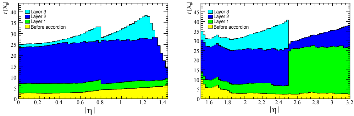
Figure 3.8: The material budget in terms of radiation length X_0 for the LAr calorimeter divided in the contributions before the accordion structure (including the ID and pre-sampler) and the different accordion layers.
