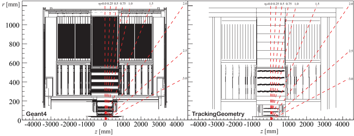
Figure 15: The material hit map of the Inner Detector in the rz plane created with the ATLAS Geant4 simulation and its simplified representation by the TrackingGeometry after the material mapping process. Layer objects and the boundaries of the TrackingVolume objects can be identified in the TrackingGeometry. Additionally, the layers with incorporated ReferenceMaterial (pixel and SCT Detectors) representations can be clearly identified through their diverse structure.
