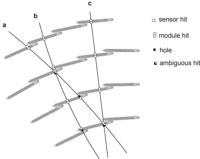
Figure 6: Simplified model of the ambiguity solving process, illustrated in the SCT Barrel. Tracks a , b , and c have been found through the seeded track finding, but share several hits. The \chi^2/n_{dof} may not be appropriate to distinguish a true from a fake track, therefore dedicated track scoring that is optimised for each sub-detector is used. In the shown example, e.g. a module hit representing measurements on both sides of the SCT silicon detector are scored relatively higher than two single hits without associated backside module. Hits in a overlap region as for track b are in particular high scored, while holes on track, i.e. an expected hit that has not been found, lead to a penalty in the track score.
