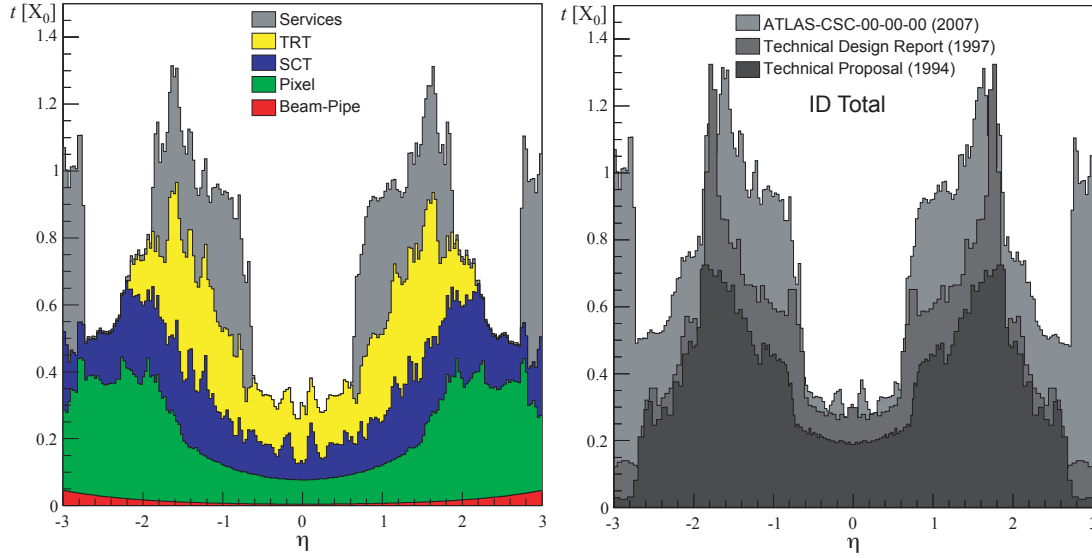
Figure 3.6: The material budget in terms of radiation length X_0 showing the cumulative contributions of the sub-detectors and detector services in the Inner Detector to the left. The right plot shows the evolution of the total material budget integrated into the detector simulation within the last ten years.
