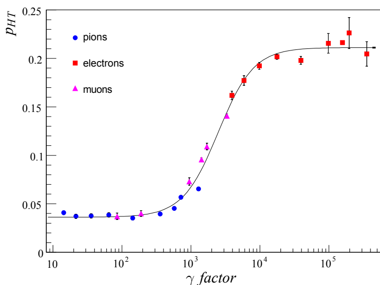
Figure 3.5: The probability of a high threshold hit in the TRT obtained from testbeam data for different particle types. Source: [3.9]
