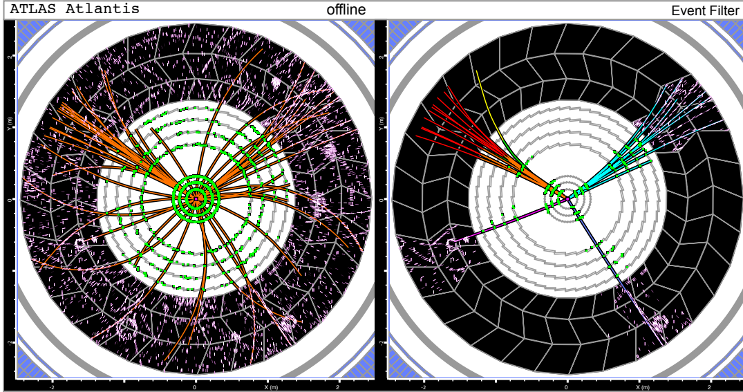
Figure 9: An simulated t\bar{t} event reconstructed with the offline and Event Filter versions of the ATLAS New Tracking. The Event filter has been executed here in the electron slice which determines a dedicated region of interest size in which the full NEWT inside-out sequence is performed. The four regions of interest found by the prior LVL1 and LVL2 trigger and associated to an electron hypothesis can be clearly distinguished.
