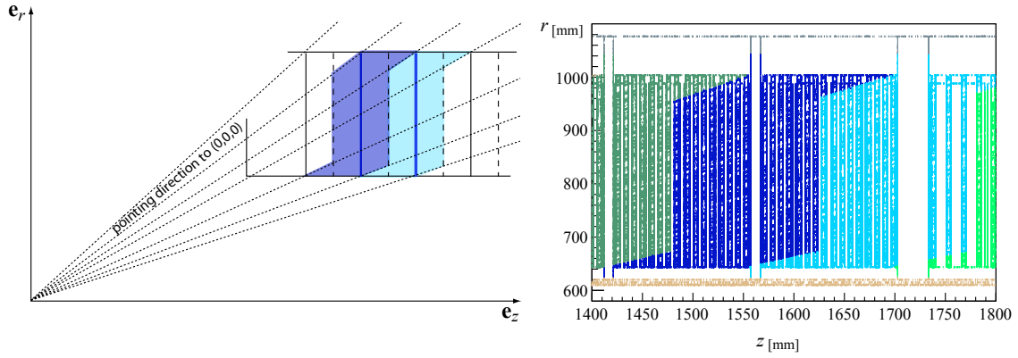
Figure 16: The Geant4 step association with pointing direction using the nominal interaction point as a pointing constraint is shown in the left illustration. The second plot shows the actual Geant4 hit map in the rz plane with the associations to different layers identified by different colors for a part of the positive TRT endcap.
