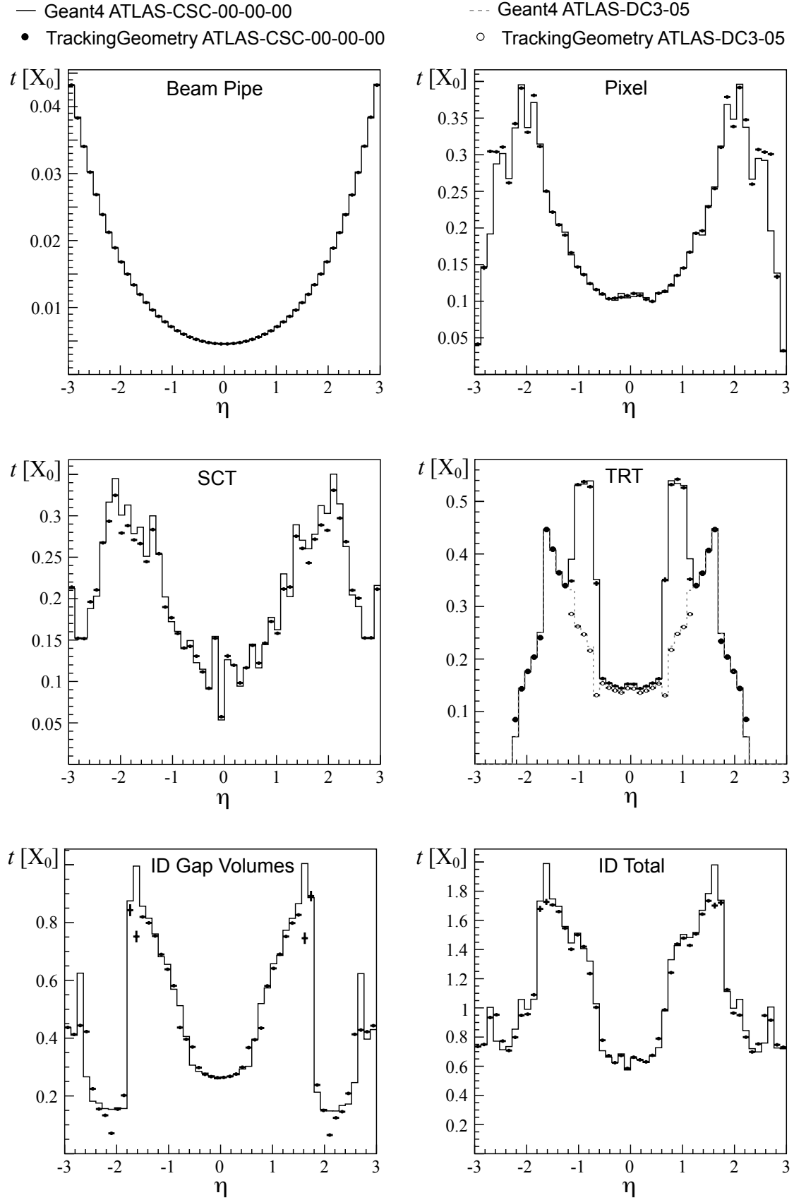
Figure 17: The material distribution in terms of radiation length thickness for the volumes of the Inner Detector TrackingGeometry in comparison with the material used in full simulation (Geant4). The material of the TrackingGeometry layers is shown. The TRT comparison also incorporates the difference between the ATLAS-CSC-00-00-00 and ATLAS-DC3-05 layout, respectively, and shows the automatic adaption of the reconstruction material description to the simulation geometry.
