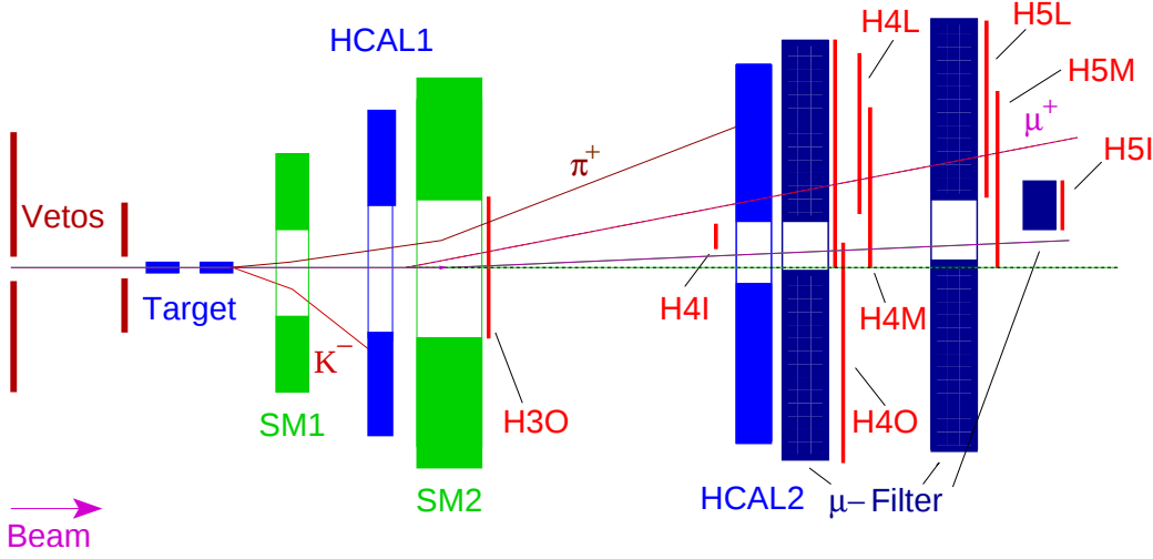
Figure 5.3: Position of the hodoscopes in the spectrometer. There are in total four subsystems: H4I & H5I, H4M & H5M, H4L & H5L and H3O & H4O.
