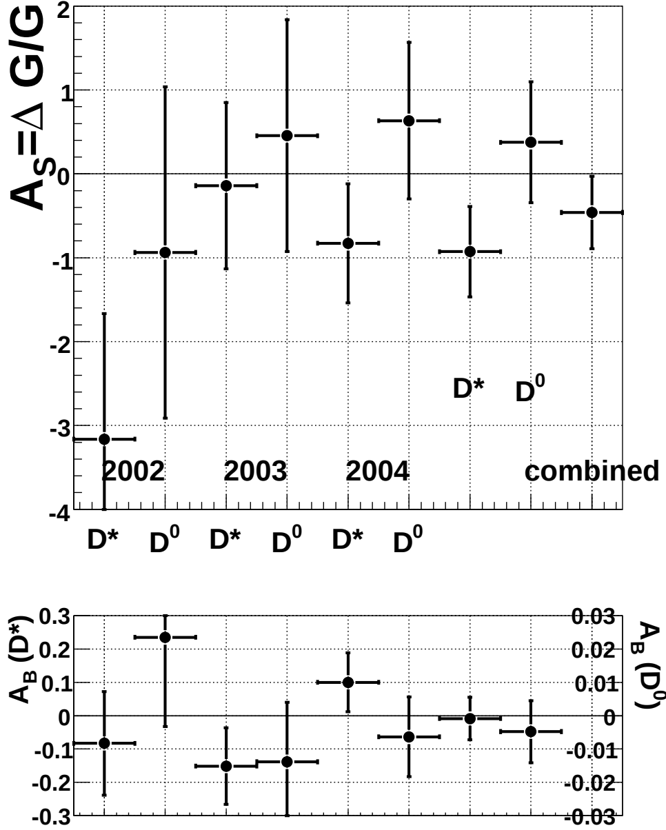
Figure 6.7: Results for A_S \equiv \Delta G/G and A_B for the two decay channels and the different years of data taking. The horizontal axis is the same for both histograms. Note that in the lower histogram the left vertical scale is for the D^* background asymmetry and the right scale for the D^0 background asymmetry.
