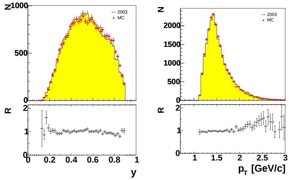
Figure 6.11: Data to MC comparison for one inclusive variable, y , and one semi-inclusive variable, the transverse momentum of the hadron with the largest p_T [29].
