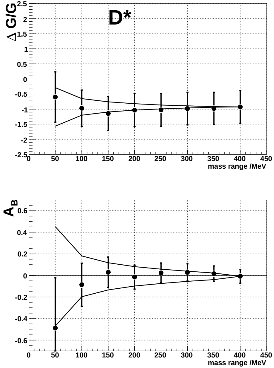
Figure E.4: Dependence of \Delta G/G and A_B on the mass range of the 7 parameter fit for D^* . The lines in the plots show the expected 1\sigma deviations from the point with the smallest statistical error at 400 MeV.
