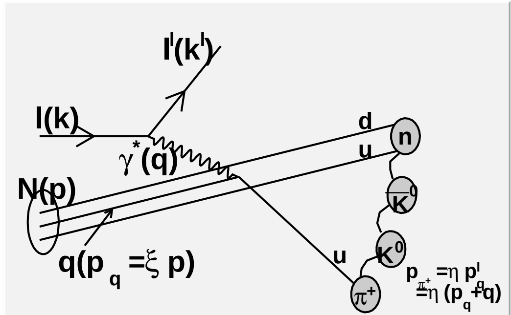
Figure 2.3: Kinematics of the deep inelastic scattering process interpreted in the Quark Parton Model (QPM). The four-vectors of the particles are given in parentheses.
