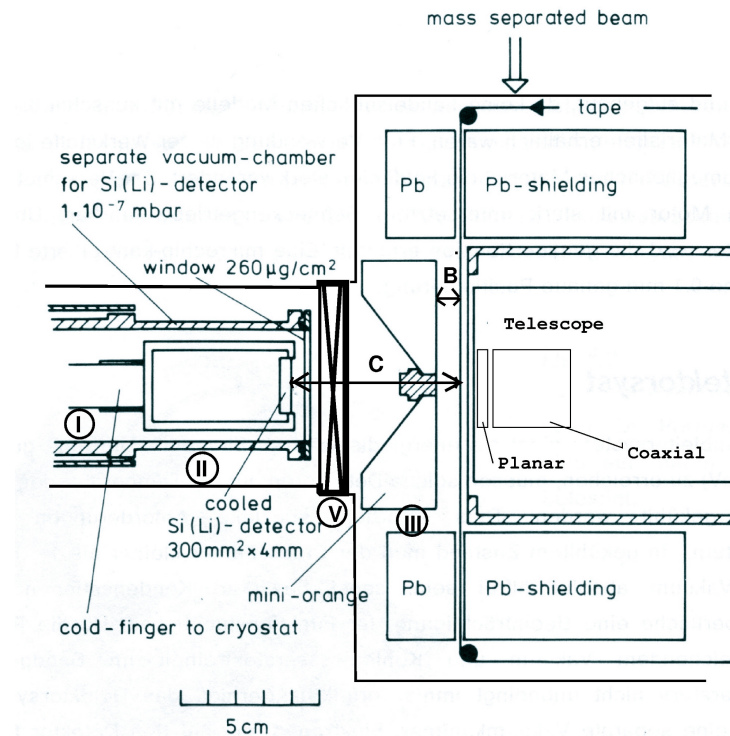
Figure 3.15: A sketch of a horizontal cross-section through the experimental setup for the conversion electron studies with the mini-orange spectrometer [81]. The mass-separated source is deposited on to a tape, which is moved periodically to place the accumulated activity in front of the mini-orange and the Ge telescope (see text). These two detectors sat at 180 degrees to one another with the source in between as shown. A co-axial Ge detector was positioned above the source at right angles to the telescope and is not shown in the figure. The distances B and C are the distances from the source to the front face of the mini-orange and the Si(Li) detector respectively. This nomenclature is used to classify the various mini-orange setups used in the experiments as can be seen in the text. It is consistent with other measurement carried out with the same spectrometer by Barden [81] and Bea et al [85]. The various independent volumes in the apparatus (see text) are marked I, II, and III respectively. There is a valve between I and II which is not shown in the figure and a valve marked V which is used to isolate II from III, the main mini-orange chamber.
