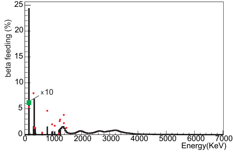
Figure 7.9: Comparison of the beta feeding obtained after the TAS analysis (continuous line) and that from the high resolution experiment (red dots) for the \beta -decay of ^{77}\text{Sr} . The beta feeding which appears as a square has been reduced by a factor of 10 so that it appears in the comparison.
