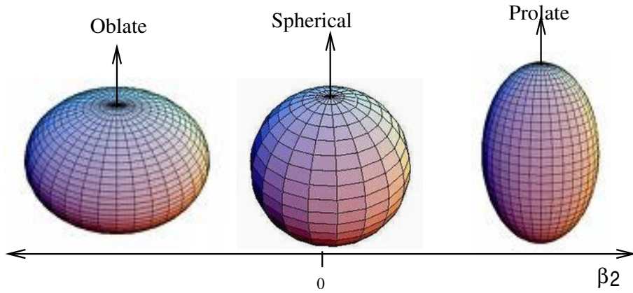
Figure 2.2: Schematic picture showing oblate, spherical and prolate shapes. The arrows for the oblate and prolate shapes indicate the symmetry axis.
