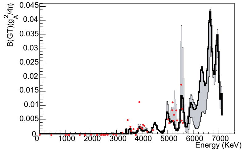
Figure 7.17: B(\text{GT}) distribution in the beta-decay of ^{78}\text{Rb} as a function of the excitation energy in the daughter nucleus (solid line) using the TAS method. The B(\text{GT}) distribution using high resolution spectroscopy (red dots) is also shown.
