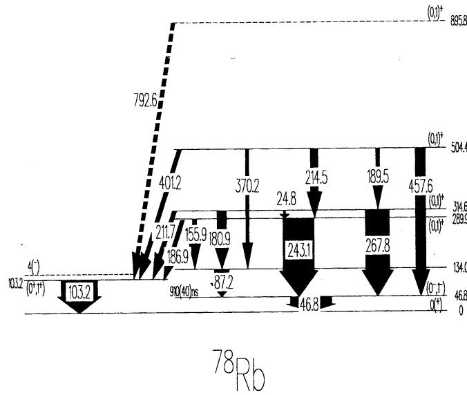
Figure 4.2: Low-lying level scheme of ^{78}\text{Rb} from Reference [79]. The authors have not included the information on the excitation energy of the isomer and it is given as "x". They predict the energy of this linking transition to be lower than the binding energy of the K_{\alpha} -shell ( \sim 13\text{keV} ) since the K-conversion peak is not observed. McNeill et al. [94] have found the excitation energy of the isomer to be 111.2 keV with an 8.6 keV highly converted linking transition to the 103 keV level. The same authors have also observed a 64.4 keV transition to the 46.8 keV level from the isomer.
