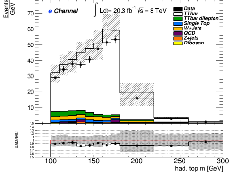
(a) Hadronic Top candidate Mass
