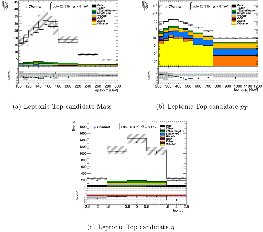
Figure 5.6: The (a) mass, (b) p_T and (c) \eta of the leptonic top in the muon channel. The distribution obtained from the real data is represented by the black points, the white histograms represent the simulation of the t\bar{t} lepton+jets signal, while colored hisograms correspond to the estimated background contamination and the hatched band represents the systematic uncertainties.
