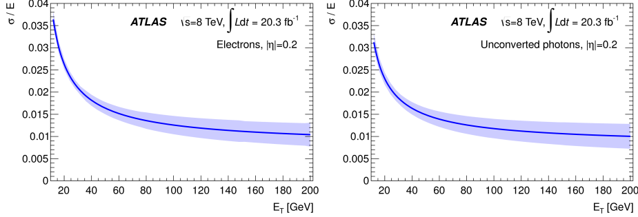
Figure 2.8: Resolution curve and its uncertainty as a function of E_T for electrons (left) and unconverted photons (right) with |\eta| = 0.2 . [51].
