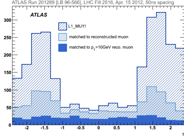
Figure 5.24: \eta distribution of Level-1 muon ROIs ( p_T > 10 GeV) with the distribution of the subset matched to an offline reconstructed muon with p_T > 3 GeV or p_T > 10 GeV [110].
