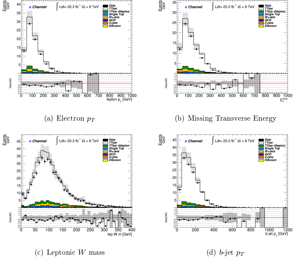
Figure 5.1: The (a) lepton p_T , (b) Missing Transverse Energy, (c) leptonic W mass and (d) b -jet p_T in the electron channel. The distribution obtained from the real data is represented by the black points, the white histograms represent the simulation of the t\bar{t} lepton+jets signal, while colored histograms correspond to the estimated background contamination and the hatched band represent the systematic uncertainties.
