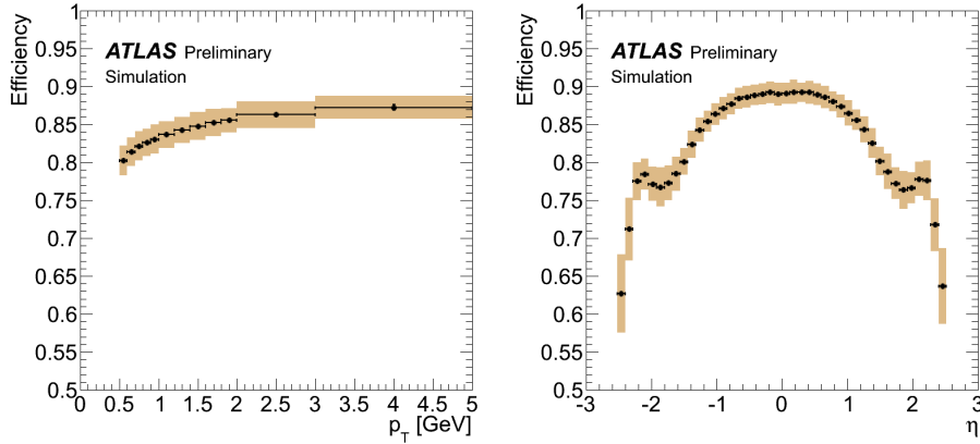
Figure 2.6: Tracking reconstruction efficiency vs transverse momentum (left) and \eta (right) . Special no-pileup 8 TeV Minimum Bias simulation was used. Tracking reconstruction efficiency is defined as a ratio between “number of matched tracks” and “number of generated charged particles” [49].
