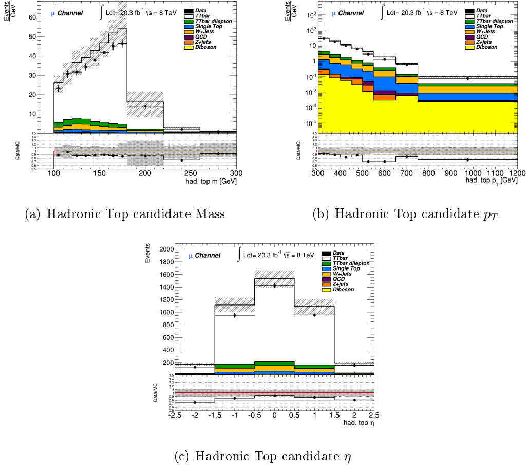
Figure 5.4: The (a) mass, (b) p_T and (c) \eta of the hadronic top in the muon channel. The distribution obtained from the real data is represented by the black points, the white histograms represent the simulation of the t\bar{t} lepton+jets signal, while colored hisograms correspond to the estimated background contamination and the hatched band represents the systematic uncertainties.
