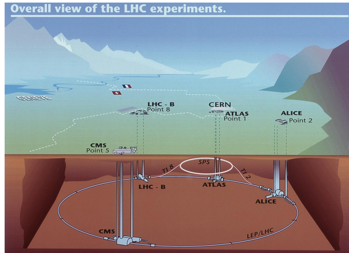
Figure 2.2: An LHC tunnel overview (not in scale)
