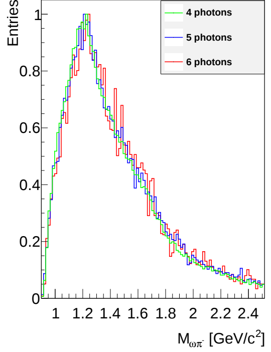
(b) \omega\pi^- mass (normalized)
