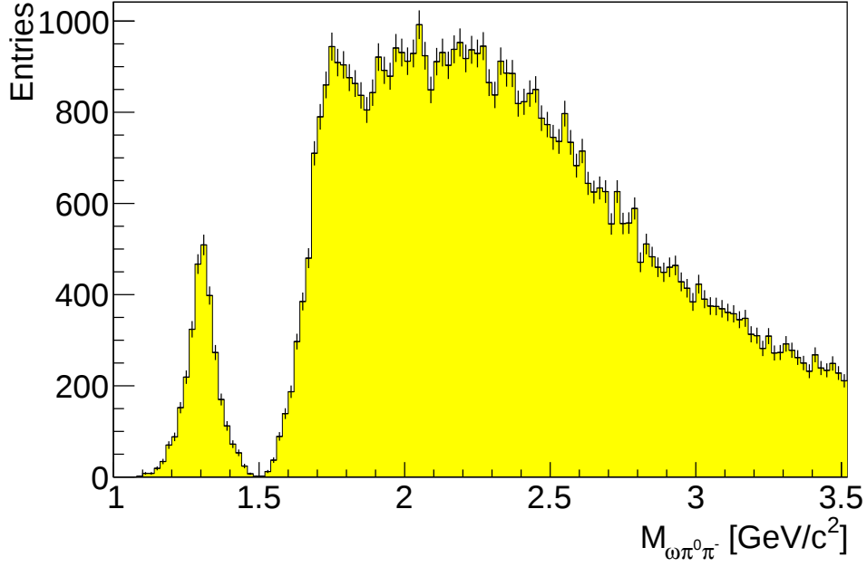
Fig 3.20: Total invariant mass of events fulfilling neither the negative nor the neutral b_1(1235) -cut.
