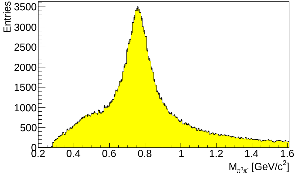
Fig 3.9: Invariant mass of \pi^0\pi^- -system after the succesful cut on exactly one good \omega . The peak at around 770 \text{ MeV}/c^2 can be explained with the decay of \rho(770)^- -mesons.
