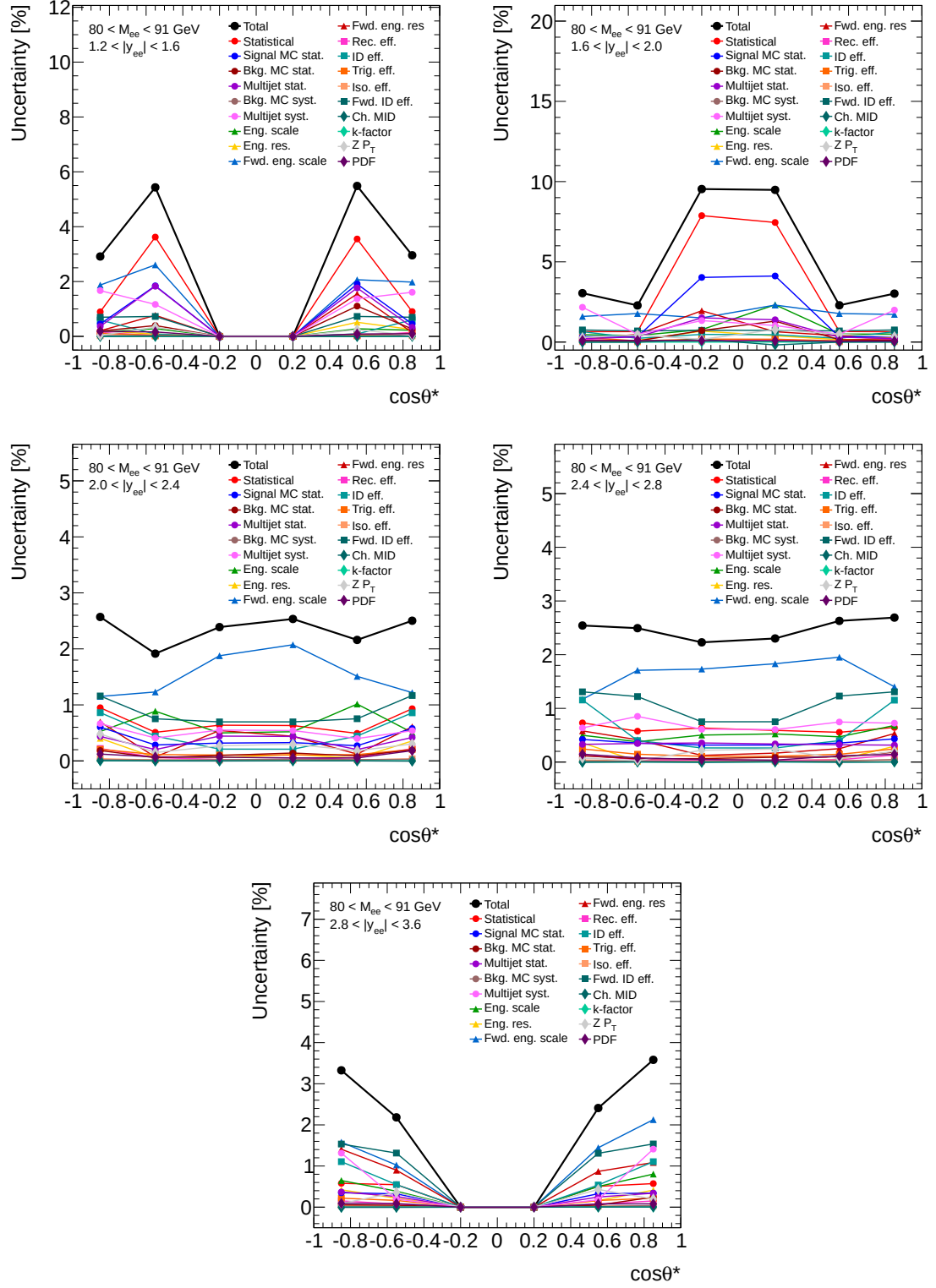
Figure B.18: Uncertainties propagated to \frac{d^3\sigma}{dM_{ee}d|y_{ee}|d\cos\theta^*} for invariant mass bin M_{ee} \in [80, 91] GeV and for the entire rapidity range of interest, 1.2 < |y_{ee}| < 3.6 .
