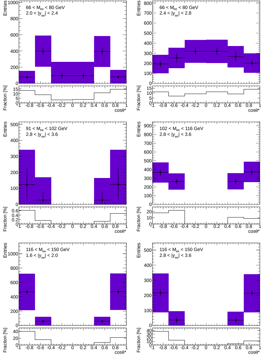
Figure B.11: Multijet background plotted in bins of \cos \theta^* for several different invariant mass and rapidity ranges. Both the statistical (error bars) and total (error band) uncertainties are shown. The fraction of multijet events in the signal data is shown in the bottom panels of the plots.
