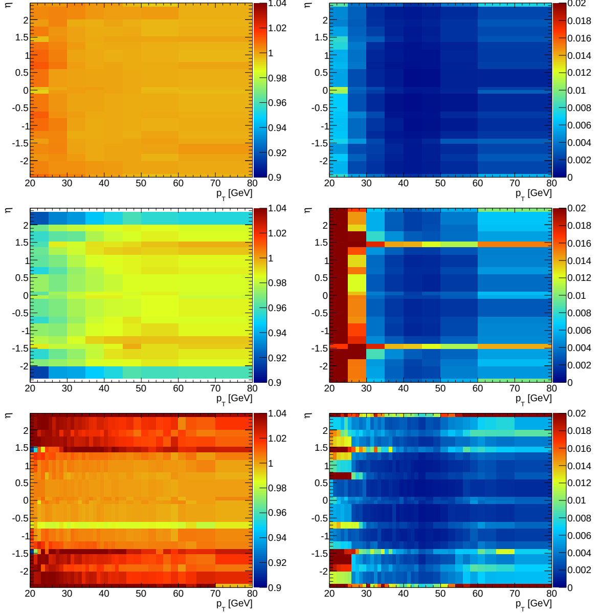
Figure 5.4: EGamma efficiency scale factors (left) and their corresponding absolute uncertainties (right). These two-dimensional plots corresponds to reconstruction (top), medium identification (middle), and trigger (bottom) scale factors. The EF trigger requires two electrons with p_T > 12 GeV that satisfy loose identification per event.
