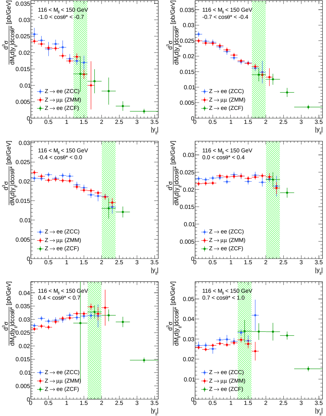
Figure C.15: Central-central, muon-muon, and central-forward three-dimensional differential cross-section \frac{d^3\sigma}{dM_{\ell\ell}d|y_{||}|d\cos\theta^*} results for invariant mass bin M_{\ell\ell} \in [116, 150] GeV and for the entire polar angle range of interest, -1.0 < \cos\theta^* < 1.0 .
