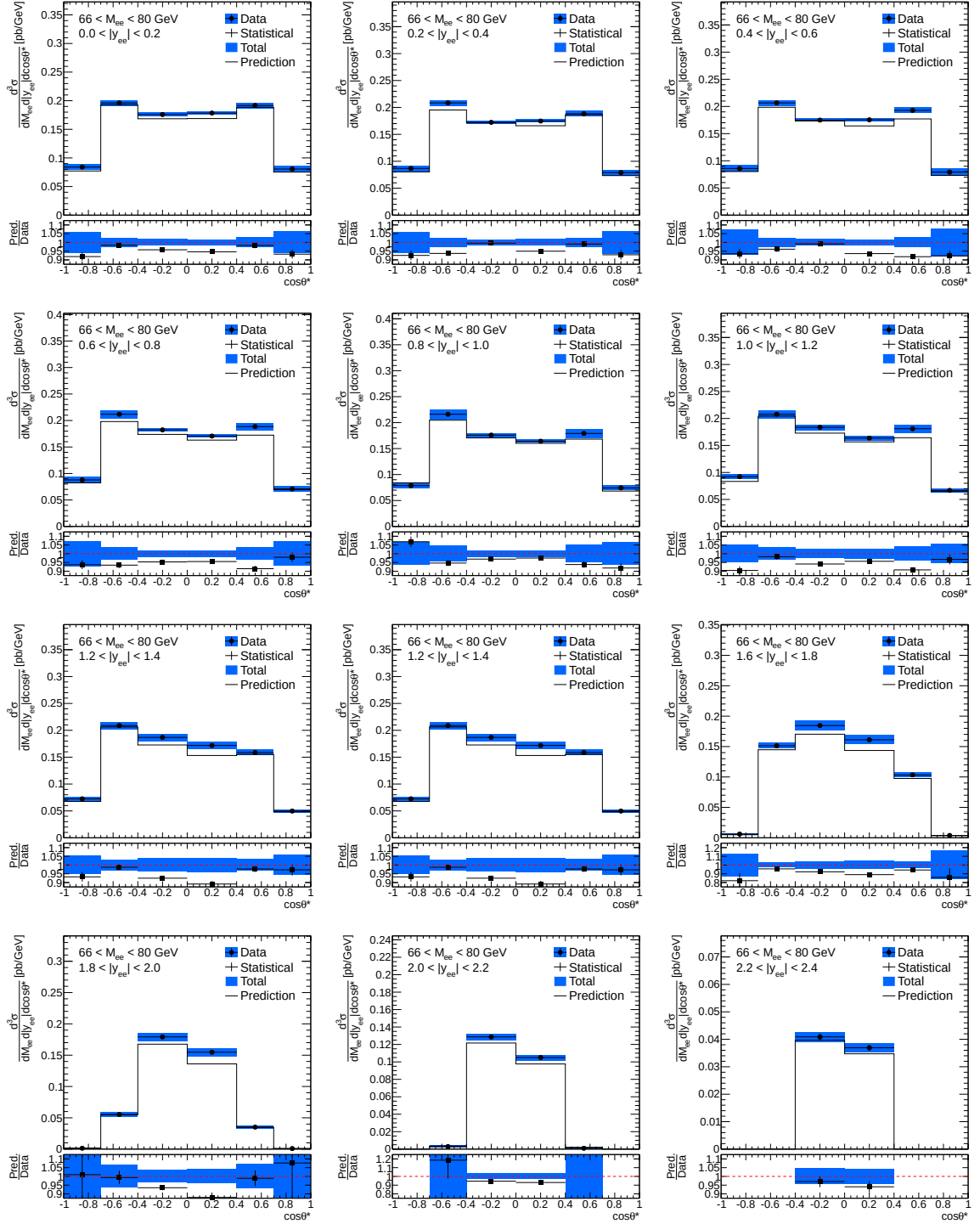
Figure 9.2: Three-dimensional differential cross-section \frac{d^3\sigma}{dM_{ee}dy_{ee}|d\cos\theta^*|} results for invariant mass bin M_{ee} \in [66, 80] GeV and for the entire rapidity range of interest, 0.0 < |y_{ee}| < 2.4 .
