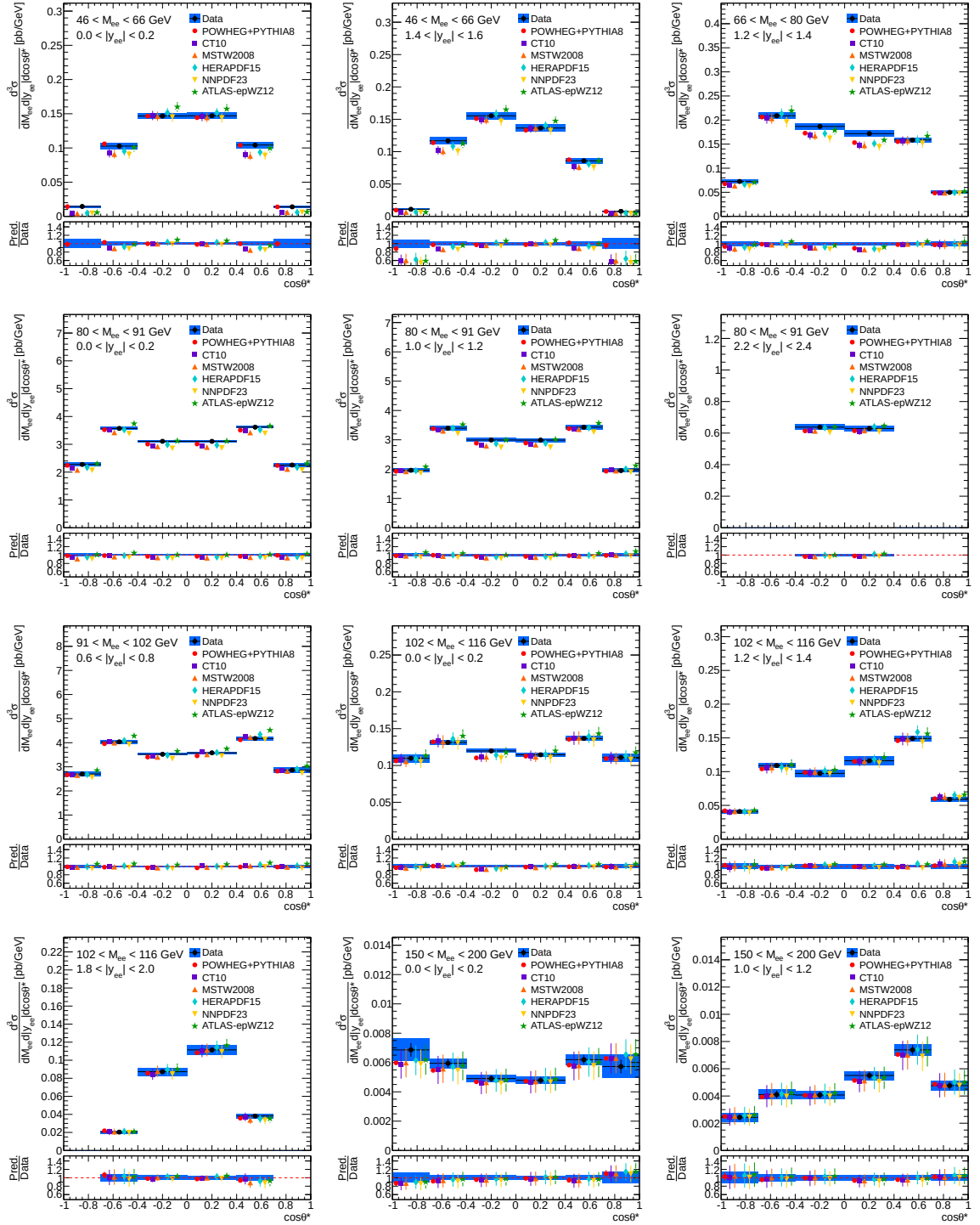
Figure 9.10: Differential cross-section distributions of data and theory predictions. The data is compared with the signal MC (POWHEG+PYTHIA8) and MCFM calculations using several popular PDF sets.
