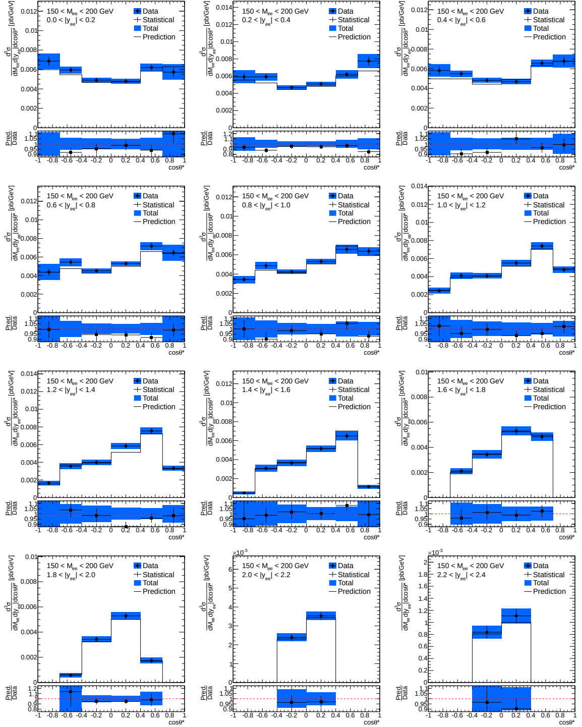
Figure 9.7: Three-dimensional differential cross-section \frac{d^3\sigma}{dM_{ee} d|y_{ee}| d\cos\theta^*} results for invariant mass bin M_{ee} \in [150, 200] GeV and for the entire rapidity range of interest, 0.0 < |y_{ee}| < 2.4 .
