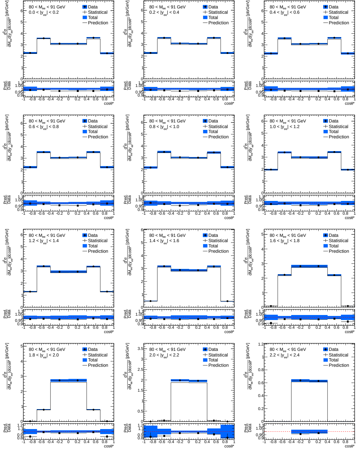
Figure 9.3: Three-dimensional differential cross-section \frac{d^3\sigma}{dM_{ee} d|y_{ee}| d\cos\theta^*} results for invariant mass bin M_{ee} \in [80, 91] GeV and for the entire rapidity range of interest, 0.0 < |y_{ee}| < 2.4 .
