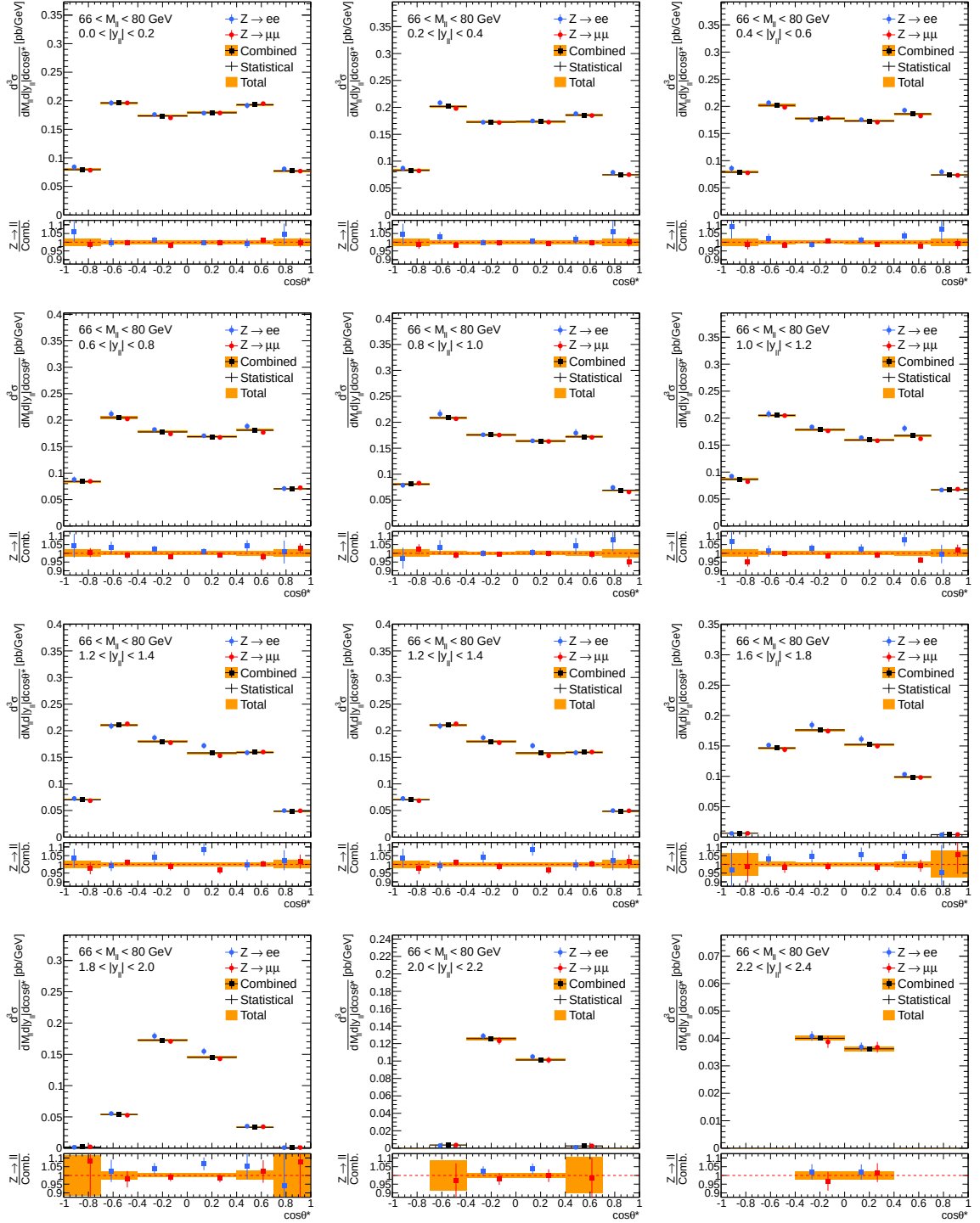
Figure C.5: Combined three-dimensional differential cross-section \frac{d^3\sigma}{dM_{\ell\ell}d|y_{\ell\ell}|d\cos\theta^*} results for invariant mass bin M_{\ell\ell} \in [66, 80] GeV and for the entire rapidity range of interest, 0.0 < |y_{ee}| < 2.4 .
