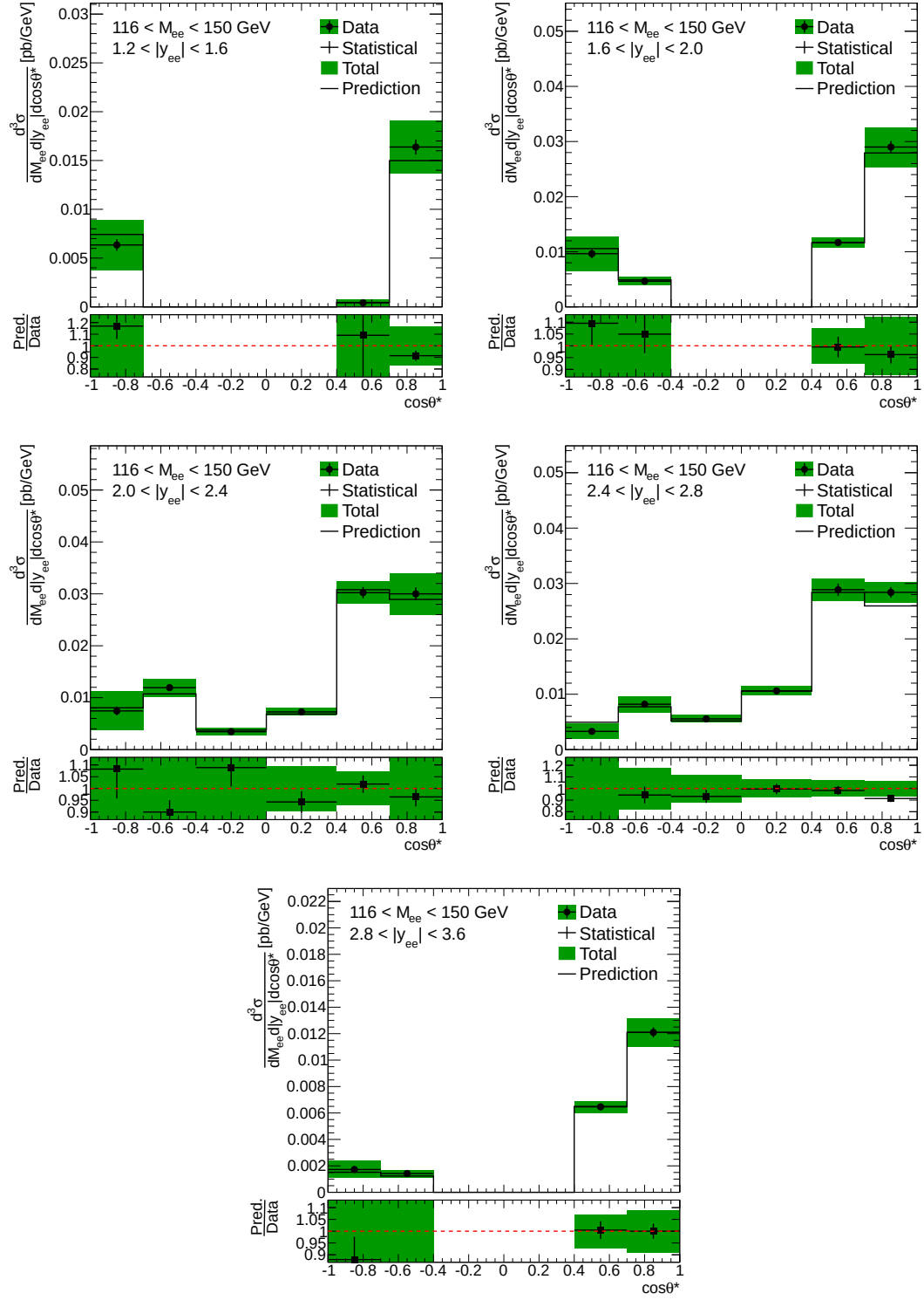
Figure B.26: Three-dimensional differential cross-section \frac{d^3\sigma}{dM_{ee}d|y_{ee}|d\cos\theta^*} results for invariant mass bin M_{ee} \in [116, 150] GeV and for the entire rapidity range of interest, 1.2 < |y_{ee}| < 3.6 .
