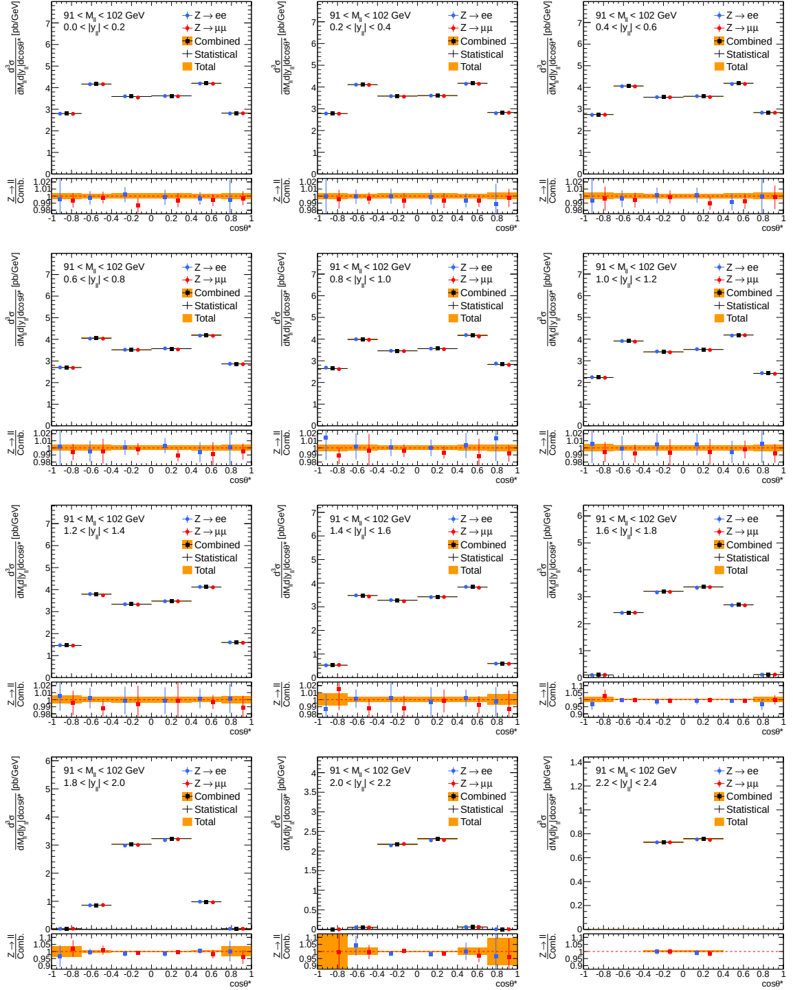
Figure C.7: Combined three-dimensional differential cross-section \frac{d^3\sigma}{dM_{\ell\ell} dy_{\ell\ell} d\cos\theta^*} results for invariant mass bin M_{\ell\ell} \in [91, 102] GeV and for the entire rapidity range of interest, 0.0 < |y_{ee}| < 2.4 .
