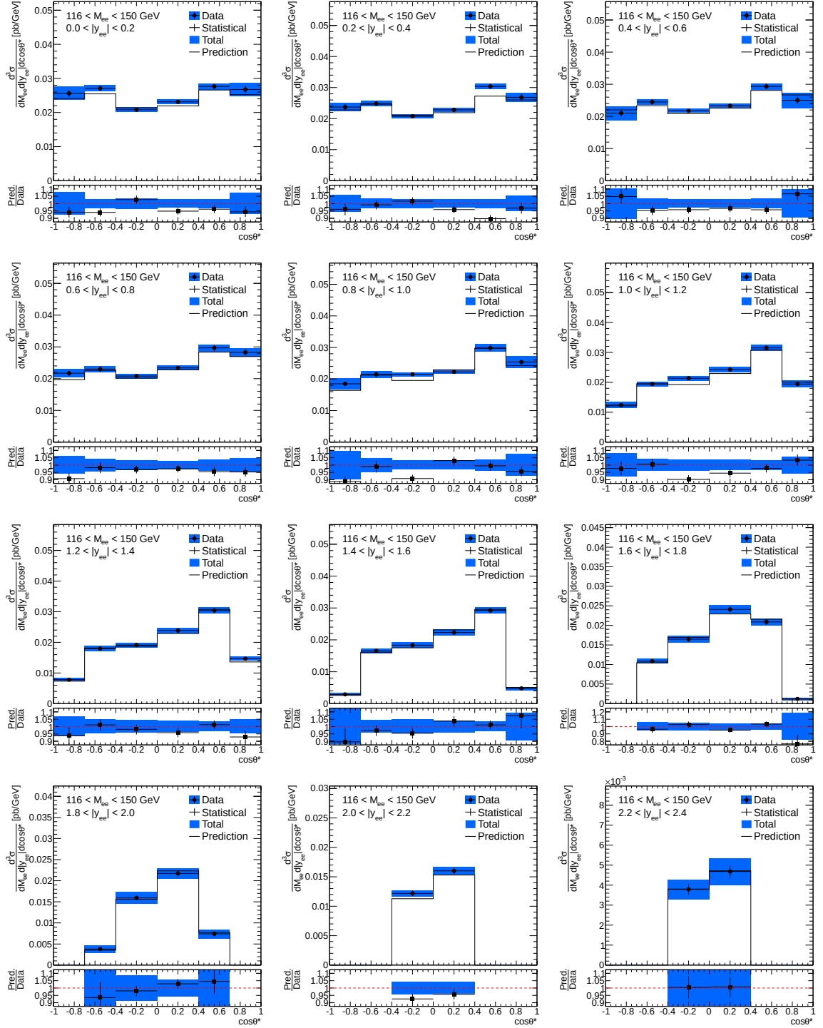
Figure 9.6: Three-dimensional differential cross-section \frac{d^3\sigma}{dM_{ee} d|y_{ee}| d\cos\theta^*} results for invariant mass bin M_{ee} \in [116, 150] GeV and for the entire rapidity range of interest, 0.0 < |y_{ee}| < 2.4 .
