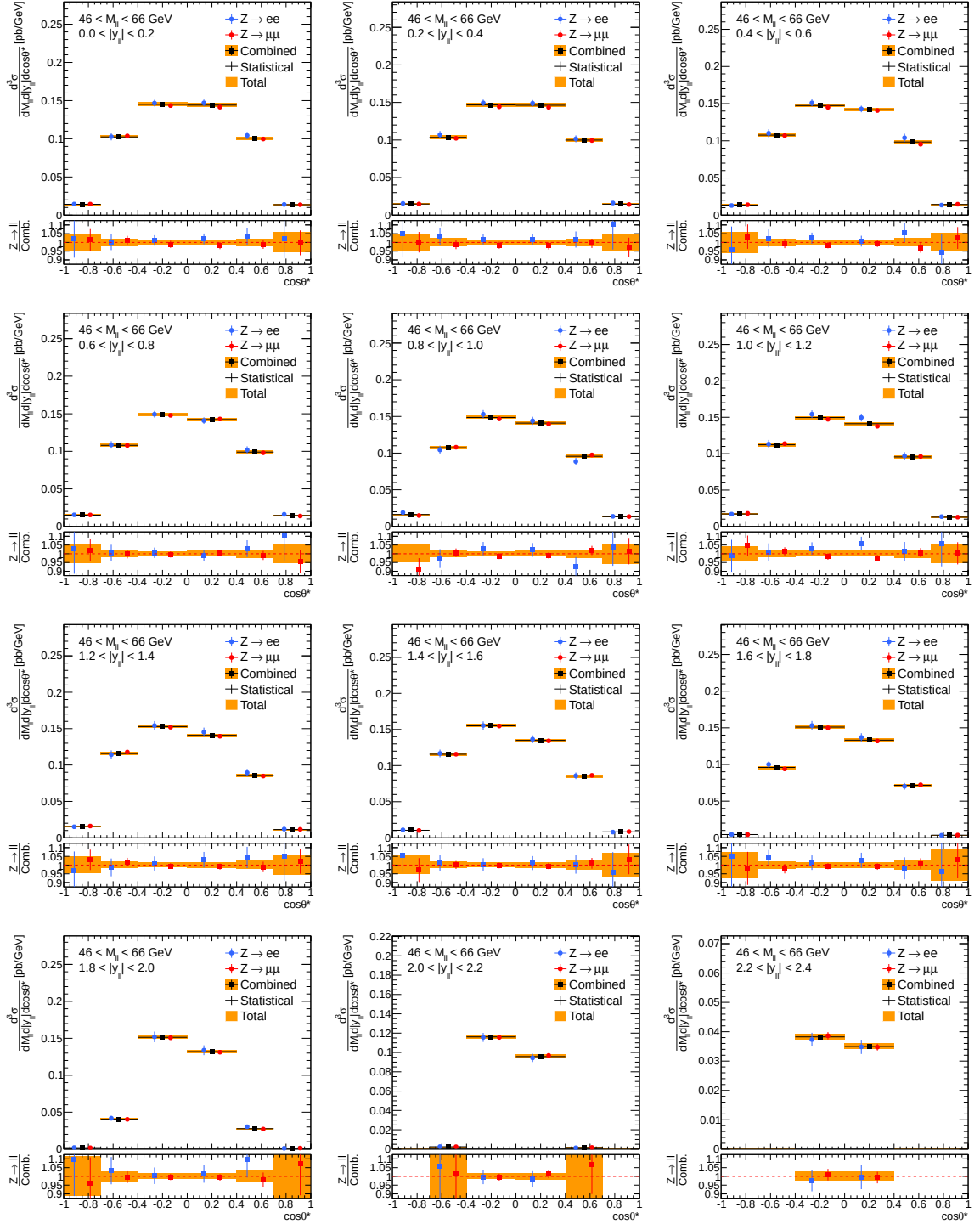
Figure C.4: Combined three-dimensional differential cross-section \frac{d^3\sigma}{dM_{\ell\ell} dy_{\ell\ell} d\cos\theta^*} results for invariant mass bin M_{\ell\ell} \in [46, 66] GeV and for the entire rapidity range of interest, 0.0 < |y_{ee}| < 2.4 .
