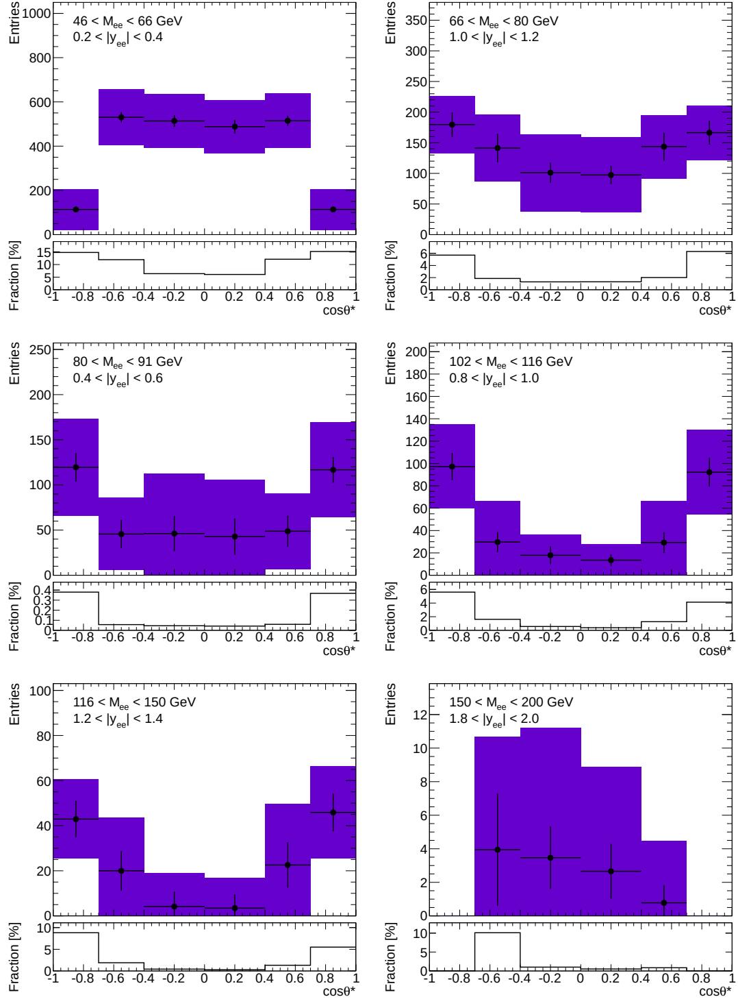
Figure 7.6: Multijet background plotted in bins of \cos \theta^* for several different invariant mass and rapidity ranges. Both the statistical (error bars) and total (error band) uncertainties are shown. The fraction of multijet events in the signal data is shown in the bottom panels of the plots.
