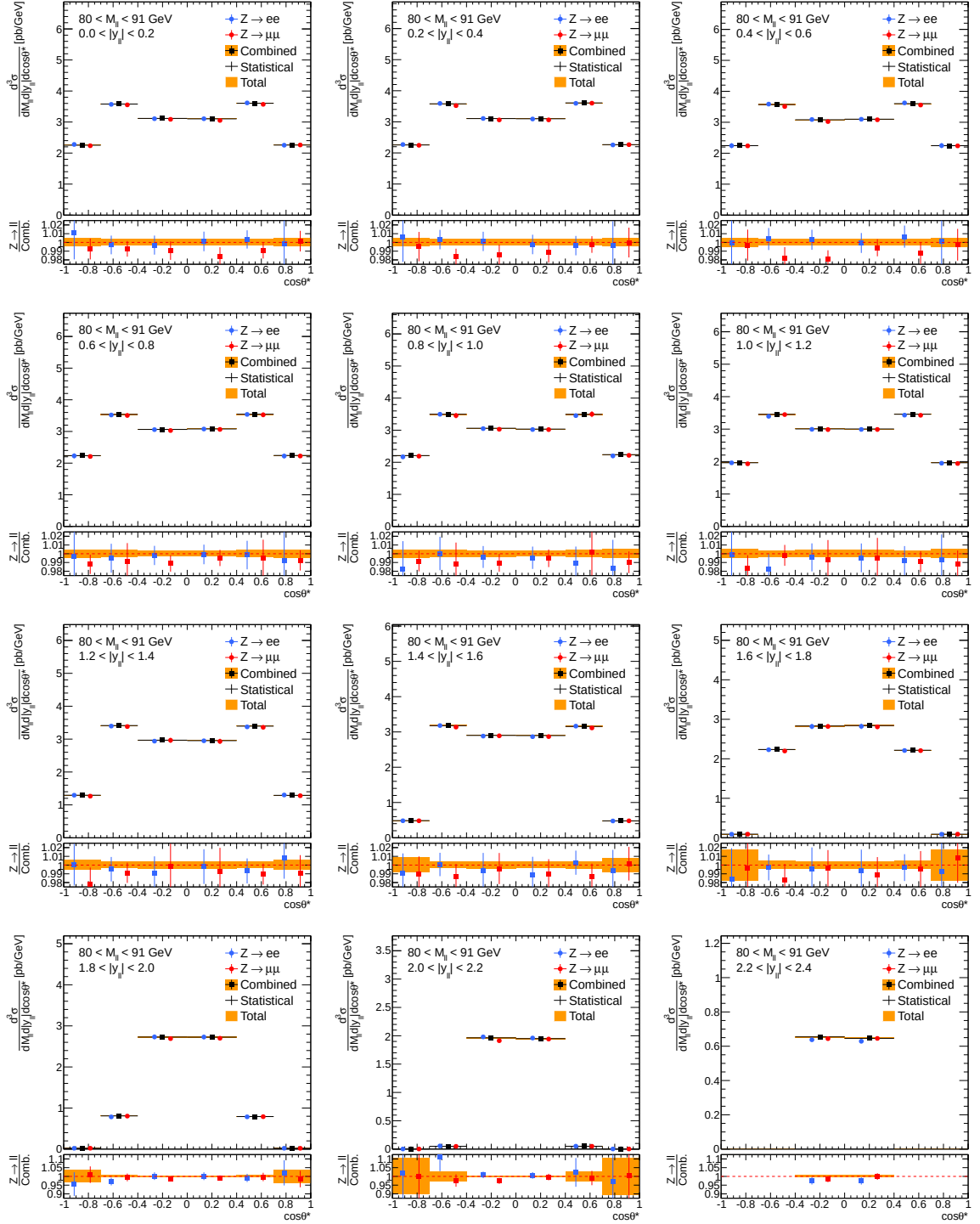
Figure C.6: Combined three-dimensional differential cross-section \frac{d^3\sigma}{dM_{\ell\ell} dy_{\ell\ell} d\cos\theta^*} results for invariant mass bin M_{\ell\ell} \in [80, 91] GeV and for the entire rapidity range of interest, 0.0 < |y_{ee}| < 2.4 .
