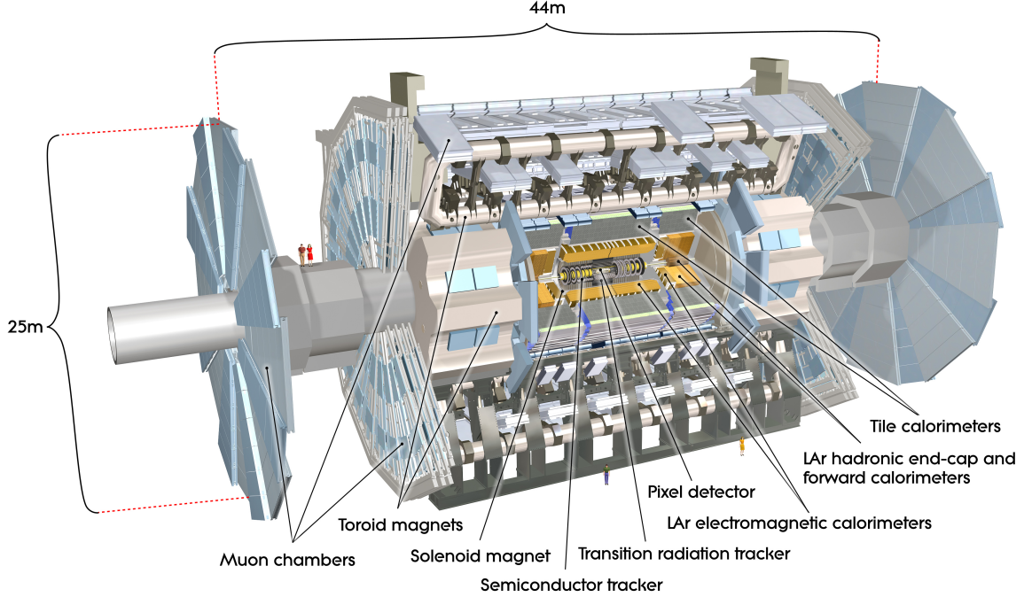
Figure 3.2: The ATLAS detector with its subdetectors labelled.
