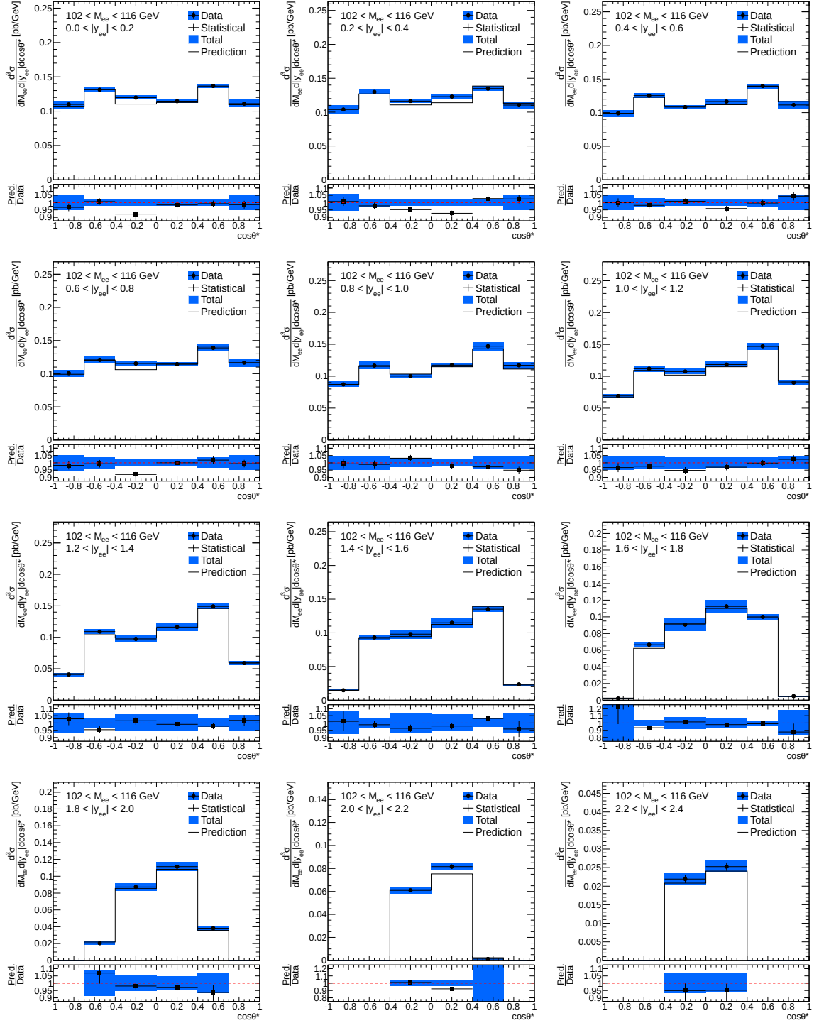
Figure 9.5: Three-dimensional differential cross-section \frac{d^3\sigma}{dM_{ee} d|y_{ee}| d\cos\theta^*} results for invariant mass bin M_{ee} \in [102, 116] GeV and for the entire rapidity range of interest, 0.0 < |y_{ee}| < 2.4 .
