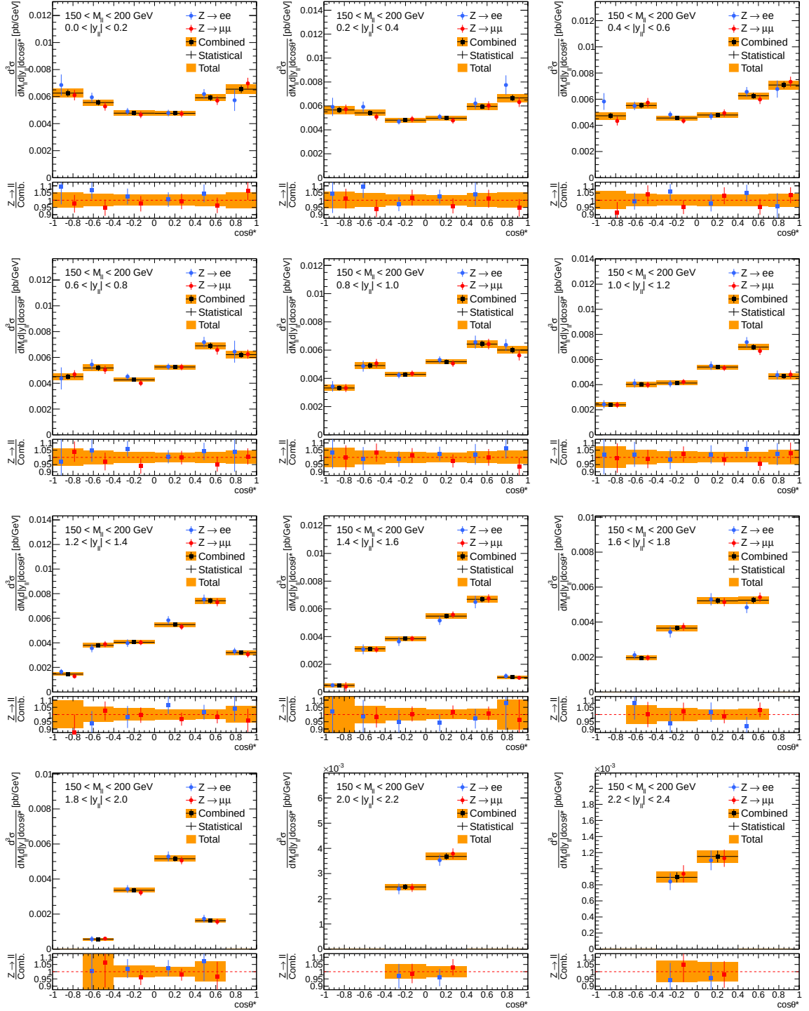
Figure C.10: Combined three-dimensional differential cross-section \frac{d^3\sigma}{dM_{\ell\ell} dy |d \cos \theta^*|} results for invariant mass bin M_{\ell\ell} \in [150, 200] GeV and for the entire rapidity range of interest, 0.0 < |y_{ee}| < 2.4 .
