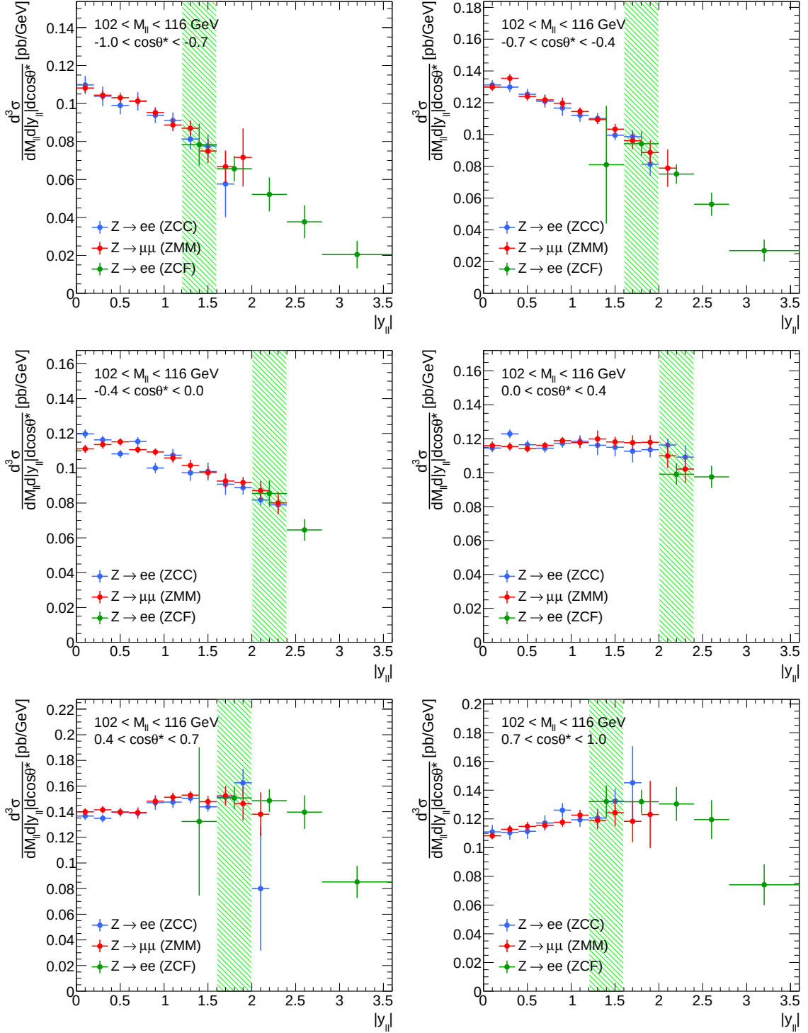
Figure C.14: Central-central, muon-muon, and central-forward three-dimensional differential cross-section \frac{d^3\sigma}{dM_{\ell\ell}d|y_{||}|d\cos\theta^*} results for invariant mass bin M_{\ell\ell} \in [102, 116] GeV and for the entire polar angle range of interest, -1.0 < \cos\theta^* < 1.0 .
