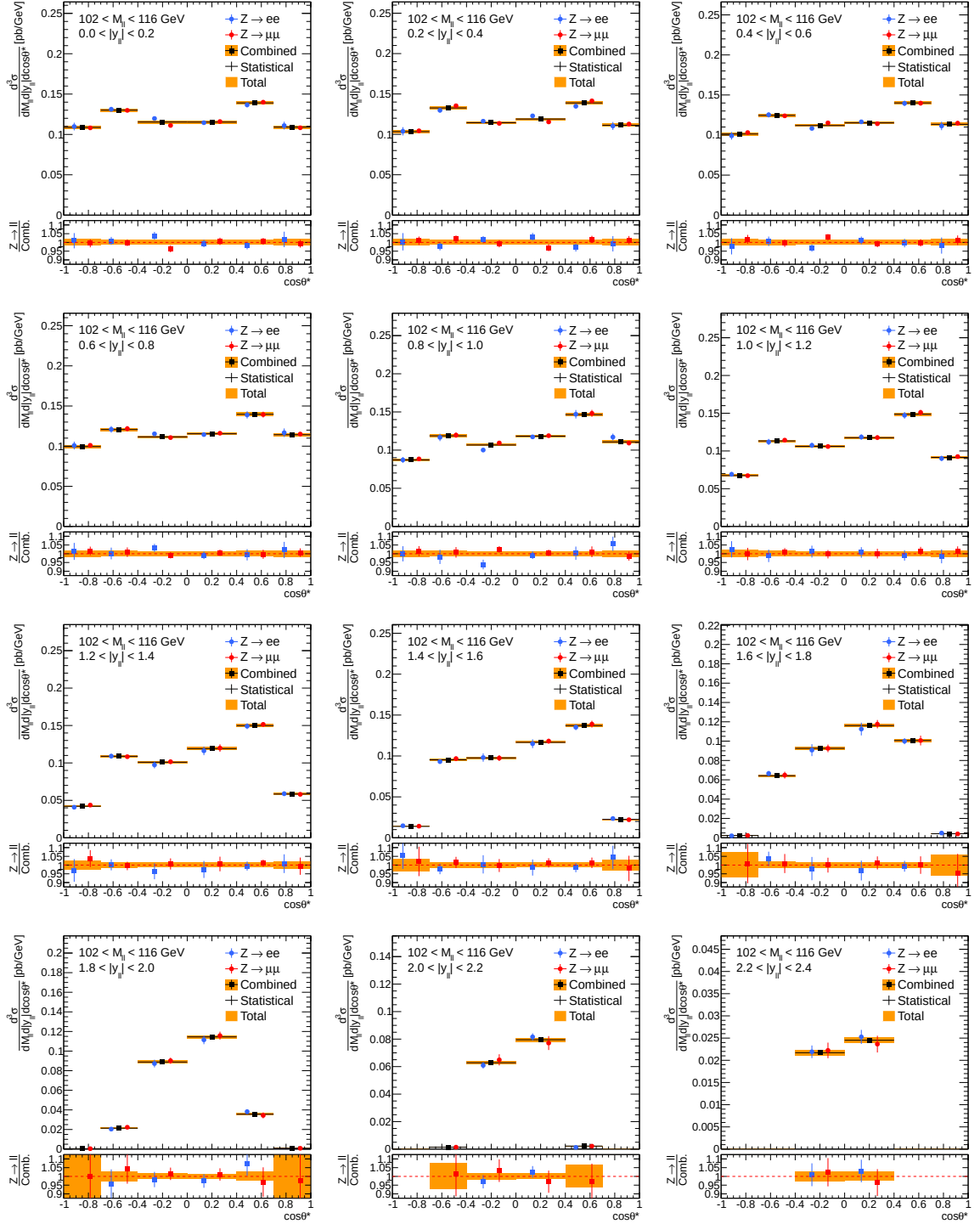
Figure C.8: Combined three-dimensional differential cross-section \frac{d^3\sigma}{dM_{\ell\ell}d|y_{\ell\ell}|d\cos\theta^*} results for invariant mass bin M_{\ell\ell} \in [102, 116] GeV and for the entire rapidity range of interest, 0.0 < |y_{ee}| < 2.4 .
