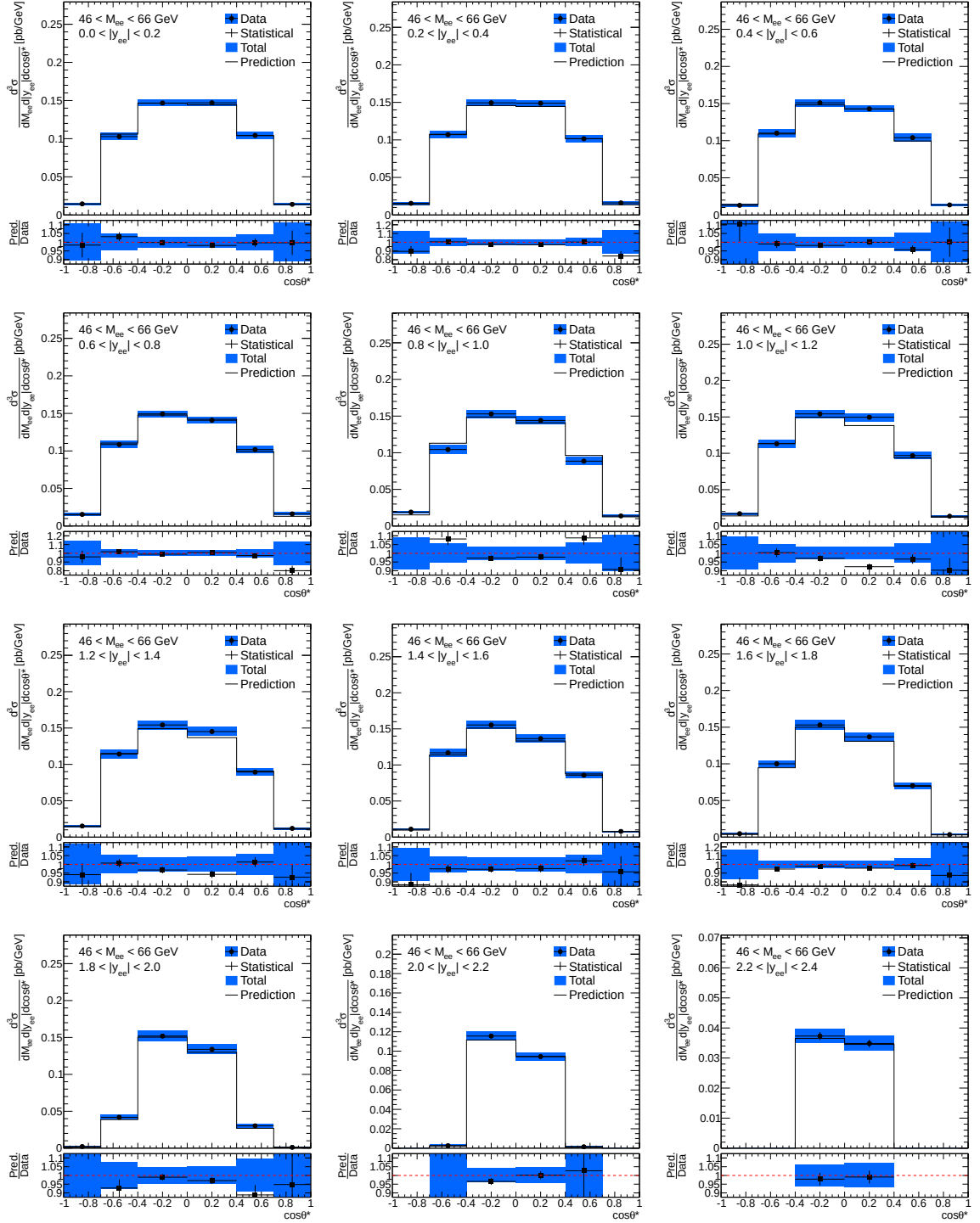
Figure 9.1: Three-dimensional differential cross-section \frac{d^3\sigma}{dM_{ee} d|y_{ee}| d\cos\theta^*} results for invariant mass bin M_{ee} \in [46, 66] GeV and for the entire rapidity range of interest, 0.0 < |y_{ee}| < 2.4 .
