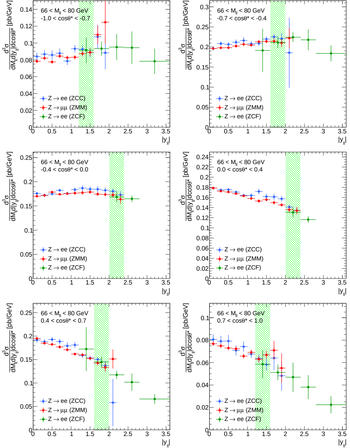
Figure C.11: Central-central, muon-muon, and central-forward three-dimensional differential cross-section \frac{d^3\sigma}{dM_{\ell\ell}d|y_{\ell\ell}|d\cos\theta^*} results for invariant mass bin M_{\ell\ell} \in [66, 80] GeV and for the entire polar angle range of interest, -1.0 < \cos\theta^* < 1.0 .
