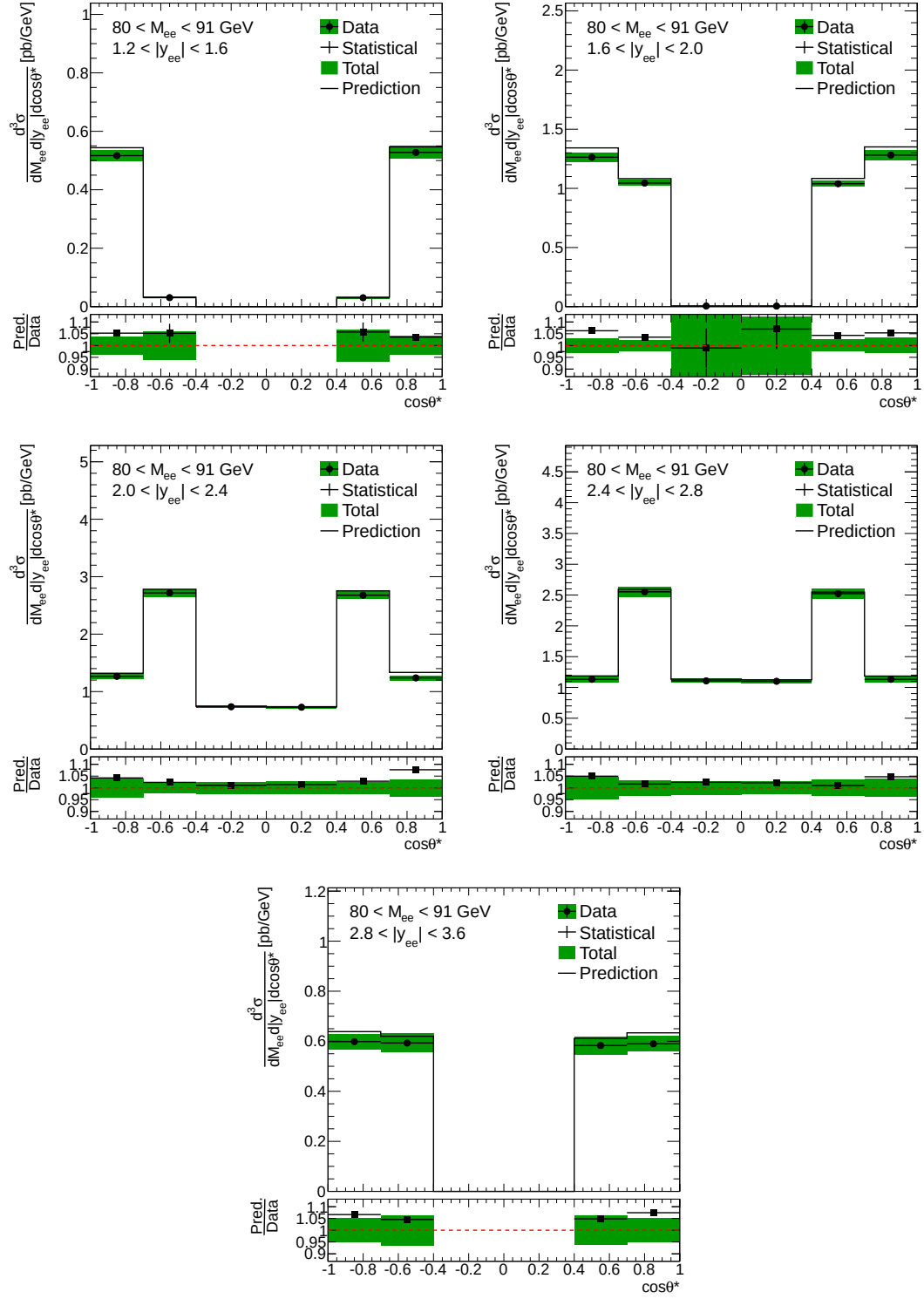
Figure B.23: Three-dimensional differential cross-section \frac{d^3\sigma}{dM_{ee}d|y_{ee}|d\cos\theta^*} results for invariant mass bin M_{ee} \in [80, 91] GeV and for the entire rapidity range of interest, 1.2 < |y_{ee}| < 3.6 .
