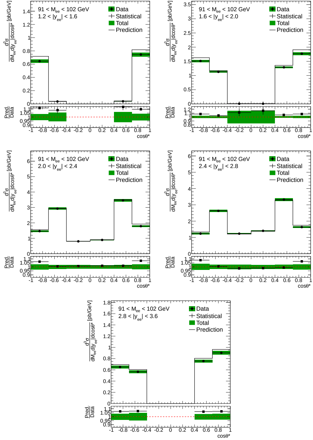
Figure B.24: Three-dimensional differential cross-section \frac{d^3\sigma}{dM_{ee}d|y_{ee}|d\cos\theta^*} results for invariant mass bin M_{ee} \in [91, 102] GeV and for the entire rapidity range of interest, 1.2 < |y_{ee}| < 3.6 .
