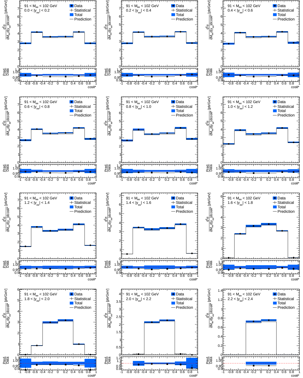
Figure 9.4: Three-dimensional differential cross-section \frac{d^3\sigma}{dM_{ee}d|y_{ee}|d\cos\theta^*} results for invariant mass bin M_{ee} \in [91, 102] GeV and for the entire rapidity range of interest, 0.0 < |y_{ee}| < 2.4 .
