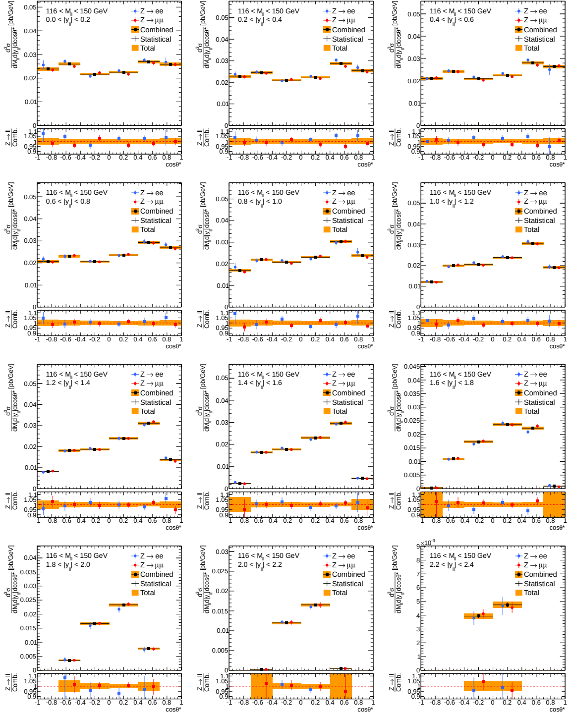
Figure C.9: Combined three-dimensional differential cross-section \frac{d^3\sigma}{dM_{\ell\ell} dy_{\ell\ell} d\cos\theta^*} results for invariant mass bin M_{\ell\ell} \in [116, 150] GeV and for the entire rapidity range of interest, 0.0 < |y_{ee}| < 2.4 .
