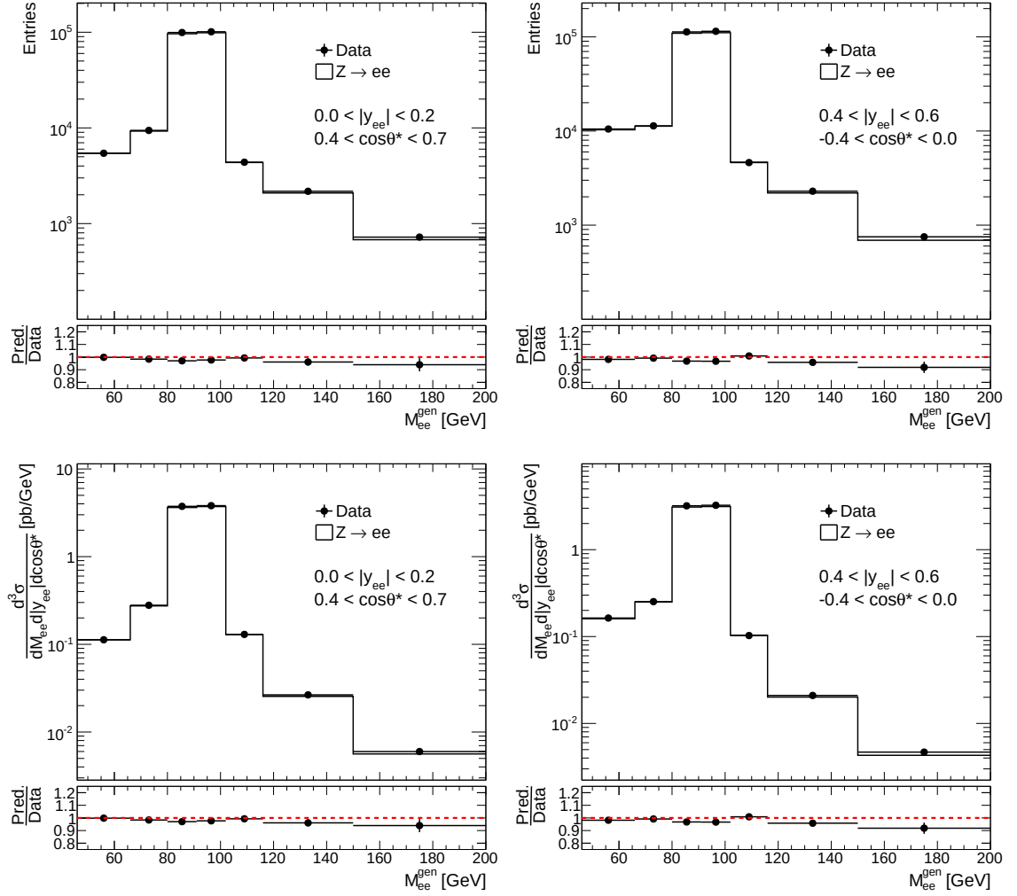
Figure 7.15: Unfolded invariant mass distributions at dressed-level (top) and their corresponding three-dimensional differential cross-sections (bottom).
