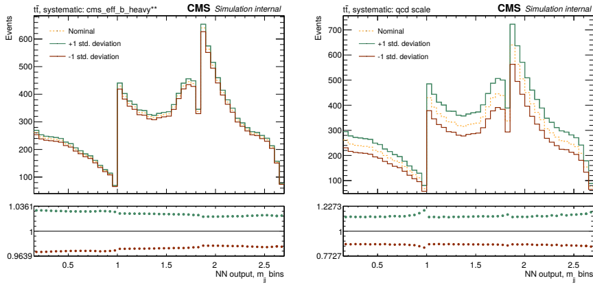
Figure 3.17. Effect of heavy-flavour jet b tagging efficiency uncertainties (left) and of the renormalisation and factorisation scale variations (right) on the shape and normalisation of the templates for the t\bar{t} process. The distribution of the resonant ANN evaluated at m_\chi = 400 GeV in the e^\pm \mu^\mp channel is shown (other channels yield similar behaviours). The yield in each bin of the distribution is continuously interpolated between the down (“-1 std. deviation”), nominal and up (“+1 std. deviation”) predictions, as detailed in Sec. 2.4.2.
