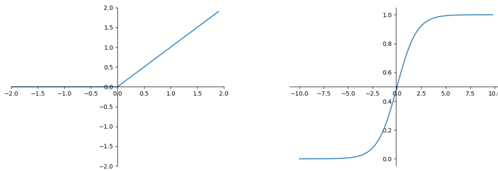
Fig. 31: Common nonlinear activation functions used in modern neural networks. Left: the Rectified Linear Unit (ReLU); Right: the sigmoid ( \sigma ) function.
