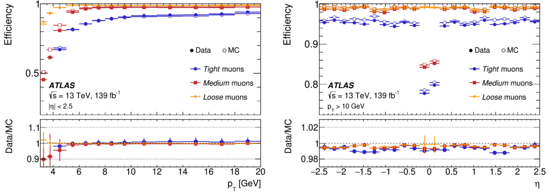
Fig. 27: ATLAS Run 2 muon reconstruction and identification efficiencies for the Loose, Medium, and Tight working points are calculated in both data and MC for (left) J/\Psi \rightarrow \mu\mu events as a function of p_T and (right) for Z \rightarrow \mu\mu events as a function of \eta . Above p_T > 15 GeV, all working points exceed 90% efficiency for |\eta| < 2.5 . For |\eta| > 0.1 , all working points exceed 95% efficiency for p_T > 10 GeV. [28]
