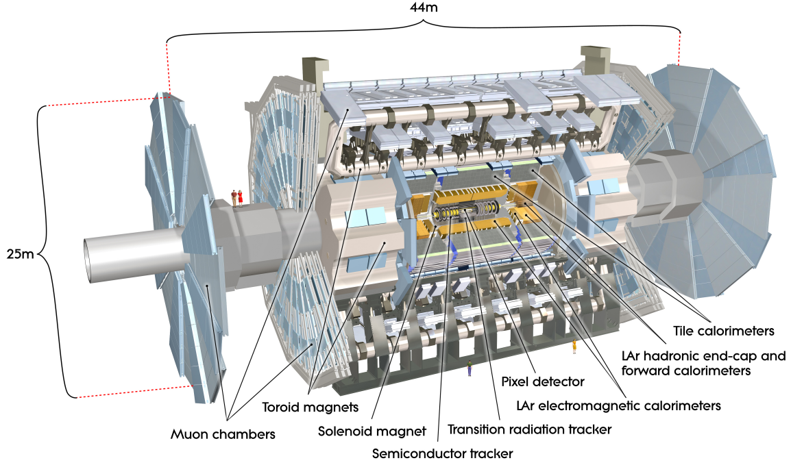
Fig. 15: The ATLAS detector, with two human figures shown standing near the leftmost muon chambers to convey a sense of scale.
