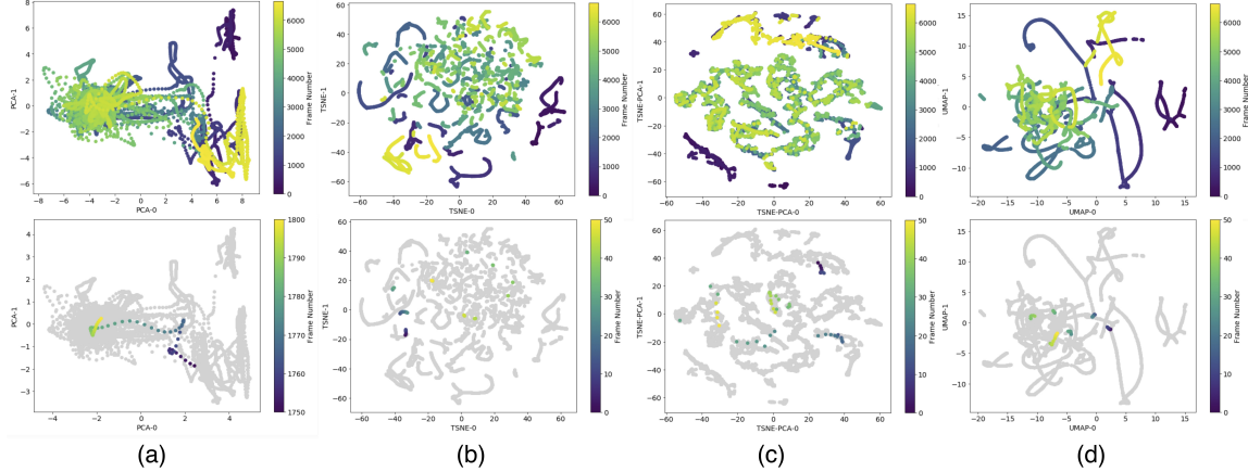
Fig. 47: A variety of 2D latent spaces are compared across multiple linear and nonlinear dimensionality-reduction techniques (excluding autoencoders): (a) PCA, (b) t-SNE, (c) t-SNE following PCA, and (d) UMAP. The top row shows full latent spaces for a subset of the training data, while the bottom row highlights the same example sequence of 50 frames in each space. All but PCA show a very segmented and discontinuous path for the sequence across the latent space. Our autoencoder techniques (see Figure 46) are comparable to PCA in terms of continuity of the paths in latent space, but have a much higher capacity to learn complex, nonlinear relationships than PCA alone.
