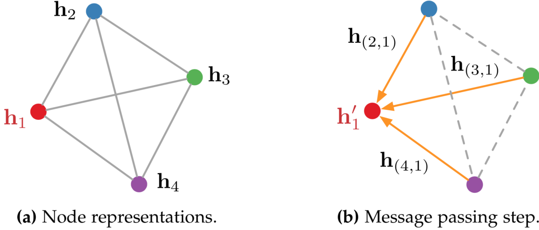
Fig. 36: An example of message passing implemented on a fully-connected graph with four nodes. Left: Each of the four nodes has a hidden node representation h_i . Right: To update the hidden representation h_1 corresponding to Node 1, messages are aggregated from each incoming edge from the neighborhood of Node 1. [36]
