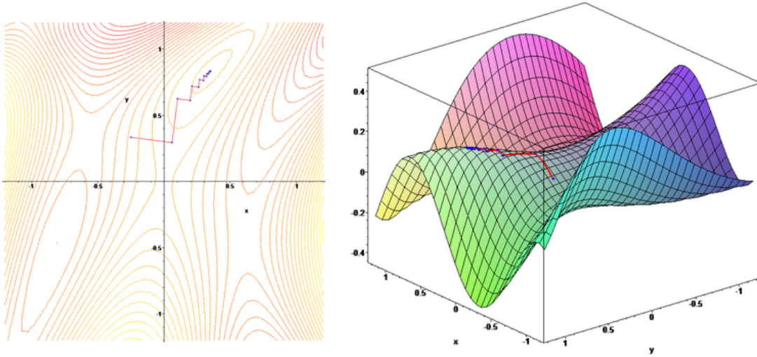
Fig. 32: An illustration of gradient descent in a challenging loss landscape ( left: in 2D; right: in 3D) shows a trajectory towards a local minimum of the loss function. Step sizes decrease as the model gets closer to the local minimum and the gradient decreases. Public domain images from Wikimedia Commons.
