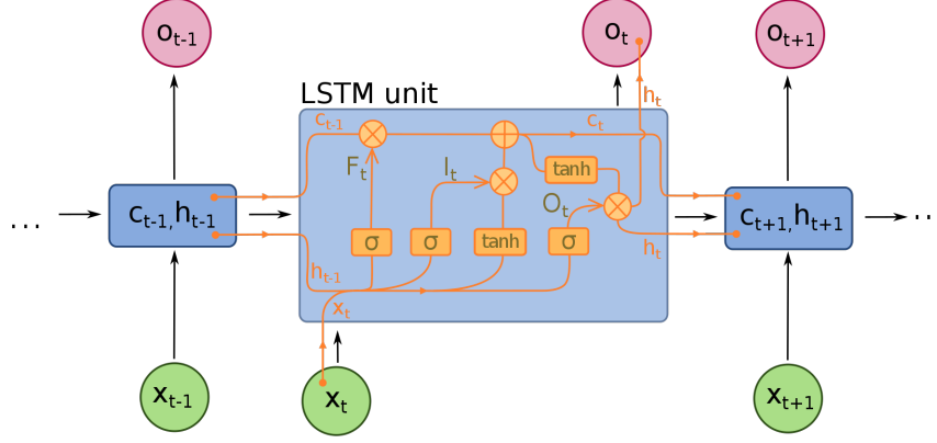
Fig. 33: A diagram of an LSTM unit, with information flowing from bottom to top. An input sequence (x_{t-1}, x_t, x_{t+1}, \dots) is fed into the LSTM cell with input gate I_t , forget gate F_t , and output gate O_t , and the cell outputs a sequence (o_{t-1}, o_t, o_{t+1}, \dots) . (Public domain image from Wikimedia Commons).
