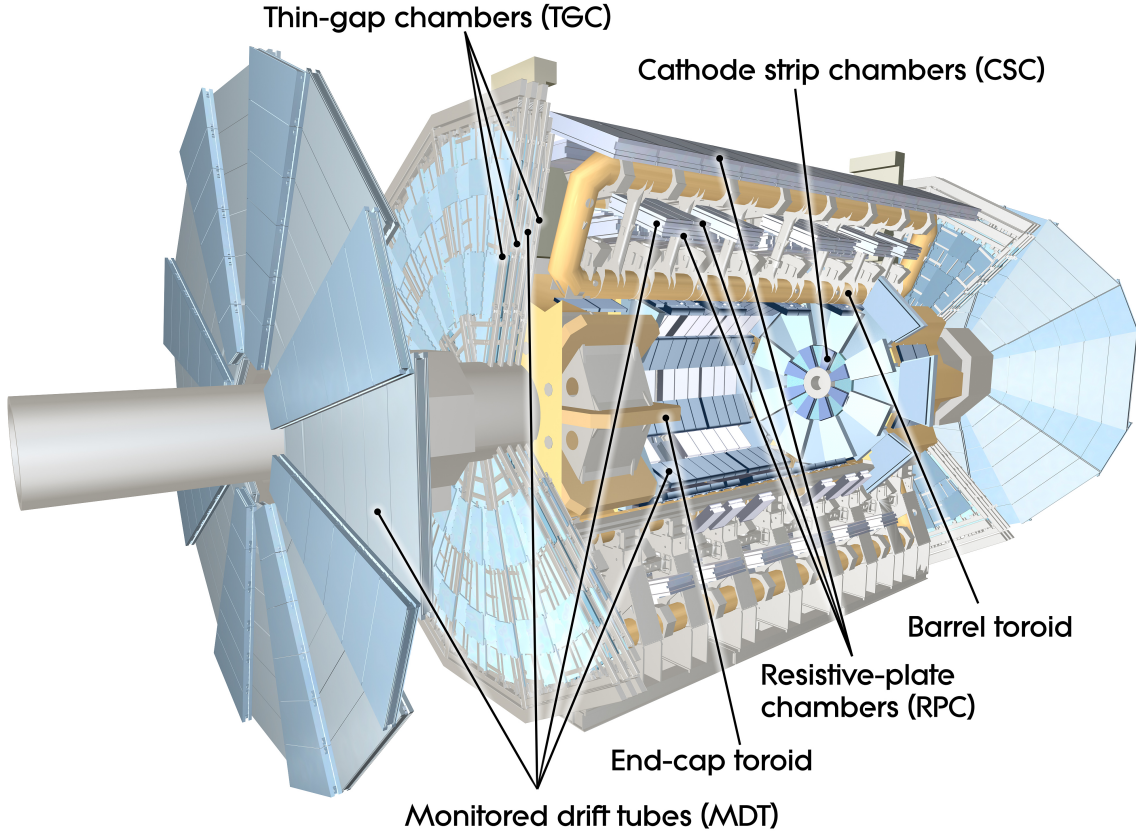
Fig. 19: The ATLAS muon spectrometer subsystem.
