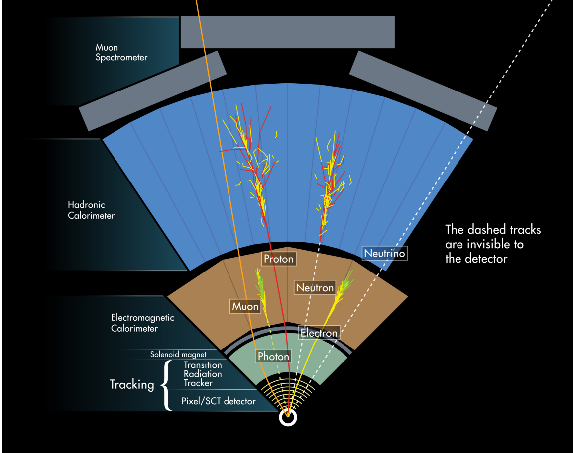
Fig. 16: A cross-sectional view of one portion of the ATLAS detector, with its Inner Detector, EM and Hadronic Calorimeters, and Muon Spectrometer. [17]
