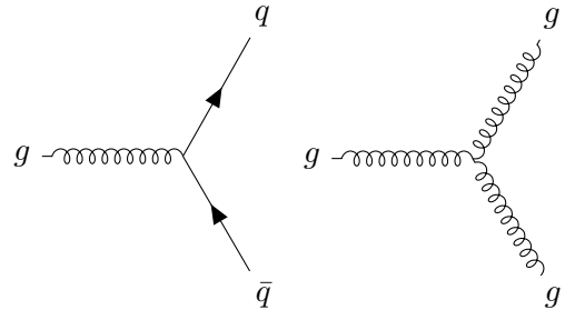
Fig. 3: Primary allowed 3-particle vertices for Quantum Chromodynamics (QCD), i.e. the strong force, where q is any flavor of quark.
