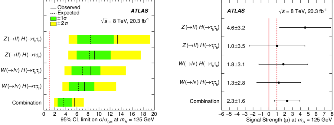
Fig. 64: The combined Run 1 VH , H \rightarrow \tau\tau measurements. On the left, the 95% confidence-level (CL) upper limits for \sigma/\sigma_{SM} for each of the four signal regions are shown, along with the combined upper limit for all four channels. Expected upper limits are shown in dotted lines, while observed upper limits are shown in solid lines. The lime green regions mark the \pm 1\sigma significance interval, while the yellow regions mark the \pm 2\sigma significance interval. On the right, the measured signal strength \mu = \sigma/\sigma_{SM} for m_H = 125 GeV is shown for each signal region individually and combined. The dashed vertical red line indicates a perfectly Standard Model-like result. Each of the four categories shows a measurement of the signal strength \mu that is consistent, within error bars, with the Standard Model prediction. [93]
