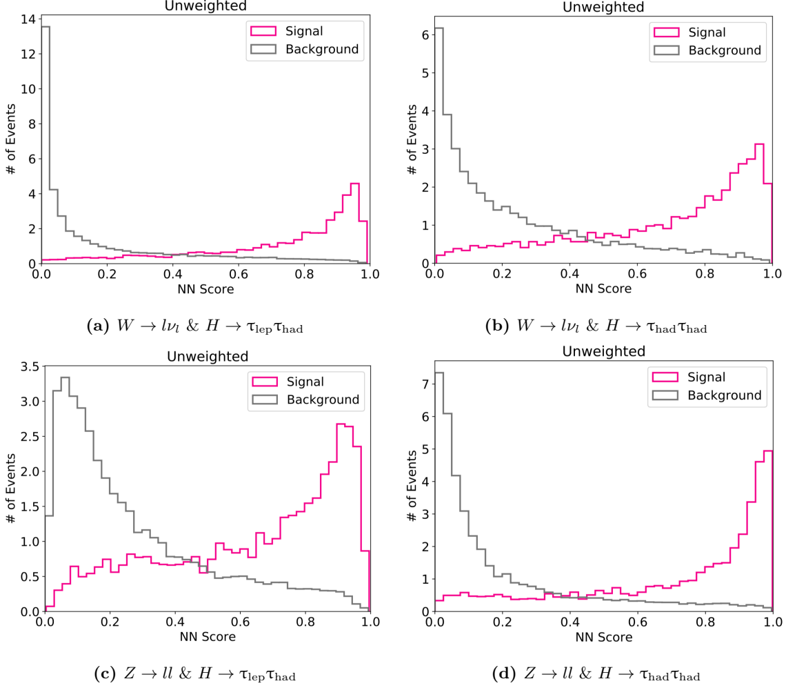
Fig. 61: Unweighted & normalized plots of test signal and background MC sorted by the neural network output score.
