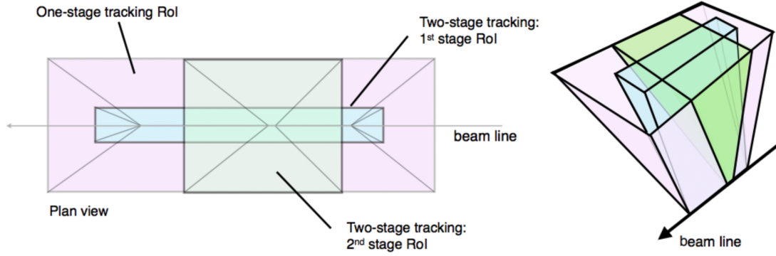
Fig. 40: The geometric ranges searched during the Fast Track Finder (FTF) in the first portion of tracking in the ATLAS HLT are shown. The pink region shows the region of interest (RoI) identified at Level 1. In blue is the first range searched: \Delta R < 0.1 and |z| < 225 mm. In green is the second range searched: \Delta R < 0.4 and |z| < 10 mm.
