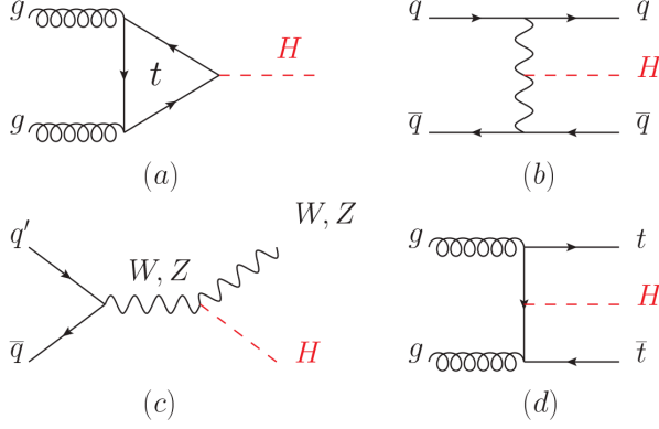
Fig. 7: Higgs boson production mechanisms. [5]
