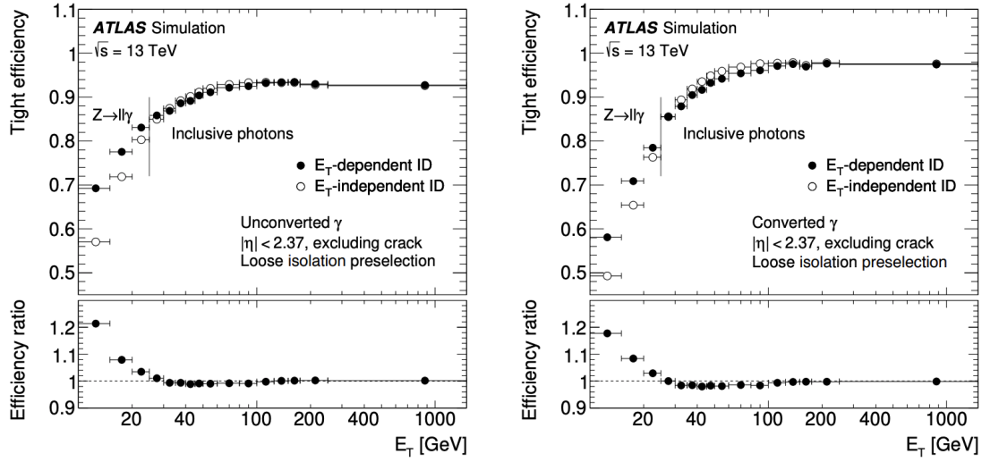
Fig. 26: Identification efficiencies versus E_T for the tight working point for unconverted (left) and converted (right) photons in |\eta| < 2.37 . For E_T < 25 GeV, events come from Z \rightarrow ll\gamma , and for E_T > 25 GeV, events come from inclusive photon production. [27]
