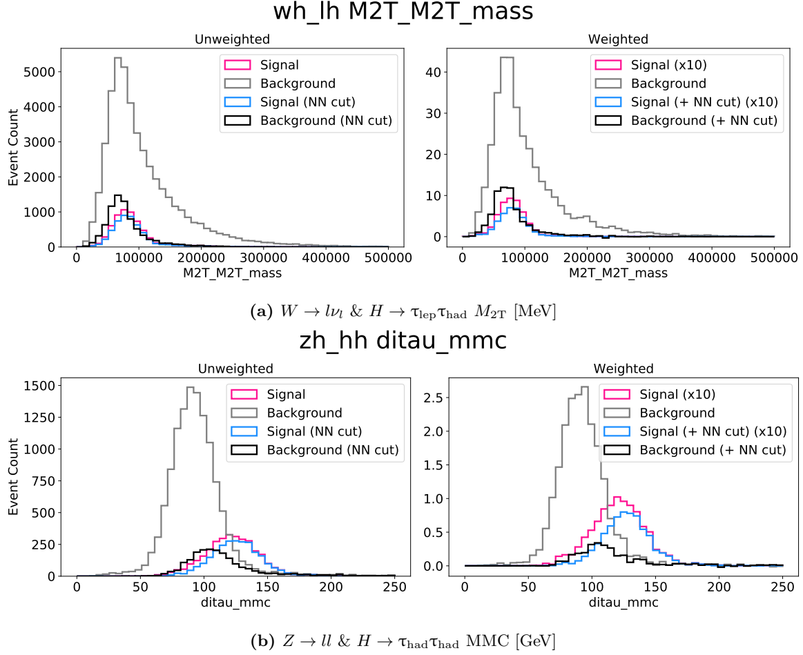
Fig. 62: Example unweighted and MC-weighted distributions of M_{2T} (above, in the WH LepHad channel) and MMC (below, in the ZH HadHad channel) for signal and background before (in pink and grey) and after (in blue and black) the cut on the neural network output score show a large decrease in background events with relatively few signal events lost by comparison. The peaks of the signal mass distributions move very little following the neural network score cut and are also still fairly distinct from the peaks of the diboson backgrounds. The signal has been given an additional weight factor of 10X in the weighted histograms for the purposes of visibility during plotting.
