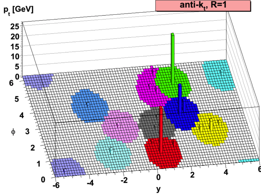
Fig. 28: The clustering results of the anti- k_t jet-finding algorithm for a parton-level event are shown as a function of \phi , y , and p_T . [29]
