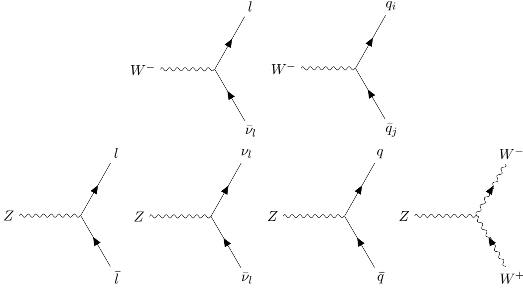
Fig. 4: Primary allowed 3-particle vertices for the electroweak (EW) force. Notably, flavor-changing neutral currents are disallowed, meaning the Z must couple with fermions of the same flavor.
