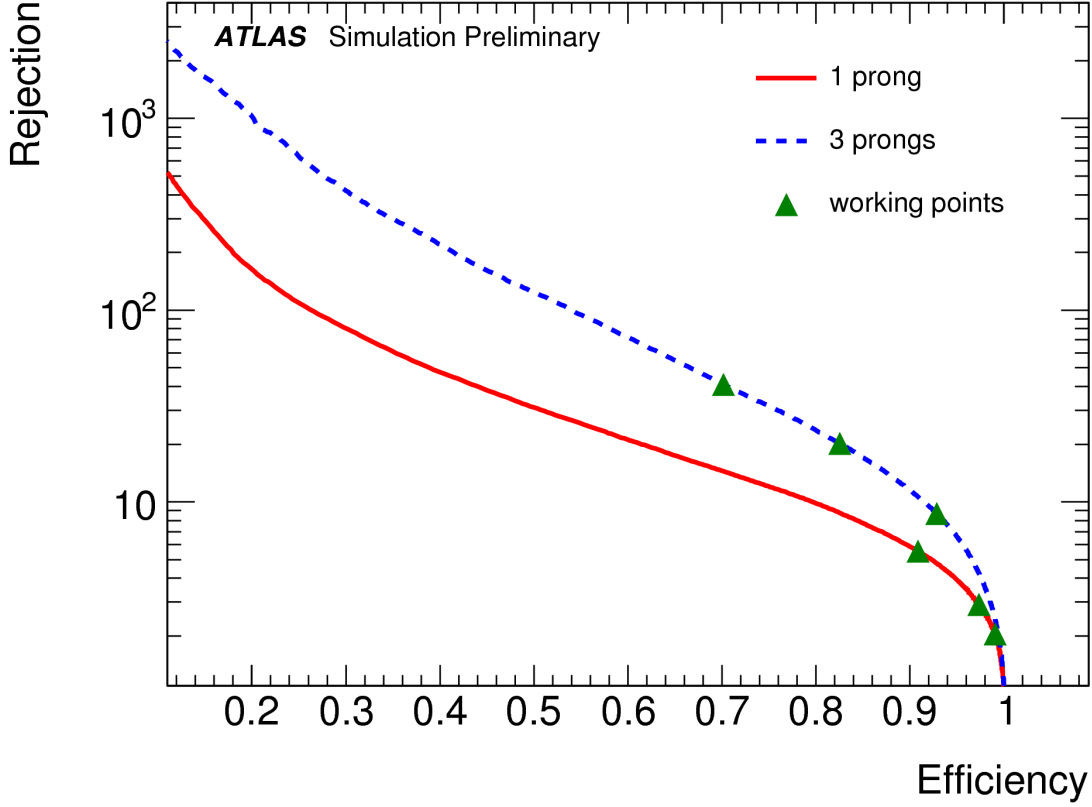
Fig. 41: Background rejection vs. signal efficiency curves for the 1-prong (solid red line) and 3-prong (dashed blue line) tau identification BDT models used in the ATLAS HLT at the beginning of Run 2. The tight , medium , and loose working points are marked with green triangles in order of decreasing rejection for each model. [39]
