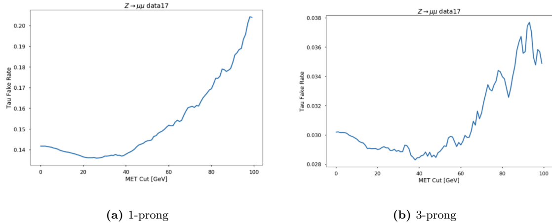
Fig. 59: The tau fake rate as a function of minimum missing E_T cut, measured in a subset of the Run 2 dataset in the fake-enriched region.
