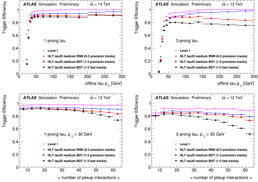
Fig. 44: Trigger efficiencies in MC simulation samples at s = \sqrt{13} TeV for tau triggers with comparable rates. In the left column are efficiencies for 1-prong taus, while in the right column are efficiencies for 3-prong taus. In the top row, the \hat{x} -axis is p_T of offline taus passing the Medium BDT working point. In the bottom row, the \hat{x} -axis is \mu , the average number of pileup interactions. The triggers using RNN tau identification (blue triangles) show better performance across each of these criteria compared to triggers using BDT tau identification with precision tracks (red squares) and fast tracks (black circles), even approaching the efficiency of the Level-1 trigger (pink crosses) for large values of offline tau p_T .
