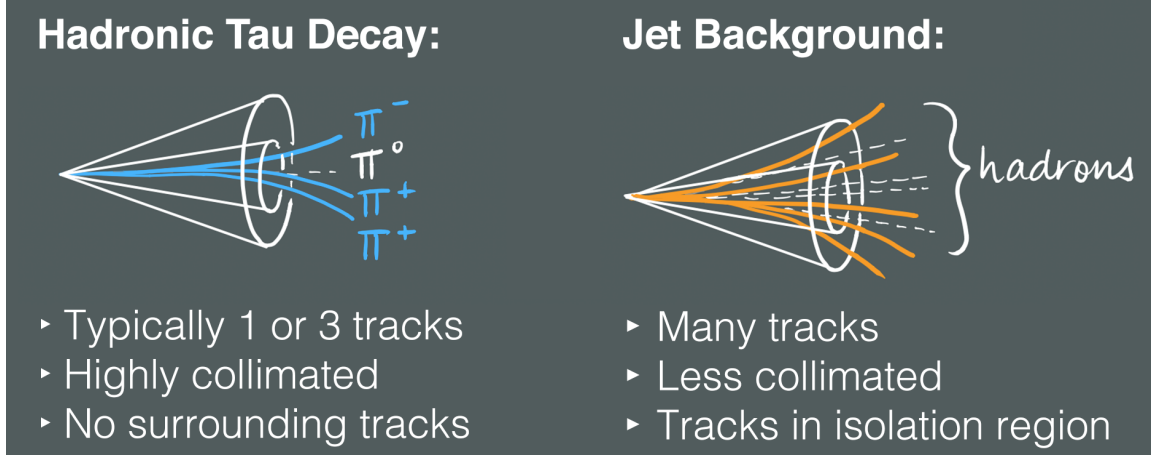
Fig. 38: A diagram of typical signatures of a hadronic tau decay versus a quark- or gluon-initiated jet used to inform hadronic tau identification strategies in the tau trigger. Hadronic taus have constrained numbers of charged tracks from charged hadrons due to charge conservation from the tau parent, and these tracks tend to be collimated in the core region ( \Delta R < 0.2 ) surrounding the reconstructed tau’s center of mass for tau candidates with the same E_T . Quark- or gluon-initiated jets do not have the same charged track number constraints, and depending on their origin, the tracks can tend to be less collimated than those of a hadronic tau. This means that some charged tracks may appear in the isolation region ( 0.2 < \Delta R < 0.4 ) surrounding the core.
