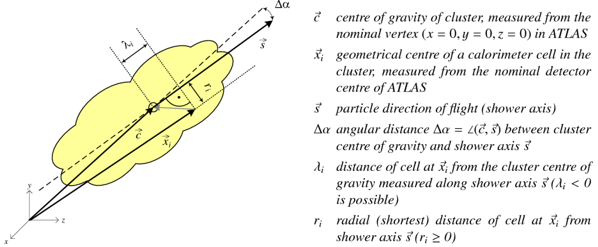
Fig. 42: A diagram of an example calorimeter cluster with its corresponding geometrical cluster moments related to \lambda_{\text{cluster}} and r_{\text{cluster}} . [45]
