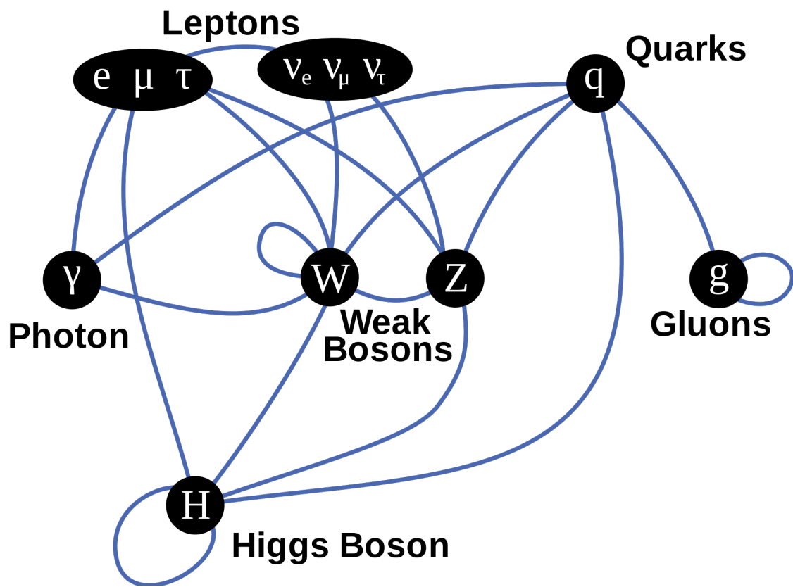
Fig. 1: The fundamental particles of the Standard Model are shown as black circles, while the connections between them indicate how they interact. The photon only interacts with charged particles: the charged leptons and the W boson. The weak bosons, W and Z , interact with all leptons and quarks. Gluons, however, only couple with quarks. Lastly, the Higgs boson couples with every particle that has a mass except neutrinos – the charged leptons, quarks, and weak bosons. (Public domain image from Wikimedia Commons).
