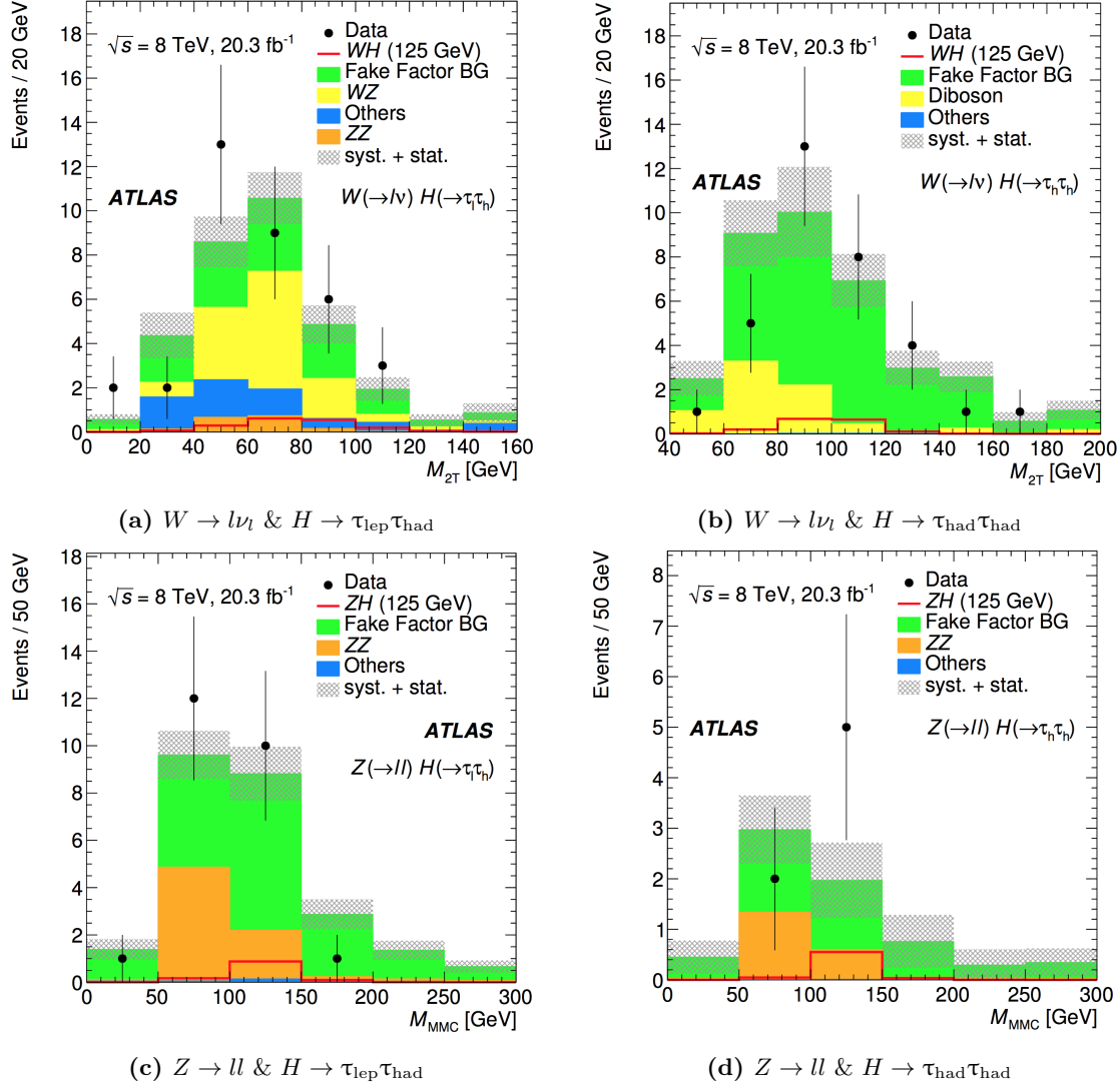
Fig. 63: Expected signal, expected backgrounds, and observed data from Run 1 in each of the four main analysis categories as a function of the reconstructed Higgs boson mass variables. “Others” refers primarily to t\bar{t} events.
