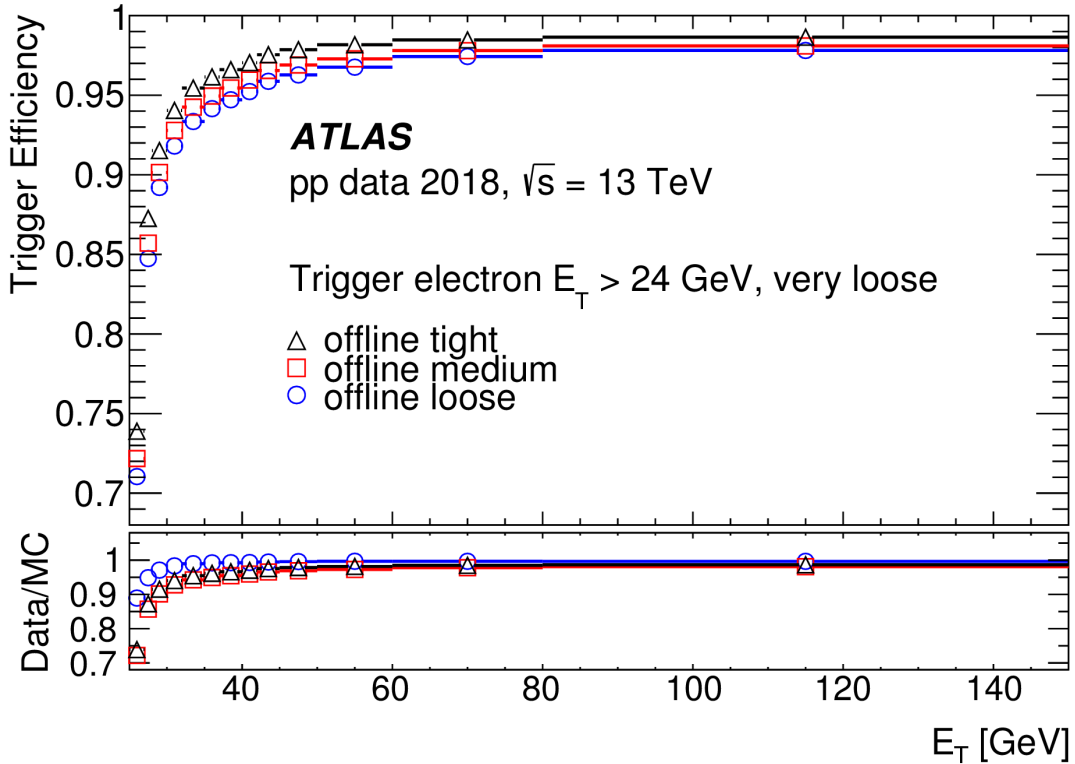
Fig. 54: Efficiency of the HLT_e24_lhvloose_nod0 trigger versus offline electron E_T for 2018 datataking. A steep turn-on curve in efficiency starting at the minimum trigger p_T threshold demonstrates the benefit of applying a slightly higher p_T requirement on our triggered objects. [27]
