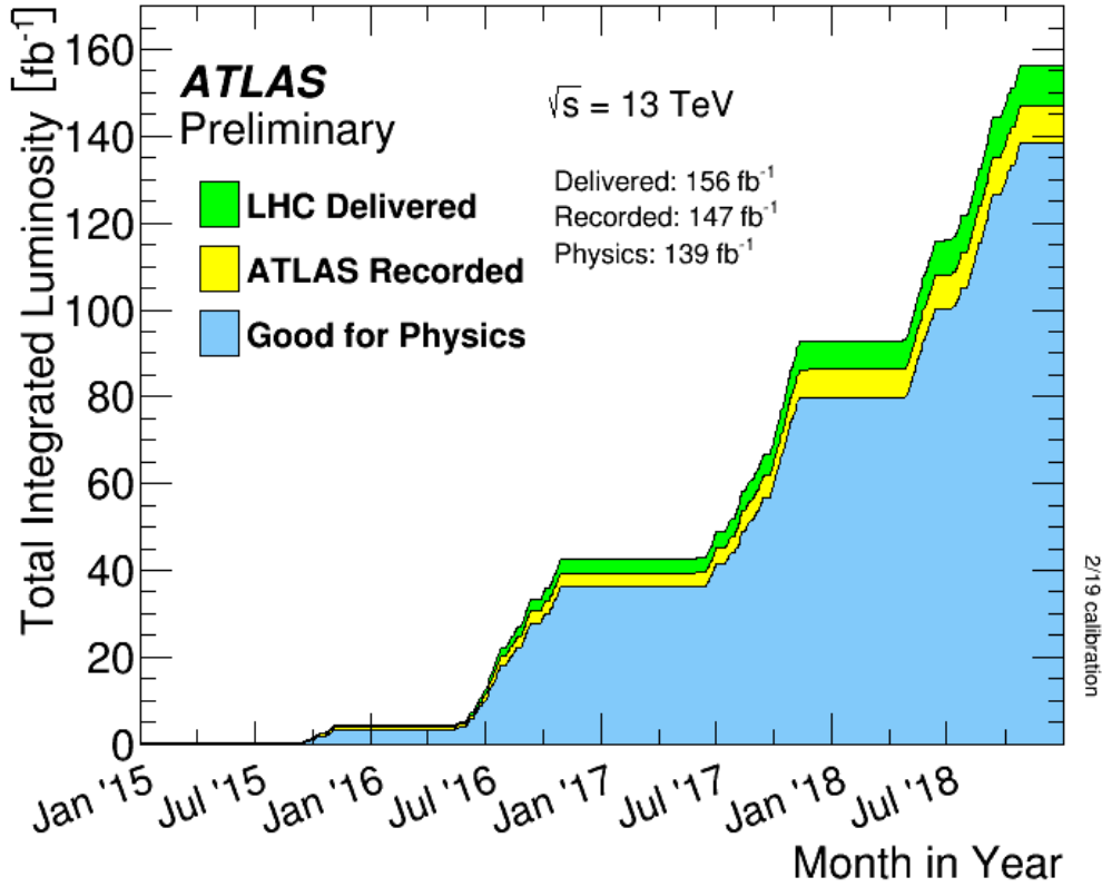
Fig. 14: The cumulative integrated luminosity collected at the LHC over time during Run 2 shows a total amount of data delivered by the LHC to the ATLAS Experiment of 156 \text{ fb}^{-1} (in green). The vast majority of this data is recorded by ATLAS (in yellow), but some data is lost at this stage due to inefficiencies in the data acquisition process and the need to ramp up the voltages of the tracking detectors and pixel system preamplifiers before recording data. Finally, “good for physics” (in blue) denotes data where all physics objects have been reconstructed with good data quality. [14]
