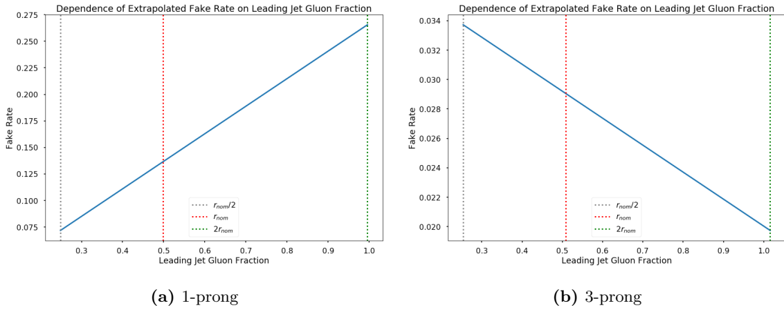
Fig. 60: The extrapolated tau fake rate as a function of gluon jet fraction for the 1-prong and 3-prong cases. As in Run 1, the 1-prong and 3-prong cases are anti-correlated. The three vertical lines correspond to r_{\text{nom}}/2 , r_{\text{nom}} , and 2r_{\text{nom}} , from left to right.
