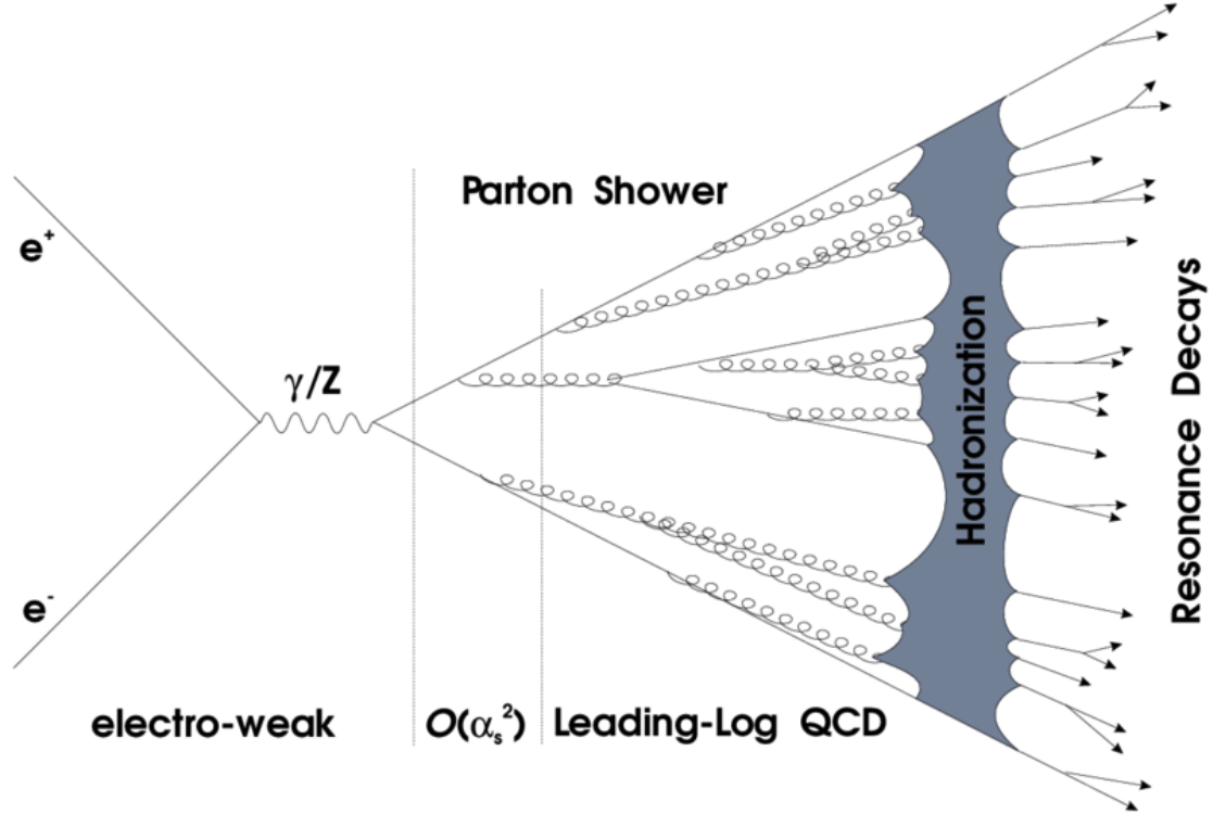
Fig. 22: An example schematic of a QCD hadronization process emerging from electron-positron annihilation into two quarks. From the two final state quarks, we see cascades of partons radiating in parton showers, and then a hadronization stage, followed by the decays of those hadrons. [26]
