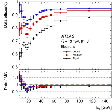
Fig. 25: Electron identification efficiencies measured in Z \rightarrow ee data events as a function of E_T are shown for three working points: loose (blue), medium (red), and tight (black). [27]
