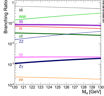
Fig. 8: Higgs boson branching ratios. [5]
