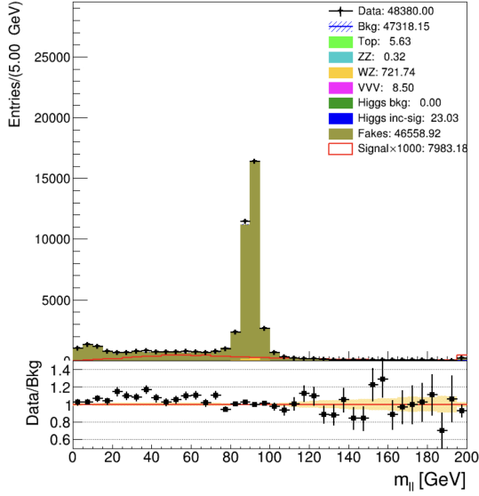
(a) W \rightarrow l\nu_l & H \rightarrow \tau_{\text{lep}}\tau_{\text{had}} (Dilepton mass)
