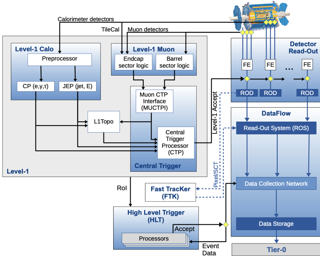
Fig. 21: A schematic of the ATLAS Trigger & Data Acquisition system, including the Level-1 (L1) trigger, the High Level Trigger (HLT), and the flow of data from the detector to permanent storage in the offline Tier-0 computing facility. The Fast Tracker (FTK), shown in this diagram, was planned for rapid track reconstruction at the L1 accept rate in Run 2, but the project was cancelled in 2019 and it was not used by the HLT in Run 2. [24]
