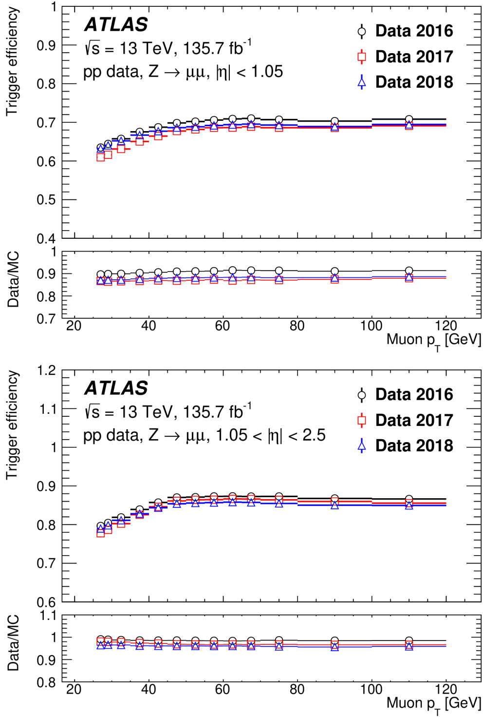
Fig. 55: Efficiency of passing the single muon trigger HLT_mu26_ivarmedium or HLT_mu50 as a function of muon p_T in the barrel (above, |\eta| < 1.05 ) and endcap regions (below, 1.05 < |\eta| < 2.5 ). [28]
