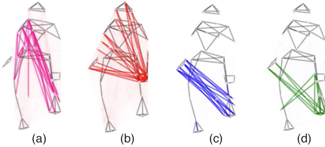
Fig. 52: The top 1% of edges, ranked by the normalized magnitude of each edge's log-probability, for the four learned edge types on the same batch of test data. (a) represents a non-edge, while the other edge types show directed edges going primarily from (b) the left hand to the upper body, (c) right hand to left foot, and (d) left foot to both hands.
