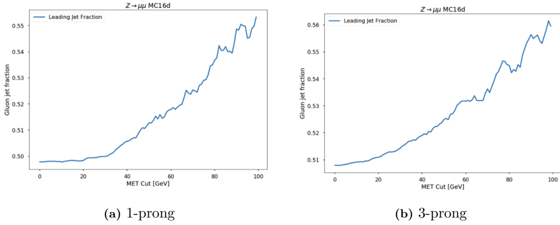
Fig. 58: The fraction of leading jets that are gluon-initiated vs. quark-initiated as a function of minimum missing E_T cut for events with a 1-prong or 3-prong leading tau.
