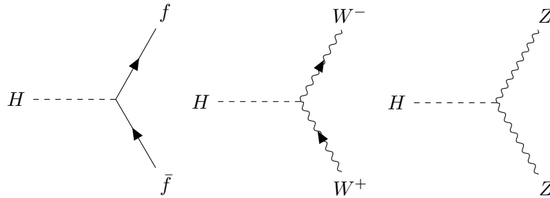
Fig. 5: Primary allowed 3-particle vertices for the Higgs boson.
