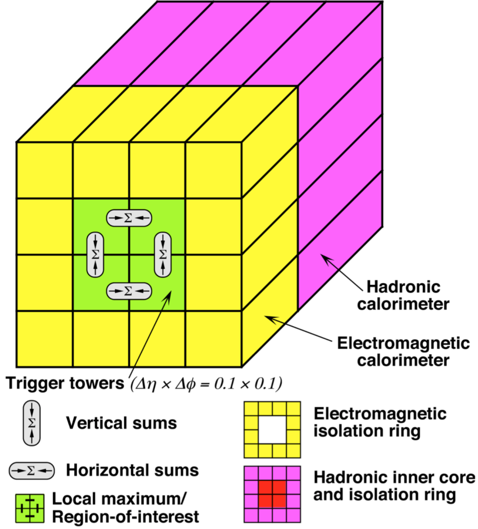
Fig. 39: The Level 1 ATLAS calorimeter towers, with a granularity of \Delta\eta \times \Delta\phi = 0.1 \times 0.1 and a coverage of |\eta| < 2.5 , are shown. The core region of a tau candidate at Level 1 of the trigger is shown in lime green, with its surrounding isolation region in the Electromagnetic and Hadronic calorimeters shown in yellow and pink, respectively. [40]
