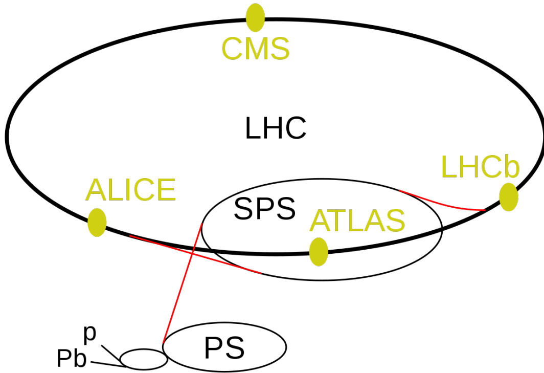
Fig. 11: This schematic of the LHC shows the path of protons (labeled “p” in the bottom left) as they move through a series of linear and circular accelerators before finally reaching the LHC’s main ring, where they receive their final bursts of energy from the RF cavities in order to reach their maximum speed. The four main LHC experiments (in yellow) show the locations of beam crossings and therefore particle collisions.
