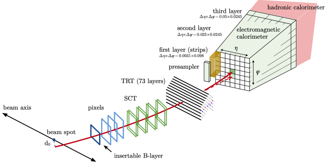
Fig. 23: The red arrow shows an example path of an electron moving through the trackers of the ATLAS inner detector in a curved trajectory before interacting with the EM calorimeter. The red dashed arrow indicates the path of a photon produced as a result of the electron interacting with the tracking material. [27]
