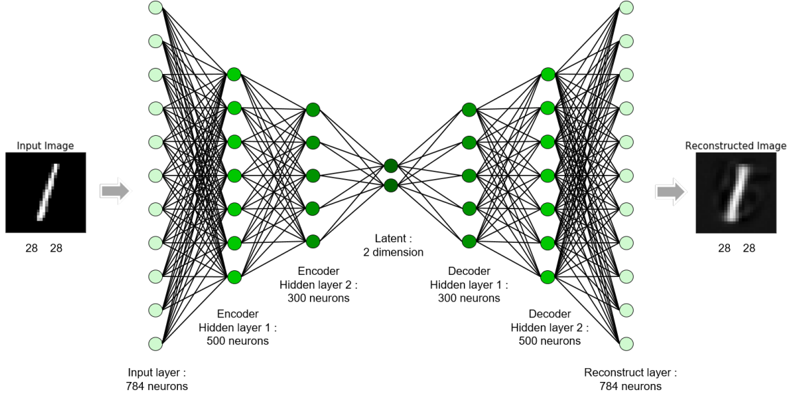
Fig. 34: An example diagram of an autoencoder designed to reconstruct input images of hand-written digits. The input image is split into 784 pixels and fed through the encoder, on the left, until the data has been transformed into an abstract 2-dimensional latent vector. Then, that latent vector is augmented through the decoder until the output matches the dimensions of the input. Once well-trained, the autoencoder’s 2-dimensional latent space has learned a useful representation of the input data such that the image is able to be reconstructed fairly well using a starting point of just 2 dimensions instead of the original 784.
