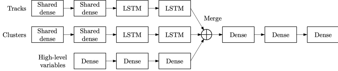
Fig. 43: A diagram of the three branches included in the overall RNN architecture for tracks, clusters, and tau identification variables. [41]
