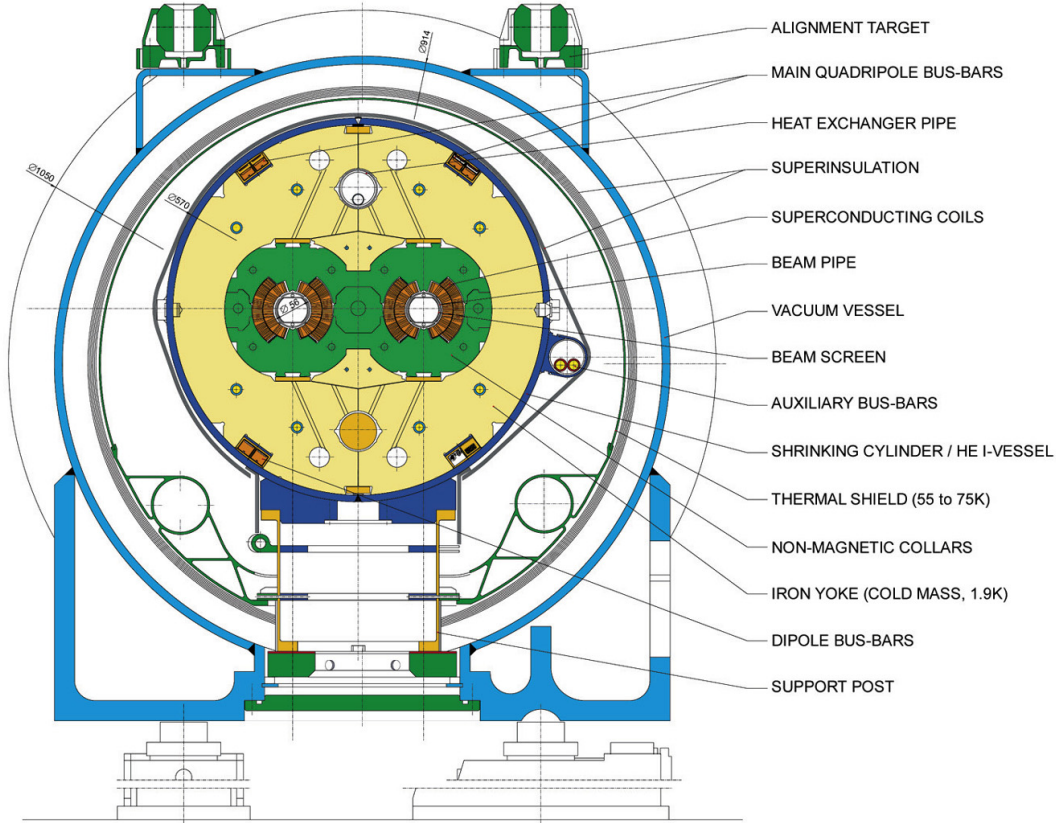
Fig. 12: A cross-sectional view of a dipole magnet at the LHC showing the two beam pipes surrounded by superconducting coils and an iron yoke cooled to a temperature of around 2 Kelvin – colder than the average temperature of empty space.
