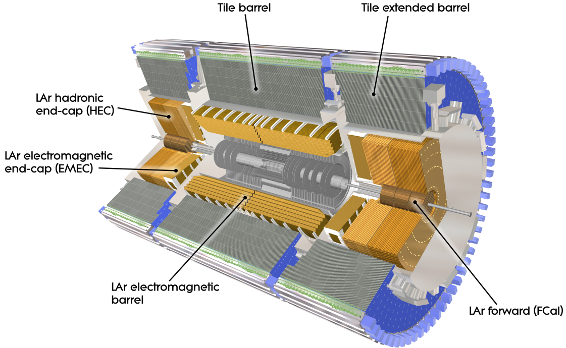
Fig. 18: The ATLAS calorimeter system, including the EM (LAr) & Hadronic (Tile) calorimeters.
