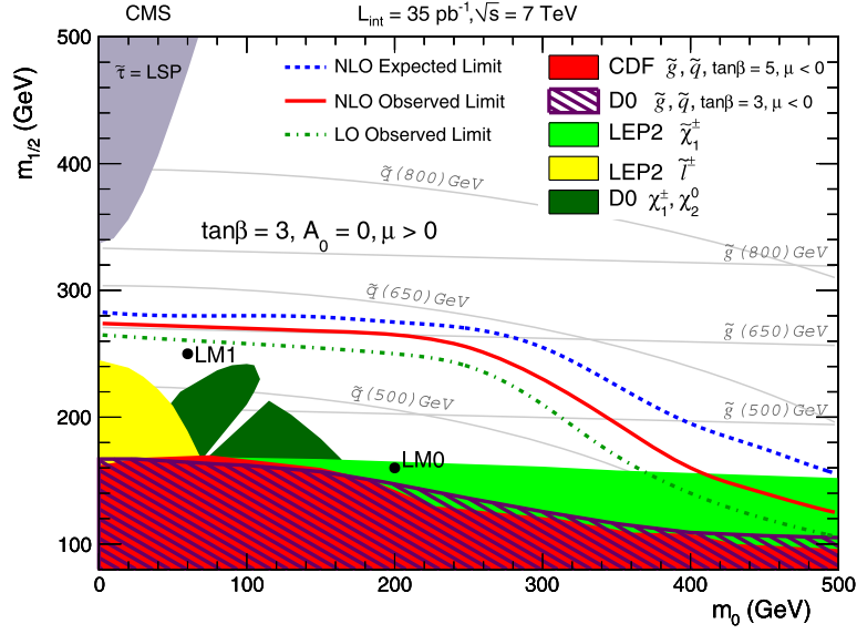
Figure 5.8: Measured (red line) and expected (dashed blue line) 95% CL exclusion contour at NLO in the CMSSM ( M_0, M_{1/2} ) plane ( \tan\beta = 3 , A_0 = 0 GeV, \text{sign}|\mu| > 0 ). The measured LO exclusion contour is also shown as well (dashed green line). The area below the curves is excluded by the measurements presented here. Exclusion limits obtained from previous experiments are presented as filled areas in the plot. Black lines indicate constant squark and gluino masses. For reference, the plot shows the two benchmark points LM0 and LM1 (though it should be noted that for these particular benchmark points, \tan\beta = 10 ).
