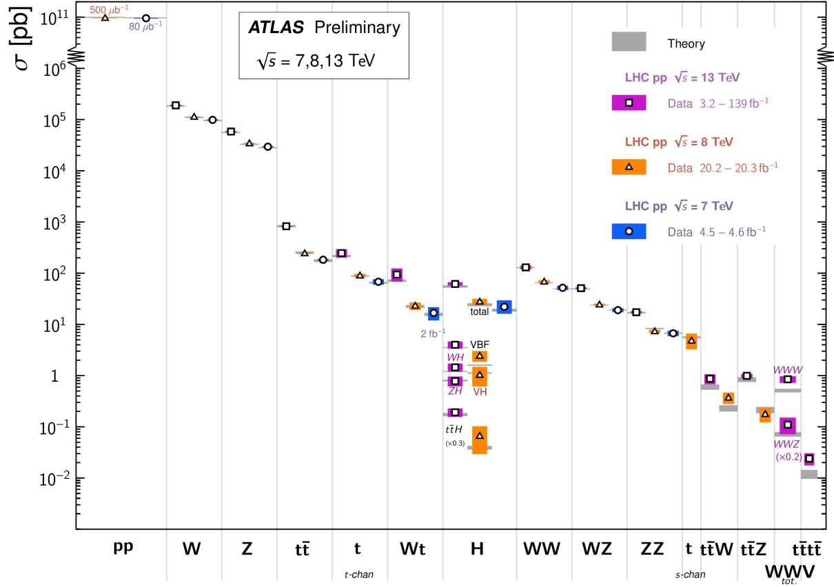
Figure 2.2: Production cross sections of different final states measured by the ATLAS experiment at the LHC. Comparison with the SM theory predictions is also shown [33].
