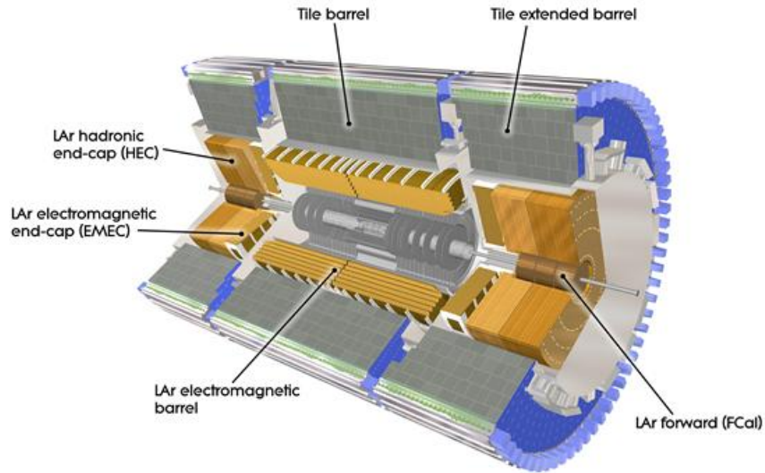
Figure 3.4: Schematic diagram of the ATLAS calorimeter system, with the different segments and the technology used labeled [4].
