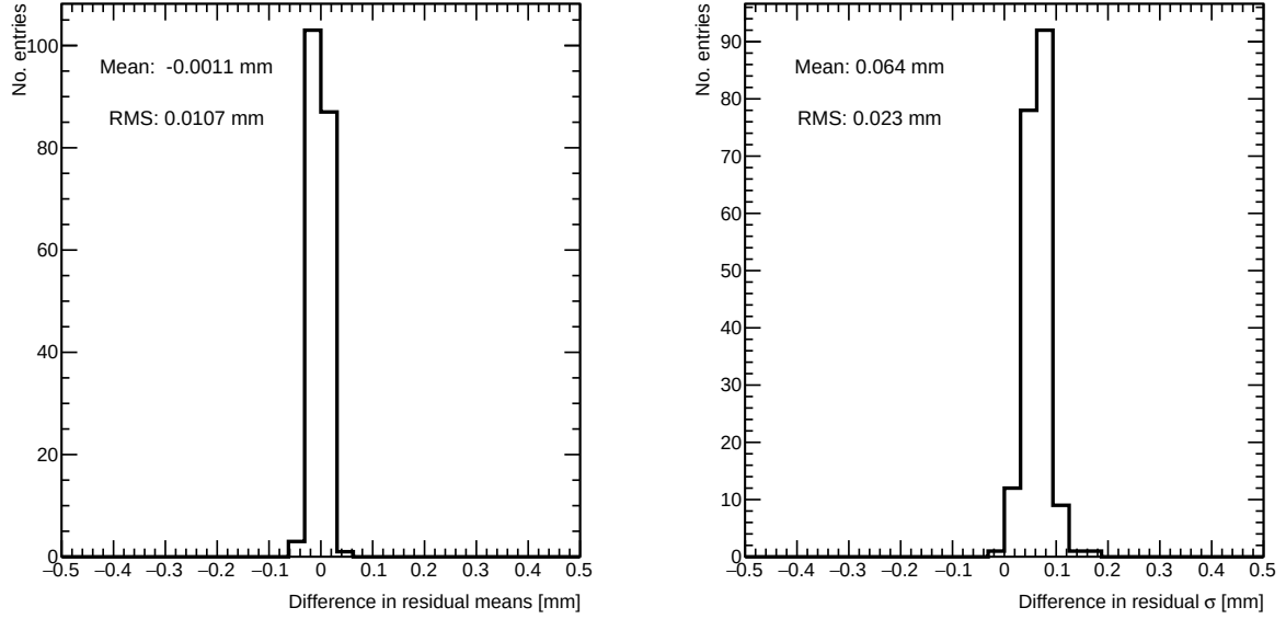
Figure C.7: Difference in residual distribution means and \sigma 's with and without DNL correction for residuals on layer 4 obtained using reference layers 1 and 2 for sample quadruplet, QL2.P.8.
