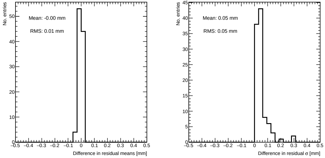
(b) Difference in residual distribution means (left) and \sigma 's (right) for a Gaussian and double Gaussian fit, for all residual distributions in 100 mm by 100 mm bins on layer 2 built from clusters on layers 1 and 3 for sample quadruplet QL2.P.8.
