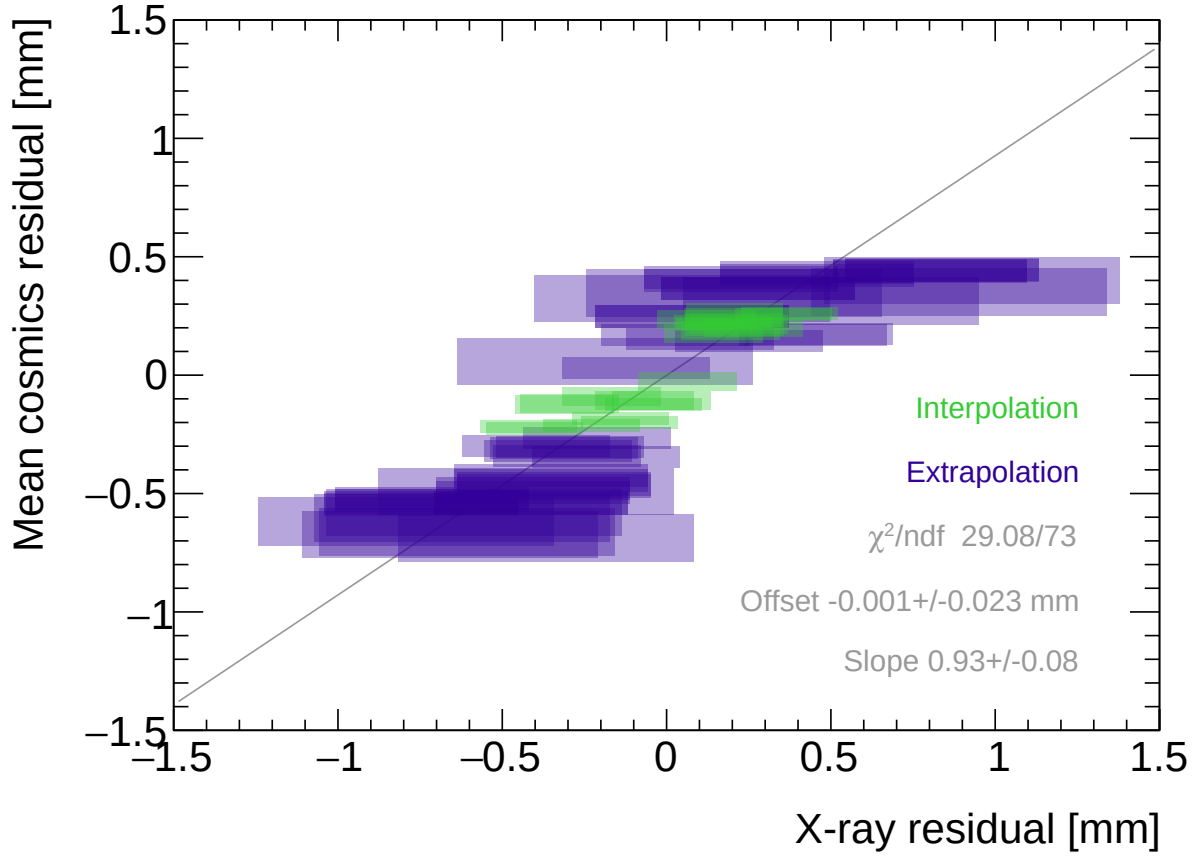
Figure 7.2: Correlation plot between x-ray and mean cosmics residuals for all tracking combinations for QL2.P.11. Each rectangle is centered on an x-ray and mean cosmics residual pair calculated at a given x-ray gun position and for a certain tracking combination. The width of the rectangles in x and y are the uncertainty in the x-ray and mean cosmics residual respectively. A printer-friendly version of this plot is available in Appendix D .
