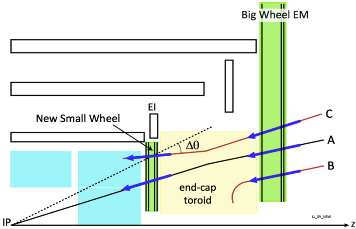
Figure 4.1: A schematic diagram of a quarter cross section of the ATLAS muon spectrometer, with the interaction point (IP) in the bottom left corner. Three possible tracks are labeled. Ideally, track A would be triggered on while track B and C discarded. With the old small wheel, all three tracks would be recorded. With the NSW, only track A would be recorded [5].
