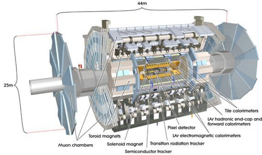
Figure 3.2: Schematic diagram of the ATLAS experiment, with the various detector subsystems labelled [4].
