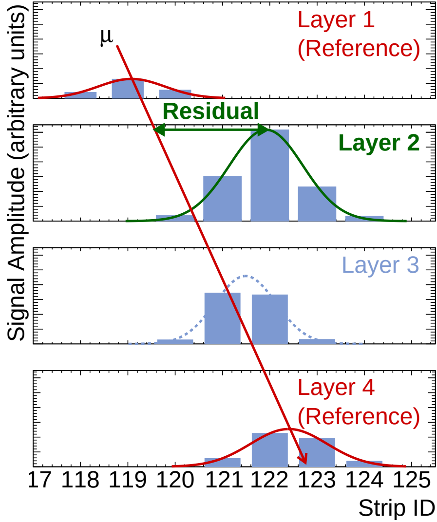
Figure 5.4: Representation of a muon event recorded by an sTGC quadruplet. The charge clusters measured using strip electrodes are fit with a Gaussian distribution and the fitted mean is taken as the reconstructed muon position. A track is built from the chosen reference layers, 1 and 4, and the track residual is calculated on layer 2. The clusters come from a real muon, but their positions were modified to highlight the non-zero value of the residual on layer 2.
