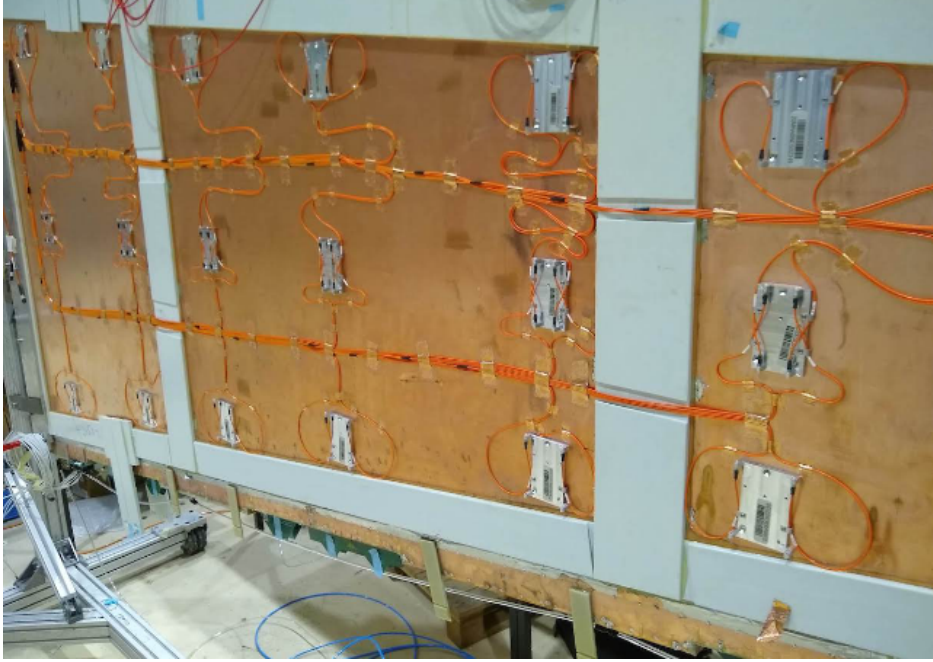
Figure 4.5: A sTGC wedge with alignment platforms (silver) installed on the quadruplet. Optical fibres (orange) are routed to the alignment platforms. Cameras on the frames of the NSWs will record light from the optical fibres to monitor in real-time the position the alignment platforms in the ATLAS coordinate system.
