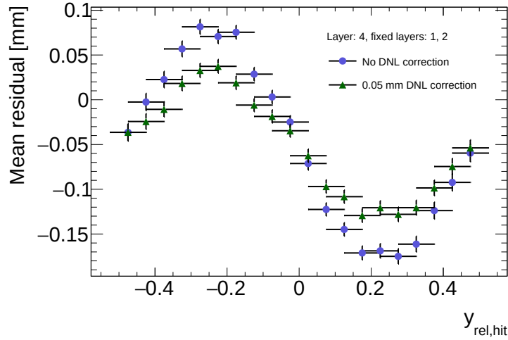
Figure C.6: Effect applying a 50 \mu\text{m} DNL correction to the profile of the residuals sorted by y_{rel} for residuals built from clusters on layers 1 and 2 and extrapolated to layer 4 of quadruplet, QL2.P.8.
