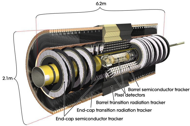
Figure 3.3: Schematic diagram of the ATLAS experiment’s inner detector, with the different segments and the technology used labeled [4].
