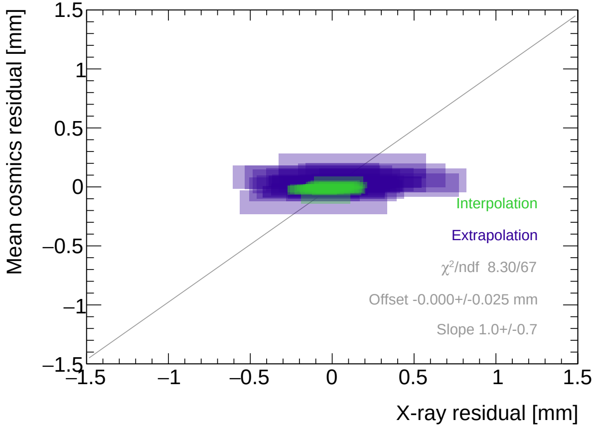
Figure 7.3: Correlation plot between x-ray and mean cosmics residuals for all tracking combinations for QL2.P.8. Each rectangle is centered on an x-ray and mean cosmics residual pair calculated at a given x-ray gun position and for a certain tracking combination. The width of the rectangles in x and y are the uncertainty in the x-ray and mean cosmics residuals respectively. A printer-friendly version of this plot is available in Appendix D .
