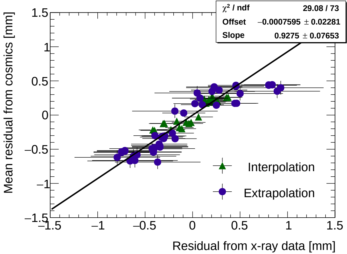
Figure D.1: Correlation plot between x-ray and mean cosmics residuals in 100 mm by 100 mm bins for all tracking combinations for QL2.P.11. This is a printable version of Figure 7.2 in Section 7.1.
