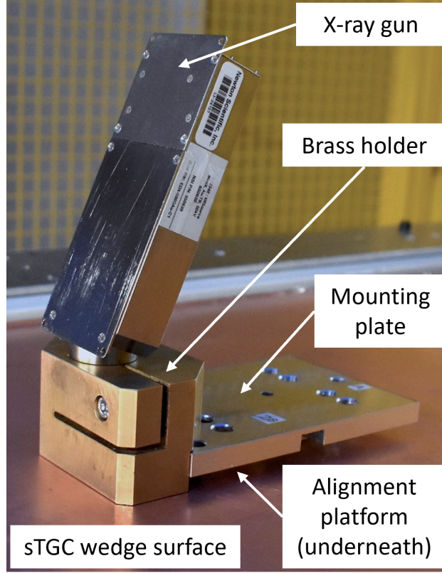
Figure 6.1: The x-ray gun mounted to an alignment platform on the surface of a sTGC wedge. Adapted from [8].
