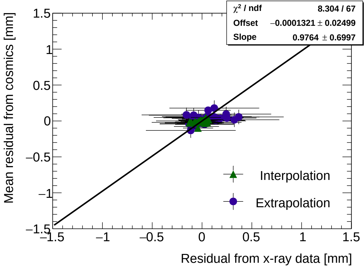
Figure D.2: Correlation plot between x-ray and mean cosmics residuals in 100 mm by 100 mm bins for all tracking combinations for QL2.P.8. This is a printable version of Figure 7.3 in Section 7.1.
