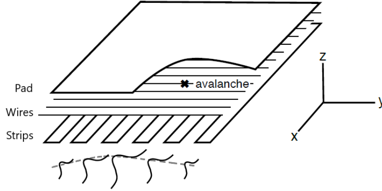
Figure 5.2: Schematic diagram representing the three types of electrodes in a stGC detector. The position of the ionization avalanche is extracted from the wires and strips that picked up the avalanche signal. The signals on individual strips are sketched. Clustering is the process by which a Gaussian function (represented by the grey dashed line) is fitted to the distribution of the signal amplitude on individual contiguous strips; a sample cluster is shown in Figure 5.3. In this work, the x(y) -coordinate will always refer to the coordinate perpendicular to the wires (strips). The z -coordinate is perpendicular to the stGC surface [58, 56].
