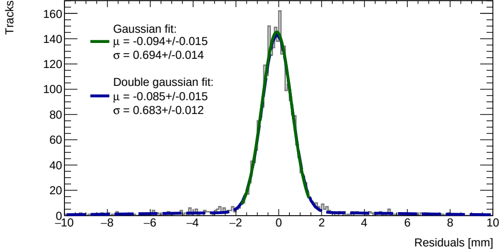
Figure C.1: Residual distribution for track residuals on layer 4 built from clusters on layers 1 and 2 for x \in [-3.00, 97.00] mm, y \in [394.60, 494.60] mm, fit with a double Gaussian and a single Gaussian in a range of \pm 1 RMS from the histogram mean.
