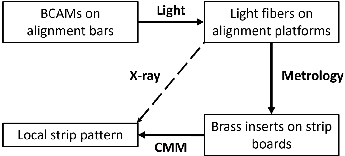
Figure 4.6: Schematic diagram showing how the different elements of the sTGC alignment system relate to one another. The solid arrows denote the planned alignment scheme. The dashed arrow shows the modification being finalized now. This figure was originally designed by Dr. Benoit Lefebvre.
