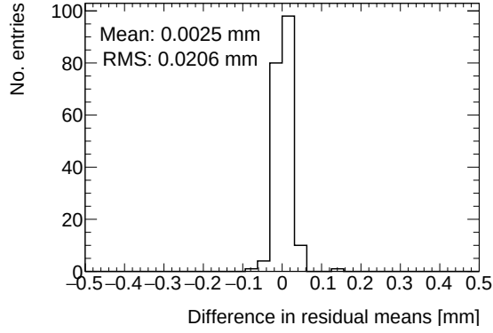
(a) Difference in residual means for residuals on layer 4 built from clusters on layers 1 and 2.
