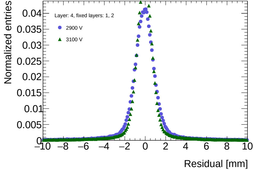
Figure C.3: Residual distribution for tracks on layer 4 built from clusters on layers 1 and 2 for sample quadruplet QL2.P.8 for data collected at 2.9 kV and 3.1 kV.
