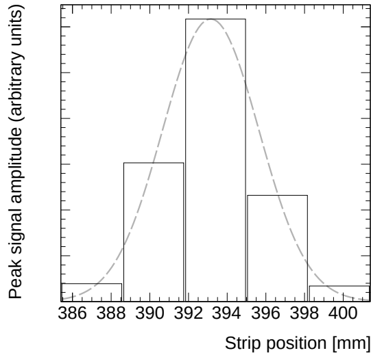
Figure 5.3: A sample cluster resulting from signal recorded on a group of contiguous strips after the passing of a muon. The grey dashed line represents the result of a fit to a Gaussian distribution.
