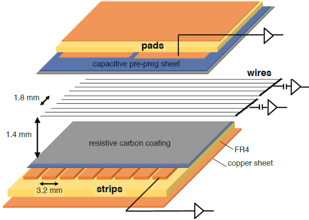
Figure 4.3: Internal structure of an sTGC, zoomed into the area under a pad. High voltage is applied to wires suspended in the gas volume to create an electric field. A passing muon causes an ionization avalanche that is picked up by the wire, strip and pad electrodes [8].
