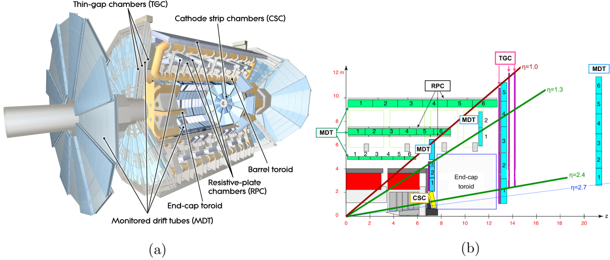
Figure 3.5: Schematic diagram of the ATLAS muon spectrometer. Figure (a) shows a 3D projection of the system with the different types of chambers and different parts of the toroidal magnet system labeled [4]. Figure (b) shows a projection of one quarter of the muon spectrometer, with the interaction point in the bottom left corner. The small wheel is just left of the end cap toroid, the big wheel is to its right, and the outer wheel is the rightmost structure [51].
