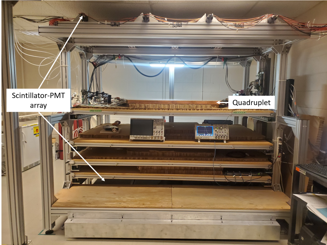
Figure 5.1: Cosmic muon hodoscope at McGill University with a sTGC quadruplet module in the test bench.
