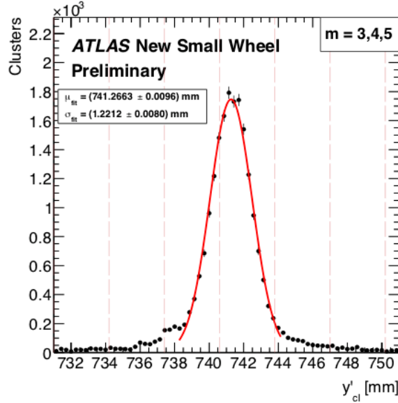
Figure 6.2: An example distribution of x-ray cluster mean positions after the analysis selection cuts and DNL corrections are applied. The strip cluster multiplicity, m , was limited to 3, 4 or 5. The red curve is a Gaussian fit of the distribution and the pink dashed lines denote the edges of the strips [8].
