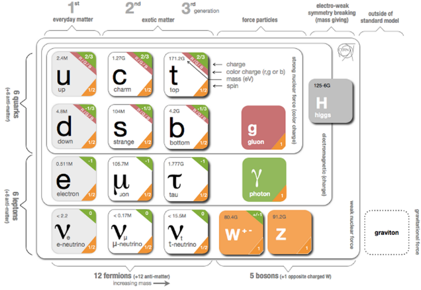
Figure 2.1: Schematic diagram of all elementary particles in the SM. Particles are grouped according to their properties and the forces through which they interact with other particles [16].
