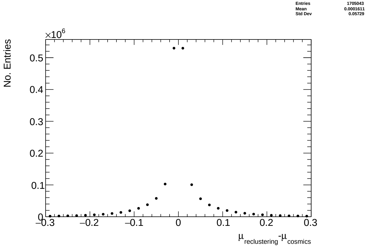
Figure A.1: The difference between cluster means calculated with Guo's method [66] and Minuit2 for ROOT [65] for data collected with QL2.P.8 at 3.1 kV.
