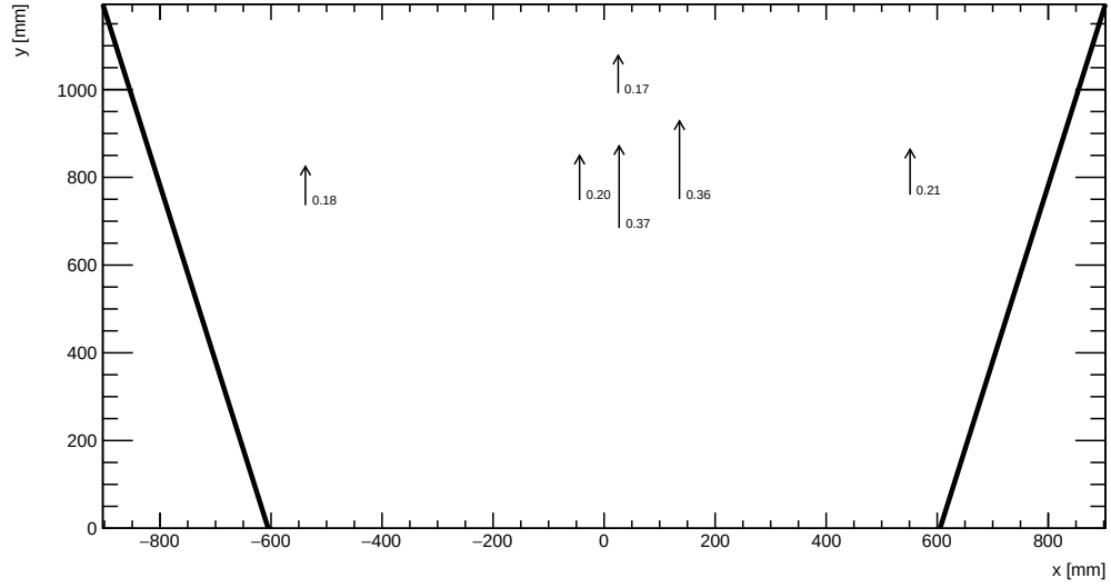
(a) X-ray residuals on quadruplet QL2.P.11 layer 2 obtained using reference layers 1 and 3.
