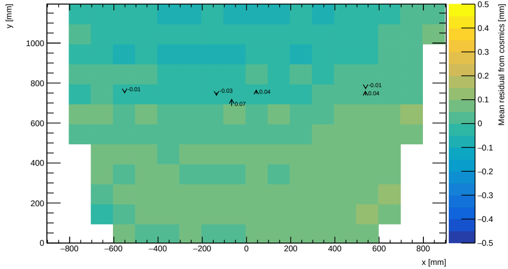
(b) Means cosmics and x-ray residuals on sTGC layer 2 of quadruplet QL2.P.8 obtained using reference layers 1 and 3.
