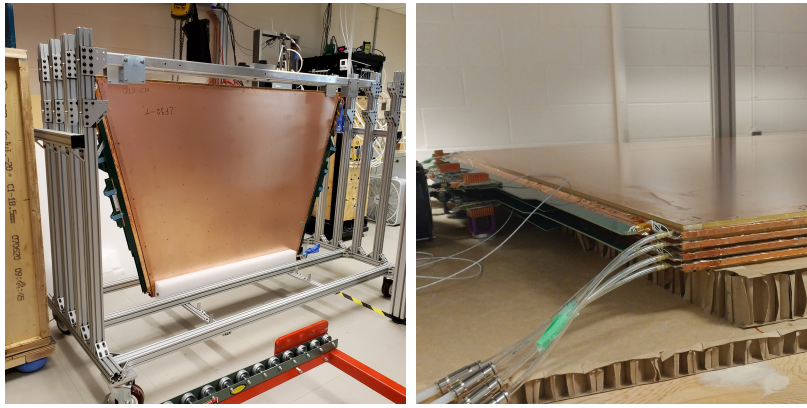
(a) A sTGC quadruplet module. The left image highlights the trapezoidal shape of a quadruplet module. The right image shows the corner at the short edge, where the four sTGC layers and each layer's gas inlet are visible. The gas outlets and high voltage cables are located along the long edge near the corner in the back left of the photo. The green printed circuit boards along the sides are the adaptor boards where the front end electronics are attached.
