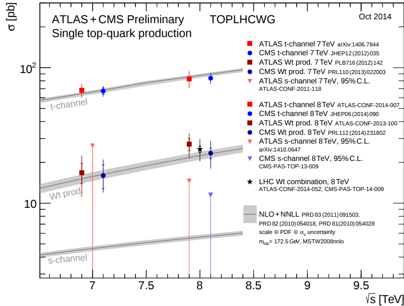
Figure 2.10: Summary of LHC measurements of the single top-quark production cross-sections as a function of \sqrt{s} compared to a theoretical prediction. Only upper limits are given for the s -channel production [67].
