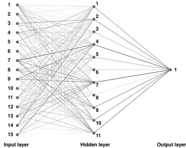
Figure 9.4: Graphical representation of the trained neural network for the training of signal against all backgrounds. The line darkness depends on the weight factors of the connections. The darker a line, the larger is the corresponding weight factor. The meaning of the numbers is discussed in the text.
