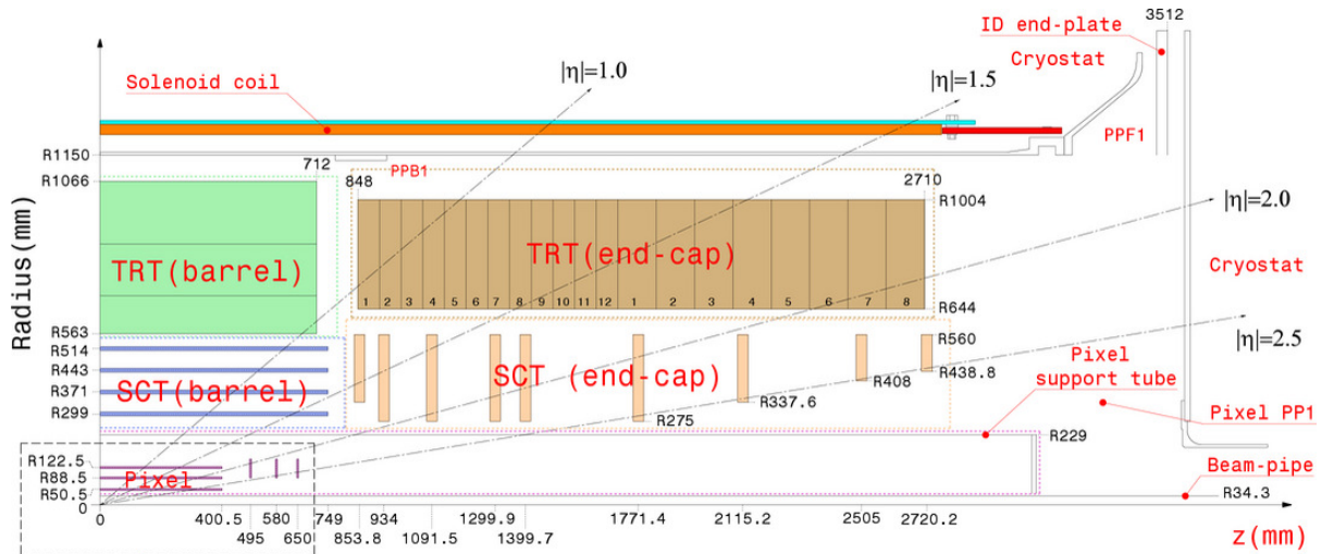
Figure 3.4: Technical drawing of the Inner Detector components' dimensions [83].
