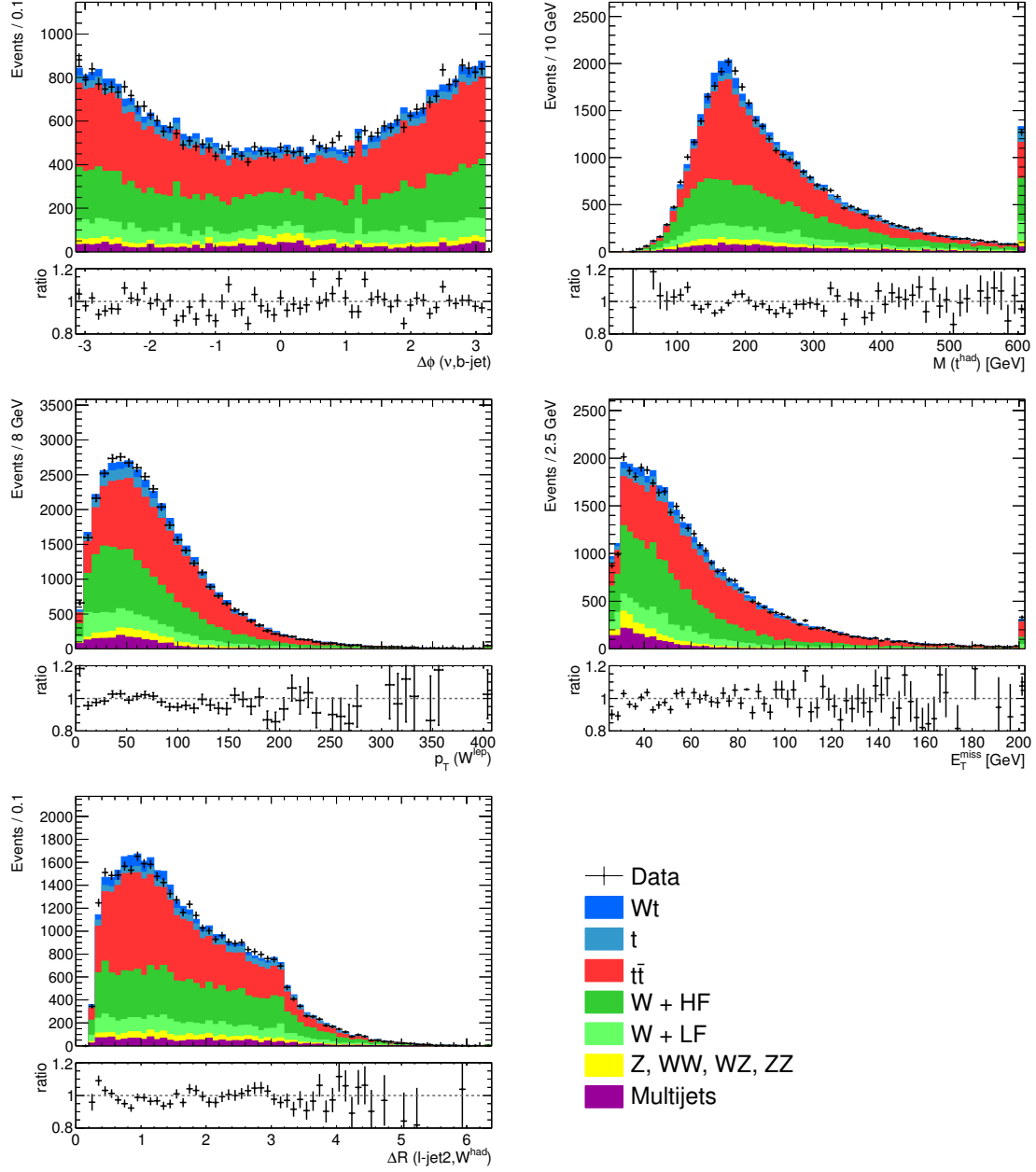
Figure B.5: Distributions of variables used in the network training against t\bar{t} production. Electron and muon channels are merged. The simulation distributions are normalized to the measured luminosity. The ratio of data and simulation is shown in the bottom plot.
