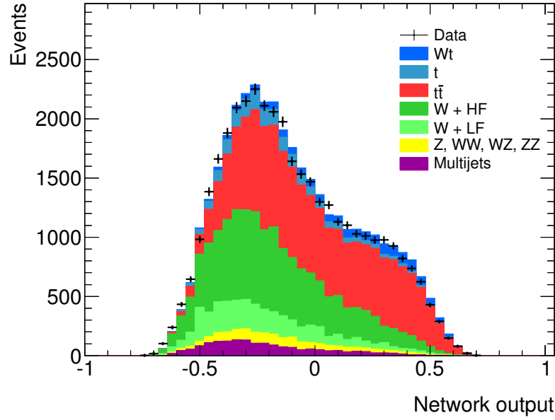
Figure 9.8: Neural network output distribution for the training of the signal against all backgrounds. All simulation contributions are weighted to the data luminosity according to their theoretically predicted cross-sections.
