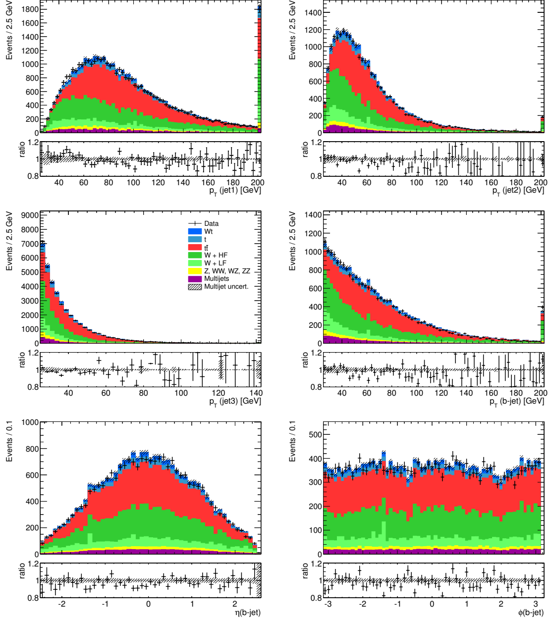
Figure 7.5: Control distributions of selected jet variables. Electron and muon channels are merged. The jet numbering follows the p_T ordering of the jets. Jet1 is the hardest jet in the event. The simulation distributions are normalized to the measured luminosity. The hashed area corresponds to the uncertainty resulting from the multijet estimation. The ratio of data and simulation is shown in the bottom plot.
