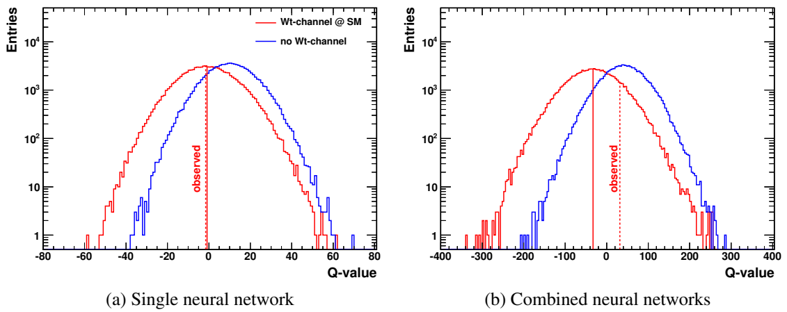
Figure 10.7: Distributions of Q -values determined using 100 000 pseudo-experiments evaluating the non-signal hypothesis in blue and the signal hypothesis in red for the single neural network training (a) and the combination of two neural network trainings (b). The vertical red line indicates the median of the distribution for the signal hypothesis corresponding to the Q -value. The dashed vertical line indicates the position of the observed Q -value.
