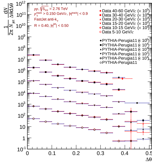
Figure 6.41: \Delta\theta distribution of corrected data compared to MC for R=0.4 .
