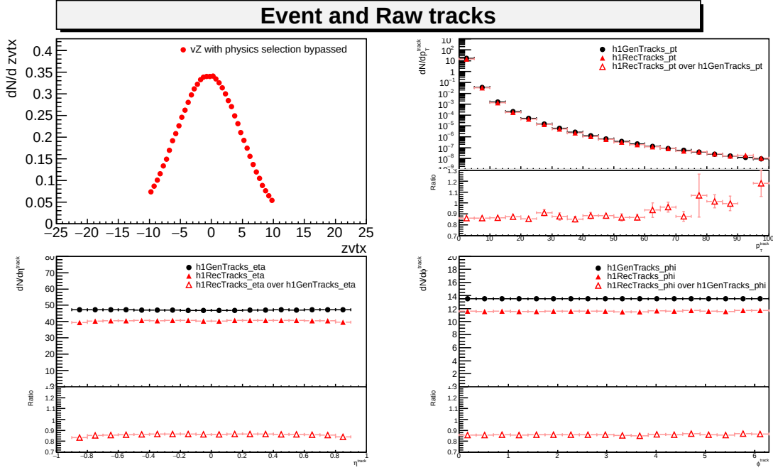
Figure 5.5: MC event and track distributions
