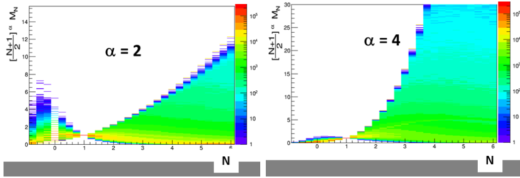
Figure 7.2: Comparison of the impact of the scaling power \alpha on the 2-Dimension FFM ( R=0.4 , Data). Left: \alpha = 2 ; right: \alpha = 4 .
