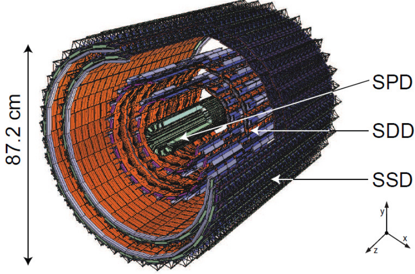
Figure 2.4: ALICE ITS layout
