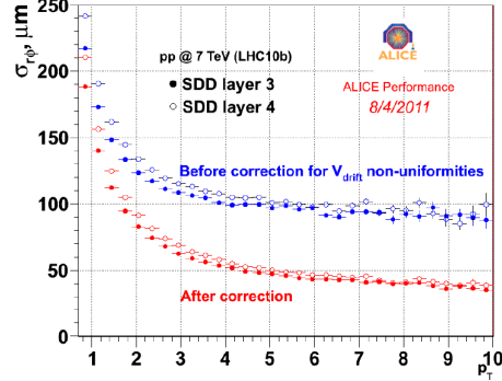
Figure 2.8: SDD resolution in the r\phi plane before (blue) and after (red) correcting for drift speed non-uniformities in the detector on layer 3 (full) and 4 (open)
