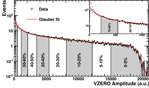
Figure 4.1: Distribution of the VZERO scintillators amplitudes sum for event compared to Glauber fit [82].
