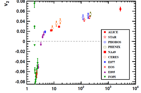
Figure 1.29: v_2 as a function of the energy available in the centre of mass of the collision. ALICE data is from Pb-Pb collisions at \sqrt{s_{NN}} = 2.76 TeV in the centrality class 20-30% and it is compared to results from lower energies experiment at similar centralities.
