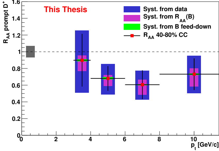
Figure 4.16: D^+ R_{AA} for centrality classes 40-80%. Error bars are statistical uncertainties, blue area is the systematic uncertainties from data (yield extraction, p-p cross-section), the purple band represents the systematic uncertainty due to feed-down R_{AA} and the green band the uncertainty on feed-down subtraction.
