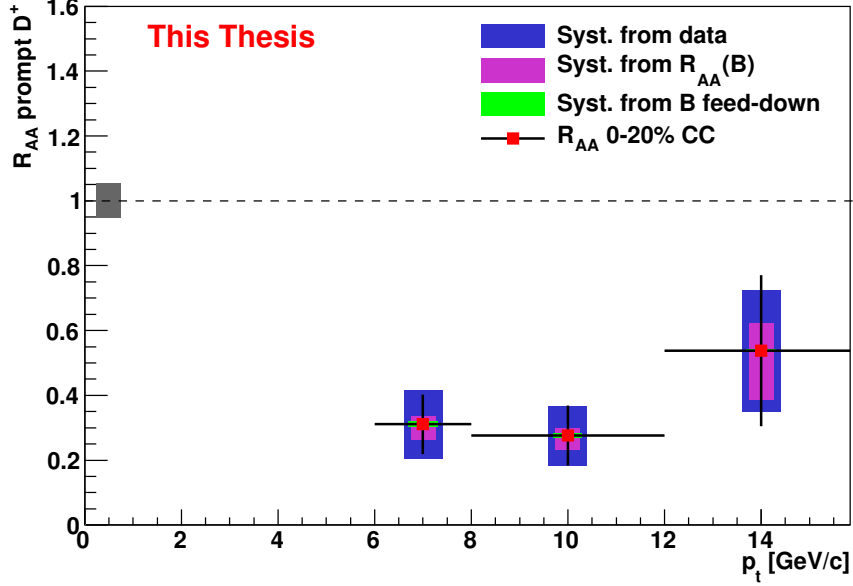
Figure 4.15: D^+ R_{AA} for centrality classes 0-20%. Error bars are statistical uncertainties, blue area is the systematic uncertainties from data (yield extraction, p-p cross-section), the purple band represents the systematic uncertainty due to feed-down R_{AA} and the green band the uncertainty on feed-down subtraction.
