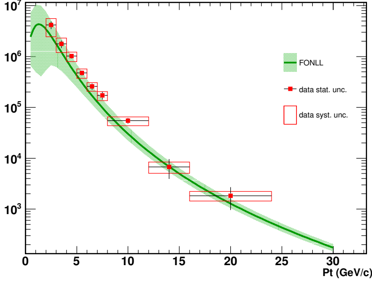
Figure 3.19: Primary D^+ corrected yield as function of p_t compared with FONLL predictions, where the FONLL distribution was rescaled to the integral of the data. The y-axis is the p_t differential corrected yield in arbitrary unit.
