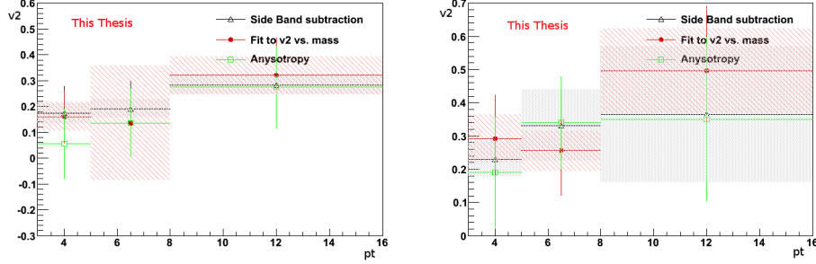
Figure 4.30: D^+ v_2 in 30-50% (left) and 50-80% (right) centrality collisions. Results from three different methods are shown: the in-plane versus out-of-plane anisotropy (green), the fit of v_2 versus invariant mass (red) and side band subtraction (black). The red and grey band are systematic uncertainties on the fit and side band subtraction methods respectively. Error bars are statistical uncertainties.
