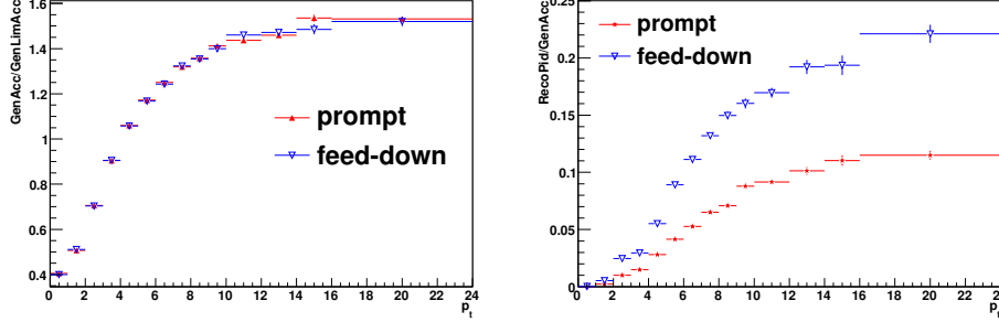
Figure 3.15: Efficiencies from simulated proton-proton collisions at \sqrt{s} = 7 TeV. Left: ratio between the number of D^+ generated in the p_t and \eta fiducial acceptance of the central barrel and those generated in |y| < 0.5 from minimum bias MonteCarlo. Right: ratio between the number of reconstructed and selected D^+ and the number of D^+ generated in |y| < 0.5 from charm enriched Montecarlo. Red are prompt D^+ , blue are feed down.
