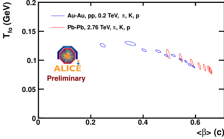
Figure 1.14: 1- \sigma confidence contour plot for the temperature and velocity boost parameters of the blast-wave fit on the identified particle spectra at RHIC (blue) and ALICE (red).
