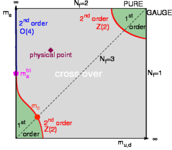
Figure 1.7: Change of the phase transition behaviour and critical temperature depending of the quark masses value. Calculation made on a 3 flavours lQCD[9]
