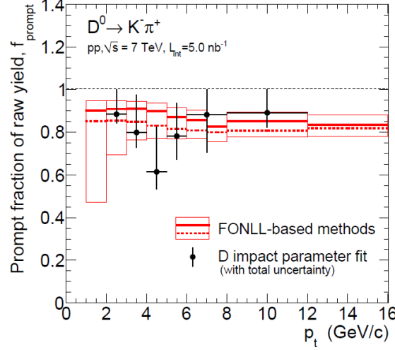
Figure 3.28: prompt fraction of the D^0 raw yield as a function of p_t for the two FONLL-based methods (solid: central value, from Eq. 3.2; dashed: alternative method, 3.7) and for the impact parameter fit method (circles); the boxes show the envelope of the uncertainty bands of the two FONLL-based methods; the error bars show the total uncertainty from the impact parameter fit, including the statistical and systematic contributions.
