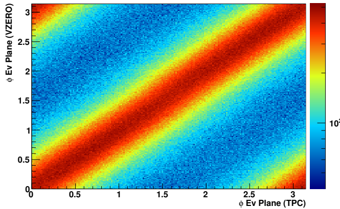
Figure 4.24: Event plane angle measured with the VZERO detector versus the one determined from the distribution of charged tracks in the TPC.
