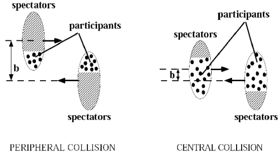
Figure 1.10: Geometry of a collision between two nuclei. Left: in a peripheral collision, with large impact parameter b the number of colliding nucleons (participants) is small, and most of the energy is carried away by the spectator nucleons that do not interact. Right: in a central collision with small impact parameter many nucleons are involved in the collision.
