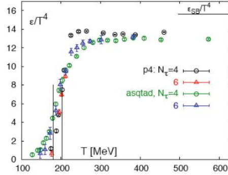
Figure 1.6: Evolution of the energy density as function of the temperature. Calculation made with 2 light ( u, d ) and one heavier flavour ( s ) at 0 barionic density. Phase transition occur at 192 \pm 11 MeV (F. Karsch, [7]). open circles (triangles) are calculated using a lattice with 4 (6) steps in the time dimension. Black and red points are based on a 1-link plus 3 bended links terms fermion action. Blue and green points are calculated using a static quark potential [8]
