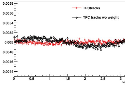
Figure 4.21: Distribution of the event plane measured from charged tracks in the TPC with (red) and without (black) \phi weights corrections
