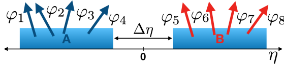
Figure 2.7: Sketch of the side view of a detector, showing example of eight-particle correlation with 2-subevent method with an additional |\Delta\eta| gap between the subevents.
