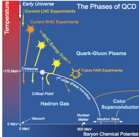
Figure 1.3: Phase diagram of nuclear matter. Figure adapted from [5].
