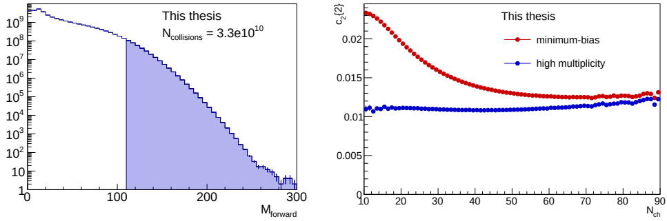
Figure F.1: Left: Distribution of multiplicity in the forward region of the V0 detector acceptance. The blue area represents the region of high multiplicity events used for the comparison with data. Right: Measurement of c_2\{2\} as a function of multiplicity at mid-rapidity for all PYTHIA 8 generated collisions (representing the minimum-bias events in real data) and high multiplicity events obtained based on the forward multiplicity selection. Similar effect of the trigger selection as in real data is observed.
