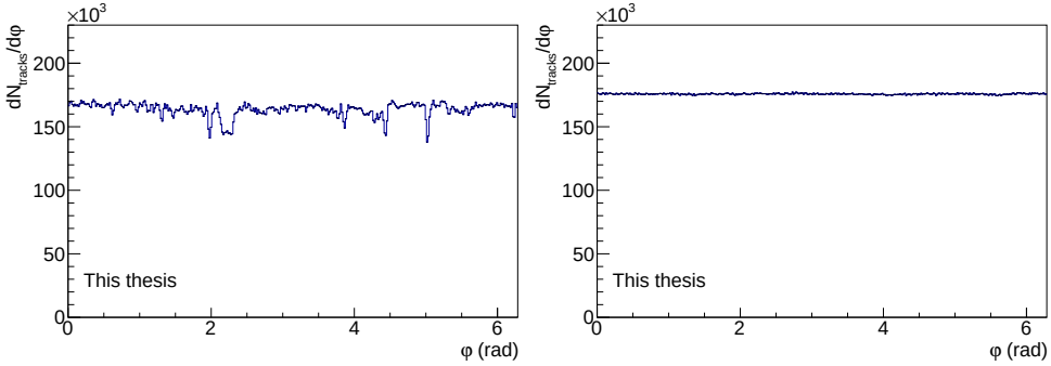
Figure 5.1: Left: Event-averaged \phi distribution of the LHC16k period of pp collisions. The regions with non-uniform acceptance can be clearly seen. Right: The same \phi distribution after the weight application to account for non-uniform acceptance. The distribution is uniform, as was intended.
