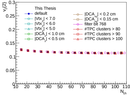
Figure 5.10: Comparison of v_2\{2\} results from pp collisions as a function of N_{\text{ch}} (corrected for inefficiencies) for default cuts, and different variations of these cuts.
