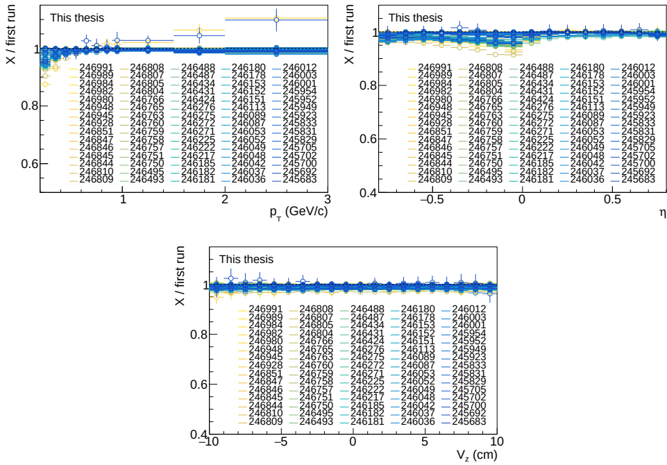
Figure B.5: Ratio of detector efficiency as a function of p_T (left), \eta (right) and V_z (bottom) from different runs in the LHC150 period in Pb–Pb collisions to the first run of that period.
