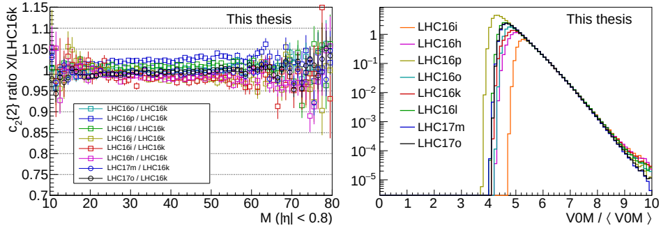
Figure 4.6: Left: Ratio of c_2\{2\} from different periods to the LHC16k period. The effect of the rising trigger threshold due to V0 ageing is visible based on the deviations of the measurements from different periods with respect to the chosen default LHC16k period. Right: Comparison of VOM/\langle VOM \rangle distributions for different periods. Periods which were chosen to be combined for final data analysis show similar thresholds of the high multiplicity trigger.
