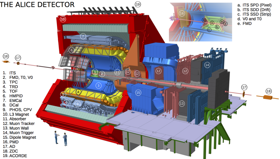
Figure 3.2: Schematic view of the ALICE detector during the Run2 data taking [64]. It consists of a central barrel and a forward muon arm. The central part of the detector is contained within a large magnet. The main detectors that will be used for the analysis described in this thesis are the ITS, TPC and V0.
