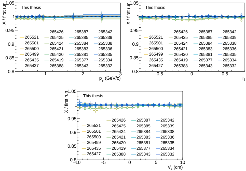
Figure B.2: Ratio of detector efficiency as a function of p_T (left), \eta (right) and V_z (bottom) from different runs of the LHC16q period in p–Pb collisions to the first run of that period.
