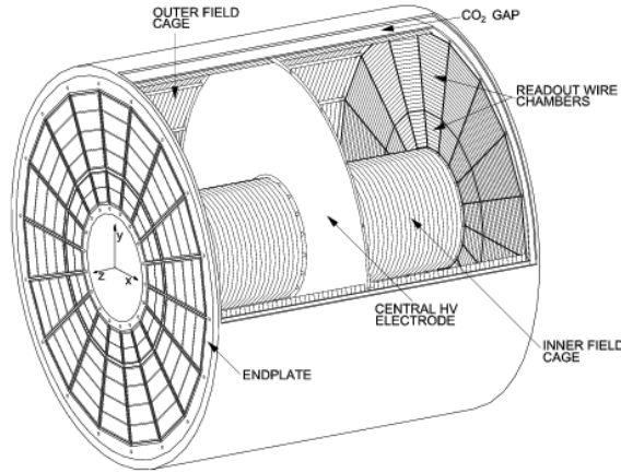
Figure 3.4: Schematic view of the TPC [68]. It has a cylindrical shape with inner radius of 85 cm, outer radius 250 cm, and a length of 500 cm. A high voltage cathode is placed in the center, and readout chambers are located at both sides of the TPC. A resistive coating of CO_2 surrounds the TPC in order to isolate the rest of the ALICE detectors from the large electric field inside of the TPC.
