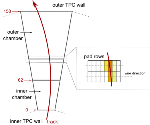
Figure 3.5: Illustration of the signal readout in the TPC (side view on the transverse r - \phi plane) [69]. The incident particle (track) traverses the TPC and ionises the gas molecules. The created electrons drift towards the endcap readout chambers, where the position of the signal is determined from the position of the anode wire and the readout pad.
