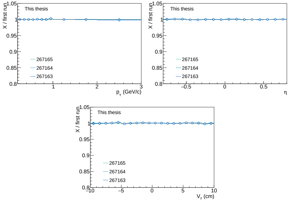
Figure B.3: Ratio of detector efficiency as a function of p_T (left), \eta (right) and V_z (bottom) from different runs of the LHC16t period in p-Pb collisions to the first run of that period.
