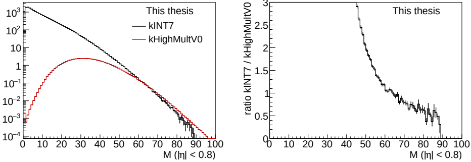
Figure 4.2: Left: Distribution of number of particles (tracks in ITS+TPC) from the kINT7 trigger (black color) and the kHighMultV0 trigger (red color). The distributions are scaled by the integral between M = (60, 80) . Right: Ratio of the number of particles from the kINT7 trigger to the kHighMultV0 trigger. The ratio is not constant, showing that there is no region of multiplicity where the two triggers would give similar results.
