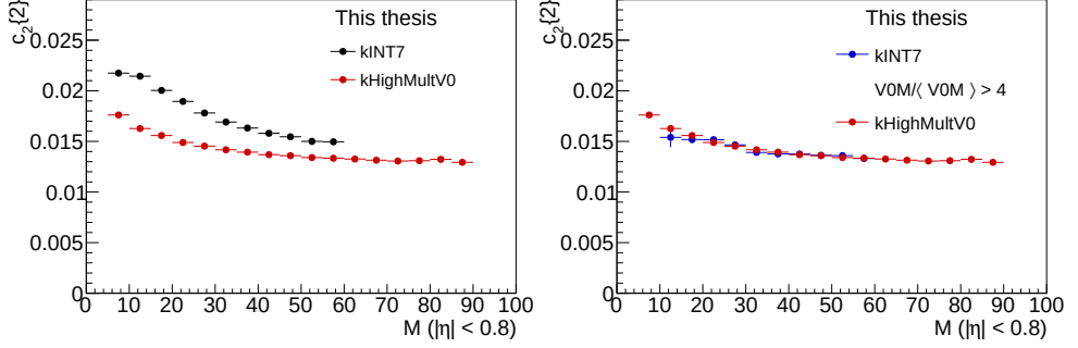
Figure 4.3: Left: c_2\{2\} as a function of multiplicity at mid-rapidity for the kINT7 and the kHighMultV0 trigger. The results of kINT7 trigger are systematically higher than from the kHighMultV0 trigger. Right: c_2\{2\} for the kHighMultV0 trigger and the kINT7 trigger after the cut V0M/\langle V0M \rangle > 4 .
