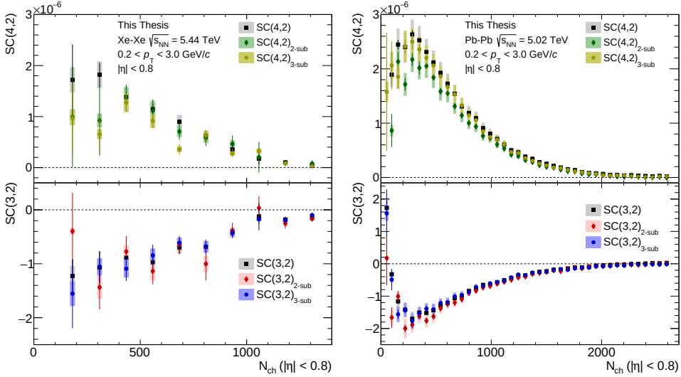
Figure 6.6: Multiplicity dependence of SC(4,2) (upper panels) and SC(3,2) (bottom panels) using the standard, 2- and 3-subevent method in 5.44 TeV Xe–Xe collisions (left) and in 5.02 TeV Pb–Pb collisions (right). The measurements using the different methods are compatible.
