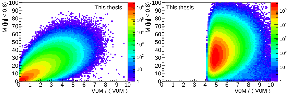
Figure 4.1: Distribution of the number of tracks at mid-rapidity, M(|\eta| < 0.8) , vs. V0M/\langle V0M \rangle for the kINT7 trigger (left) and for the kHighMultV0 trigger (right). The cut on V0M/\langle V0M \rangle > 4 in kHighMultV0 is apparent.
