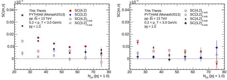
Figure 2.9: Left: Multiplicity dependence of SC(m,n) and SC(m,n)_{2-sub} in PYTHIA 8 simulations of \sqrt{s} = 13 TeV pp collisions. A clear decrease of the signal is observed. Right: Multiplicity dependence of SC(m,n)_{2-sub} and SC(m,n)_{3-sub} in PYTHIA 8 simulations of \sqrt{s} = 13 TeV pp collisions. The two methods produce compatible results within the statistical uncertainties.
