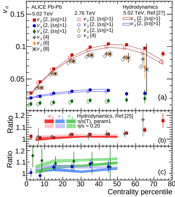
Figure 1.8: Flow coefficients as a function of collision centrality in \sqrt{s_{NN}} = 5.02 TeV Pb-Pb collisions. Measurements are compared to hydrodynamic calculations. Figure taken from [32].
