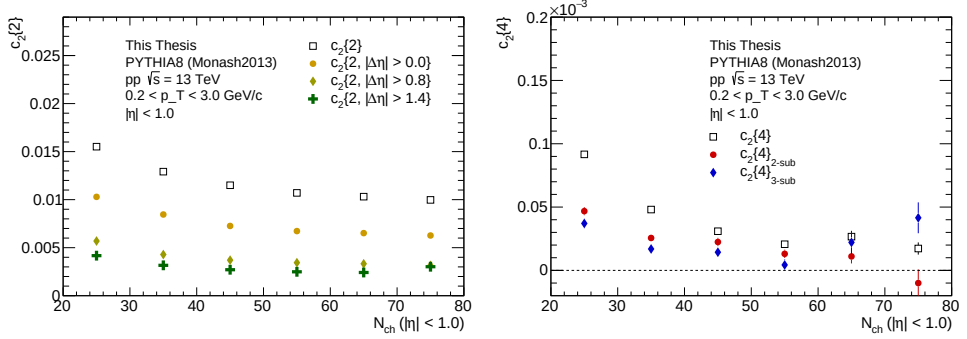
Figure 2.8: Left: Multiplicity dependence of c_2\{2\} (open marker) and c_2\{2, |\Delta\eta|\} (filled markers) in PYTHIA 8 simulations of \sqrt{s} = 13 TeV pp collisions. A decrease of the signal with increasing |\Delta\eta| gap is observed. Right: Multiplicity dependence of c_2\{4\} (open markers), c_2\{4\}_{2\text{-sub}} (filled red markers) and c_2\{4\}_{3\text{-sub}} (filled blue markers) in PYTHIA 8 simulations of \sqrt{s} = 13 TeV pp collisions. A decrease of the c_2\{4\} with the subevent method can be seen.
