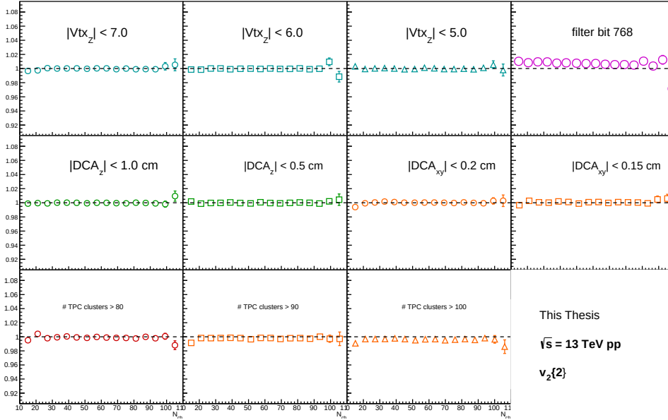
Figure 5.11: Ratio of v_2\{2\} results from pp collisions with variation of cuts to the results with default cuts, intended for systematic studies.
