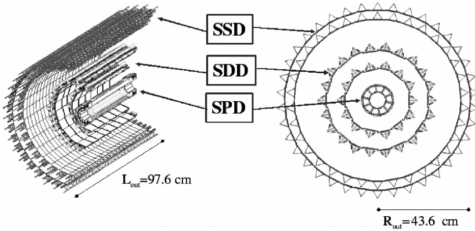
Figure 3.3: Schematic view of the ALICE Inner Tracking System (ITS) detector [66]. It is composed of three detectors: the Silicon Pixel Detector (SPD) closely surrounding the beam pipe, then the Silicon Drift Detector (SDD) and finally the Silicon Strip Detector (SSD), furthest from the beam pipe. Each detector consists of 2 layers.
