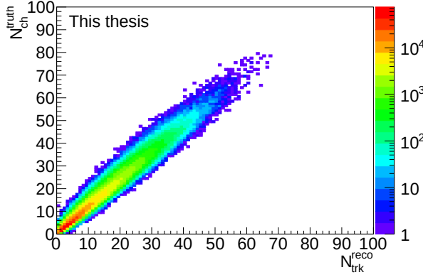
Figure 5.5: Response matrix: correlation between the number of generated particles N_{\text{ch}}^{\text{truth}} and the number of reconstructed tracks N_{\text{trk}}^{\text{reco}} . The matrix is taken from the PYTHIA 8 Monte Carlo simulation of pp collisions.
