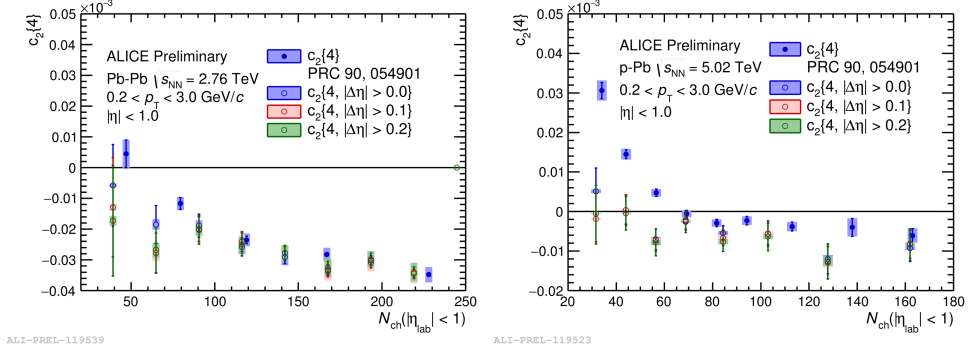
Figure E.9: Left: Multiplicity dependence of c_2\{4\} and c_2\{4, |\Delta\eta|\} in Pb-Pb collisions. No significant differences between the measurements are observed, apart from the lowest multiplicity region. Right: Multiplicity dependence of c_2\{4\} and c_2\{4, |\Delta\eta|\} in p-Pb collisions. A significant decrease of c_2\{4\} can be observed in p-Pb collisions, which is more pronounced at low multiplicities.
