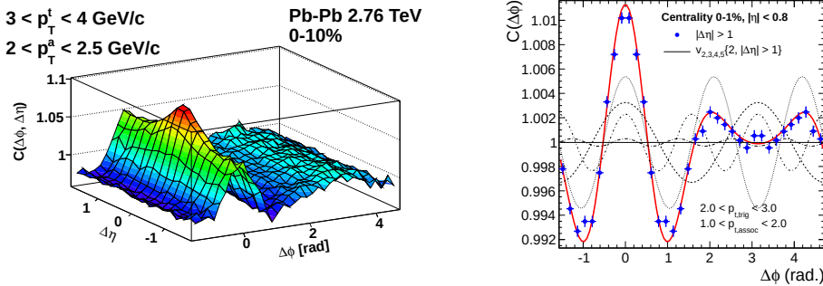
Figure 1.7: Left: Di-hadron correlation in 2.76 TeV Pb–Pb collisions, measured as a function of relative difference in azimuthal angle \phi and pseudorapidity \eta . Figure taken from [30]. Right: Projection of the di-hadron correlation in 2.76 TeV Pb–Pb collisions onto the \Delta\phi plane. The near-side jet peak was removed with a|\Delta\eta| > 1.0 . Figure taken from [31].
