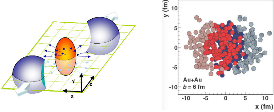
Figure 1.6: Left: Illustration of a peripheral collision with almond shaped overlap region. Figure taken from [28]. Right: Glauber simulation of a heavy-ion collision with constituent nucleons, showing that the overlap geometry does not have a perfect elliptic-like shape, but it contains several geometries combined together which can be studied with Fourier decomposition. Figure taken from [12].
