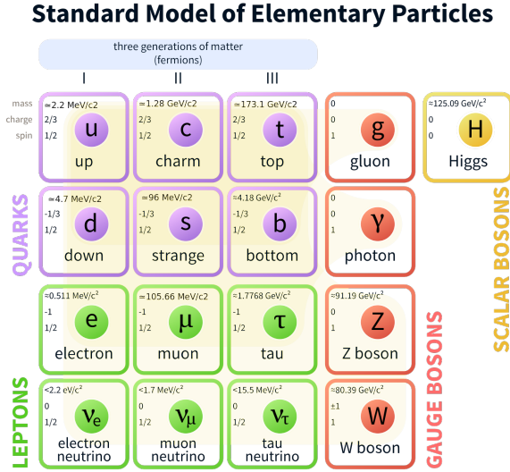
Figure 1.1: Standard model of elementary particles. Figure taken from [1].
