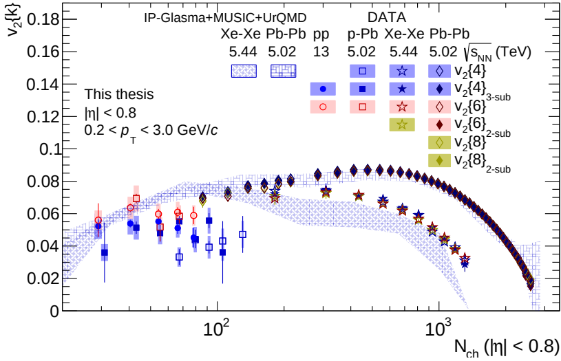
Figure 6.14: Multiplicity dependence of v_2\{m\} for m > 2 with the standard and the subevent method for small (pp and p–Pb) and large (Xe–Xe and Pb–Pb) collision systems. The Xe–Xe and Pb–Pb results are compared to the IP-Glasma+MUSIC+UrQMD calculations [85, 86].
