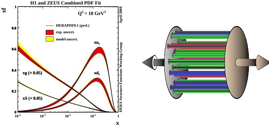
Figure 1.4: Left: Parton distribution functions PDFs of the valence u and d quarks, the sea quarks S and gluons g . Figure taken from [11]. Right: Illustration of the Glasma phase of a heavy-ion collision, with the colour electric and magnetic fields spanning across long range in rapidity. Figure taken from [8].
