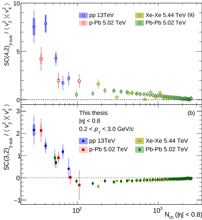
Figure 6.17: Multiplicity dependence of normalised SC(4,2)_{3\text{-sub}} (top) and SC(3,2)_{3\text{-sub}} (bottom) for small (pp and p-Pb) and large (Xe-Xe and Pb-Pb) collision systems. The v_n in the denominator are taken from the two-particle cumulant measurements with the largest available |\Delta\eta| gap.
