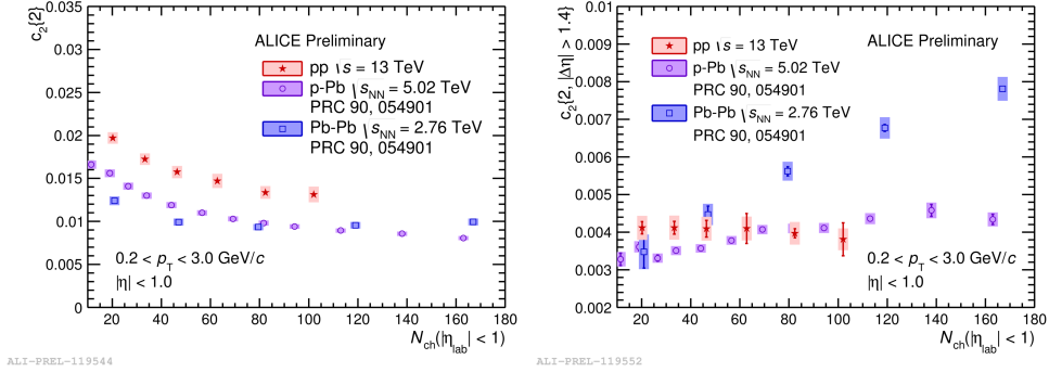
Figure E.3: Left: Multiplicity dependence of c_2\{2\} in pp, p-Pb and Pb-Pb collisions. A decreasing trend with multiplicity can be seen. Right: Multiplicity dependence of c_2\{2, |\Delta\eta| > 1.4\} from pp, p-Pb and Pb-Pb collisions. The |\Delta\eta| gap induces a decrease of the measurements. The measurements from p-Pb and Pb-Pb collisions are taken from [47].
