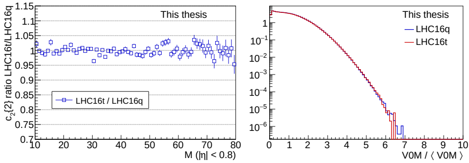
Figure 4.7: Left: Ratio of c_2\{2\} from LHC16t to LHC16q period. The results are compatible with each other, thus the periods can be combined for the final data analysis. Right: Comparison of V0M/\langle V0M \rangle distributions for LHC16q and LHC16t periods. The distributions are consistent.
