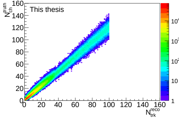
Figure 5.7: Extended response matrix: correlation between the number of generated particles ( N_{\text{ch}}^{\text{truth}} ) and the number of reconstructed tracks ( N_{\text{trk}}^{\text{reco}} ). This matrix will be used for the correction of x-axis of the measurements from the high multiplicity trigger in pp collisions.
