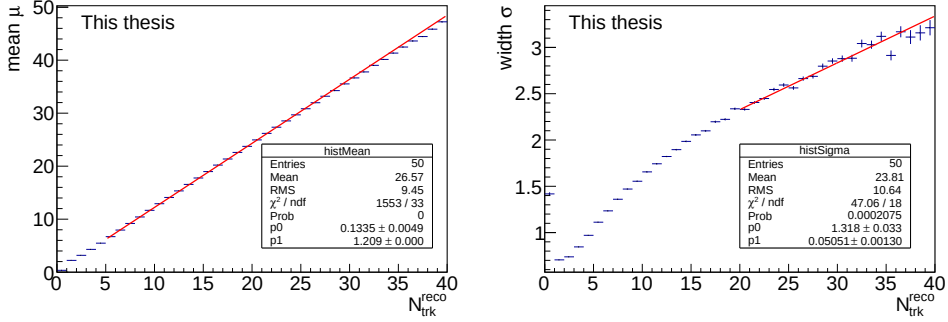
Figure 5.6: The mean \mu (left panel) and width \sigma (right panel) of a Gaussian fit to the y-axis projection of the response matrix in each bin of N_{\text{trk}}^{\text{reco}} . Both distributions are fitted with a linear function to estimate the dependence at high multiplicities.
