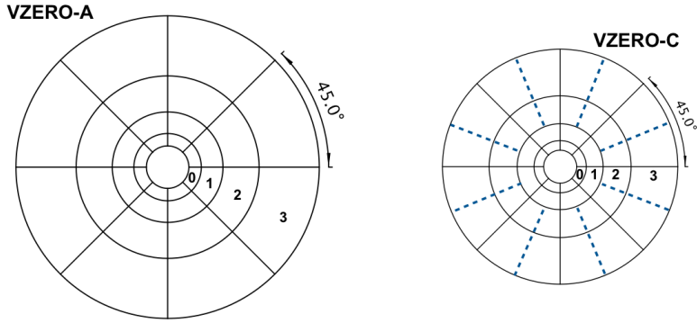
Figure 3.6: Illustration of the layout of the V0 detector rings [70]. Both V0A and V0C rings are scintillator counters divided into 4 rings, where each is further divided into 8 segments. The V0C is located closer to the interaction point and has smaller diameter due to spatial constraints from the hadron absorber of the muon arm. The scintillator segments split by the dashed lines are connected to the same photomultiplier.
