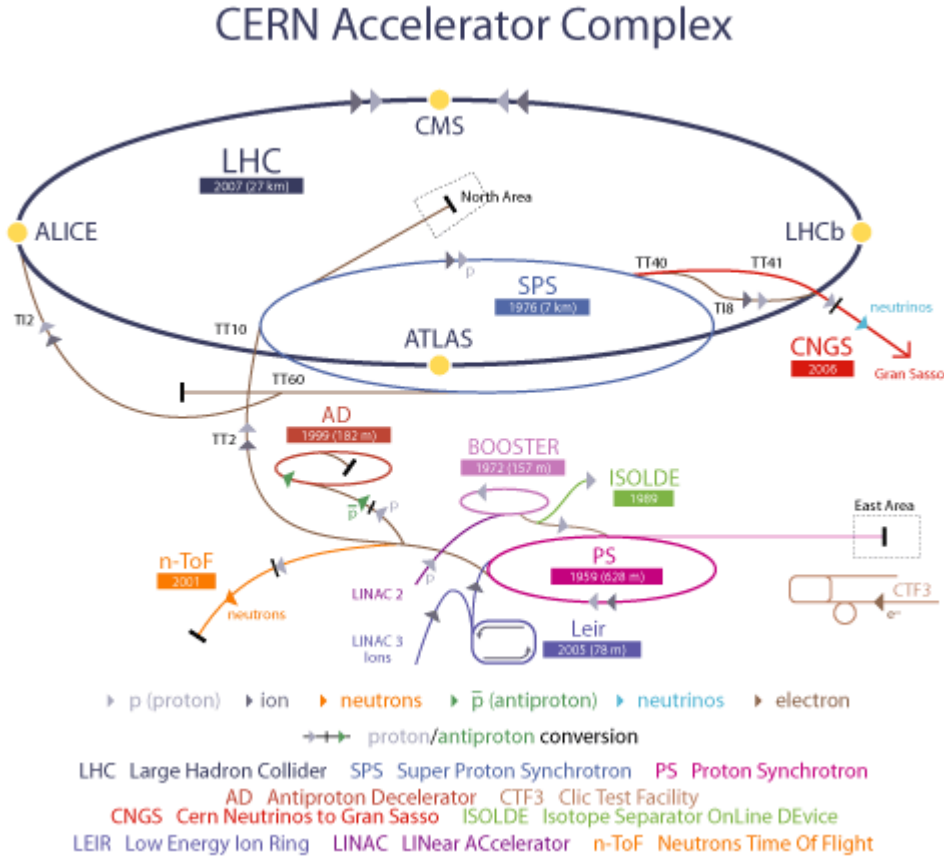
Figure 2.1: Schematic layout of the CERN accelerator's complex
