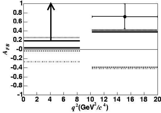
Figure 1.13: BaBar : A_{FB}(q^2) in B \rightarrow K^* l^+ l^- . The points with error bars are data, with the arrow at low q^2 in A_{FB} indicating the 95% CL allowed region. The lines represent the predictions of the SM (solid lines), C_7^{\text{eff}} = -C_7(\text{SM}) (dotted lines), C_9^{\text{eff}} C_{10}^{\text{eff}} = -C_9 C_{10}(\text{SM}) (dashed lines), and C_7^{\text{eff}}, C_9^{\text{eff}} C_{10}^{\text{eff}} = -C_7(\text{SM}), -C_9 C_{10}(\text{SM}) (dot-dashed lines) with the form factor model in LCSR approach.
