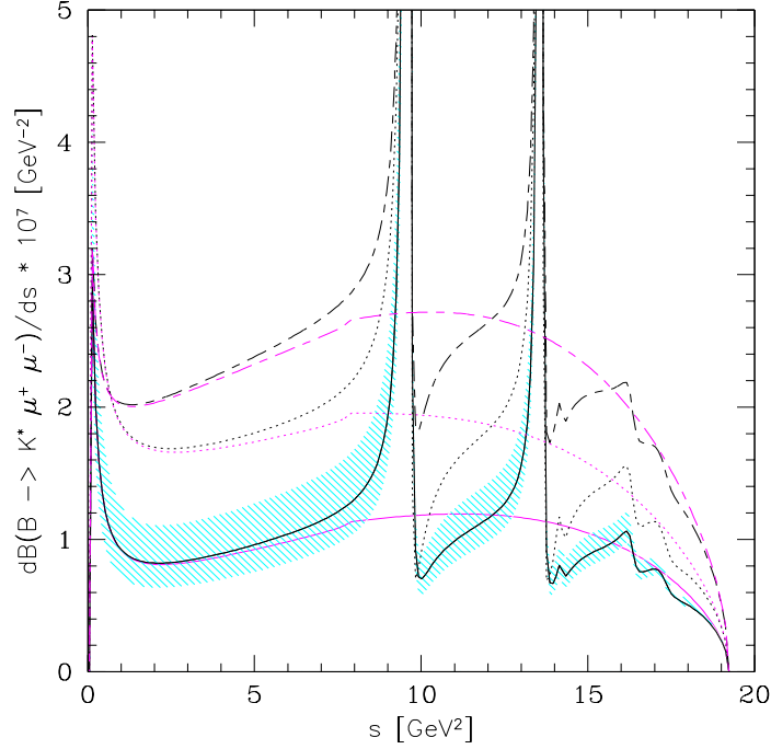
Figure 1.9: The dilepton invariant mass distribution in B \rightarrow K^* \mu^+ \mu^- decays, using the form factors from LCSR as a function of s . The legends are the same as in Figure 1.8.
