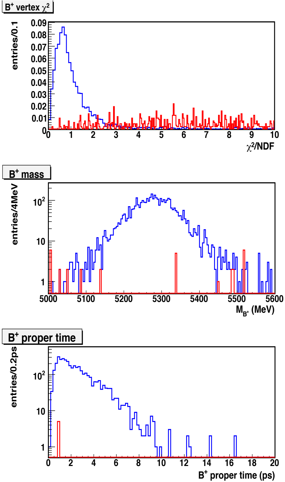
Figure 4.11: B^+ reconstruction \chi^2/\text{NDF} (normalized), mass and proper time distributions for signal (blue) and background (red).
