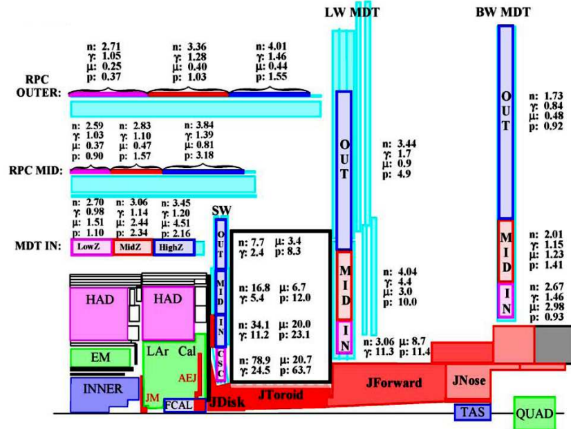
Figure 6.2: Fluences in the muon chambers locations at high luminosity L = 10^{34} \text{ cm}^{-2} \text{ s}^{-1} as predicted by GECALOR. The neutron and \gamma fluence is in units of \text{kHz/cm}^2 and the \mu and proton fluence in \text{Hz/cm}^2 .
