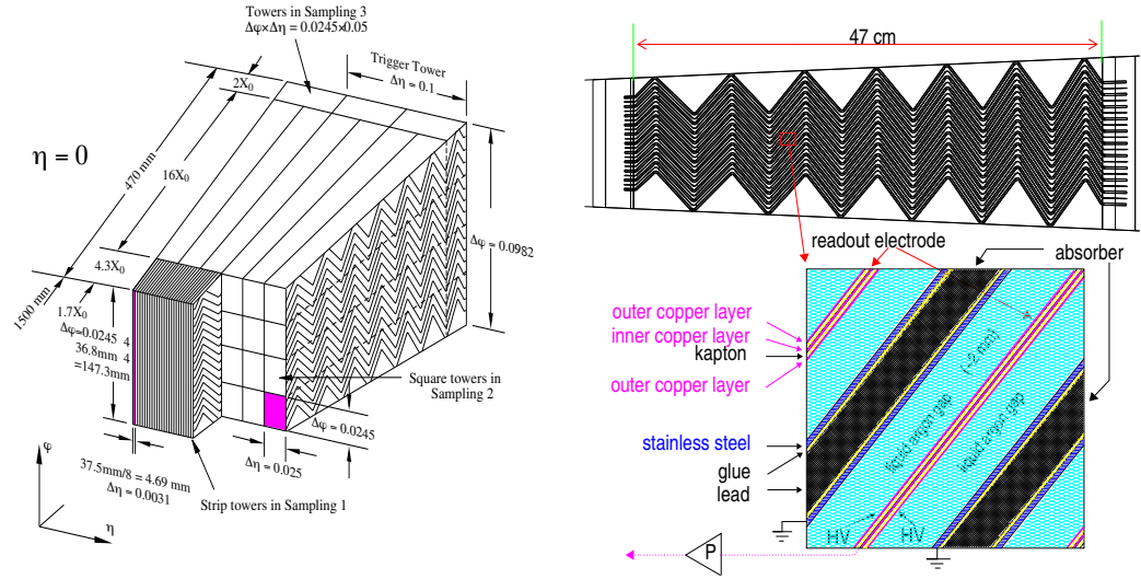
Figure 2.11: Readout scheme of the EM Calorimeter, in evidence the accordion structure.
