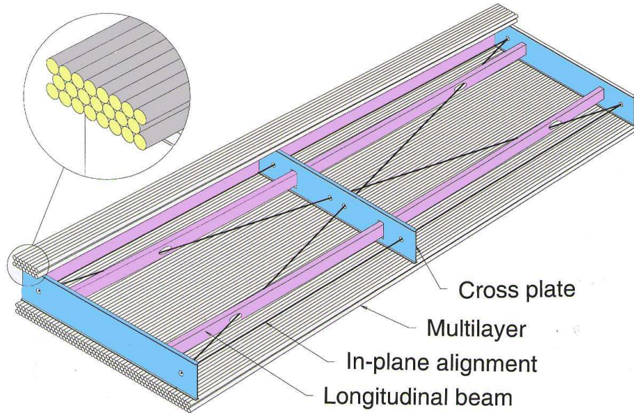
Figure 2.15: Schematic drawing of an MDT chamber. All the structural elements are shown (2x3 layers of tubes).
