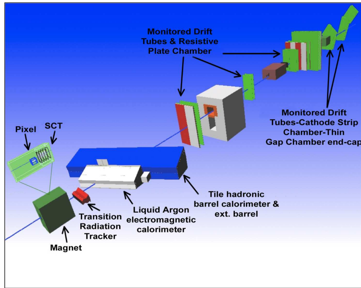
Figure 5.12: Combined Test Beam simulated layout.
