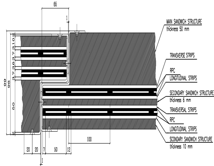
Figure 2.18: Structure of an RPC chamber.
