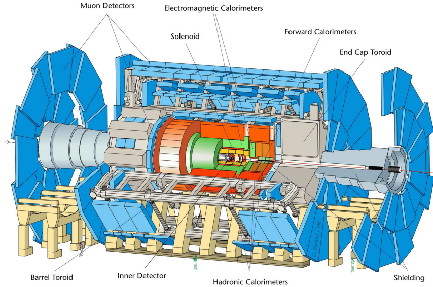
Figure 2.2: Three dimensional view of the ATLAS detector.
