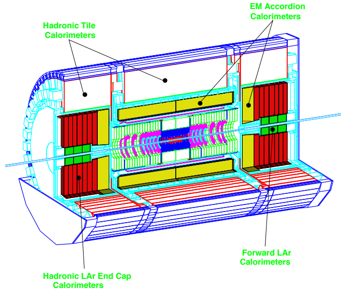
Figure 2.9: Layout of the Calorimeter system.
