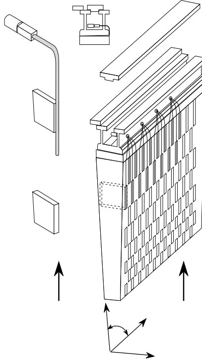
Figure 2.13: View of a Tile module.
