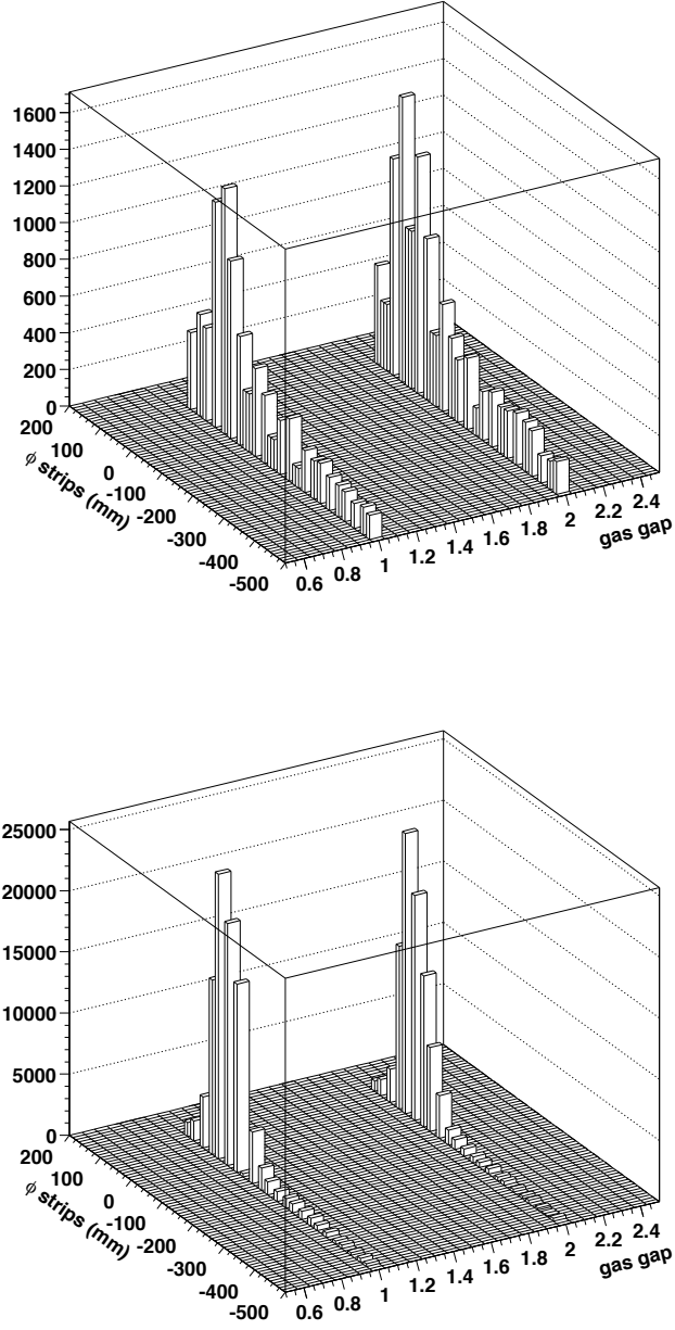
Figure 5.8: Beam profile on the RPC \phi -strips of the middle barrel station: on the top the two layers of the first chamber are shown and on the bottom the two layers of the second chamber.
