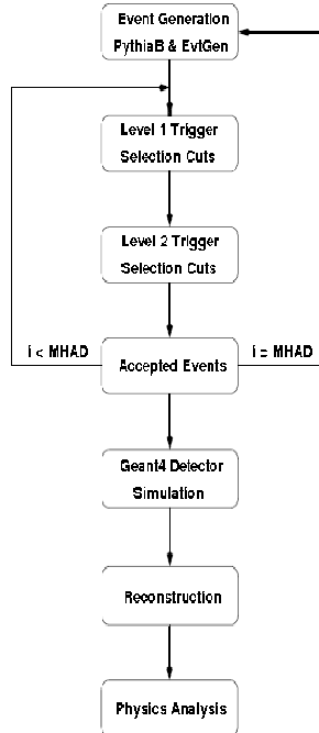
Figure 3.6: Flow diagram of the production procedure for b -events in ATLAS.
