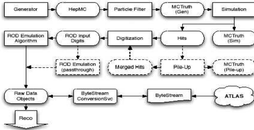
Figure 3.7: Processing stages in the simulation data flow.
