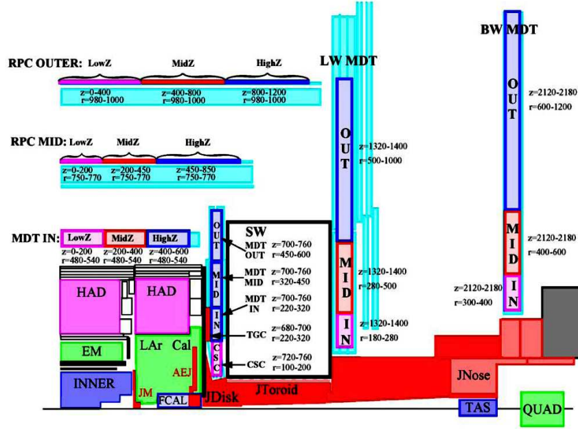
Figure 6.1: Scoring regions used by GECALOR to quote fluences in the Muon System.
