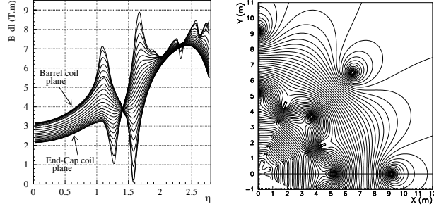
Figure 2.5: Right picture: magnetic toroid field map in the transition region; lines are drawn in a plane perpendicular to the beam axis in the middle of an end-cap toroid. Left picture: toroid bending power \int B dl of the azimuthal field component, integrated between the first and the last muon chamber, as a function of the pseudorapidity.
