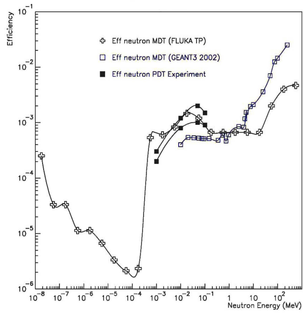
Figure 6.4: MDT efficiency for neutrons.
