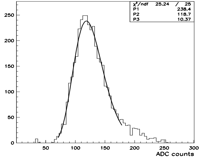
Figure 6.10: Typical ADC spectrum and fit parameters.
