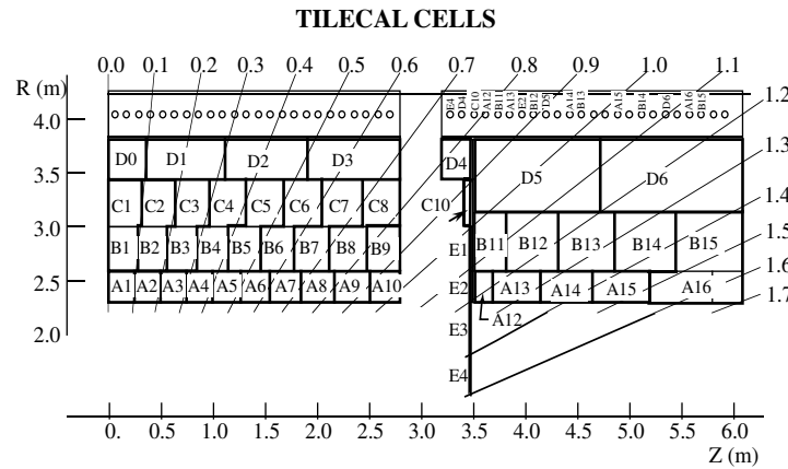
Figure 2.12: Trigger tower scheme of the Tile Calorimeter.
