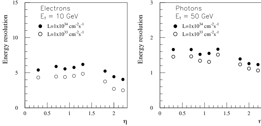
Figure 2.10: Different energy resolutions for electrons (left plot) and photons (right plot) at high (black points) and low luminosity (empty circles). The comparison is for electrons with E_T = 10 GeV and photons with E_T = 50 GeV.
