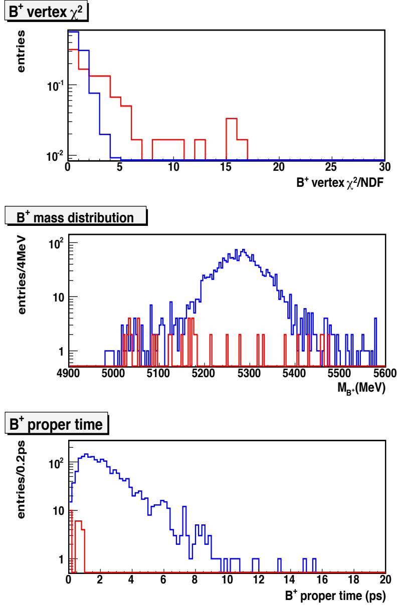
Figure 4.14: B^+ \chi^2/NDF (normalized), mass and proper time distributions for signal (blue) and background (red).
