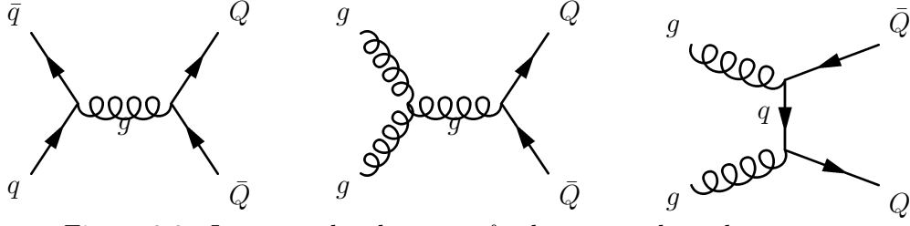
Figure 3.3: Lowest order diagrams for heavy quark production.
