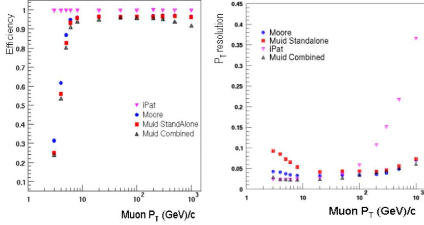
Figure 3.11: Efficiency (left) and p_T resolution (right) as a function of p_T for MOORE, MUID standalone, iPatRec, MUID combined.
