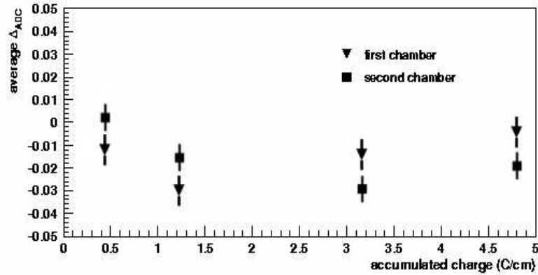
Figure 6.11: ADC peak mean relative variation with respect to the accumulated charge for the two test chambers.
