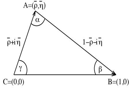
Figure 1.1: Unitarity triangle.
