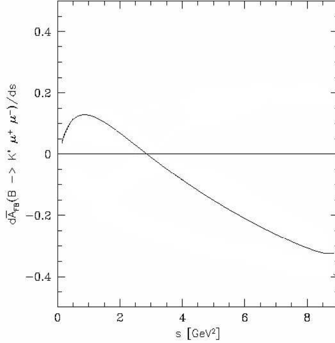
Figure 1.7: The forward-backward asymmetry in B \rightarrow K^*\mu^+\mu^- decay ([21]).
