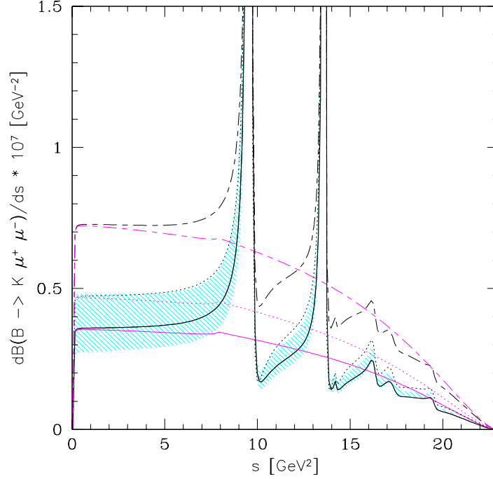
Figure 1.8: The dilepton invariant mass distribution in B \rightarrow K\mu^+\mu^- decays, using the form factors from LCSR as a function of dimuon invariant mass s . The solid line represents the SM and the shaded area depicts the form factor-related uncertainties. The dotted line corresponds to the SUGRA model with R_7 = -1.2 , R_9 = 1.03 and R_{10} = 1 . The long-short dashed lines correspond to an allowed point in the parameter space of the MIA-SUSY model, given by R_7 = -0.83 , R_9 = 0.92 and R_{10} = 1.61 . The corresponding pure SD spectra are shown in the lower part of the plot.
