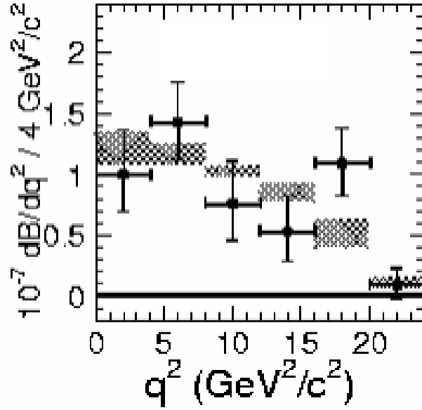
Figure 1.15: Belle : the q^2 distribution of B \rightarrow Kl^+l^- . Points with error bars show the data, while the hatched bands show the range of the SM predictions.
