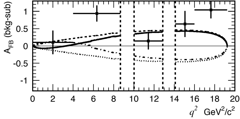
Figure 1.14: Belle : fit result for the negative C_7 solution (solid) projected onto the background subtracted forward-backward asymmetry, and forward-backward asymmetry curves for several input parameters, including the effects of efficiency; C_7 positive case (dashed), C_{10} positive case (dot-dashed) and both C_7 and C_{10} positive case (dotted). The pairs of dashed lines are the boundaries of the J/\psi and \psi' veto regions.
