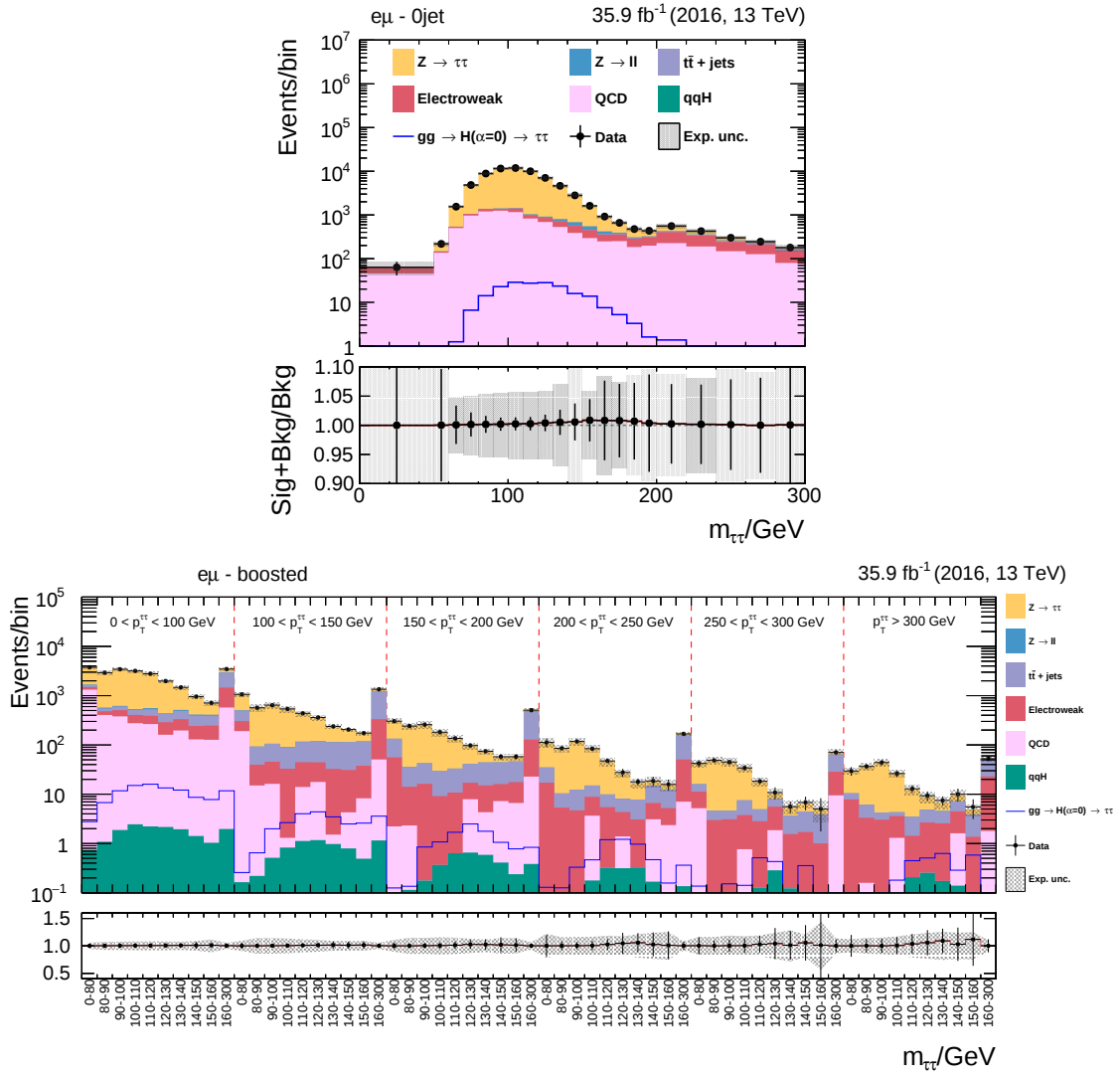
Fig. A.17.: Prefit distributions of the 0\text{-jet} and \text{boosted} categories in the e\mu channel using the MELA approach.
