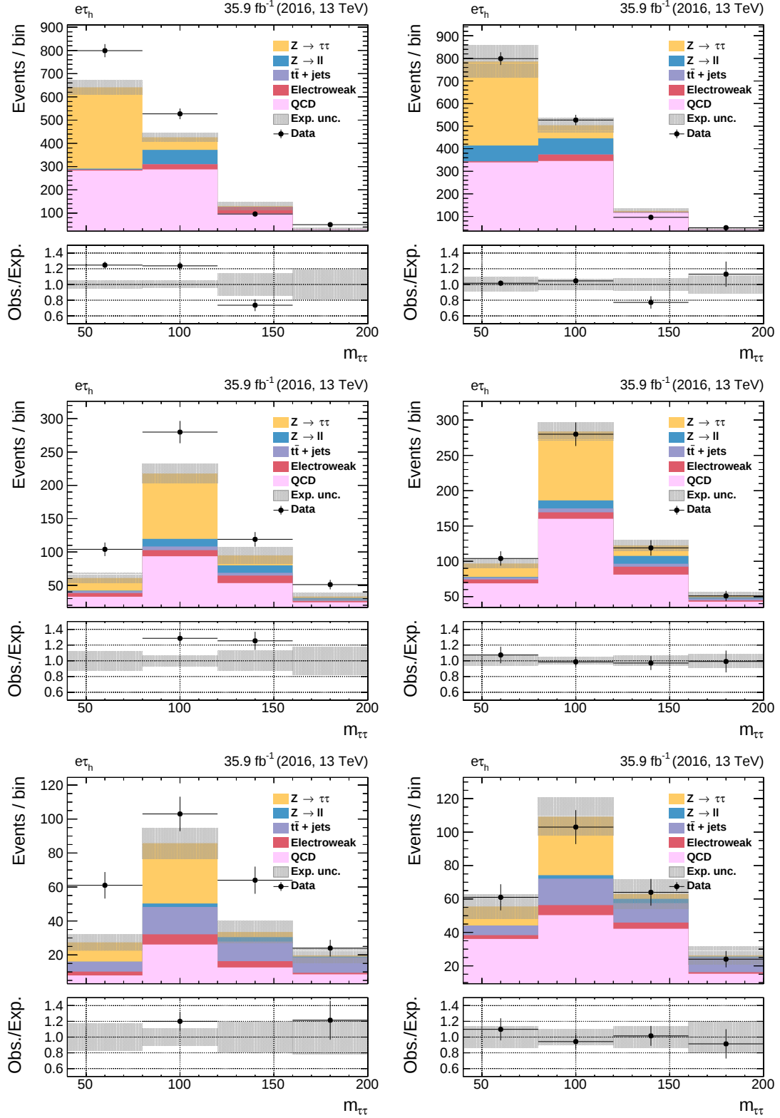
Fig. 3.21.: Prefit (left) and Postfit (right) distributions in the e\tau_h channel for the near sideband for the 0-jet (upper row), boosted (middle row) and dijet (bottom row) categories. During the fit, the QCD rate is pulled by the fit to find an optimal normalization of the background to describe data.
