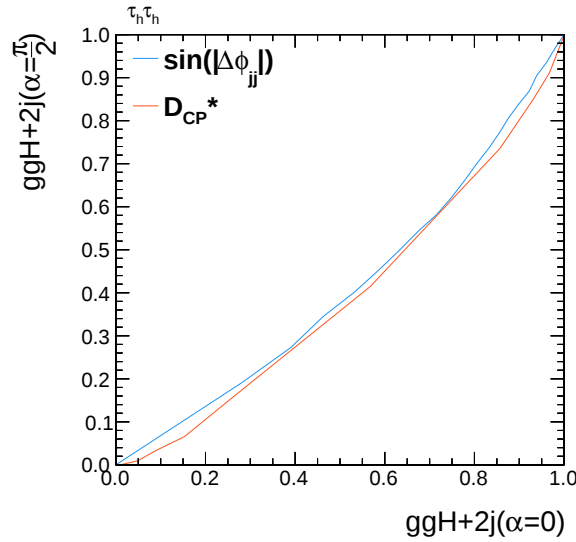
Fig. 3.8.: Comparison of ability to separate scalar and pseudoscalar fermionic couplings in the \tau_h\tau_h channel in the dijet boosted category. It can be seen, that the MELA approach has more potential to distinguish between scalar and pseudoscalar hypotheses.
