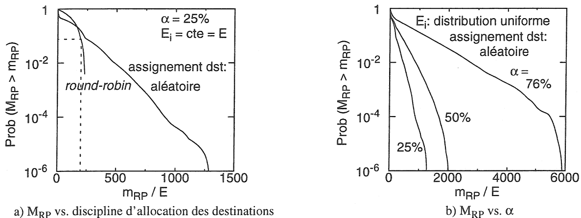
Figure 6-7: Distribution de M_{RP}
