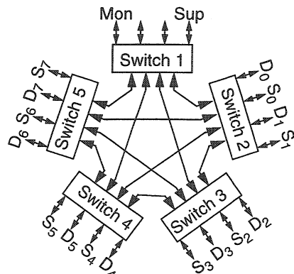
a) 20-node star with five 8-port switches
