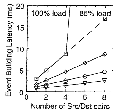
a) Event building 18-node star network
