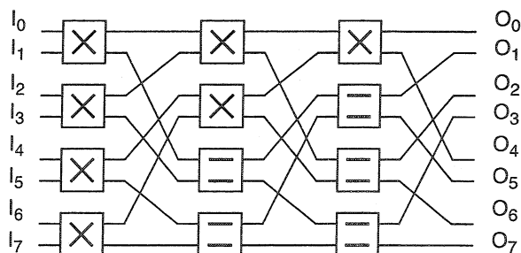
Figure 2. Omega Network
