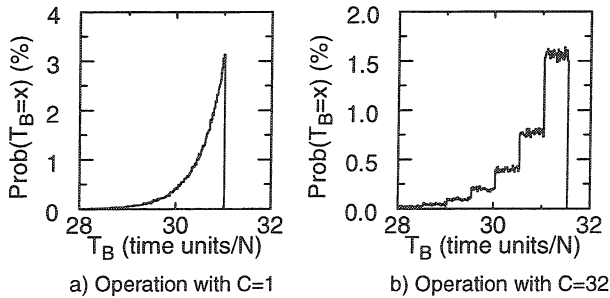
Figure 4: Event Building latency distribution
