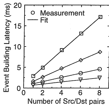
b) Event building 20-node star network
