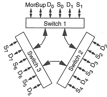
b) 18-node star with three 8-port switches
