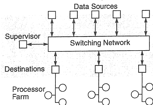
Figure 1. Event Builder
