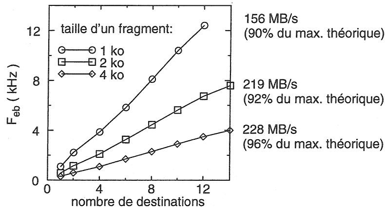
Figure 9-15: Performance en mode event builder .
