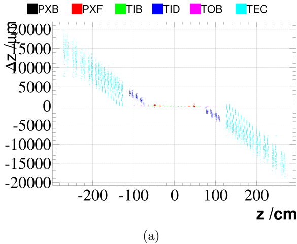
Figure 7.13: The dz - z distribution of the alignment procedure without (a) and with (b) the TID and TEC end cap disks constraints.
