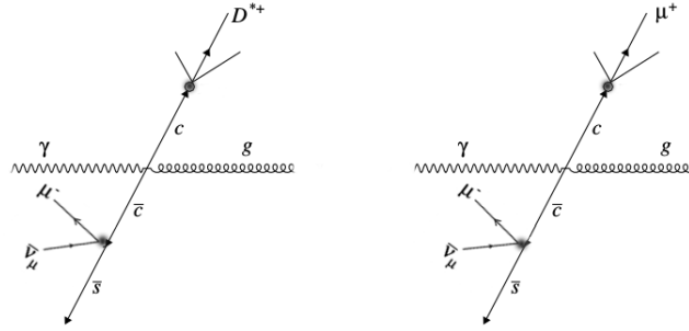
Figure 5.3: Illustration of the two similar topologies of c\bar{c} events. The sketch shows the topology of events with the production of D^*\mu (left) and \mu\mu (right) pairs.
