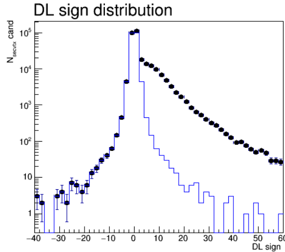
Figure 7.22: The decay length distribution of the B candidates. The distributions shows the B decay distribution which was used to clean the B signal.
