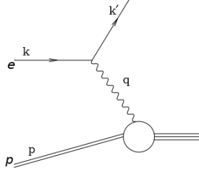
Figure 1.3: Lepton-proton scattering via exchange of boson.
