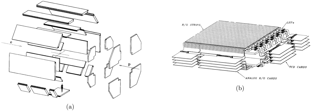
Figure 2.7: Exploded view of the rear and barrel muon detectors (a), and layout sketch of the single element of a BMUO chamber [61].
