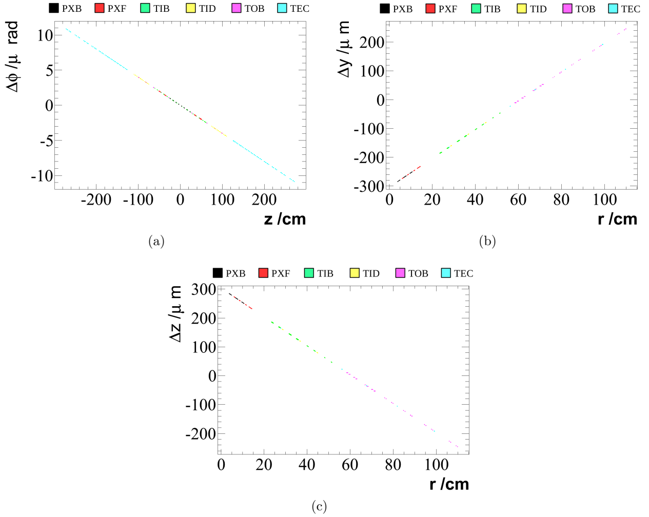
Figure 7.4: The misalignment for the three weak modes : twist (a), sagitta(b) and telescope (c). Linear misalignment functions are applied to the six tracker parts. The different components are marked with six different colors. A single point shows the position for the single or grouped modules. This depends on the granularity during the alignment procedure.
