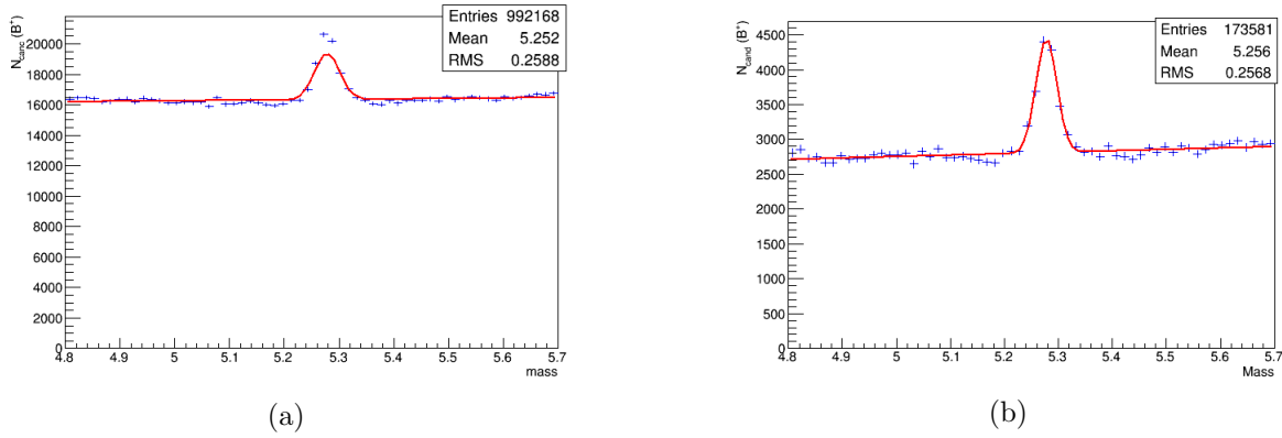
Figure 7.21: Invariant mass distribution of B^+ candidates. The left distribution shows the invariant mass without decay length cut, and with cut on decay length > 0.1 mm, plot (b).
