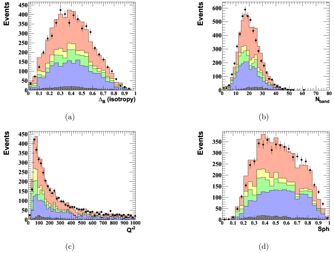
Figure 7.26: The isotropy(a), instanton band(b), quark virtuality(c) and sphericity(d) variables with instanton events included.
