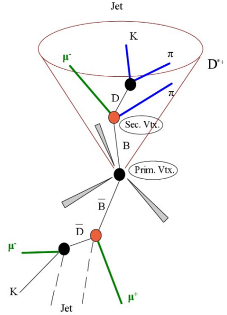
Figure 3.1: The example event illustration.
