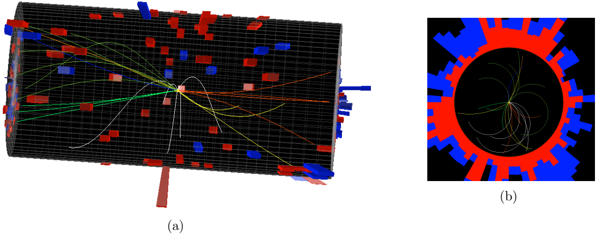
Figure 7.23: The CMS detector sketch with track collection example. The detector is shown in the y - z plane (a) and the x - y plane (b).
