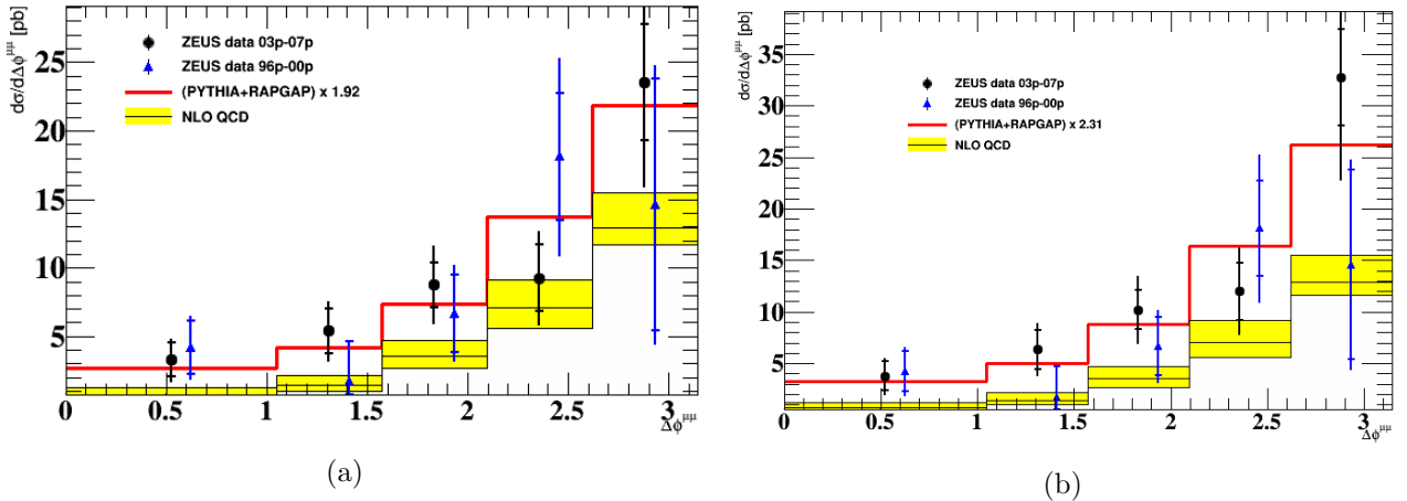
Figure 6.2: Differential cross section in \Delta\phi^{\mu\mu} bins. The dimuon events satisfy cuts on p_T and on \eta listed at the beginning of this section. The HERA II analysis (black points) are compared to the HERA I (blue triangles) and to the NLO QCD prediction from FMNR \otimes PYTHIA (yellow band) and with LO PYTHIA and RAPGAP (red line). The left part corresponds to the measured differential cross section with the S_{cc} = 1.37 . The right part is measured with the S_{cc} = 1.12 , scale factor obtained after the DL fit procedure.
