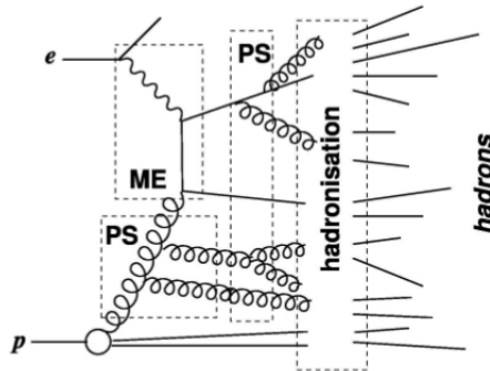
Figure 1.14: Structure of an event generated by a BGF process in ep collisions. The image is taken from [117].
