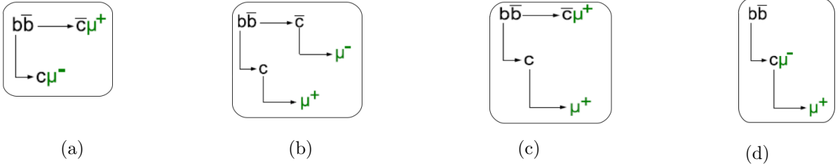
Figure 4.1: Muon pair sources in e^\pm p collisions.
