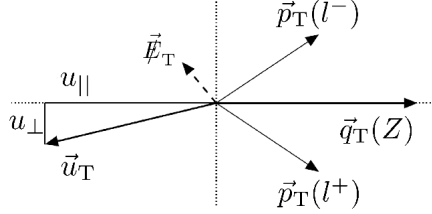
Figure 5.5 – Schematic view of the Z boson transverse momentum \vec{q}_T , the hadronic recoil \vec{u}_T with its parallel and perpendicular projections along \vec{q}_T , and the \vec{E}_T . [104]
