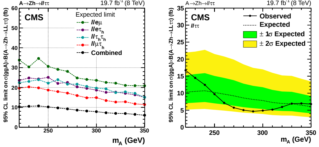
Figure 10.9 – Left: Comparison between the expected limits in the four di-tau final states. Right: Observed and expected upper limits at 95% on the production cross section times branching fraction, for the combination of all the final states studied in this analysis. [123]
