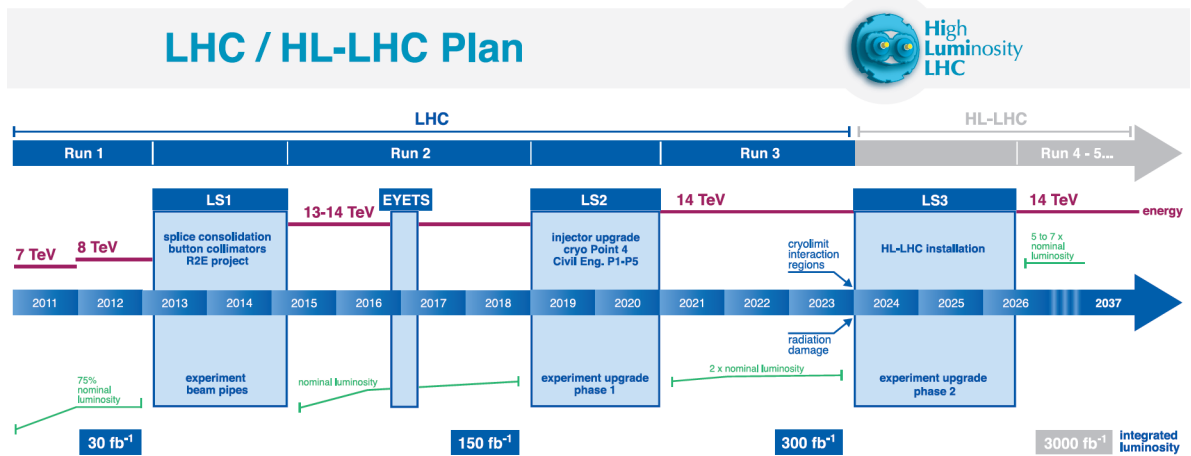
Figure 4.3 – Overview of LHC schedule until 2037. The integrated luminosity collected in Phase-1 is expected to reach 300 \text{fb}^{-1} , while 3000 \text{fb}^{-1} should be collected by the end of Phase-2. [82].
