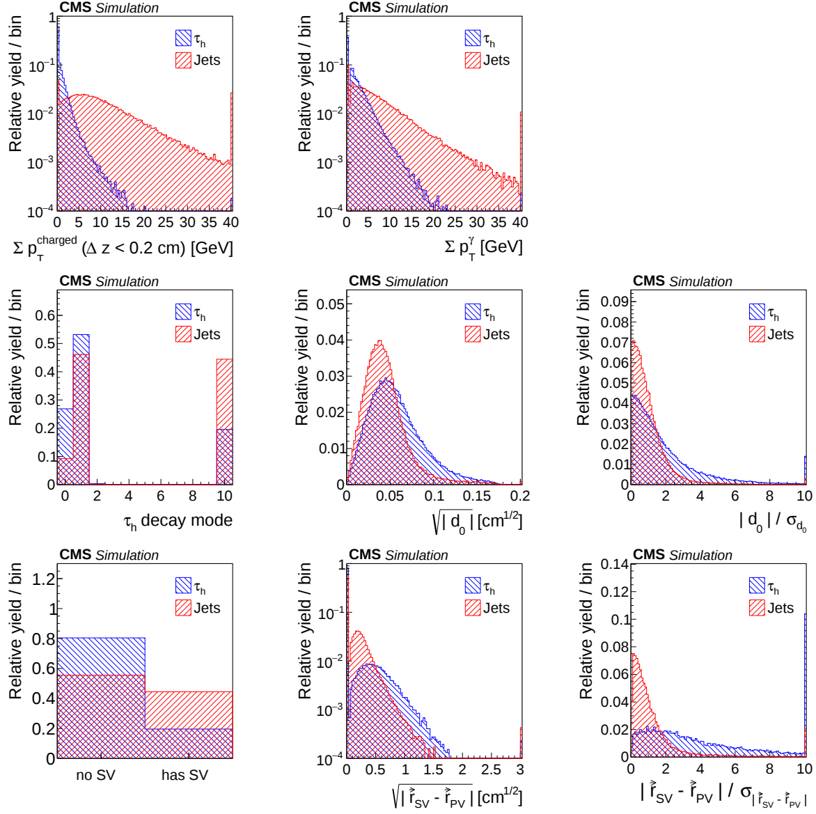
Figure 6.1 – Input variables distributions, normalized to unity, for the MVA-based isolation discriminator for simulated Z/\gamma^* \rightarrow \tau\tau (blue) with real hadronic taus and W+\text{jets} (red) events with jets. In the \tau decay mode plot the entry 0 represents the decay mode "one prong", 1 and 2 represent the decay modes "one prong plus one strip" and "one prong plus two strips" respectively and the entry 10 represents the "three prongs" decay mode. [103]
