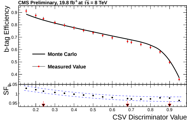
Figure 5.2 – B-tagging efficiency as a function of the CSV discriminator threshold, in 8 TeV simulations and data. The arrows indicate the three working points in Run-1. For information, the misidentification probabilities for jets with p_T between 80 and 120 GeV are, for the loose, medium and tight working points respectively, 0.0990 \pm 0.0004 , 0.0142 \pm 0.0002 and 0.0016 \pm 0.0001 , where the quoted uncertainties are statistical only. [99]
