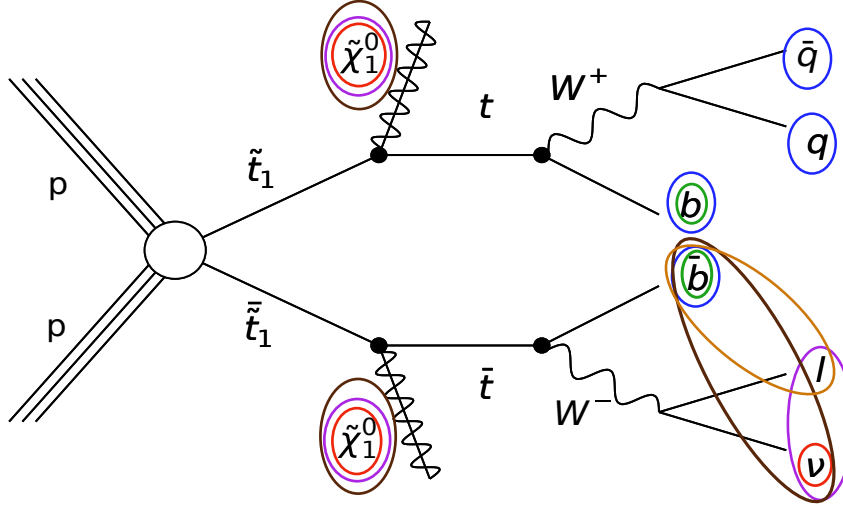
Figure 5.5: Diagram of the T2tt signal model supporting the choice of N_J (blue), E_T^{miss} (red), M_T (magenta), \min\Delta\phi(j_{1,2}, E_T^{miss}) (brown) and M_{\ell b} (orange) as discriminating variables [130].
