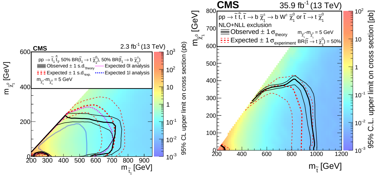
Figure 5.16: The exclusion limits at 95% CL on the T2tb model corresponding to an integrated luminosity of 2.3 fb -1 [129] (left) and 35.9 fb -1 [128] (right). The interpretation is provided in the context of SMS, in the plane of the stop mass vs the LSP mass. The color code shows the 95% CL upper limit on the cross section assuming a branching ratio of 50% in \tilde{t}_1 \rightarrow t\tilde{\chi}_1^0 and 50% in \tilde{t}_1 \rightarrow b\tilde{\chi}_1^\pm . The red and black contours represent the expected and observed exclusion limits, respectively. The blue and magenta lines in the left plot show the expected limits of 1 \ell and 0 \ell analyses, respectively. The area below the black thick curve indicates the excluded region of the signal points.
