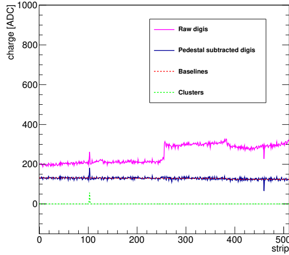
Figure 2.7: Example of data from one tracker module undergoing zero suppression and clustering. The raw digis are shown in pink. From the raw digis the pedestals are subtracted and the resulting digis are shown in blue. From pedestal subtracted digis the baselines shown in red are computed and subtracted. The final clusters are shown in green.
