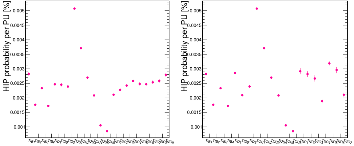
Figure 2.24: The average probability of a HIP event per PU for layers (left, right) of TIB, TOB, and wheels (left) or rings (right) of the TID and TEC partitions of the silicon strip tracker, computed from the data run 281604.
