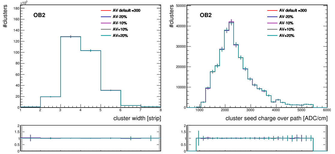
Figure 3.13: On-track cluster width (left) and cluster seed charge (right) in simulation for the OB2 geometry and for different values of the applied voltage AV . The simulated distributions are normalized by the same factors as in the left plots of Figs. 3.4 and 3.6, respectively. In the ratio plots the default simulation is divided by different simulation scenarios.
