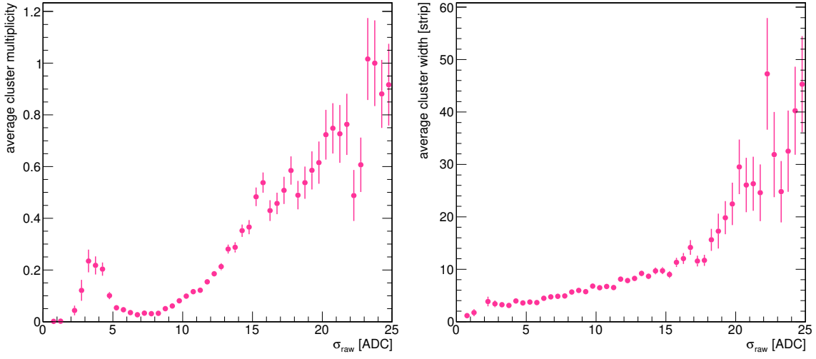
Figure 2.29: The average cluster multiplicity (left) and average cluster width (right) as a function of \sigma_{raw} of the non-collision events after the HIP for the run 281604.
