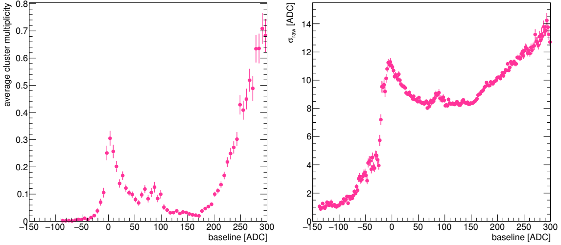
Figure 2.30: The average cluster multiplicity (left) and \sigma_{raw} (right) as a function of the baseline of the non-collision events after the HIP for the run 281604.
