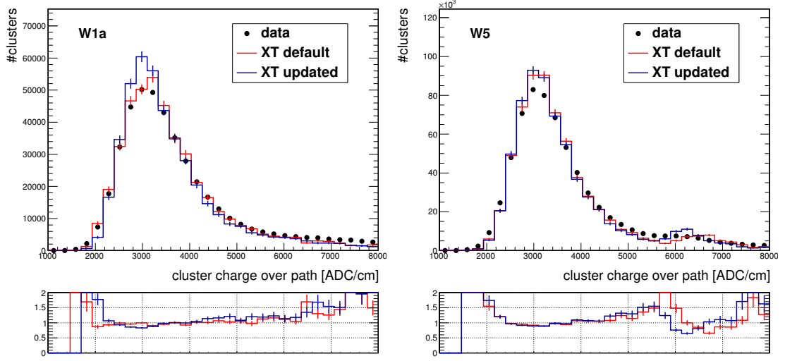
Figure 3.48: Distribution of the on-track cluster charge in data and simulation for the W1a (left) and W5 (right) geometries, for current (default) and newly updated cross talk parameters ( XT ). The simulated distributions are rescaled to the number of clusters in data. The bottom plots represent the data to simulation ratios.
