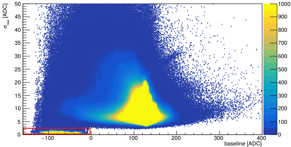
Figure 2.12: The 2-D distribution of the \sigma_{raw} of raw digis (y-axis) versus the baseline (x-axis) for the run 273162. The baselines selected as HIP events are indicated by a red box.
