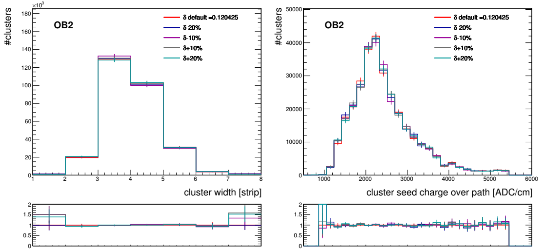
Figure 3.10: On-track cluster width (left) and cluster seed charge (right) in simulation for the OB2 geometry and for different values of the delta ray production cut-off \delta . The simulated distributions are normalized by the same factors as in the left plots of Figs. 3.4 and 3.6, respectively. In the ratio plots the default simulation is divided by different simulation scenarios.
