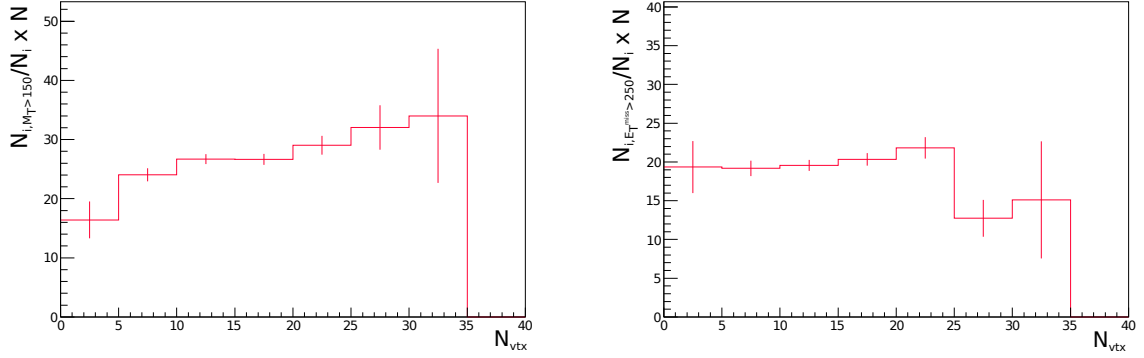
Figure 5.13: The evolution of the fraction of events with M_T > 150 GeV (left) and E_T^{\text{miss}} > 250 GeV (right), multiplied by the total number of events, as a function of the reconstructed primary vertex multiplicity. The study has been performed in the context of the 2015 analysis.
