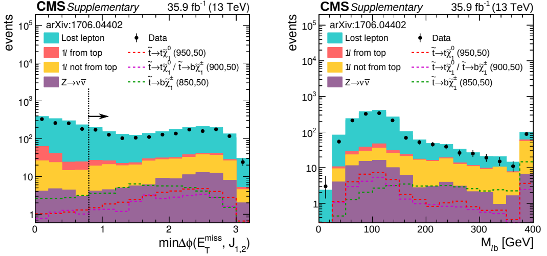
Figure 5.7: Data (black dots), background (full colored histograms) and signal (dashed lines) distributions of the \min\Delta\phi(j_{1,2}, E_T^{\text{miss}}) (left) and M_{\ell b} (right) variables after applying the baseline selection. The cut on \min\Delta\phi(j_{1,2}, E_T^{\text{miss}}) is not applied in the the left plot, but only indicated by the black arrow [144].
