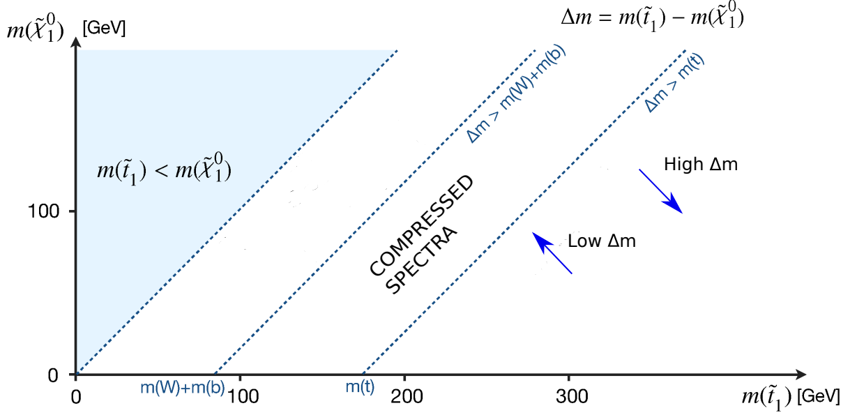
Figure 5.4: The plane of stop ( \tilde{t}_1 ) versus LSP ( \tilde{\chi}_1^0 ) masses [137].
