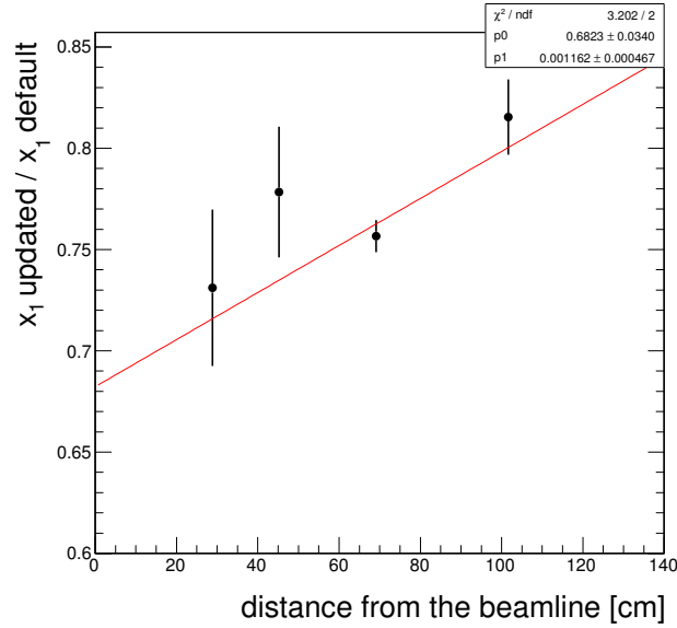
Figure 3.43: The ratio of the new measurement of the x_1 parameter (updated) to the default value currently used in simulation (default) as a function of the distance from the beamline of the four different barrel geometries. The result of a linear fit is indicated in red.
