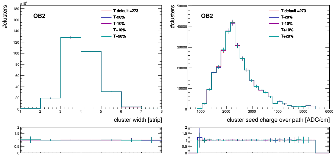
Figure 3.17: On-track cluster width (left) and cluster seed charge (right) in simulation for the OB2 geometry and for different values of the temperature T . The simulated distributions are normalized by the same factors as in the left plots of Figs. 3.4 and 3.6, respectively. In the ratio plots the default simulation is divided by different simulation scenarios.
