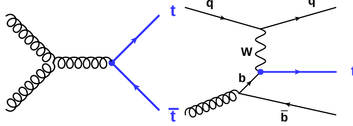
Figure 2.2: Mechanisms of top quark production. Left: top quark pair production via gluon fusion. Right: electroweak t-channel single top quark production.
