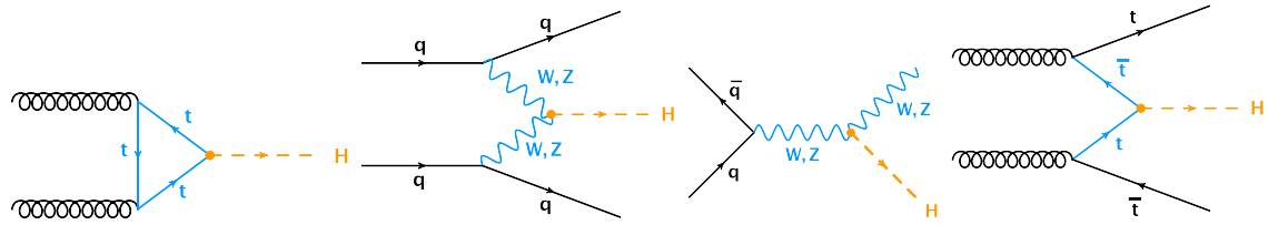
Figure 2.3: The main Higgs-boson production mechanisms. The Feynman diagrams are arranged according to the cross sections of the shown processes. In decreasing order of cross section from left to right: gluon fusion, vector-boson fusion, associated production of vector bosons, and associated production of top quarks.
