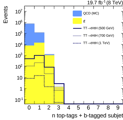
Figure 7.8: Multiplicity of CA15 jets with p_T > 200 GeV that are tagged by the HEPTopTagger and contain a subjet that is b tagged by the CSV algorithm at medium working point. Events with at least one of these jets are selected. In this distributions only events passing the preselection and containing at least two CA15 jets are regarded. Furthermore, one of the CA15 jets in all of these events is tagged by the HEPTopTagger algorithm. Events in the first bin contain a top-tagged CA15 jet, but no b-tagged subjet is found within this jet. The statistical uncertainty in the two background contributions is depicted by the grey hashed error bands.
