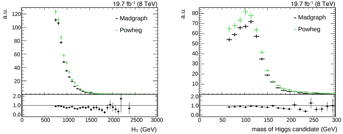
Figure B.2: Comparison of the H_T (left) and Higgs-candidate mass (right) distributions for t\bar{t} events simulated with MADGRAPH and POWHEG. The p_T -reweighting scale factors are applied to the events in the MADGRAPH sample only.
