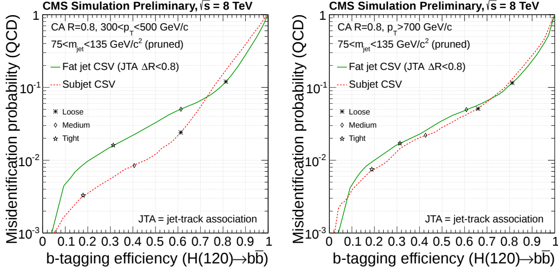
Figure 5.15: Performance of the Higgs-tagging algorithm (red) compared to the performance of direct application of the b-tagging algorithm to CA8 jets. In this comparison the CSV b-tagging algorithm at medium working point is used. Left: 300 < p_T(\text{jet}) < 500 GeV. Right: p_T(\text{jet}) > 700 GeV [14].
