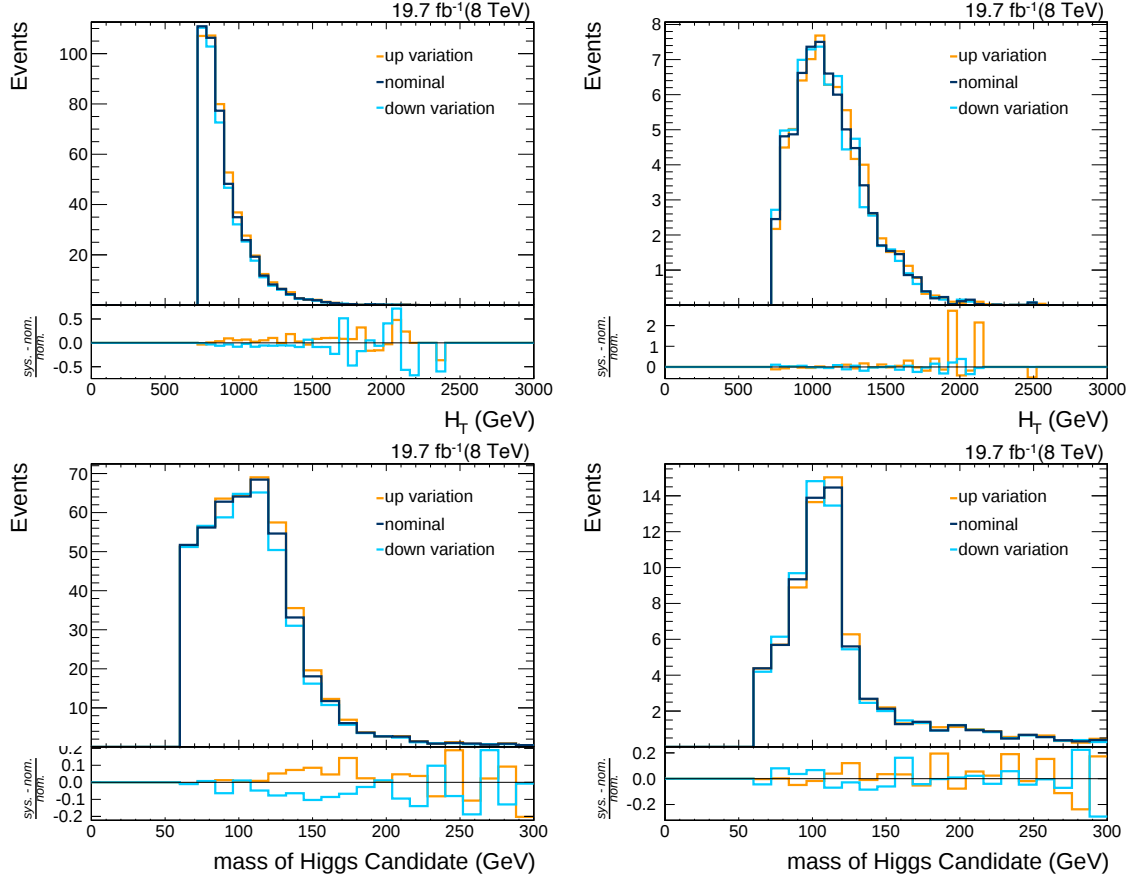
Figure 7.18: Impact of the uncertainties in the subject energy scale on rate and shape of the H_T (top) and Higgs-candidate mass (bottom) distributions for t\bar{t} events (left) and signal events simulated with a T' -quark mass of 700 GeV (right). The relative impact of the upward and downward variation of the uncertainty with respect to the nominal distribution is shown in the bottom part of each plot.
