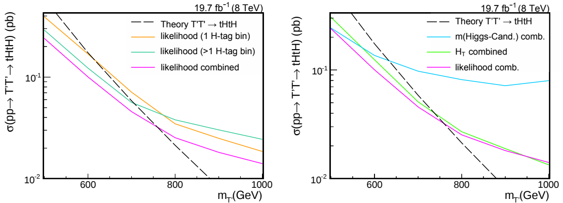
Figure 7.32: Comparison of the expected upper exclusion limits at 95% confidence level on the cross section for T'-quark pair production. Left: limits obtained from the likelihood variable L in the single (orange) and multi (blue) Higgs-tag categories and in a simultaneous analysis of both categories (magenta). Right: limits obtained from the H_T (green), Higgs-candidate mass (blue), and likelihood (magenta) variables in simultaneous analysis of the single and multi Higgs-tag categories.
