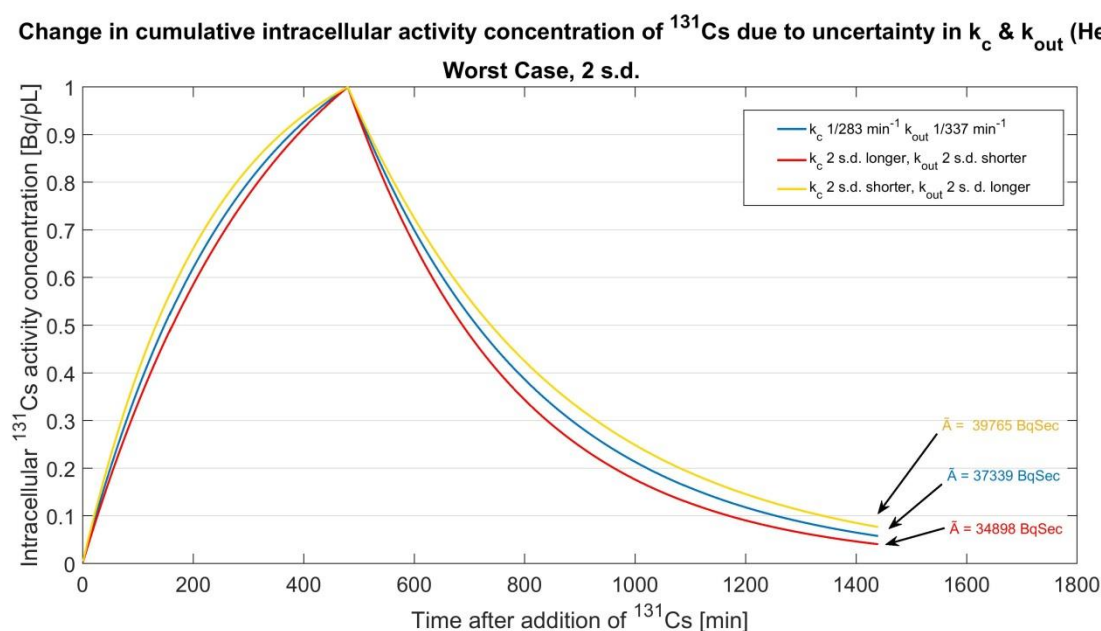
Figure 8.1 Uncertainty in cumulative activity concentration due to variations in k_c & k_{out}
