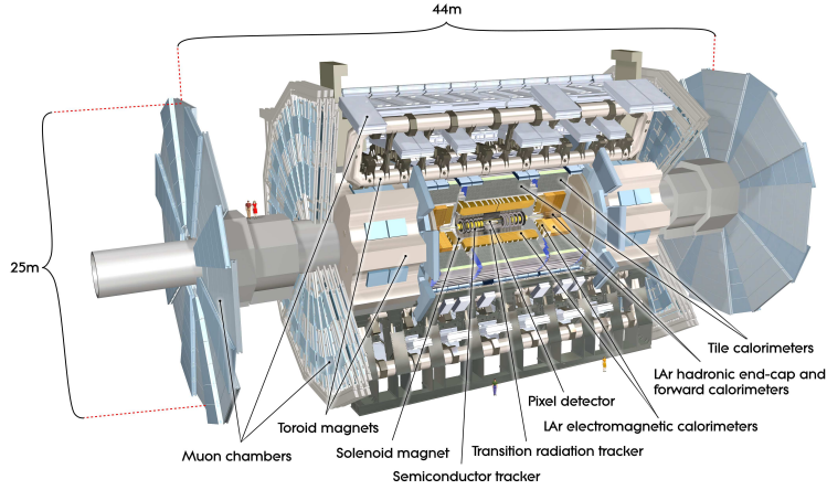
Figure 2.1: Cut-away view of the ATLAS detector. The dimensions of the detector are 25 m in height and 44 m in length. The overall weight of the detector is approximately 7000 tonnes.
