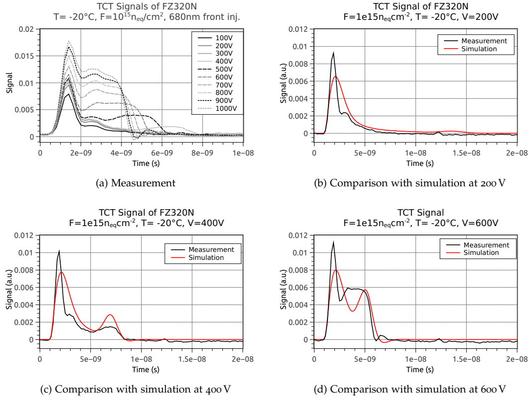
Figure 11.13: TCT signals and comparison with simulation at F = 10^{15} \text{ n}_{eq}/\text{cm}^2 (p):
