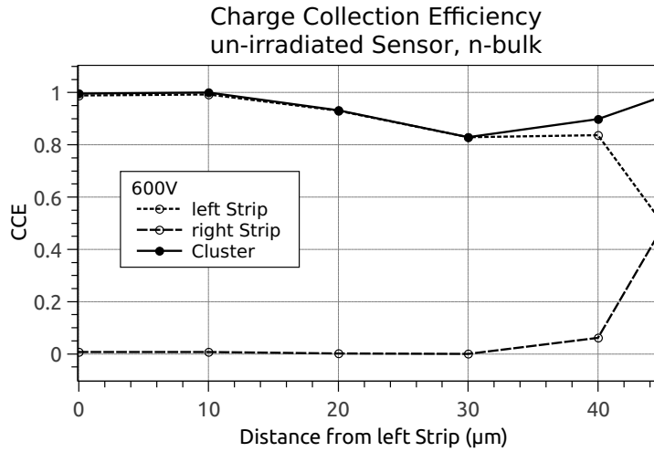
Figure 8.32: Charge collection efficiency of a un-irradiated n-bulk strip sensor with pitch 90\text{ }\mu\text{m} geometry: In the center of the strip, 100% of the charge is collected. At 30\text{ }\mu\text{m} , 15% less charge is collected. At the center of the pitch, each strip collects 50% of the signal.
