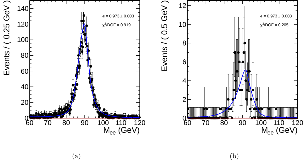
Figure 9.14: The fits for the ID→Trig step in the Ecal Endcap. The data is in black, background fit in red, and signal+background fit in blue: (a) passing sample, (b) failing sample.
