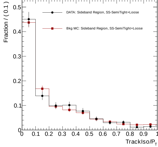
Figure 7.9: The background template extracted from the data (black) and the background MC (red).
