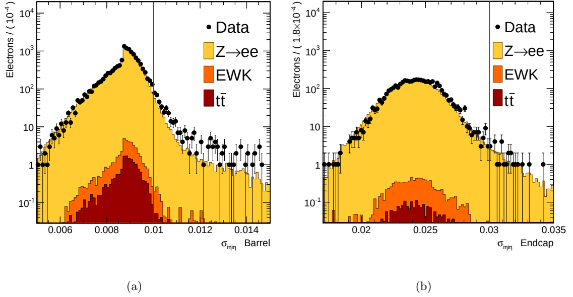
Figure 6.16: The \sigma_{in\eta} distribution of the associated electrons: (a) Ecal Barrel, (b) Ecal Endcap.
