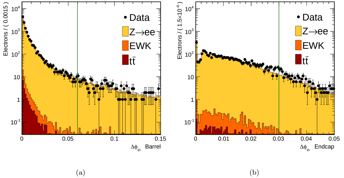
Figure 6.17: The \Delta\phi_{in} distribution of the associated electrons: (a) Ecal Barrel, (b) Ecal Endcap.
