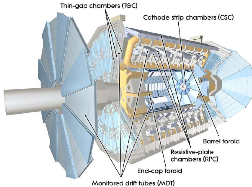
FIGURE 4.8: Cut-away view of the ATLAS muon system. [55]
