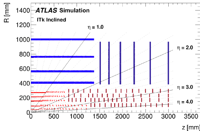
FIGURE 4.11: Schematic layout of the ITk for the HL-LHC phase of ATLAS. The horizontal axis is the axis along the beam line with zero being the interaction point. The vertical axis is the radius measured from the interaction point [73].
