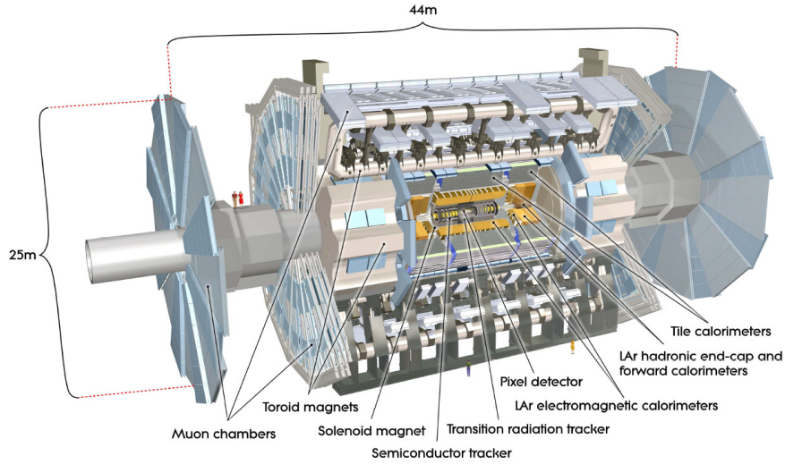
FIGURE 4.5: Overview of the ATLAS detector with its main components. [55]
