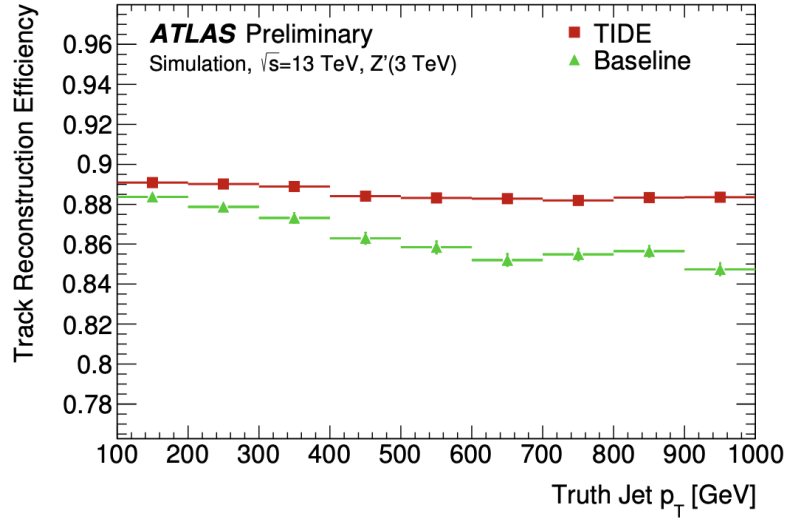
FIGURE 4.16: The average efficiency to reconstruct primary tracks in jets as a function of jet p_T . Two track reconstruction algorithms are shown : green triangles label the baseline reconstruction (no neural network) and red squares label the TIDE (tracking in dense environment) optimised reconstruction using neural networks [75].
