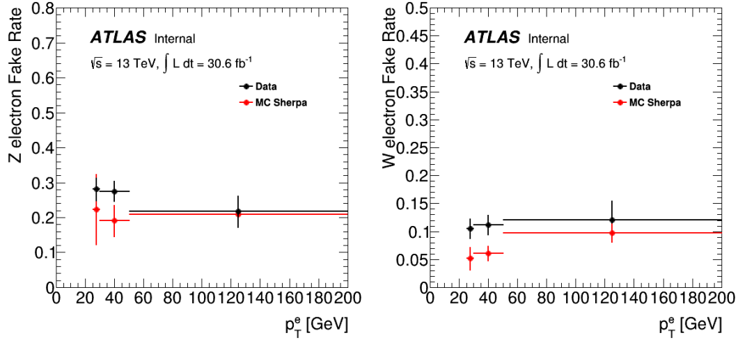
FIGURE 5.19: Distributions of the electron fake rate as a function of p_T in the Z+jets control region, using the Z electron selection on the left. The electron fake rate using the W electron selection is shown on the right.
