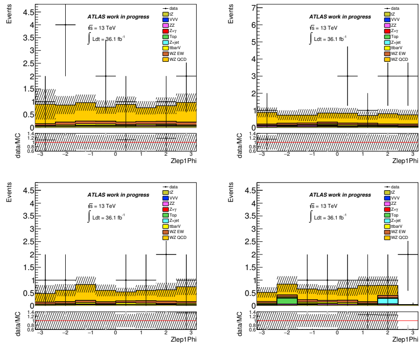
FIGURE II.3: Distributions of the Z leading lepton \Phi for the \mu\mu\nu\mu top left, \mu\mu\nu e top right, ee\nu\mu bottom left and ee\nu e bottom right decay channels.
