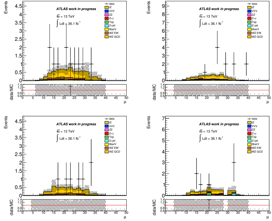
FIGURE II.14: Distributions of the average number of interactions per bunch crossing for the \mu\mu\nu\mu top left, \mu\mu\nu e top right, ee\nu\mu bottom left and ee\nu e bottom right decay channels.
