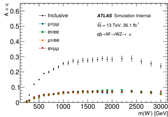
FIGURE 5.13: The signal selection acceptance times efficiency ( A \times \epsilon ), defined as the ratio of the number of \text{MC} signal events in the q\bar{q} category to the number of generated signal events, as a function of the \text{HVT} resonance mass. The error bars represent the total statistical and systematic uncertainties.
