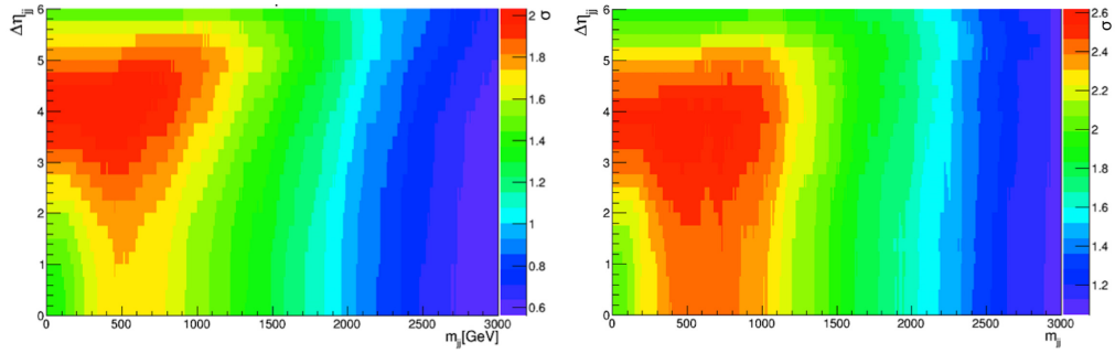
FIGURE 5.9: 2D scan of the variables m_{jj} and |\Delta\eta_{jj}| for the 200 GeV GM mass point (left) and the 250 GeV HVT mass point(right), the colour corresponds to the expected signal significance Z as defined in equation 5.5.
