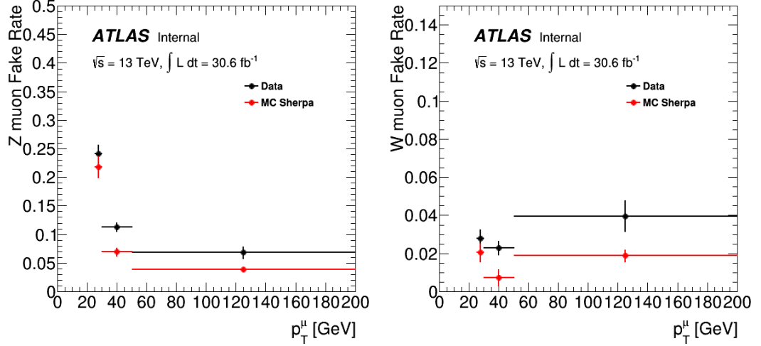
FIGURE 5.18: Distributions of the muon fake rate as a function of p_T in the Z+jets control region, using the Z muon selection on the left. The muon fake rate using the W muon selection is shown on the right.
