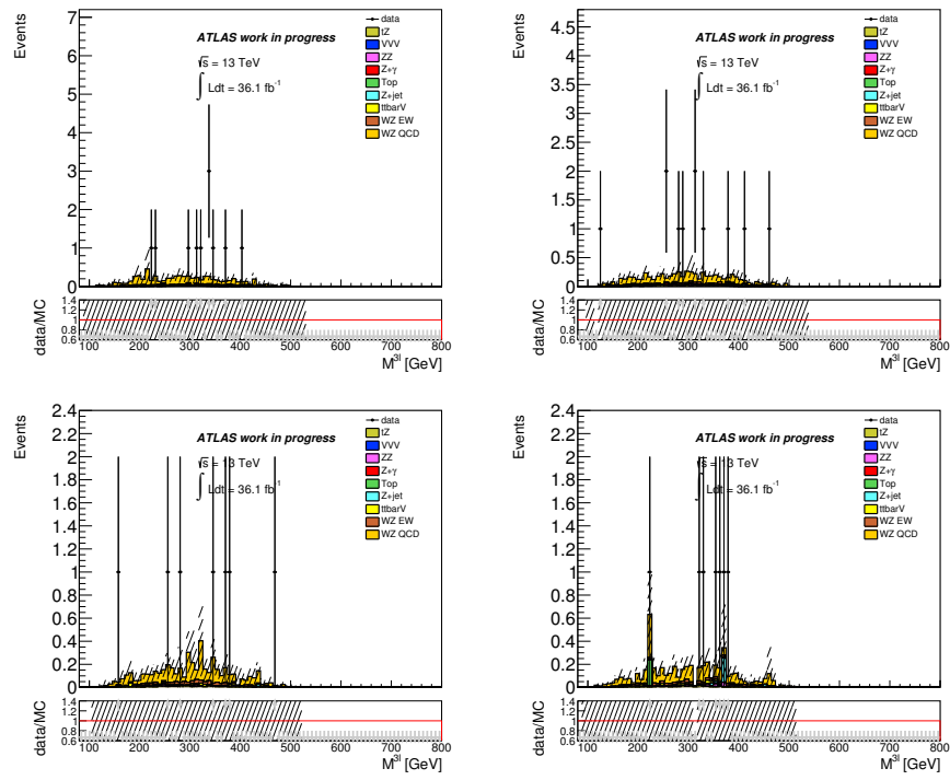
FIGURE II.11: Distributions of the three lepton invariant mass for the \mu\mu\nu\mu top left, \mu\mu\nu e top right, ee\nu\mu bottom left and ee\nu e bottom right decay channels.
