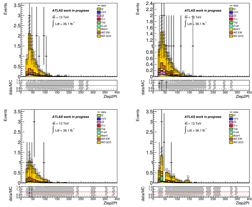
FIGURE II.4: Distributions of the Z sub-leading lepton p_T for the \mu\mu\nu\mu top left, \mu\mu\nu e top right, ee\nu\mu bottom left and ee\nu e bottom right decay channels.
