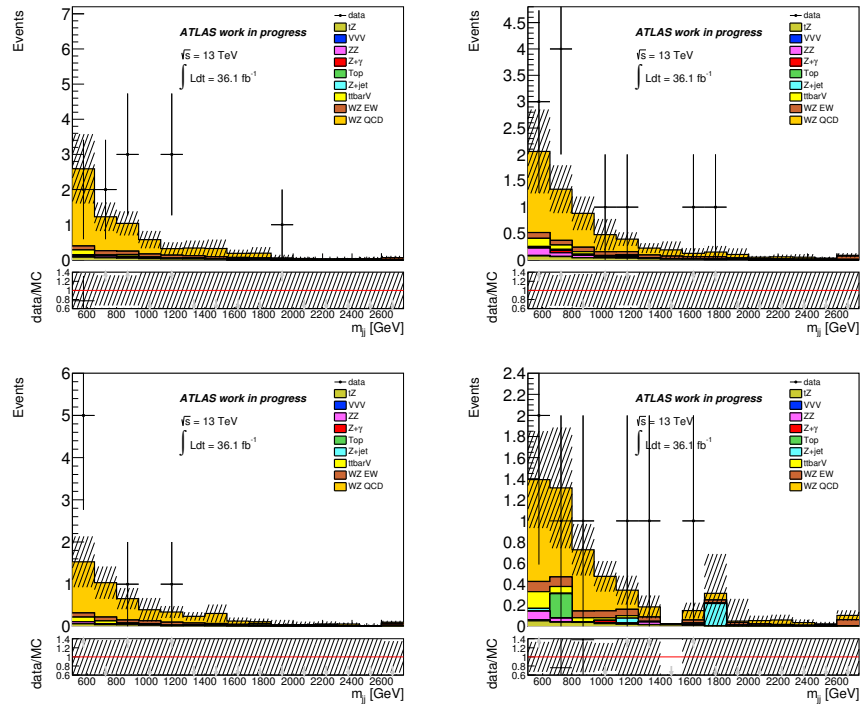
FIGURE II.13: Distributions of the di-jet invariant mass for the \mu\mu\nu\mu top left, \mu\mu\nu e top right, ee\nu\mu bottom left and ee\nu e bottom right decay channels.
