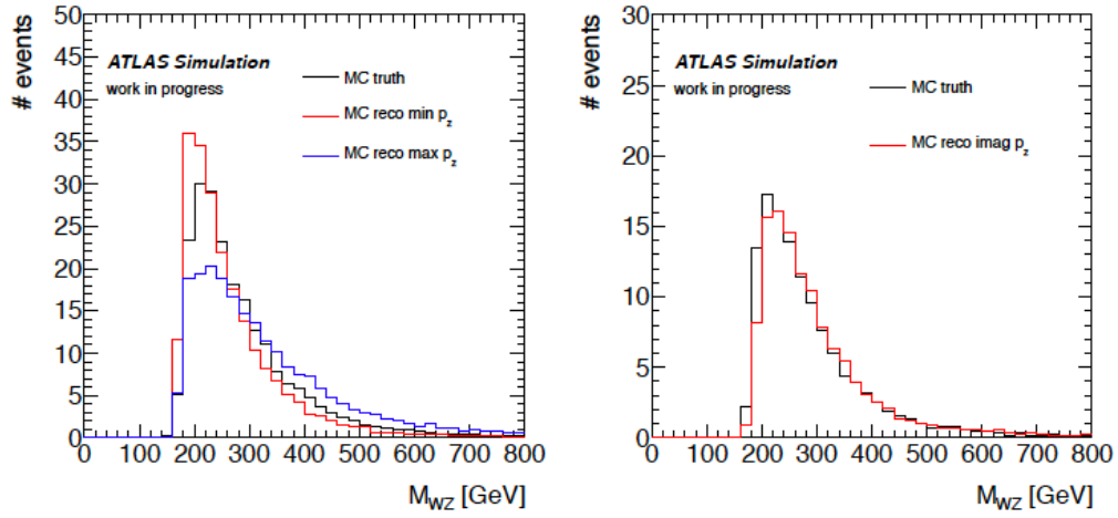
FIGURE 5.6: The plot on the left shows the reconstructed and truth WZ mass distribution obtained with MC. In black the truth WZ mass is shown, the red and blue curves show the reconstructed WZ mass when the minimum or maximum real solution of equation 5.4 are used. The plot on the right shows the truth and reconstructed WZ mass for complex solutions, in this case only the real part of the p_z^v solution is kept. [12]
