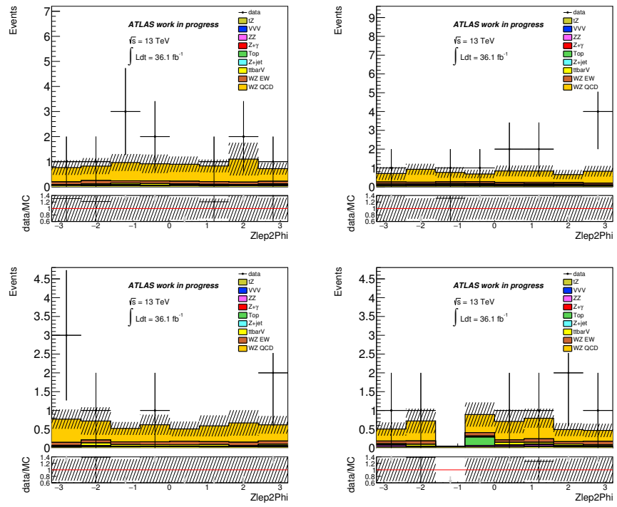
FIGURE II.6: Distributions of the Z sub-leading lepton \Phi for the \mu\mu\nu\mu top left, \mu\mu\nu e top right, ee\nu\mu bottom left and ee\nu e bottom right decay channels.
