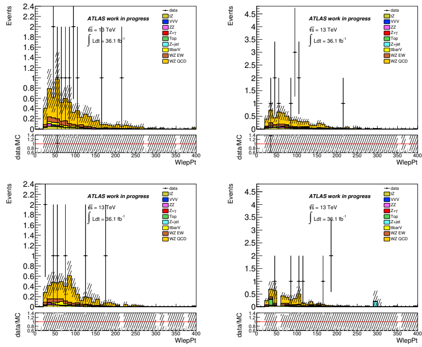
FIGURE II.7: Distributions of the W lepton p_T for the \mu\mu\nu\mu top left, \mu\mu\nu e top right, ee\nu\mu bottom left and ee\nu e bottom right decay channels.
