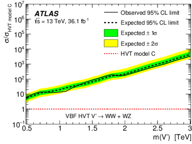
FIGURE 5.37: Observed and expected 95% C.L. upper limits on the V' cross section times branching fraction to WW or WZ for the \text{HVT} benchmark model, relative to the cross section times branching fraction for \text{HVT} model C. Results are shown for \text{VBF} production mechanisms. The model predictions are also shown. [83]
