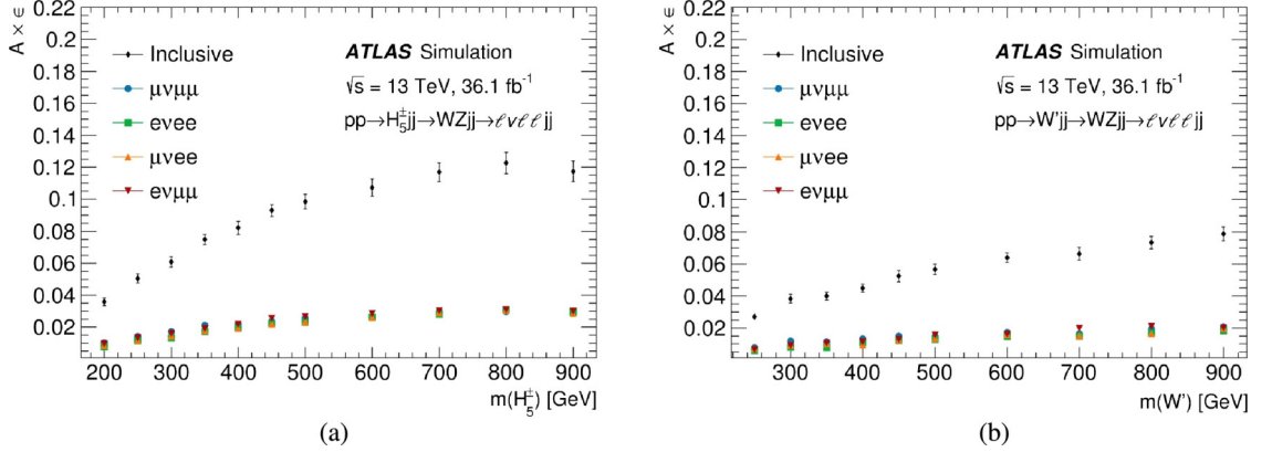
FIGURE 5.10: The signal selection acceptance times efficiency ( A \times \epsilon ), defined as the ratio of the number of MC signal events in the VBF category to the number of generated signal events, as a function of the H_5^\pm (a) and HVT (b) resonance mass. The error bars represent the total statistical and systematic uncertainties.
