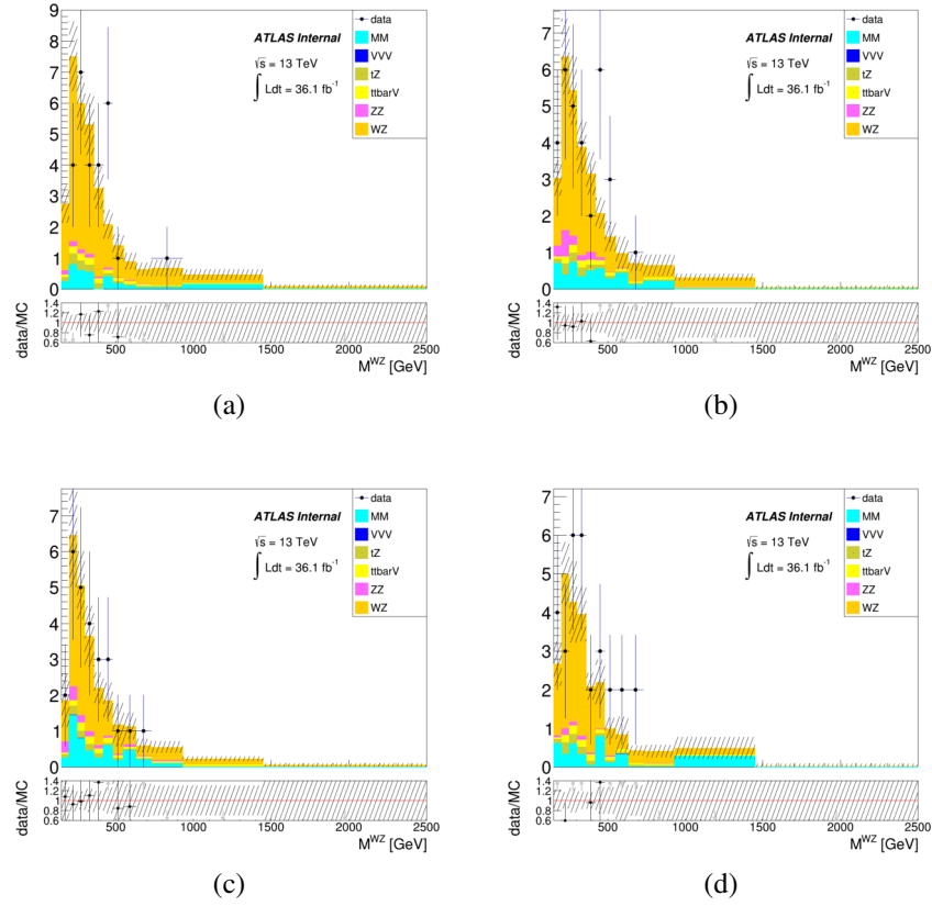
FIGURE 5.32: Control distributions of the invariant mass m_{WZ} separated by channels \mu^+\mu^-\mu^\pm (a), \mu^+\mu^-e^\pm (b), e^+e^-e^\pm (c), e^+e^-\mu^\pm (d). All MC expectations are scaled to the integrated luminosity of the data using the predicted MC cross sections of each sample.
