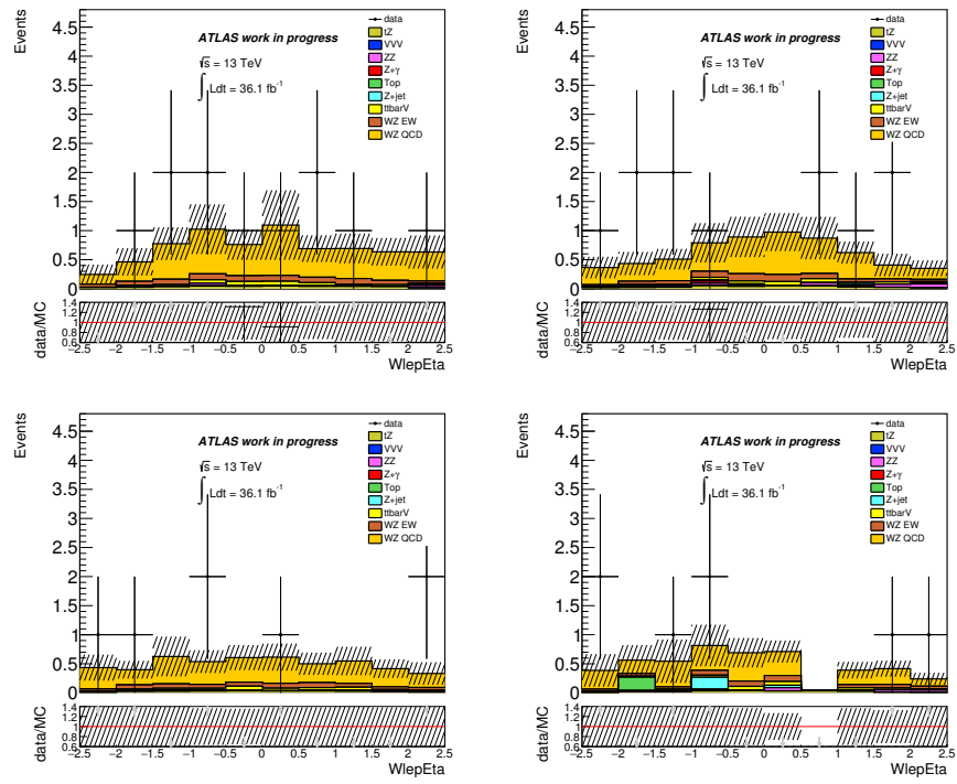
FIGURE II.8: Distributions of the W lepton \eta for the \mu\mu\nu\mu top left, \mu\mu\nu e top right, ee\nu\mu bottom left and ee\nu e bottom right decay channels.
