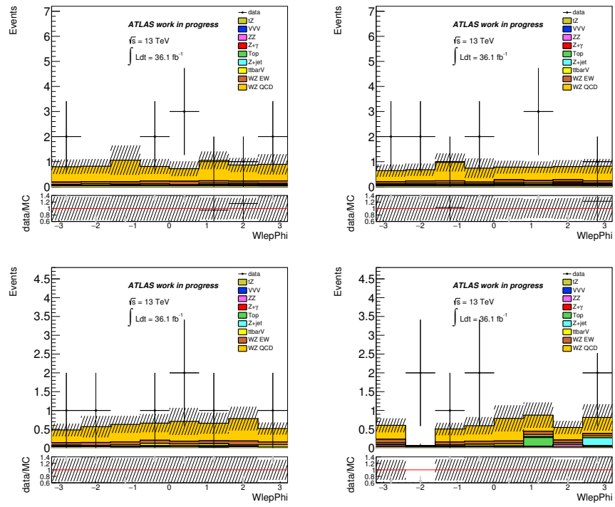
FIGURE II.9: Distributions of the W lepton \Phi for the \mu\mu\nu\mu top left, \mu\mu\nu e top right, ee\nu\mu bottom left and ee\nu e bottom right decay channels.
