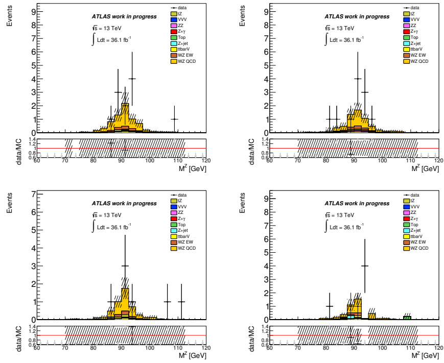
FIGURE II.10: Distributions of the Z boson invariant mass for the \mu\mu\nu\nu top left, \mu\mu\nu e top right, ee\nu\nu bottom left and ee\nu e bottom right decay channels.
