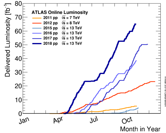
FIGURE 4.2: Cumulative integrated luminosity obtained in 8 years of data taking by the ATLAS experiment [54].
