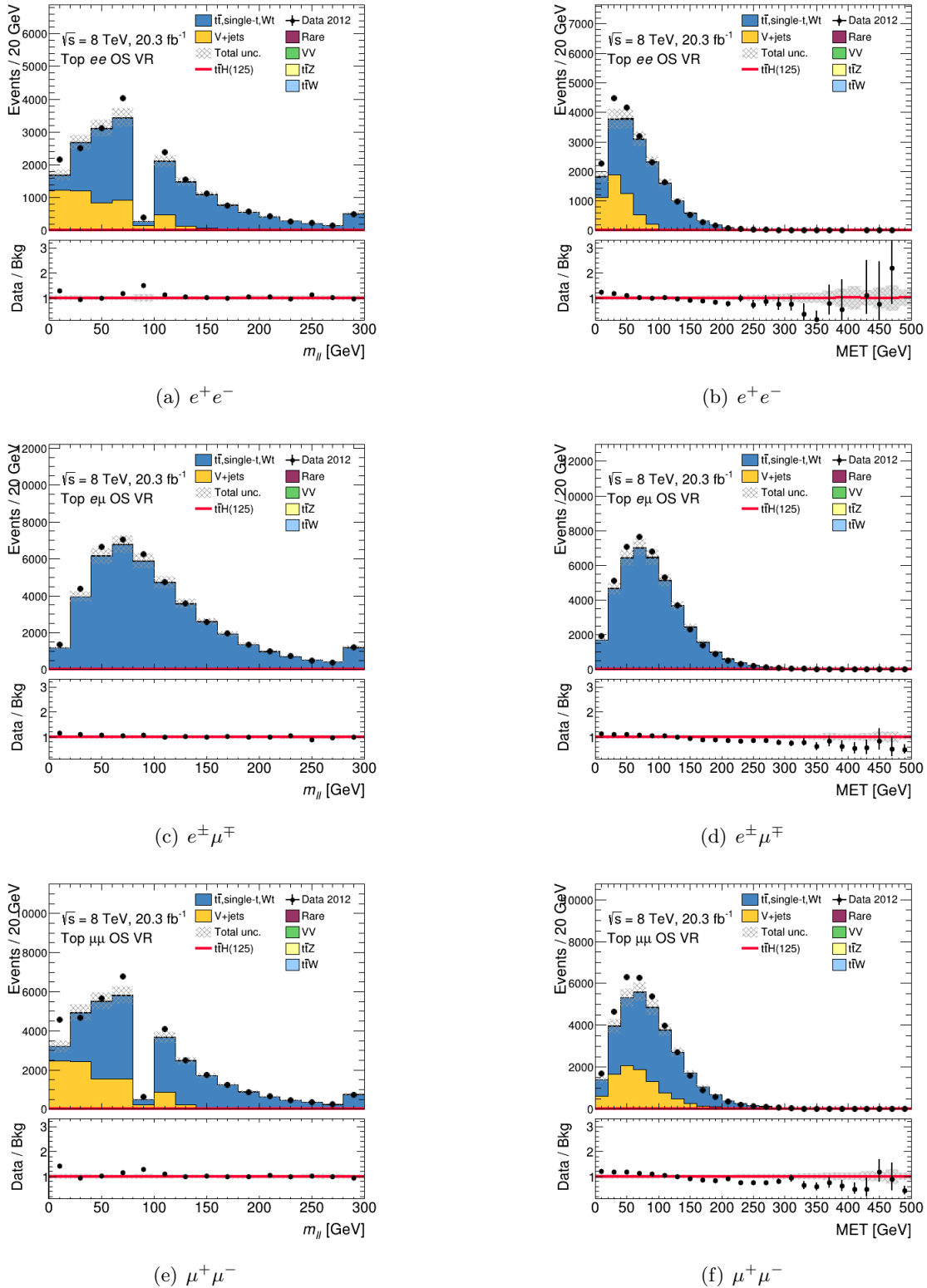
Figure C.14: Distributions of the di-lepton invariant mass (left) and E_T^{\text{miss}} (right) in the t\bar{t} opposite-sign validation region for e^+e^- (top), e^\pm\mu^\mp (centre) and \mu^+\mu^- (bottom) events. Events in data (black dots) are compared to the expected stacked contributions from prompt background processes. The expected signal contributions are overlaid to the backgrounds (red line). The lower panel shows the ratio of observed events in data to expected Standard Model events. The error bars on the data points show the statistical uncertainty and the dashed band shows the total uncertainties of the background predictions.
