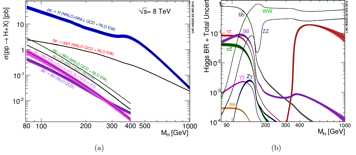
Figure 1.1: The cross-sections of the main Higgs boson production modes in proton-proton collisions for a centre-of-mass energy of 8 TeV (left) and the Higgs boson decay branching ratios (right) as a function of the Higgs boson mass [14] [15]. The coloured bands represent the theoretical uncertainties.
