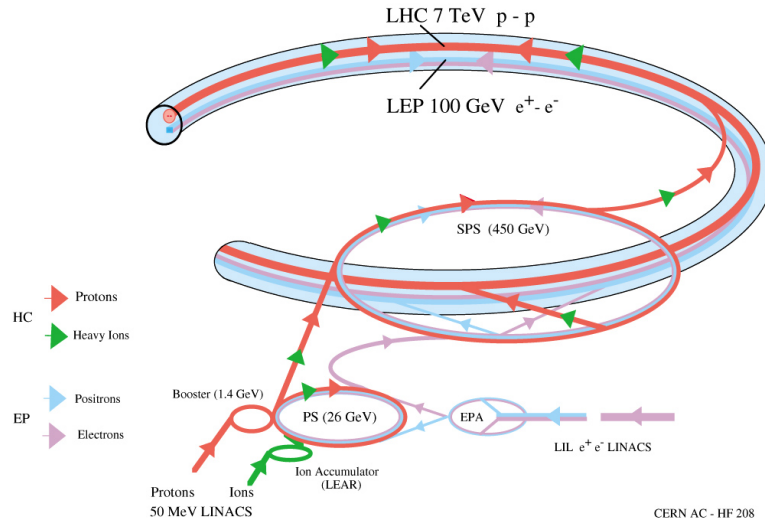
Figure 2.1: Schematic view of the LHC accelerator complex. [88]
