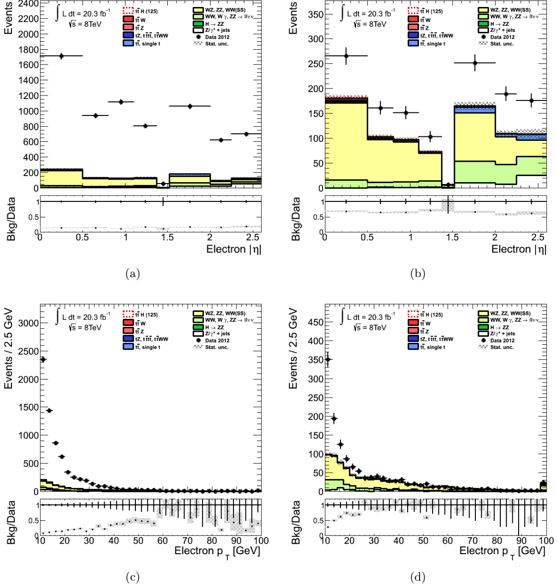
Figure 6.7: The |\eta| (top) and p_T (bottom) distributions of electrons passing (right) and failing (left) the tight selection in the W^\pm + \text{jets} same-sign lepton non-prompt region. Events in data (black dots) are compared to the expected stacked background contributions, non-prompt background excluded. Overflow events are added to the last bin. The lower panel shows the fraction of expected background yields. The error bars on the data points and the dashed band on the simulated background show the statistical uncertainties.
