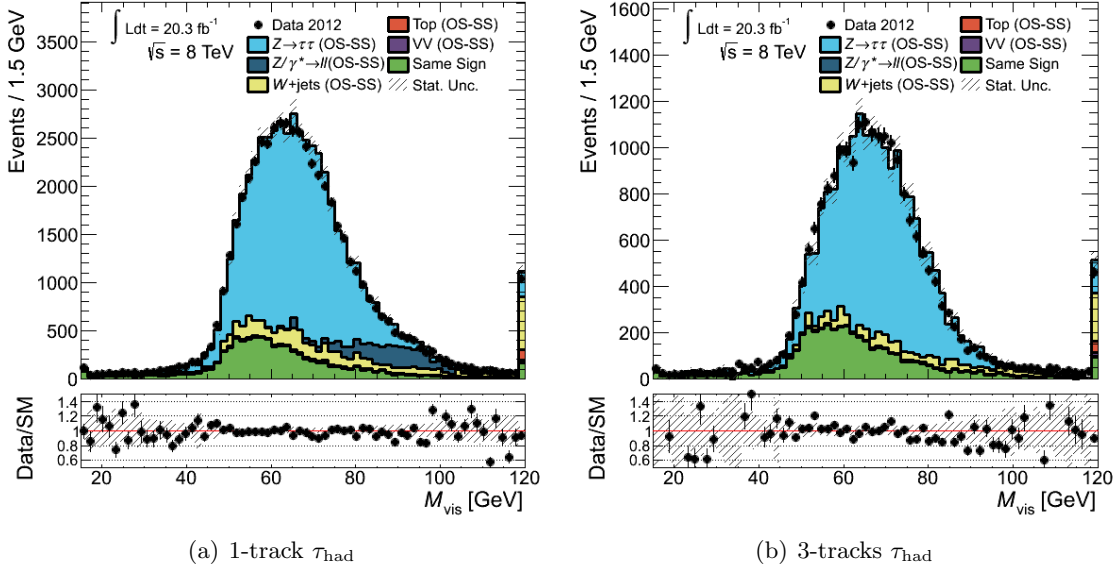
Figure 3.4: The M_{\text{vis}} distribution after the optimized selection for \tau_{\text{had}} with one (a) or three (b) associated tracks. Events in data (black dots) are compared to the expected stacked contributions from Z \rightarrow \tau^+\tau^- (light blue) and background processes determined as described in Section 3.3. Only statistical uncertainties are shown. Underflow and overflow events are added to the first and last bin, respectively. The lower panel shows the ratio of observed events in data to the sum of expected signal and background events.
