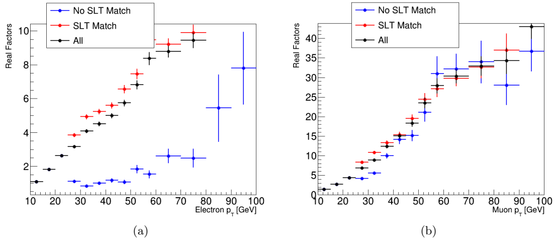
Figure C.7: Real factors r_\ell^{FF} as a function of the lepton p_T calculated on electrons (left) and muons (right) that activate the trigger (red), fail its activation (blue) and either activate it or not (black). The error bars account for the statistical uncertainty.
