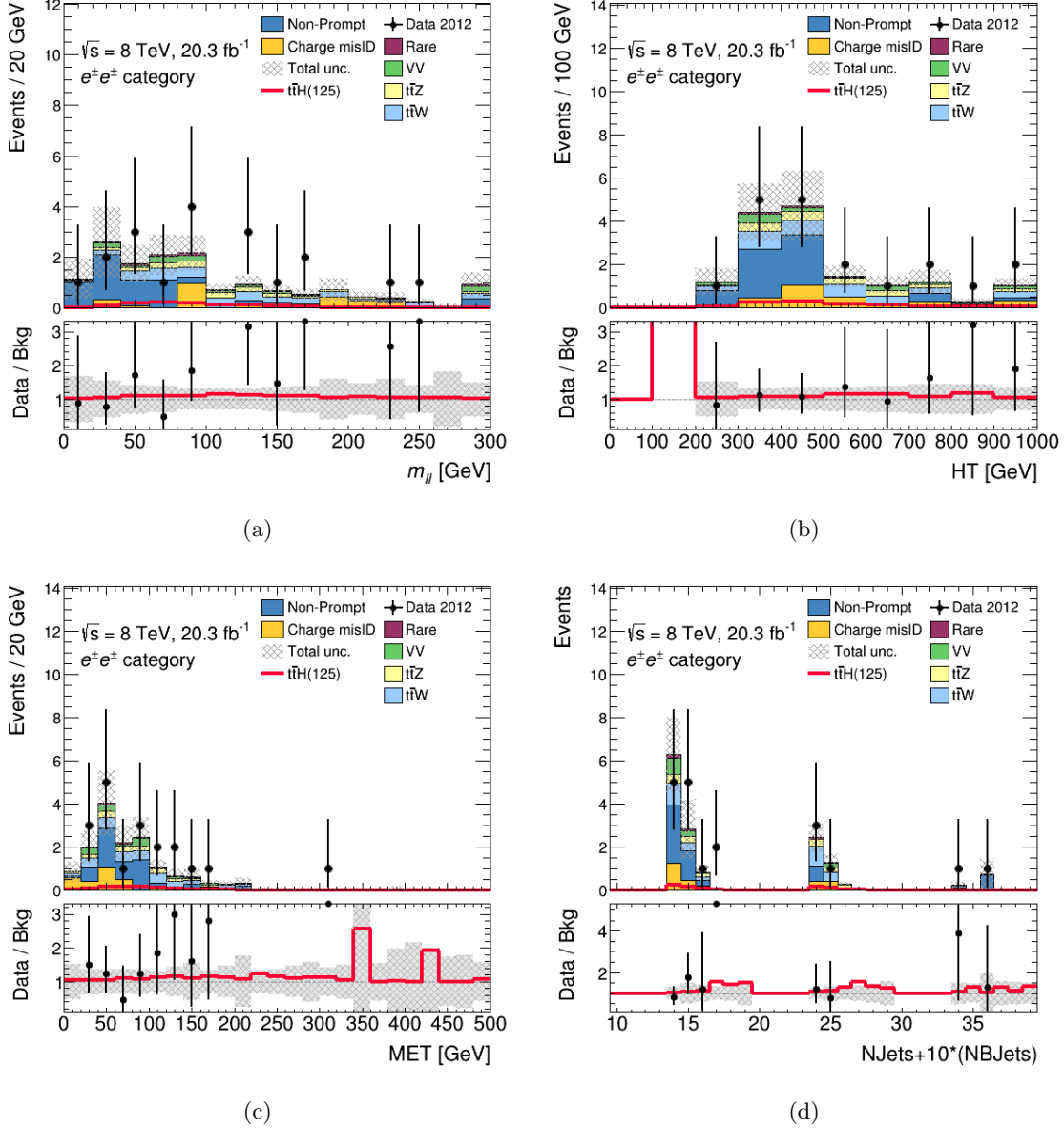
Figure C.24: Distributions of the di-lepton invariant mass (a), the H_T (b), the E_T^{miss} (c) and the combined jet and b -jet multiplicities (d) in the e^\pm e^\pm 2\ell 0\tau_{had} signal regions. In case of N(jet) > 9 events, these are accounted in the 9 + 10 \cdot N(b\text{-jet}) interval of the N(jet) + 10 \cdot N(b\text{-jet}) plot to avoid mixing with events with an additional b -jet. Events in data (black dots) are compared to the expected stacked contributions from Standard Model background processes. The expected signal contributions are overlaid to the backgrounds (red line). The lower panel shows the ratio of observed events in data to expected Standard Model events. The error bars on the data points show the statistical uncertainty and the dashed band shows the total uncertainties of the background predictions.
