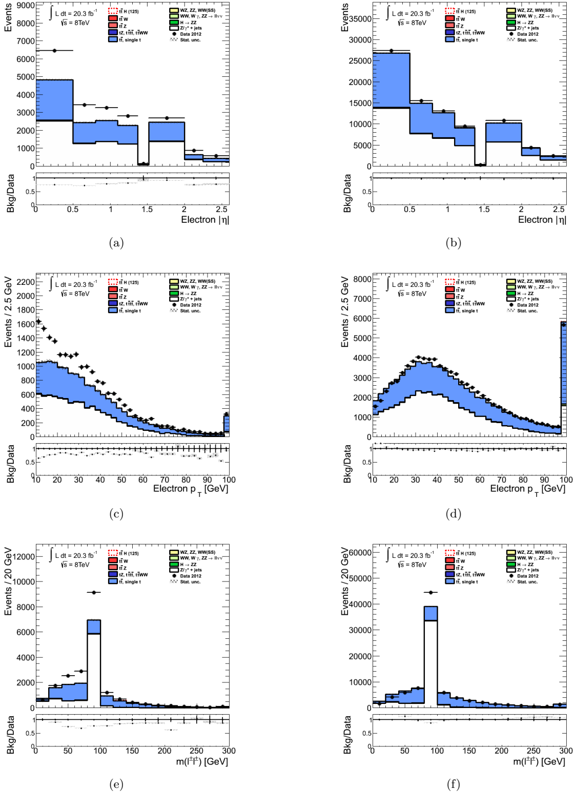
Figure C.4: Distributions of the electron |\eta| (top), the electron p_T (centre) and m(e^\pm, \ell^\mp) (bottom) in events with a loose electron passing (right) and failing (left) the tight selection in the prompt region. The plot shows the distribution of the invariant mass of the two opposite-sign leptons in the event. Events in data (black dots) are compared to the expected stacked contributions from prompt Standard Model processes. Overflow events are added to the last bin. The lower panel shows the ratio of observed events in data to expected Standard Model events. The error bars on the data points and the dashed band on the simulated background show the statistical uncertainties.
