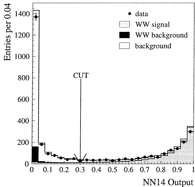
Figure 4.10: The output of the neural network, showing the discrimination between signal and background events.
