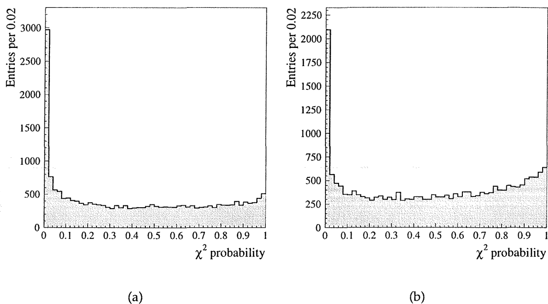
Figure 5.7: The \chi^2 probability distribution for (a) ABCFIT and (b) KINFIT for WW Monte Carlo events. These plots show a largely flat distribution, indicating that most events fit the kinematic fit hypothesis well. Roughly 10% of events fail the kinematic fit hypothesis in some way leading to large \chi^2 values and thus a peak at small values of \chi^2 probability.
