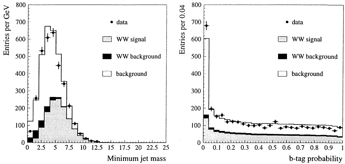
Figure 4.9: Neural network variables 13–14, (see text). The open histogram represents the total Monte Carlo expectation, the contribution from WW Monte Carlo is shaded. Data are shown as points.
