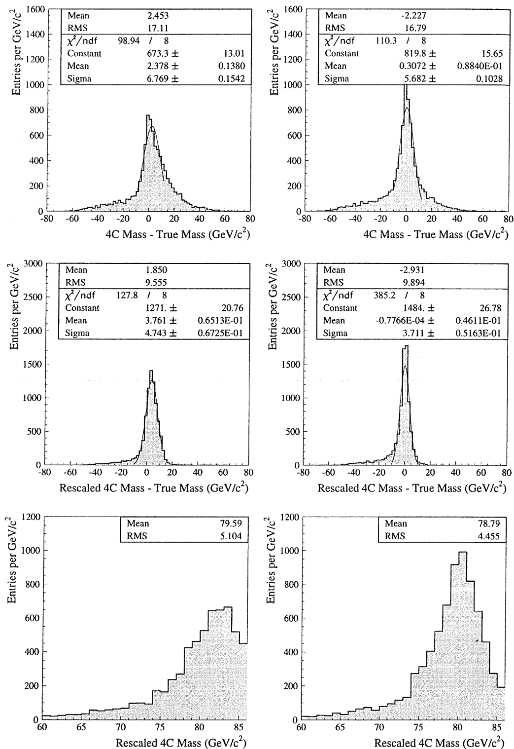
Figure 5.18: The mass resolution before (left hand plots) and after (right hand plots) selecting and removing ISR photons observed in the ALEPH detector, obtained from WW Monte Carlo events containing an ISR candidate photon. The top plots are the result of a 4C kinematic fit, the middle plots after rescaling, and the bottom plots the result of applying the jet pairing and mass window algorithm.
