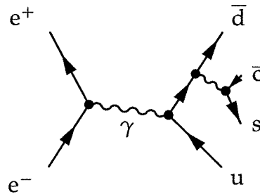
Figure 3.12: One of the CC11 diagrams of four-fermion production.
