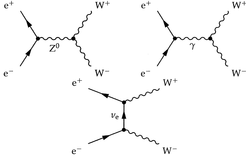
Figure 2.1: The CC03 diagrams of WW production. The top two diagrams are the annihilation diagrams while the third is the exchange diagram.
