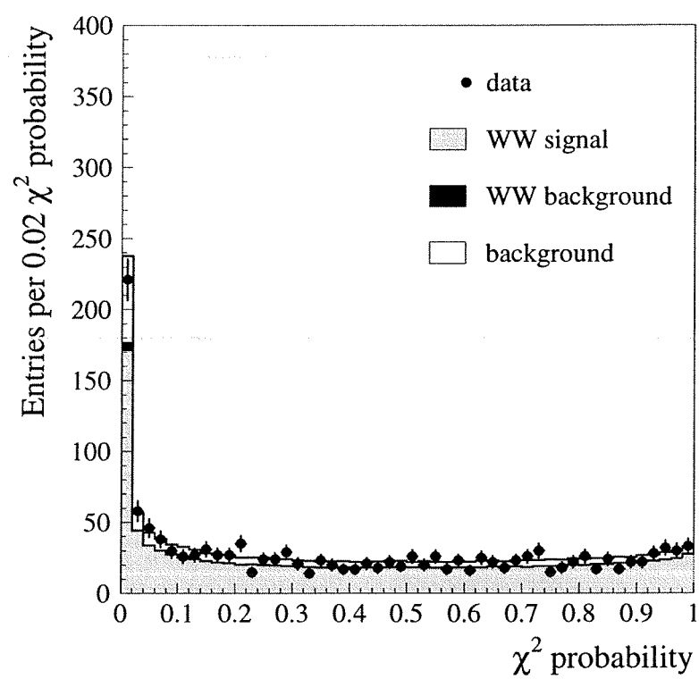
Figure 5.8: A comparison of the data and Monte Carlo distributions of the ABCFIT \chi^2 probability.
