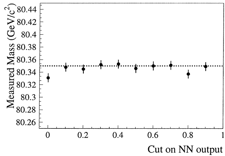
Figure 4.14: The measured W mass for a sample of Monte Carlo as a function of the cut on the neural network output. The true W mass is 80.35 \text{ GeV}/c^2 , as shown by the dotted line.
