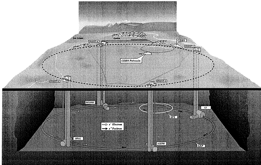
Figure 3.1: An overview of the LEP accelerator.
