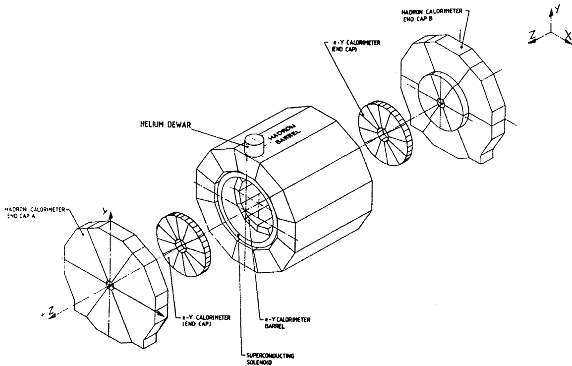
Figure 3.11: The ALEPH Hadron Calorimeter.
