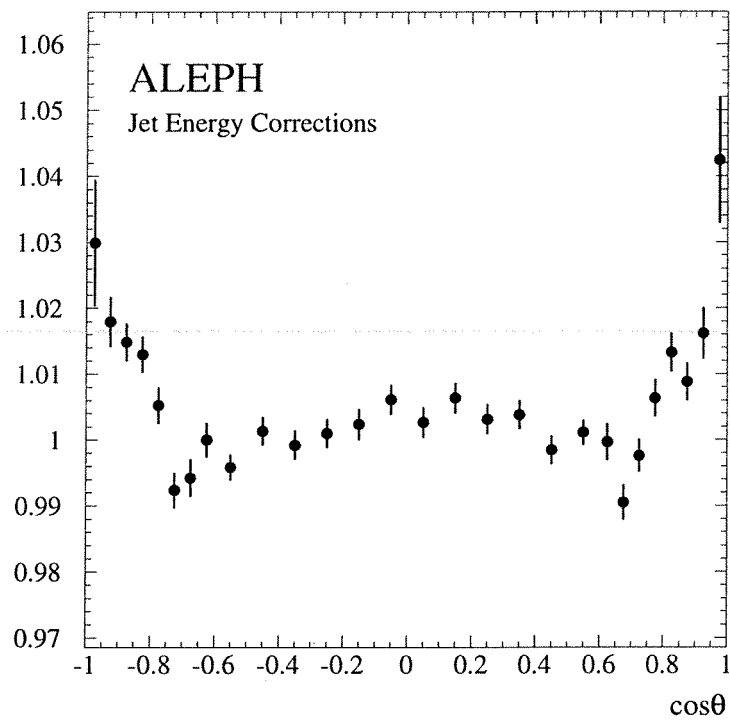
Figure 5.1: The ratio \frac{(E_{jet}/E_{beam})_{data}}{(E_{jet}/E_{beam})_{MC}} derived from 1998 Z^0 data and Monte Carlo as a function of jet polar angle, taken from Reference [74].
