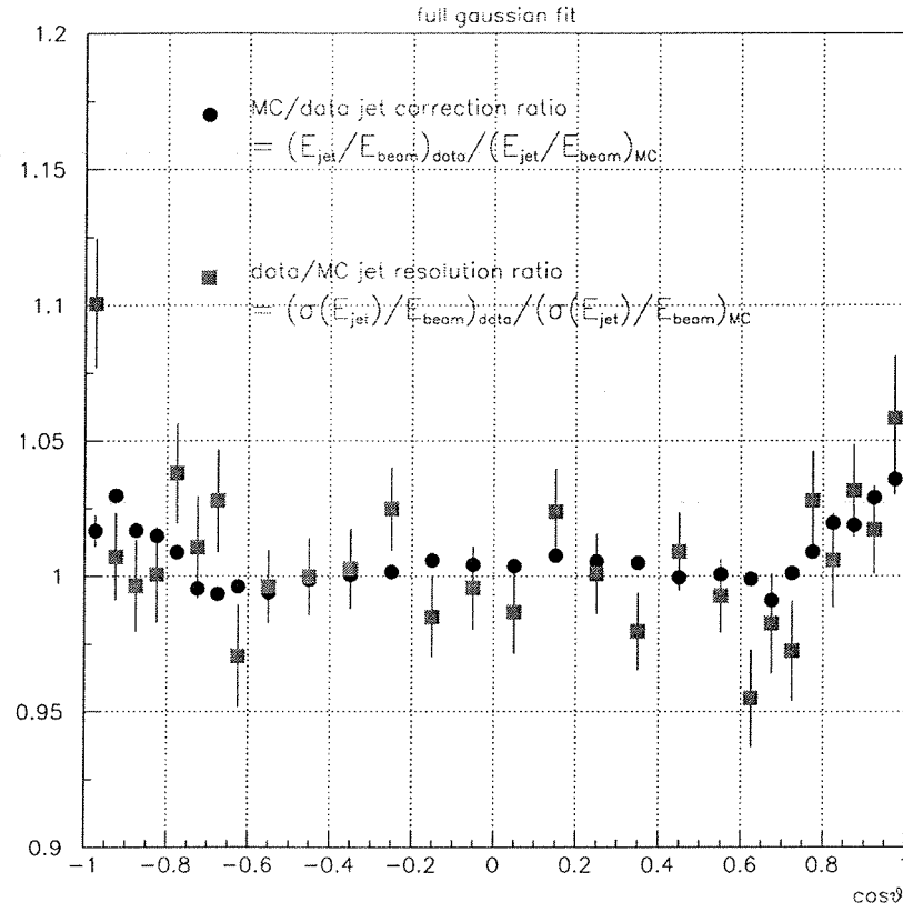
Figure 7.1: The ratios \frac{(E_{jet}/E_{beam})_{data}}{(E_{jet}/E_{beam})_{MC}} and \frac{(\sigma_{E_{jet}}/E_{beam})_{data}}{(\sigma_{E_{jet}}/E_{beam})_{MC}} as a function of polar angle.
