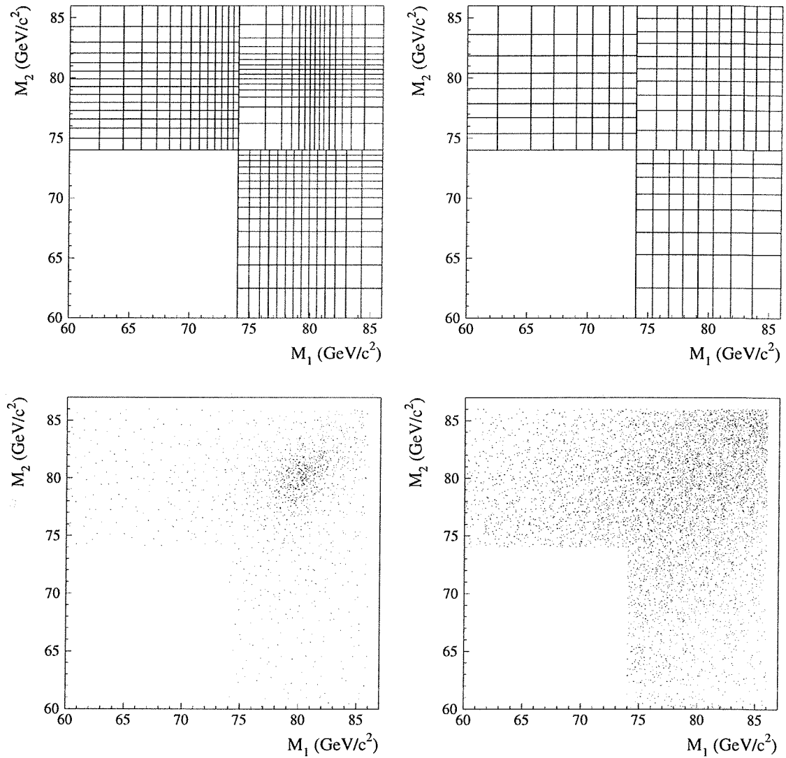
Figure 6.2: The top plots show the binning used for signal (left) and background (right). All bins contain more than the minimum of 200 entries. The bottom plots show the scatter plots of the Monte Carlo used to construct the probability density function for signal(left) and background(right).
