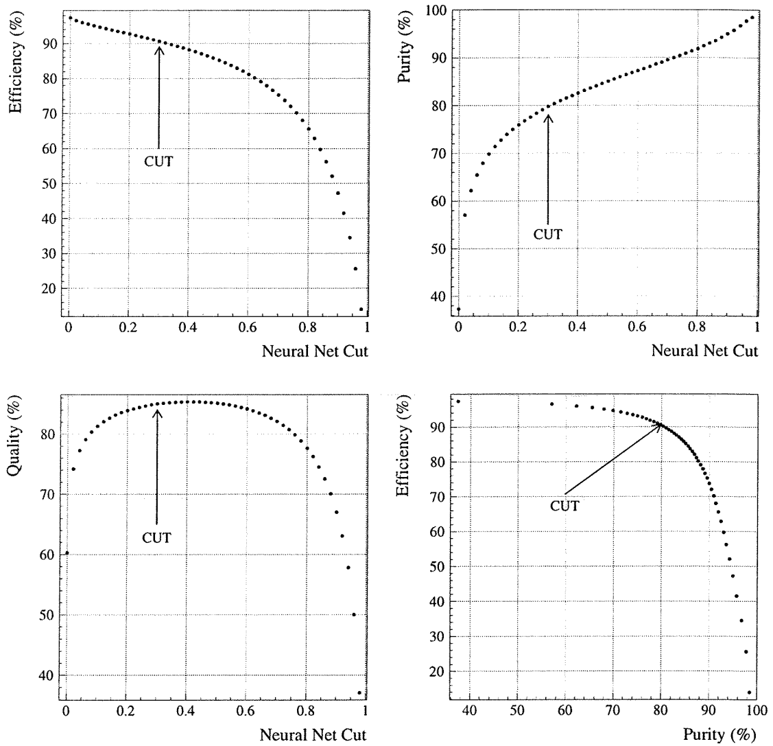
Figure 4.11: Efficiency, purity and quality of the neural network as a function of the cut on the output value. The final plot shows the efficiency as a function of the purity. The selection criteria used in the analysis is indicated by the arrow in each plot.
