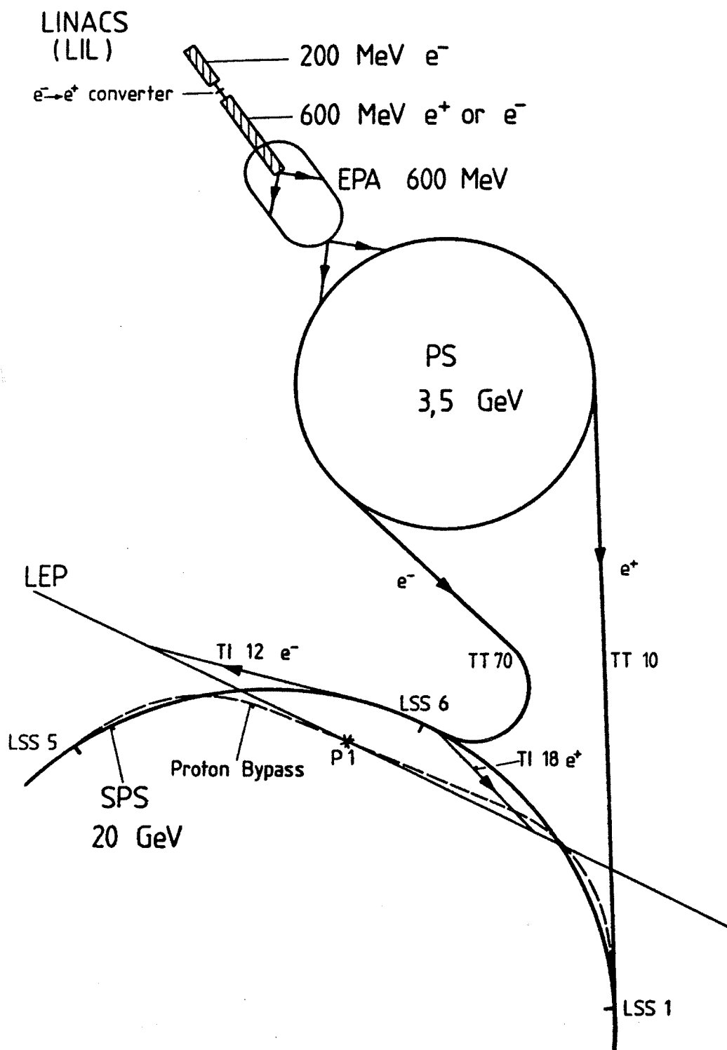
Figure 3.2: The LEP injection scheme.
