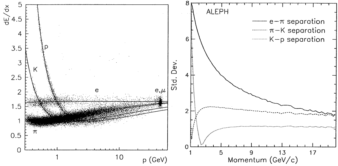
Figure 3.9: The left figure shows the measured dE/dx versus particle momentum for a sample of about 40,000 tracks. Each track was required to have at least 150 dE/dx measurements. The fitted parametrisation is shown for electrons, muons, pions, kaons and protons. The right figure shows the average dE/dx separation in standard deviations between different particle types as a function of momentum. This has been computed using all tracks in hadronic Z^0 decays having at least 50 dE/dx measurements. Taken from Reference [48].
