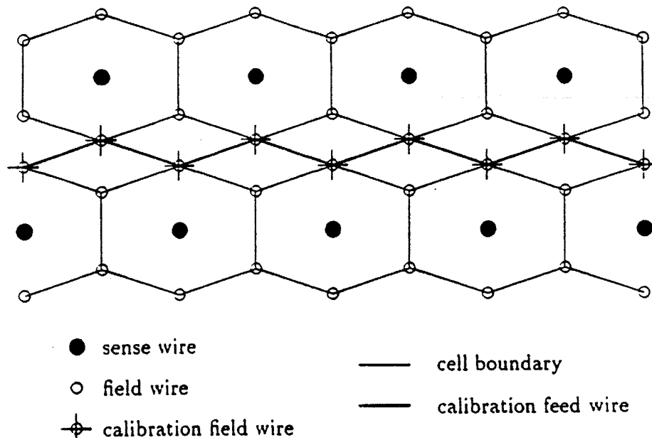
Figure 3.6: The ITC cell structure.
