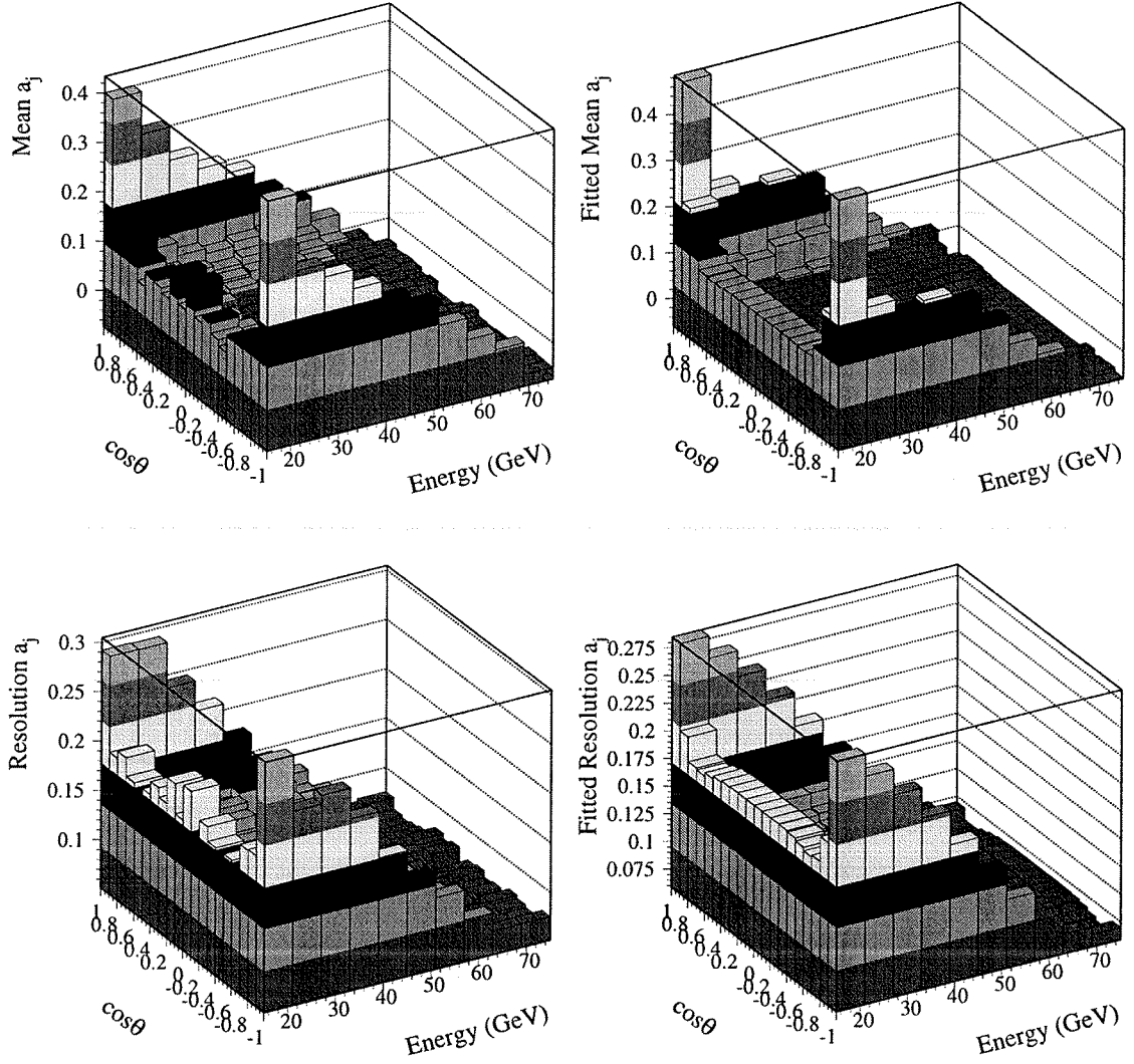
Figure 5.5: Distributions of the measured and fitted mean and resolution of the ABCFIT correction factor a_j .
