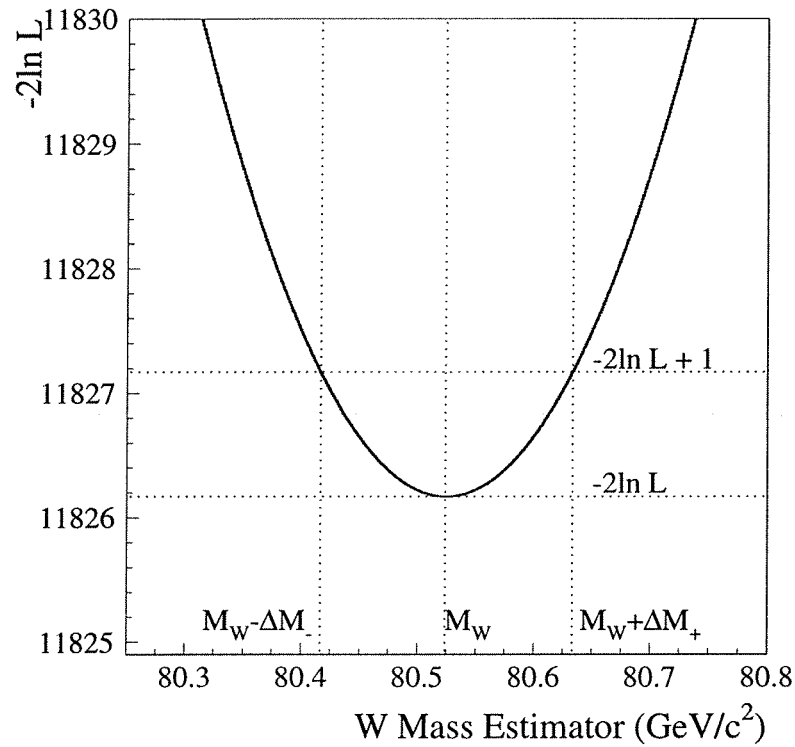
Figure 6.3: The quantity -2 \ln \mathcal{L} (see text) as a function of the W mass. The fitted mass is given by the minimum of this quantity. The parabolic behaviour of the likelihood is clearly shown.
