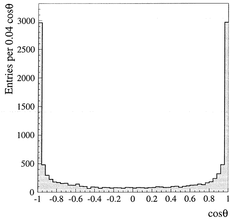
Figure 5.16: The angular distribution of ISR photons produced within the ALEPH angular acceptance in WW Monte Carlo events selected as fully hadronic candidates.
