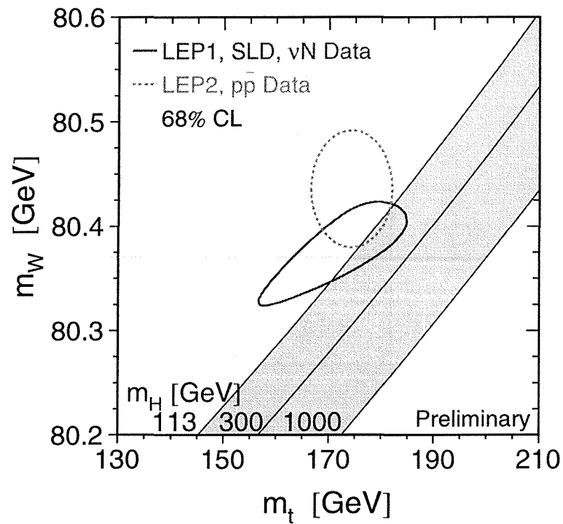
Figure 8.5: Comparison of direct (dashed line) and indirect (solid line) W mass measurements. Also shown are the predictions for a range of Higgs boson masses as a function of the W mass and top quark mass.
