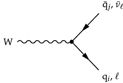
Figure 2.3: W boson decay into quark-antiquark, q_i \bar{q}_j , (where the subscripts i, j denote different quark flavours) or lepton antineutrino, \ell \bar{\nu}_\ell .
