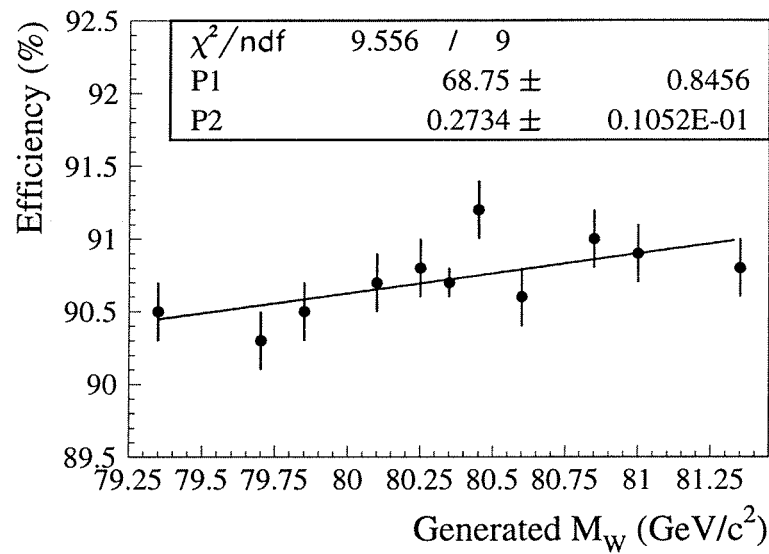
Figure 4.13: The neural network efficiency as a function of W mass value input to the Monte Carlo. Little dependence on the W mass is seen. The parameters P1 and P2 are the offset and slope of a straight line fit to the data in the plot. The \chi^2/\text{ndf} of the fit is also given.
