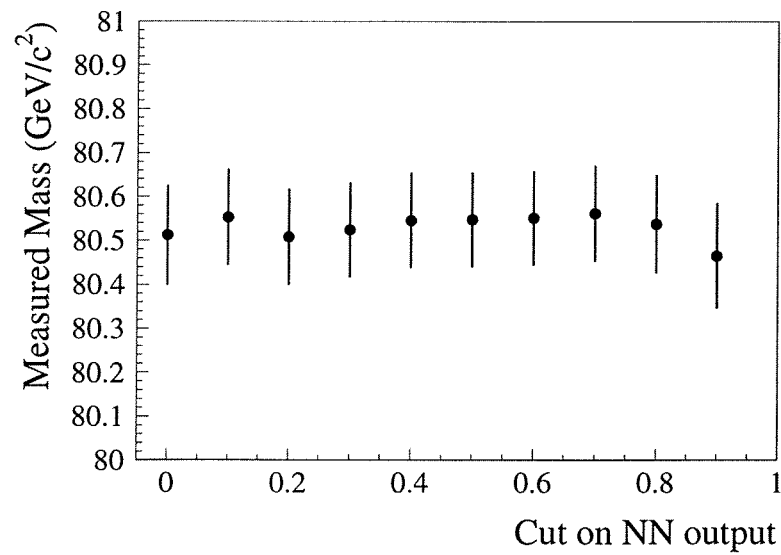
Figure 6.6: The measured W mass as a function of the cut on the neural network output.
