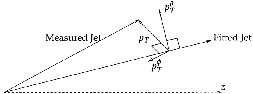
Figure 5.3: The parameters p_T^\theta and p_T^\phi .
