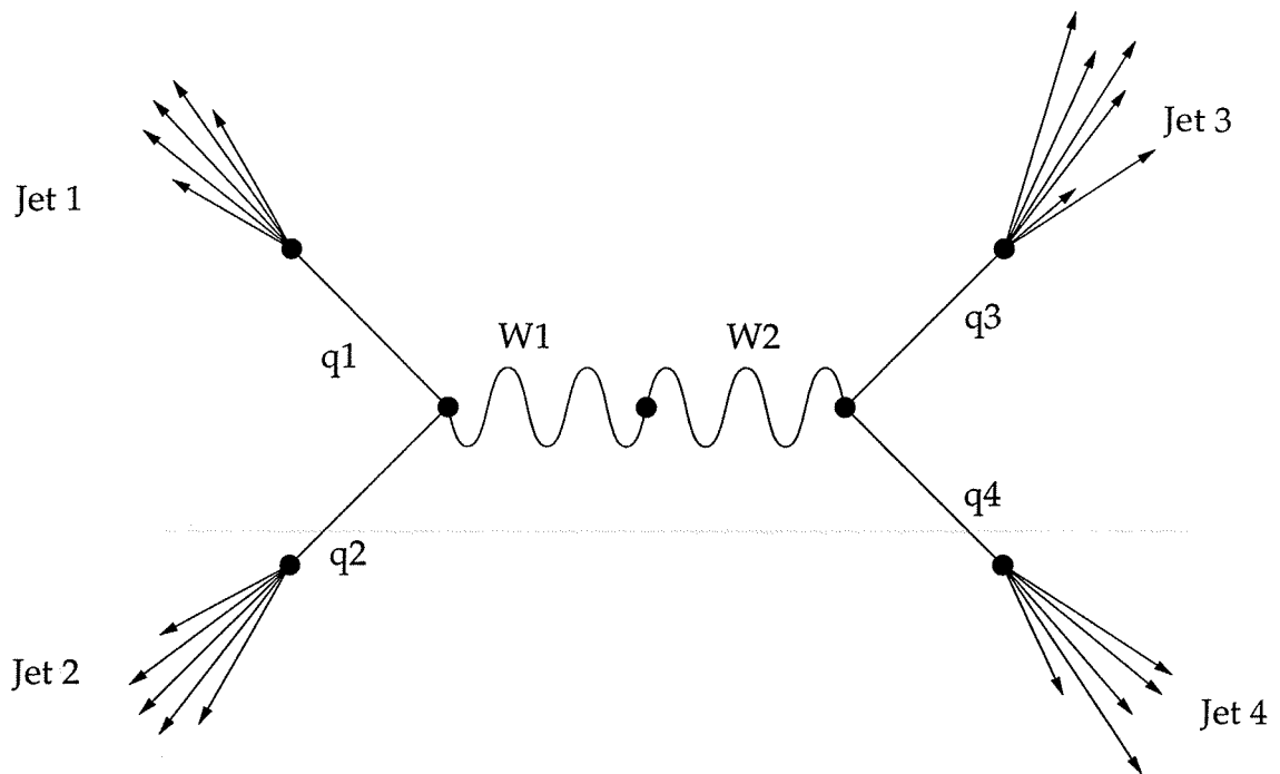
Figure 4.1: A schematic fully hadronic event.
