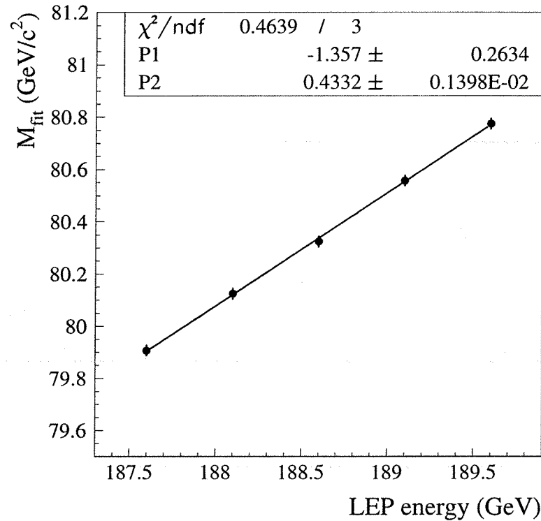
Figure 7.3: The fitted W mass as a function of the LEP centre of mass energy (points). The result of a straight line fit to the points with slope P2 and offset P1 is shown on the plot as the solid line.
