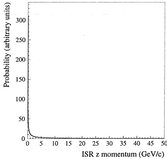
Figure 5.12: The ISR probability distribution as a function of ISR z momentum.
