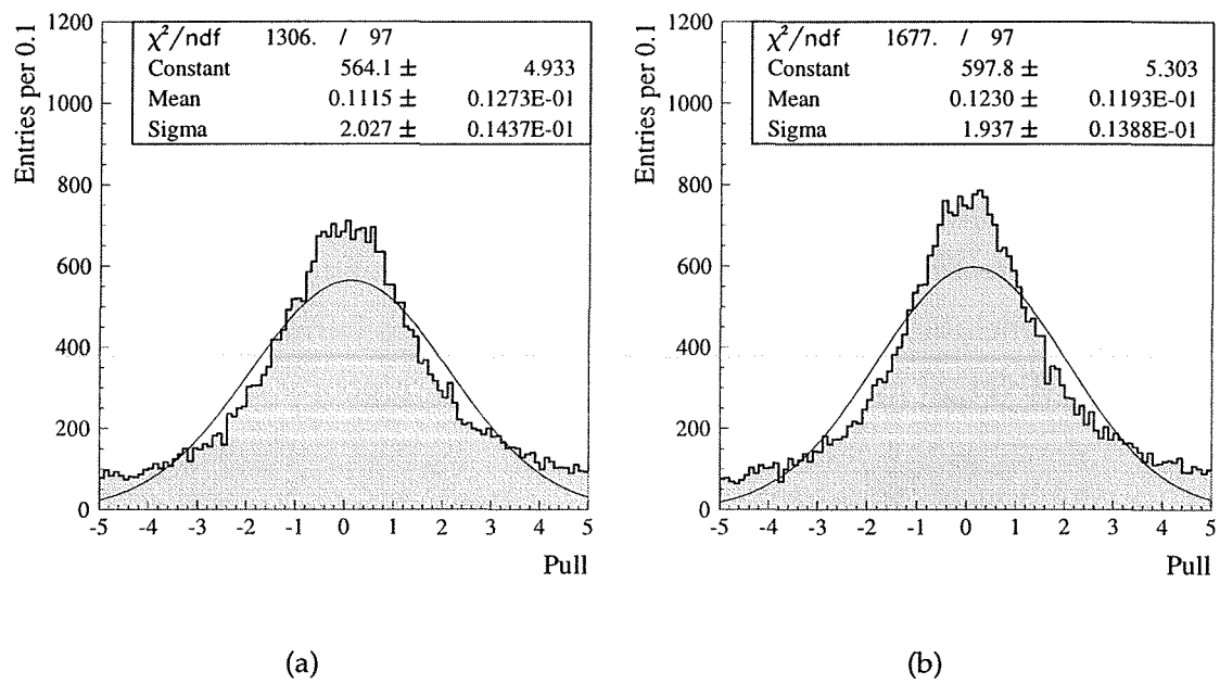
Figure 5.9: The pull distributions for (a) ABCFIT and (b) KINFIT. This distribution should be a Gaussian of unit width with a mean of zero. It is clear that this is not the case, indicating that the errors on the fitted dijet masses are not properly understood.
