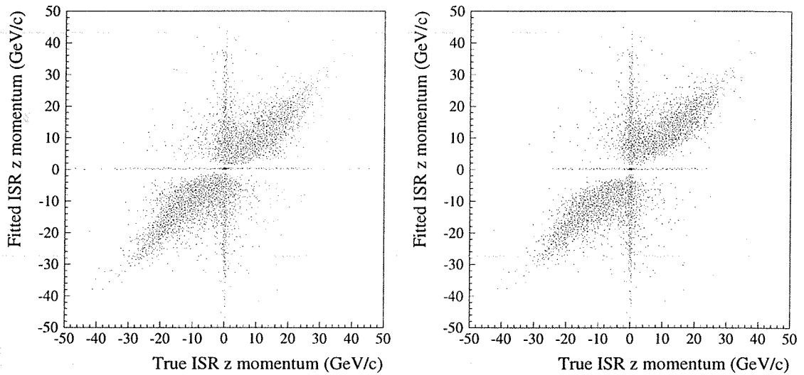
Figure 5.14: The fitted ISR z momentum plotted against the true ISR z momentum, obtained using WW Monte Carlo events. The left hand plot is for all selected events, the right hand plot just those with a bad 4C kinematic fit \chi^2 probability.
