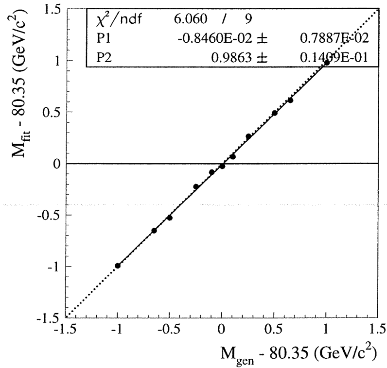
Figure 6.5: The fitted W mass, M_{\text{fit}} , versus the generated W mass M_{\text{gen}} (relative to the reference mass of 80.35 \text{ GeV}/c^2 ) for eleven different Monte Carlo samples (points). The result of a straight line fit to the points is shown as a solid line and the values of the slope, P2, and offset, P1, are given in the plot together with the \chi^2 of the fit. The dotted line has slope 1 and offset 0.
