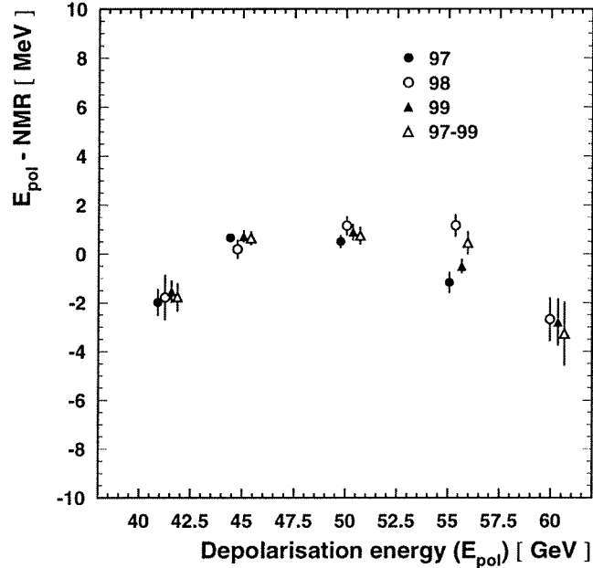
Figure 3.3: Comparison of NMR and RDP measurements, taken from [45].
