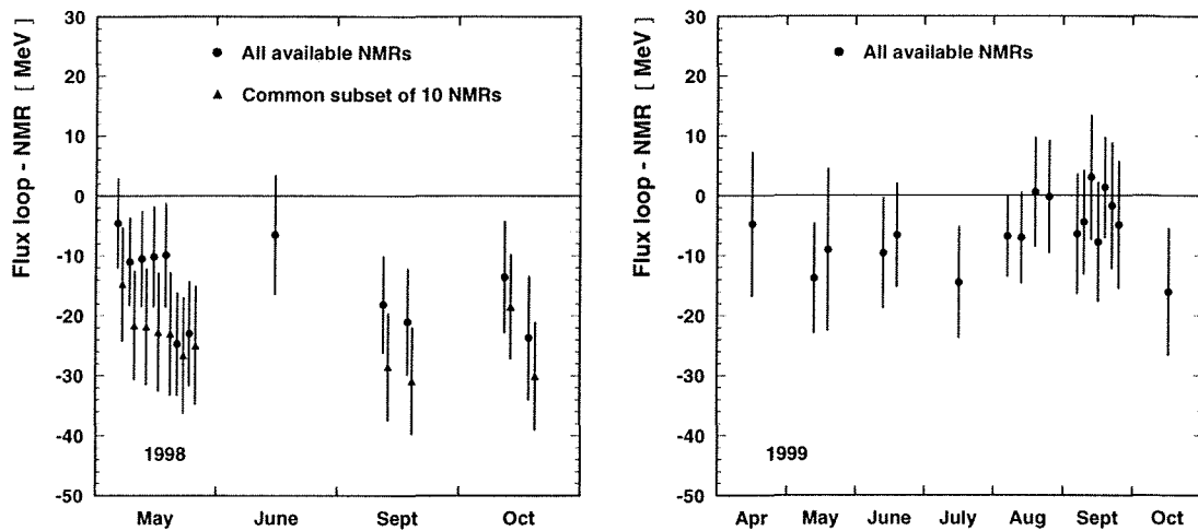
Figure 3.4: Comparison of flux loop and NMR measurements, taken from [45].
