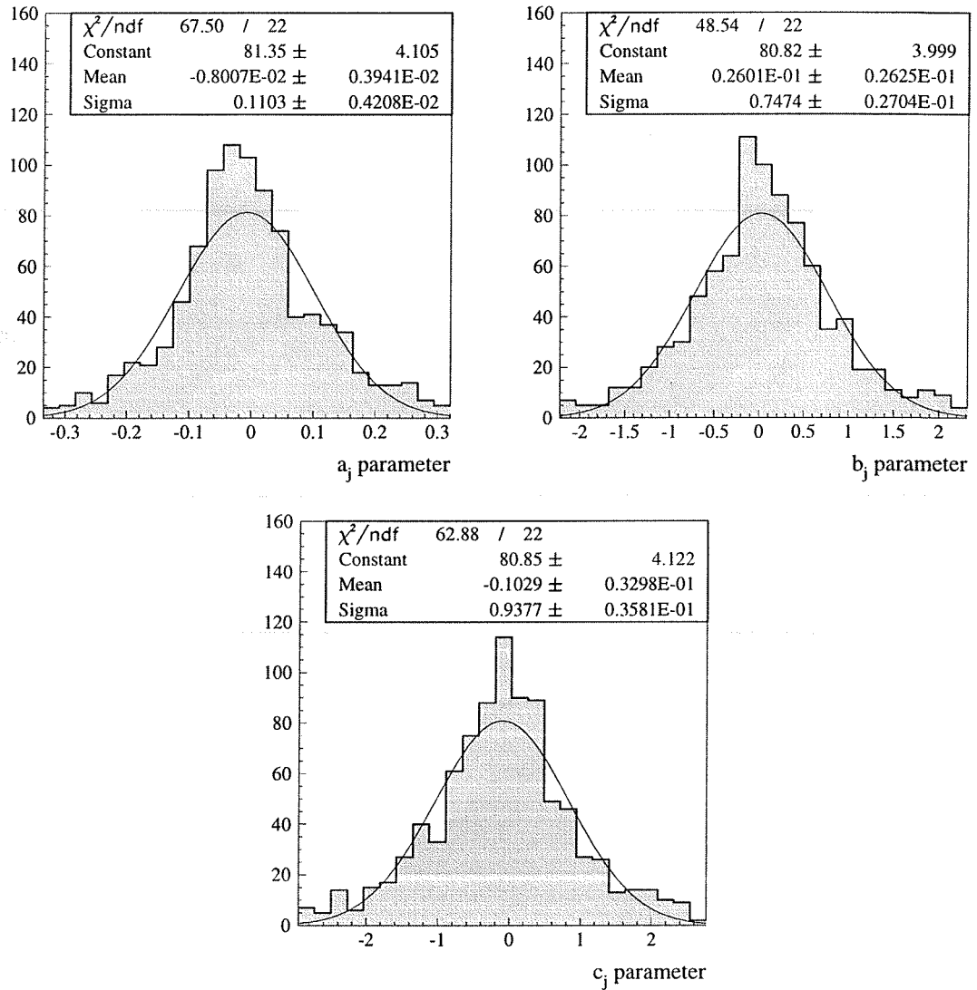
Figure 5.4: Distributions of the ABCFIT parameters a_j , b_j and c_j for jets in the range 45 \text{ GeV} < E < 51 \text{ GeV} , 0.0 < \cos \theta < 0.1 , together with fitted Gaussian distributions. The \chi^2 of the fit is shown together with the mean and resolution.
