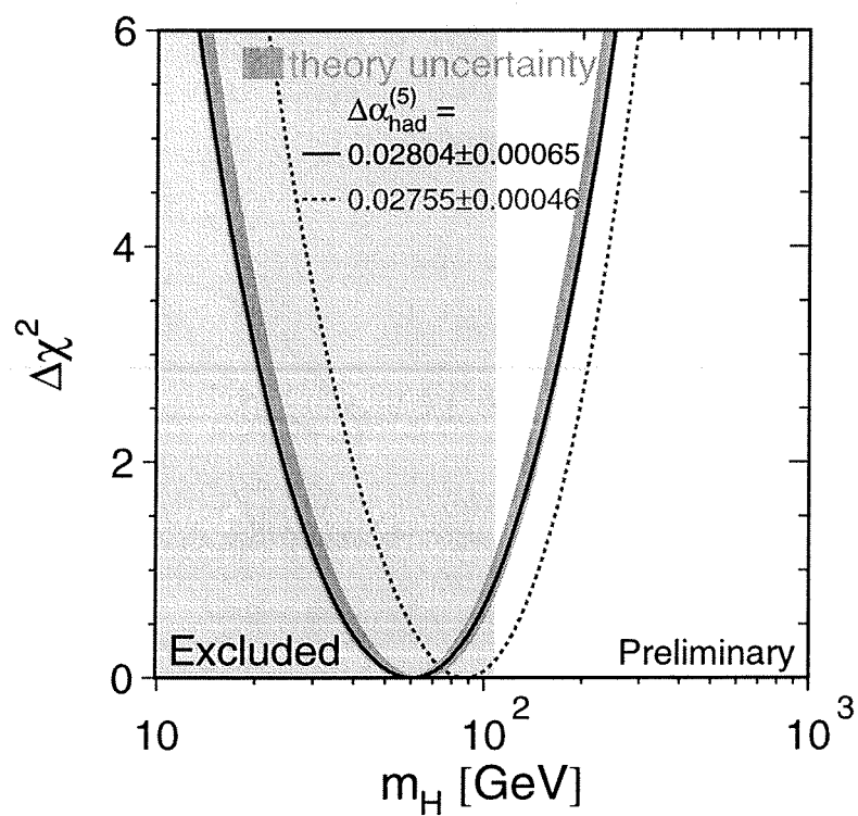
Figure 8.6: The change in \chi^2 as a function of the Higgs mass (see text).
