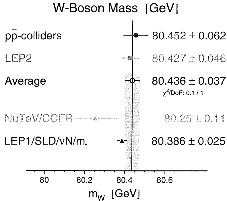
Figure 8.4: The world average W mass at the time of the 2000 summer conferences. The value labelled p\bar{p} -collider is the average hadron collider W mass measurement from Equation 8.6 and that labelled LEP2 is the LEP average measurement from Equation 8.4. Also shown are the measurements obtained from neutrino-nucleon scattering experiments NuTeV and CCFR and the indirect measurement (labelled LEP1/SLD/ \nu N/m_t ) obtained from a global fit to electroweak data as described in the text.
