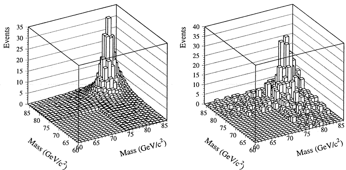
Figure 5.21: The two dimensional reconstructed mass distributions for Monte Carlo (left) and data (right). The statistical fluctuations in the data sample are clear.
