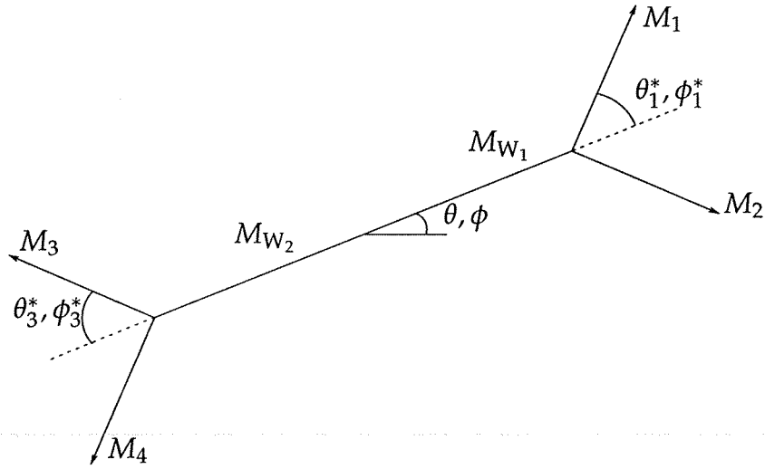
Figure 5.2: Variables describing W pair decay.
