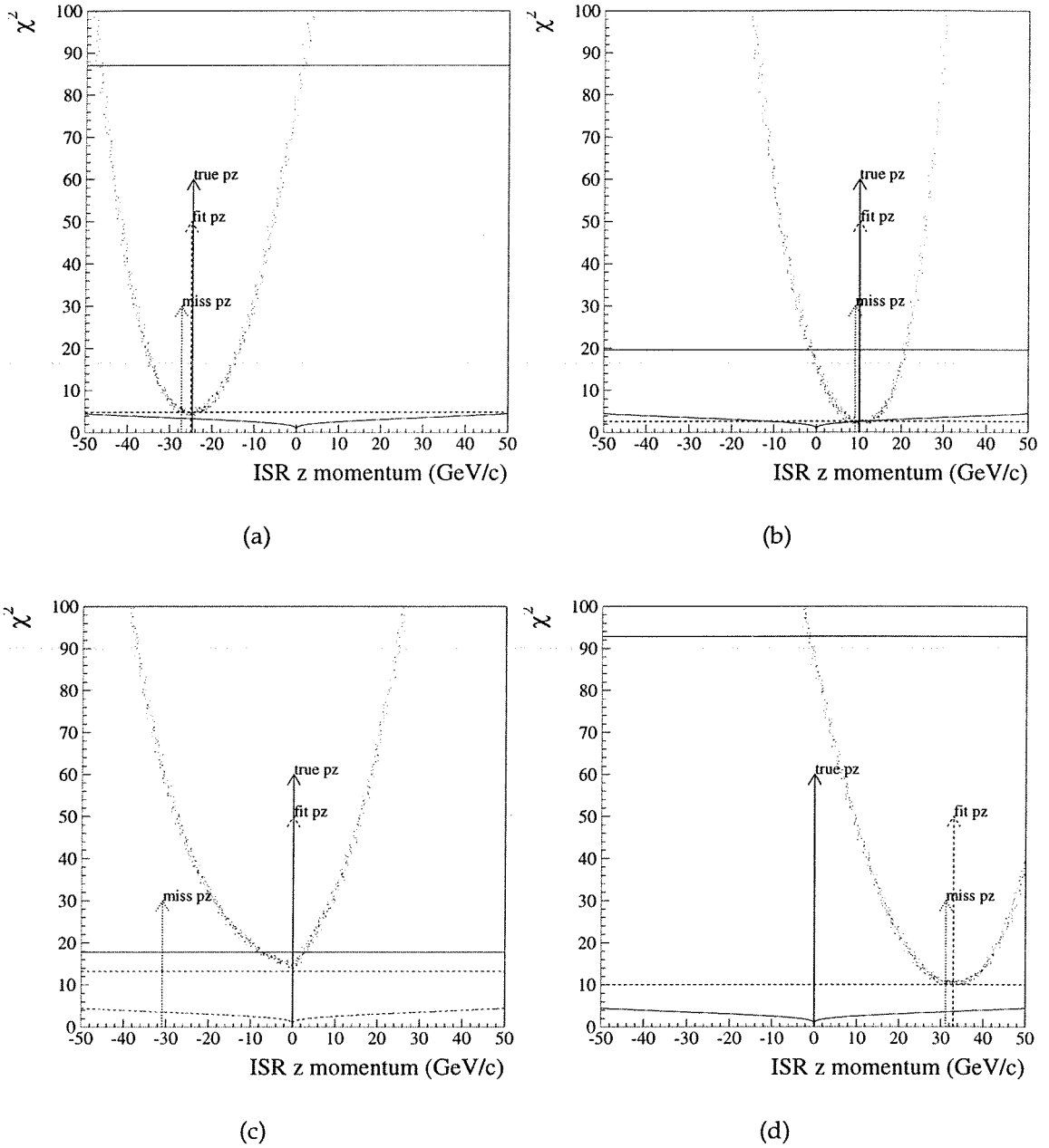
Figure 5.13: Examples of including the ISR hypothesis in the kinematic fit for four different events. The plot shows the values of the likelihood type function which is minimised. The arrows show the true ISR z momentum, the fitted ISR z momentum and the overall missing z momentum in the event. Figures (a), (b) and (c) show good fits where the fitted z momentum is a reasonable representation of the true z momentum. Figure (d) shows an example of an event in which the fitted momentum is the missing z momentum rather than the true ISR z momentum.
