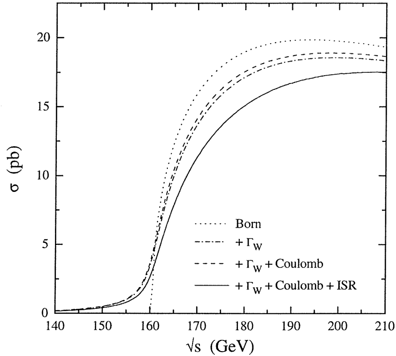
Figure 2.2: The cross section for e^+e^- \rightarrow W^+W^- as a function of centre of mass energy, \sqrt{s} , in various approximations:
