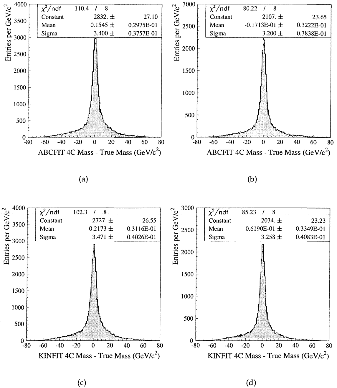
Figure 5.6: The difference between the dijet mass after kinematic fitting and the true W mass. Figures (a) and (b) show the results after ABCFIT, Figures (c) and (d) the results of KINFIT. Figures (a) and (c) are obtained using all WW Monte Carlo events selected as hadronic candidates. The positive bias due to initial state radiation is shown by the results of the fit to the peak position. Figures (b) and (d) are obtained using just those events with an ISR energy of less than 0.5 GeV. The bias in the mass is much smaller.
