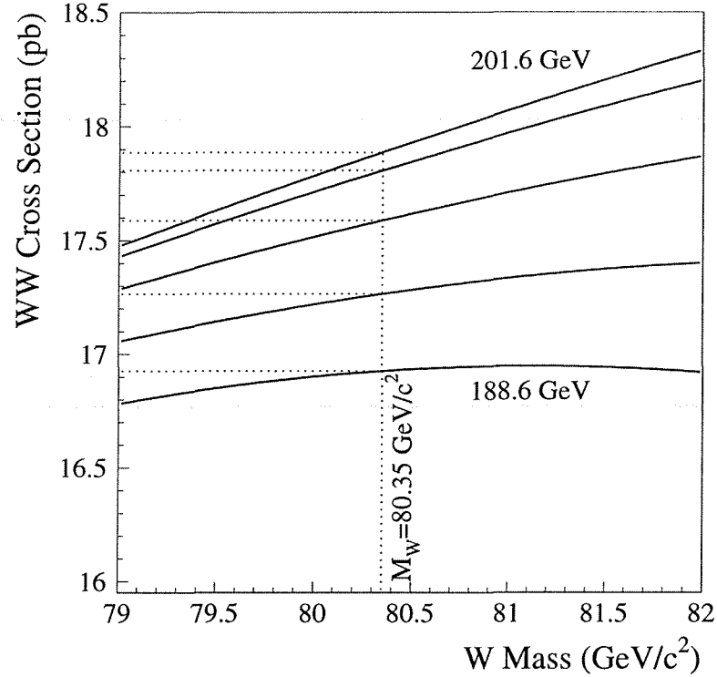
Figure 6.1: The parametrisation of the WW cross section as a function of the W mass, for centre of mass energies between 188.6 GeV (bottom curve) and 201.6 GeV (top curve).
