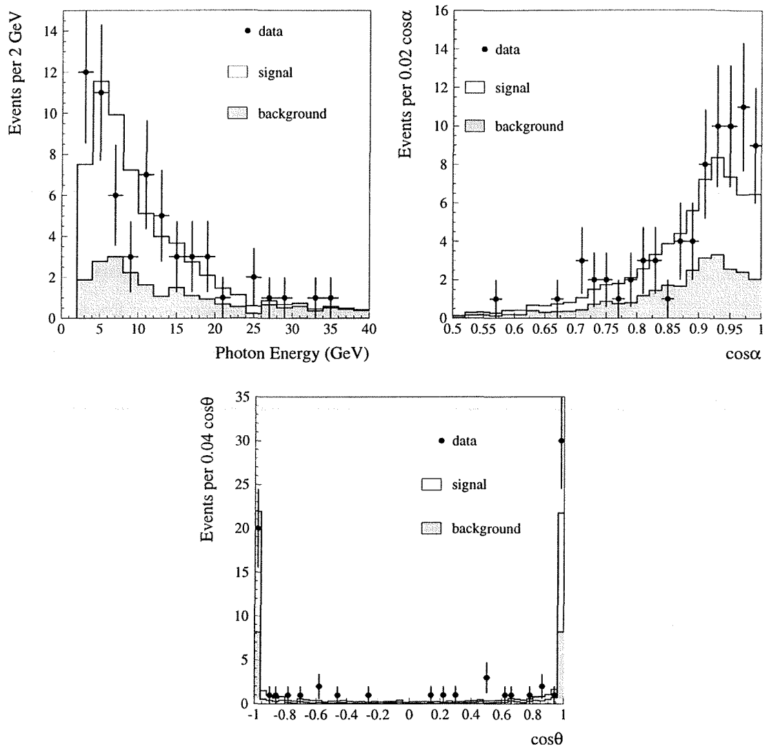
Figure 5.19: The comparison between data and Monte Carlo simulation for the ISR photon energy, angular separation, \cos \alpha , and angular distribution, \cos \theta , for hadronic WW candidate events containing an ISR candidate photon. The Monte Carlo distributions are represented by the histograms and are separated into signal, ie true WW events, and background, non WW events.
