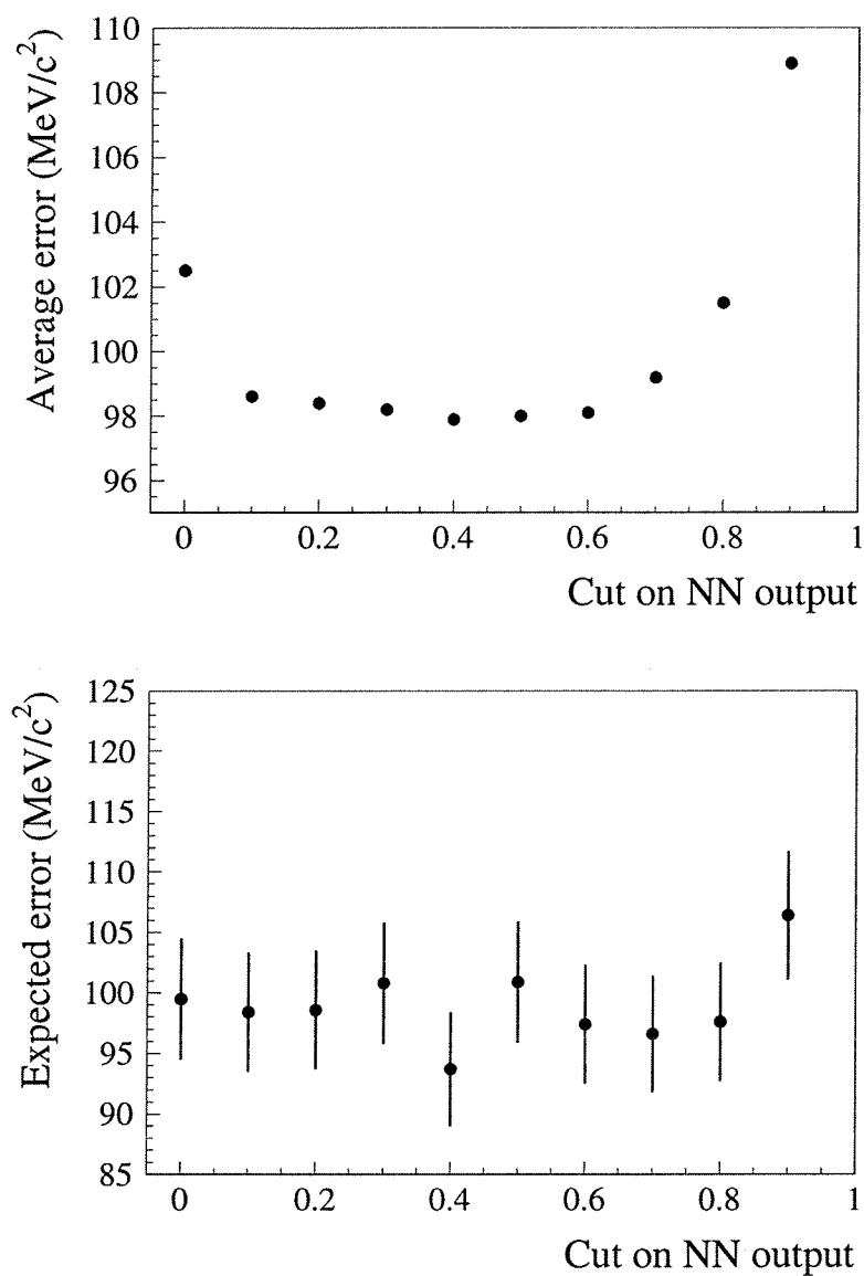
Figure 4.12: The expected statistical uncertainty on M_W as a function of the cut on the neural network output. The top plot is the average W mass error for 200 Monte Carlo samples the same size as the data, the bottom plot is the r.m.s. of the mass distribution for the same samples.
