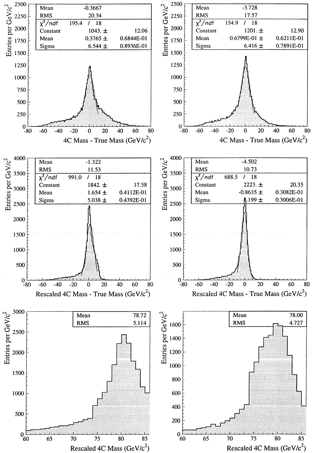
Figure 5.15: The mass resolution before (left hand plots) and after (right hand plots) accounting for collinear ISR in the kinematic fit for selected WW Monte Carlo events with \mathcal{P}(\chi^2) < 0.01 . The top plots are the result of a 4C kinematic fit, the middle plots after rescaling, and the bottom plots the result of applying the jet pairing and mass window algorithm.
