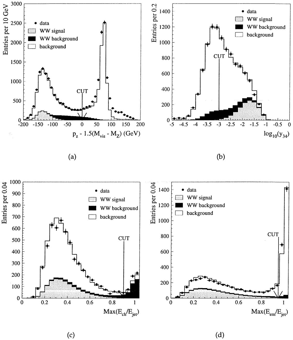
Figure 4.3: The preselection variables (see text) for the \sqrt{s} = 188.6 GeV data and Monte Carlo.
