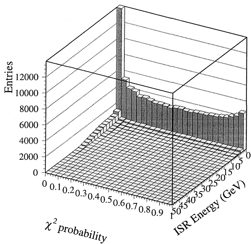
Figure 5.11: The ABCFIT kinematic fit \chi^2 probability as a function of the energy lost through initial state radiation. Events where a large amount of energy has been lost are more likely to fail the kinematic fit.
