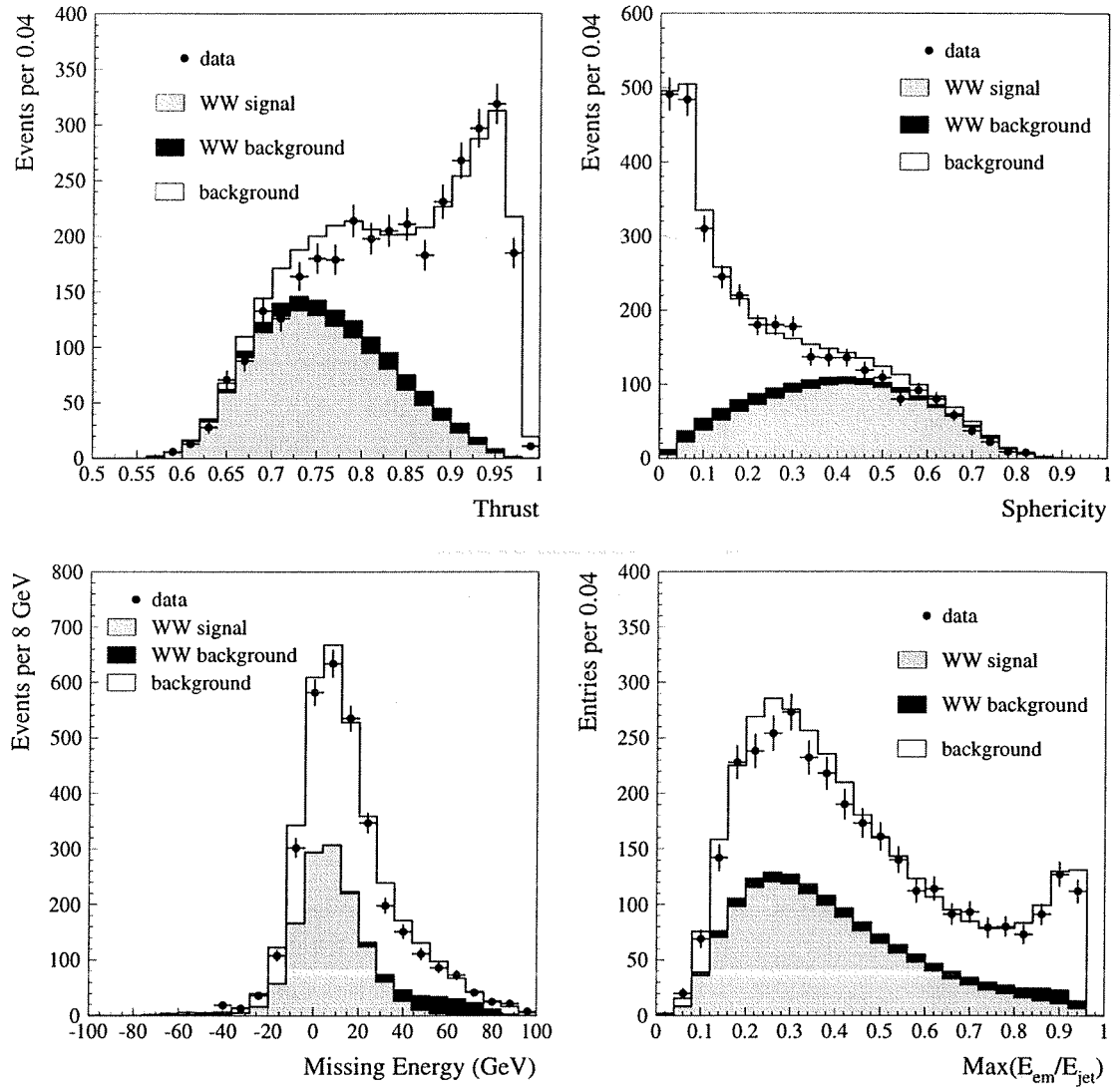
Figure 4.6: Neural network variables 1–4, (see text). The open histogram represents the total Monte Carlo expectation, the contribution from WW Monte Carlo is shaded. Data are shown as points.
