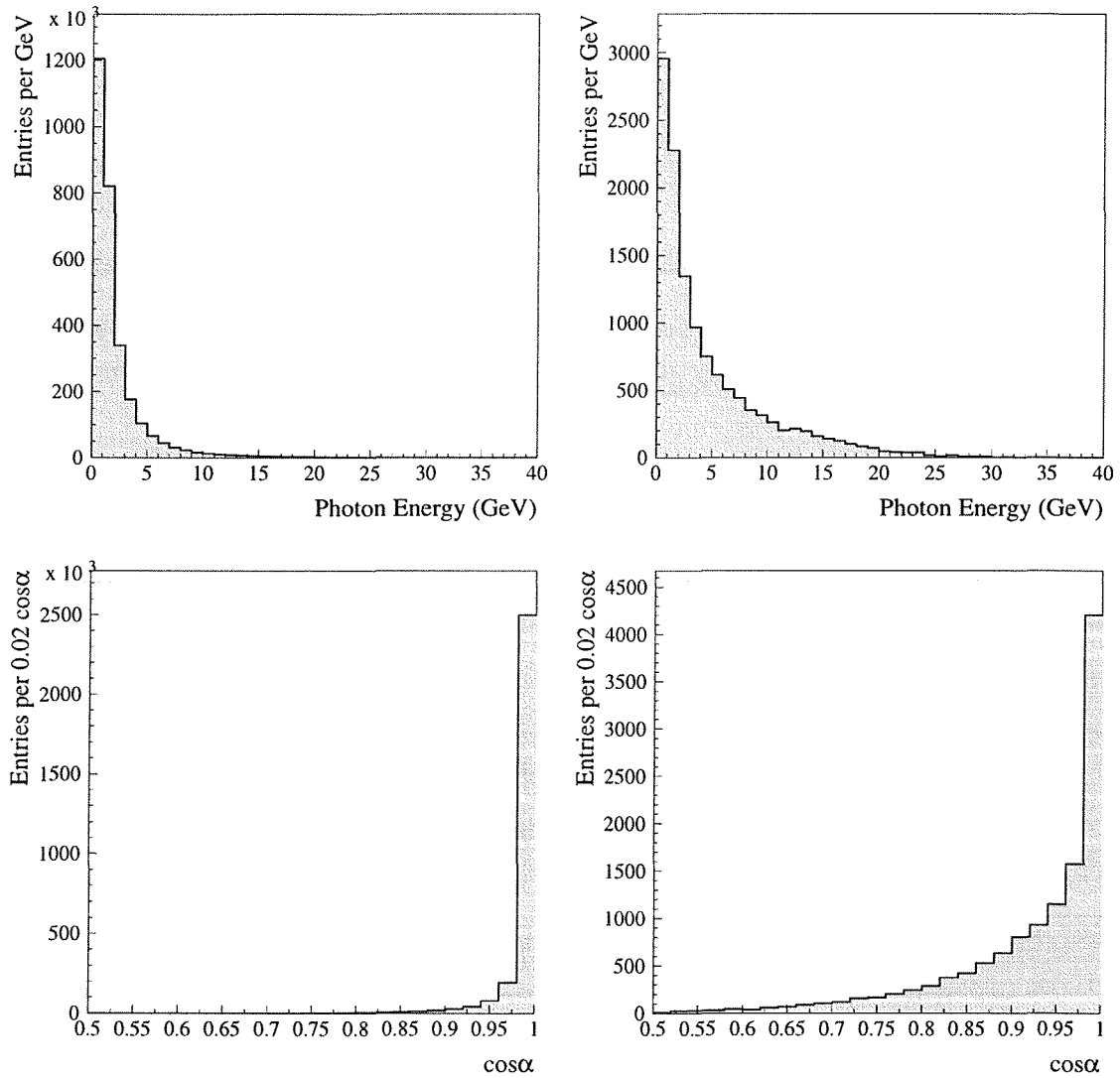
Figure 5.17: The energy and isolation angle distributions of all photons (left) and ISR photons (right) in WW Monte Carlo events selected as fully hadronic candidates. It can be seen that a greater proportion of ISR photons have a high energy and larger isolation angle than for hadronisation photons. The difference in the scales of the y-axes should be noted
