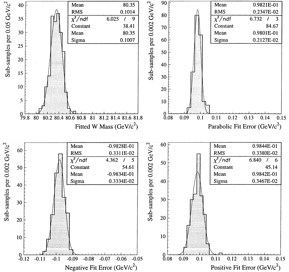
Figure 6.4: Fitted W mass and fit errors from 200 subsamples of Monte Carlo (see text). The fitted mass is shown in the top left plot. The other plots show the distributions of the positive and negative statistical uncertainty, and the parabolic uncertainty.
