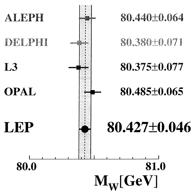
Figure 8.3: The LEP average W mass at the time of the 2000 summer conferences.
