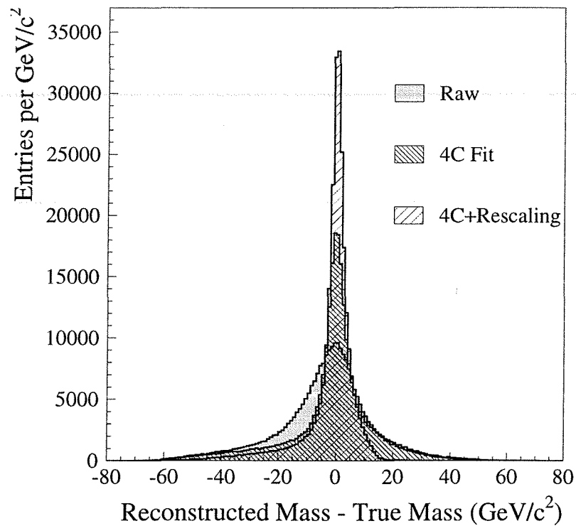
Figure 5.10: The reconstructed dijet mass resolution for measured jets, after a 4C kinematic fit and after rescaling with the beam energy.
