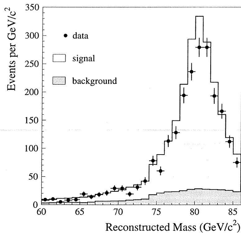
Figure 5.20: The reconstructed mass distribution for the \sqrt{s} = 188.6 GeV data and Monte Carlo. The WW Monte Carlo has been generated with an input mass of 80.35 \text{ GeV}/c^2 . The Monte Carlo distributions are represented by the histograms and are separated into signal, ie true hadronic WW events, and background, all other events.
