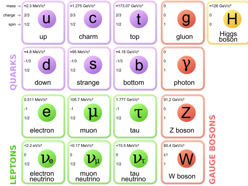
Figure 2.1: Standard Model particles [7]
