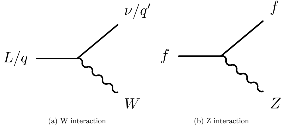
Figure 2.5: Weak interactions.
