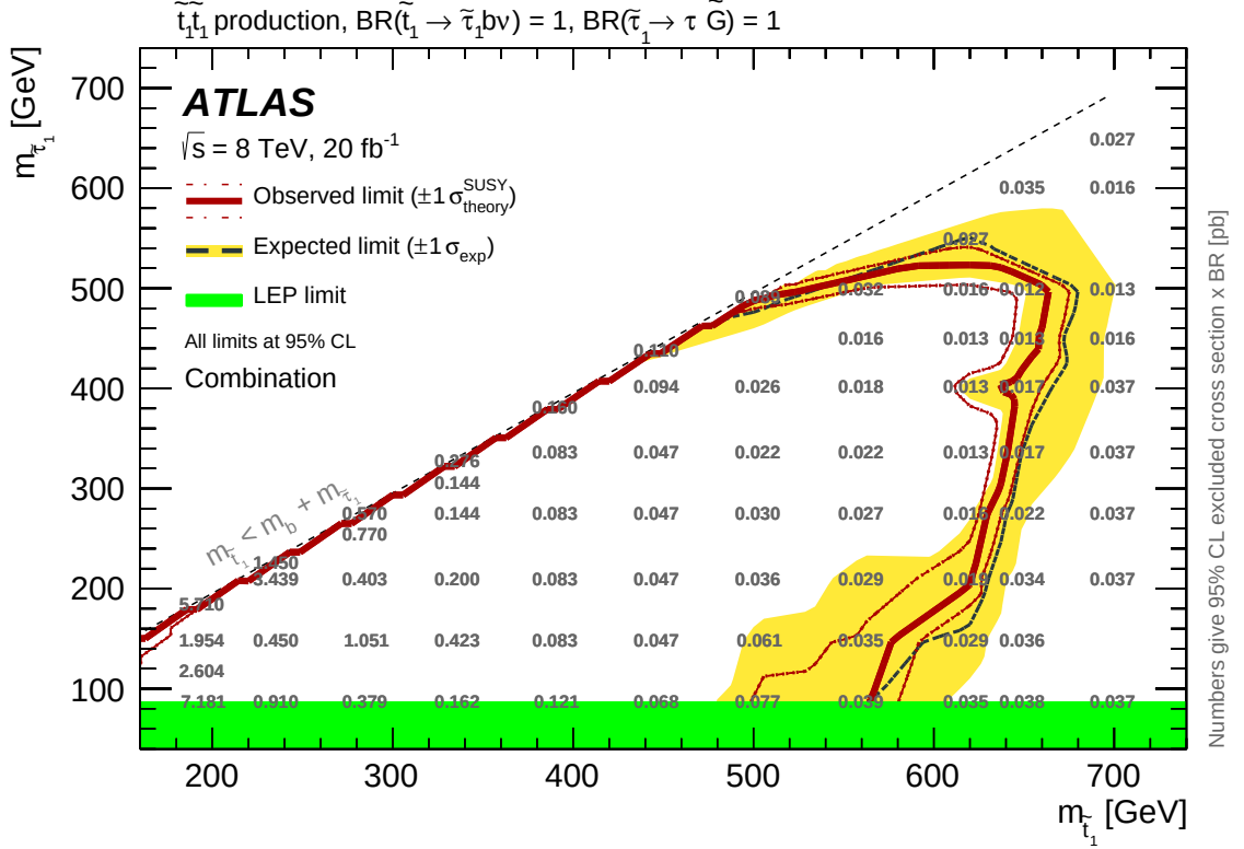
Figure 9.7: Observed and expected exclusion contours at 95% CL in the stop-stau mass plane from the combination of all selections. The dashed and solid lines show the 95% CL expected and observed limits, respectively, including all uncertainties except for the theoretical signal cross-section uncertainty. The band around the expected limit shows the \pm 1\sigma expectation. The dotted \pm 1\sigma lines around the observed limit represent the results obtained when varying the nominal signal cross-section up or down by the theoretical uncertainty. The numbers indicate the 95% CL excluded cross-section times branching ratio in picobarns. This figure was taken from Reference [57].
