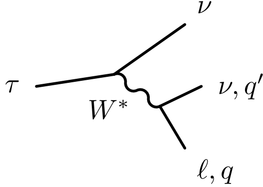
Figure 2.7: Tau-lepton decays
