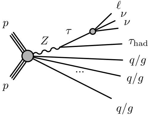
Figure 6.7: Z +jets
