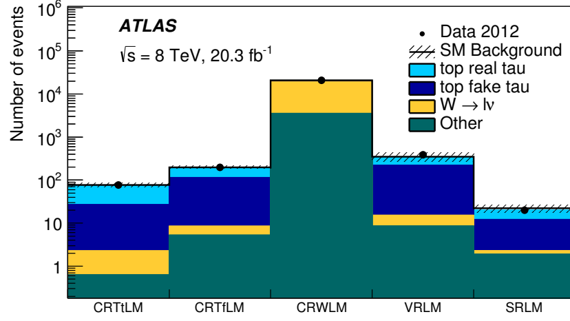
Figure 8.1: Background yields and composition after applying the background-only fit scale factors to the three CRs, the VR, and the SR in the lepton–hadron channel low-mass selection. Combined statistical and systematic uncertainties are shown as shaded bands. The observed number of events and the total (constrained) background are the same by construction in the CRs.
