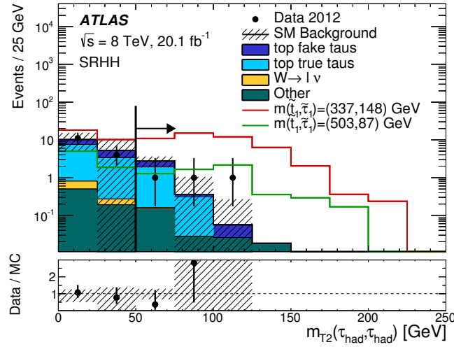
Figure 8.9: SRHH N-1: Distribution of m_{T2}(\tau_{\text{had}}, \tau_{\text{had}}) for events passing all the hadron-hadron signal region requirements, except that on m_{T2}(\tau_{\text{had}}, \tau_{\text{had}}) . The contributions from all SM backgrounds are shown as a histogram stack; the bands represent the total uncertainty. The background yields have been rescaled by the post-fit normalisation factors. The distributions expected for two signal models are also shown. This figure was taken from Reference [57]. The line and arrow show the cut on the plotted variable that is required for the hadron-hadron selection.
