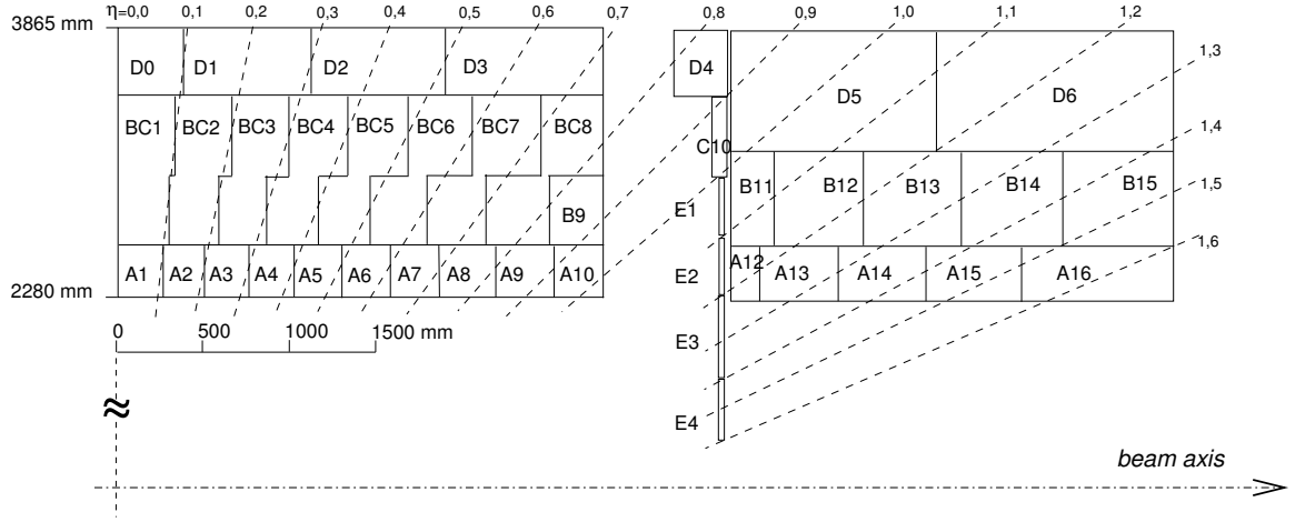
Figure 3.11: A sketch of the tile calorimeter readout fibre groupings used to create the approximately projective geometry in pseudorapidity [68].
