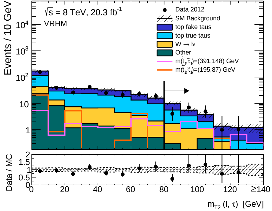
Figure 6.20: VRHM N-1: Distribution of m_{T2}(\ell, \tau_{\text{had}}) after the VRHM selection except for the cut on m_{T2}(\ell, \tau_{\text{had}}) . This validation region differs from SRHM by the inversion of the E_T^{\text{miss}} cut ( E_T^{\text{miss}} < 150 \text{ GeV} ) and a looser cut of m_{T2}(\ell, \tau_{\text{had}}) > 80 \text{ GeV} . The contributions from all SM backgrounds are shown as a histogram stack; the bands represent the total uncertainty. The distributions expected for the two signal optimisation points are also shown. The line and arrow show the cut on the plotted variable that is required for the VRHM selection.
