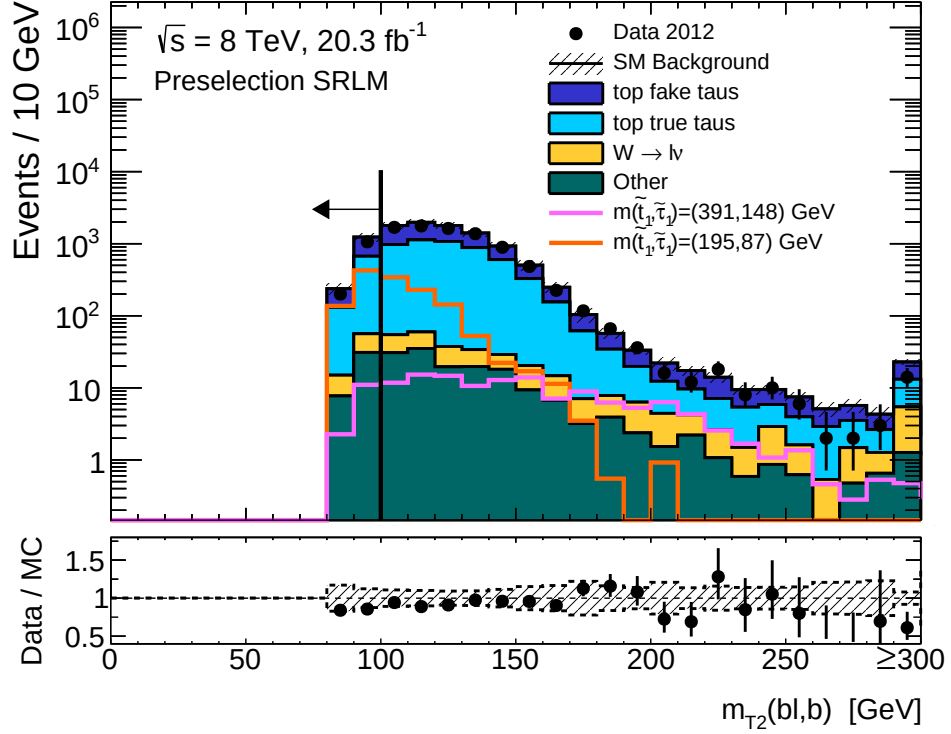
Figure 6.11: Distribution of the transverse mass constructed from the b -jet plus light charged lepton and the second b -jet, m_{T2}(b\ell, b) , for events passing the SRLM preselection requirements. The contributions from all SM backgrounds are shown as a histogram stack; the bands represent the total uncertainty. The distributions expected for the two signal optimisation points are also shown. The distribution includes corrections to the p_T of the \tau_{\text{had}} , which will be discussed in Section 6.5.7. The line and arrow show the cut on the plotted variable that is required for the SRLM selection.
