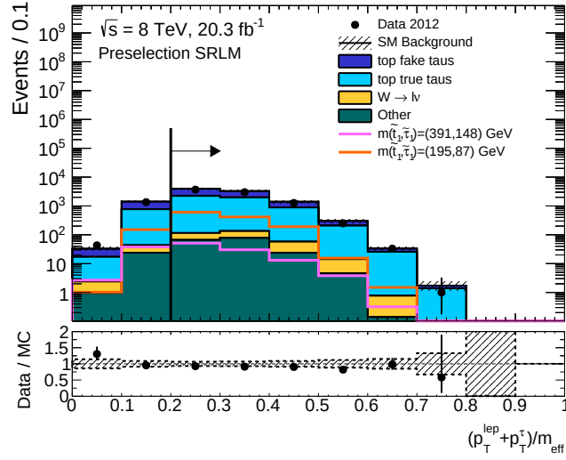
Figure 6.14: Distribution of the (p_T^\ell + p_T^{\tau_{\text{had}}})/m_{\text{eff}} for events passing the SRLM preselection requirements. The contributions from all SM backgrounds are shown as a histogram stack; the bands represent the total uncertainty. The distributions expected for the two signal optimisation points are also shown. The distributions include corrections to the p_T of the \tau_{\text{had}} , which will be discussed in Section 6.5.7. The line and arrow show the cut on the plotted variable that is required for the SRLM selection.
