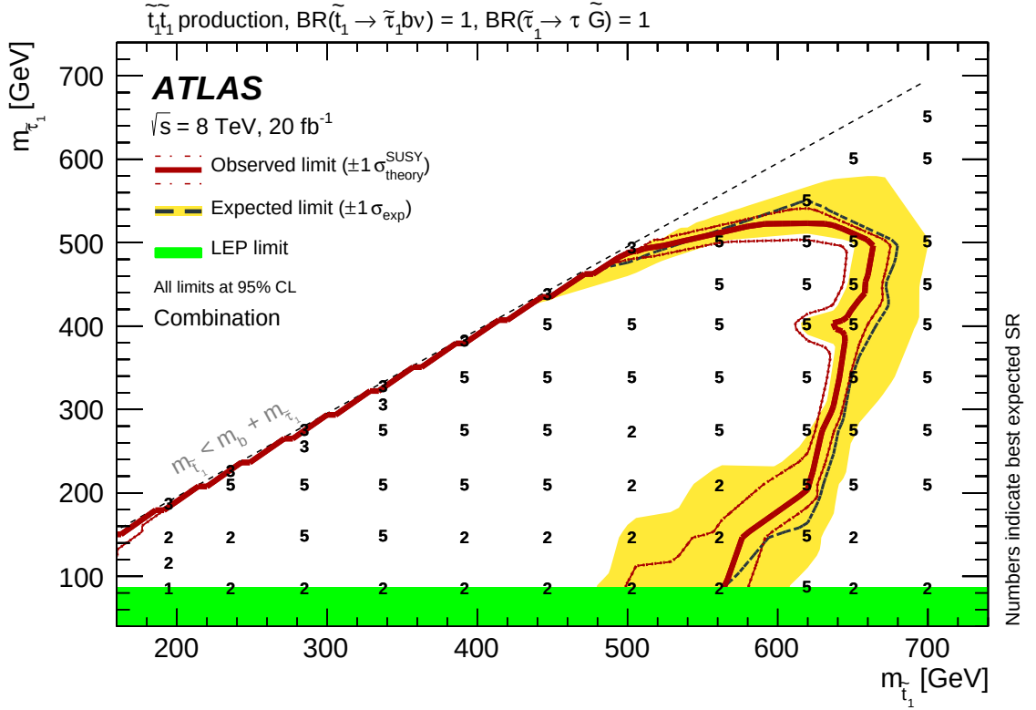
Figure 9.6: Observed and expected exclusion contours at 95% CL in the stop-stau mass plane from the combination of all selections. The dashed and solid lines show the 95% CL expected and observed limits, respectively, including all uncertainties except for the theoretical signal cross-section uncertainty. The band around the expected limit shows the \pm 1\sigma expectation. The dotted \pm 1\sigma lines around the observed limit represent the results obtained when varying the nominal signal cross-section up or down by the theoretical uncertainty. The numbers indicate which analysis gave the best exclusion for the combined: 1=lepton-hadron SRLM, 2=hadron-hadron, 3=lepton-lepton, 5=lepton-hadron SRHM. This figure was taken from Reference [57].
