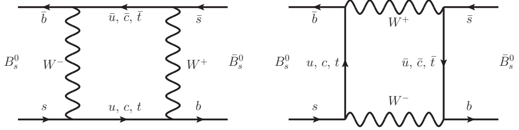
Figure 2.2: Feynman diagrams representing the second order weak interactions that give rise to B_s^0 - \bar{B}_s^0 mixing. The particles that propagate in the loop correspond to quarks with charge 2/3 . Since the t quark dominates these transitions, given the quark-mass hierarchies, V_{ts}V_{tb}^* is the dominant CKM factor in this diagram, introducing the CP -violating phase.
