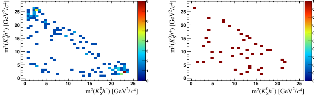
Figure 5.5: Additional events recovered by the (left) Hlt2Topo2BodySimpleTOS and Hlt2Topo3BodySimpleTOS decisions for Down-Down and Long-Long K_s^0 categories, respectively. Notice that many of these events populate the boundaries of the Dalitz plot, and therefore, are of great interest for this analysis.
