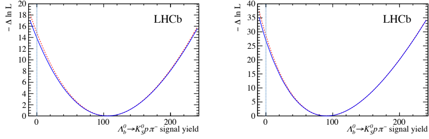
Figure 6.10: Likelihood profile of the \Lambda_b^0 \rightarrow K_s^0 p \pi^- signal yield for the (left) Down-Down and (right) Long-Long categories. The dashed red line is the statistical-only profile, while the solid blue line also includes the systematic uncertainties.
