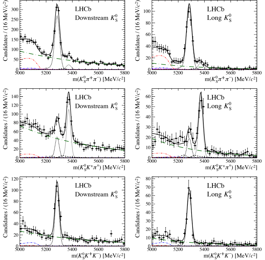
Figure 6.3: Invariant mass distributions for (top) K_S^0 \pi^+ \pi^- , (middle) K_S^0 K^\pm \pi^\mp and (bottom) K_S^0 K^+ K^- candidates for the Loose selection, separated in the (left) Down-Down and (right) Long-Long K_S^0 categories. Each component of the fit model is displayed: the B^0 ( B_s^0 ) signal components are the black short-dashed (dotted) lines; misidentified decays are the black dashed lines; partially reconstructed contributions from B to open charm decays (red dash triple-dotted), charmless hadronic decays (blue dash double-dotted), B^0 \rightarrow \eta' K_S^0 (violet dash single-dotted) and charmless radiative decays (pink short-dash single-dotted lines); and combinatorial background (green long-dash dotted line).
