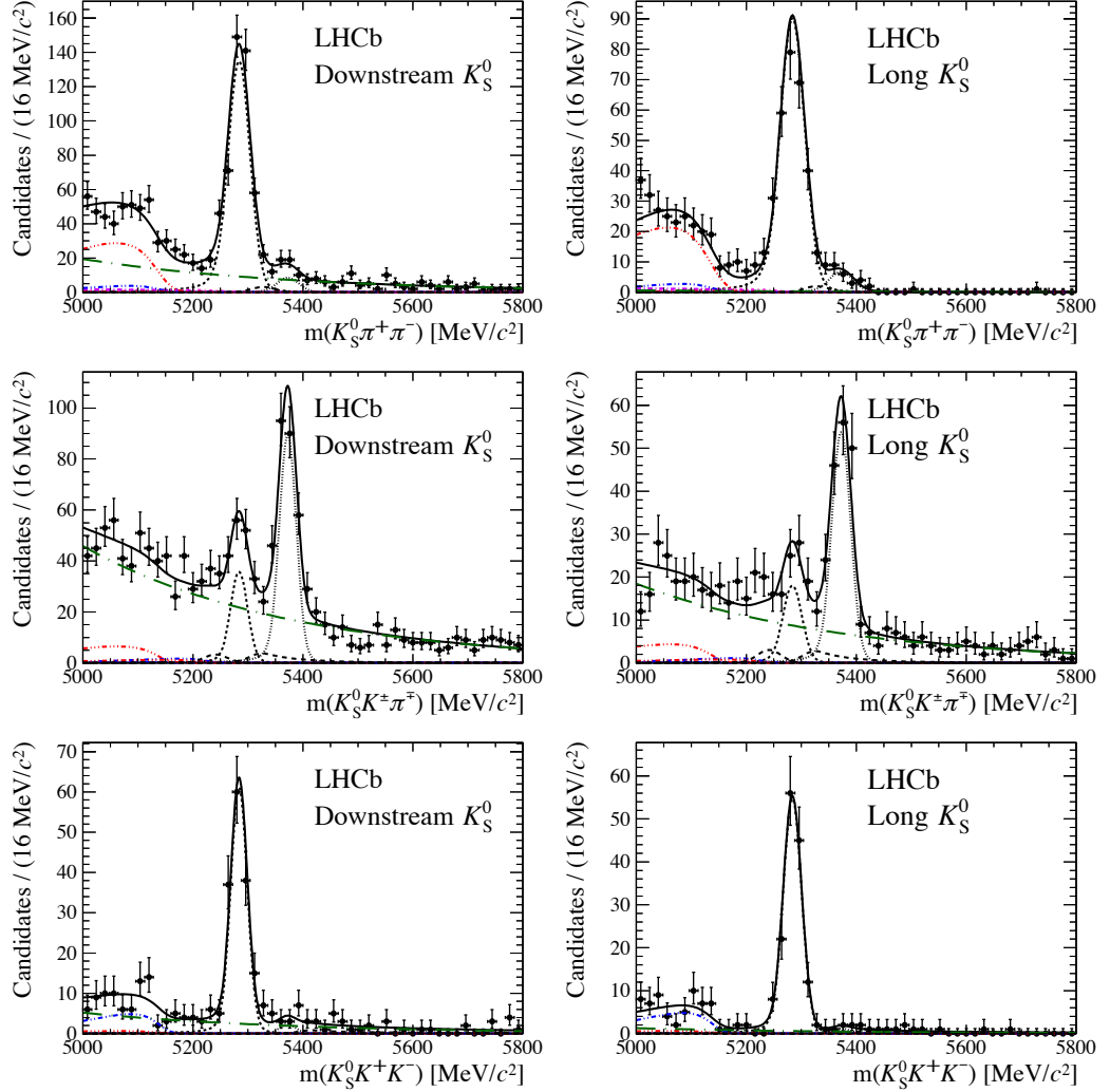
Figure 6.4: Invariant mass distributions for (top) K_S^0 \pi^+ \pi^- , (middle) K_S^0 K^\pm \pi^\mp and (bottom) K_S^0 K^+ K^- candidates for the Tight selection, separated in the (left) Down-Down and (right) Long-Long K_S^0 categories. Refer to Fig. 6.3 for components details.
