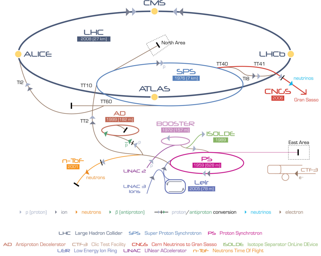
Figure 4.1: Schematic view of the CERN accelerator complex [116] with the location of the four main experiments at the LHC.
