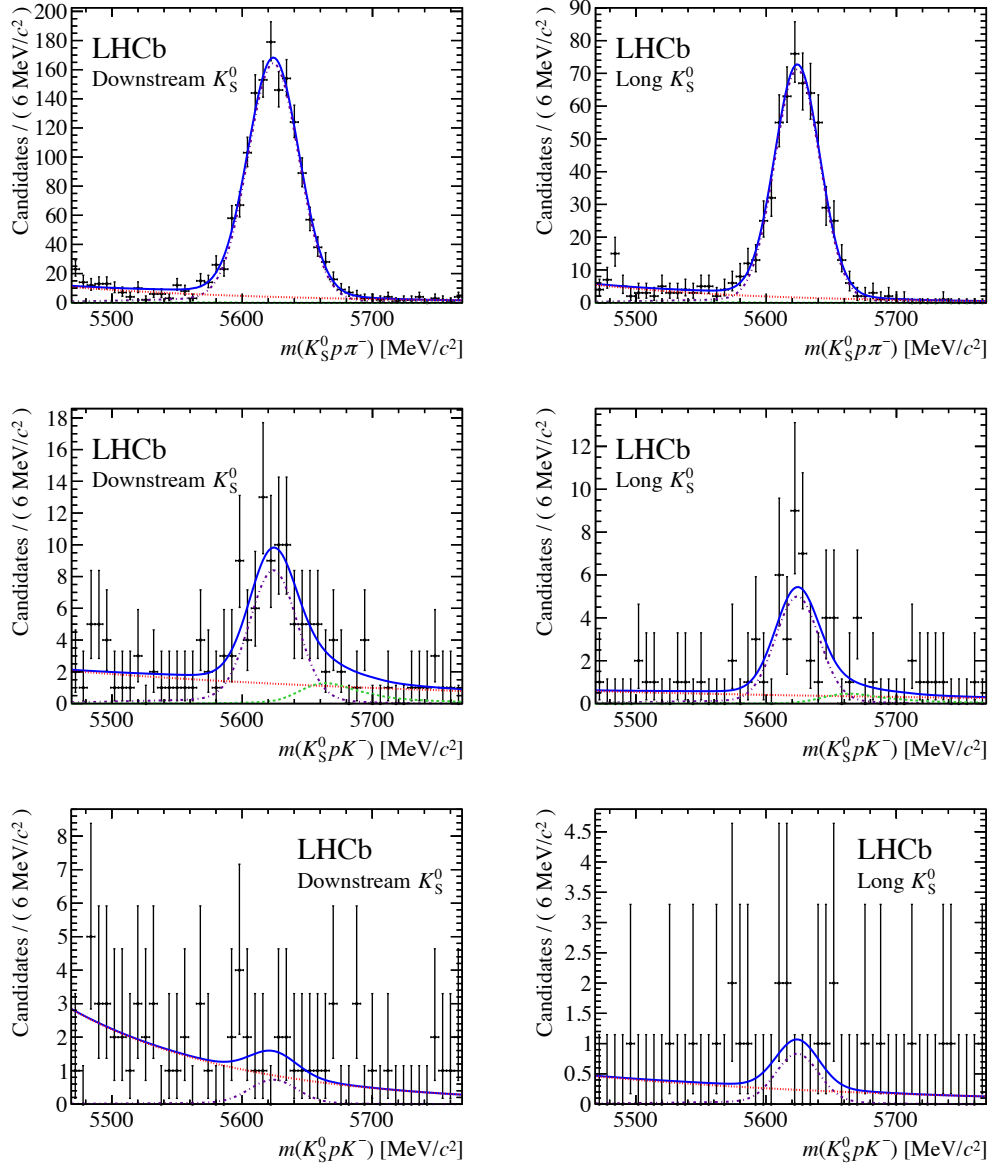
Figure 6.9: Invariant mass distribution of (top) \Lambda_b^0 \rightarrow \Lambda_c^+(p K_S^0) \pi^- , (middle) \Lambda_b^0 \rightarrow \Lambda_c^+(p K_S^0) K^- and (bottom) \Lambda_b^0 \rightarrow D_s^-(K_S^0 K^-) p candidates for the (left) Down-Down and (right) Long-Long K_S^0 categories. Refer to Fig. 6.8 for components details.
