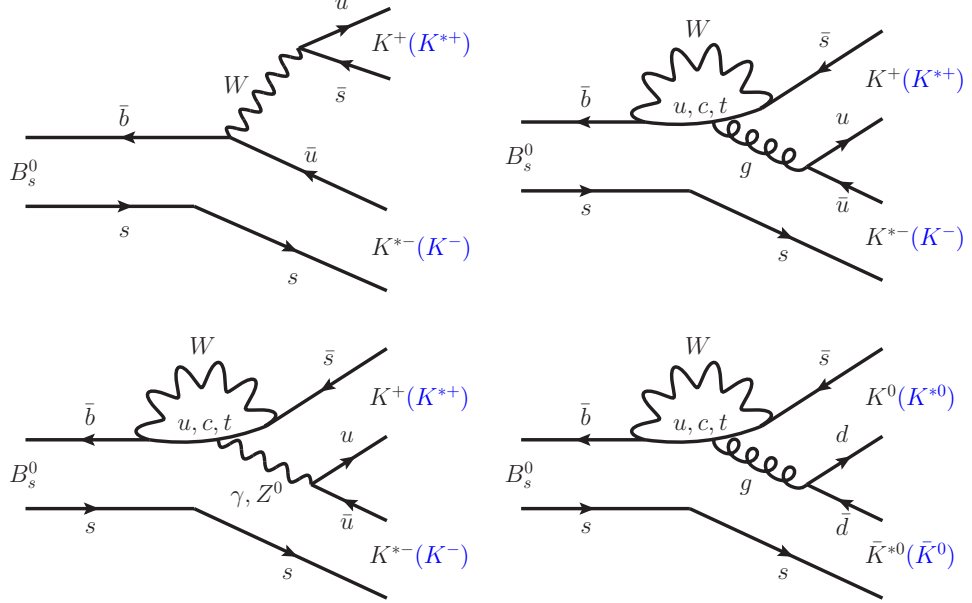
Figure 3.1: Feynman diagrams for (top left) external tree, (top right) gluonic penguin and (bottom left) EWP contributions for B_s^0 \rightarrow K^{*\pm} K^\mp decays; and (bottom right) gluonic penguin amplitude for the B_s^0 \rightarrow \bar{K}^{*0} K^0 (K^{*0} \bar{K}^0) decay mode.
