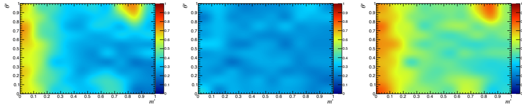
Figure 5.1: L0 efficiency variation as a function of the B_s^0 \rightarrow K_S^0 K^+ \pi^- square Dalitz plot position for (left) L0HadronTOS , (middle) L0GlobalTIS and (right) L0HadronTOS or L0GlobalTIS decisions.
