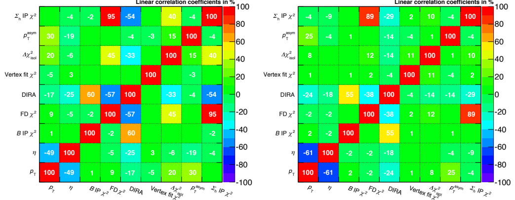
Figure 5.8: Correlations between training variables for (left) simulated B^0 \rightarrow K_S^0 \pi^+ \pi^- decays and (right) background from high mass sideband.
