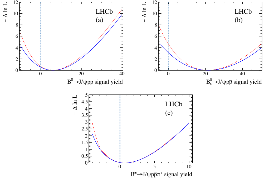
Figure A.3: Negative log-likelihood profiles for the (a) B^0 \rightarrow J/\psi p \bar{p} , (b) B_s^0 \rightarrow J/\psi p \bar{p} , and (c) B^+ \rightarrow J/\psi p \bar{p} \pi^+ signal yields. The red dashed line corresponds to the statistical-only profile while the blue line includes all the systematic uncertainties.
