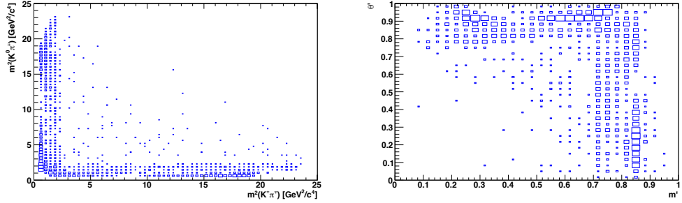
Figure 3.6: Simulated distributions for the (left) standard and (right) square Dalitz plot for B_s^0 \rightarrow \bar{K}^0 K^\pm \pi^\mp decays.
