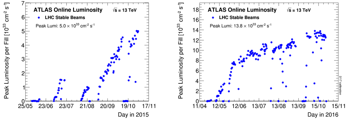
Figure 3.3: Peak luminosity recorded by the ATLAS detector for each day in 2015 (left) and 2016 (right).
