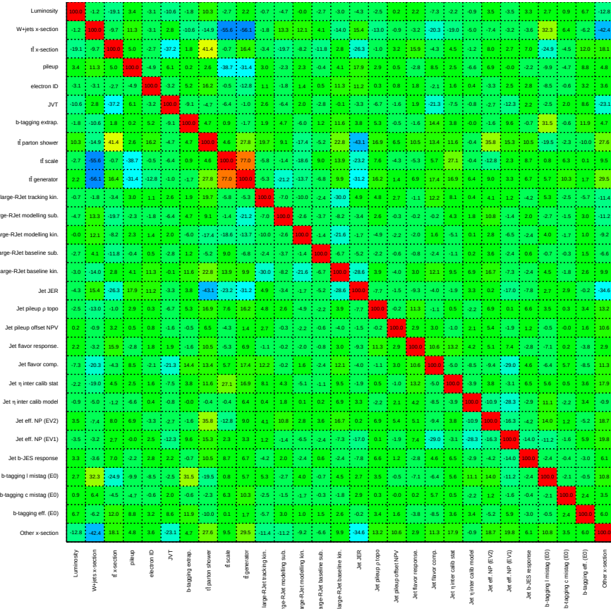
Figure 5.25: Correlation matrix showing the correlations of the nuisance parameters for the fit to the Asimov dataset in the signal+background hypothesis. The correlation scale legend corresponds to 100% (red), 0% (green) and -100% (violet). Only nuisance parameters with a correlation coefficient of at least 10% with any other parameter are displayed.
