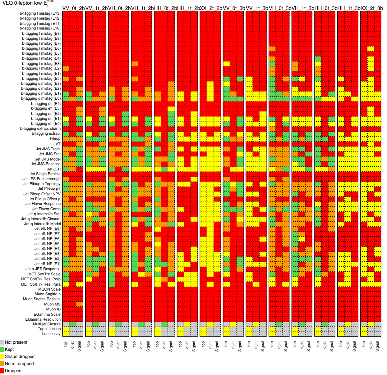
Figure 5.64: Summary of the pruning of the systematic uncertainties. The uncertainties that have the shape (normalization) component removed are yellow (orange) and those that are red were completely dropped from the fit. Uncertainties are green if both shape and normalization remain in the fit.
