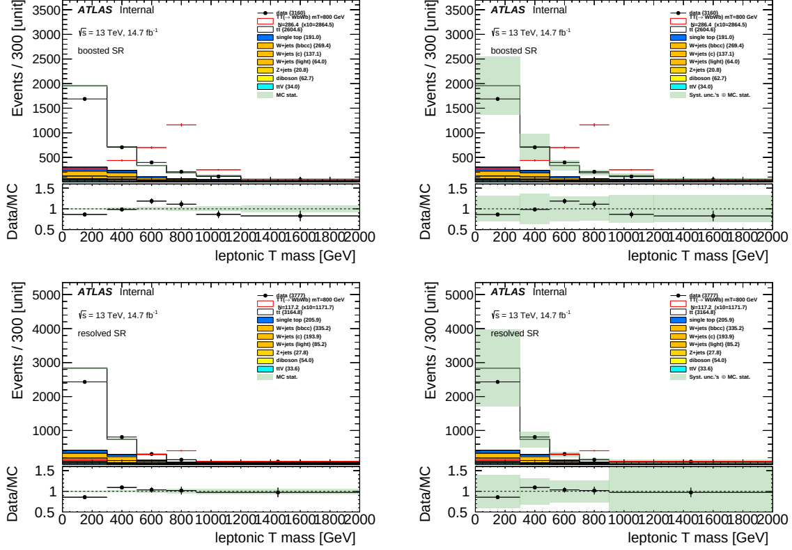
Figure 5.13: Comparison of data and MC for the boosted (top) and resolved (bottom) signal regions in the \ell + jets channel before (left) and after (right) the inclusion of the detector and t\bar{t} background modeling systematics. No fake estimate is present in these comparisons.
