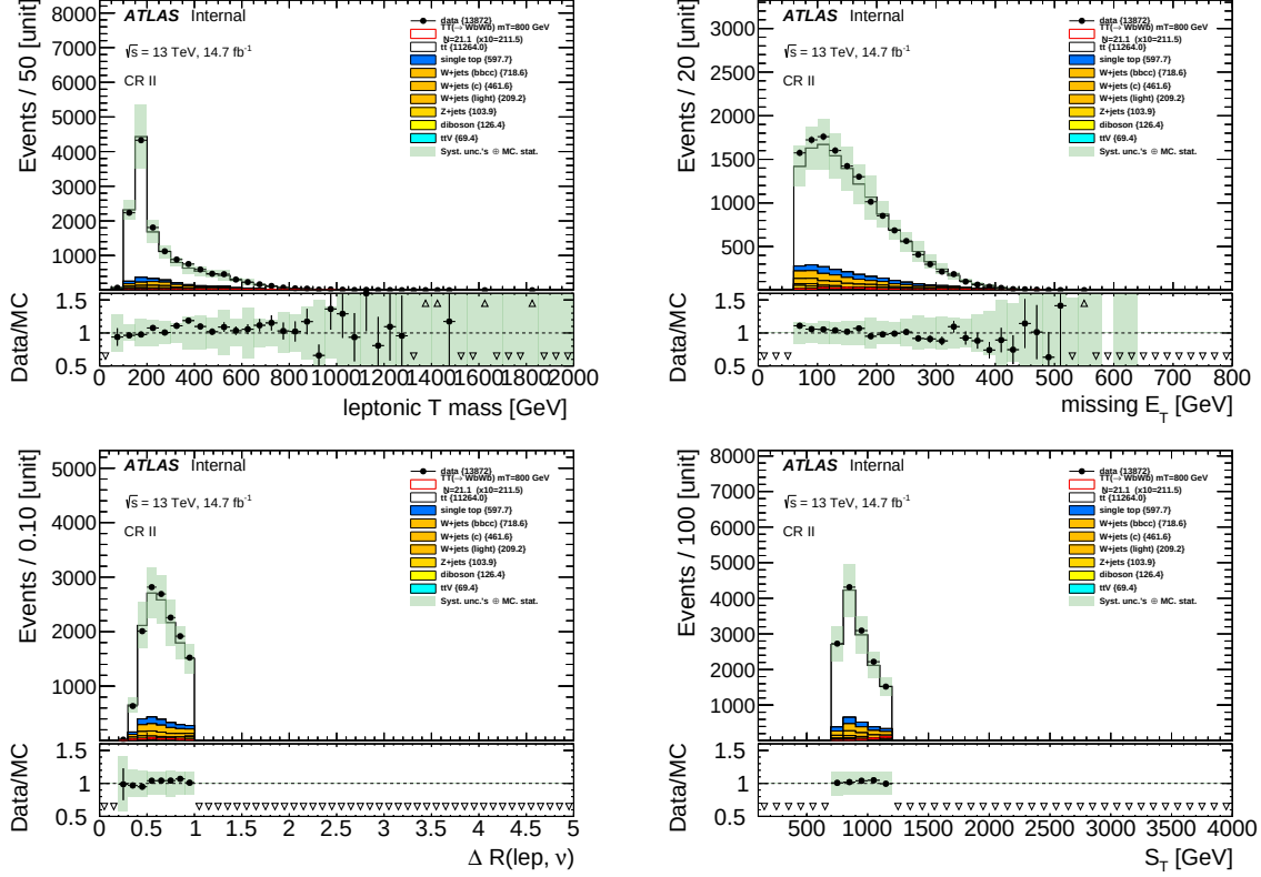
Figure 5.9: Data and MC comparison in CR2. The green band represents MC statistical uncertainties, as well as all t\bar{t} modeling and detector-related systematic uncertainties.
