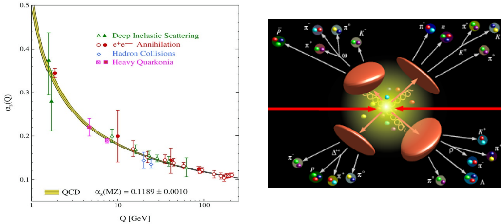
Figure 1.4: Running coupling \alpha_s as a function of the interaction energy ( \alpha_s = g_s^2/4\pi ) and representation of the confinement effect after the emission of quarks or gluons issued from an interaction. It can be observed how quarks and gluons scatter out of the collision point. As partons move away, g_s running coupling increases and at one point, quark-antiquark pairs are created from the vacuum and combine with the outgoing partons to form hadrons.
