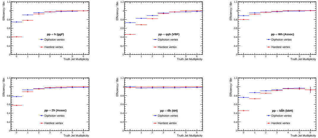
Figure 6.15: Truth Higgs boson production vertex identification efficiency using the diphoton or the hardest vertex method. Efficiency is presented as a function of the number of truth jets in the event.
