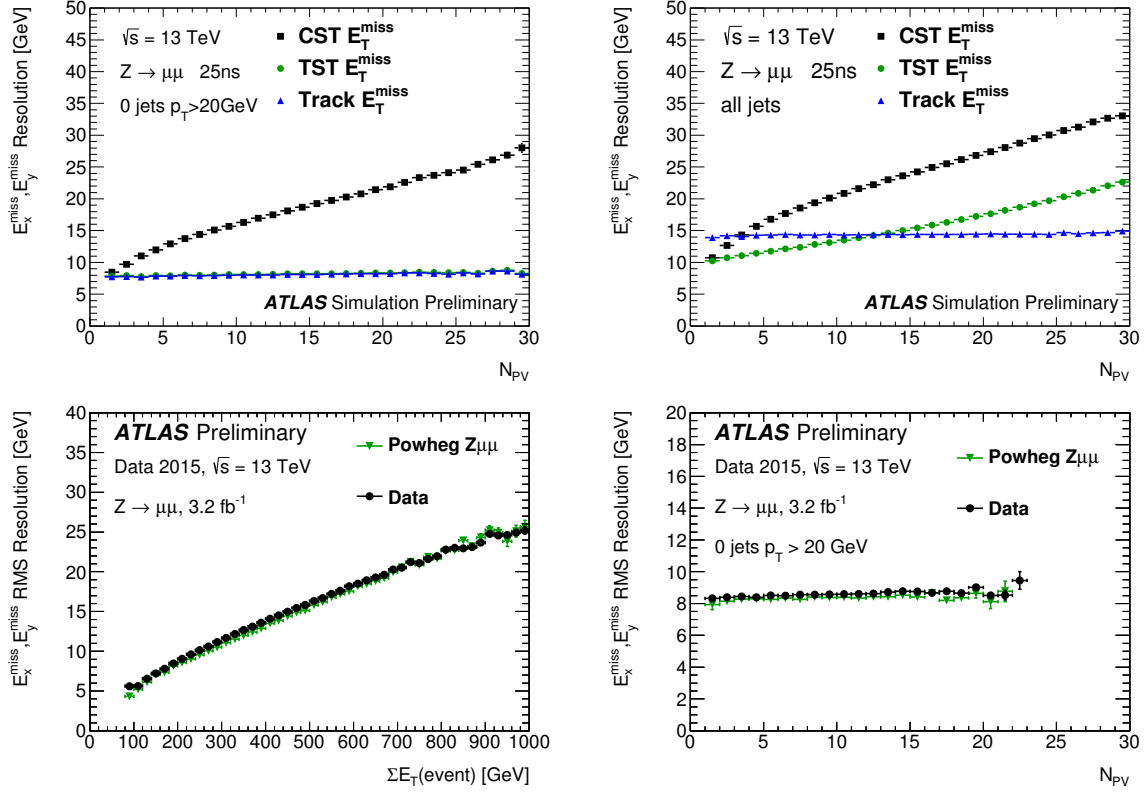
Figure 6.12: Resolution (RMS) of the E_{x,y}^{\text{miss}} distributions using CST, TST and Track- E_T^{\text{miss}} on Z \rightarrow \mu^- \mu^+ MC samples (upper plots) and comparison between TST E_T^{\text{miss}} in 2015 data (3.2 \text{fb}^{-1} ) and MC. Resolution is presented as a function of the number of primary vertices in the event in the upper plots, either considering all events (left) or events with no reconstructed jet (right) [18]. Bottom left plot presents the comparison between data and MC on 0-jet events as a function of the NPV and \sum |E_T| using TST reconstruction scheme, both for events Z \rightarrow \mu^- \mu^+ [19].
