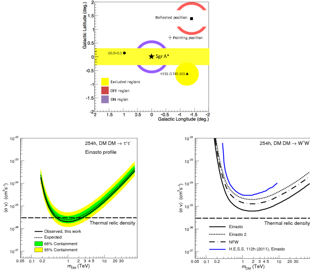
Figure 1.22: Summary of H.E.S.S. 10-year observation and results on the GC \gamma -ray spectrum. The top plot presents the signal (ON) and background (OFF) regions observed to study the galactic background. The bottom left plot presents the limits on WIMP thermal averaged cross-section \langle\sigma v\rangle depending on the DM particle mass using the Einasto [97] profile distribution. The bottom right plot presents the dependence of H.E.S.S. limits on the DM spatial distribution model. All plots are taken from [96].
