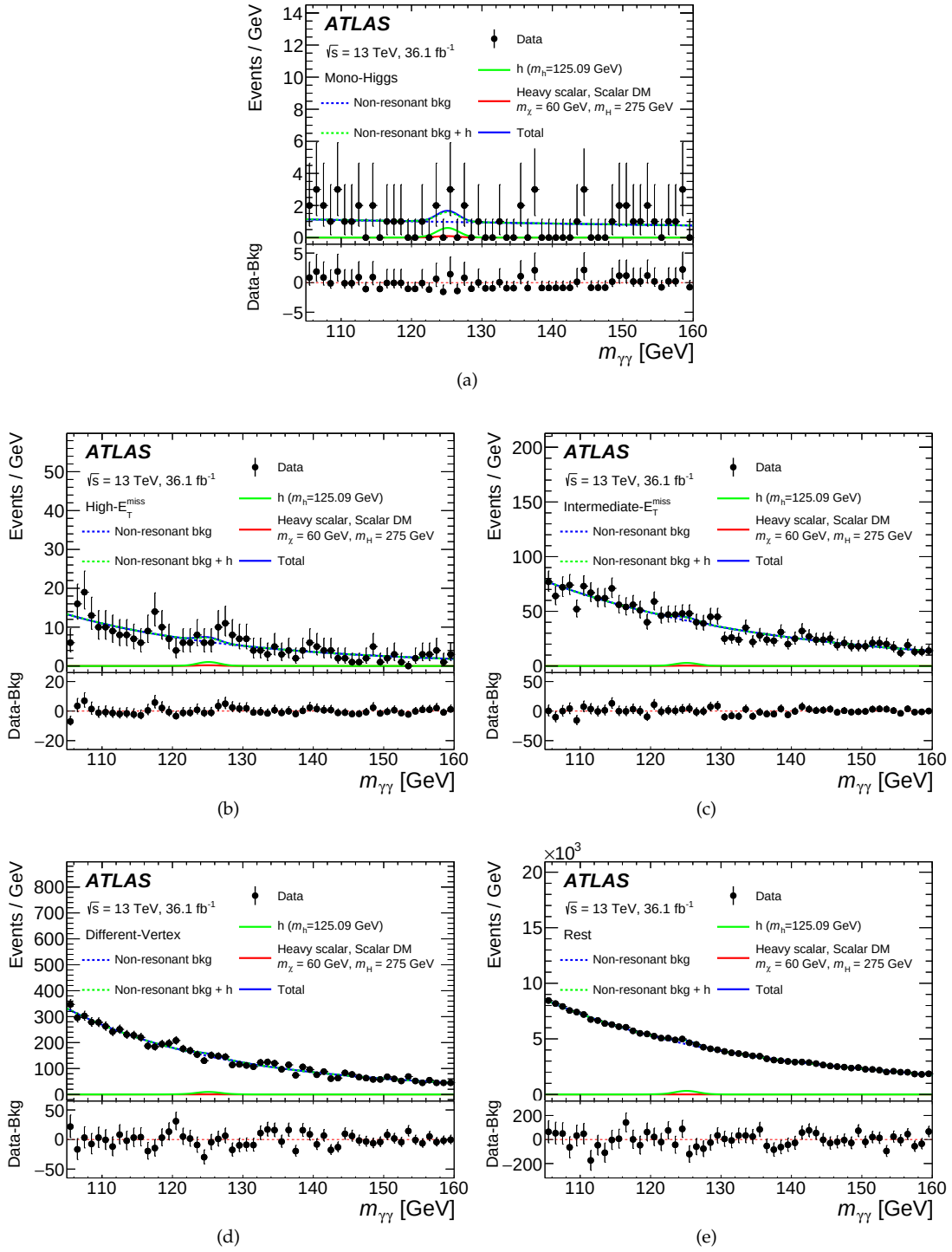
Figure 7.41: Diphoton invariant mass distribution for data and the corresponding fitted signal and background in the five categories, (a) Mono-Higgs category, (b) High- E_T^{\text{miss}} category, (c) Intermediate- E_T^{\text{miss}} category, (d) Different-Vertex category and (e) Rest category taken from Ref. [3]. On each plot, the data (dots with asymmetric error bars) is shown. The error bars represent the central Poissonian confidence intervals at 68% CL. The simultaneous fit result including a heavy-scalar signal (solid red line), SM Higgs boson (solid green line), the non-resonant background (dashed blue line) and the non-resonant background plus the SM Higgs boson (dashed green line) are shown as well as the sum of all those contributions (solid blue line). The fitted heavy-scalar signal shown here corresponds to m_H = 275 GeV and scalar DM m_\chi = 60 GeV.
