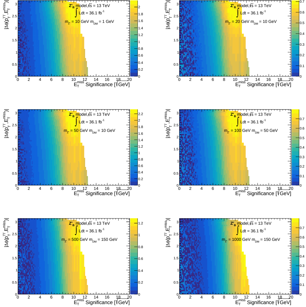
Figure 7.12: Significance scan for various masses of the Z'_B boson and DM particle depending on the S_{E_T^{\text{miss}}} and \Delta\phi(p_T^{\gamma\gamma}, E_T^{\text{miss}}) variables for the Z'_B model. Event weights are applied and signal and background samples are scaled to their corresponding cross-sections or purity ( \gamma\gamma and \gamma +jet).
