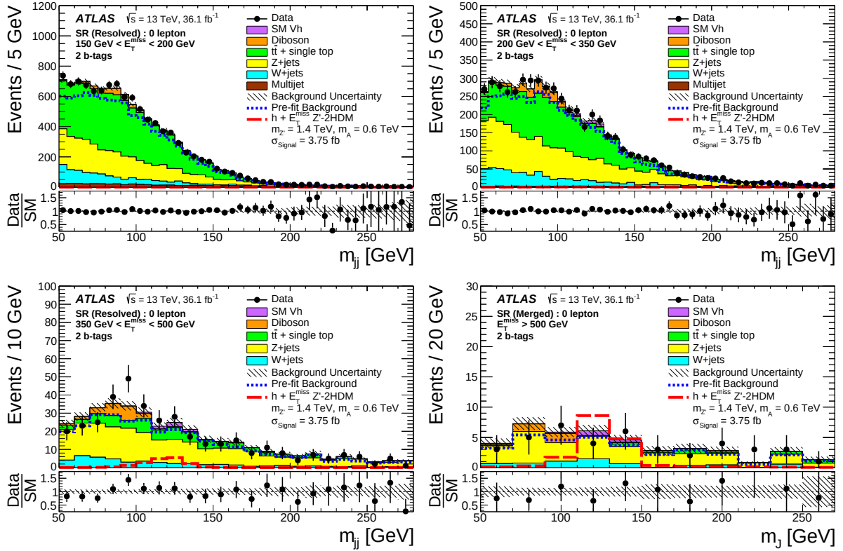
Figure 7.44: Distributions of the invariant mass of the Higgs boson candidates m_{h,\text{reco}}=m_{jj}, m_j with two b-tags in the SR for the four E_T^{\text{miss}} categories that are used as inputs to the fit. The upper panels show a comparison of data to the SM expectation before (dashed lines) and after the fit (solid histograms) with no signal included. The lower panels display the ratio of data to SM expectations after the fit, with its systematic uncertainty considering correlations between individual contributions indicated by the hatched band. The expected signal from a representative Z' -2HDM model is also shown (long-dashed line). [59]
