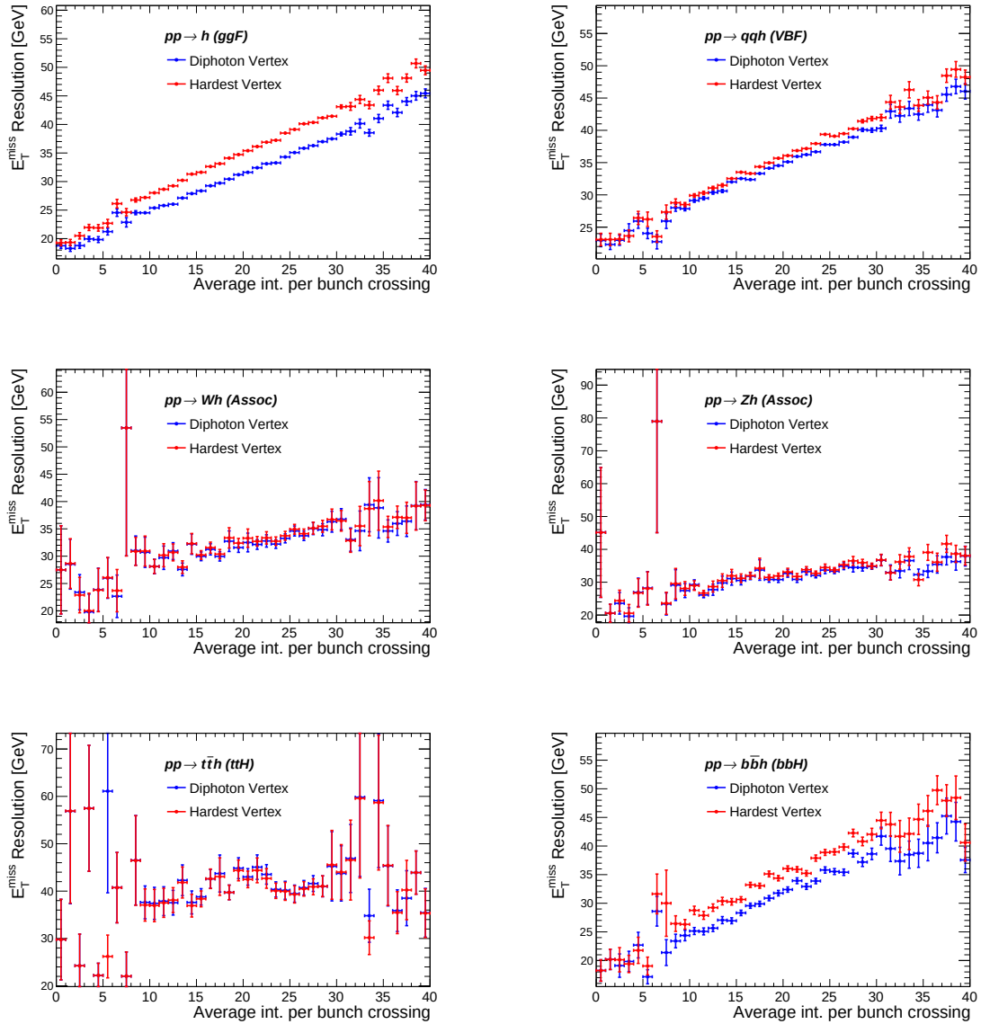
Figure 6.21: E_T^{\text{miss}} resolution estimated as the RMS of the E_T^{\text{miss}} distribution depending on the average number of interactions per bunch crossing. Truth information is subtracted and TST reconstruction is compared to soft-terms either associated with the hardest vertex or to the diphoton vertex of the event.
