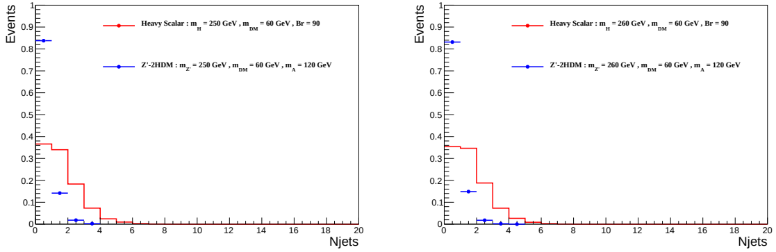
Figure B.20: Comparison of kinematic distributions between Z'-2HDM and Heavy scalar models for the same mediator and DM particle masses ( m'_Z = 250 or 260 GeV, m_\chi = 60 GeV)
