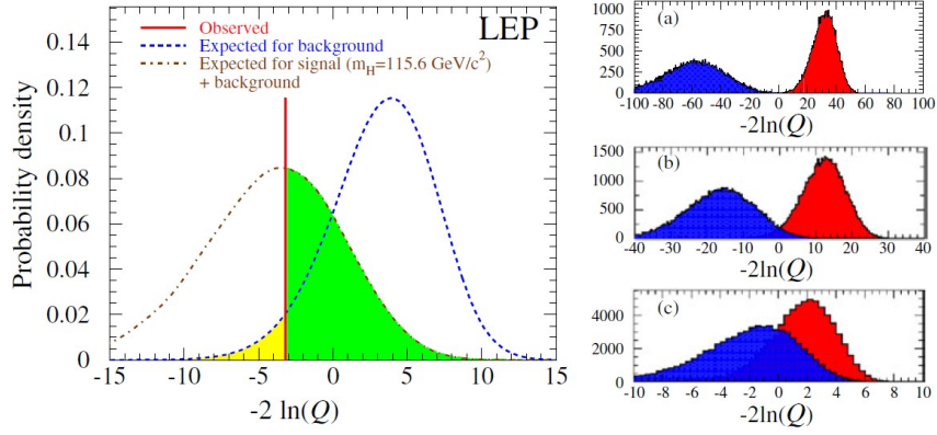
Figure A.2: On the left, the pdf of the test statistics for the Higgs search at LEP for the background (right) and signal+background hypotheses (left) are illustrated. The light yellow region to the left of the observation is 1 - CL_b and the dark green is CL_{s+b} . On the right, the evolution of the pdfs is presented with falling search sensitivity from (a) to (c) as the Higgs mass hypothesis is increased and the production cross-section falls [3].
