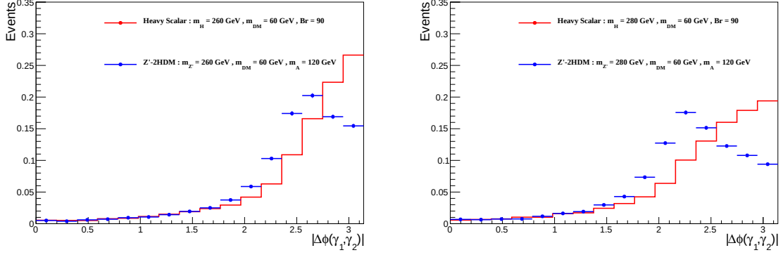
Figure B.12: Comparison of kinematic distributions between Z'-2HDM and Heavy scalar models for the same mediator and DM particle masses ( m'_Z = 260 or 280 GeV, m_\chi = 60 GeV)
