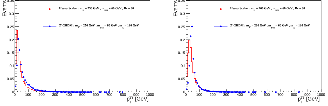
Figure B.24: Comparison of kinematic distributions between Z'-2HDM and Heavy scalar models for the same mediator and DM particle masses ( m'_Z = 250 or 260 GeV, m_\chi = 60 GeV)
