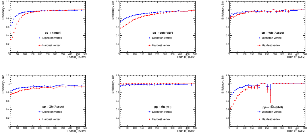
Figure 6.16: Truth Higgs boson production vertex identification efficiency using the diphoton or the hardest vertex methods. Efficiency is presented as a function of the transverse momenta of the truth diphoton system. Photons are previously matched as children of the truth Higgs boson.
