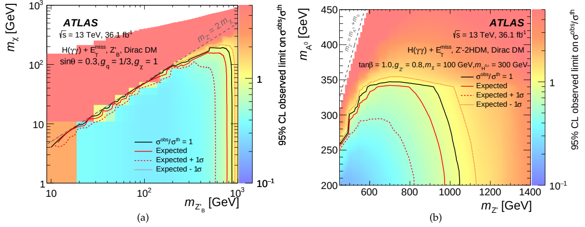
Figure 7.39: The ratios of the observed and expected 95% CL upper limits on the signal cross-section to the predicted signal cross-sections for (a) the Z'_B model in the (m_\chi, m_{Z'_B}) plane and (b) the Z' -2HDM model in the (m_{A^0}, m_{Z'}) plane [3]. For the Z'_B model, the mixing angle \sin \theta = 0.3 , and the coupling values g_q = 1/3 and g_\chi = 1 are used. In the scenario of Z' -2HDM model, the ratio of the two-Higgs-doublet vacuum expectation values \tan \beta = 1.0 , Dirac fermion DM mass m_\chi = 100 GeV, and the coupling value g_{Z'} = 0.8 are used. The masses of the neutral CP-even scalar ( H^0 ) and the charged scalars ( H^\pm ) from Z' -2HDM model are set to 300 GeV. The plus and minus one standard deviation expected exclusion curves are also shown as red dashed and dotted lines. The regions below the lines (i.e. with \sigma^{\text{obs}}/\sigma^{\text{th}} < 1 ) are excluded. In both figures, the gray dashed line corresponds to the boundary of the region above which the Z' boson is produced off-shell.
