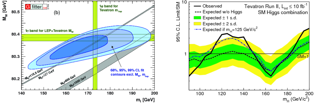
Figure 1.6: Prediction of the mass of the Higgs boson by comparing the measured masses of the top and the W boson and measured 95 % CL limits on the Higgs production cross-section at Tevatron with 10 \text{ fb}^{-1} integrated luminosity [48, 49].
