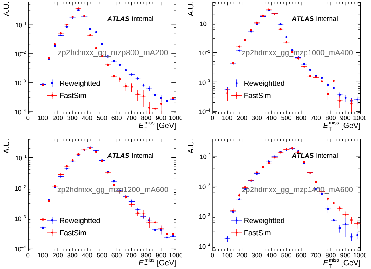
Figure 7.33: Comparison of the MET spectrum obtained either from the reweighted base sample or with a FastSim sample for different points in the parameter space of the Z' - 2HDM model
