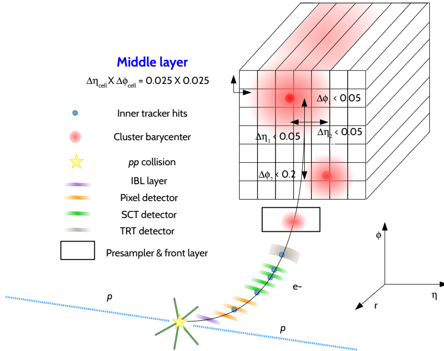
Figure 4.5: Picture illustrating the cluster-track matching for electrons and converted photons in the EM barrel calorimeter.
