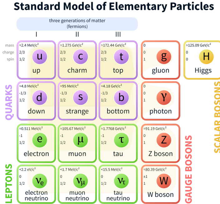
Figure 1.5: General picture of elementary particles and force carriers included in the Standard Model [30].
