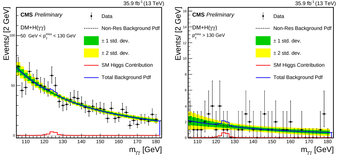
Figure 7.47: The dashed black line presents the fitted non-resonant background and the solid red line, the SM h \rightarrow \gamma\gamma contribution for both categories (left: low- p_T^{\text{miss}} ; right: high- p_T^{\text{miss}} ) category. The sum of the non-resonant and resonant background shapes is shown in blue [62].
