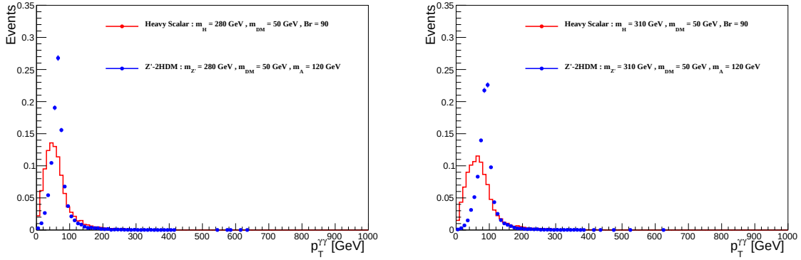
Figure B.23: Comparison of kinematic distributions between Z'-2HDM and Heavy scalar models for the same mediator and DM particle masses ( m'_Z = 280 or 310 GeV, m_\chi = 50 GeV)
