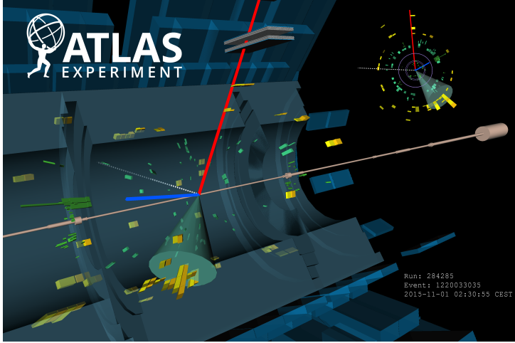
Figure 6.10: Example of an event with large E_T^{\text{miss}} in ATLAS data: display of event 1220033035 in run 284285 recorded by ATLAS in LHC proton-proton collisions at a centre-of-mass energy of 13 TeV. This candidate is likely to be the production of a W boson in association with a single top quark in the dilepton channel. Two opposite charged leptons are reconstructed. The reconstructed electron is represented by the blue line and the reconstructed muon is represented by the red line. One b-jet is identified and represented by an azure cone and the missing transverse momentum coming from a neutrino is represented by the dotted white line [12].
