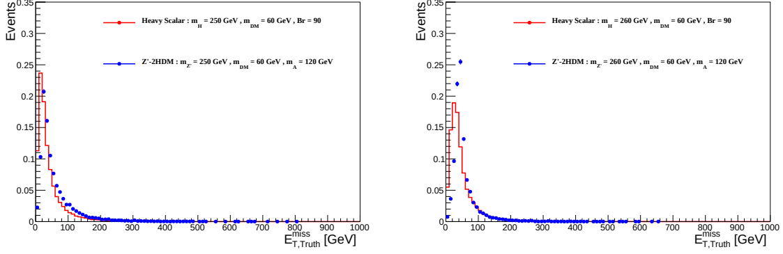
Figure B.3: Comparison of E_T^{\text{miss}} spectrum of Z'-2HDM versus Heavy scalar model for same mediator and DM particle masses ( m'_{Z'} = 250 or 260 \text{ GeV} , m_\chi = 60 \text{ GeV} )
