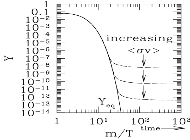
Figure 1.19: Evolution of the dark matter abundance before and at the moment of freeze-out. It can be observed that at one moment the dark matter decoupled from the interaction with the rest of the plasma species and for that time onward, its relic density remained constant [81].
