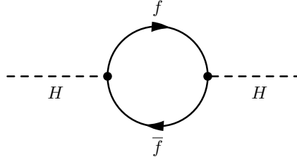
Figure 1.13: Fermion loop corrections to the Higgs self-interaction term. The dominant contribution corresponds to the top loop, due to the large t - h coupling.
