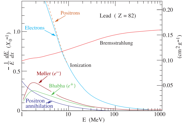
Figure 3.3: Electron (or positron) fractional loss of energy in lead [6].
