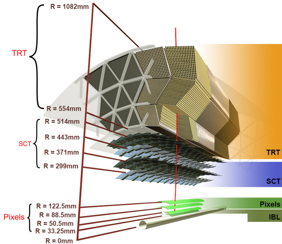
Figure 2.11: Illustration of the barrel region of the inner tracker showing the different subdetector layers and structures traversed by a charged particle created in collision point during Run II [18].
