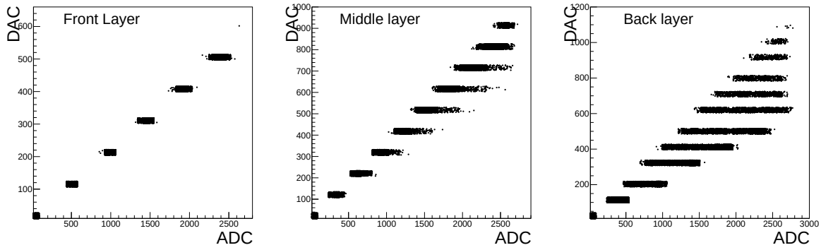
Figure 3.22: Run 00314180: DAC versus ADC_{peak} obtained in a high gain run for the 3 layers of the electromagnetic calorimeter.
