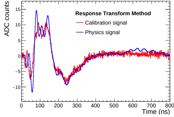
Figure 5.15: Calibration (red) and physics cross-talk signal presented in a middle cell layer of the calibration run 00227022. This cell corresponds to the previous neighbour in \eta of a pulsed cell of the calibration run. Physics shape is determined using the RTM method.
