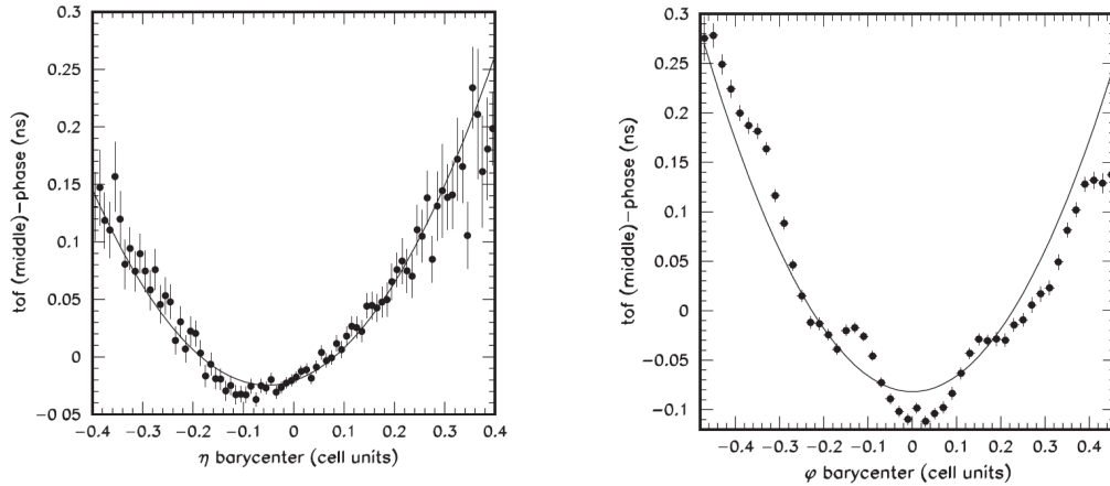
Figure 3.28: Difference between reconstructed OF time and trigger time depending on the barycenter of energy deposition in between cells in \eta and \phi [9].
