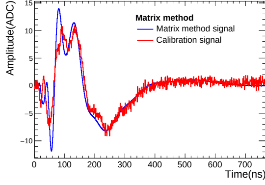
Figure 5.16: g(t)_{\text{xtalk}}^{\text{phys}} after using matrix inversion.
