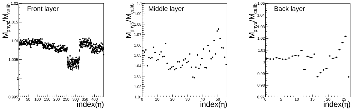
Figure 3.25: Run 00314179: value of \frac{M_{\text{phys}}}{M_{\text{calib}}} for (a) the front layer, (b) the middle layer and (c) for the back layer of the electromagnetic barrel.
