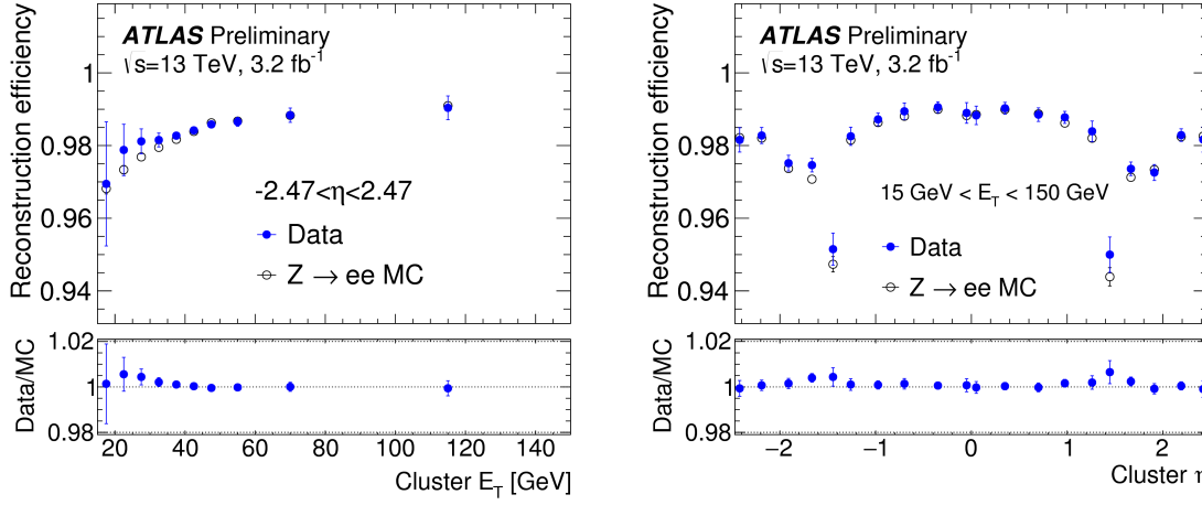
Figure 4.8: Measured reconstruction efficiencies for electrons as a function of E_T integrated over the full pseudorapidity range (left) and as a function of pseudo-rapidity for 15 \text{ GeV} < E_T < 150 \text{ GeV} (right) for the 2015 dataset. The shown uncertainties are statistical plus systematic errors [6].
