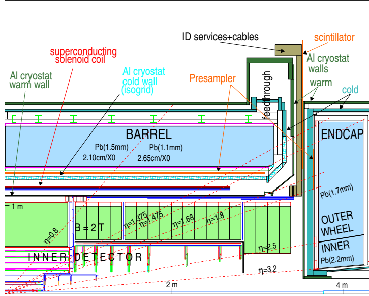
Figure 3.7: Section of the calorimeter showing the barrel and the end-cap together with \eta projections [12].
