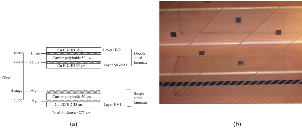
Figure 3.11: Electrode components of the liquid argon (a) and electrodes high-voltage layers before bending, cut into small compartments connected by ink resistors (b) ([10]).
