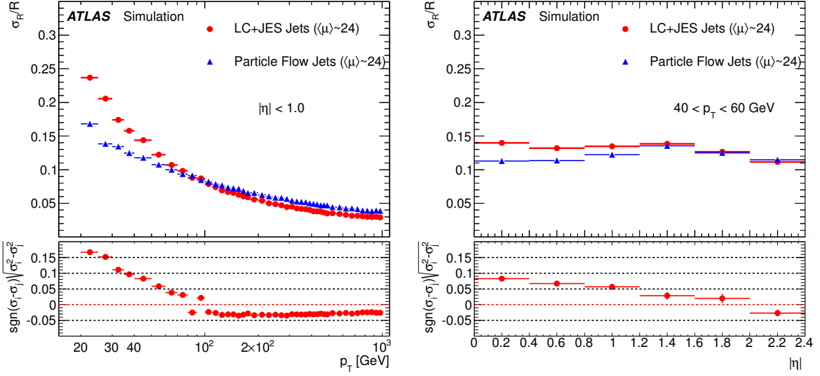
Figure 7.49: The jet transverse momentum resolution as determined in dijet MC events for calorimeter jets and particle flow jets with regard to the (a) jet transverse momentum and the (b) jet pseudo-rapidity [1].
