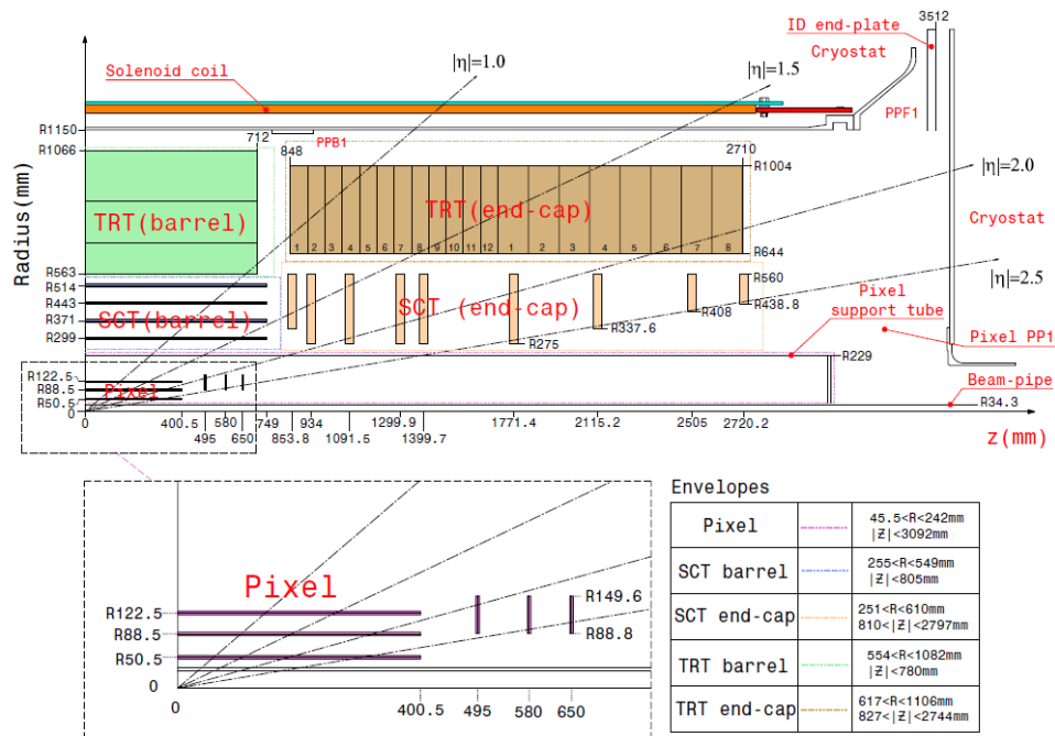
Figure 2.12: Views of a quarter section of the tracker not including the insertable B layer [2].
