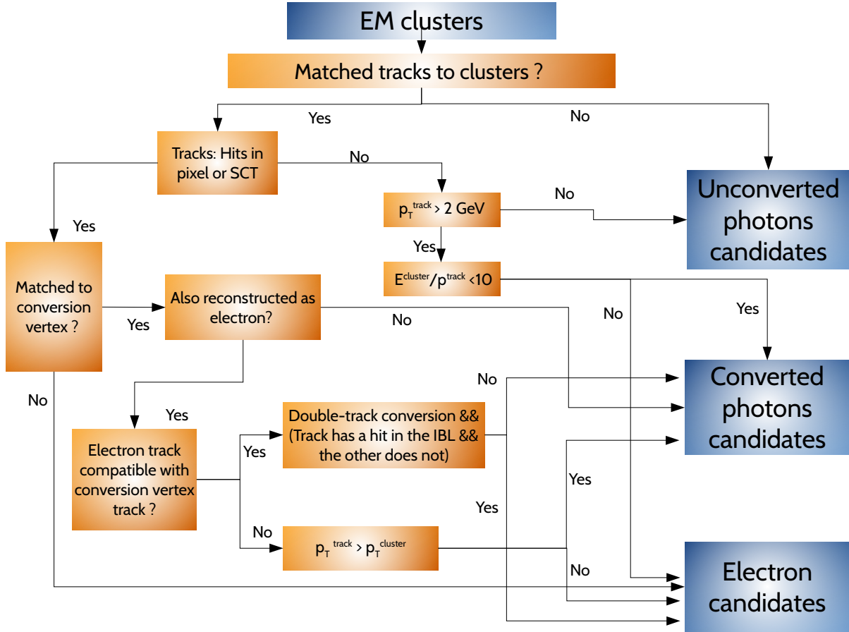
Figure 4.7: Scheme of the decision tree to initially separate electron, converted photon and unconverted photon candidates.
