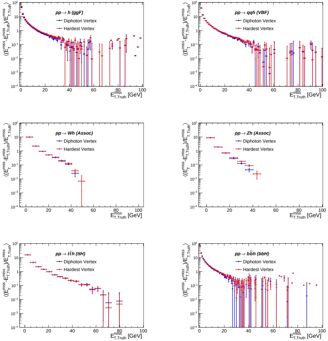
Figure 6.19: TST E_T^{\text{miss}} linearity as a function of E_{T,\text{Truth}}^{\text{miss}} for different Higgs production. TST reconstruction is compared with soft-terms either associated with the hardest vertex or to the diphoton vertex of the event.
