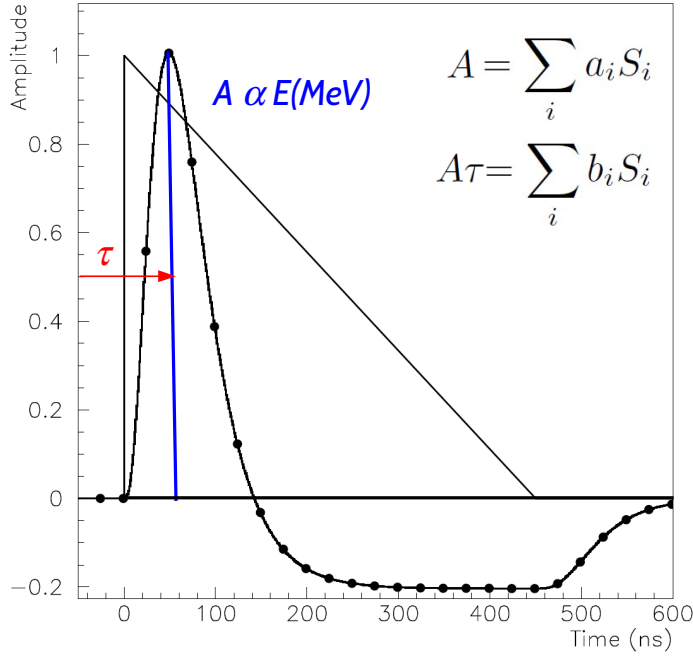
Figure 3.17: Sketch of the peaking time and amplitude of the physics signal and the estimation using optimal filtering coefficients (OFCs). The amplitude is proportional to the energy deposited in the cell.
