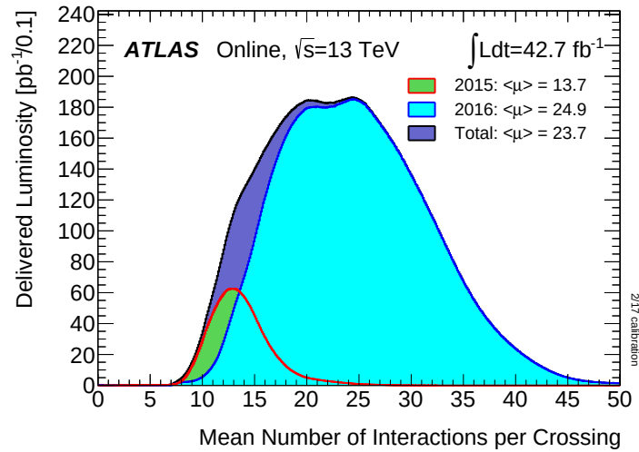
Figure 2.6: Registered number of interactions per bunch crossing during the data taking periods of 2015 and 2016, with pp collisions at \sqrt{s} = 13 TeV [14].
