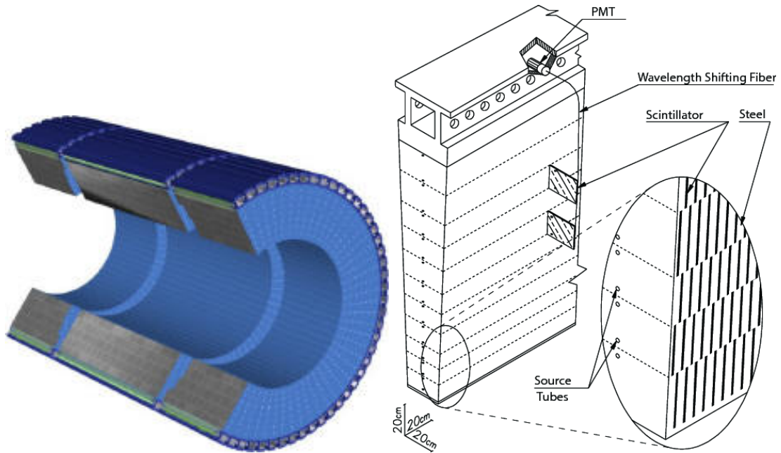
Figure 2.15: Schematic view of the tile calorimeter central region (left) and a slice of the tile calorimeter barrel (right) showing the disposition of the absorbers, the scintillating tiles and the readout PMT's [2].
