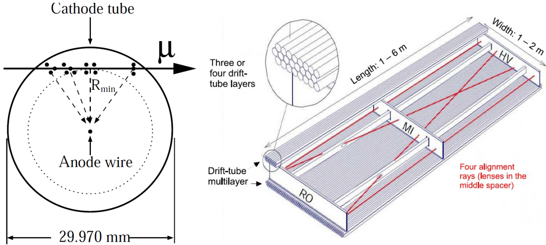
Figure 2.17: Section of an MDT tube (left) and schema of the structure of one MDT chambers (right) [2].
