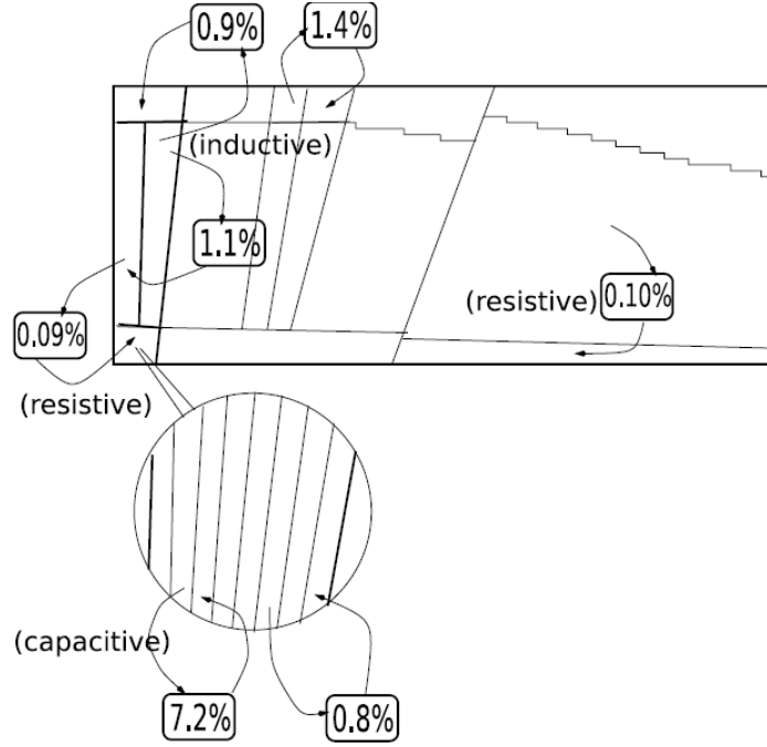
Figure 5.8: Schema of the different cross-talk magnitudes using the peak-peak estimation [8].
