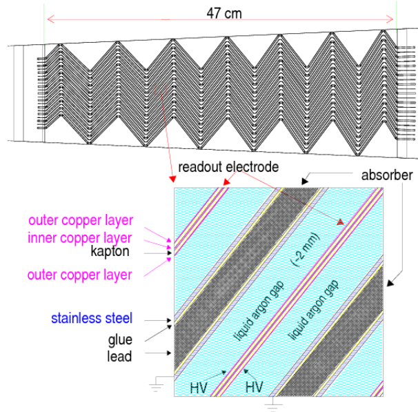
Figure 3.9: Schema of the absorber and electrode disposition in the EM calorimeter barrel.
