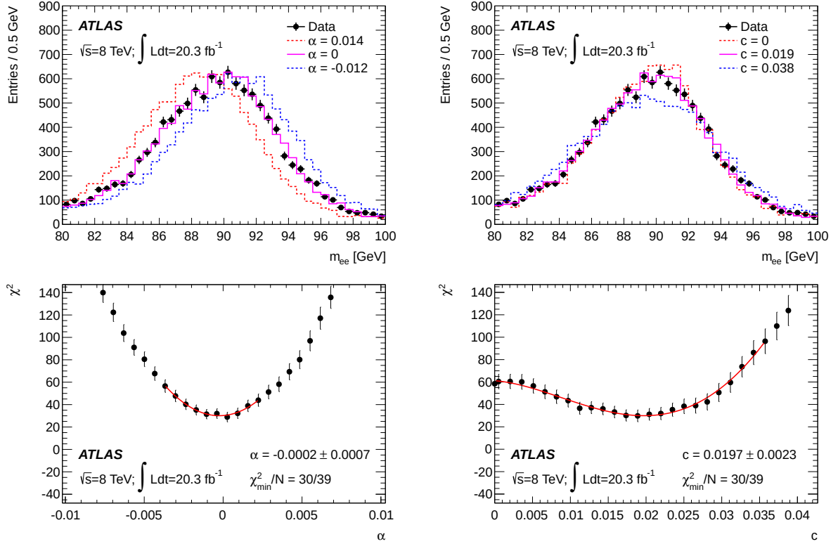
Figure 4.23: Top plots: electron pair invariant mass distribution for Z \rightarrow ee candidates in data compared to MC templates. Different values of \alpha_{ij} (left) are tested for a fixed value of c'_{ij} and viceversa (right). One electron is within 1.63 < \eta < 1.74 and the other, within 2.3 < \eta < 2.4 . Bottom plots: \chi^2 as a function of \alpha_{ij} (left) and c'_{ij} (right) [2].
