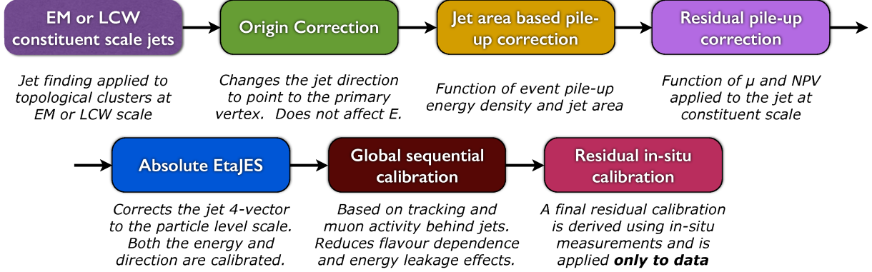
Figure 6.1: Calibration scheme of EM and LCW jets [4].
