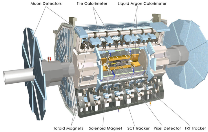
Figure 2.8: Schema of the ATLAS detectors and the different subdetectors [2].
