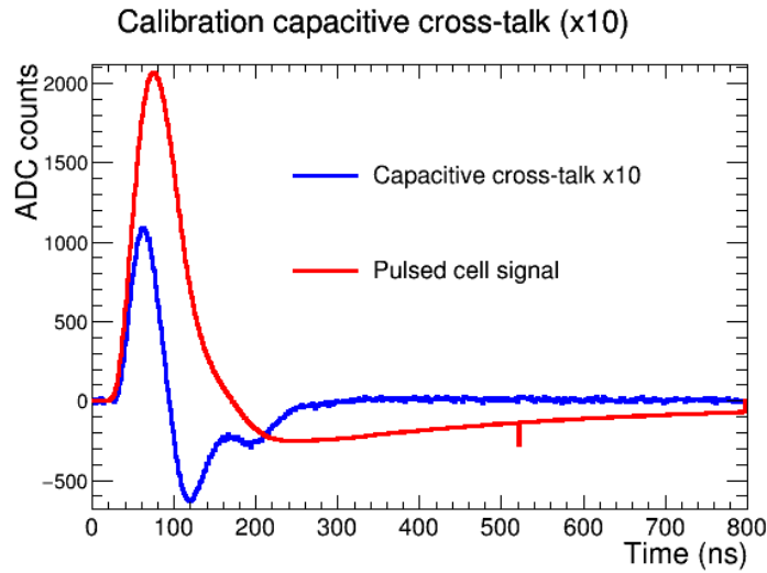
Figure 5.2: Capacitive cross-talk shape obtained from calibration data. A cell is pulsed in the front layer of the EM barrel. The cross-talk shape is retrieved from its closest neighbouring cell in \eta .
