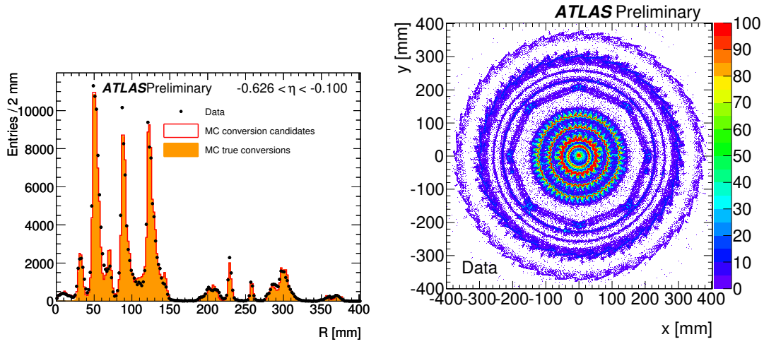
Figure 4.1: Distance to the beamline of reconstructed conversion vertices (left) and spatial distribution of reconstructed conversion vertices (right) in the transverse plane measured on 14\text{nb}^{-1} during June-July 2010 [1].
