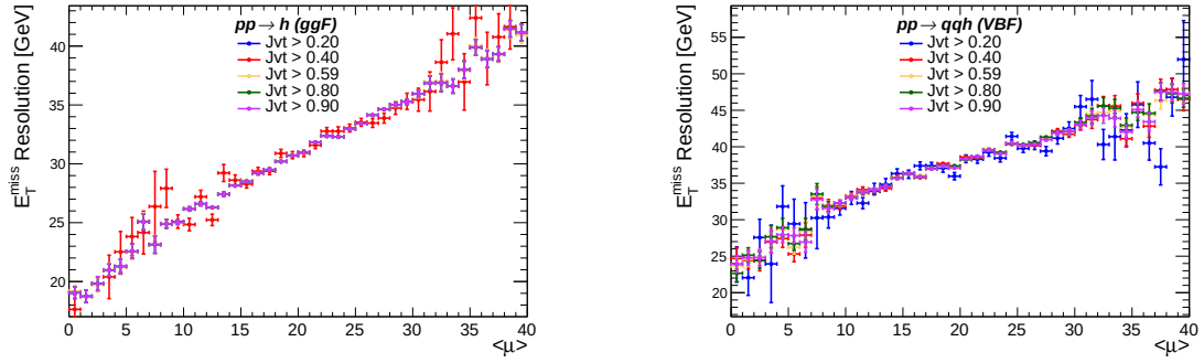
Figure 6.22: Dependence of E_T^{\text{miss}} resolution as a function of the jet-vertex-tagger cut applied to central jets of the event ( 20 \text{ GeV} < p_T < 60 \text{ GeV} , |\eta| < 2.4 ). Resolution is shown versus the average number of interactions per bunch crossing. Truth E_T^{\text{miss}} is subtracted and soft-terms are computed using tracks associated with the diphoton vertex of the event.
