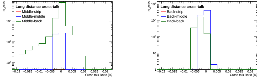
Figure 5.34: Long distance contribution derived on physics cross-talk shapes.
