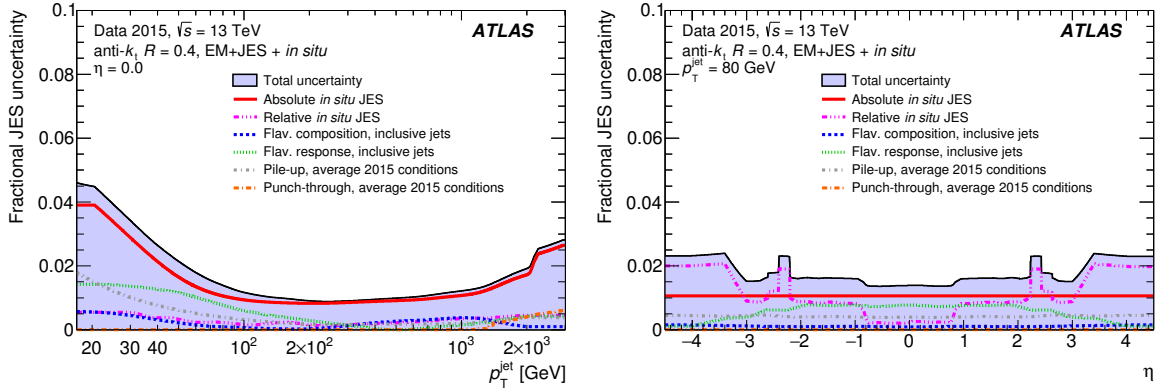
Figure 6.3: Combined uncertainty in the JES of fully calibrated jets as a function of (a) jet p_T at \eta = 0 and (b) \eta at p_T = 80 \text{ GeV} . Absolute in-situ JES corresponds to Z/\gamma +jet and multijet calibrations and relative in-situ calibration corresponds to \eta intercalibration. More systematic errors are presented corresponding to pileup, punch-through (one of the corrections of the GSC step) and jet flavour uncertainties are also included [5].
