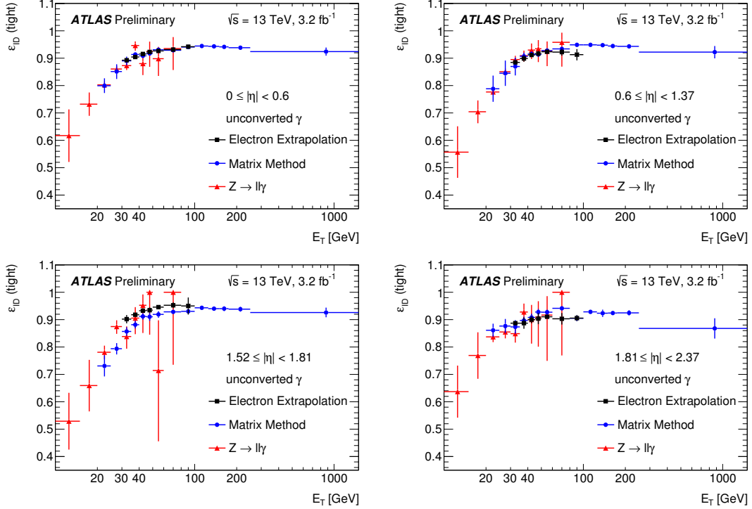
Figure 4.13: Tight identification efficiency for unconverted photons depending on \eta and E_T . Efficiencies are tested using three methods providing similar results.
