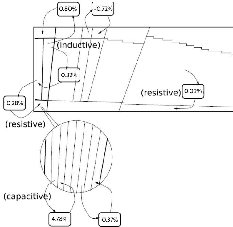
Figure 5.32: Illustration of the obtained cross-talk values obtained on physics signals. Cross-talk and signal energies are estimated using the full calibration chain. OF method uses 5 samples of the signal.
