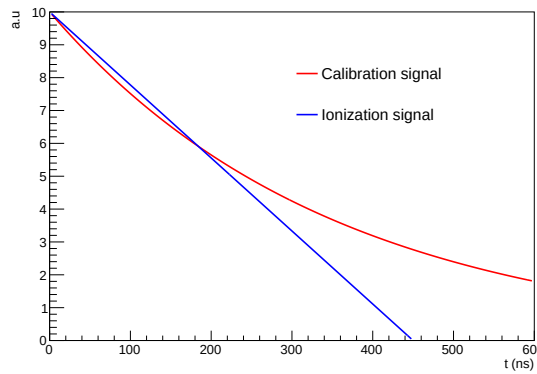
Figure 3.18: Representation of the calibration exponential pulse and ionization triangular signal.
