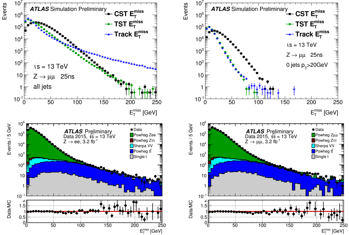
Figure 6.11: E_T^{\text{miss}} distributions using CST, TST and Track- E_T^{\text{miss}} on Z \rightarrow \mu^- \mu^+ MC samples (upper plots) and comparison between TST E_T^{\text{miss}} in 2015 data ( 3.2 \text{ fb}^{-1} ) and MC. Upper left plot presents the distributions considering all events and the upper right plot, considering events with no reconstructed jet [18]. Bottom left plot presents the comparison between data and MC on Z \rightarrow e^- e^+ final state and bottom right plot, on Z \rightarrow \mu^- \mu^+ final state [19].
