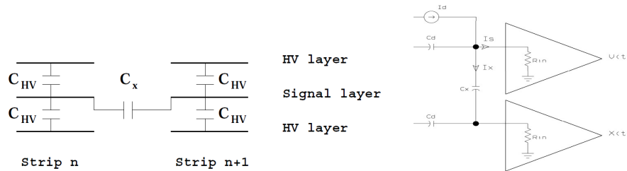
Figure 5.1: (left) Illustration of the capacitive coupling C_x between cells on a single electrode and comparison with the capacitive coupling C_{HV} between the inner layer and the two HV outer layers of the electrode. (right) Readout chain model used to estimate the capacitive coupling signal. In this model, C_d = C_{HV}
