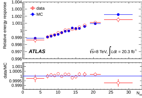
Figure 4.22: Pileup stability of the energy response in data and simulation [2].
