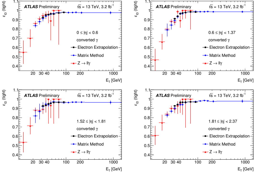
Figure 4.14: Tight identification efficiency for converted photons depending on \eta and E_T . Efficiencies are tested using three methods providing similar results.
