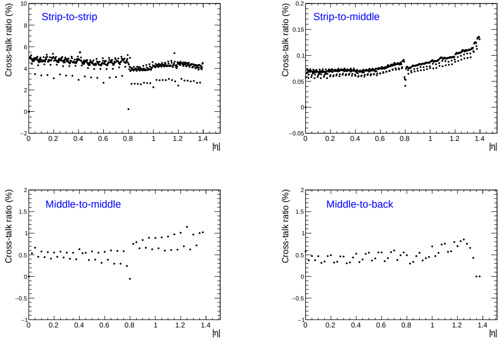
Figure 5.11: Cross-talk magnitude dependence on |\eta| . This magnitude represents the ratio of the cross-talk energy divided by the pulsed cell energy. Both energies are derived using the OF method explained in Section 3.5 where calibration OFCs were applied.
