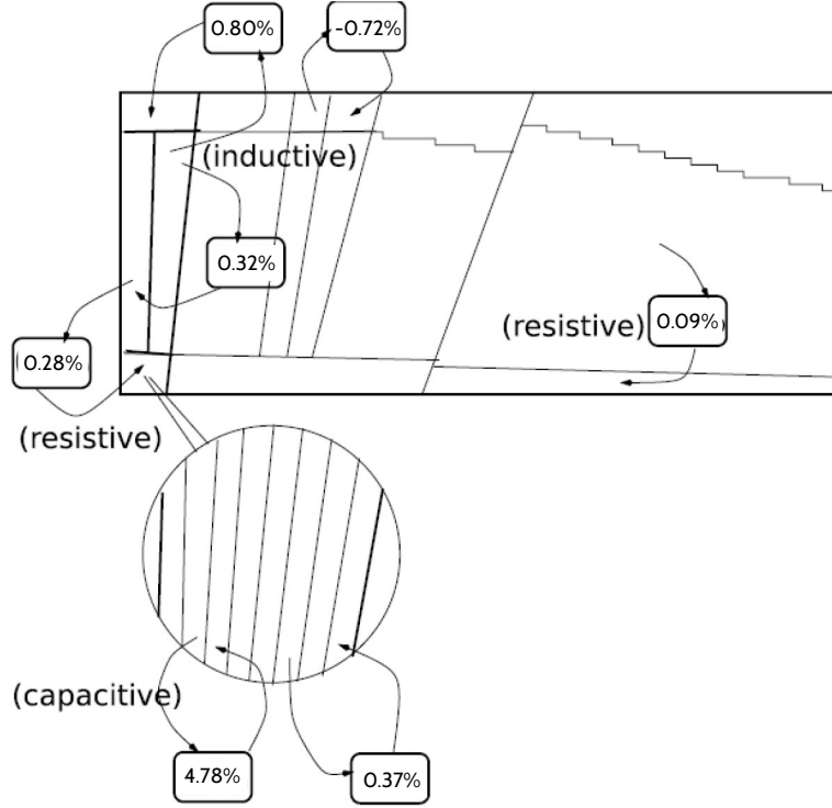
Figure 5.30: Illustration of the obtained cross-talk values obtained on physics signals. Cross-talk and signal energies are estimated using the full calibration chain. OF method uses 4 samples of the signal.
