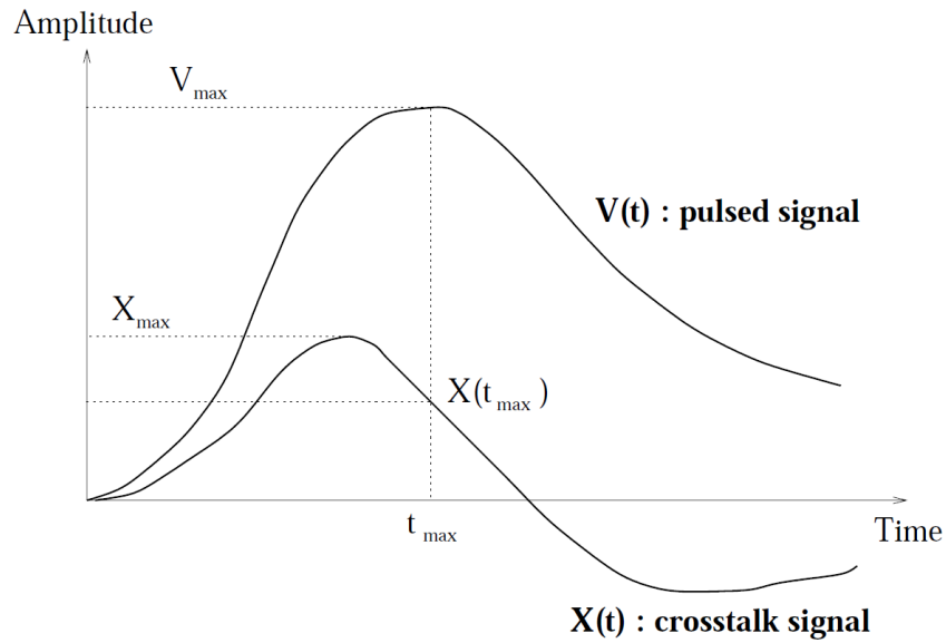
Figure 5.6: Diagram of the related quantities entering the cross-talk determination [4].
