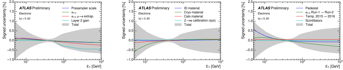
Figure 4.25: Uncertainties for the electron energy calibration using 2015 dataset with 3.2\text{fb}^{-1} total luminosity [18].
