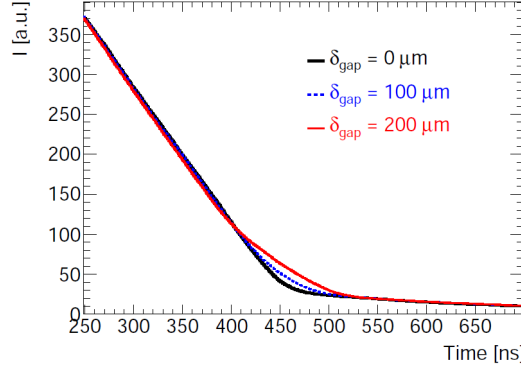
Figure 3.12: Current as a function of time for a perfect centering of the electrode with \delta_{\text{gap}} = 0 \mu\text{m} and \delta_{\text{gap}} = 100 \mu\text{m} and \delta_{\text{gap}} = 200 \mu\text{m} [14].
