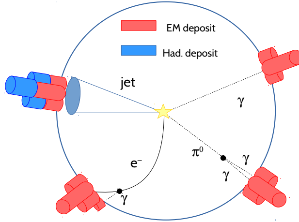
Figure 4.2: Schema of the expected energy deposits for jets, electrons, unconverted photons and neutral pions. Solid (dotted) lines represent tracks that (don't) leave traces in the inner detector. Red color stands for electromagnetic energy deposits in any of the calorimeters while blue color represent hadronic energy deposits.
