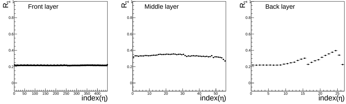
Figure 3.24: Run 00314180: value of R_1 from the fit of the DAC versus ADC distributions in Figure 3.22 with Equation 3.30.
