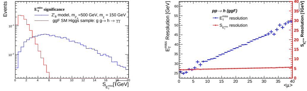
Figure 7.8: Left plot: S_{E_T^{miss}} distributions comparing events from a Z'_B simulated sample ( m_{Z'_B} = 500 GeV and m_\chi = 150 GeV) against events from the ggF SM Higgs simulated sample. It can be observed the discriminating power of this variable between samples presenting genuine E_T^{miss} ( Z'_B sample) or fake E_T^{miss} (ggF sample). Right plot: comparison of the S_{E_T^{miss}} and E_T^{miss} resolution dependence in a ggF SM Higgs sample, where fake E_T^{miss} is expected. Arbitrary units are used given that the aim of this plot is to compare the slope both distributions. It can be observed a higher pileup resilience of the S_{E_T^{miss}} variable than the E_T^{miss} .
