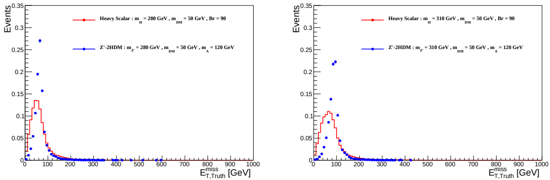
Figure B.2: Comparison of E_T^{\text{miss}} spectrum of Z' -2HDM versus Heavy scalar model for same mediator and DM particle masses ( m'_Z = 280 or 310 GeV, m_\chi = 50 GeV)
