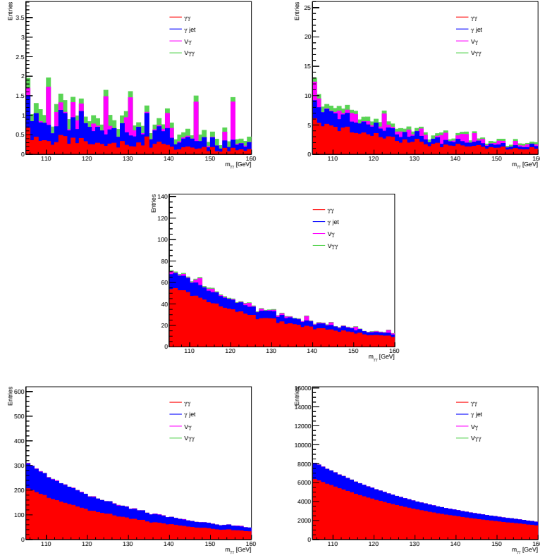
Figure 7.24: Merged non-resonant background distributions. \gamma\gamma contribution is normalized to 79% of number of events in data in the inclusive category and \gamma +jet to 19% following data-driven measurements. V\gamma and V\gamma\gamma contributions are normalized to their predicted cross-section times the 36.1\text{fb}^{-1} luminosity.
