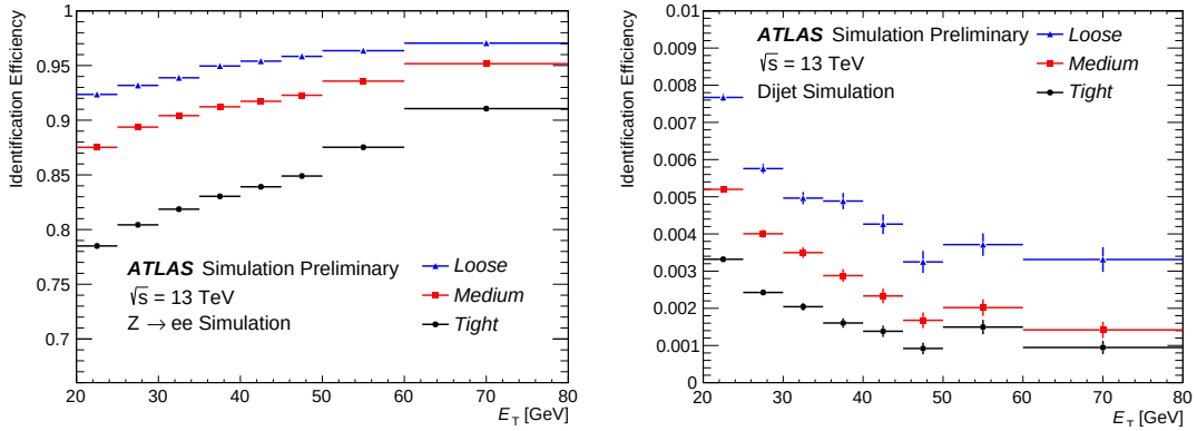
Figure 4.10: The efficiency to identify electrons from Z \rightarrow ee decays (left) and the efficiency to identify hadrons as electrons (background rejection, right) estimated using simulated dijet samples. The efficiencies are obtained using Monte Carlo simulations, and are measured with respect to reconstructed electrons. The candidates are matched to true electron candidates for Z \rightarrow ee events. For background rejection studies the electrons matched to true electron candidates are not included in the analysis [6].
