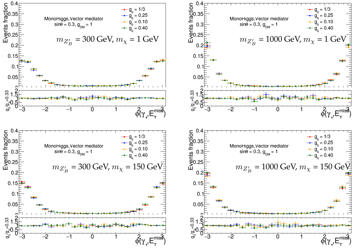
Figure C.3: \Delta\phi(\gamma_1, E_T^{\text{miss}}) distributions of the Z'_B model of four mass points ( m_{Z'_B}, m_\chi ) and four different values of g_q .
