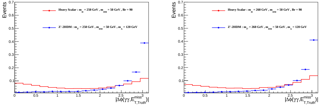
Figure B.14: Comparison of kinematic distributions between Z'-2HDM and Heavy scalar models for the same mediator and DM particle masses ( m'_Z = 250 or 260 GeV, m_\chi = 50 GeV)
