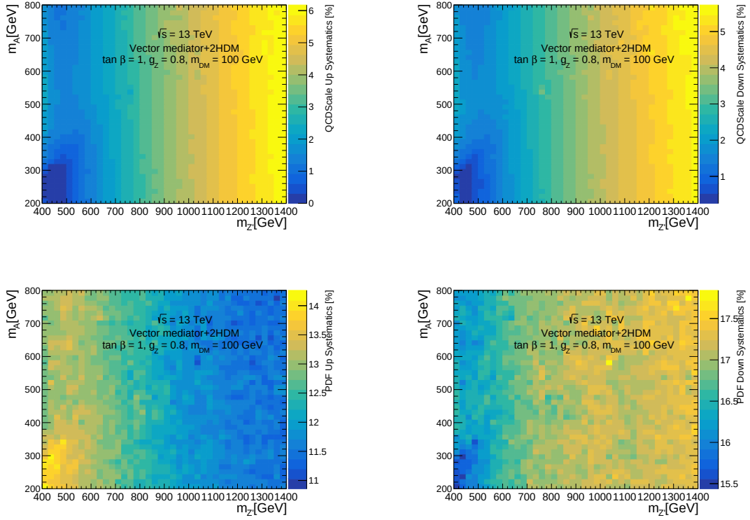
Figure 7.27: QCD (top) and PDF (bottom) systematic relative variation (%) for Z' -2HDM model comparison for different m_A and m_{Z'} .
