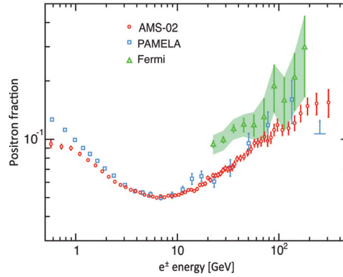
Figure 1.23: Positron excess observed by PAMELA, Fermi-LAT and AMS-02 [101].
