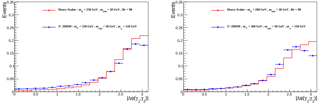
Figure B.10: Comparison of kinematic distributions between Z'-2HDM and Heavy scalar models for the same mediator and DM particle masses ( m'_Z = 250 or 260 GeV, m_\chi = 50 GeV)
