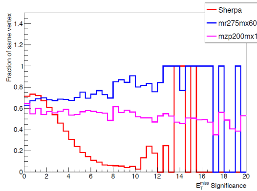
Figure 7.16: Event rate of coincidence between the diphoton vertex and the hardest vertex of the event. Rates as function of the S_{E_T^{\text{miss}}} variable are presented. Red curve correspond to event rates for the diphoton non-resonant background sample while blue and pink curves show event rates for a chosen benchmark sample for the heavy-scalar and Z'_B models, respectively. This demonstrates that the background is reduced when the two vertices coincide.
