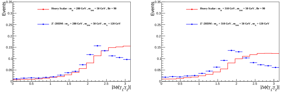
Figure B.11: Comparison of kinematic distributions between Z'-2HDM and Heavy scalar models for the same mediator and DM particle masses ( m'_Z = 280 or 310 GeV, m_\chi = 50 GeV)
