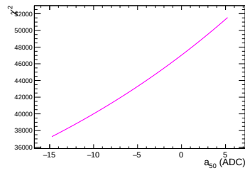
(e) \chi^2 for different a_{50} values
