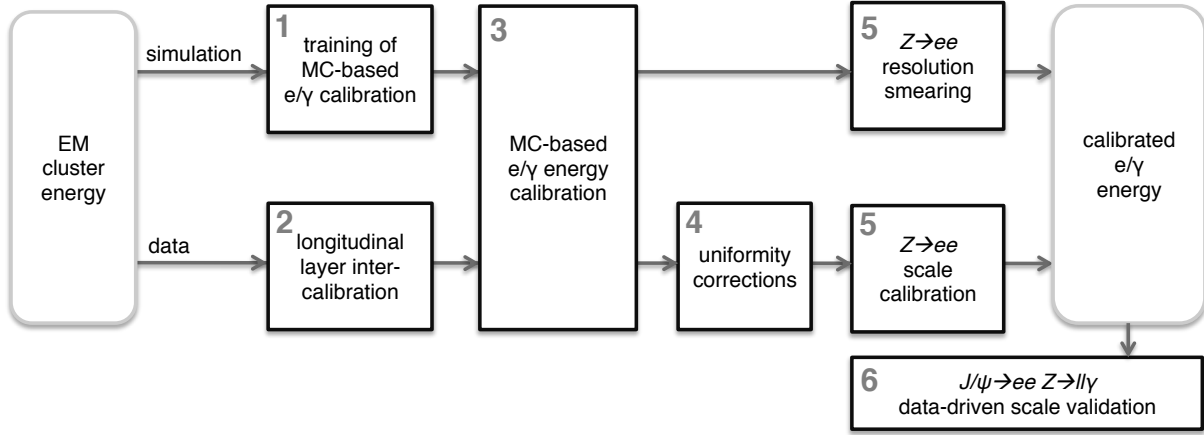
Figure 4.18: Calibration scheme for electrons and photons [2].
