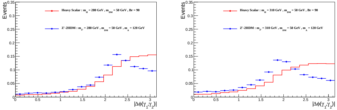
Figure B.13: Comparison of kinematic distributions between Z'-2HDM and Heavy scalar models for the same mediator and DM particle masses ( m'_Z = 280 or 310 GeV, m_\chi = 50 GeV)
