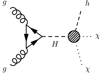
Figure 1.30: Feynman diagrams of the production of DM ( \chi ) in association with a SM-like Higgs boson ( h ) arising from the heavy-scalar model.
