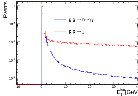
Figure 4.17: Comparison of the corrected ptcone20 isolation transverse energies for photons from the gluon-fusion h \rightarrow \gamma\gamma MC sample and a jj sample, where the photon is faked by a jet.
