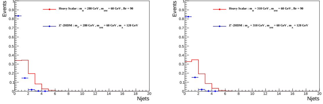
Figure B.21: Comparison of kinematic distributions between Z'-2HDM and Heavy scalar models for the same mediator and DM particle masses ( m'_Z = 280 or 310 GeV, m_\chi = 60 GeV)
