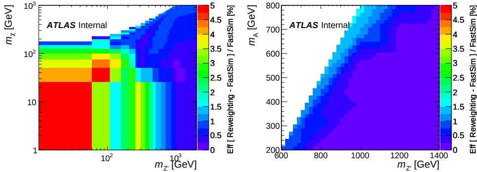
Figure 7.32: Relative differences of selection efficiencies for the Z'_B and Z' -2HDM models computed using a FastSim MC sample or the reweighted base sample as explained in the text.
