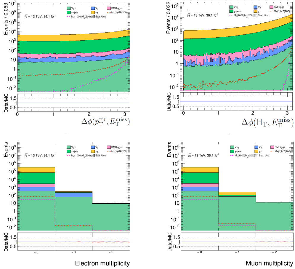
Figure 7.9: Distributions of the \Delta\phi(p_T^{\gamma\gamma}, E_T^{\text{miss}}) (top-left), \Delta\phi(H_T, E_T^{\text{miss}}) (top-right), N_e (bottom-left) and N_\mu (bottom-right) based on simulated samples for signal models, SM Higgs models and non-resonant background.
