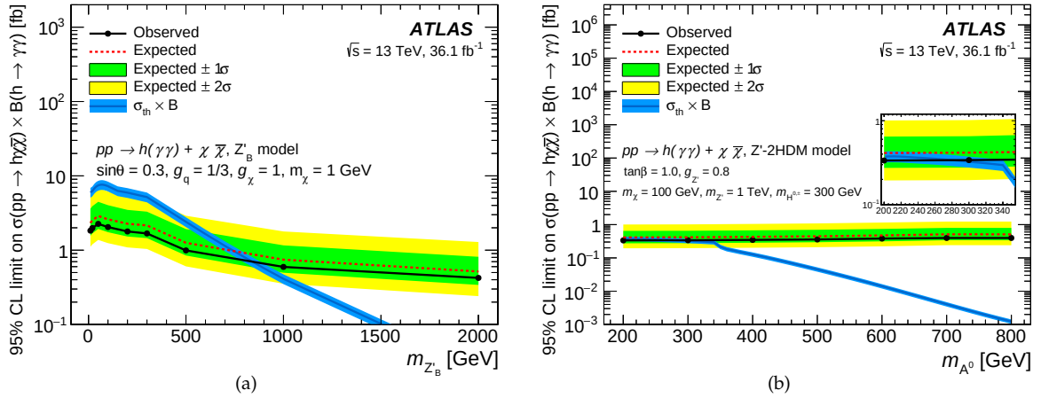
Figure 7.38: Expected (dashed lines) and observed (solid lines) 95% CL upper limits on \sigma(pp \rightarrow h\chi\bar{\chi}) \times \mathcal{B}(h \rightarrow \gamma\gamma) for (a) the Z'_B model for g_q = 1/3 , g_\chi = 1 , \sin \theta = 0.3 and Dirac fermion DM m_\chi = 1 GeV and (b) the Z' -2HDM model for \tan \beta = 1 , g_{Z'} = 0.8 , m_{Z'} = 1000 GeV and Dirac fermion DM m_\chi = 100 GeV, as a function of m_{Z'_B} and m_{A^0} , respectively [3]. The masses of the neutral CP-even scalar ( H^0 ) and the charged scalars ( H^\pm ) from Z' -2HDM model are set to 300 GeV. The theoretical predictions of \sigma(pp \rightarrow h\chi\bar{\chi}) \times \mathcal{B}(h \rightarrow \gamma\gamma) for these two models (dark-blue lines with blue bands representing their associated theoretical systematic uncertainties) are also shown. The inset shows a zoomed-in view of the same figure in narrower ranges of both the x and y axes.
