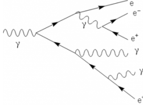
Figure 3.2: Schema of a shower for an incoming photon.
