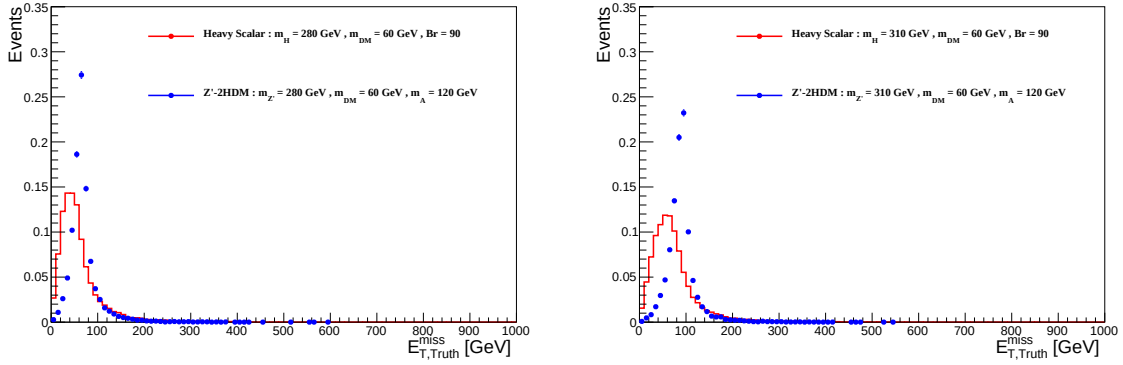
Figure B.4: Comparison of E_T^{\text{miss}} spectrum of Z'-2HDM versus Heavy scalar model for same mediator and DM particle masses ( m'_{Z'} = 280 or 310 \text{ GeV} , m_\chi = 60 \text{ GeV} )
