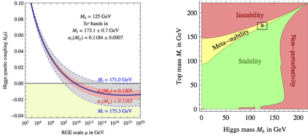
Figure 1.15: Stability of the Higgs potential extrapolated to the Planck scale from [59].
