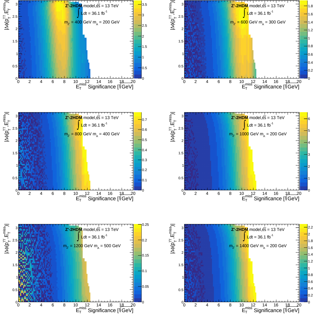
Figure 7.13: Significance scan for various masses of the Z' boson and pseudo-scalar A^0 depending on the S_{E_T^{\text{miss}}} and \Delta\phi(p_T^{\gamma\gamma}, E_T^{\text{miss}}) variables for the Z' -2HDM model. Event weights are applied and signal and background samples are scaled to their corresponding cross-sections or purity ( \gamma\gamma and \gamma +jet).
