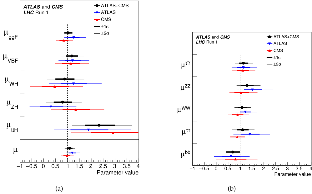
Figure 1.8: Combined measurements of the SM Higgs-like resonance production and decay couplings using 2011-2012 ATLAS+CMS data from LHC Run I at \sqrt{s} = 7 and 8 TeV [55]. All production modes are considered while only b\bar{b} , \gamma\gamma , \tau^+\tau^- , W^\pm W^\mp and ZZ final state branching cross-section \times branching ratios are extracted in units of the SM predictions.
