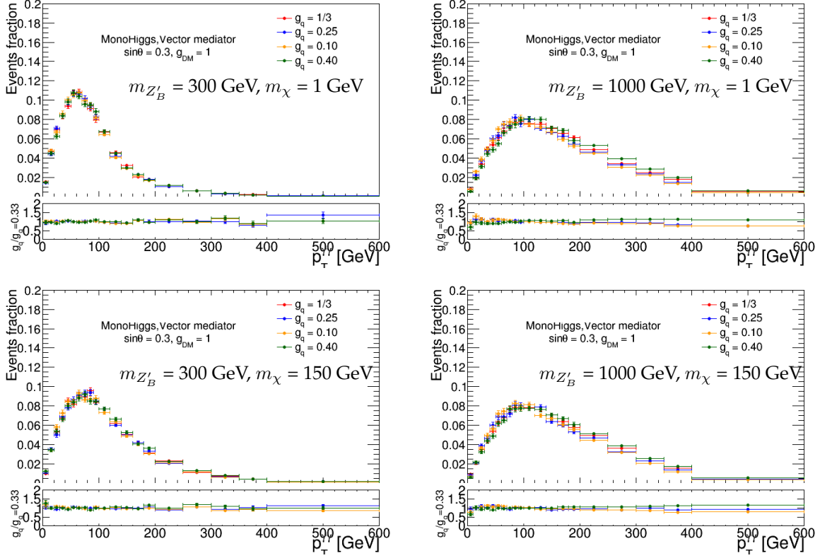
Figure C.1: p_T^{\gamma\gamma} distributions of the Z'_B model of four mass points ( m_{Z'_B}, m_\chi ) and four different values of g_q .
