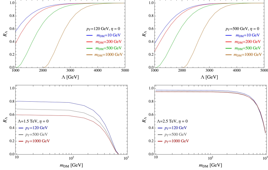
Figure 1.25: The ratio R_\Lambda for \sqrt{s} = 8 TeV at |\eta| = 0 from [102]. A mono-jet EFT is used. These plots show the validity of the EFT depending on the hard-jet p_T and/or m_\chi . It can be observed that EFT is valid only considering large values of \Lambda . For lower values, a part of the generated events presents interactions with Q_{tr} > \Lambda , where predictions are no longer valid.
