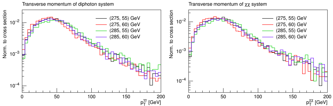
Figure 7.1: Heavy scalar model comparison for several mass points in the [m_H, m_\chi] plane.
