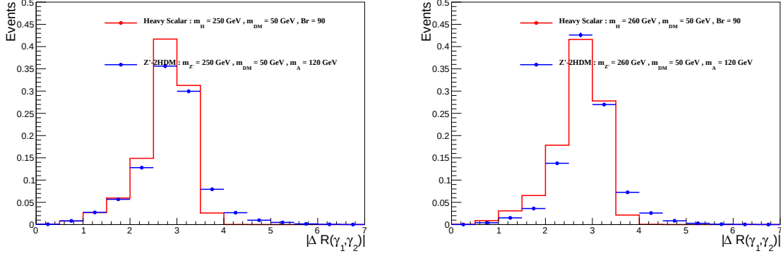
Figure B.6: Comparison of kinematic distributions between Z'-2HDM and Heavy scalar models for the same mediator and DM particle masses ( m'_{Z'} = 250 or 260 GeV, m_\chi = 50 GeV)
