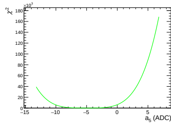
(c) \chi^2 for different a_5 values
