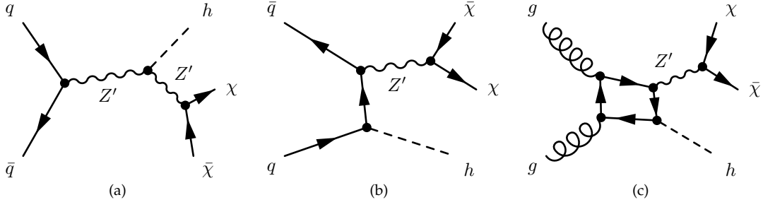
Figure 1.26: Feynman diagrams of the production of DM ( \chi ) in association with a SM-like Higgs boson ( h ) arising from Z'_B models: born process (a); t-channel production of the Z'_B (b); and leading NLO box diagram producing mono-Higgs signals in the final state (c). The latter diagram is not simulated since signal events are produced at leading-order in QCD, as explained in Section 7.1.
