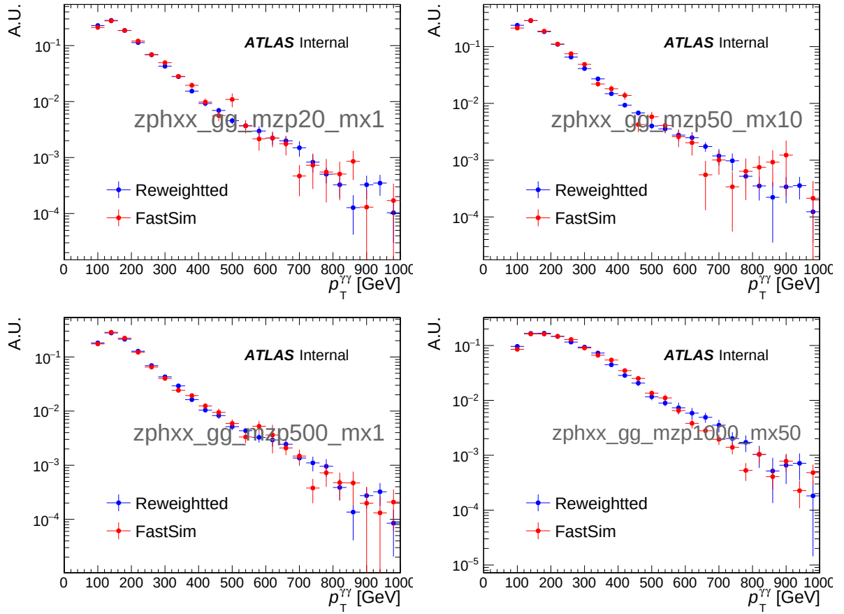
Figure 7.36: Comparison of the diphoton pair transverse energy spectrum obtained either from the reweighted base sample or with a FastSim sample for different points in the parameter space of the Z'_B model
