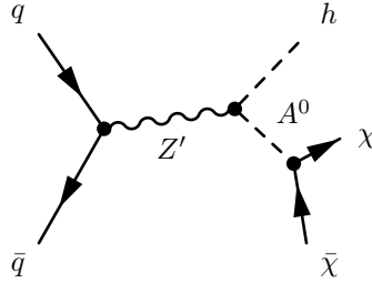
Figure 1.28: Feynman diagrams of the production of DM ( \chi ) in association with a SM-like Higgs boson ( h ) arising from Z' -2HDM model.
