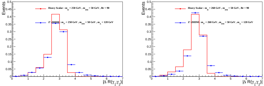
Figure B.5: Comparison of kinematic distributions between Z'-2HDM and Heavy scalar models for the same mediator and DM particle masses ( m'_{Z'} = 250 or 260 \text{ GeV} , m_\chi = 50 \text{ GeV} )
