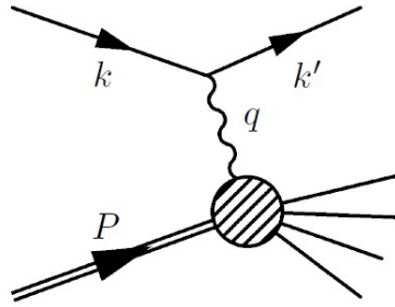
Figure 1.1: Feynman diagram of the Deep Inelastic Scattering process. An electron interacts with a quark inside the proton. The scattered electron energy and angular distributions provide information about the structure inside the proton.
