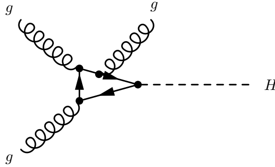
Figure 6.18: Feynman diagram of ggF Higgs production including soft-radiation from t\bar{t} loop that could be rejected by jet selection cuts and introduce a bias in E_T^{\text{miss}} .
