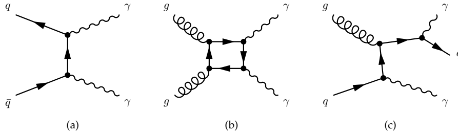
Figure 7.5: Dominant Feynman diagrams of the \gamma\gamma background.
