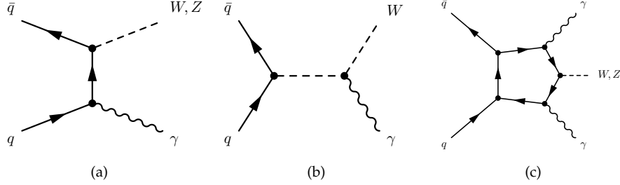
Figure 7.7: Dominant Feynman diagrams of the V\gamma (a,b) and V\gamma\gamma (c) backgrounds.
