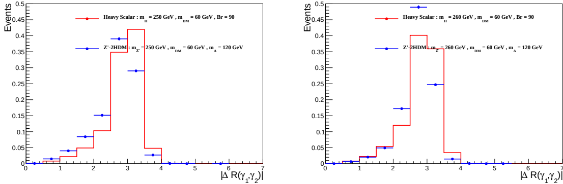
Figure B.8: Comparison of kinematic distributions between Z'-2HDM and Heavy scalar models for the same mediator and DM particle masses ( m'_{Z'} = 250 or 260 GeV, m_\chi = 60 GeV)
