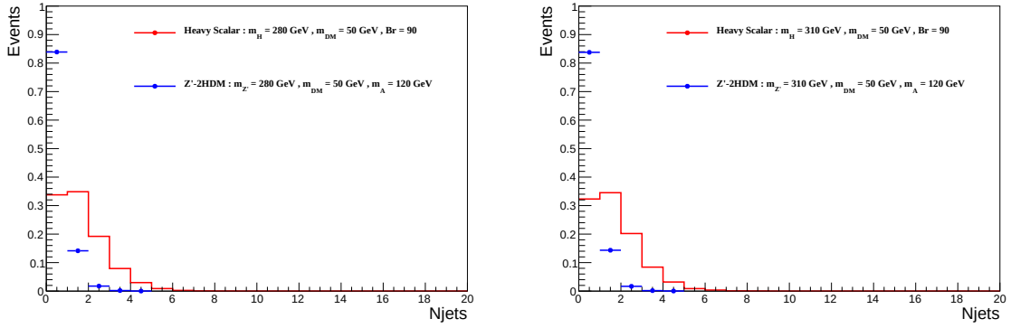
Figure B.19: Comparison of kinematic distributions between Z'-2HDM and Heavy scalar models for the same mediator and DM particle masses ( m'_Z = 280 or 310 GeV, m_\chi = 50 GeV)
