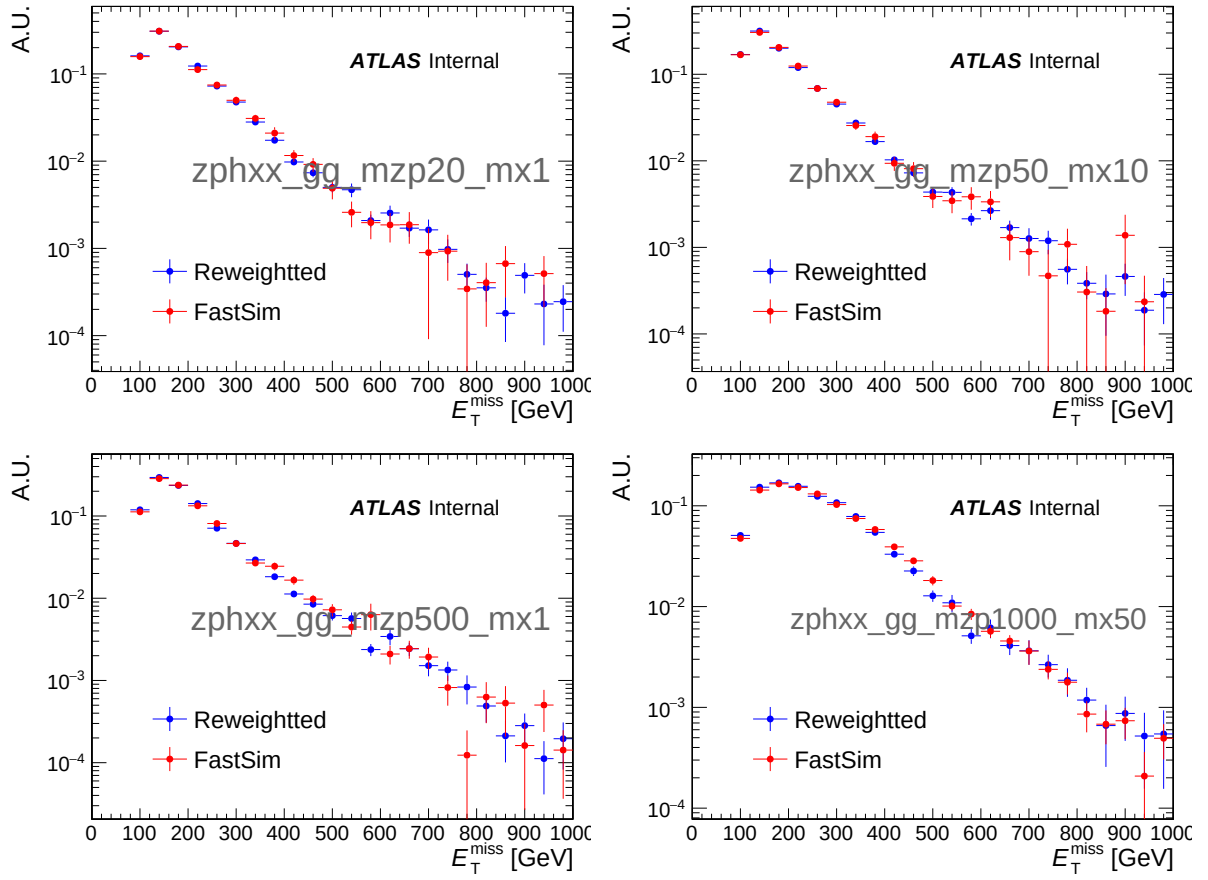
Figure 7.35: Comparison of the MET spectrum obtained either from the reweighted base sample or with a FastSim sample for different points in the parameter space of the Z'_B model
