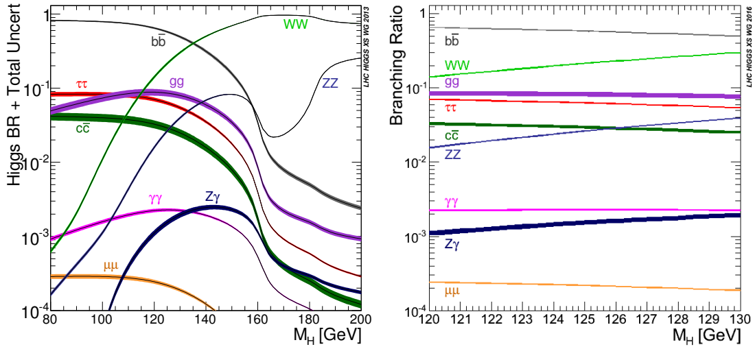
Figure 1.12: Branching ratios of the Standard Model Higgs boson decay modes as a function of the Higgs mass. Left plot shows the mass dependence of the branching ratio inside a region of m_h \in [80, 200] \text{ GeV} and right plot shows this dependence around the combined ATLAS+CMS 2011-2012 Higgs-like resonance mass m_h \approx 125.09 \text{ GeV} [56].
