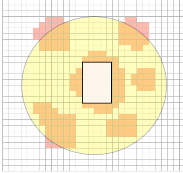
Figure 4.15: Schema of the topoetcone variable: the grid represents the middle calorimeter cells in the \eta and \phi directions. The electron or photon is located in the center of the yellow cone representing the isolation cone. Topological clusters are represented in red. Those whose barycenter falls into the isolation cone are included in the isolation computation. The 5 \times 7 cells white rectangle corresponds to the subtracted core cells. Energy around this core corresponds to the energy leakage that needs to be corrected [13].
