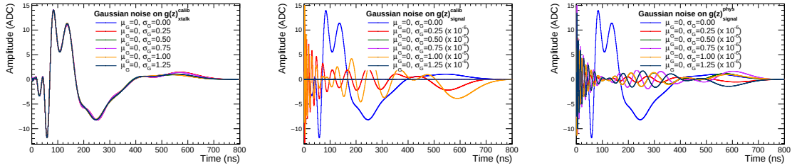
Figure 5.17: g(t)_{\text{xtalk}}^{\text{phys}} estimated using the matrix inversion method. Left plot presents the obtained signal when a gaussian noise centered at zero and with varying \sigma is added to all terms of g(t)_{\text{xtalk}}^{\text{calib}} . Center and right plots present instead the obtained physics cross-talk shape when the gaussian noise is applied to g(z)_{\text{direct}}^{\text{calib}} or g(z)_{\text{direct}}^{\text{phys}} , respectively.
