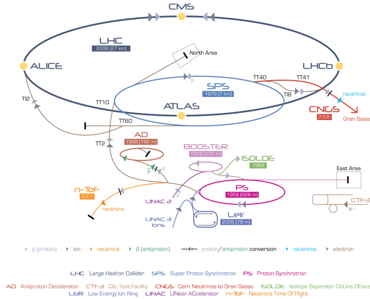
Figure 2.3: CERN acceleration complex [10].
