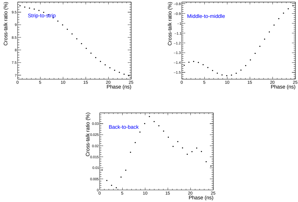
Figure 5.33: Sampling phase dependence of cross-talk magnitude.
