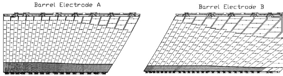
Figure 5.3: Layout of the resistors on the HV layer for the Electrode A and Electrode B of the LAr EM barrel [3].
