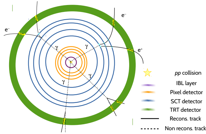
Figure 4.6: Picture illustrating the three track pairs that can be used to reconstruct conversion vertices. The rightmost pair represents Si-Si tracks; the bottom right pair represents TRT-TRT tracks and the last one, Si-TRT tracks. In addition, the bottom left photon presents two tracks from which one escapes detection (single-track conversion vertex).
