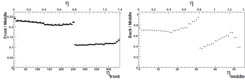
Figure 5.7: Gain factors ratio (MeV / ADC ) between front and middle layers (left) and back and middle layers (right) [8].
