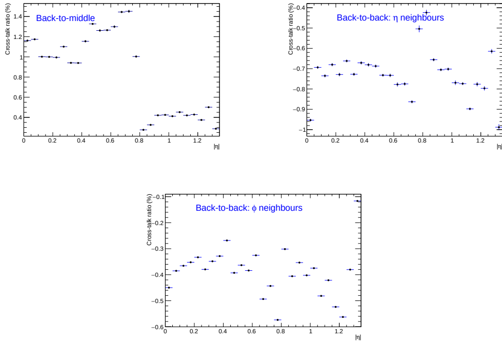
Figure 5.29: Cross-talk magnitude as a function of \eta with pulsed cells in the back layer. Distributions between the same layer have been divided into the cross-talk contribution between adjacent cells in \phi , with \Delta\eta = 0 and adjacent cells in \eta , with \Delta\phi = 0 .
