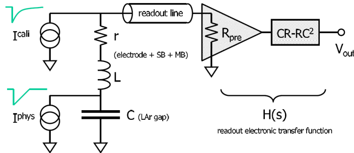
Figure 3.19: Basic equivalent circuit of the liquid argon detector cell readout [17].
