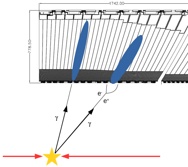
Figure 3.5: Schematic view of the effect that interactions upstream the calorimeter may present in the lateral shower development of two photons. The yellow star indicates the collision point. Red arrows present the two opposite bunches of protons and dark blue ellipses represent the shower of the incoming photons.
