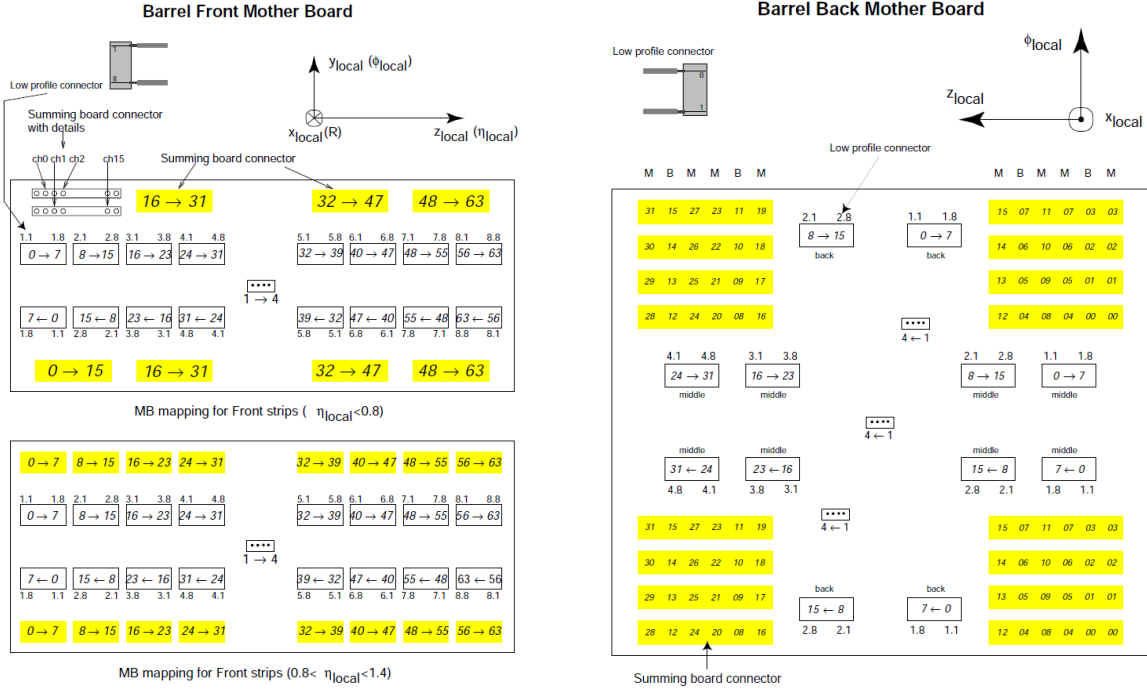
Figure 3.13: Front (left) and back (right) mother boards for the LAr barrel. Numbers on the connectors are attributed to each cell depending on their position [15].
