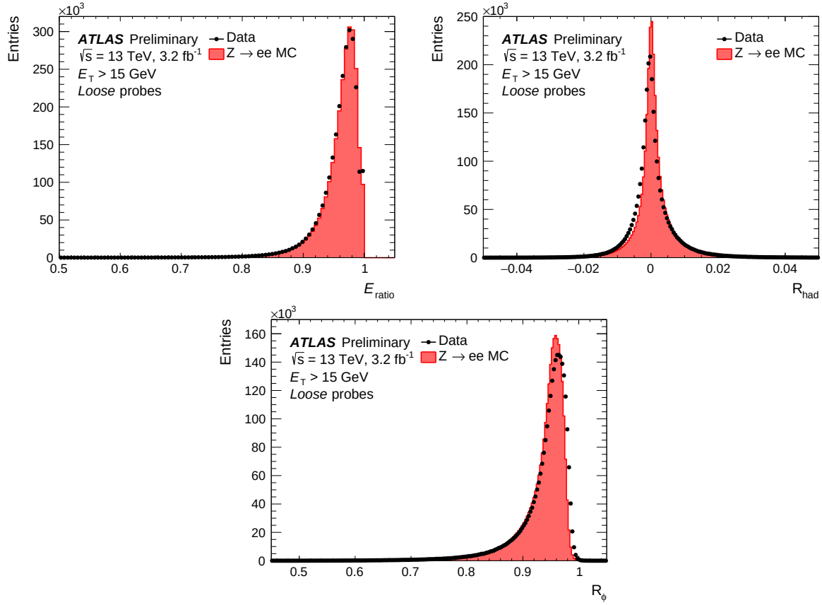
Figure 5.36: Distributions of variables ( E_{\text{ratio}} , R_{\text{had}} and R_{\phi} ) used in the electron identification. They are measured using a tag-and-probe method on Z \rightarrow ee samples for probes passing the electron loose identification [15].
