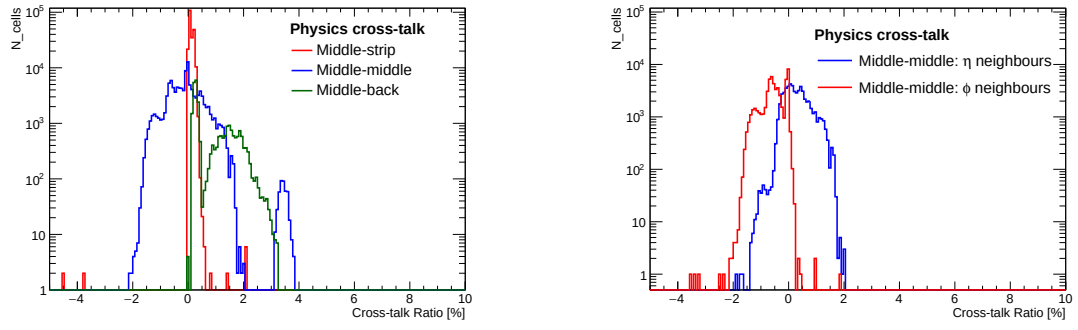
Figure 5.26: Left: distributions of the cross-talk ratios between pulsed cells in the middle layer and cells in the front, middle and back layers. Right: distribution of the cross-talk ratios between pulsed cells in the middle layer and their adjacent cells in \eta and \phi .
