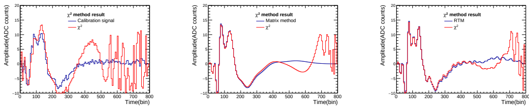
Figure 5.19: \chi^2 method output using an initial shape: left figure, calibration signal; center figure, using the physics cross-talk output of the matrix method; and right figure, using the physics shape from applying RTM method.
