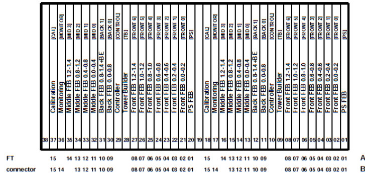
Figure 3.15: Boards distribution in the front-end crates for the barrel [15]
