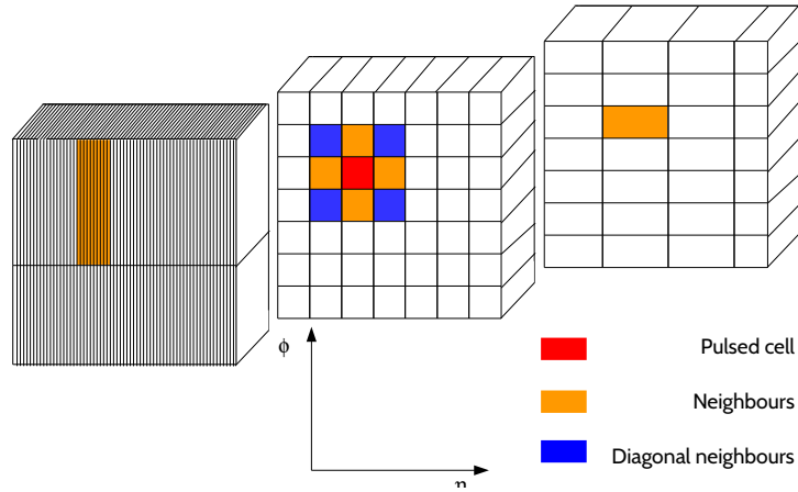
Figure 5.23: Illustration of the neighbours (orange) to a pulsed cell (red) assumed to receive a sizeable cross-talk contribution. Diagonal neighbours (blue) are not considered to receive cross-talk in this study.
