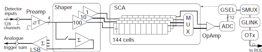
Figure 3.16: Diagram of the FEB architecture [8].
