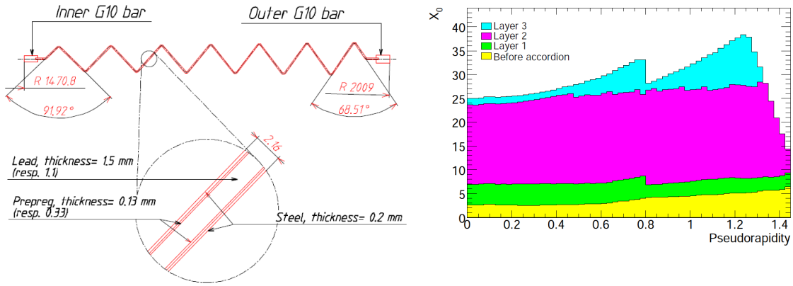
Figure 3.10: Left: schema of the absorber bending angle and composition [3]. Right: cumulative amount of material found by particles traversing the detector expressed as radiation lengths X_0 [8]. It can be observed an increase of the cumulative material in the EM calo with \eta . It can be observed the lead thickness change at \eta = 0.8 .
