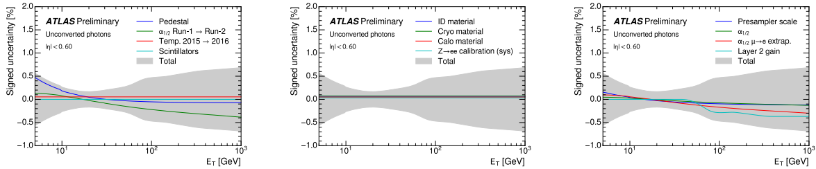
Figure 4.26: Uncertainties for the unconverted photons energy calibration using 2015 dataset with 3.2\text{fb}^{-1} total luminosity [18].
