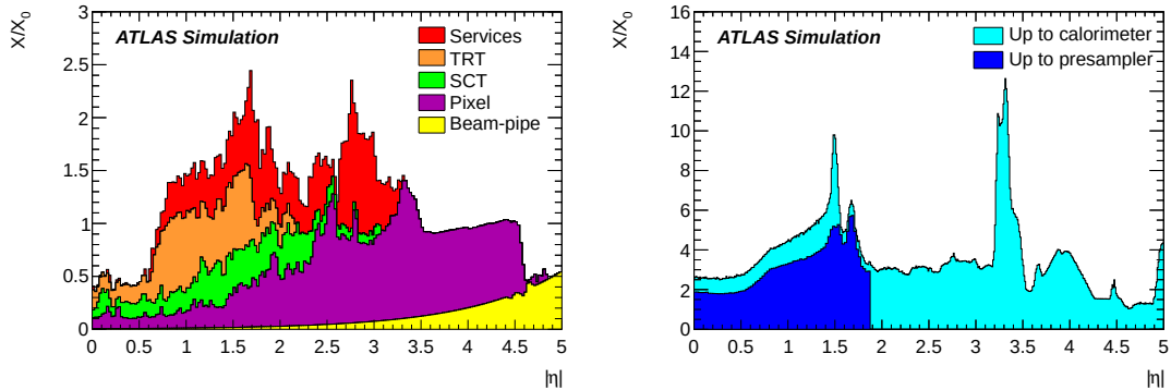
Figure 4.3: Material traversed by a particle in the ID (left) and the calorimeter (right) as a function of the pseudorapidity [2].
