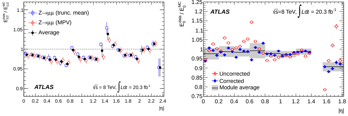
Figure 4.19: Energy scales \alpha_{1/2} and \alpha_{PS} values depending on \eta for Run I [2]. Presented \alpha_{1/2} values are derived using two methods for estimating Z \rightarrow \mu\mu mean deposited energy in the first and second layer (fitting to a Landau or truncated mean of the distribution). \alpha_{PS} values are presented before and after correcting the presampler energy in MC from passive material mismodeling.
