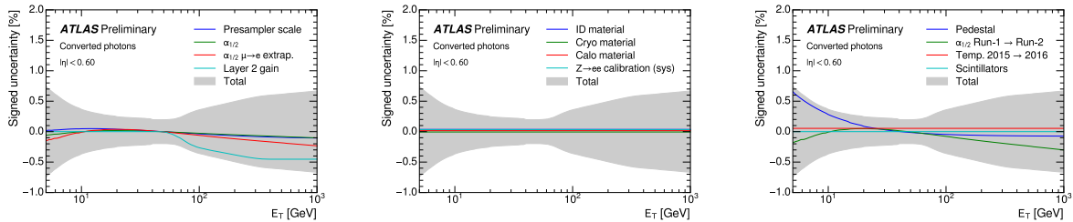
Figure 4.27: Uncertainties for the converted photons energy calibration using 2015 dataset with 3.2\text{fb}^{-1} total luminosity [18].
