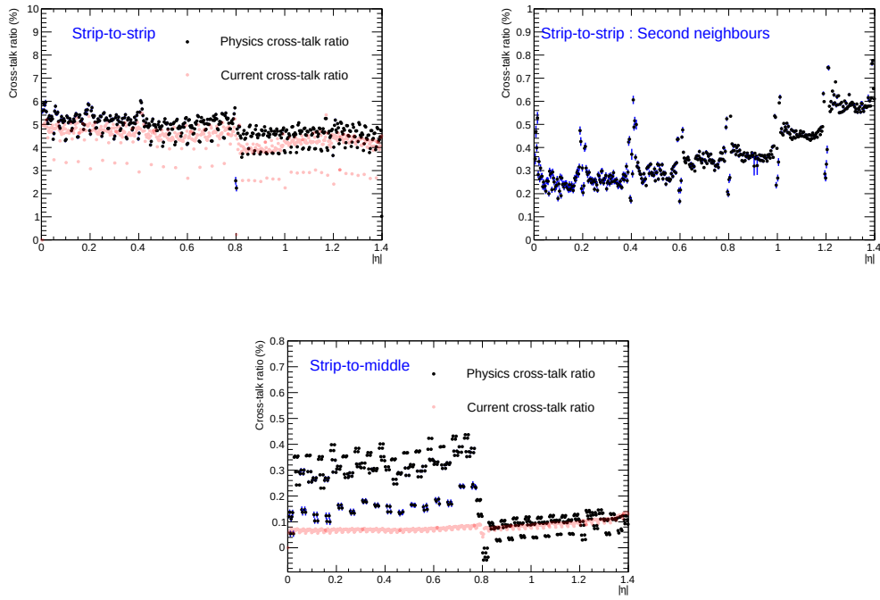
Figure 5.25: Cross-talk magnitude as a function of \eta with pulsed cells in front layer. Therefore, the strip-to-strip contribution corresponds to the cross-talk between adjacent cells in \eta . In addition, the cross-talk between strips separated by two cells in \eta is presented. Strip-to-middle contribution is evaluated between a pulsed strip and its corresponding middle cells. Distributions with calibration cross-talk results are overlaid.
