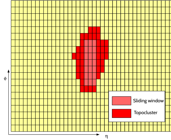
Figure 4.4: Schema of the calorimeter cells introduced in sliding-window and topocluster algorithms.
