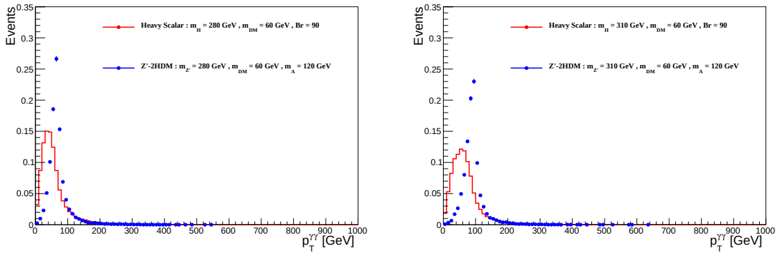
Figure B.25: Comparison of kinematic distributions between Z'-2HDM and Heavy scalar models for the same mediator and DM particle masses ( m'_Z = 280 or 310 GeV, m_\chi = 60 GeV)
