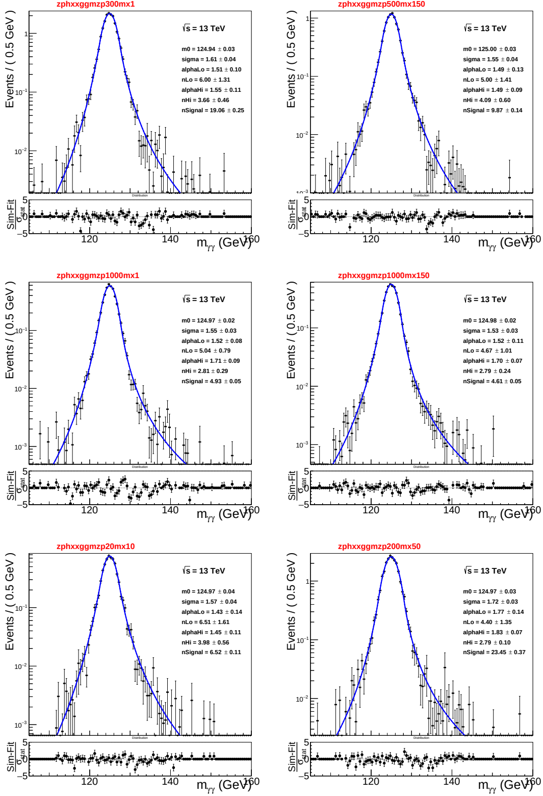
Figure 7.20: Fitted diphoton mass spectra of some Z'_B signals in the mono-Higgs category.
