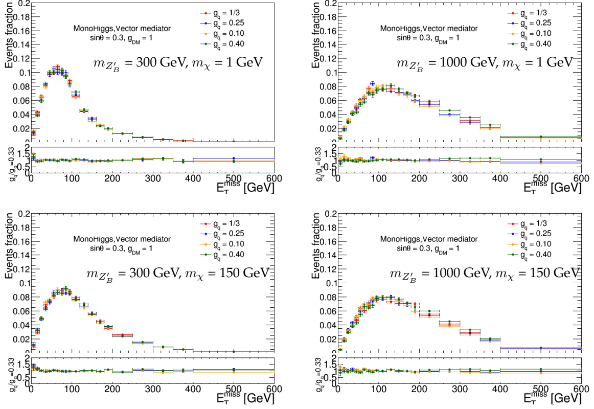
Figure C.2: E_T^{\text{miss}} distributions of the Z'_B model of four mass points ( m_{Z'_B}, m_{\chi} ) and four different values of g_q .
