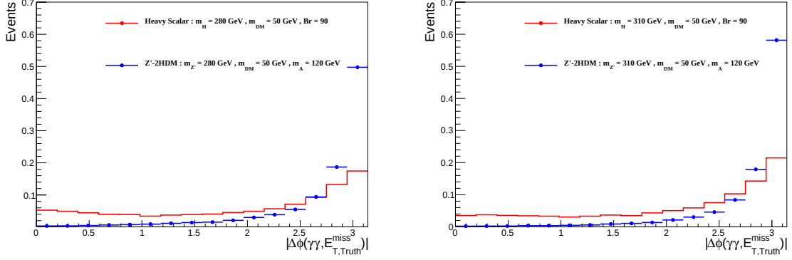
Figure B.15: Comparison of kinematic distributions between Z'-2HDM and Heavy scalar models for the same mediator and DM particle masses ( m'_Z = 280 or 310 GeV, m_\chi = 50 GeV)
