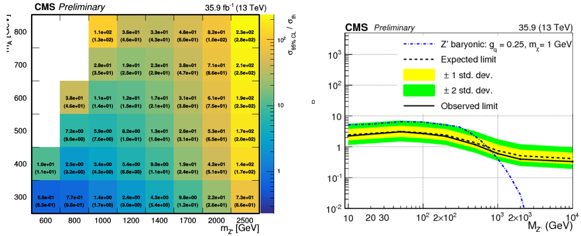
Figure 7.48: The observed (expected) 95% CL limits on the signal strength ( \sigma_{95\%CL}/\sigma_{th} ) for all Z' -2HDM mass points shown in a grid of m_{Z'} and m_{A^0} . Regions presenting values lower than 1 can be considered excluded by the analysis. The theoretical cross-section for each point is calculated assuming g_{Z'} = 0.8 . Right: 95 % CL upper limits on cross-section for the baryonic Z' scenario as a function of m_{Z'} for m_\chi = 1 GeV. The theoretical cross-section (blue) is calculated assuming g_q = 0.25 and \sin\theta = 0.3 [62].
