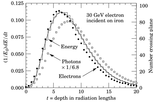
Figure 3.6: Simulation of a 30 GeV electron-induced cascade in iron. It is shown the fraction of energy deposited in the iron per radiation length. The curve is a gamma-function fit to the distribution for electrons. Circles indicate the number of electrons with total energy greater than 1.5 MeV crossing planes at X_0/2 intervals (scale on right) and the squares the number of photons with E \geq 1.5 MeV crossing the planes (scaled down to have the same area as the electron distribution). This figure is taken from [6].
