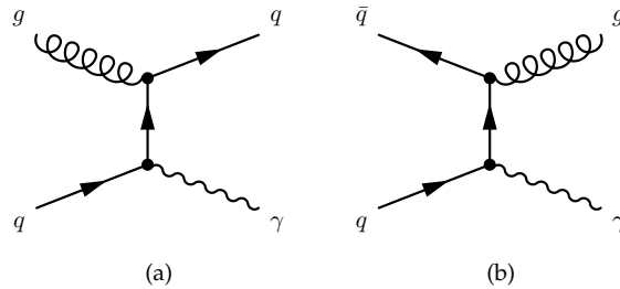
Figure 7.6: Dominant Feynman diagrams of the \gamma j background.
