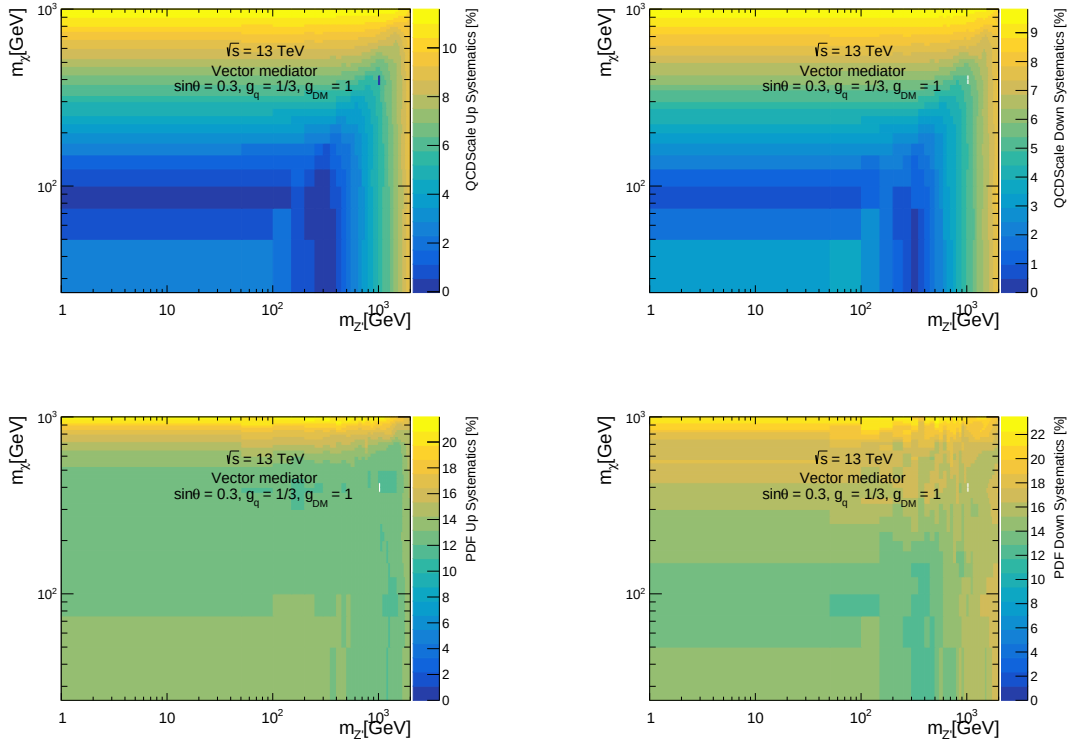
Figure 7.26: QCD (top) and PDF (bottom) systematic relative variation (%) for Z'_B model comparison for different DM mass and m_{Z'_B} .
