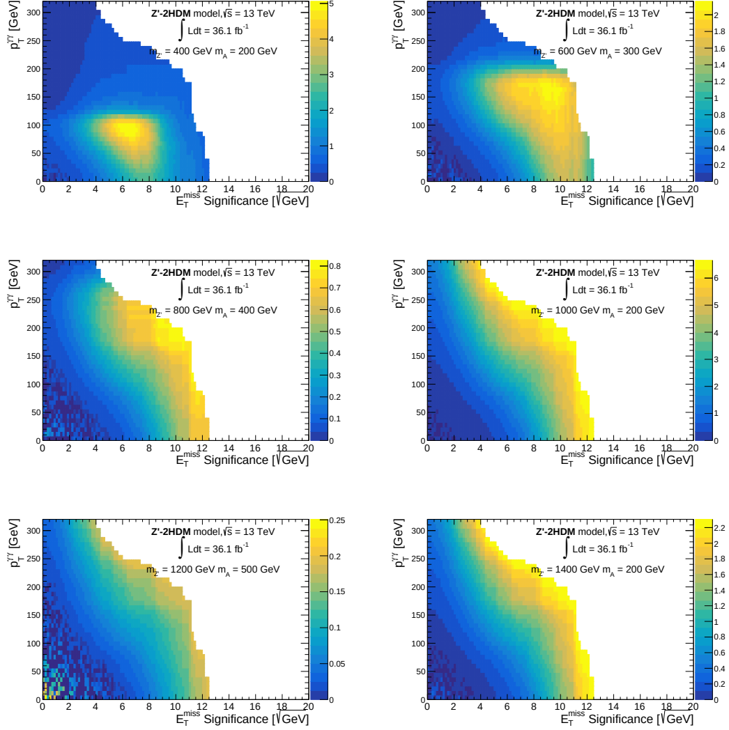
Figure 7.11: Significance scan for various masses of the Z' boson and pseudo-scalar A^0 depending on the S_{E_{\text{miss}}} and p_{\text{T}}^{\gamma} variables for the Z' -2HDM model. Event weights are applied and signal and background samples are scaled to their corresponding cross-sections or purity ( \gamma\gamma and \gamma +jet).
