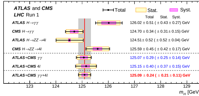
Figure 1.7: Individual and combined values of the SM Higgs-like resonance using 2011-2012 ATLAS+CMS data at \sqrt{s} = 7 and 8 TeV [54]. h \rightarrow \gamma\gamma and h \rightarrow 4\ell are used because they offer the best mass resolution. Mass measurements are performed allowing strength parameters for selected production and decay modes to vary in the fit. It is done in order to obtain a mass measurement as independent as possible of SM assumptions. The red vertical line and the gray shaded column indicate the central value and the total uncertainty of the combined measurement.
