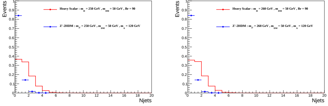
Figure B.18: Comparison of kinematic distributions between Z'-2HDM and Heavy scalar models for the same mediator and DM particle masses ( m'_Z = 250 or 260 GeV, m_\chi = 50 GeV)
