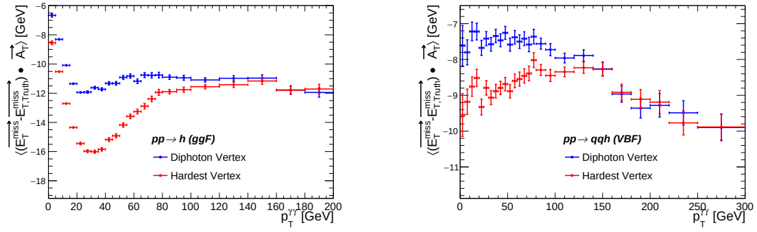
Figure 6.20: Reconstructed E_T^{\text{miss}} distributions subtracted from truth information for different Higgs production. TST reconstruction is compared to soft-terms either associated with the hardest vertex or to the diphoton vertex of the event.
