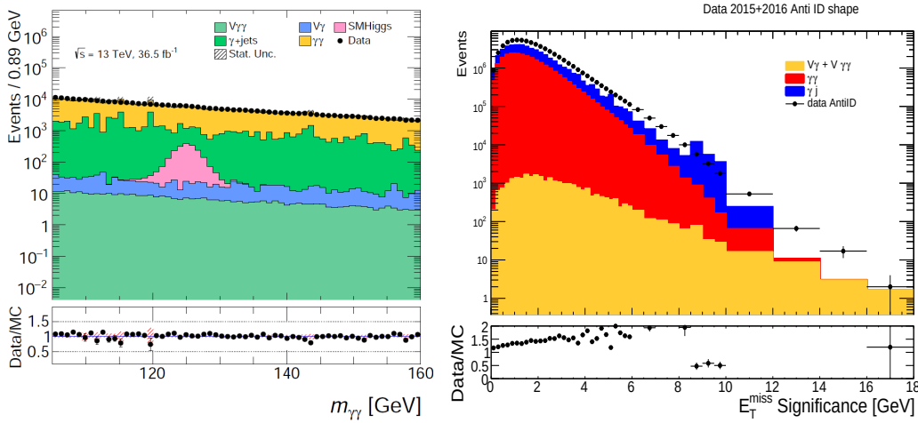
Figure 7.23: Comparison of Pythia8 \gamma +jet sample in the signal (left) and the control region (right). One can clearly observe that large fluctuations are present in this sample due to bad MC modeling. \gamma\gamma , V\gamma and V\gamma\gamma MC contributions are also included in both plots. Control region plot shows the S_{E_T^{\text{miss}}} distribution since contribution of the \gamma +jet is extracted from this variable.
