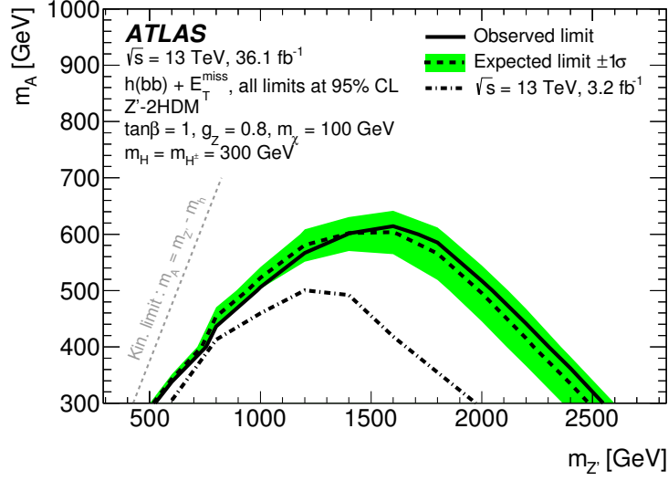
Figure 7.45: Exclusion contours for the Z' -2HDM scenario in the (m_{Z'}, m_{A^0}) plane for \tan\beta = 1 , g_{Z'} = 0.8 , and m_\chi = 100 GeV. The observed limits (solid line) are consistent with the expectation under the SM-only hypothesis (dashed line) within uncertainties (filled band). Observed limits from previous ATLAS results at \sqrt{s} = 13 TeV (dash-dotted line) [31] are also shown. [59]
