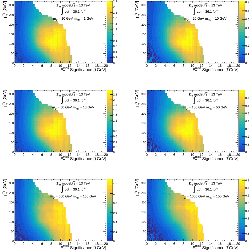
Figure 7.10: Significance scan for various masses of the Z'_B boson and DM particle depending on the S_{E_T^{\text{miss}}} and p_T^{\gamma\gamma} variables for the Z'_B model. Event weights are applied and signal and background samples are scaled to their corresponding cross-sections or purity ( \gamma\gamma and \gamma +jet).
