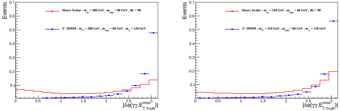
Figure B.17: Comparison of kinematic distributions between Z'-2HDM and Heavy scalar models for the same mediator and DM particle masses ( m'_Z = 280 or 310 GeV, m_\chi = 60 GeV)
