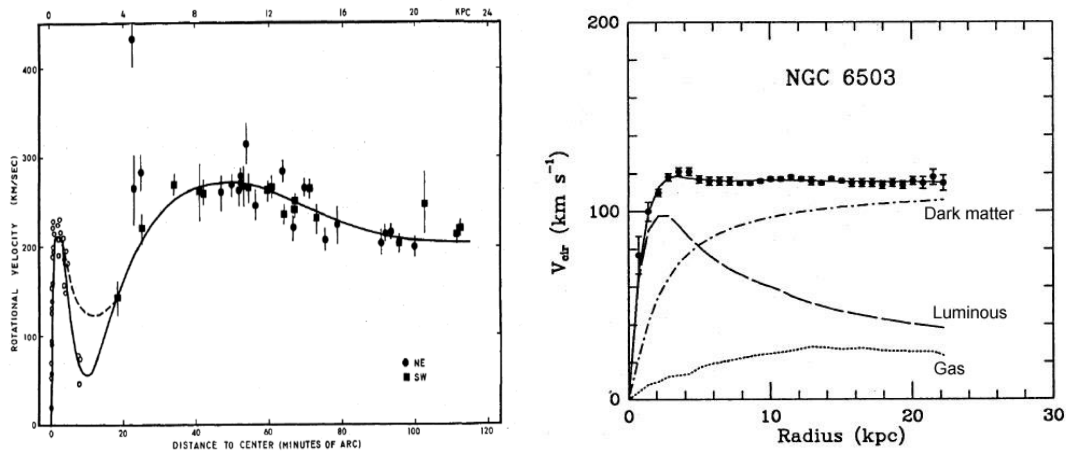
Figure 1.16: Rotational curves for (a) Andromeda galaxy, presented by Vera Rubin and Kent Ford in their article [73]; and (b) of the galaxy NGC 6503 [75]. Both galaxies are spiral.
