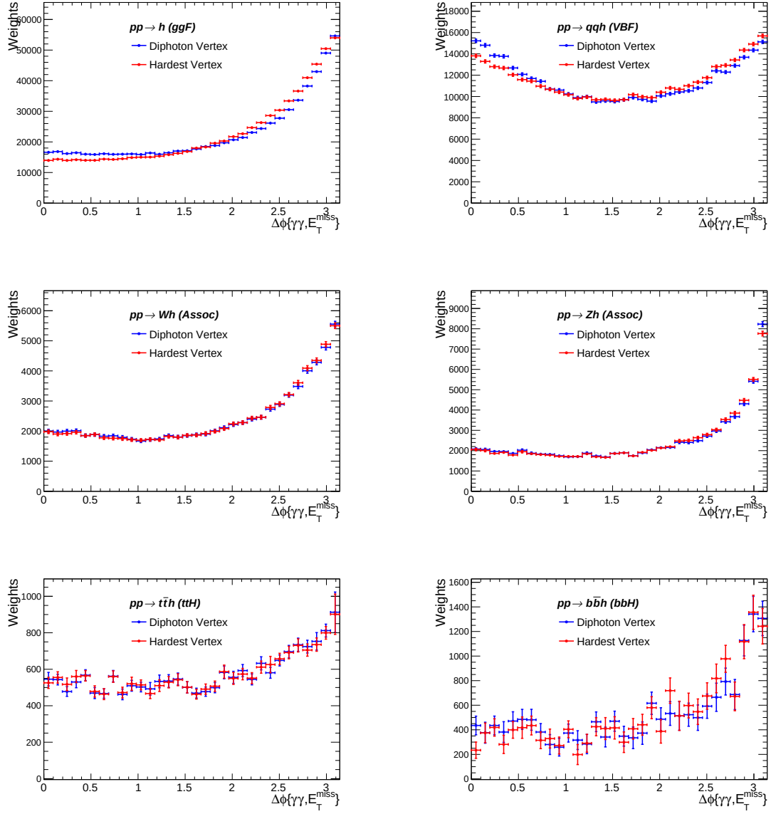
Figure 6.23: Distributions of the relative azimuthal angle between the diphoton transverse momentum and the E_T^{\text{miss}} either computed from either hard or diphoton vertex TST E_T^{\text{miss}} . No truth information is subtracted.
