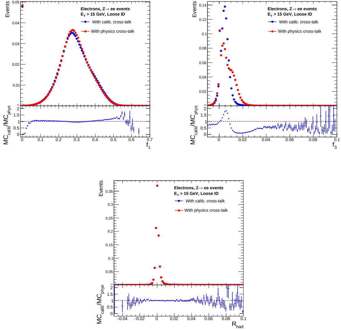
Figure 5.38: Distributions of variables ( R_{had} , f_1 and f_3 ) used in the electron identification. Measured on Z \rightarrow ee events simulated without any pileup effects. Electrons are required to pass loose identification and to present E_T > 15 GeV and |\eta| < 1.475 . Calibration cross-talk stands for the current cross-talk values introduced in the simulation (Table 5.1) and the physics cross-talk estimated using 4 samples (Table 5.2).
