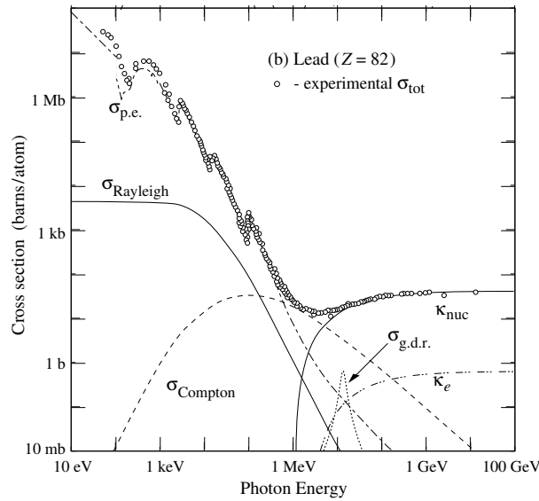
Figure 3.4: Photon total cross-sections as a function of energy in lead, showing the contributions of different processes [6], where the different cross-sections are: \sigma_{p.e.} , the atomic photoelectric effect cross-section; \sigma_{\text{Rayleigh}} for Rayleigh scattering-atom; \sigma_{\text{Compton}} stands for Compton scattering off an electron cross-section; \kappa_{\text{nuc}} accounts for the pair e^+e^- production by nuclear field and \kappa_e by the electron field; and \sigma_{g.d.r.} accounts for photonuclear interactions.
