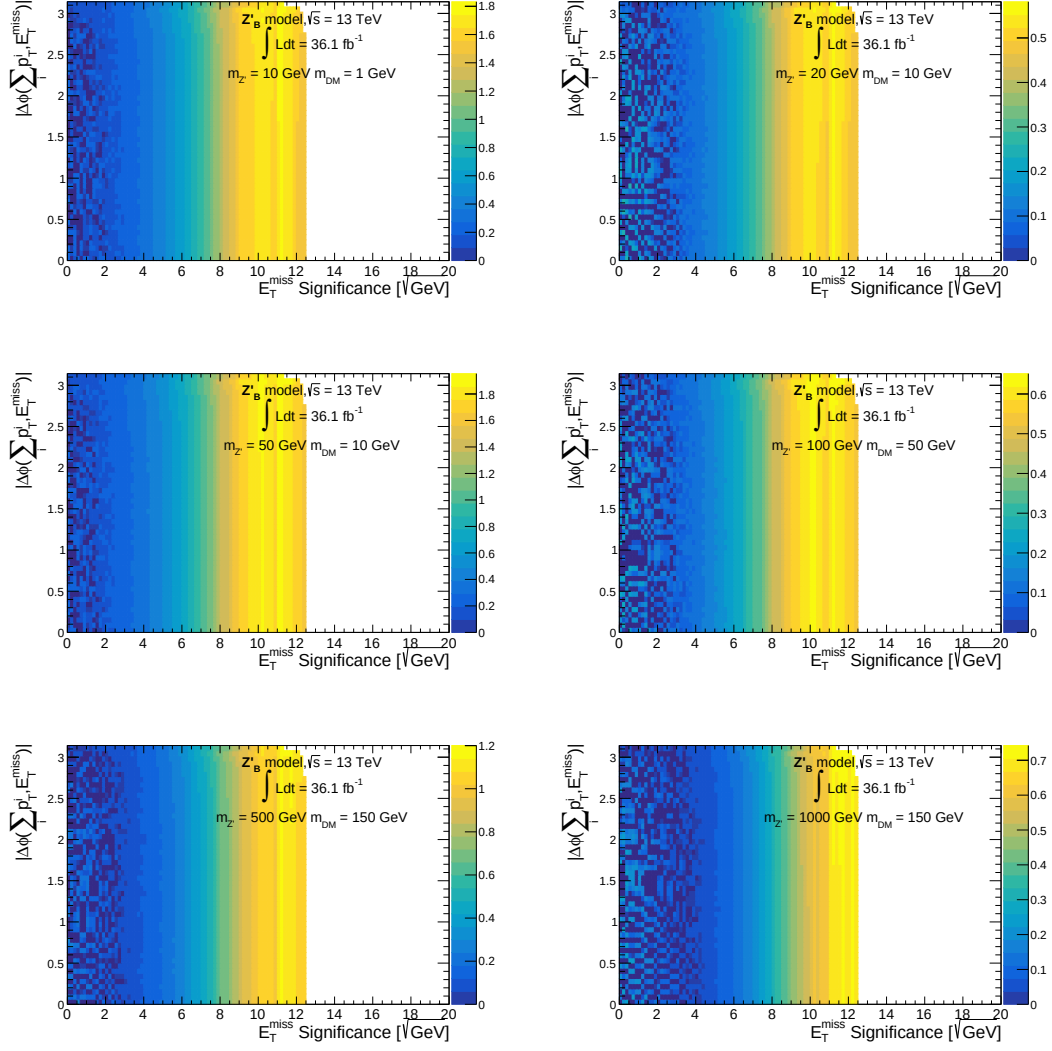
Figure 7.14: Significance scan for various masses of the Z'_B boson and DM particle depending on the S_{E_T^{\text{miss}}} and \Delta\phi(H_T, E_T^{\text{miss}}) variables for the Z'_B model. Event weights are applied and signal and background samples are scaled to their corresponding cross-sections or purity ( \gamma\gamma and \gamma +jet).
