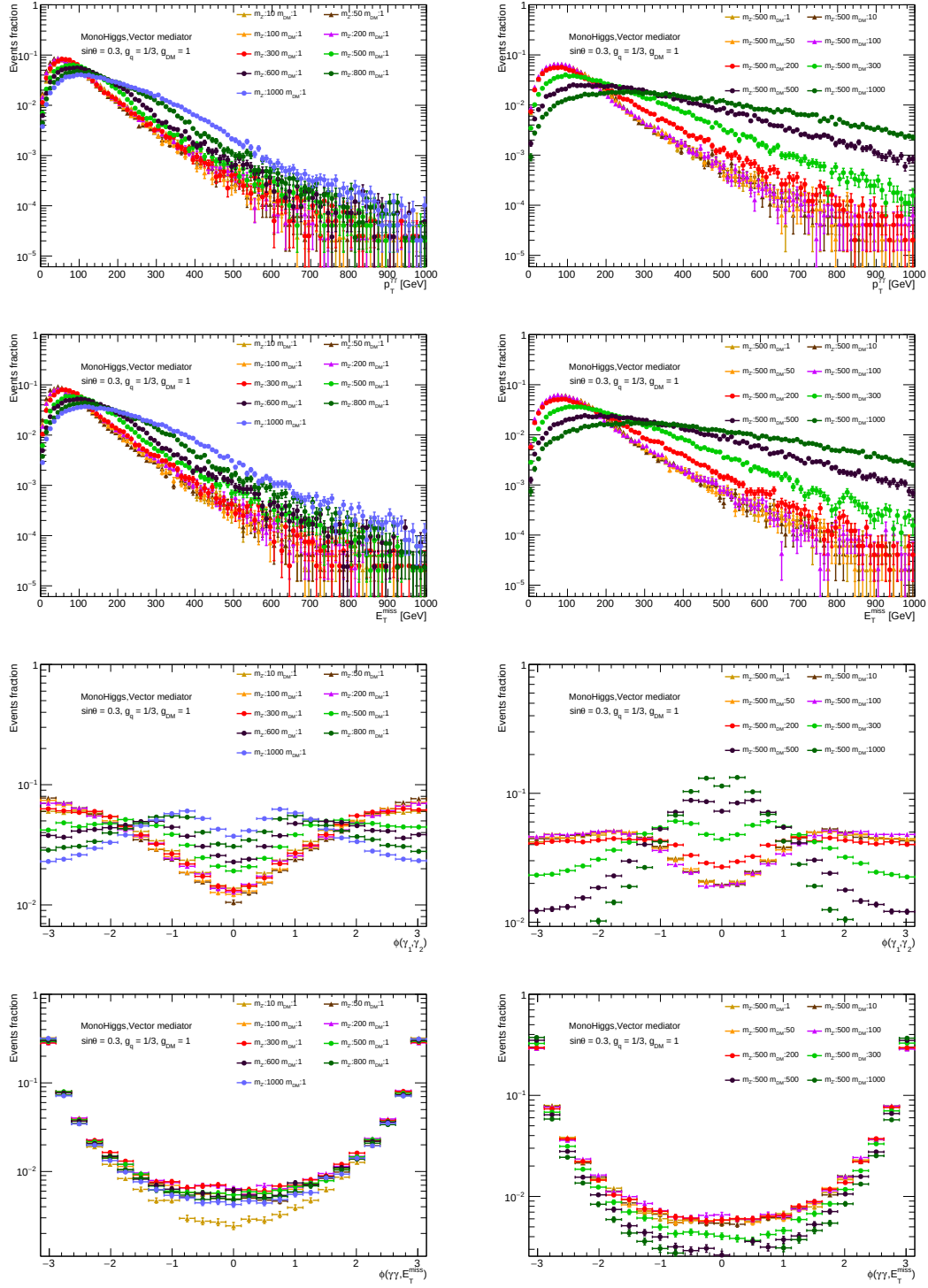
Figure 7.2: Z'_B model comparison for several mass points in the [m_{Z'_B}, m_\chi] plane ( g_q = 1/3 , g_{DM} = 1 and \sin\theta = 0.3 ). Left column: comparison for a fixed m_\chi . Right column: comparison for a fixed m_{Z'_B} . The two rows on the top present the p_T^{\gamma\gamma} and E_T^{\text{miss}} distributions for different simulated samples. It can be observed that at larger m_{Z'_B} and m_\chi , both distributions tend to higher values. Concerning the two bottom rows, they present the angular azimuthal difference between the two photons direction and the diphoton system and the E_T^{\text{miss}} . It can be observed that at larger m_{Z'_B} and m_\chi , the former distribution tend to peak at values closer to zero, indicating that both photons are closer (more boosted). This is not the case however, while m_{Z'_B} \gtrsim m_\chi , in which case both photons tend to be separated given that the intermediate h momentum should not be high. The latter present lower number of events in the central region and a more defined peak at \pi at larger m_{Z'_B} and m_\chi difference, which indicates a larger back-to-back topology between the \gamma\gamma and the \chi\bar{\chi} systems.
