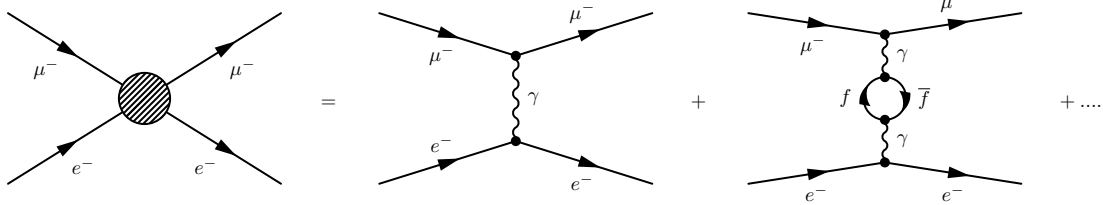
Figure 1.2: Feynman diagrams representing the leading order contributions to the interaction between an initial electron and a muon in the t-channel. The tree-level diagram corresponds to the exchange of a photon between the electron and the muon. In addition, the leading order loop correction to the electron-muon interaction is also shown.
