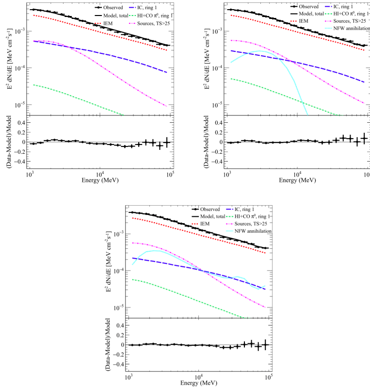
Figure 1.21: \gamma -ray data measured by Fermi-LAT in a region of size 15^\circ \times 15^\circ around the galactic center. It is found that model fits better the \gamma -ray spectra when including a contribution of WIMP dark matter annihilation distributed at the galactic center following a Navarro-Frenk-White profile distribution. Two possible distributions are considered, being shown on the center plot results using the standard NFW distribution and, on the right plot, a NFW distribution corrected with a power law [93]. In this pictures, one of the four IEM's is presented.
