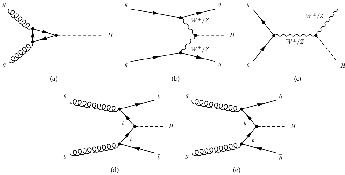
Figure 1.9: Example of the leading order Feynman diagrams for Higgs production at LHC: gluon fusion production (a), vector-boson fusion (b), associated production (c) and t\bar{t}H (d) and b\bar{b}H (e).
