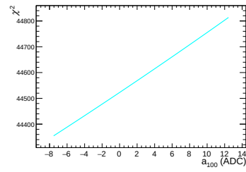
(f) \chi^2 for different a_{100} values
