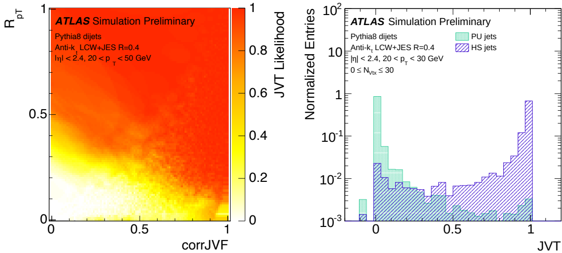
Figure 6.6: Left: JVT values depending on the corrJVF and R_{pT} . Right: JVT distributions for pileup and hard jets estimated on Pythia8 dijet MC events [7].
