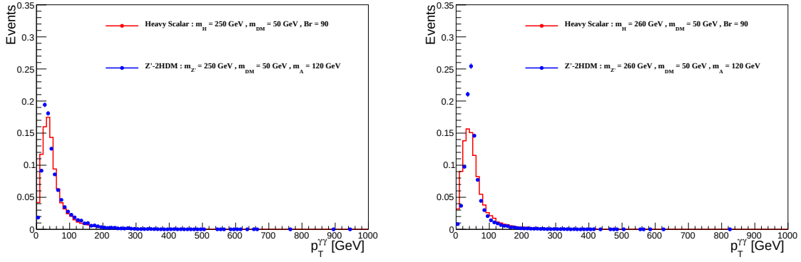
Figure B.22: Comparison of kinematic distributions between Z'-2HDM and Heavy scalar models for the same mediator and DM particle masses ( m'_Z = 250 or 260 GeV, m_\chi = 50 GeV)
