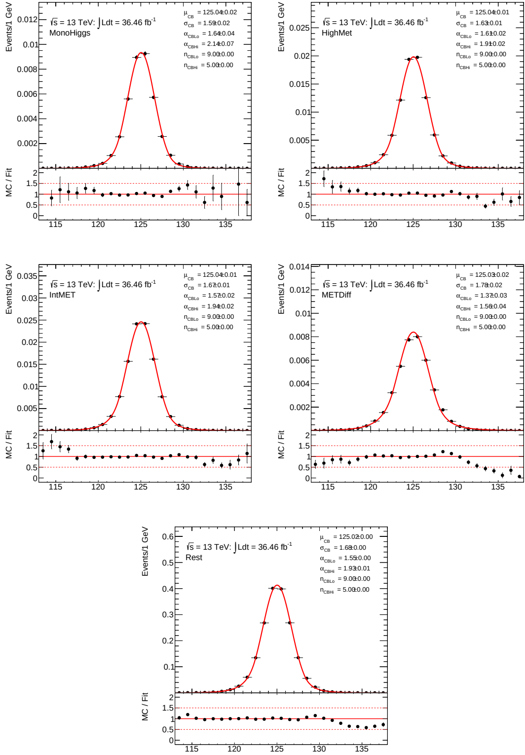
Figure 7.22: Results of a single fit of a DSCB function (lines) for a sample where all Standard Model Higgs processes are summed.
