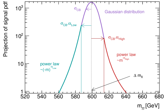
Figure 7.18: Description of the double-sided Crystal Ball function parameters, for a signal mass m_X = 600 GeV. Different parameters are described in the text.
