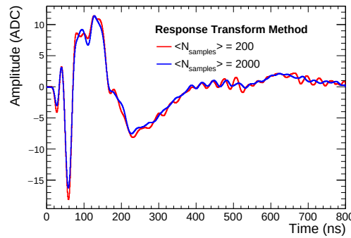
Figure 5.22: Comparison of the cross-talk signal in the same electronic cell if signals are averaged over 200 or 2000 samples.
