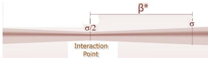
Figure 2.4: Illustration of the \beta^* parameter in Eq. 2.2 [11].
