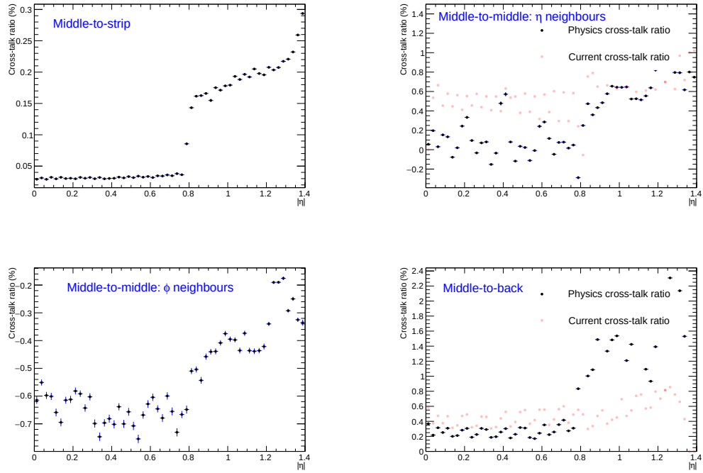
Figure 5.27: Cross-talk magnitude as a function of \eta with pulsed cells in the middle layer. Distributions between the same layer have been divided into the cross-talk contribution between adjacent cells in \phi , with \Delta\eta = 0 and adjacent cells in \eta , with \Delta\phi = 0 . Distributions with calibration cross-talk results are overlaid.
