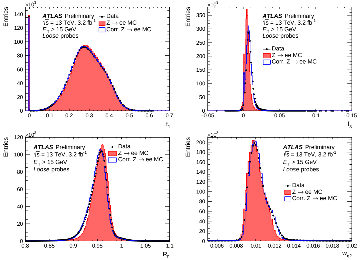
Figure 5.35: Distributions of variables ( f_1 , f_3 , w_{\eta_2} and R_{\eta} ) used in the electron identification. They are measured using a tag-and-probe method on Z \rightarrow ee samples for probes passing the electron loose identification [15]. Corrected MC stand for the MC distributions corrected using the fudge factors and the widths determined in the study.
