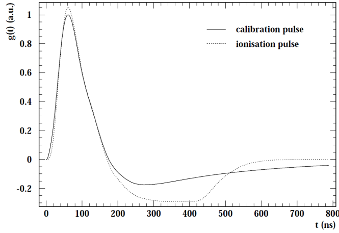
Figure 3.21: Comparison between calibration and physics pulse [17].
