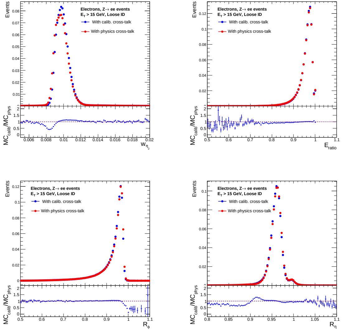
Figure 5.37: Distributions of variables ( E_{ratio} , w_{\eta_2} , R_\eta and R_\phi ) used in the electron identification. Measured on Z \rightarrow ee events simulated without any pileup effects. Electrons are required to pass loose identification and to present E_T > 15 GeV and |\eta| < 1.475 . Calibration cross-talk stands for the current cross-talk values introduced in the simulation (Table 5.1) and the physics cross-talk estimated using 4 samples (Table 5.2).
