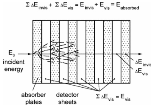
Figure 3.1: Shower development and energy depositions in a sampling calorimeter [1].
