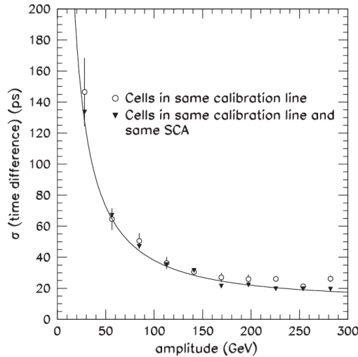
Figure 3.27: Resolution on the time difference between cells in calibration runs as a function of the amplitude [9].
