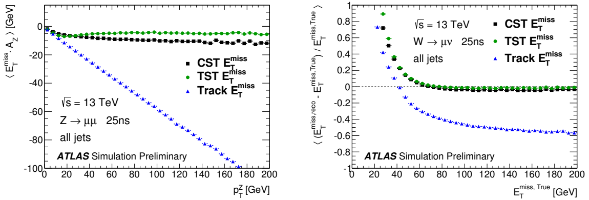
Figure 6.13: (Left) Scale of the E_T^{\text{miss}} on the axis defined by the transverse momentum of the Z boson studied on Z \rightarrow \mu^- \mu^+ MC samples as a function of p_T^Z . (Right) linearity as a function of E_{T, \text{truth}}^{\text{miss}} on W \rightarrow \mu\nu MC events.
