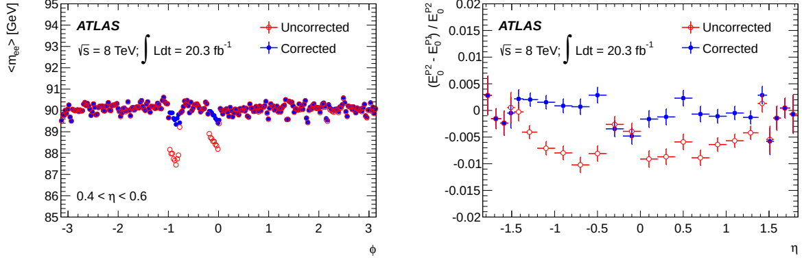
Figure 4.21: Left: average value of m_{ee} as a function of the azimuthal position of the leading decay electron with 0.4 < \eta < 0.6 before and after the HV correction. Right: relative difference in the raw PS energy response due to the change in HV settings, as a function of \eta , before and after correction of the residual HV dependence [2].
