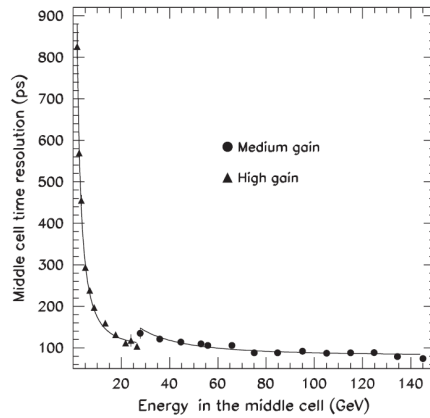
Figure 3.29: Time resolution (ps) as a function of the hottest middle layer cell.
