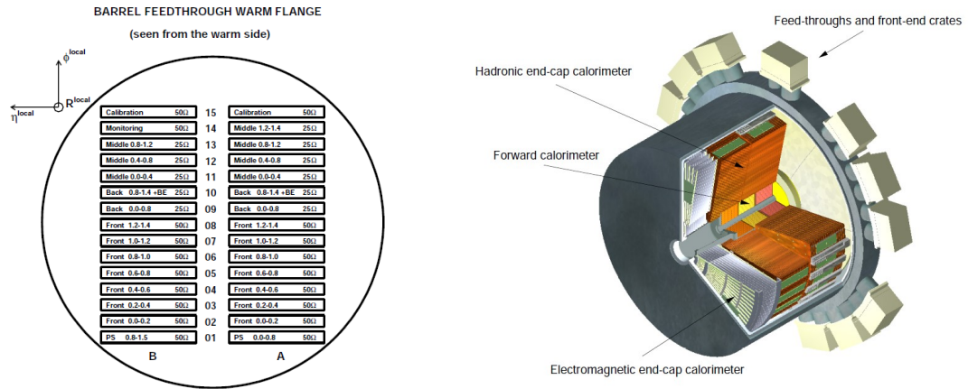
Figure 3.14: Feedthrough connectors distribution (left) [15] and feedthrough distribution in the cryostat of the end-cap (right), similar to the distribution of the feedthroughs around the barrel cryostat [8].
