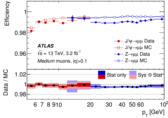
Figure 6.9: Reconstruction efficiency for the Medium muon selection as a function of the p_T of the muon, in the region 0.1 < |\eta| < 2.5 as obtained with Z \rightarrow \mu^+\mu^- and J/\psi \rightarrow \mu^+\mu^- events in 2015 data and MC [9].
