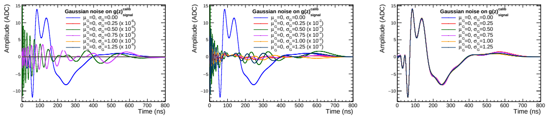
Figure 5.18: g(t)_{\text{xtalk}}^{\text{phys}} estimated using the matrix inversion method. Left, center and right plots show the obtained signal when a gaussian noise centered at zero and with varying \sigma is added to the first 20 terms, 20 th -50 th terms and 50 th -100 th of g(t)_{\text{signal}}^{\text{calib}} , respectively. It can be observed that large fluctuations are obtained when the first samples are affected by noise, even by a small contribution.
