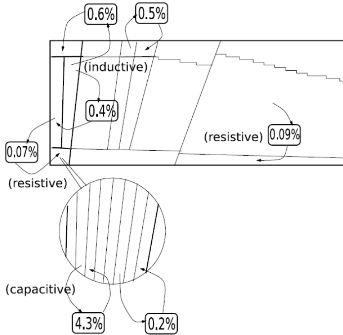
Figure 5.9: Schema of the different cross-talk magnitudes using the under-peak to peak estimation [8].
