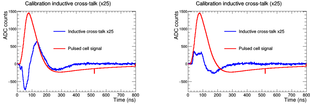
Figure 5.5: Inductive cross-talk shape obtained from calibration data. A cell is pulsed in the middle layer of the EM barrel. The cross-talk shape on the left is retrieved from its closest neighbouring cell in \eta while the one on the right is retrieved from its adjacent cell in the back layer.
