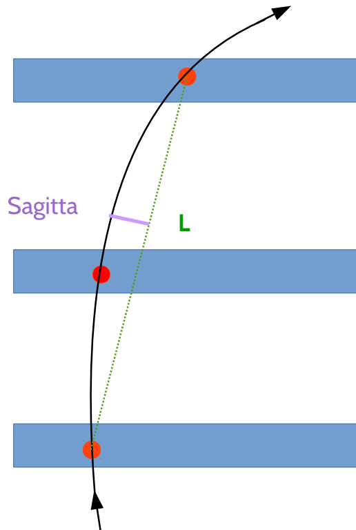
Figure 6.8: Illustration of the sagitta parameter.
