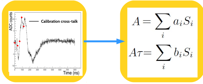
Figure 5.10: Schema of how cross-talk energy is estimated using the optimal filtering method on calibration signals .
