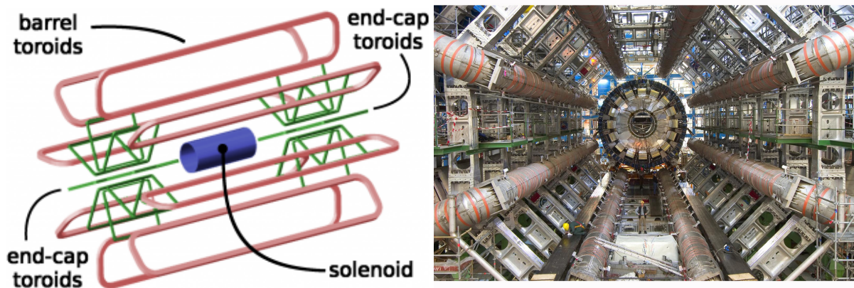
Figure 2.10: Illustration of the magnet system layout (a) and photograph of the final installation of the ATLAS detector (b), where barrel toroids may be observed in the foreground.
