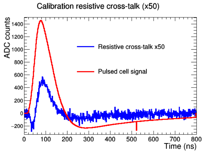
Figure 5.4: Resistive cross-talk shape obtained from calibration data. A cell is pulsed in the middle layer of the EM barrel. The cross-talk shape is retrieved from one of its neighbouring cell in the front layer.
