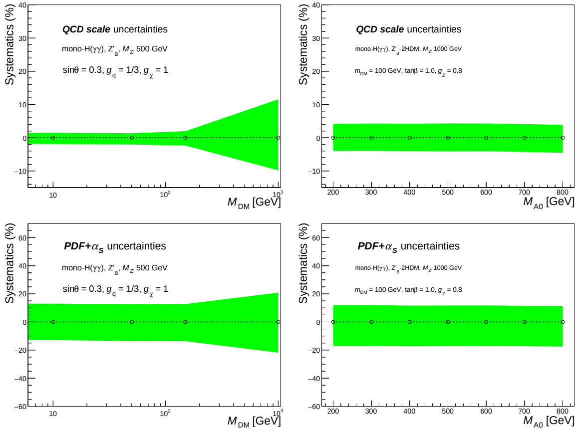
Figure 7.25: Relative scale (top) and PDF (bottom) uncertainty for Z'_B (left) and Z' -2HDM (right) models.
