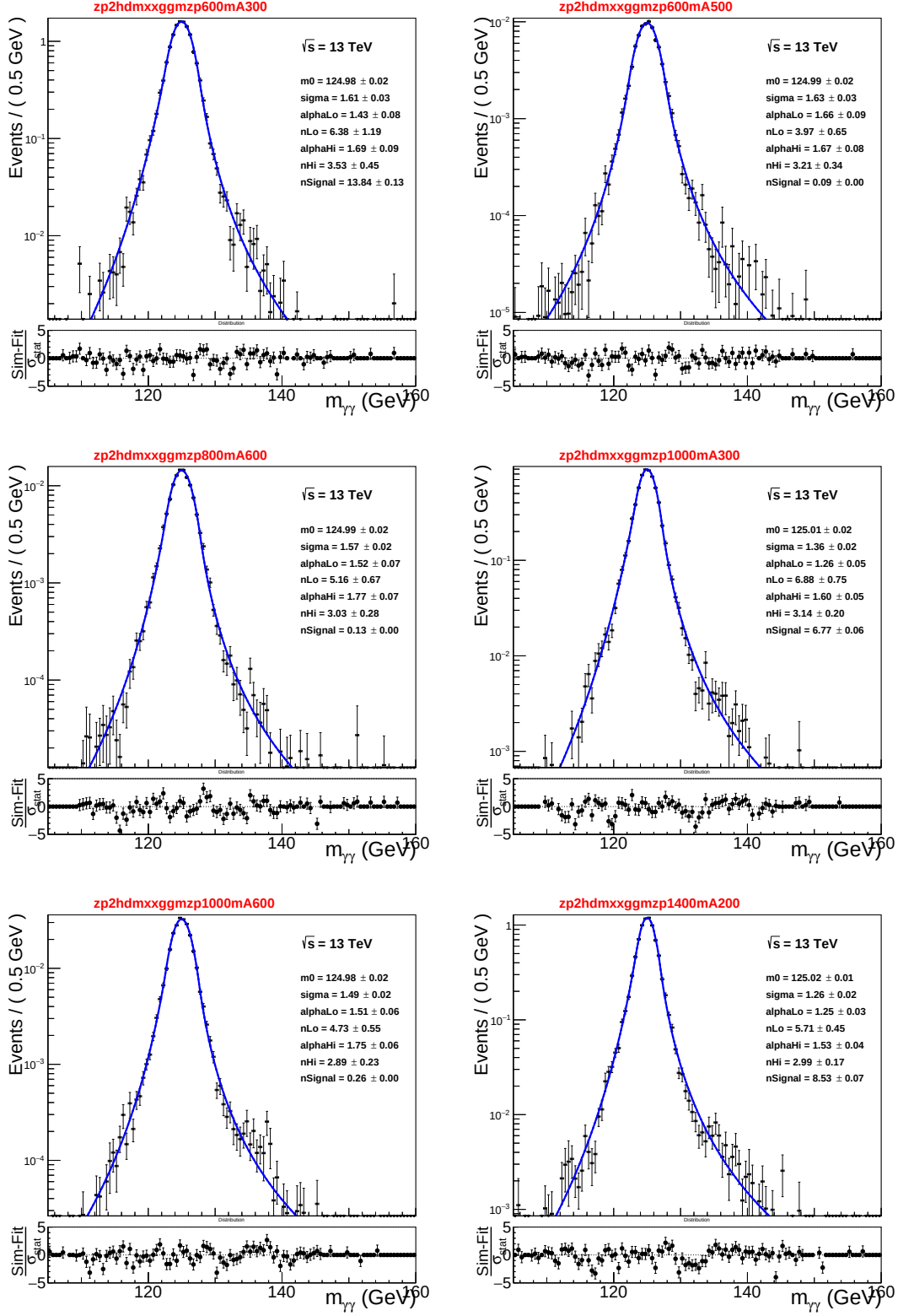
Figure 7.19: Fits of the Z' -2HDM signal line-shape for different sets of signal samples (red title).
