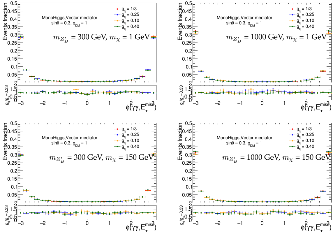
Figure C.4: \Delta\phi(\gamma\gamma, E_T^{\text{miss}}) distributions of the Z'_B model of four mass points (m_{Z'_B}, m_\chi) and four different values of g_q .
