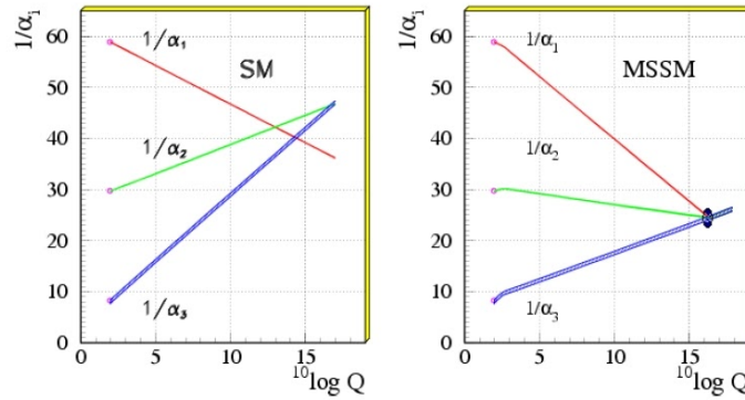
Figure 1.14: Standard Model and Minimal Supersymmetric Standard Model electromagnetic, weak and strong running couplings. Coupling unification in MSSM (plot taken from [58]).
