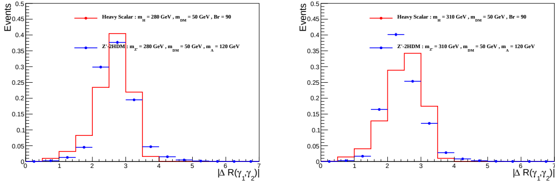
Figure B.7: Comparison of kinematic distributions between Z'-2HDM and Heavy scalar models for the same mediator and DM particle masses ( m'_{Z'} = 280 or 310 GeV, m_\chi = 50 GeV)
