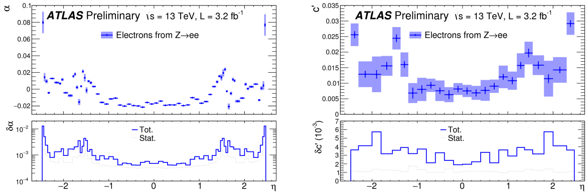
Figure 4.24: (a) Energy scale factor \alpha and (b) additional constant term c' for energy resolution from Z \rightarrow ee events as a function of \eta . The uncertainty bands on the top plots represent the total uncertainties on these quantities, while the thin black (resp. thick blue) lines at the bottom represent the statistical (resp. total) uncertainties. [18].
