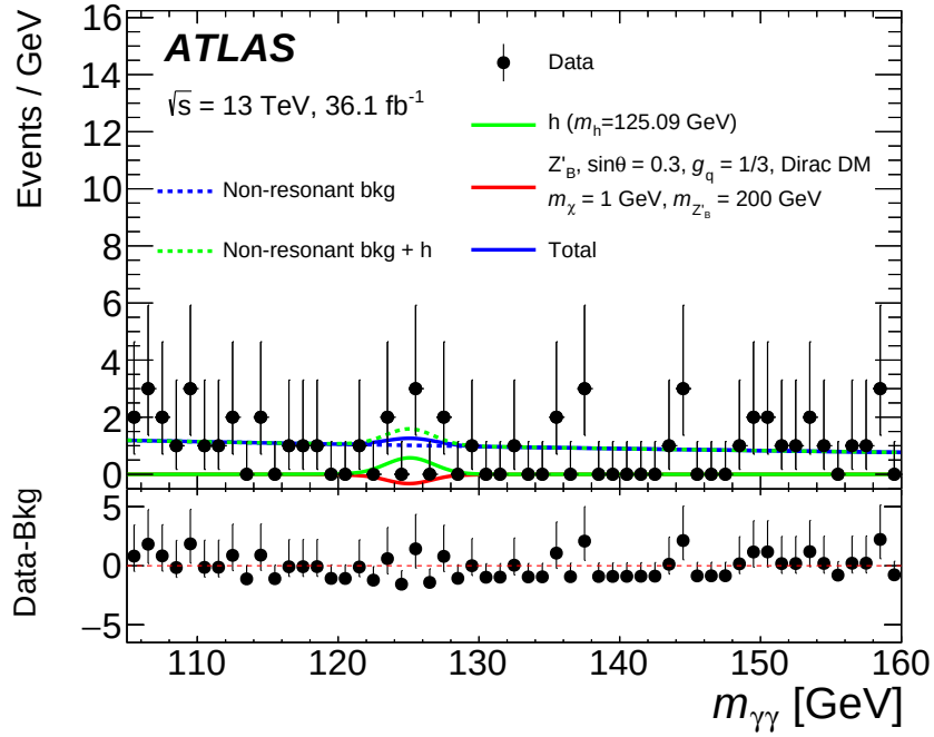
Figure 7.37: Diphoton invariant mass distribution for data and the corresponding fitted signal and background in the Mono-Higgs category for the Z'_B benchmark model fit using g_q = 1/3 , g_\chi = 1 , \sin \theta = 0.3 and Dirac fermion DM m_\chi = 1 GeV as an illustration [3]. A negative best-fit DM signal is found. The data is shown as dots with asymmetric error bars that represent central Poissonian confidence intervals at 68% CL. The fitted signal (solid red line), SM Higgs boson (solid green line), non-resonant background (dashed blue line) and the non-resonant background plus the SM Higgs boson (dashed green line) are shown as well as the total of all those contributions (solid blue line).
