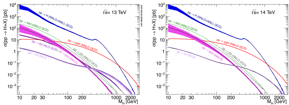
Figure 1.10: Higgs production cross-section for leading production modes. The left plot shows production the cross-section at \sqrt{s} = 13 TeV while the right plot at \sqrt{s} = 14 TeV. Bolded regions correspond to the Higgs cross-section uncertainties.
