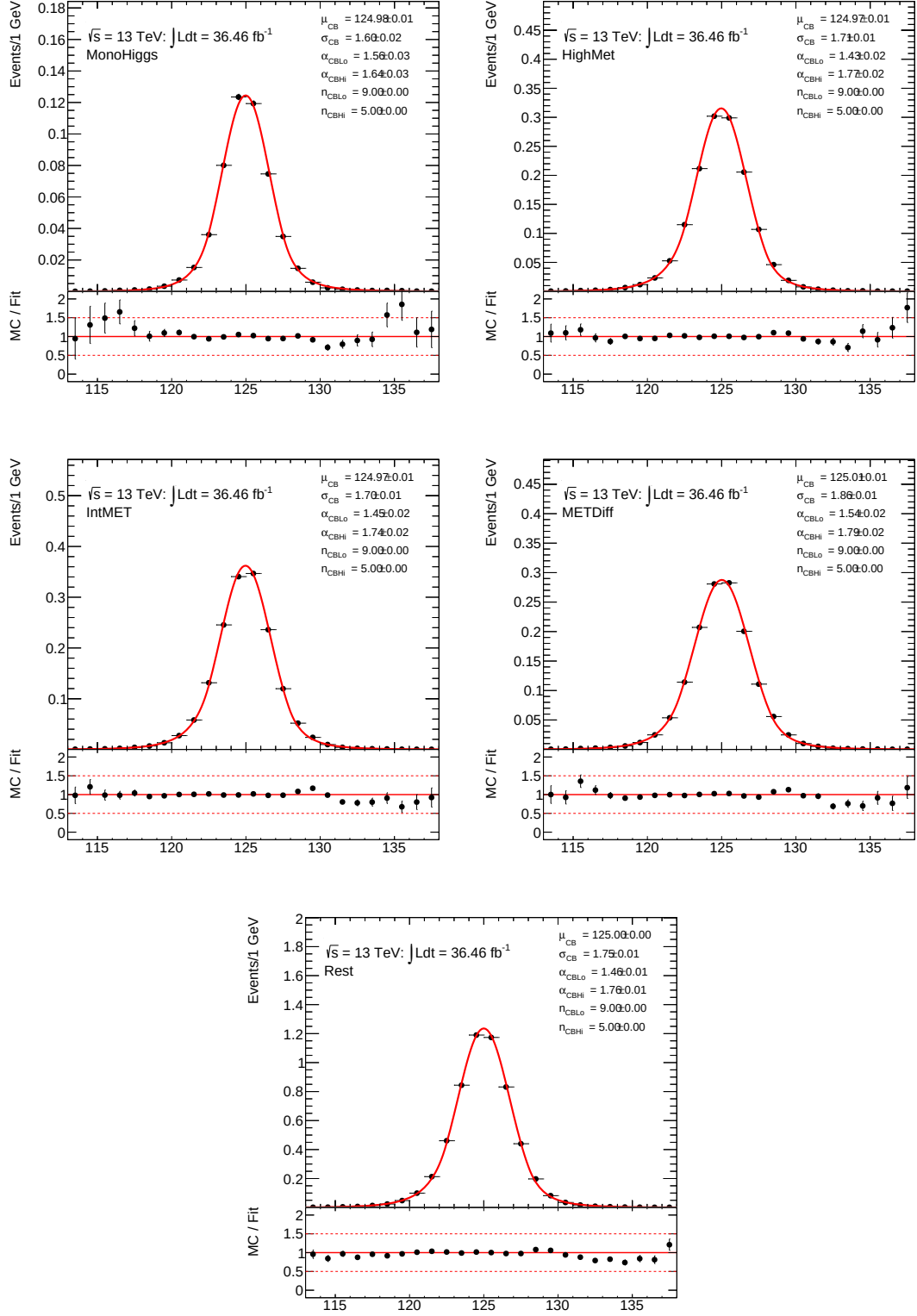
Figure 7.21: Results of a single fit of a DSCB function (lines) for a sample where all Heavy scalar processes are summed.
