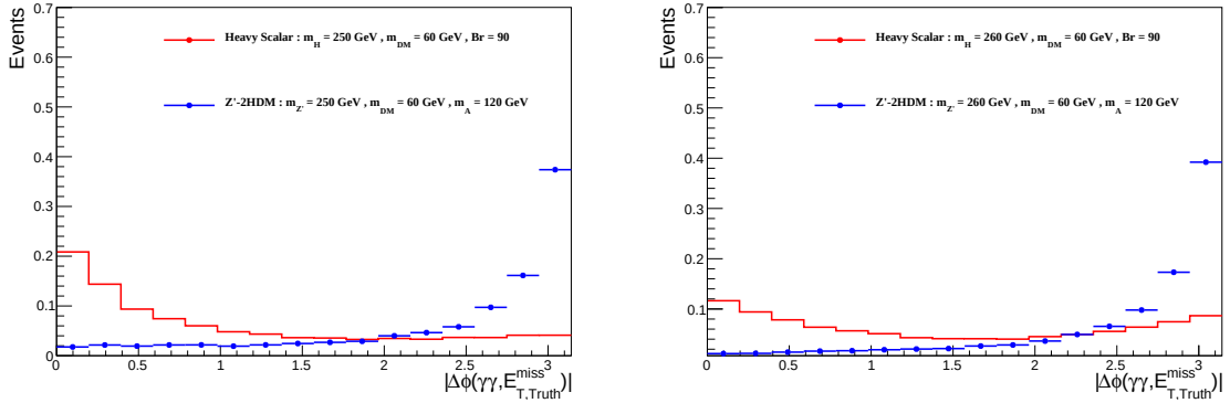
Figure B.16: Comparison of kinematic distributions between Z'-2HDM and Heavy scalar models for the same mediator and DM particle masses ( m'_Z = 250 or 260 GeV, m_\chi = 60 GeV)
