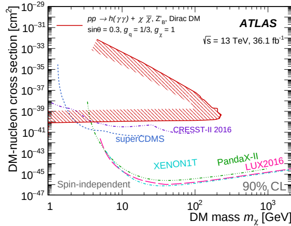
Figure 7.40: A comparison of the inferred limits to the constraints from direct detection experiments on the spin-independent DM–nucleon cross section in the context of the Z'_B simplified model with vector couplings [3]. Limits are shown at 90% CL. The results from this analysis, in which the region inside the contour is excluded, are compared with limits from the LUX [51], PandaX-II [52], XENON [53], superCDMS [54], and CRESST-II [55] experiments. The comparison is model-dependent and solely valid in the context of this model, assuming Dirac fermion DM, mixing angle \sin \theta = 0.3 , and the coupling values g_q = 1/3 and g_\chi = 1 . The impact of renormalization-group evolution effects [56, 57] when comparing collider and direct detection limits is not taken into consideration here.
