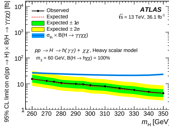
Figure 7.42: Observed and expected 95% CL upper limits on the \sigma(pp \rightarrow H) \times \mathcal{B}(H \rightarrow \gamma\gamma\chi\chi) with a scalar DM candidate mass of 60 GeV as a function of the heavy-scalar-boson mass in the range 260 \text{ GeV} < m_H < 350 \text{ GeV} [3]. A 100% branching fraction is assumed for H \rightarrow h\chi\chi . The theoretical prediction for the model (dark-blue lines with blue bands representing their associated theoretical systematic uncertainties) is also shown. The theoretical cross-section is assumed to be equal to that of a SM Higgs boson with the same mass produced in gluon–gluon fusion.
