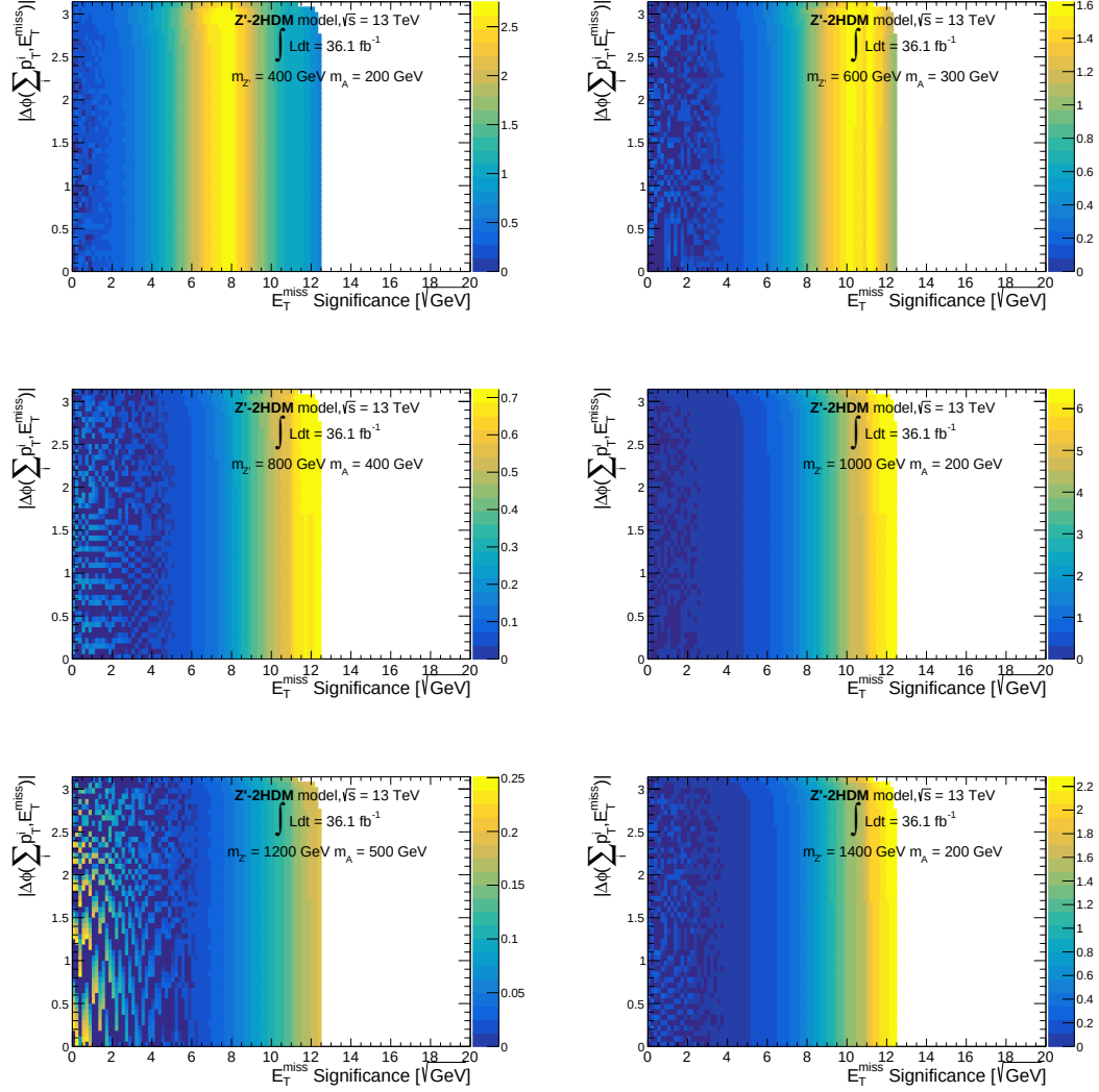
Figure 7.15: Significance scan for various masses of the Z' boson and pseudo-scalar A^0 depending on the S_{E_T^{\text{miss}}} and \Delta\phi(H_T, E_T^{\text{miss}}) variables for the Z' -2HDM model. Event weights are applied and signal and background samples are scaled to their corresponding cross-sections or purity ( \gamma\gamma and \gamma +jet).
