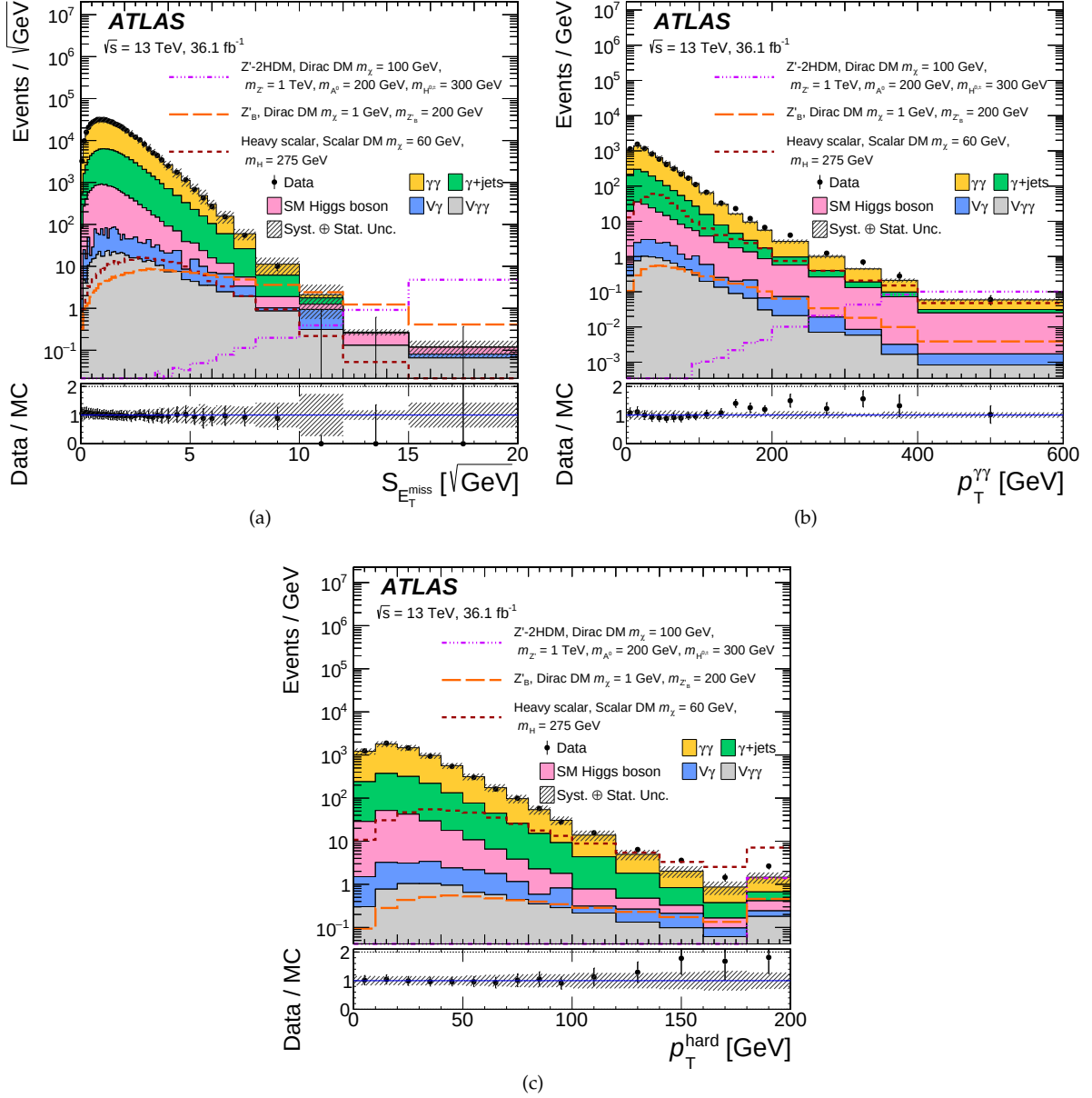
Figure 7.17: The distribution of (a) S_{E_T^{\text{miss}}} , (b) p_T^{\gamma\gamma} and (c) p_T^{\text{hard}} after the selection of diphoton candidates in 120 \text{ GeV} < m_{\gamma\gamma} < 130 \text{ GeV} [3]. Expected signal distributions are shown for a Z'_B signal with m_{Z'_B} = 200 \text{ GeV} and Dirac fermion DM m_\chi = 1 \text{ GeV} , a Z' -2HDM signal with m_{Z'} = 1000 \text{ GeV} , m_{A^0} = 200 \text{ GeV} and Dirac fermion DM m_\chi = 100 \text{ GeV} and a heavy-scalar model with m_H = 275 \text{ GeV} and scalar DM m_\chi = 60 \text{ GeV} . These overlaid signal points chosen are representative of the model kinematics. Only the sum of the MC statistical and experimental systematic uncertainties on the total background is shown as the hatched bands, while the theoretical uncertainties on the background normalization are not included. Overflow events are included in the rightmost bins.
