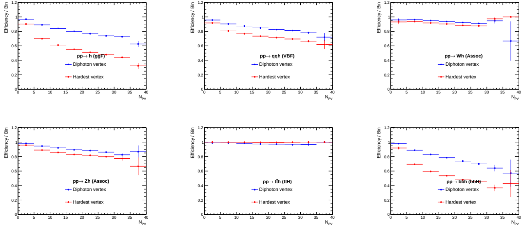
Figure 6.14: Truth Higgs boson production vertex identification efficiency using the diphoton or the hardest vertex method. Efficiency is presented as a function of the number of primary vertices.
