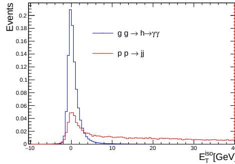
Figure 4.16: Comparison of the corrected topoetcone20 isolation transverse energies for photons from the gluon-fusion h \rightarrow \gamma\gamma MC sample and a jj sample, where the photon is faked by a jet.
