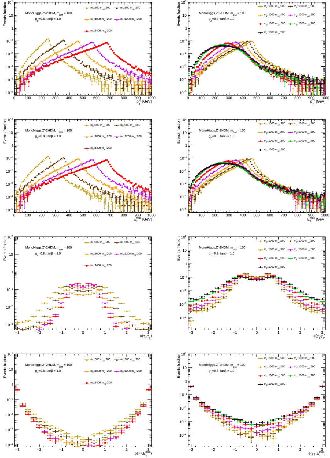
Figure 7.3: Z'-2HDM comparison for several mass points in the [m_{Z'}, m_{A^0}] plane ( g_{Z'} = 0.8 , \tan\beta = 1.0 and m_\chi = 100\text{GeV} ) Left column: comparison for a fixed m_{A^0} . Right column: comparison for a fixed m_{Z'} . The two rows on the top present the p_T^{\gamma\gamma} and E_T^{\text{miss}} distributions for different simulated samples. It can be observed that at larger m_{Z'} - m_{A^0} difference, harder are the kinematic distributions. Concerning the two bottom rows, they present the angular azimuthal difference between the two photons direction and the diphoton system and the E_T^{\text{miss}} . It can be observed that at larger m_{Z'} - m_{A^0} difference, the former distribution tend to peak at values closer to zero, indicating that both photons are closer (more boosted). The latter present lower number of events in the central region and a more defined peak at \pi at larger m_{Z'} - m_{A^0} difference, which indicates a larger back-to-back topology between the \gamma\gamma and the \chi\bar{\chi} systems.
