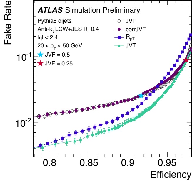
Figure 6.7: Efficiency and fake rate curves of the JVT variable in comparison with the corrJVF, R_{pT} and JVF variables [7].
