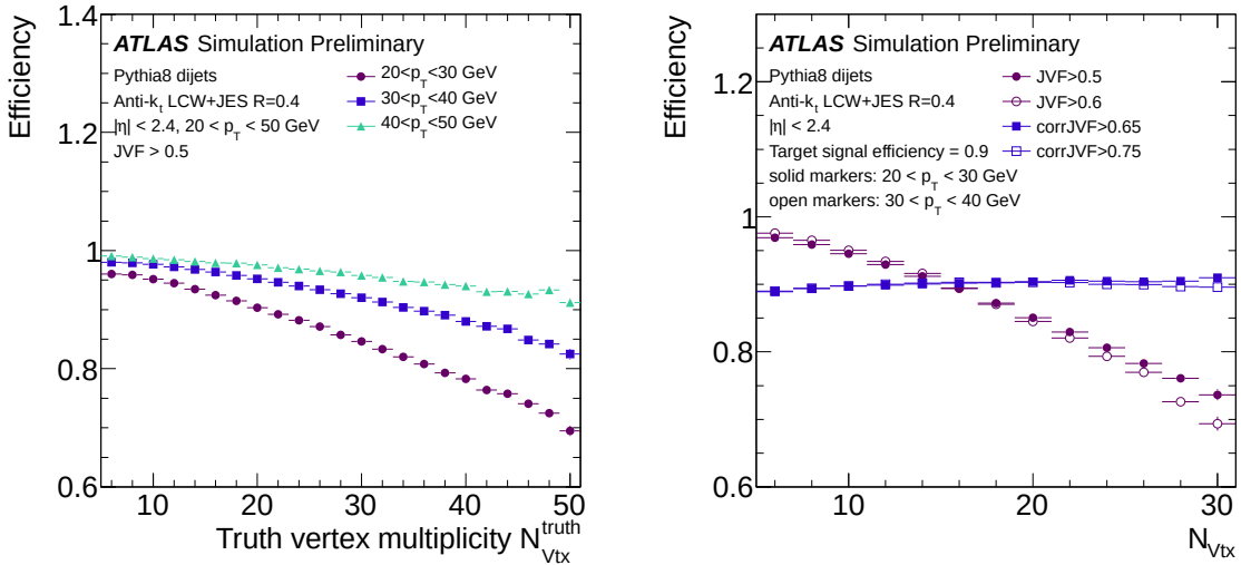
Figure 6.4: Left: performance of the JVF against pileup and for different jet p_T values. Right: comparison of corrJVF and JVF performance against pileup activity [7].
