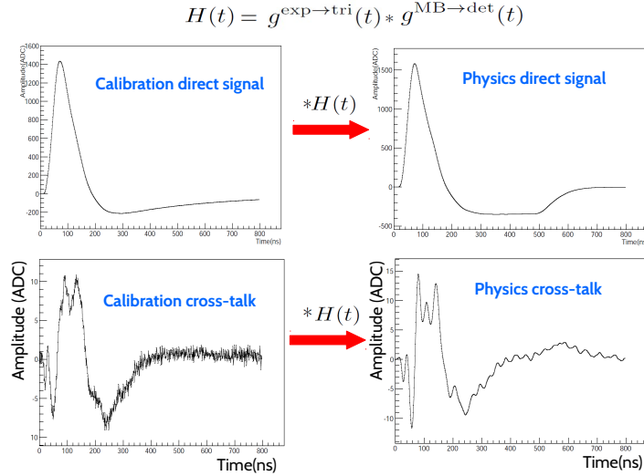
Figure 5.14: Illustration of the application of the RTM method to the cross-talk calibration shape, based on the method used for direct signals.
