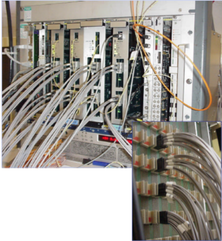
Figure 5.5: Five DSS modules feeding LVDS data to one CPM [52]
