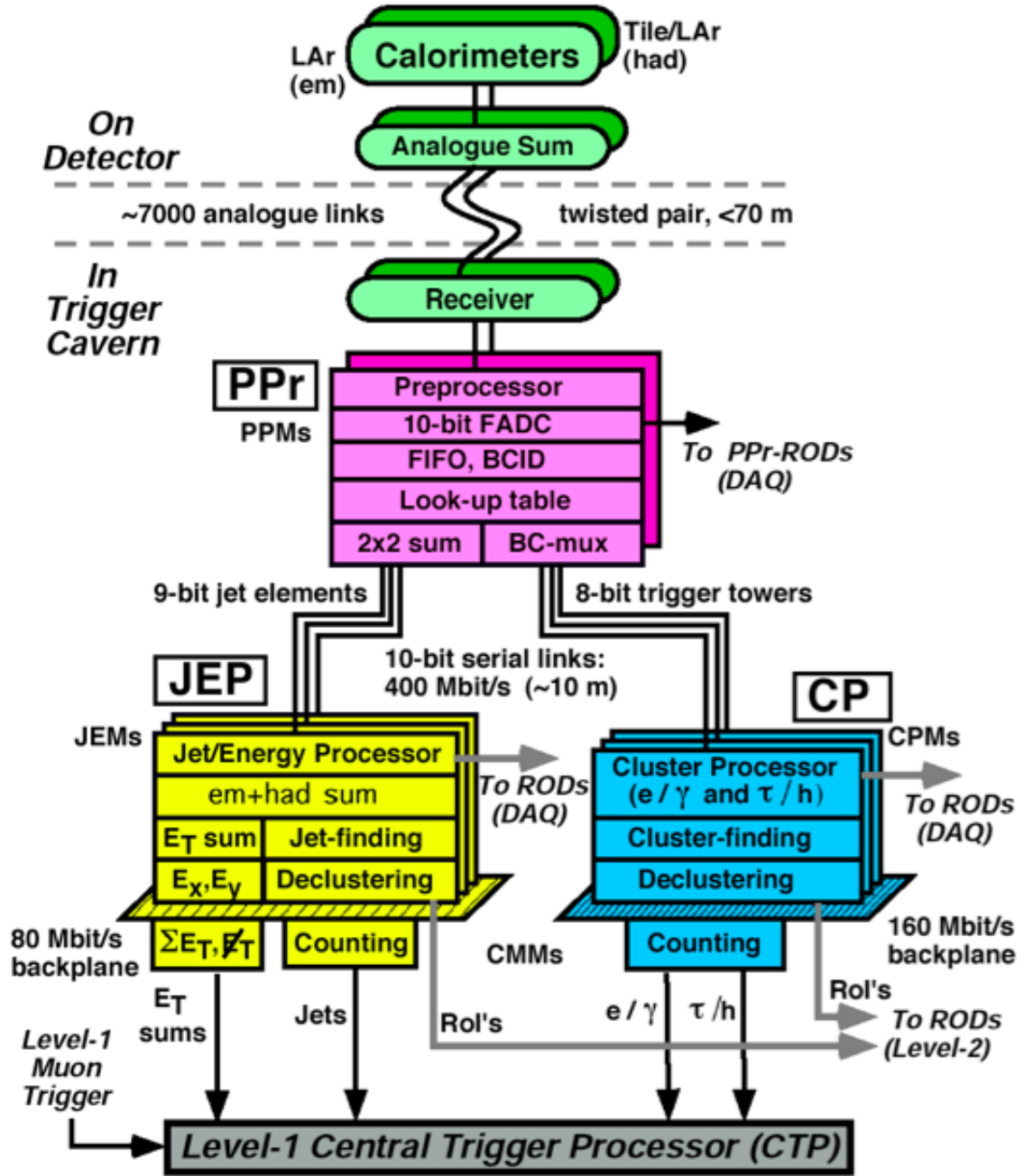
Figure 3.3: ATLAS Level-1 Calorimeter Trigger [32]
