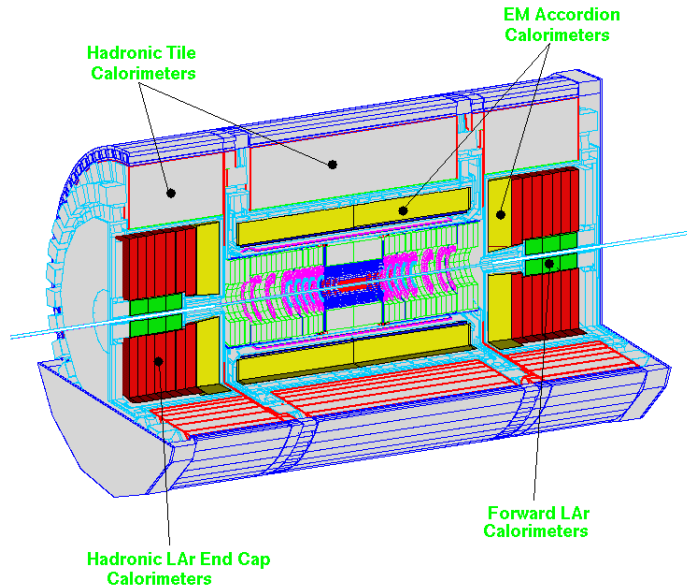
Figure 2.7: ATLAS Calorimetry [27]
