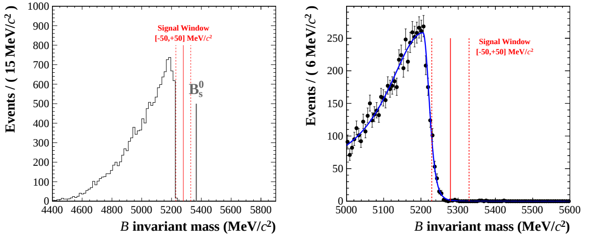
Figure 4.18.: B_s^0 \rightarrow D^0 [K\pi]_{K^*} events. Left: true 4-momentum combination only in the full mass window when the bachelor pion is lost. Right: PDF shaped using the full LHCb detector simulation. The distribution is fitted using a bifurcated gaussian with two tail parameters (Sec. 3.9.1).
