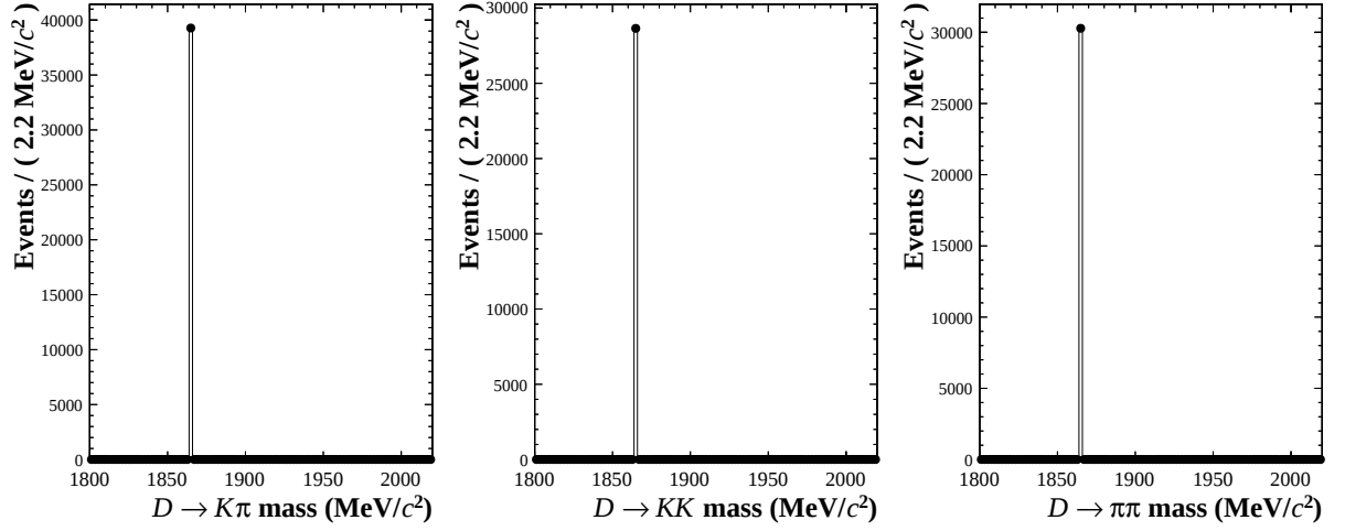
Figure 3.15.: MC: D invariant mass distributions for signal simulated, truth matched, events once the D mass is constrained to its nominal central value (approximate delta function with \text{RMS} < 1 \text{ KeV}/c^2 ).
