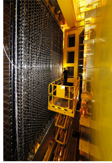
Figure 2.19.: ECAL Photomultipliers
