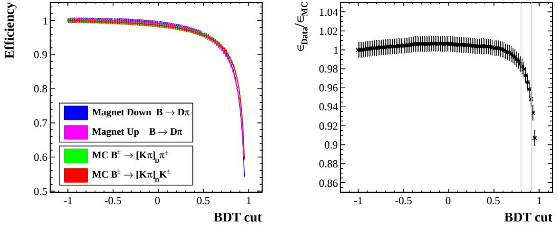
Figure 3.12.: Left: efficiencies for MC and data samples. Right: correction factor \epsilon_{\text{data}}/\epsilon_{\text{MC}} . Efficiencies are normalized to 1 for BDT = -1, e.g no MVA cut applied.
