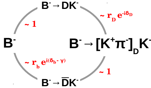
Figure 1.8.: The ADS method. Favoured B^- \rightarrow D^0 K^- decays are followed by DCS D^0 \rightarrow K^+\pi^- decays. Vice versa, colour suppressed B^- \rightarrow \bar{D}^0 K^- decays are followed by Cabibbo-favoured \bar{D}^0 \rightarrow K^+\pi^- transitions.
