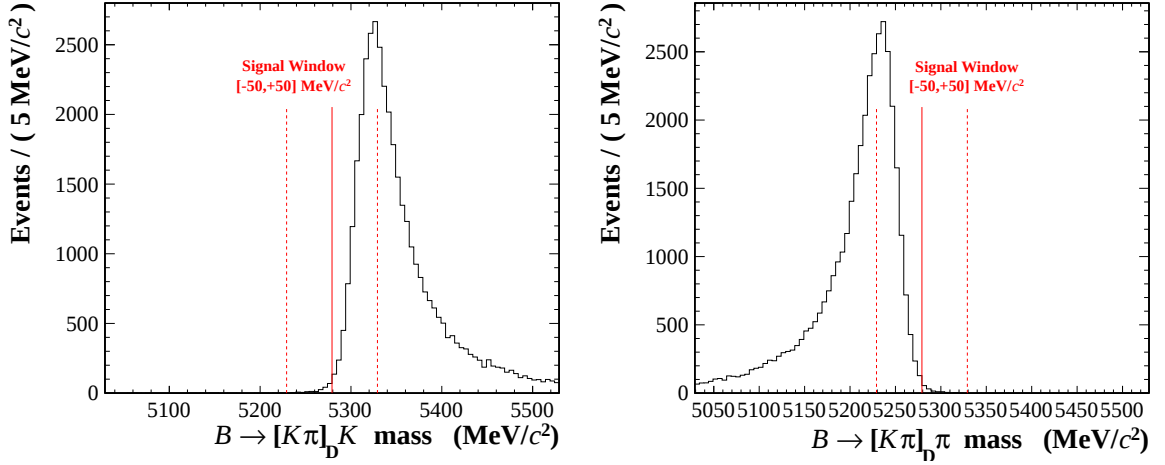
Figure 3.20.: Left: B \rightarrow [K\pi]_D \pi MC simulated events reconstructed with the B \rightarrow [K\pi]_D K mass hypothesis ( \pi misidentified as a K ). Right: B \rightarrow [K\pi]_D K MC simulated events reconstructed with the B \rightarrow [K\pi]_D \pi mass hypothesis ( K misidentified as a \pi ). Mass distributions are obtained using the full LHCb detector simulation.
