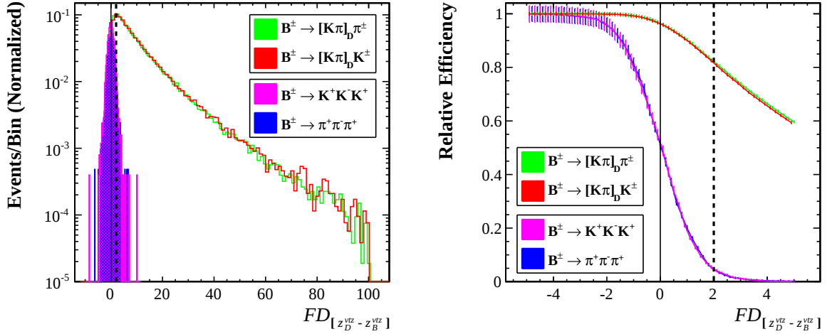
Figure 4.21.: Left: FD_{[z_D^{vtz} - z_B^{vtz}]} distributions for signal and charmless MC simulated events. Distributions have been normalized and plotted on a logarithmic scale in order to highlight the long exponential-like tail in genuine B \rightarrow [hh]_D h decays. Right: corresponding efficiencies for each FD_{[z_D^{vtz} - z_B^{vtz}]} cut.
