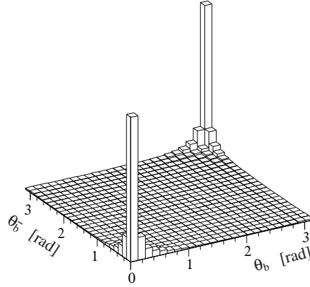
Figure 2.4.: Angular correlation between the b and \bar{b} quarks produced in pp interactions (angles formed with respect to the beam axis). Events are simulated with the PYTHIA event generator [38].
