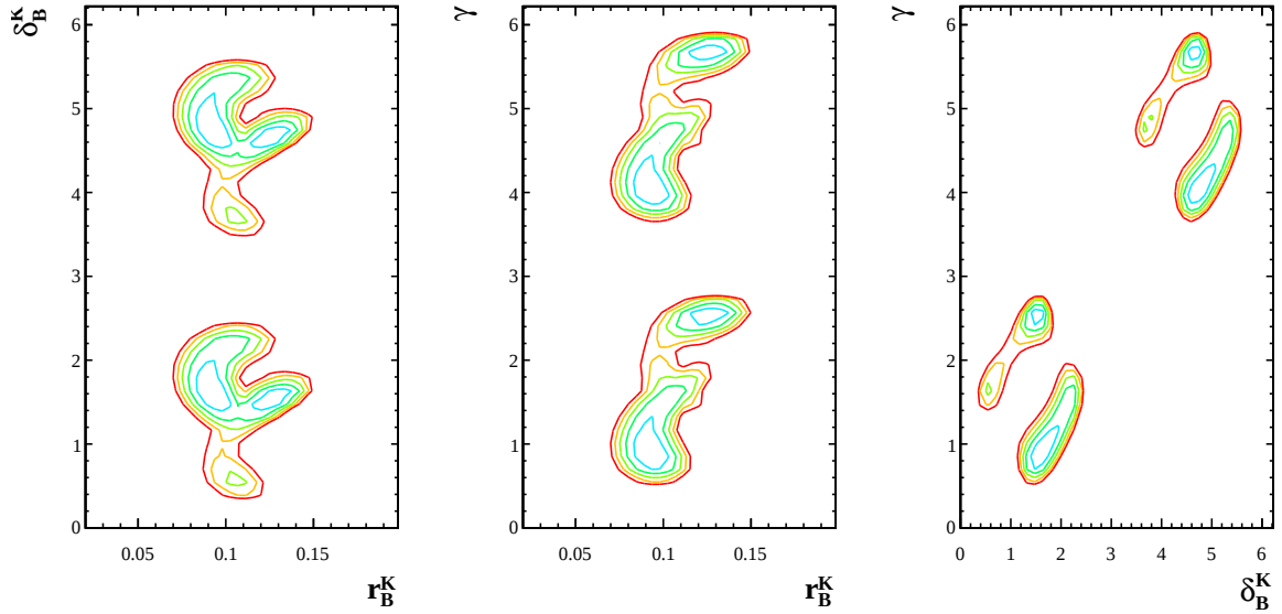
Figure 6.10.: 2D projections of the (r_B^K, \delta_B^K, \gamma) scan. Each 2D curve is obtained minimising the \Delta\chi^2 function with respect to the other variable. 1 \sigma to 5 \sigma contours are plotted.
