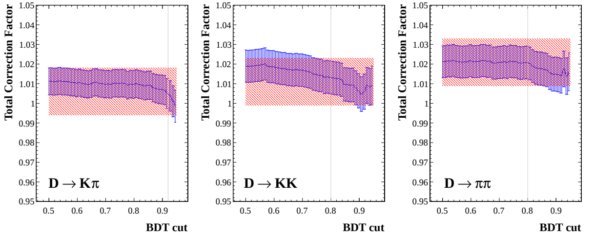
Figure 5.6.: Total correction factors with respect to BDT cut for B \rightarrow [K\pi]_D h , B \rightarrow [KK]_D h and B \rightarrow [\pi\pi]_D h signal modes. Corrections are stable over the full BDT range of interest. The shaded region indicates the used correction factor with its \pm 1\sigma associated systematic uncertainty.
