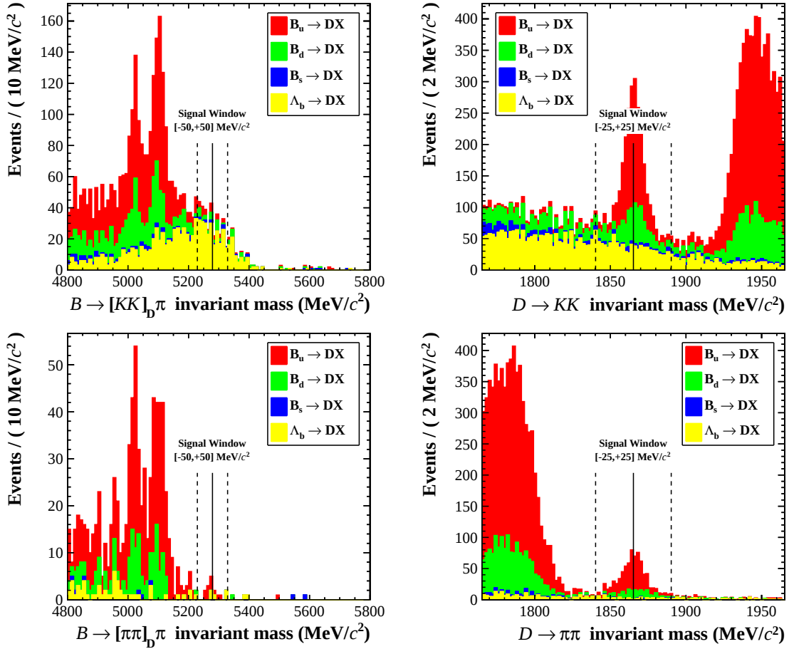
Figure 4.12.: B \rightarrow DX cocktail reconstructed as B \rightarrow [KK]_D \pi mode (Top) and as B \rightarrow [\pi\pi]_D \pi mode (Bottom). No PID requirement is applied for the bachelor and the D meson daughter tracks. The B mass distribution is plotted selecting only the events inside the D mass signal window.
