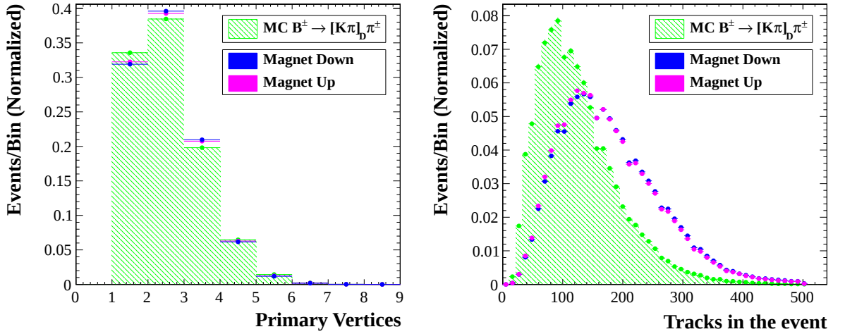
Figure 3.2.: Event variables. Left: number of reconstructed Primary Vertices (PV) in the event. Right: number of charged tracks reconstructed in the event. Both magnet Down and Up data samples have been collected with different running conditions during the year and they present a larger average number of tracks and PVs in the event compared to the simulated B \rightarrow [K\pi]_D \pi events.
