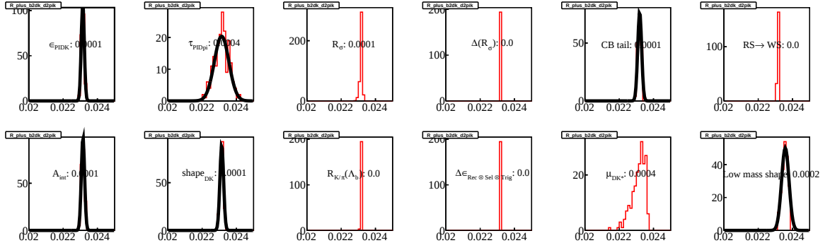
The distribution of R_K^{+} results under systematic variations
