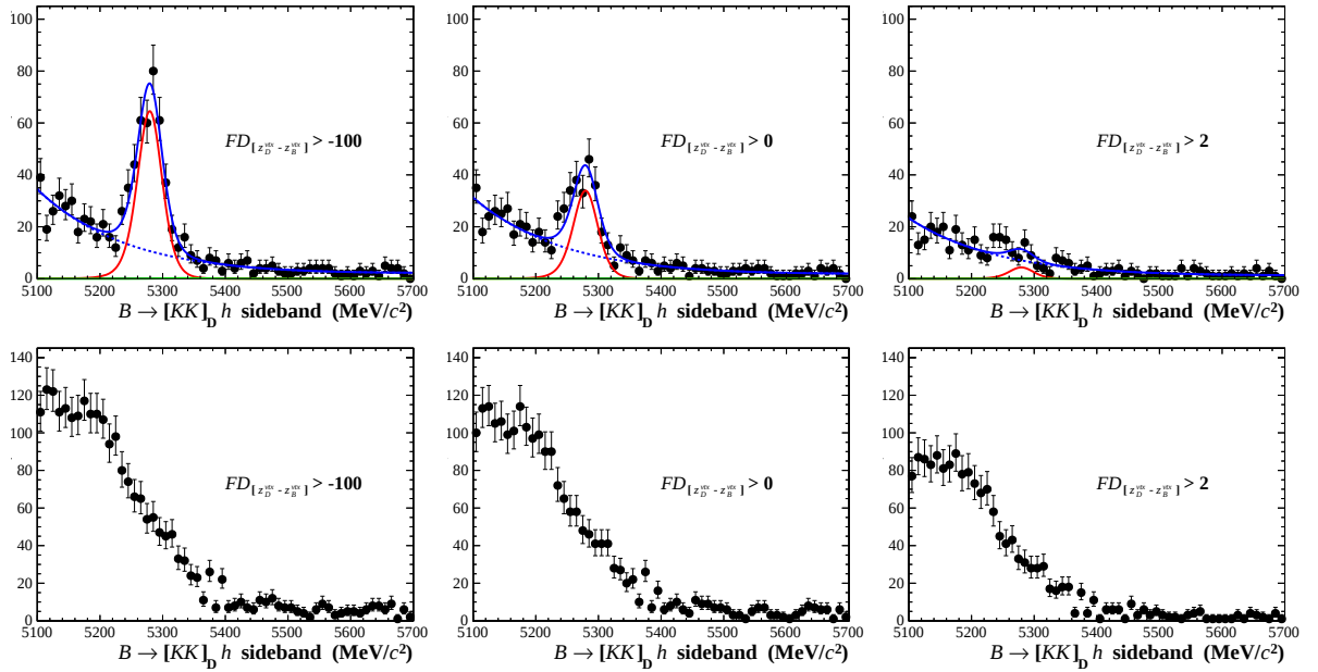
Figure 4.27.: B^+ \rightarrow K^+ K^- K^+ (top) and B^+ \rightarrow K^+ K^- \pi^+ (bottom) fits on the [KK]_D sideband. Red: B \rightarrow [KK]_D K candidates, Green: B \rightarrow [KK]_D \pi candidates (not visible in the figures). The bottom plots are dominated by the \Lambda_b \rightarrow [Kp\pi]_{\Lambda_c} h contribution.
