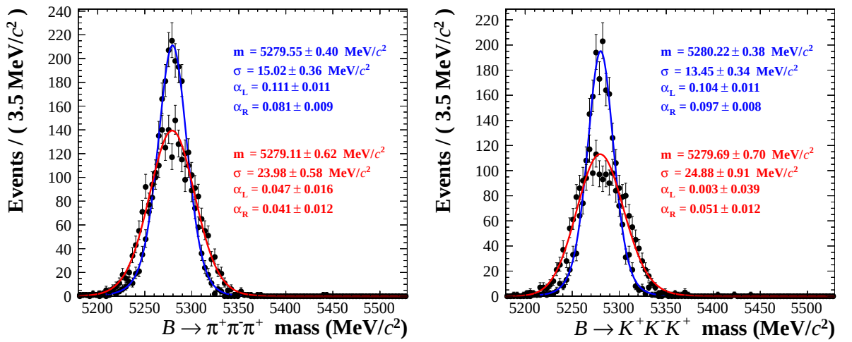
Figure 4.24.: B mass distributions for charmless MC simulated events ( m_D \in [-25, +25] MeV/c 2 applied). Blue: before D mass constraint, Red: after D mass constraint.
