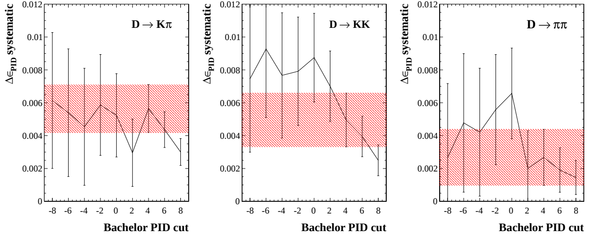
Figure 5.7.: \Delta\epsilon^{\text{PID}} systematic differences between the true \epsilon_{\text{sig}}^{\text{PID}} and the calibrated \epsilon_{\text{cal}}^{\text{PID}} for a wide range of \Delta LL_{K/\pi}^{\text{bach}} cuts. Left: corrections for B \rightarrow [K\pi]_D\pi events. Center: corrections for B \rightarrow [KK]_D\pi events. Right: corrections for B \rightarrow [\pi\pi]_D\pi events. Error bars are propagated from the statistical uncertainties on \epsilon_{\text{sig}}^{\text{PID}} and \epsilon_{\text{cal}}^{\text{PID}} , and depend on the size of the MC samples used. The shaded area highlights the obtained value for the chosen \Delta LL_{K/\pi}^{\text{bach}} > 4 cut. \Delta\epsilon^{\text{PID}} fluctuates in the 0.2 – 0.7% range.
