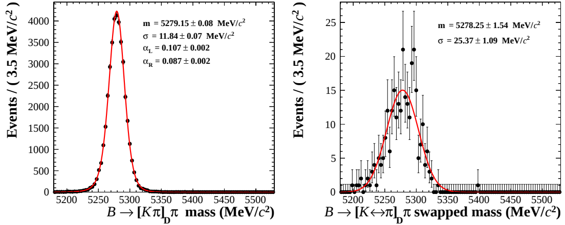
Figure 4.35.: Left: genuine signal B \rightarrow [K\pi]_D \pi events reconstructed with the correct D daughter mass hypotheses. Right: B \rightarrow [K\pi]_D \pi events reconstructed under the B \rightarrow [\pi K]_D \pi suppressed hypothesis in order to simulate the K \leftrightarrow \pi double swap. All selections and vetoes are applied on the samples: the width of the double-swapped peak is found to be about 2 times larger than the signal one.
