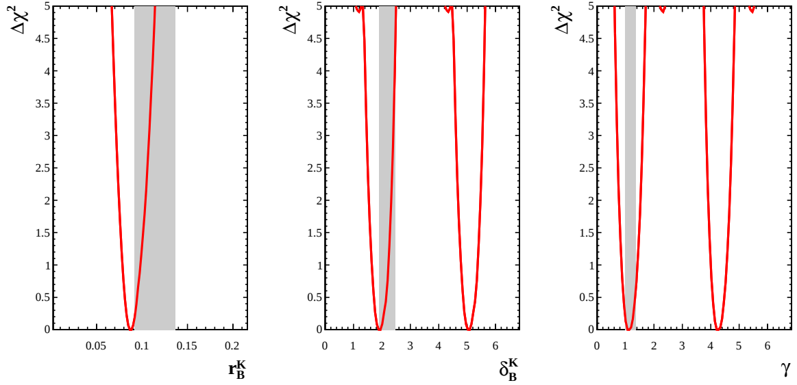
Figure 6.11.: 1D projections of the (r_B^K, \delta_B^K, \gamma) scan including the GGSZ analysis and the systematical uncertainties on r_D and \delta_D . Each curve is obtained minimising the \Delta\chi^2 function with respect to the other variables. The shaded areas indicate the current best estimated values [28].
