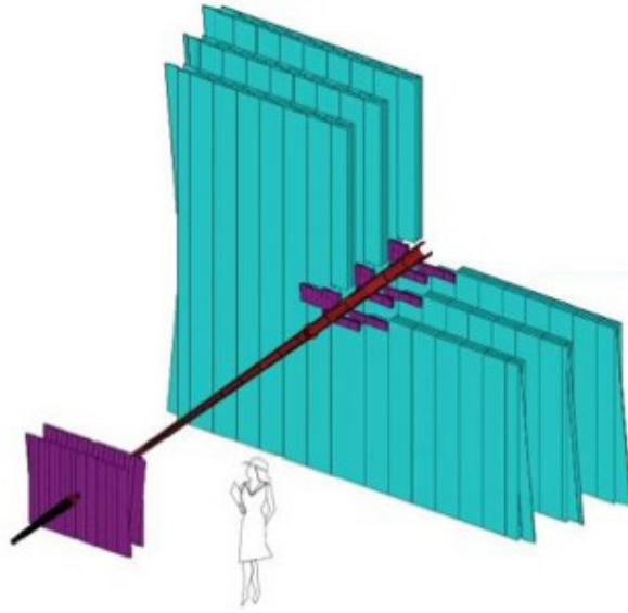
Figure 2.12.: Layout of the LHCb tracking system. The silicon microstrips of the TT and the IT are coloured in purple, the OT planes are shown in blue.
