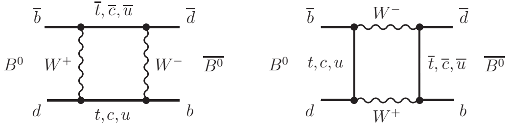
Figure 1.1.: Box diagrams for B^0\text{--}\bar{B}^0 mixing as an example of neutral meson mixing.
