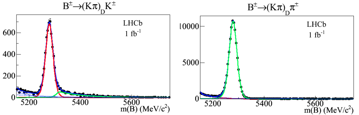
Figure 5.3.: A simultaneous fit to the favoured [K\pi]_D sample with a \Delta LL_{K/\pi}^{bach} cut at 8. The B \rightarrow D\pi width is (14.7 \pm 0.8) \text{ MeV}/c^2 and the B \rightarrow DK peak is narrower by a factor of (0.953 \pm 0.020) . A similar fit with a \Delta LL_{K/\pi}^{bach} cut at 6 gives (0.946 \pm 0.018) for the ratio.
