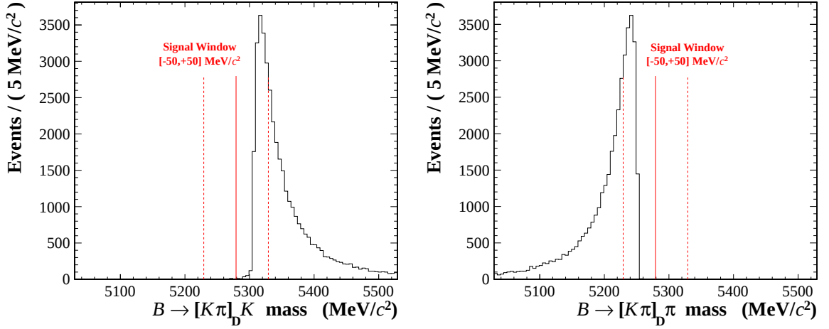
Figure 3.19.: Left: B \rightarrow [K\pi]_D \pi MC simulated events reconstructed with the B \rightarrow [K\pi]_D K mass hypothesis ( \pi misidentified as a K ). Right: B \rightarrow [K\pi]_D K MC simulated events reconstructed with the B \rightarrow [K\pi]_D \pi mass hypothesis ( K misidentified as a \pi ). The mass distributions are obtained using the combination of true 4-momenta only.
