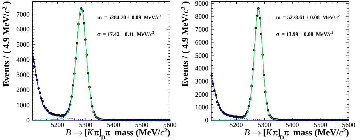
Figure 3.18.: DATA: B invariant mass distributions of the B \rightarrow [K\pi]_D \pi control sample. Left: B mass distribution before any mass constraint. Right: B mass distribution after refitting the candidates with D mass and vertex constraints.
