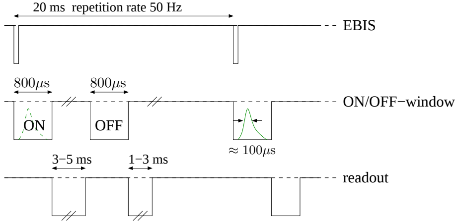
Figure 3.12: Electronics setup for T-REX, for details see text.
