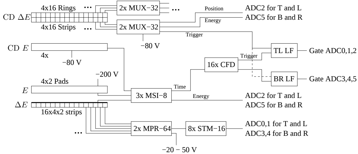
Figure 3.12: Electronics setup for T-REX, for details see text.
