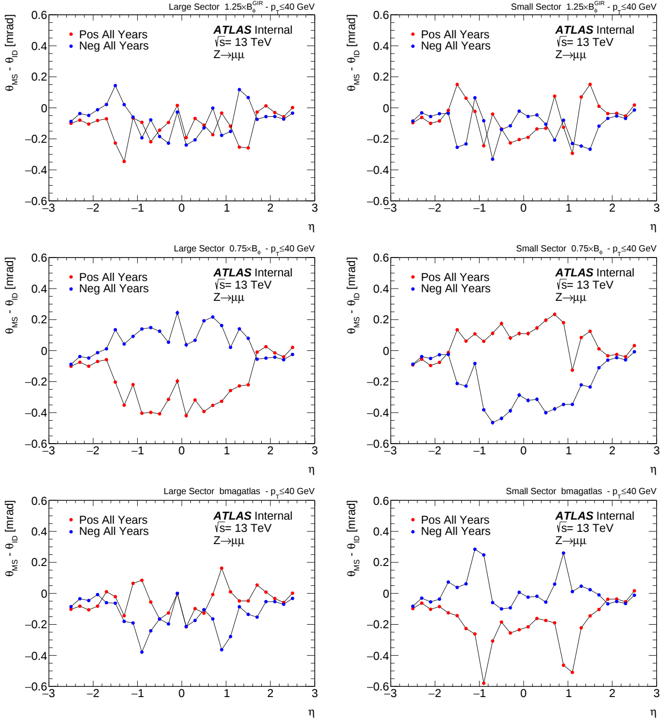
Figure 5.35: MS/ID residual \Delta\theta profiles for (top) 1.25 \times B_{\phi} , (middle) 0.75 \times B_{\phi} and (bottom) bmagatlas magnetic field maps in Z \rightarrow \mu\mu for (left) large and (right) small sectors at p_T < 40 GeV.
