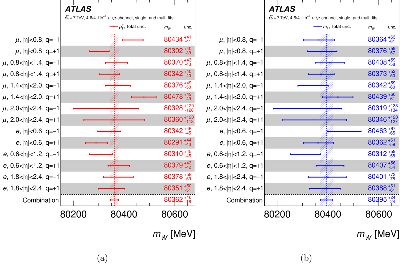
Figure 6.6: Overview of the m_W PLH fit results in all categories for the (a) p_T^\ell and the (b) m_T distributions, with the CT18 PDF set. The points labelled as "Combination" correspond to the result of a joint PLH fit to all categories.
