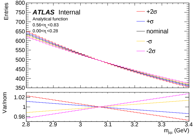
Figure 5.61: Exponential background templates. Upper panel: \pm\sigma, \pm2\sigma variations generated using analytical functions of fits with respect to the data. Bottom panel: Ratio of variations (Var) with respect to the nominal background function (nom).
