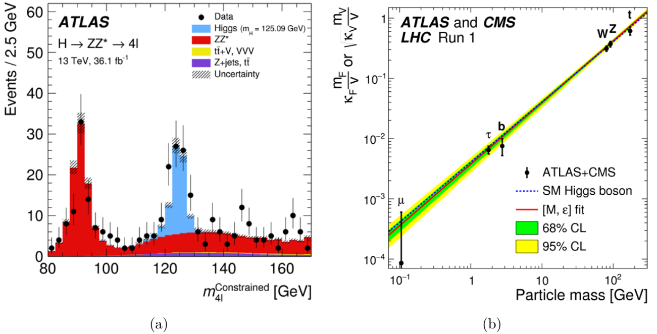
Figure 1.3: (a) Distribution of candidate Higgs events in H \rightarrow ZZ^* \rightarrow 4l at 13 TeV. The excess of events around 125 GeV is consistent with SM predictions for the Higgs boson [14] (b) Measurements of the coupling of the Higgs-boson to fermions and vector bosons as a function of the particle mass compared to the SM expectation [15].
