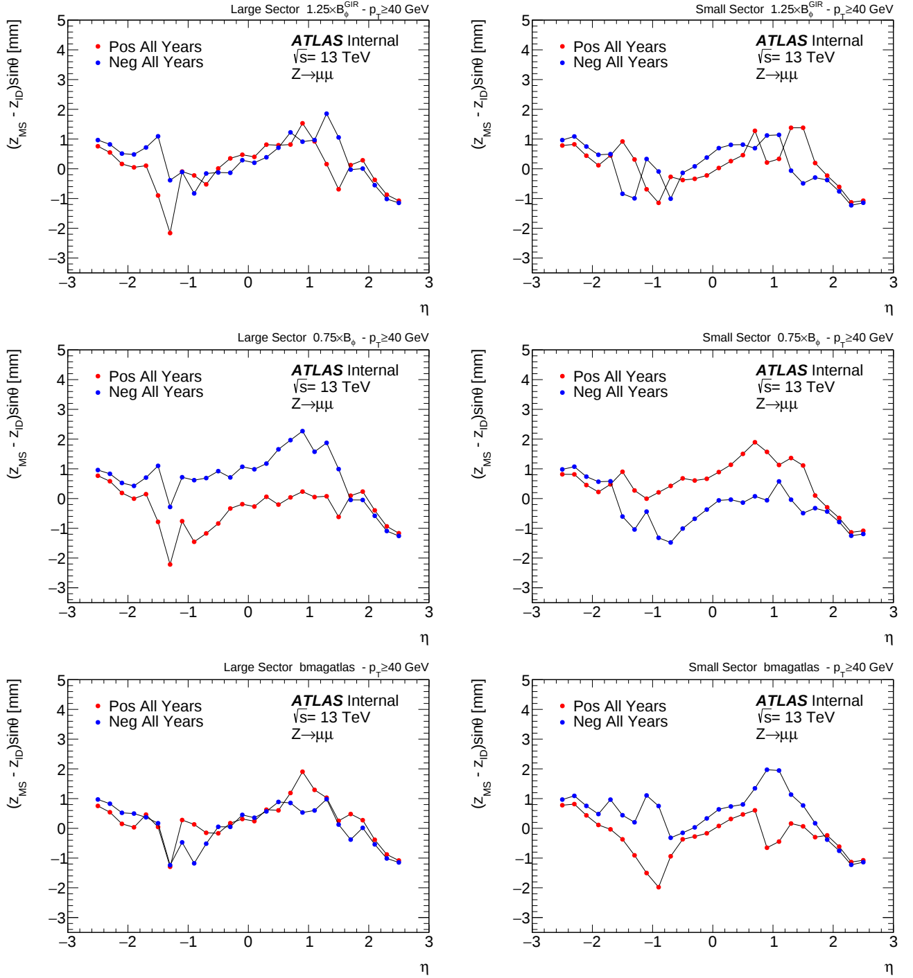
Figure 5.36: MS/ID residual \Delta z_0 \sin \theta profiles for (top) 1.25 \times B_\phi , (middle) 0.75 \times B_\phi and (bottom) bmagatlas magnetic field maps in Z \rightarrow \mu\mu for (left) large and (right) small sectors at p_T > 40 GeV.
