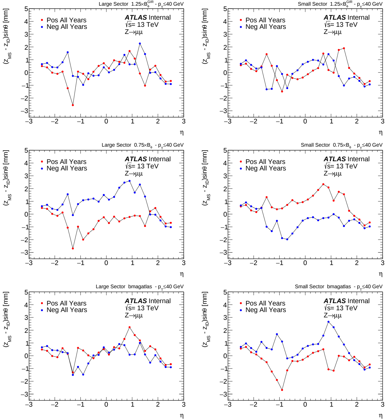
Figure 5.37: MS/ID residual \Delta z_0 \sin \theta profiles for (top) 1.25 \times B_\phi , (middle) 0.75 \times B_\phi and (bottom) bmagatlas magnetic field maps in Z \rightarrow \mu\mu for (left) large and (right) small sectors at p_T < 40 GeV.
