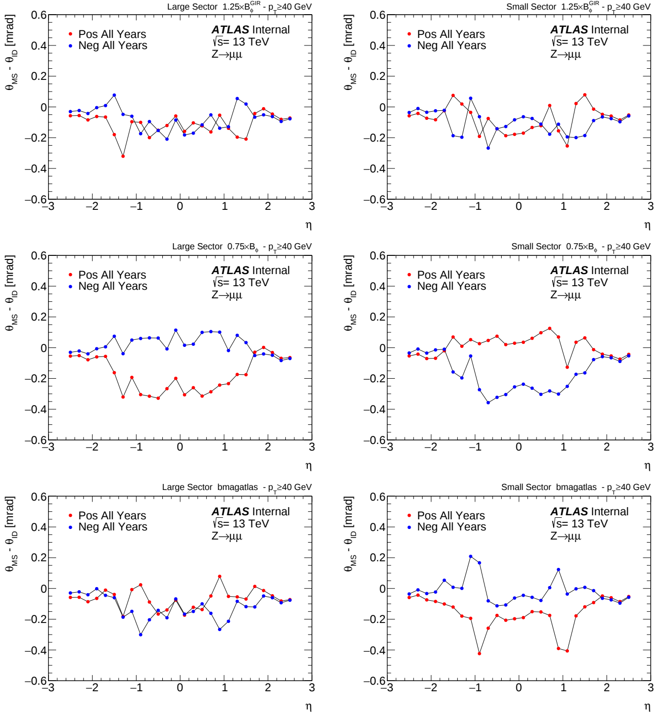
Figure 5.34: MS/ID residual \Delta\theta profiles for (top) 1.25 \times B_\phi , (middle) 0.75 \times B_\phi and (bottom) b_{\text{magatlas}} magnetic field maps in Z \rightarrow \mu\mu for (left) large and (right) small sectors at p_T > 40 GeV.
