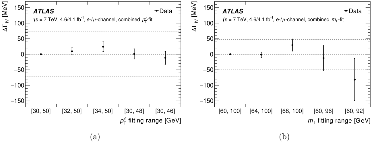
Figure 6.13: Dependence of the variation \Delta\Gamma_W of the fitted W -boson width on the (a) p_T^\ell and (b) m_T distributions. The nominal ranges are 30 < p_T^\ell < 50 GeV and 60 < m_T < 100 GeV, respectively. The outer dashed lines indicate the total measurement uncertainty for the nominal range. Results are shown for the combined fit over all categories, and for the CT18 PDF set.
