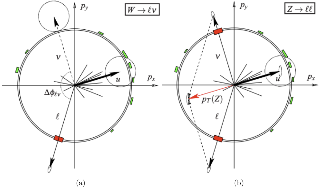
Figure 3.5: Scheme of the (a) W and (b) Z bosons decay in the transverse plane [124].
