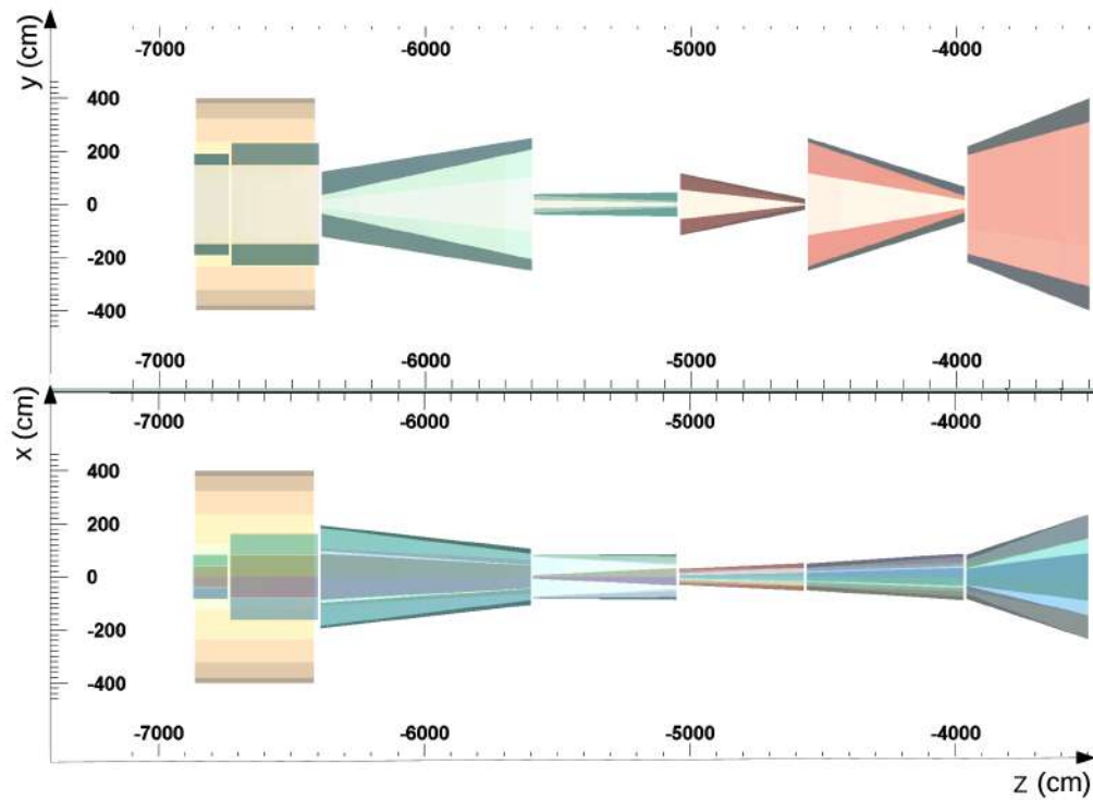
FIGURE 4.21: Geometric view of the optimized muon-shield, showing at the top, the z - y plane view, and at the bottom, the z - x plane view. SHiP software defines the origin of the coordinate system to be in the center of the decay vessel. Color shading is used to enhance the contrast between different magnetic field orientations.
