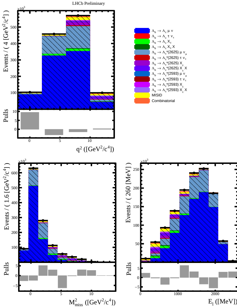
FIGURE 3.34: Multidimensional fit to isolated region.
