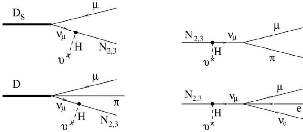
FIGURE 1.7: Feynman diagrams for the HNL production and decay [29].
