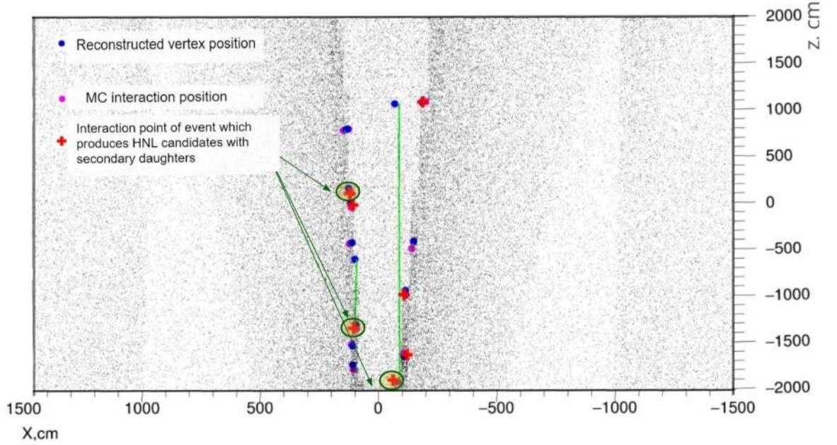
FIGURE 4.25: Position of reconstructed vertices and actual interaction point for events which survive basic selection.
