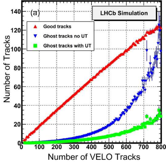
FIGURE 2.5: Simulation of the number of real reconstructed downstream tracks and ghost tracks as a function of the number of VELO tracks at a luminosity of 2 \cdot 10^{33} \text{cm}^{-2} \text{s}^{-1} . The generated sample consists of events containing inclusive b -hadron decays at 14 TeV centre-of-mass energy. The ghosts are in two categories, one not requiring, and the other requiring a UT track match [58].
