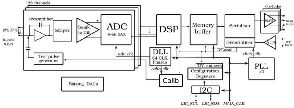
FIGURE 2.8: Block diagram of SALT128 [63].
