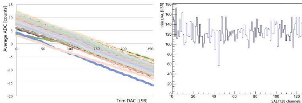
FIGURE 2.16: Example of a trim DAC scan (left) and a best trim configuration for each channel (right).
