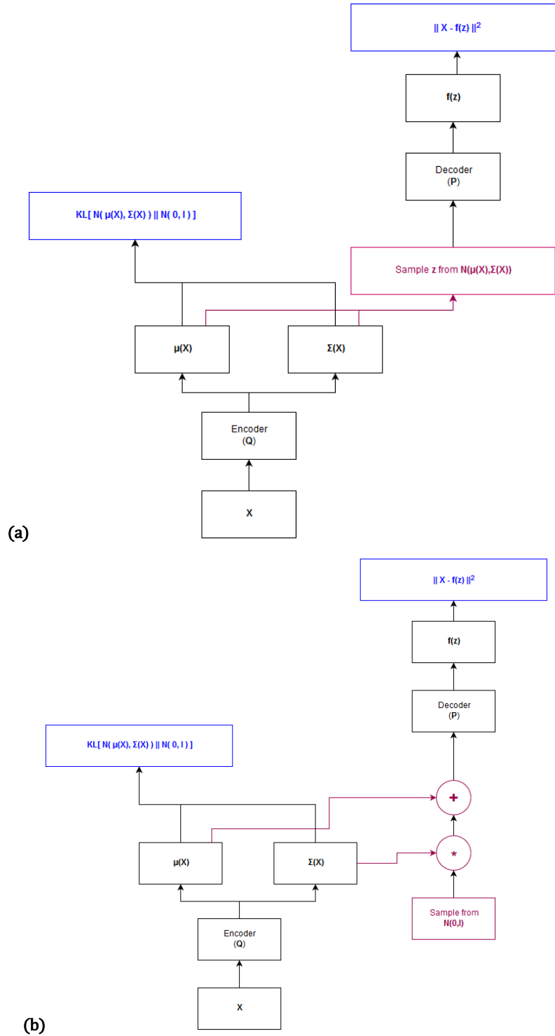
Figure 54: Training-time VAE (a) Theoretical implementation (b) Reparameterization trick, which is implemented in practice
