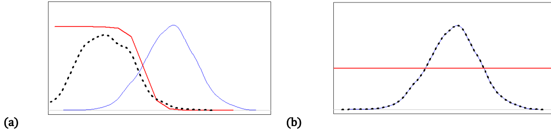
Figure 57: (a) GAN Densities during training (simplified diagram showing distributions of only a single dimension), close to convergence, P(x) is shown in black, G(z) in blue and D(G(z)) in red, (b) those same GAN densities, once the Algorithm has converged: G(z) matches P(x) perfectly and D(G(z)) outputs 0.5 everywhere
