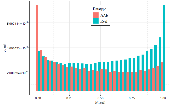
Figure 76: Distribution of P(\text{real}) estimates for AAE and real data
