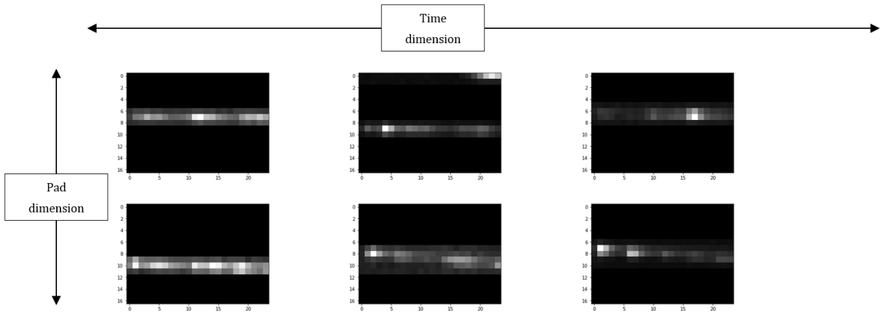
Figure 30: Six example TRD tracklets, with time-direction indicated along the x-axis and pad-direction indicated along the y-axis for each image shown
