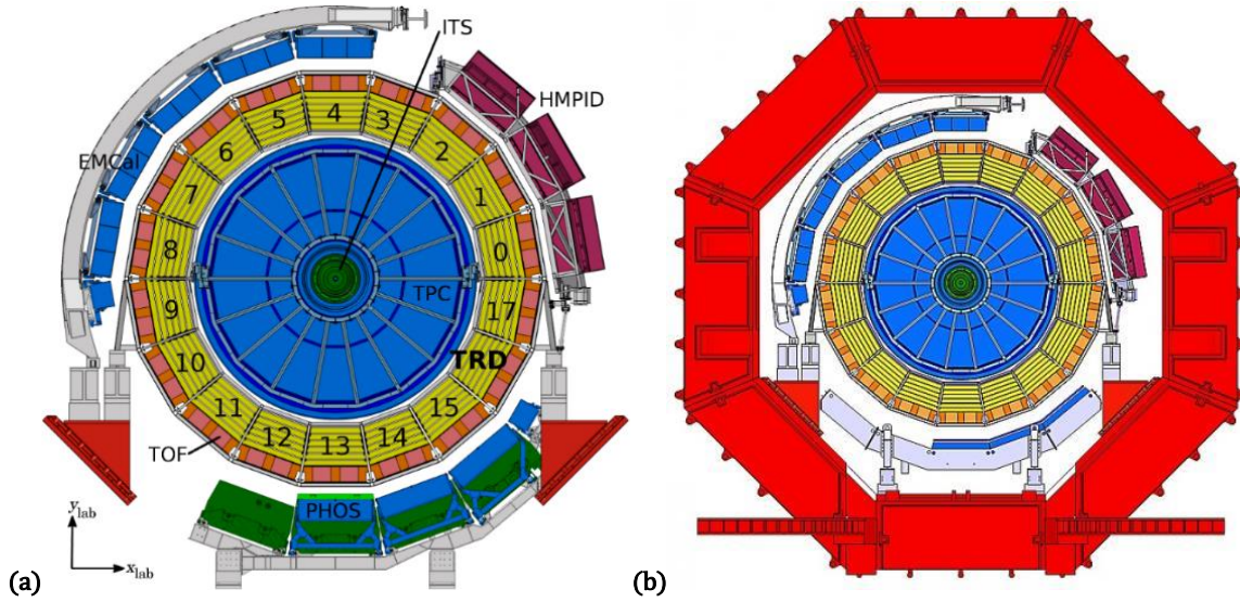
Figure 5: (a) A schematic cross-section of the ALICE detector, with the TRD shown in yellow and its 18 sectors in azimuthal angle numbered, as well as the location of other ALICE detector components: ITS, TPC, HMPID, EmCal, TOF and PHOS [38], (b) cross-section of the ALICE detector shown in context of the surrounding magnet structure [39].
