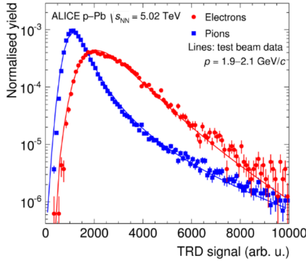
Figure 15: Total integrated charge, normalised to tracklet length, measured in a single read-out chamber for electrons and pions in pPb collisions at \sqrt{s_{NN}} \approx 5.02 \text{ TeV} . Test beam measurements were scaled by a common factor to compensate for gain differences [38].
