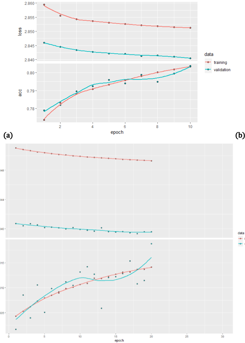
Figure 50 Training and loss curves for the most successful model, making use of Focal loss as the objective function to be minimised, trained for particles in the 2 GeV range (a) for 10 epochs, (b) for an additional 20 epochs
