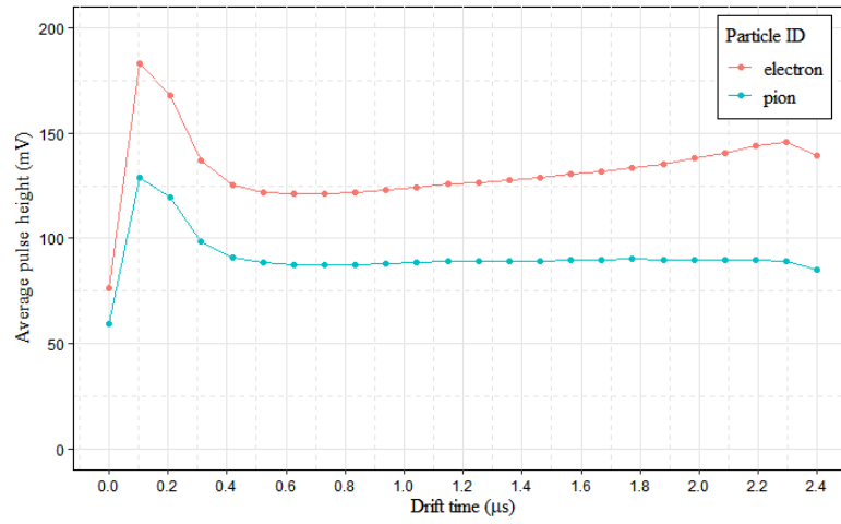
Figure 34: Time Evolution of the Average Pulse Height Signal, per Particle ID (for tracklets from the entire momentum range)
