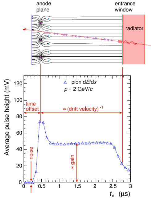
Figure 10: Main TRD signal calibration parameters, indicated as annotations on a plot of the average pulse height as a function of drift time for pions, in addition, the chamber cross-section is shown at the top for better understanding [38]
