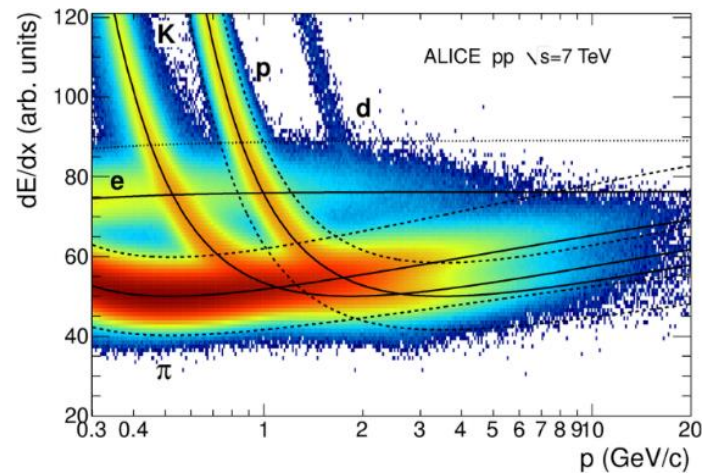
Figure 7: Bethe-Bloch curve for various subatomic particles as measured by the ALICE TPC at \sqrt{s} = 7 TeV [44]
