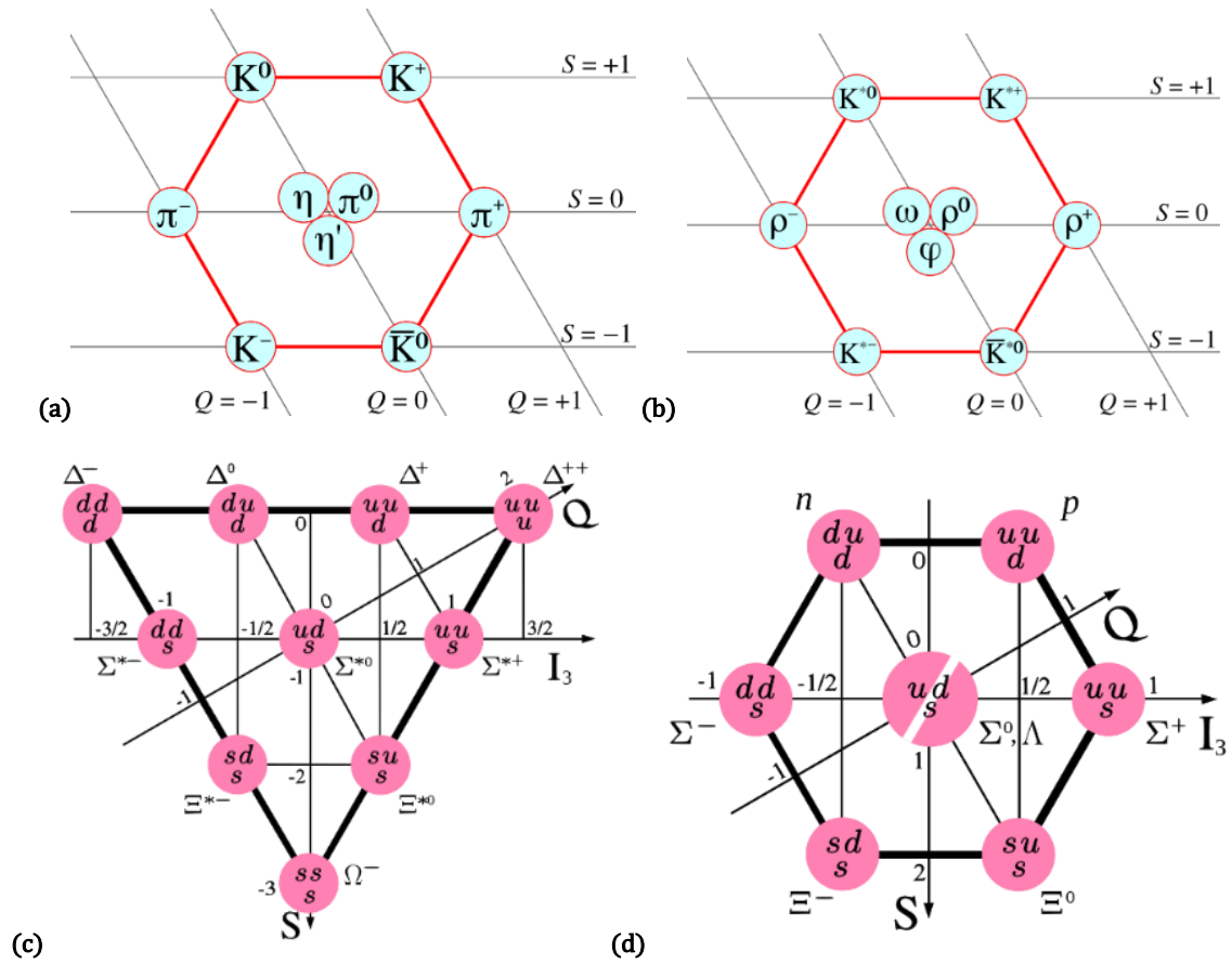
Figure 1: Mesons: (a) spin-1 nonet [10], (b) spin-0 nonet [11]; and Baryons: (c) spin-3/2 uds decuplet [12], (d) spin-1/2 uds octet [13]
