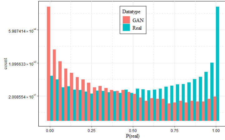
Figure 70: Distribution of P(\text{real}) estimates for GAN and real data
