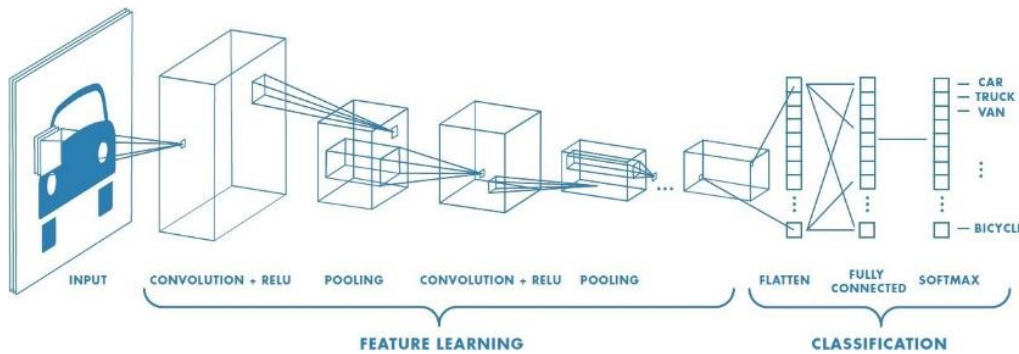
Figure 25: Simplified diagram of a convolutional neural network [69]
