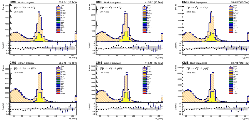
Figure B.1: Reconstructed invariant mass for the Z \rightarrow l^+l^-\gamma events in the electron (top) and muon (bottom) channels for data collected in 2016 (left), 2017 (centre) and 2018 (right).
