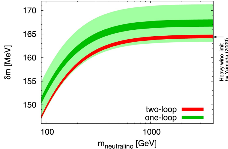
Figure 2.5: Charged and neutral wino mass splitting calculation of one-loop (green) and two-loop (red) as a function of neutralino mass [17].
