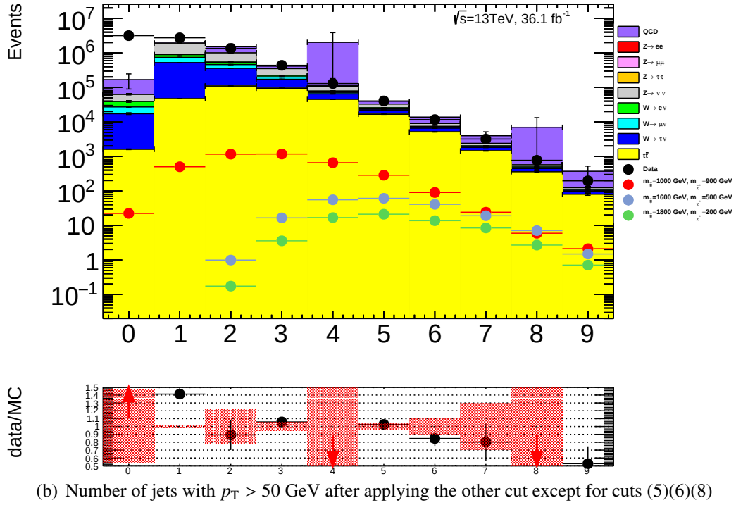
Figure 7.3: The kinematic variable distributions for the various MC background processes in the stacked histogram, the data in the black points and simulated events for the benchmark signals in coloured points. As benchmark signals, (m_{\tilde{g}}, m_{\tilde{\chi}_1^\pm}) = (1000 \text{ GeV}, 900 \text{ GeV}) in red, (1600 \text{ GeV}, 500 \text{ GeV}) in blue, and (1800 \text{ GeV}, 200 \text{ GeV}) in green are shown. The lower plot shows the ratio of data and MC in black points and MC statistical uncertainty is shown by red shade. Red arrows mean that the ratio is out of range.
