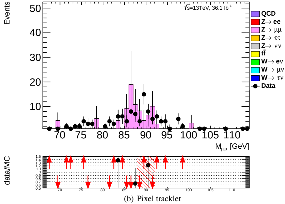
Figure 8.8: The M_{\mu\mu} distributions of each category after background correction. Various MC standard model processes are shown in the stacked histogram and data in the black points. The lower plot shows the ratio of data and MC in the black points and MC statistic uncertainty is shown by the red shade.
