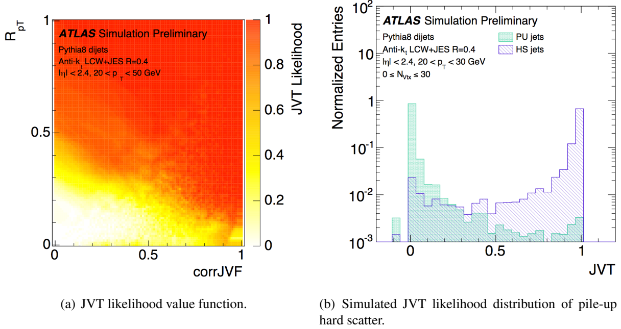
Figure 5.2: (a) The 2-dimensional JVT likelihood function and (b) simulated JVT likelihood distribution of pile-up and hard scatter [73]. Green histogram is for pileup jets and purple histogram is for hard scatter jets.
