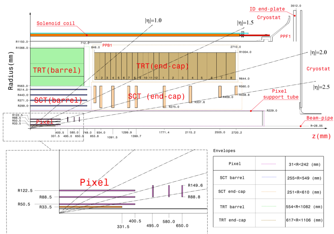
Figure 3.6: Cross-sectional view of the ATLAS inner detector. [37]
