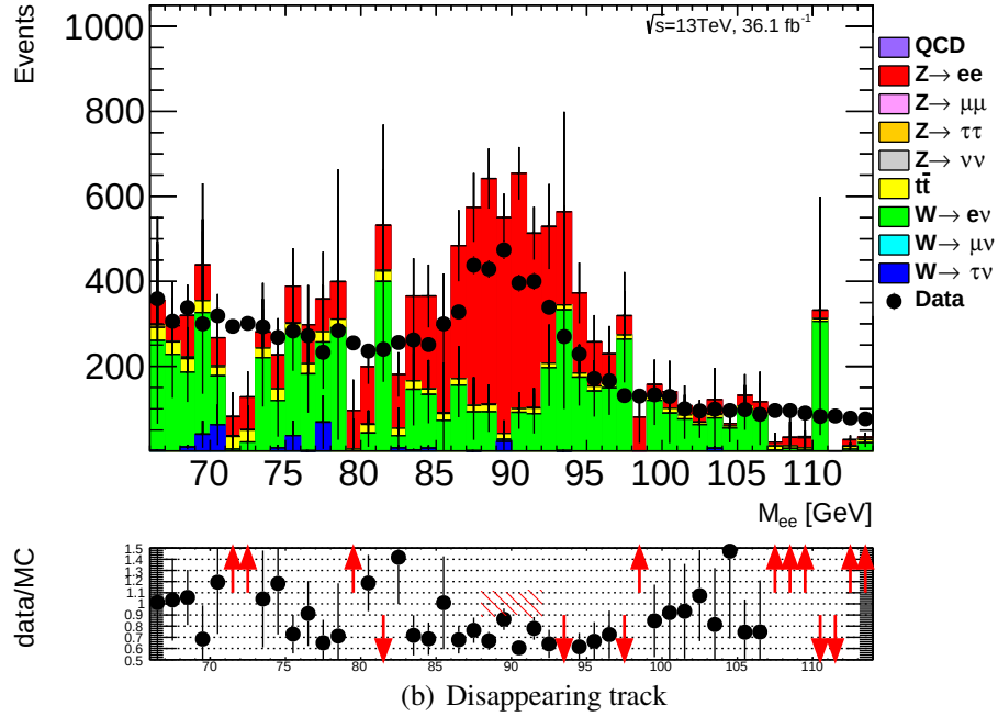
Figure 8.5: The M_{ee} distributions of each category. Various MC standard model processes are shown in the stacked histogram and data in the black points. Lower plot shows the ratio of data and MC in the black points and MC statistic uncertainty is shown by the red shade.
