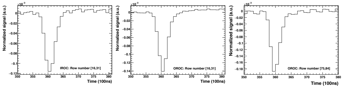
Figure 3.17.: Normalised common-mode response functions for three different pad-size regions: IROC (left), inner OROC (middle) and outer OROC (right).
