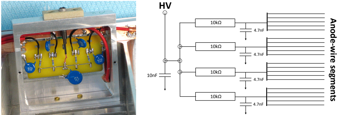
Figure 3.19.: Picture (Left) and diagram (Right) of an electric circuit of an IROC [61, 70].
