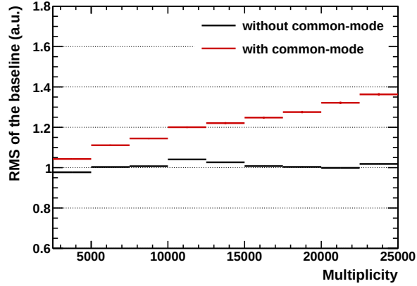
Figure 3.28.: Additional noise resulting from the common-mode effect as a function of multiplicity (total number of primary and secondary tracks).
