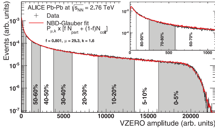
Figure 5.3.: (Black markers) Distribution of the summed amplitudes in the V0 detectors. (Red curve) the result of the Glauber model fit to the measurement. The vertical lines separate the centrality classes, which in total correspond to the most central 80% of the hadronic collisions [79].
