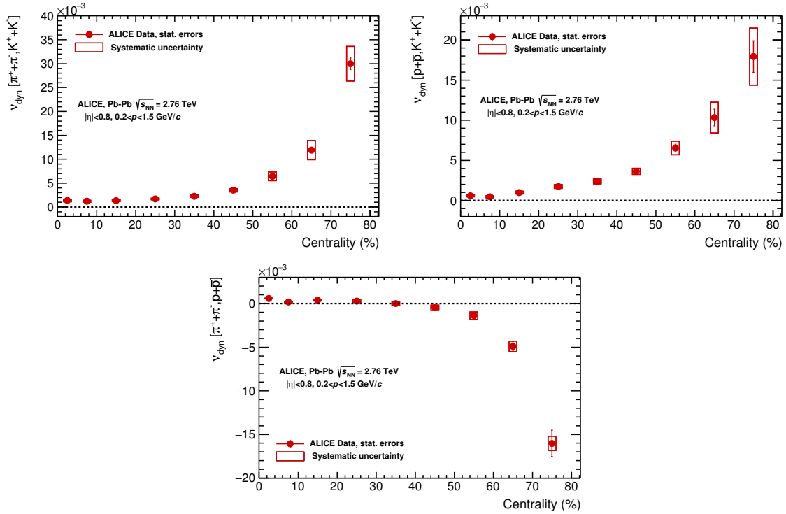
Figure 6.1.: Centrality dependence of the ALICE \nu_{\text{dyn}} results and the statistical and systematic uncertainties.
